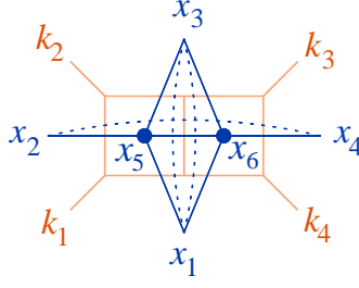
FIGURE 6. The two-loop planar double box integral (in orange) and associated dual graph (in blue).
