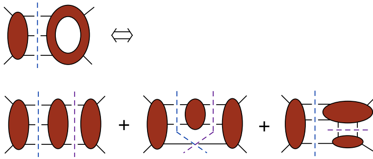
FIGURE 4. Example of generalized unitarity at three loops.
