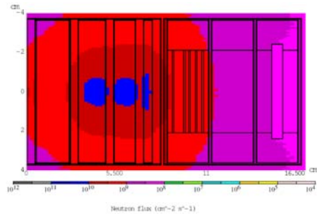
Figure 4: Neutron flux calculated by the MARS15 code
