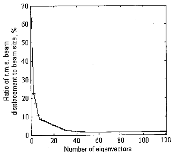
Figure 4: Calculated beam motion for the NSLS-II storage ring.
