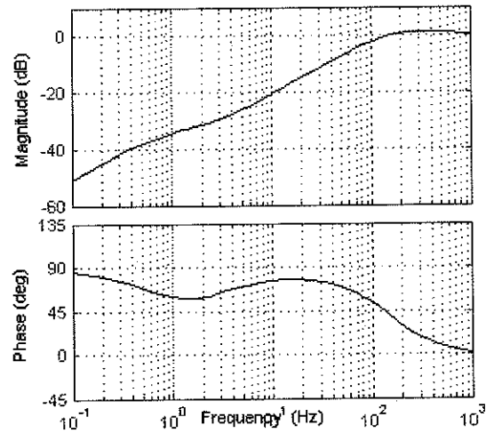
Figure 4: Calculated noise suppression by the integrated feedback. Noise is suppressed with frequencies up to 140 Hz.
