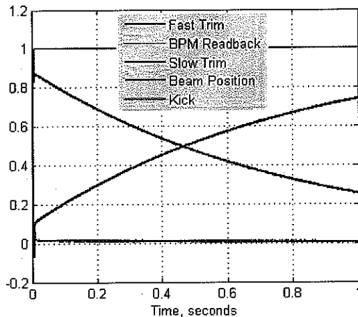
Figure 6: Response of the integrated orbit feedback system to the step with longer time scale. The strength of the fast trim is gradually decreasing while slow trim picks up the correction.
