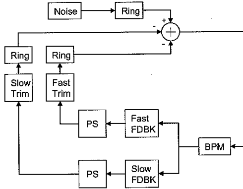
Figure 1: Simplified layout of combined fast and slow orbit feedbacks.
