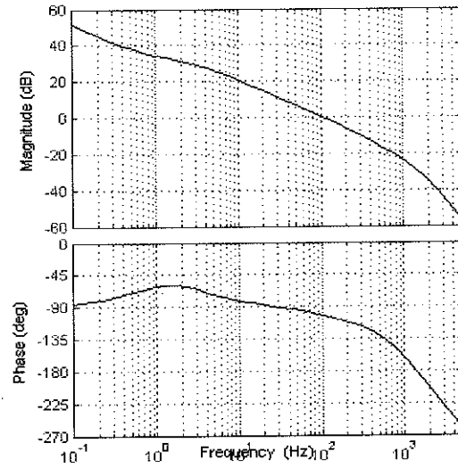
Figure 3: Bode diagram of integrated orbit feedback.
