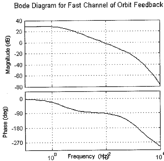
Figure 2: Bode diagram of fast channel of orbit feedback system.
