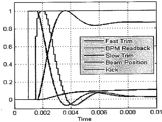
Figure 5: Response of the integrated orbit feedback system to the step.
