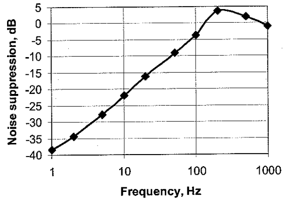
Figure 7: Suppression of noise by the integrated orbit feedback with delay and discrete time processing.
