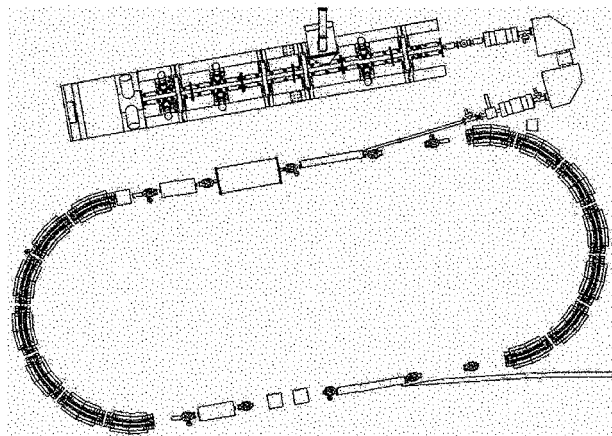
Figure 3: RCMS Rapid Cycling Medical Synchrotron.
