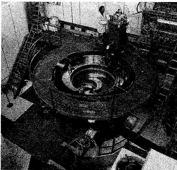
Figure 1: COMET superconducting isochronous cyclotron (partially disassembled).
