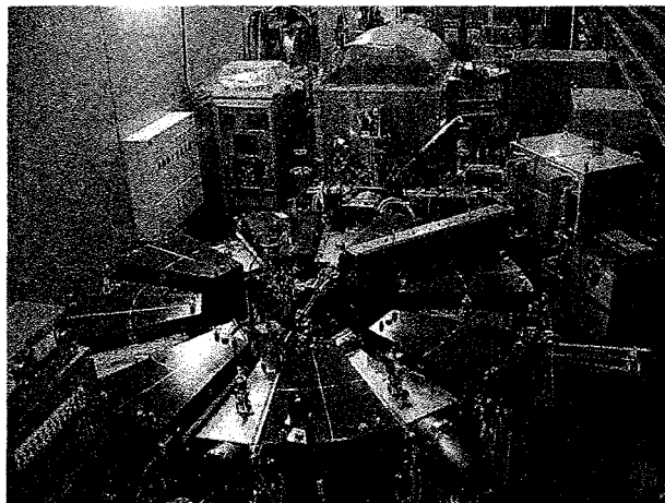
Figure 4: The KEK proof-of-principle FFAG accelerator.
