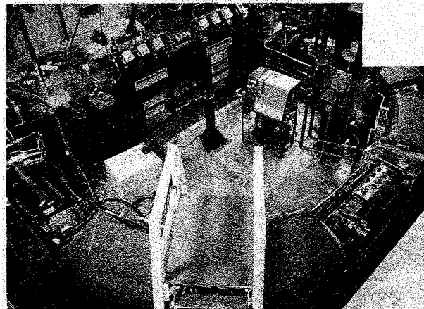
Figure 2: LLUMC weak focusing 250 MeV synchrotron.
