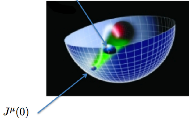
FIGURE 1. AdS representation of light-front QCD. Different values of z correspond to different scales at which the hadron is examined. The AdS boundary at z \rightarrow 0 (large circumference) corresponds to the Q \rightarrow \infty , UV, zero separation limit. Local operators are defined at the AdS boundary; hadronic transition matrix elements probe the wave function \Phi(z) (also represented in the figure) at z = 1/Q . The inner sphere at large z represents the IR confinement radius. In the figure, a small proton created by a local interpolating operator at the AdS boundary falls into AdS space pulled by the gravitational field up to its larger size allowed by confinement. Due to the warp factor the proton size shrinks by a factor z/R as observed in Minkowski space.
