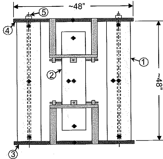
Figure 6: Layout of the test stand for user BPM post. The post under test 2 is hung between two stainless steel plates 3 and 4 mounted on two pillars 1. The pillars are made of the same carbon filament composite.
