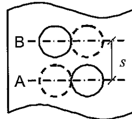
Figure 4: Location of BPM buttons with rotated geometry.
