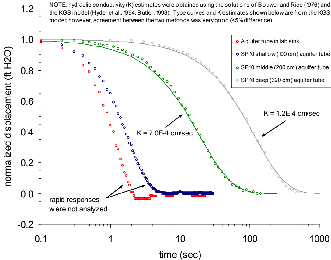
Figure 5. Slug Test Responses in Aquifer Tubes at Depths of 100 (shallow), 200 (middle), and 320 (deep) cm Below the River Bed at Spring 10 and Within a Water-Filled Laboratory Sink (control)
