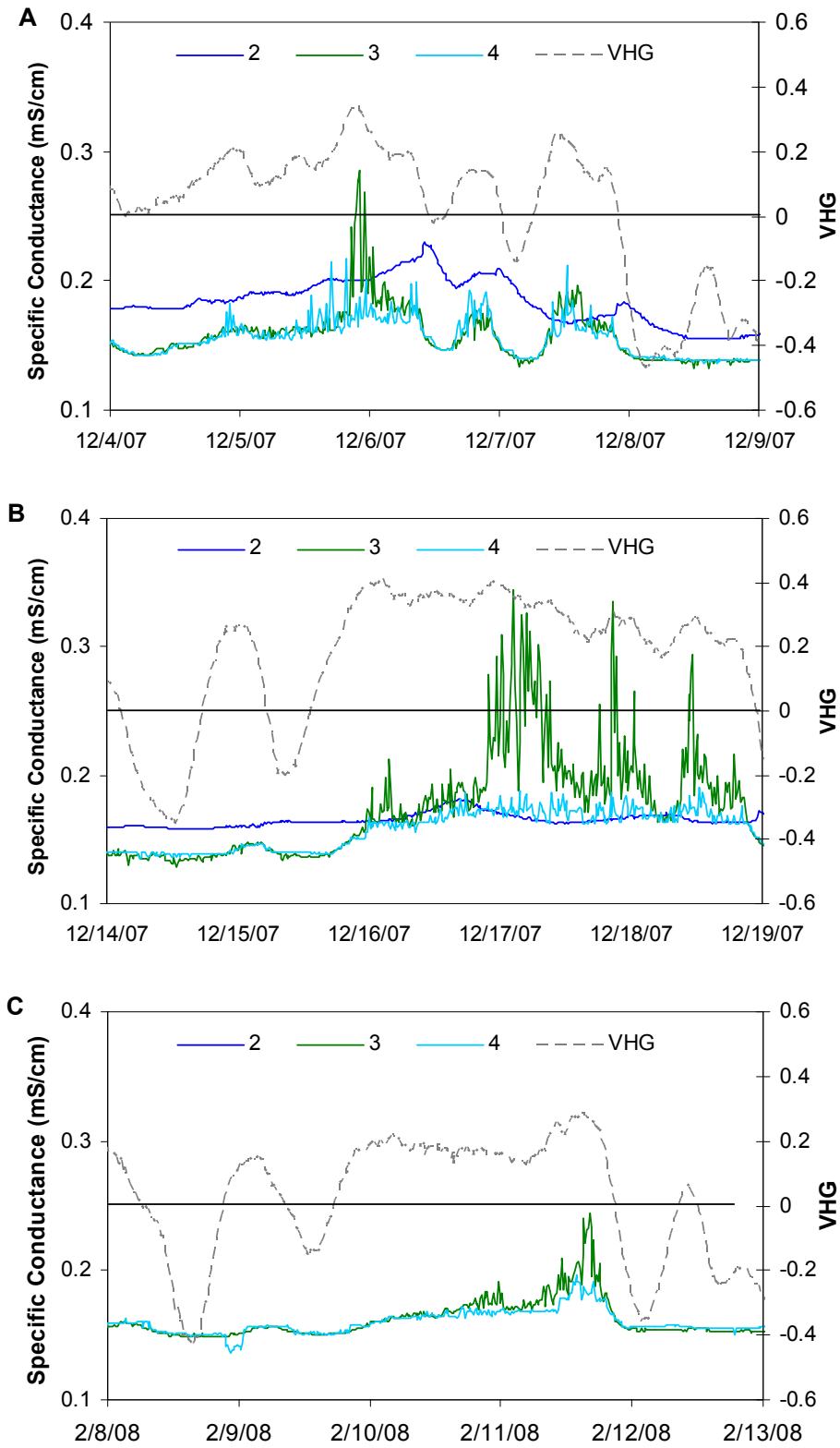
Figure 3. Specific Conductance and Vertical Hydraulic Gradients (VHG) Measured at Spring 10 Buried Probe Array, Locations 2, 3 & 4
