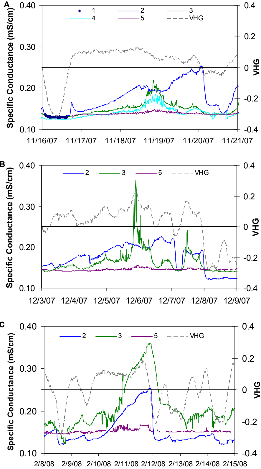
Figure 2. Specific Conductance and Vertical Hydraulic Gradients (VHG) Measured at Spring 9 Buried Probe Array, locations 1 through 5
