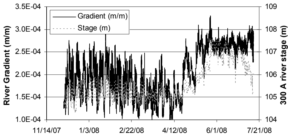
Figure 6. Columbia River Gradient and Stage Near the 300 Area
