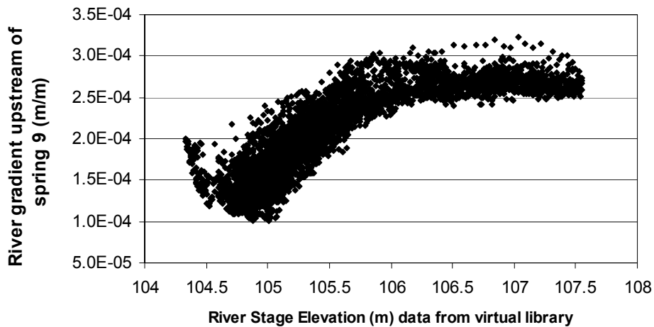
Figure 7. Columbia River Gradient as a Function of River Stage
