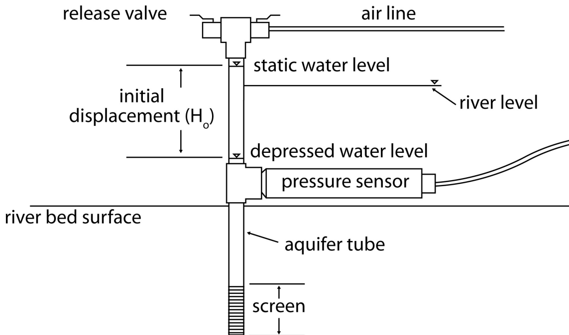
Figure 4. Equipment and Set-up used to conduct Aquifer Tube Slug Tests
