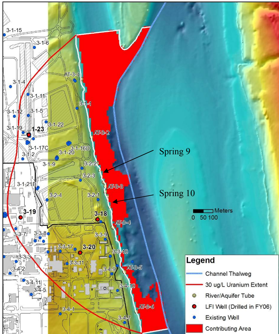
Figure 1. Map of Riverbed Area with the Potential to Discharge Uranium into the Columbia River. This area is between 105 m in elevation and the river thalweg, between the 30 \mu\text{g/L} uranium concentration contour lines onshore, and above the projected Ringold Formation. From PNNL-16805.
