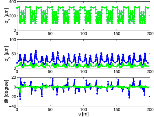
Figure 3: Horizontal/vertical beamsize and beam tilt as calculated from calibrated machine model using orbit response matrix analysis. The blue case is before coupling correction, the green one after one iteration.
