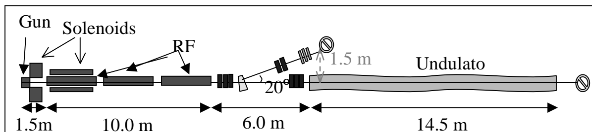
Figure 1: Schematic layout of SPARC phase 1
