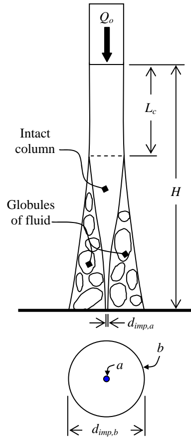
Figure 3.2. Plunging jet schematic.
