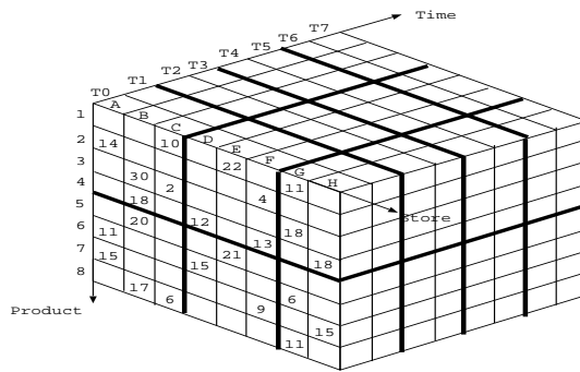
Figure 1: A 3-dimensional MOLAP representation R(\text{Product}, \text{Store}, \text{Time}, \text{Sales}) .
