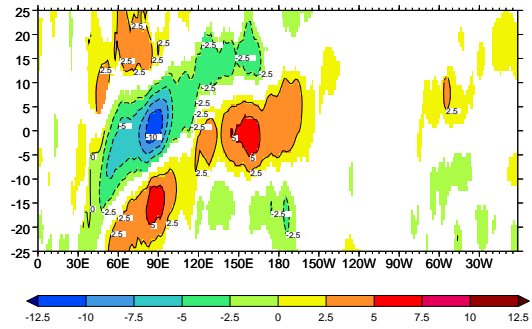
d) CGCM3.1 (T63)
