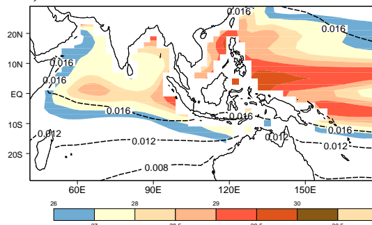
d) GFDL-CM2.0
