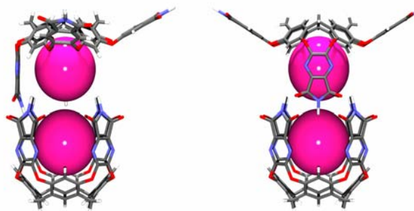
Fig. 10 Two proposed structures for the capsule which facilitate exchange with (a) two adjacent sides open and (b) two opposite sides open. 26
