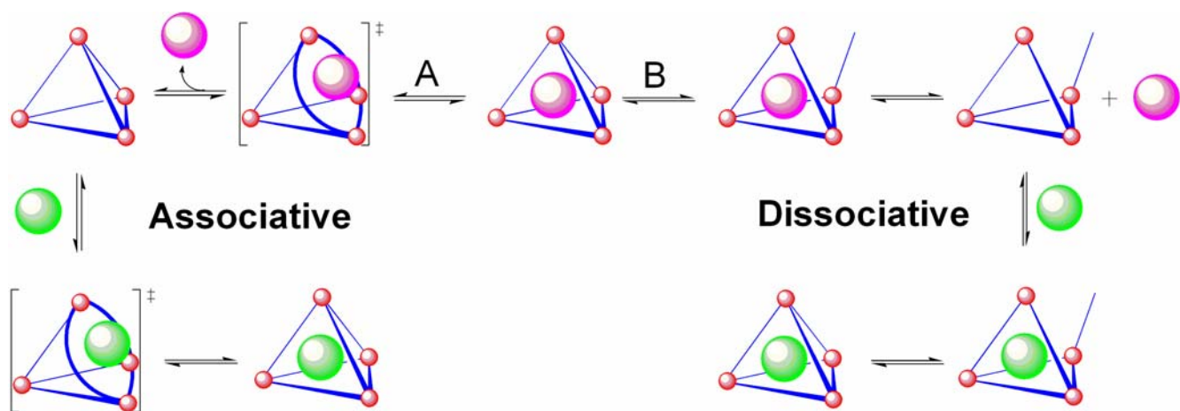
Fig. 13 Two possible guest exchange mechanisms. Expansion of the apertures along the 3-fold axis of the assembly could allow for guest exchange (left). Alternately, host rupture could also allow for guest exchange (right).
