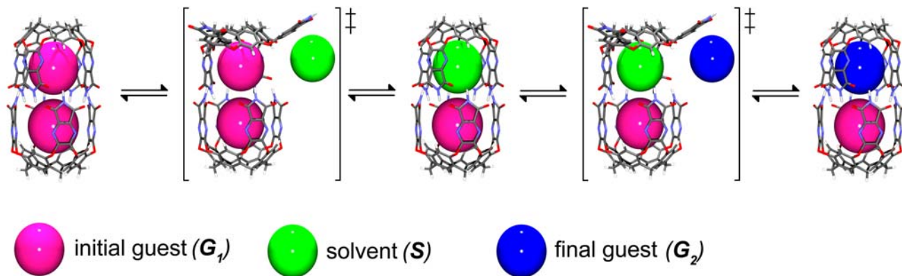
Fig. 11 Guest exchange pathway for 3 for smaller guests in which two guest molecules are encapsulated. Replacement of the initial guest ( G_1 ) by solvent ( S ) followed by subsequent exchange of the solvent for the final guest ( G_2 ) completes the exchange pathway. Note that the incoming guest must reside on the same half of the capsule as the initial guest.
