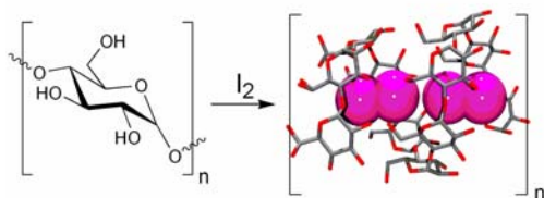
Fig. 1 In the presence of iodine, amylose, the main component of starch, forms helical polymers which encapsulate I_2 molecules. identical subunits creating an assembly with octahedral symmetry and an internal cavity of over 230 \text{ nm}^3 (Figure 2). 2 This iron-transport protein can hold up to 4500 iron atoms as ferric hydrous oxides. Such assemblies often rely on a variety of weak supramolecular interactions such as hydrogen-bonding, \pi - \pi interactions, and van der Waals interactions to hold the subunits together.
