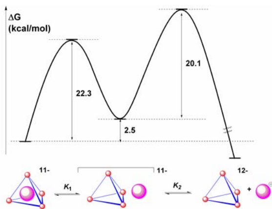
Fig. 14 Energy coordinate diagram for the dissociation of \text{Cp}^*(\text{PMe}_3)\text{Ir}(\text{Me})(\text{cis-2-butene})^+ from the \text{M}_4\text{L}_6^{12-} assembly. This initial dissociation ( K_1 ) produces an ion-pair intermediate which further dissociates ( K_2 ) to the free guest.
