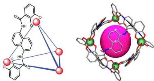
Fig. 12 Left- The edges of the tetrahedron are spanned by six bis-bidentate catechol amide ligands. Right- Crystal structure showing encapsulated \text{NEt}_4^+ .
