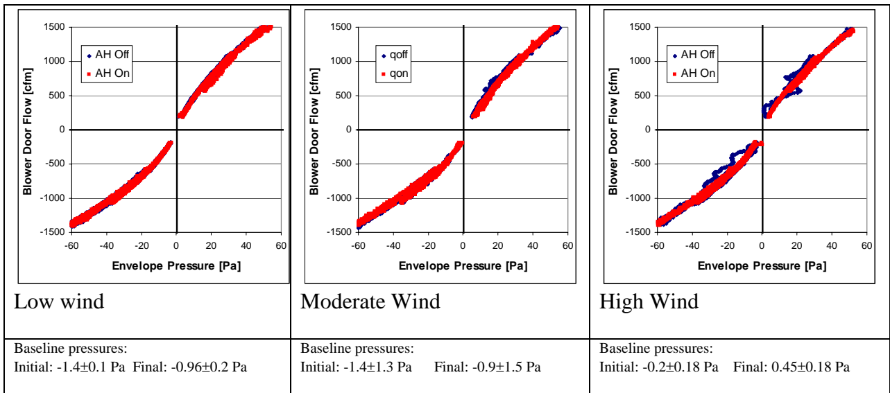
Figure 5a, 5b, and 5c: House pressure curves with the air handler off and on for Sparks 2 at low (less than 1 m/s), moderate (about 2 m/s) and high (>2.5 m/s) wind speeds averaged over the test period
