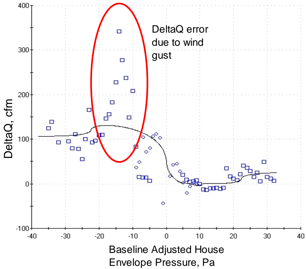
Figure 13. DeltaQ representation of data from Figure 10 showing large excursion in DeltaQ data due to a wind gust.
