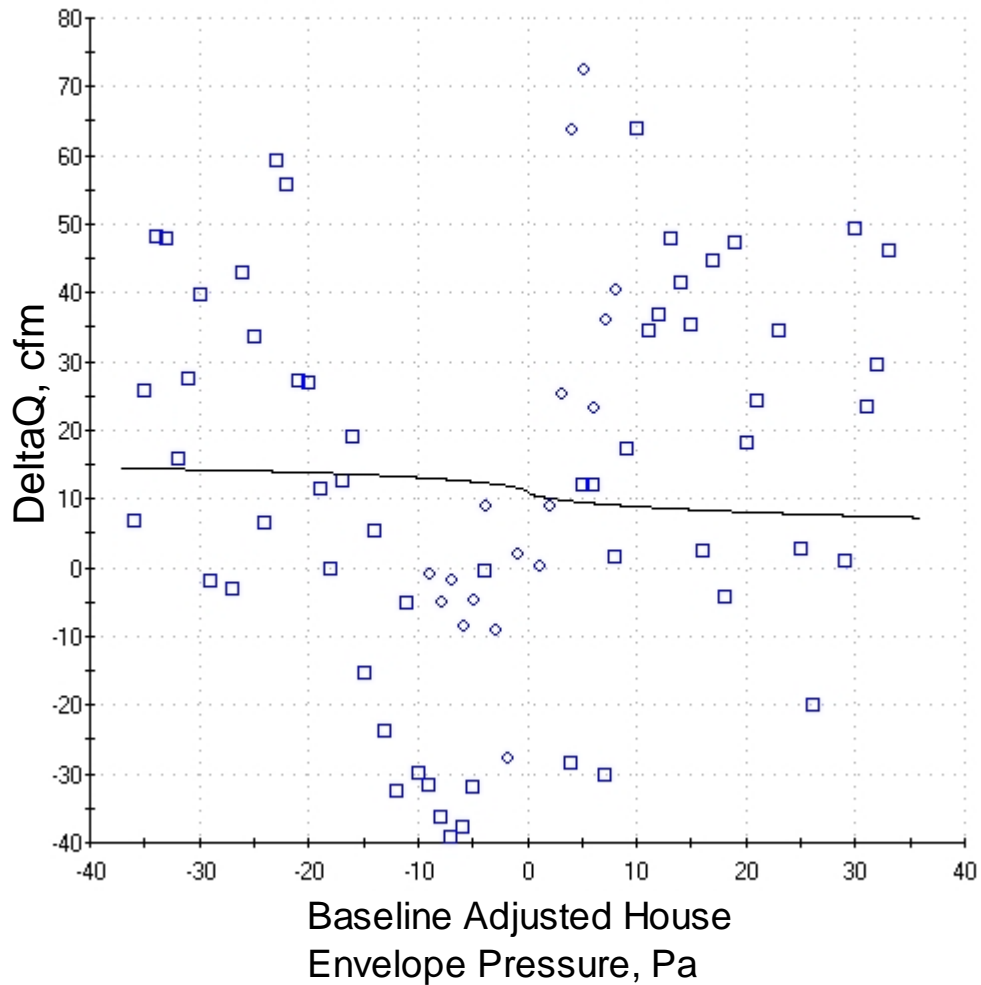
Figure 18. DeltaQ using data from Figure 17 showing random variability and no strong trends, outliers or groups of displaced data due to sustained wind gusts.
