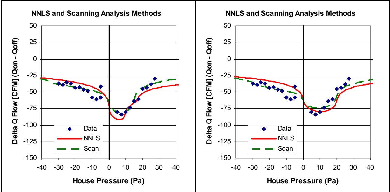
Figure 9c. No data < 5 Pa Characteristic Pressure Limit = 2 times lowest data NNLS: Q_s=0 , Q_r=69 cfm (33 L/s) Scanning: Q_s=0 , Q_r=67 cfm (32 L/s)
