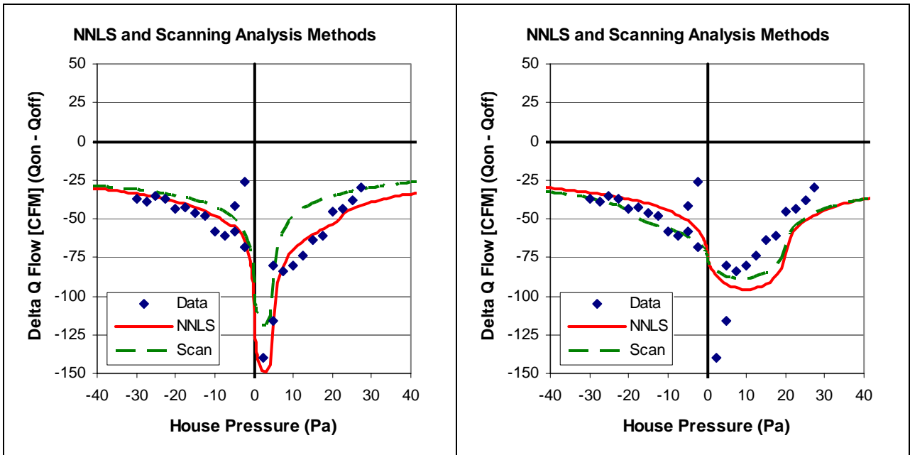
Figure 9a. All Data Characteristic Pressure Limit = 2 times lowest data NNLS: Q_s=12 cfm (6 L/s), Q_r=97 cfm (46 L/s) Scanning: Q_s=0 , Q_r=92 cfm (43 L/s)
