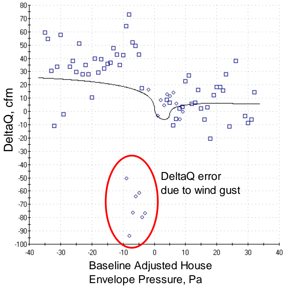
Figure 16. DeltaQ data from the test shown in Figure 14.
