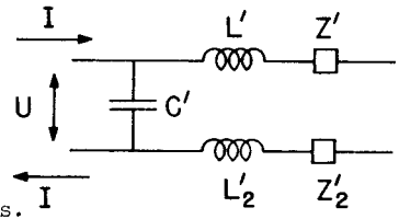
Fig. 1. Unit element of the conductor-chamber system. The inductance per unit length of the ideal transmission line, L' + L_2 , has--arbitrarily--been split into two parts.
