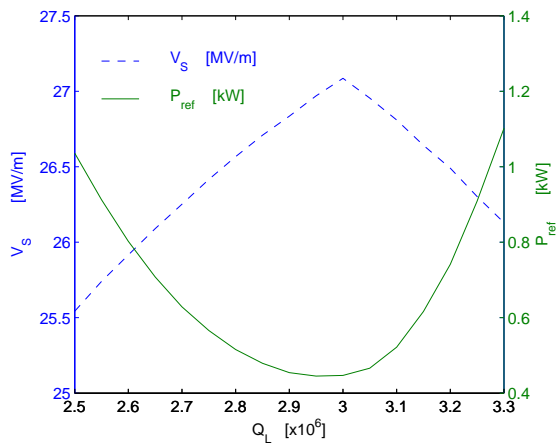
Figure 3: Variations of the vector sum gradient V_S and the total reflected power P_{ref} as a function of Q_L .
