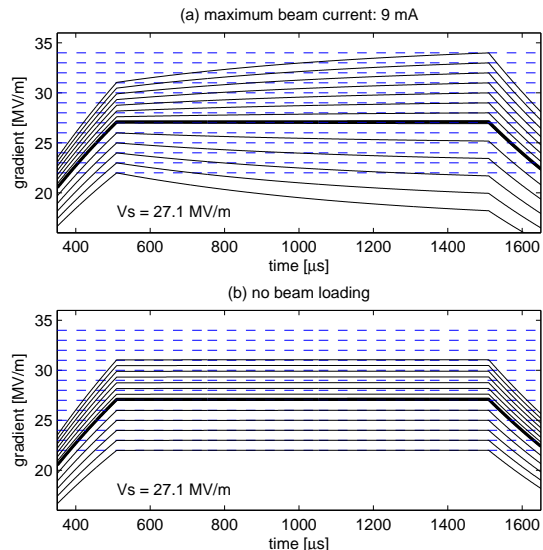
Figure 2: Amplitude plot for 13 cavities with (a) and without (b) beam.
