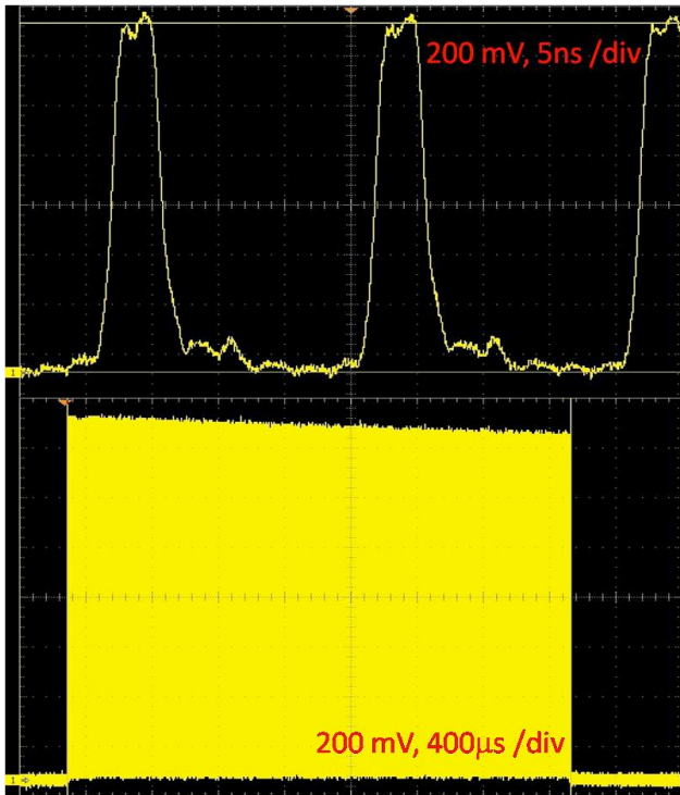
Figure 1: Kentech 1.2 kV pulser output, with 60dB attenuation. The top trace shows several 1.2 kV pulses with ~20 ns spacing. The bottom trace shows this pattern repeated for 3 ms.
