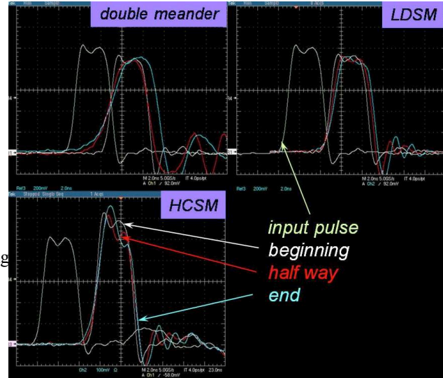
Figure 4: Pulse behavior along the meander structure.
