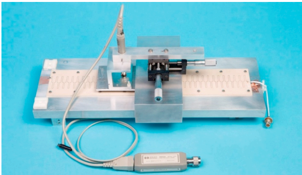
Figure 5: Coverage factor measurement fixture.
