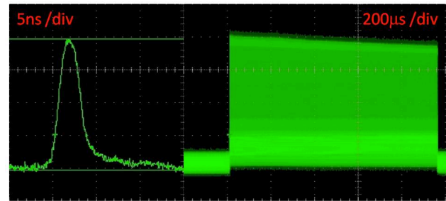
Figure 7: Combiner output.
