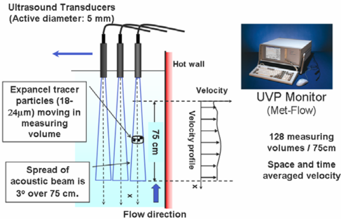
Figure III.3. Schematic of UVP transducer configuration and instrument used in project.
