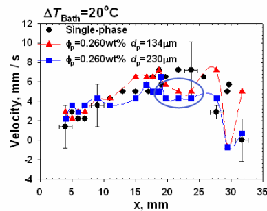
Figure III.5. UVP acquired velocity profiles for single- and two-phase, for two nominal particle sizes and given \Delta T_{\text{bath}} ; schematic of particles with opposite trajectories in BL.
