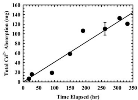
Figure I.9. Average Flame Atomic Absorption Spectroscopy data for microporous monolithic-gel \text{Cd}^{2+} filters. The waste simulant solution had an initial concentration of [\text{Cd}^{2+}] = 4.3 \text{ g}\cdot\text{l}^{-1} .
