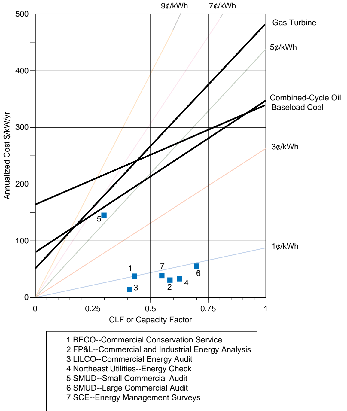
Figure 1: Screening Curve for Commercial Audit Programs. Sources: Conservation Programs--Nadel 1990; Supply Technologies--EPRI 1986
