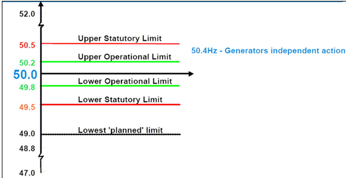
Figure C-4: Frequency Control in the UK [Morfill 2005]
