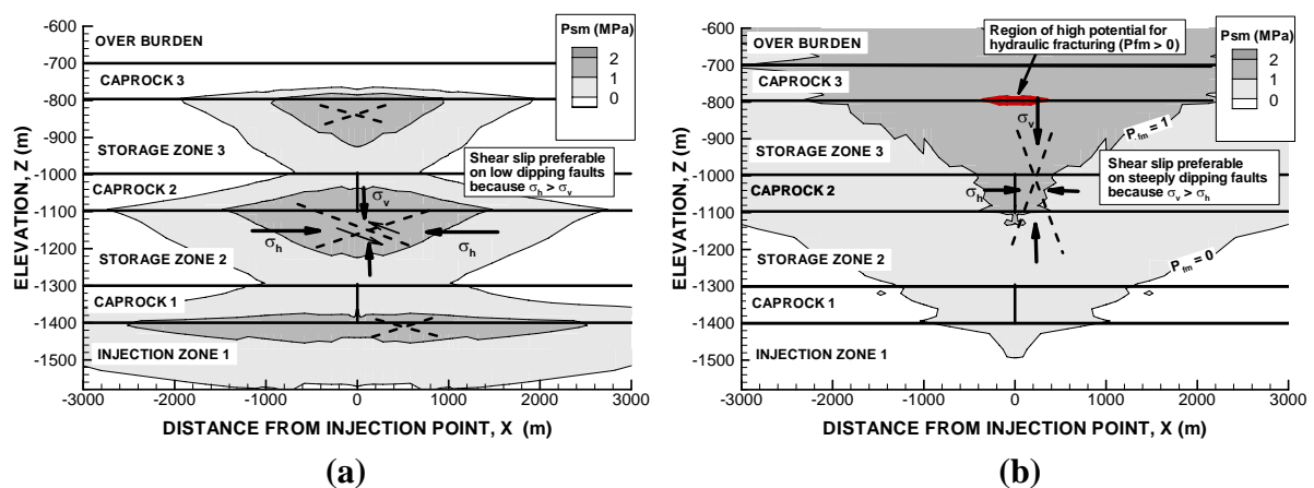
Figure 4. Calculated pressure margin for shear slip under (a) compressional stress regime and (b) extensional stress regime. The one and only location for hydraulic fracturing is also indicated in (b).
