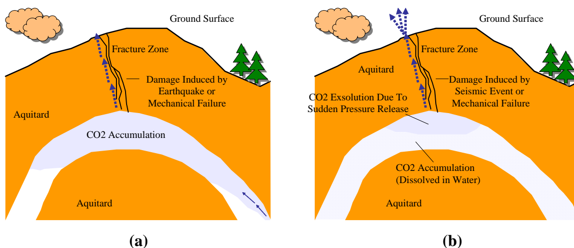
Figure 1. Sudden CO 2 leakage from secondary accumulation in shallow reservoirs. (a) CO 2 accumulates as a separate phase. (b) CO 2 is dissolved in water. A fracture or fault zone may develop as a result of geomechanical damage or in response to seismic activity.
