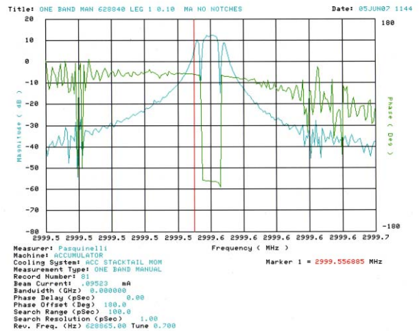
Figure 4: Single Schottky band transfer function measurement. Center frequency is at the beam revolution harmonic, red line marker off resonance frequency. Note 180-degree phase shift along with reduced amplitude response.
