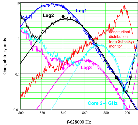
Figure 6: Top shows the Schottky signals from all longitudinal cooling systems in the Accumulator while stacking. Leg 1,2,3 refers to the Schottky signal from each individual pickup of the Stacktail system. Also included is the Stacktail longitudinal profile. Bottom shows the Schottky signals normalized to the distribution profile. The dots are the network analyzer transfer function measurements at various revolution frequencies. The close agreement indicates the transfer functions are truly representative of the system gain, which is most important for the computer model.
