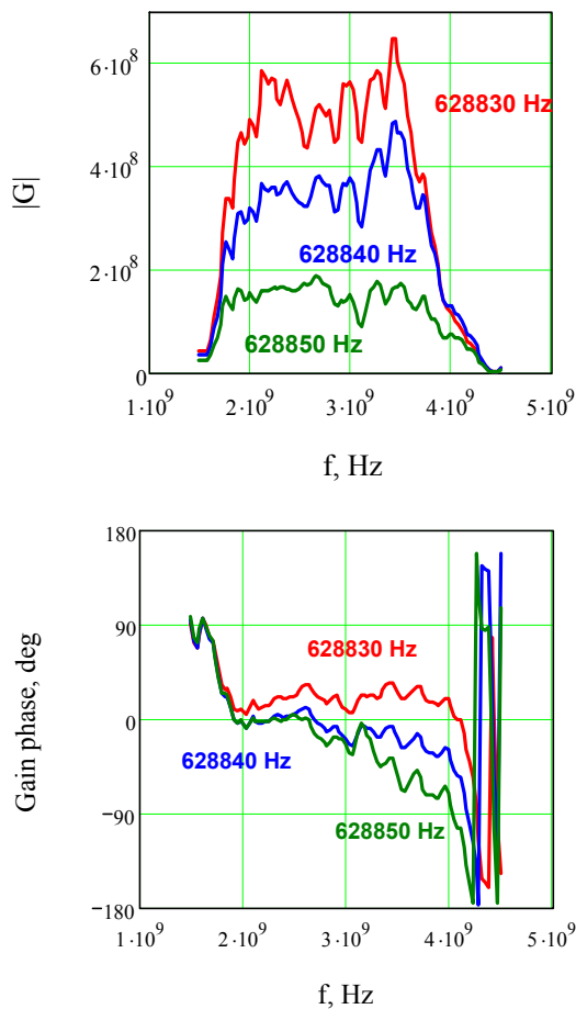
Figure 7: Transfer functions as a function of beam revolution frequency in the 2-4 GHz system bandwidth.
