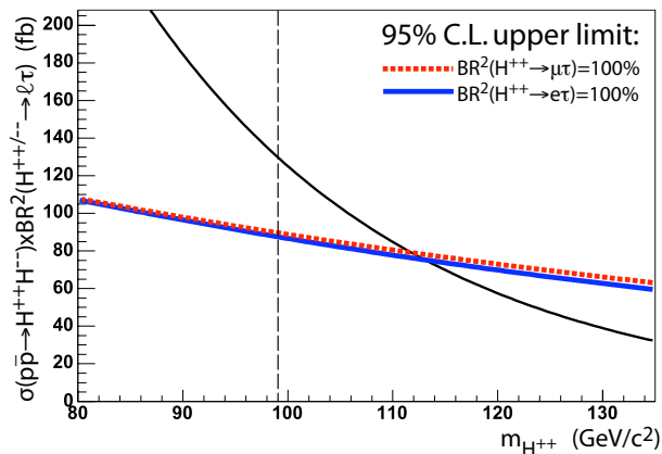
FIG. 1: Theoretical production cross sections for the pair production of left-handed H^{\pm\pm} , and 95% C.L. limit curves for \sigma(p\bar{p} \rightarrow H^{++}H^{--} \rightarrow \ell\tau) \times B^2(\ell^+\tau^+\ell^-\tau^-) , for \ell = e (solid), \mu (dashed). The vertical dashed line corresponds to limits from experiments at LEP2 for exclusive H_L^{\pm\pm} decays to any one dilepton channel [9].
