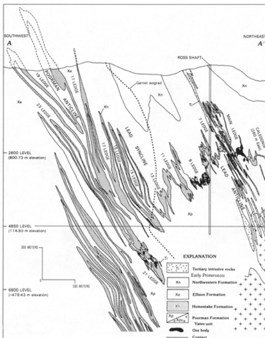
Figure 2: Geologic Cross-section, (Source: http://homestake.sdsmt.edu/HRB/Refer.htm )
