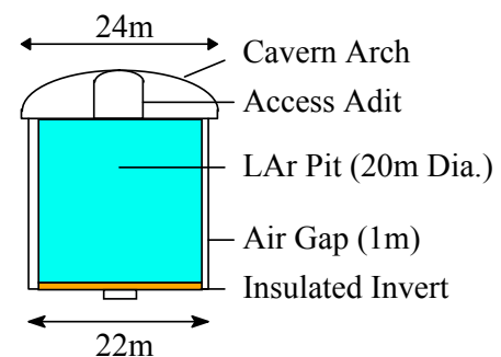
Figure 4: Low Cover LAr Cavern
