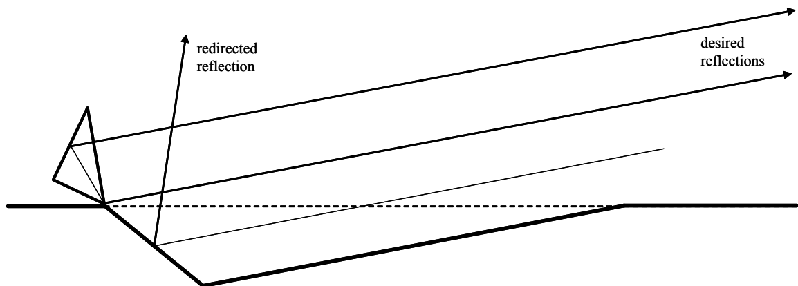
Figure 20. A pit dug in front of the reflector might also redirect otherwise problematic reflections.
