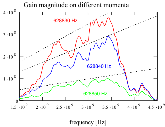
Figure 11: Stacktail gain after installation of an equalizer.
