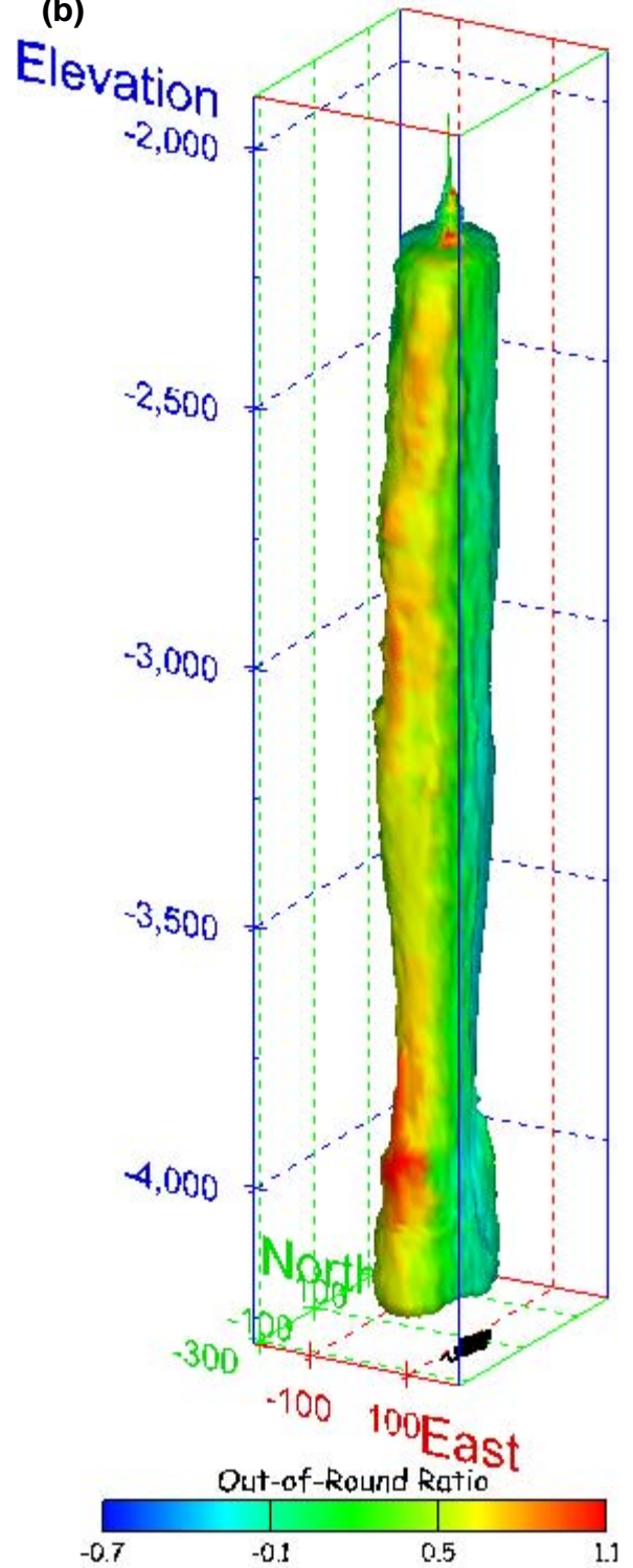
Figure 188. Sonar images of cavern BM-102, showing the geometry of the cavern colored by out-of-round ratio. View from (a) azimuth 210°, elevation 20°; (b) azimuth 150°, elevation 20°.
