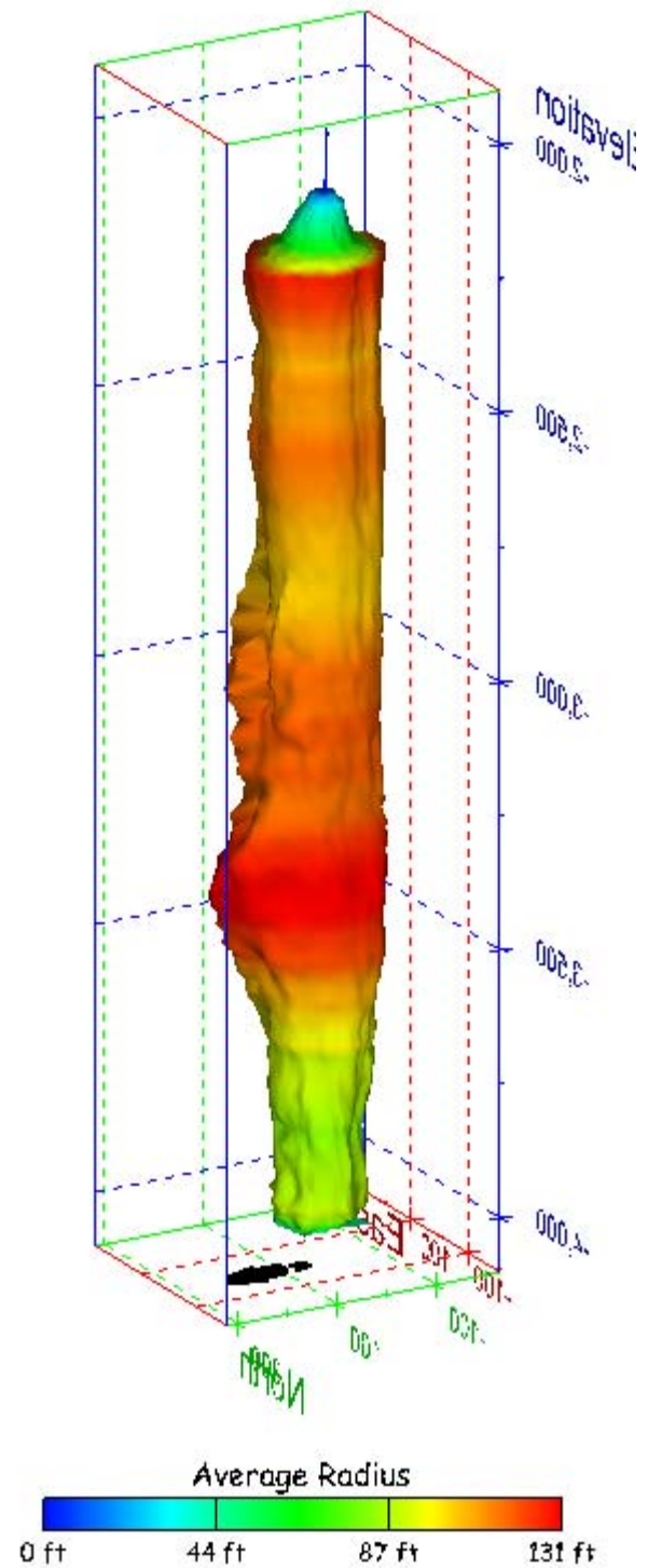
Figure 205. Sonar images of cavern BM-103, showing the geometry of the cavern colored by average radius. View from (a) azimuth 60°, elevation 20°; (b) azimuth 300°, elevation 20°.
