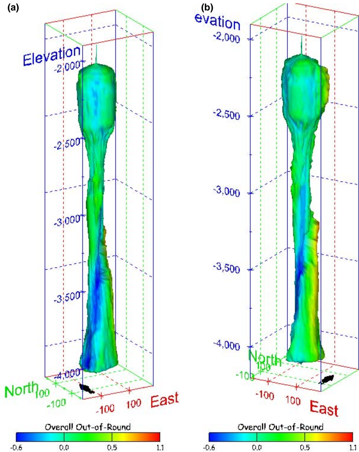
Figure 476. Sonar images of cavern BM-113, showing the geometry of the cavern colored by overall out-of-round ratio. View from (a) azimuth 210°, elevation 20°; (b) azimuth 150°, elevation 20°.
