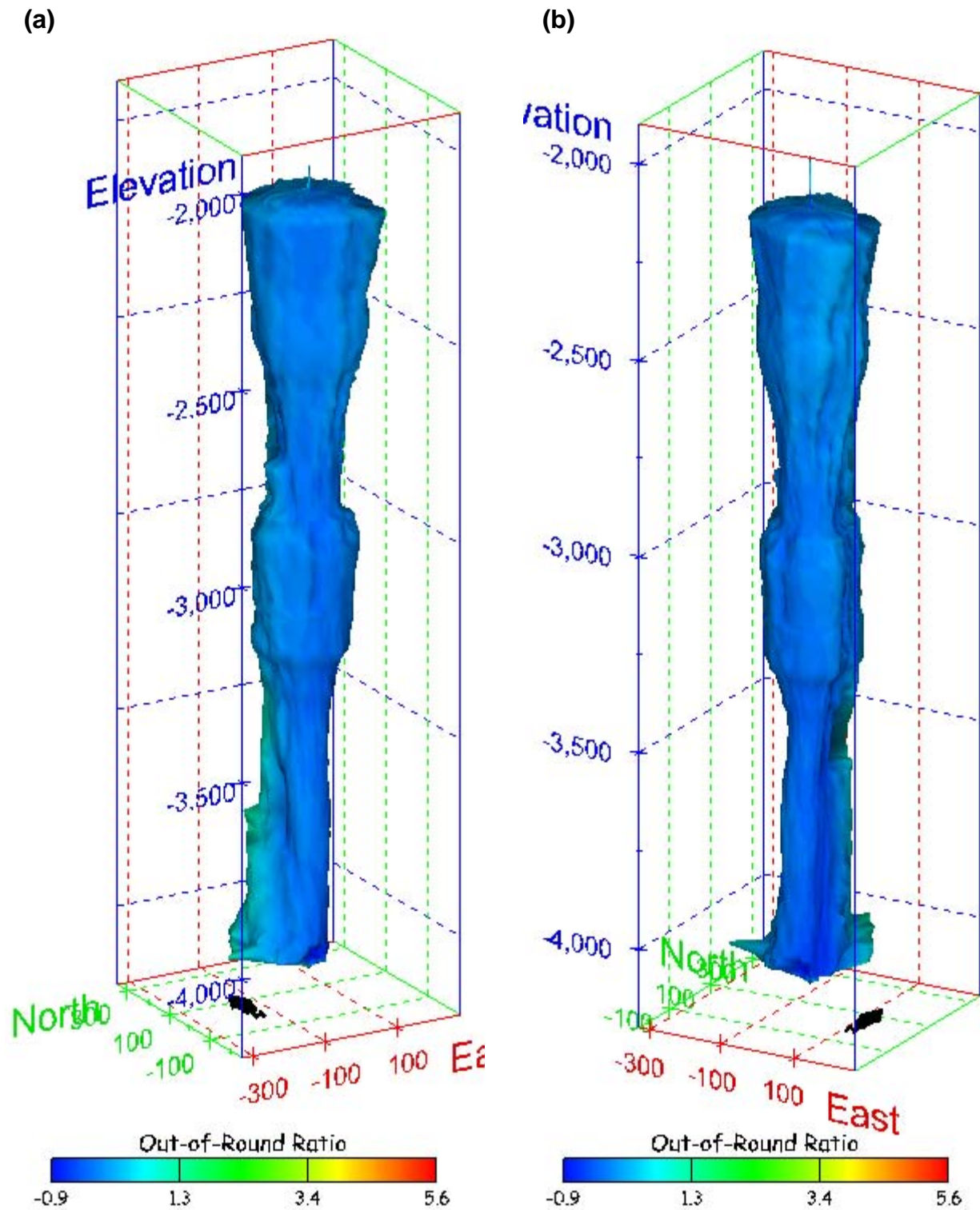
Figure 370. Sonar images of cavern BM-109, showing the geometry of the cavern colored by out-of-round ratio. View from (a) azimuth 210°, elevation 20°; (b) azimuth 150°, elevation 20°.
