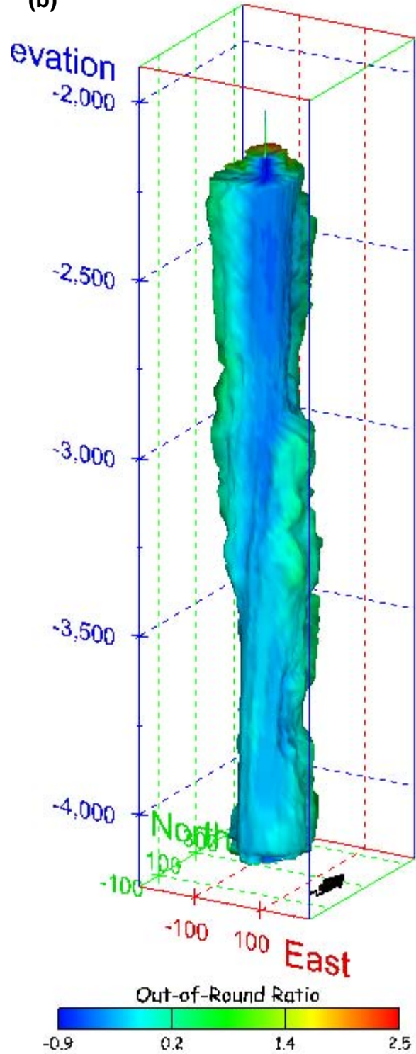
Figure 344. Sonar images of cavern BM-108, showing the geometry of the cavern colored by out-of-round ratio. View from (a) azimuth 210°, elevation 20°; (b) azimuth 150°, elevation 20°.
