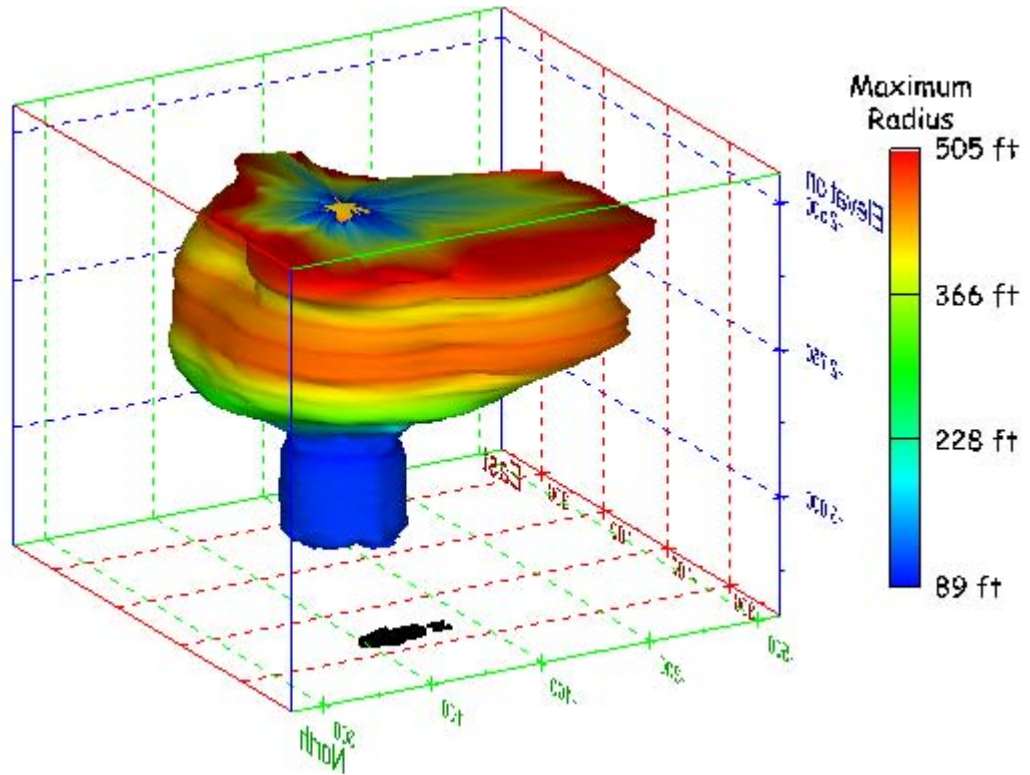
Figure 105. Sonar images of cavern BM-4, showing the geometry of the cavern colored by maximum radius. View from (a) azimuth 60°, elevation 20°; (b) azimuth 300°, elevation 20°.
