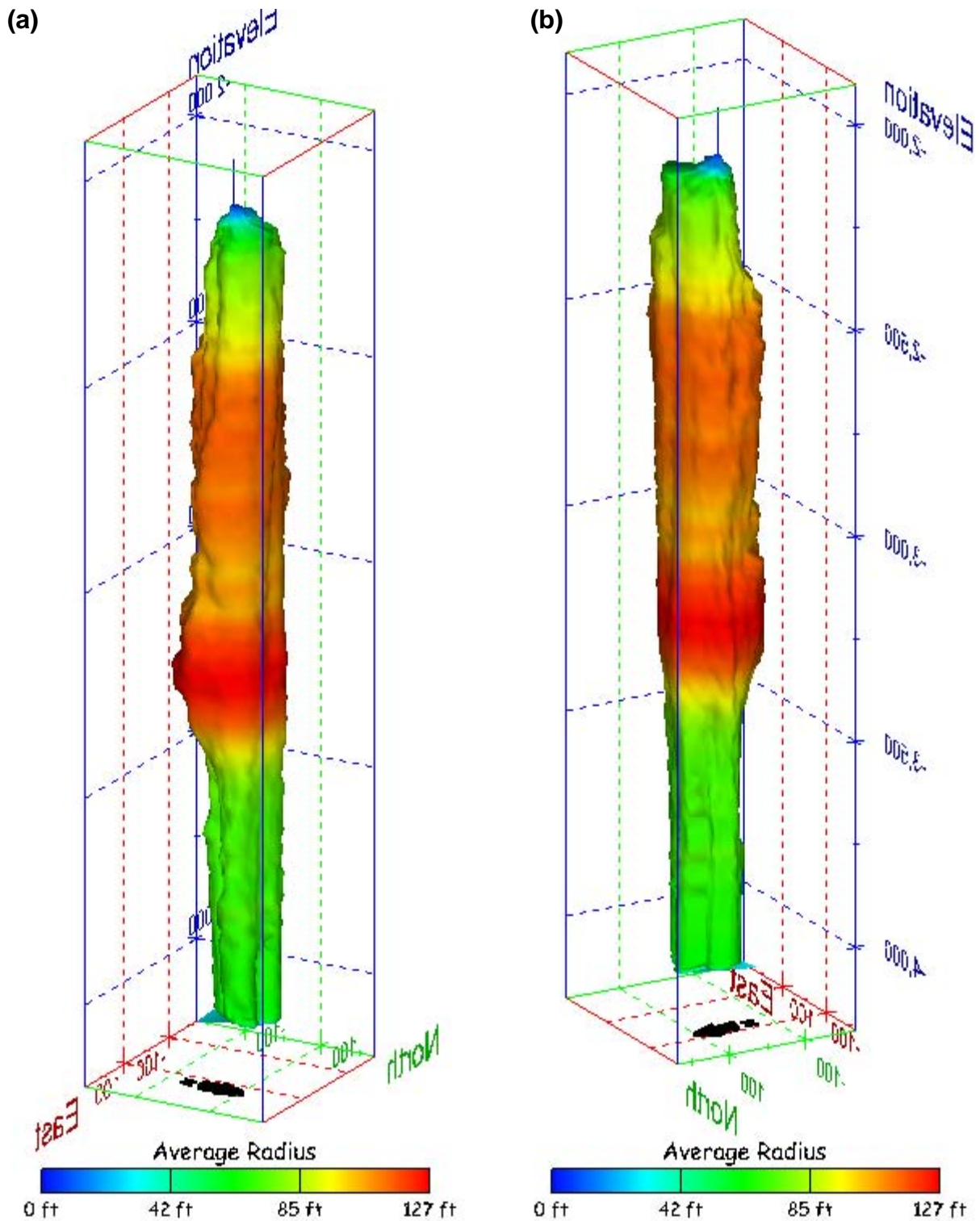
Figure 387. Sonar images of cavern BM-110, showing the geometry of the cavern colored by average radius. View from (a) azimuth 60°, elevation 20°; (b) azimuth 300°, elevation 20°.
