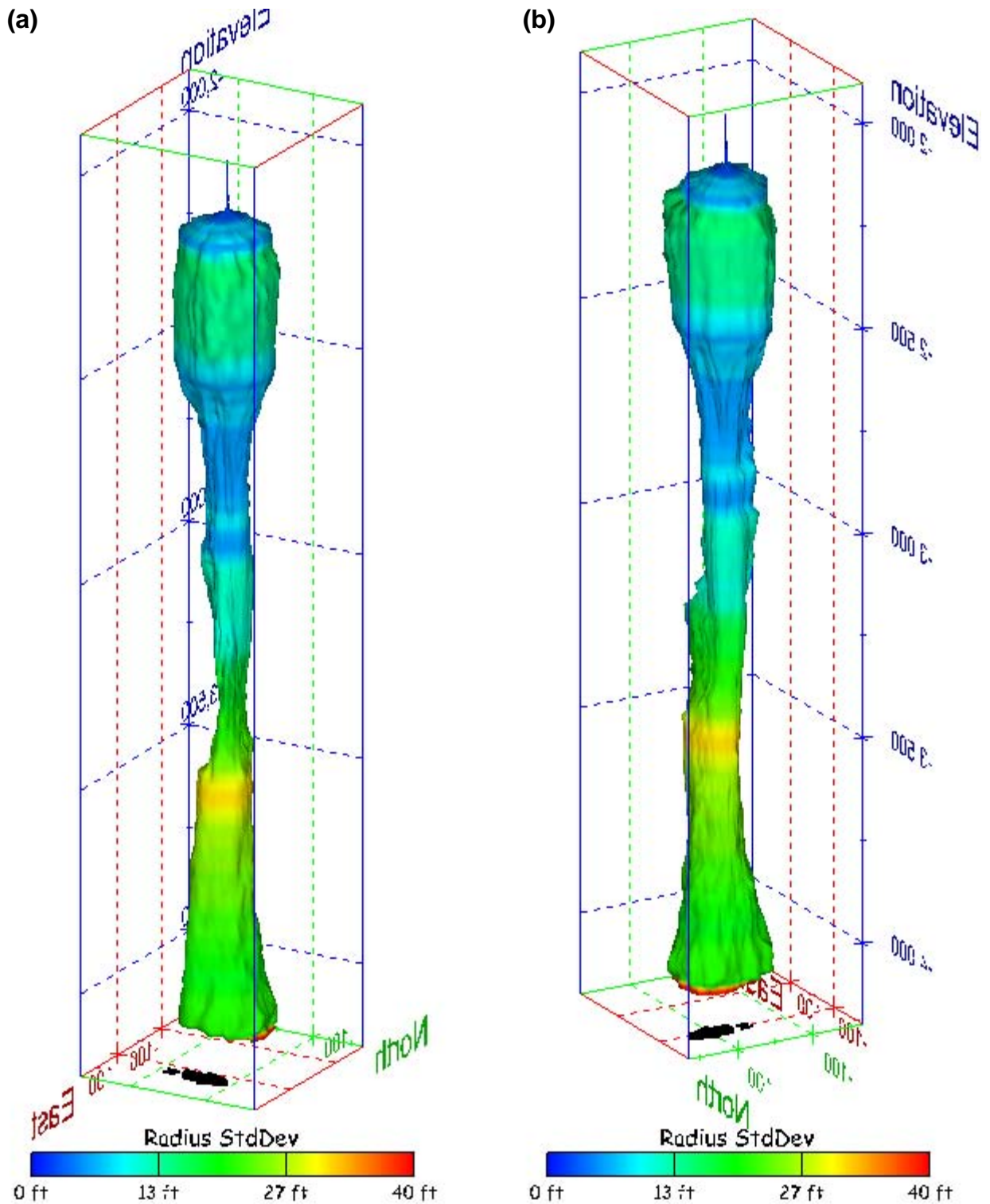
Figure 471. Sonar images of cavern BM-113, showing the geometry of the cavern colored by radius standard deviation. View from (a) azimuth 60°, elevation 20°; (b) azimuth 300°, elevation 20°.
