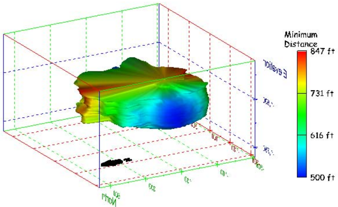
Figure 63. Sonar images of cavern BM-2, showing the geometry of the cavern colored by minimum distance to the nearest neighboring cavern. View from (a) azimuth 60°, elevation 20°; (b) azimuth 300°, elevation 20°.
