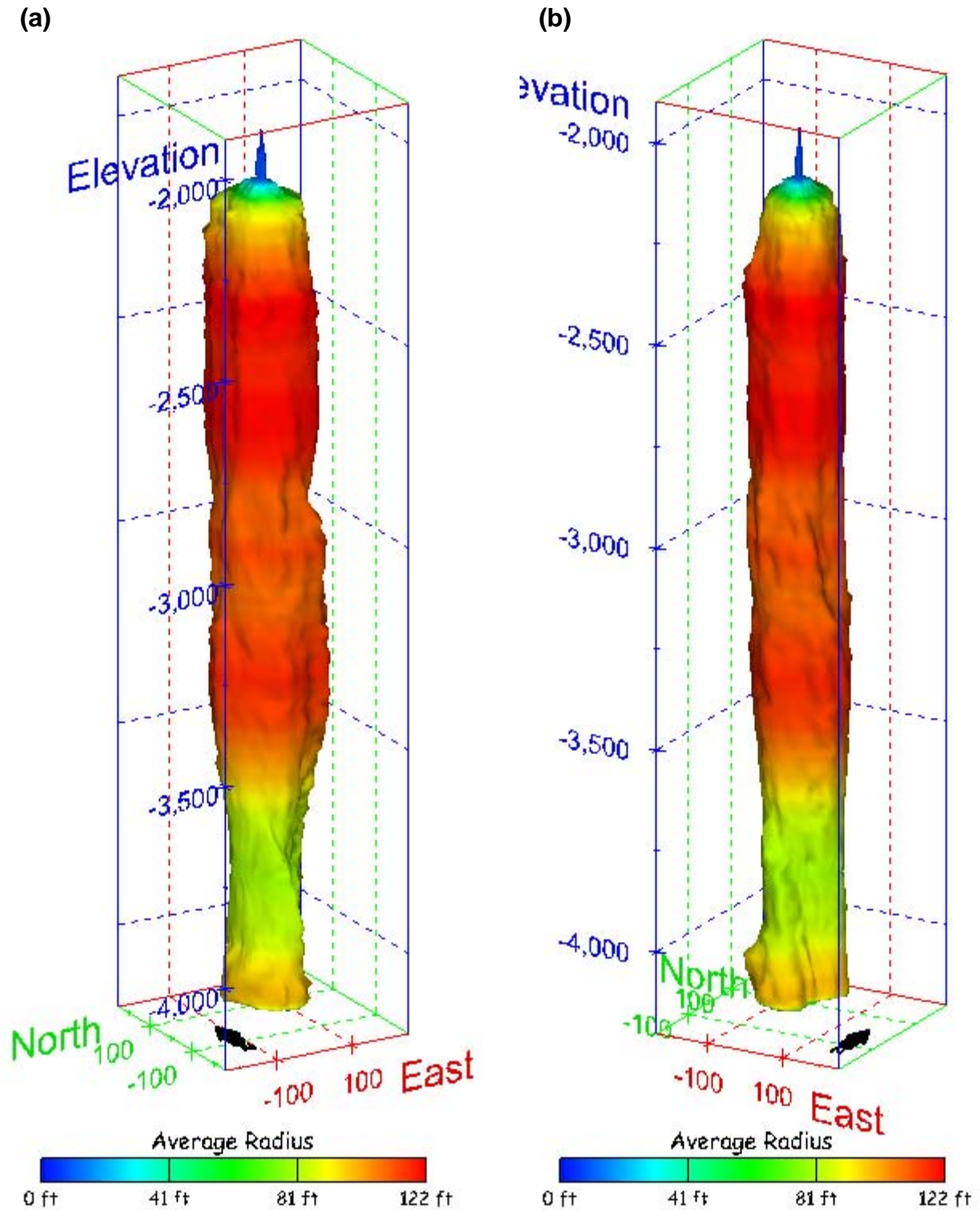
Figure 412. Sonar images of cavern BM-111, showing the geometry of the cavern colored by average radius. View from (a) azimuth 210°, elevation 20°; (b) azimuth 150°, elevation 20°.
