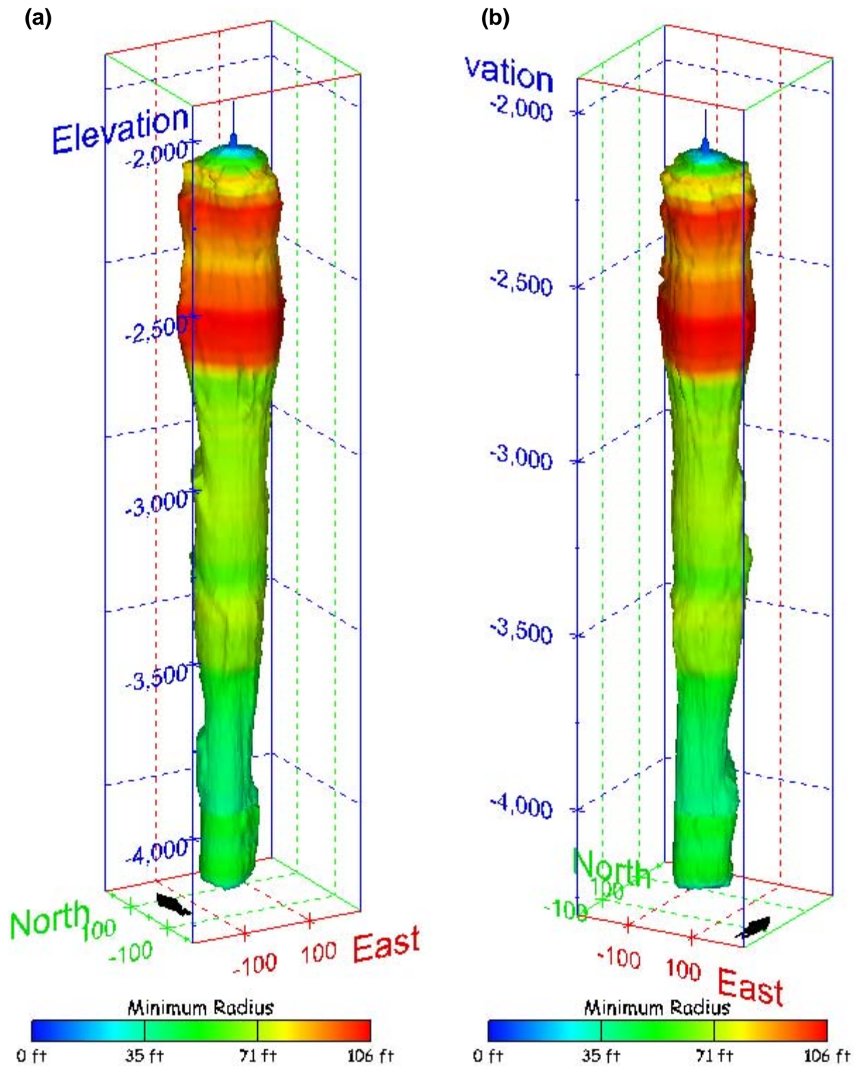
Figure 544. Sonar images of cavern BM-116, showing the geometry of the cavern colored by minimum radius. View from (a) azimuth 210°, elevation 20°; (b) azimuth 150°, elevation 20°.
