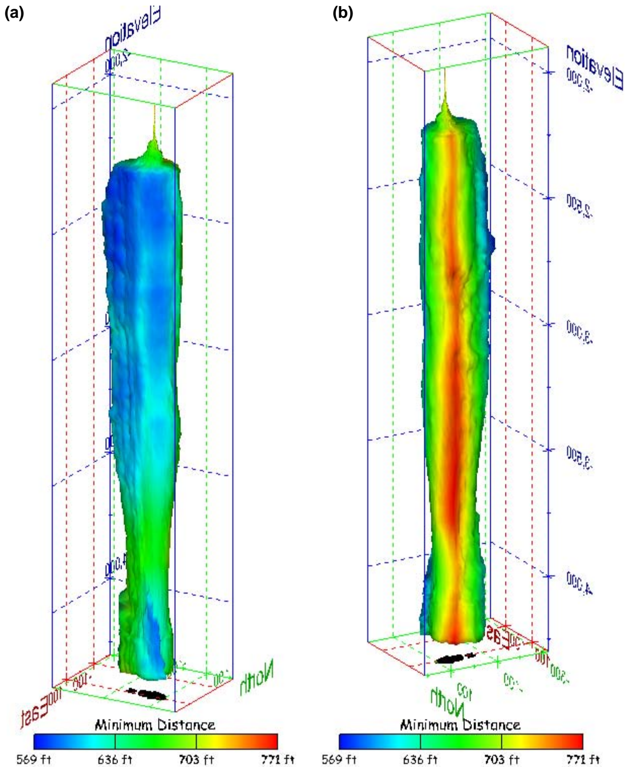
Figure 193. Sonar images of cavern BM-102, showing the geometry of the cavern colored by minimum distance to the nearest neighboring cavern. View from (a) azimuth 60°, elevation 20°; (b) azimuth 300°, elevation 20°.
