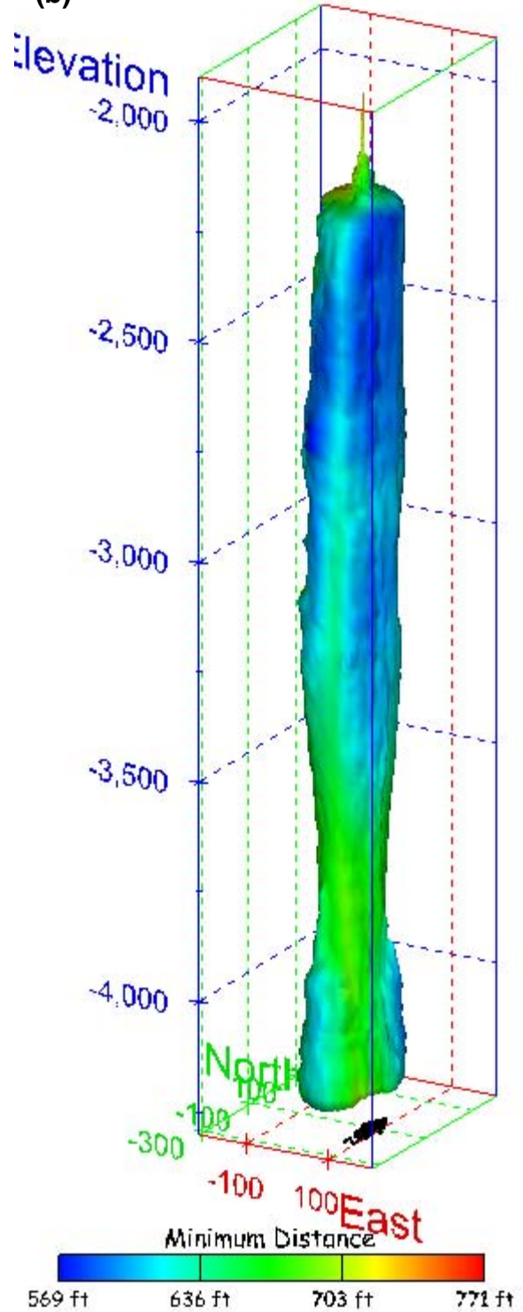
Figure 192. Sonar images of cavern BM-102, showing the geometry of the cavern colored by the minimum distance to the nearest neighboring cavern. View from (a) azimuth 210°, elevation 20°; (b) azimuth 150°, elevation 20°.
