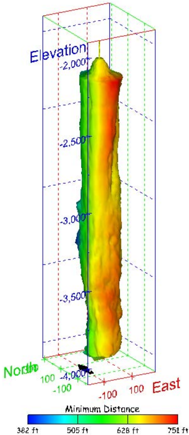
Figure 218. Sonar images of cavern BM-103, showing the geometry of the cavern colored by the minimum distance to the nearest neighboring cavern. View from (a) azimuth 210°, elevation 20°; (b) azimuth 150°, elevation 20°.
