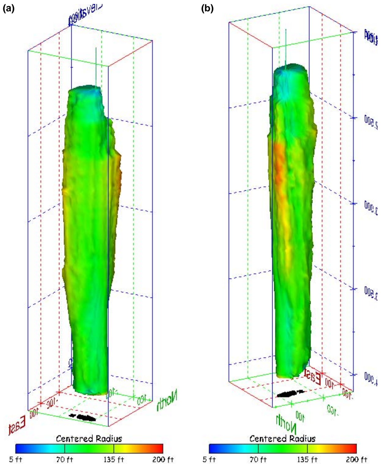
Figure 307. Sonar images of cavern BM-107, showing the geometry of the cavern colored by centered radius. View from (a) azimuth 60°, elevation 20°; (b) azimuth 300°, elevation 20°.
