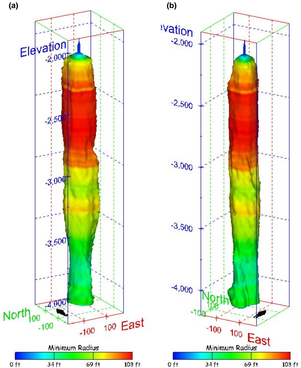
Figure 414. Sonar images of cavern BM-111, showing the geometry of the cavern colored by minimum radius. View from (a) azimuth 210°, elevation 20°; (b) azimuth 150°, elevation 20°.
