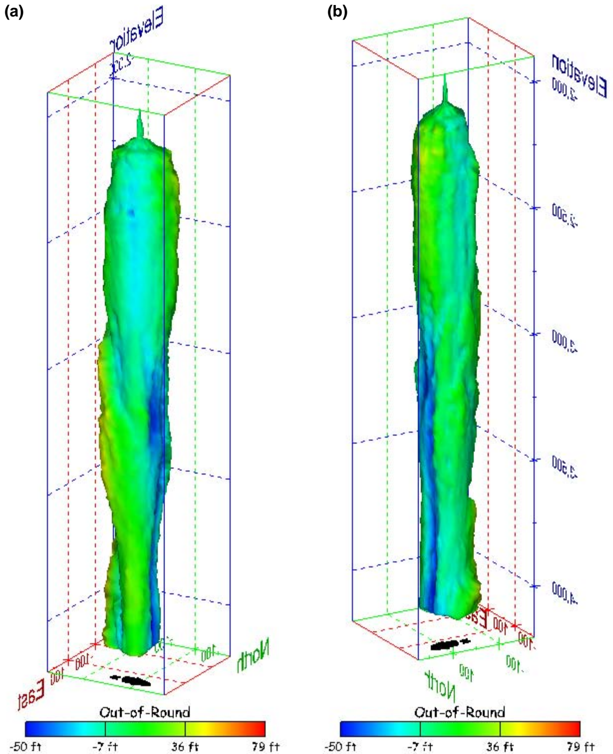
Figure 421. Sonar images of cavern BM-111, showing the geometry of the cavern colored by out-of-round distance. View from (a) azimuth 60°, elevation 20°; (b) azimuth 300°, elevation 20°.
