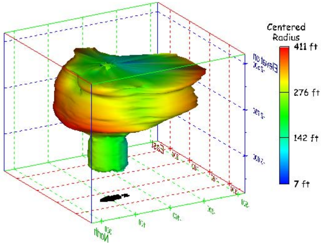
Figure 99. Sonar images of cavern BM-4, showing the geometry of the cavern colored by centered radius. View from (a) azimuth 60°, elevation 20°; (b) azimuth 300°, elevation 20°.
