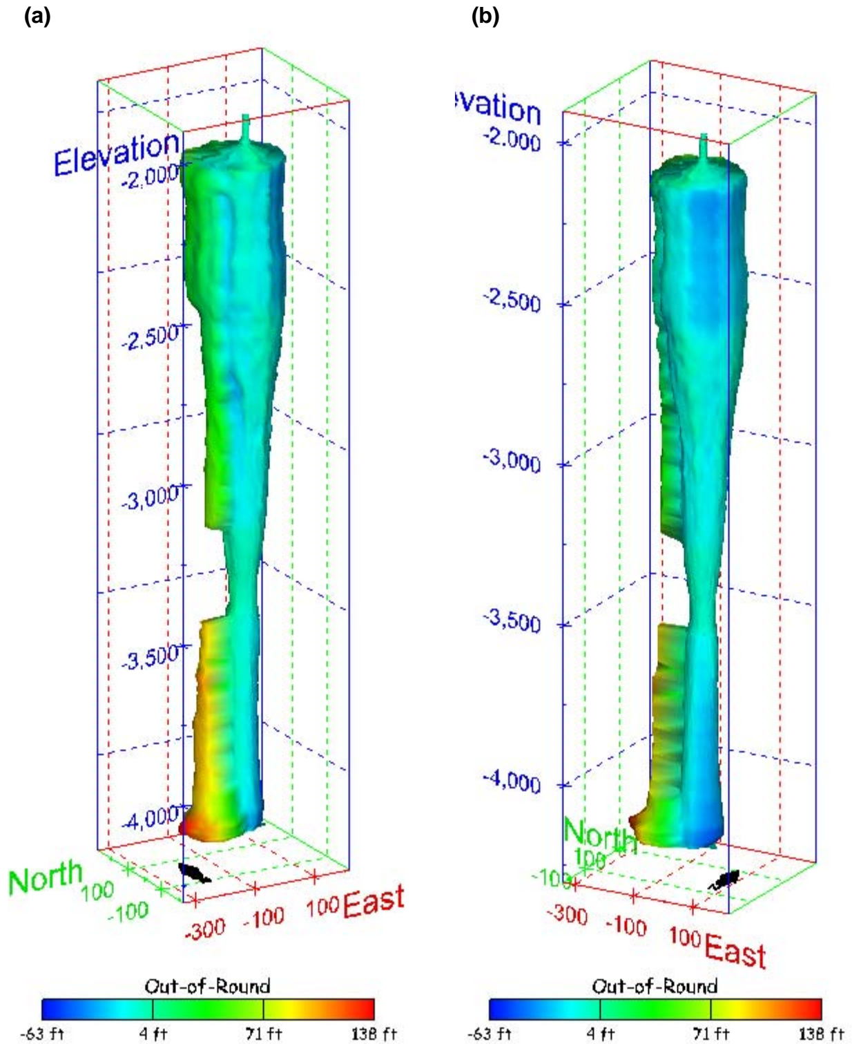
Figure 264. Sonar images of cavern BM-105, showing the geometry of the cavern colored by out-of-round distance. View from (a) azimuth 210°, elevation 20°; (b) azimuth 150°, elevation 20°.
