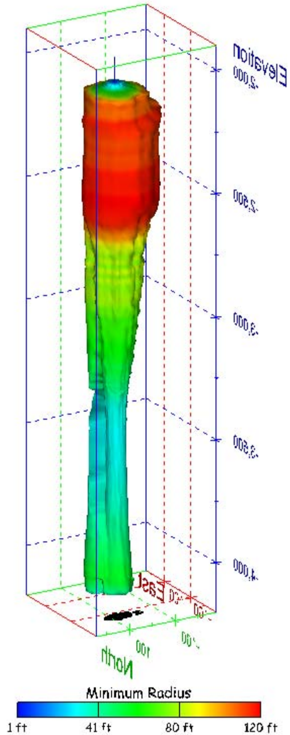
Figure 233. Sonar images of cavern BM-104, showing the geometry of the cavern colored by minimum radius. View from (a) azimuth 60°, elevation 20°; (b) azimuth 300°, elevation 20°.
