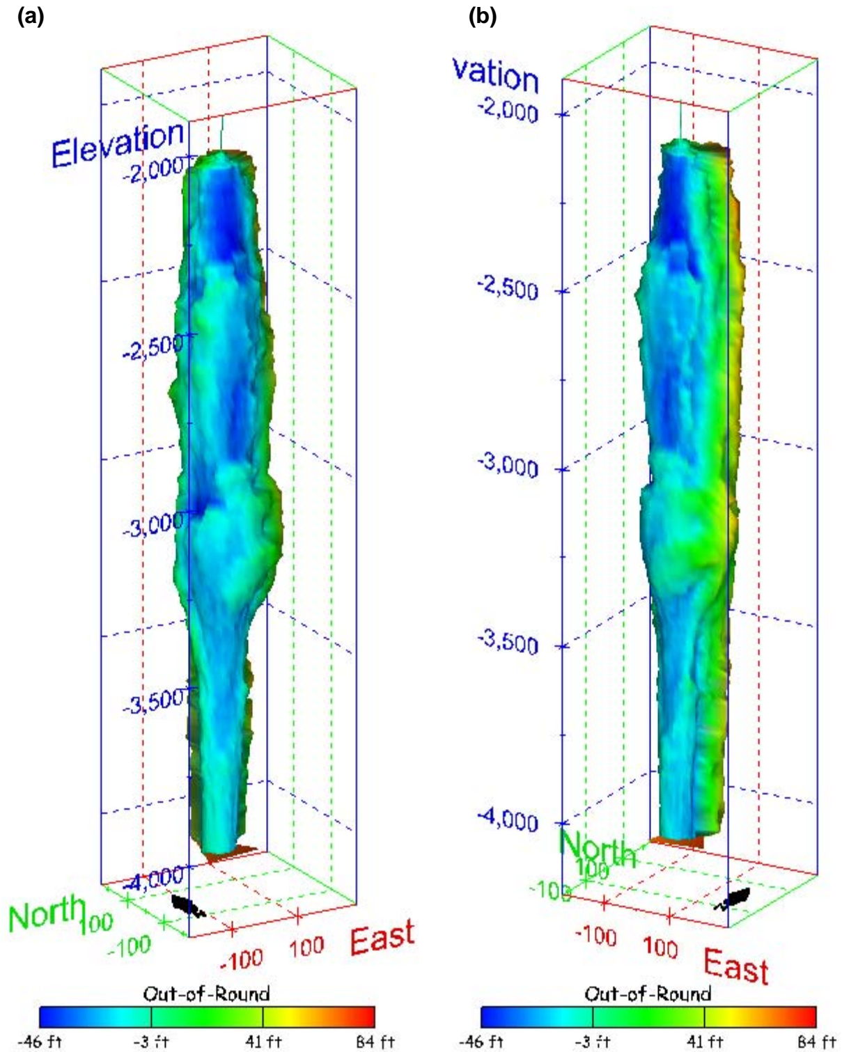
Figure 394. Sonar images of cavern BM-110, showing the geometry of the cavern colored by out-of-round distance. View from (a) azimuth 210°, elevation 20°; (b) azimuth 150°, elevation 20°.
