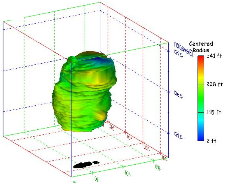
Figure 21. Sonar images of cavern BM-1, showing the geometry of the cavern colored by centered radius. View from (a) azimuth 60°, elevation 20°; (b) azimuth 300°, elevation 20°.
