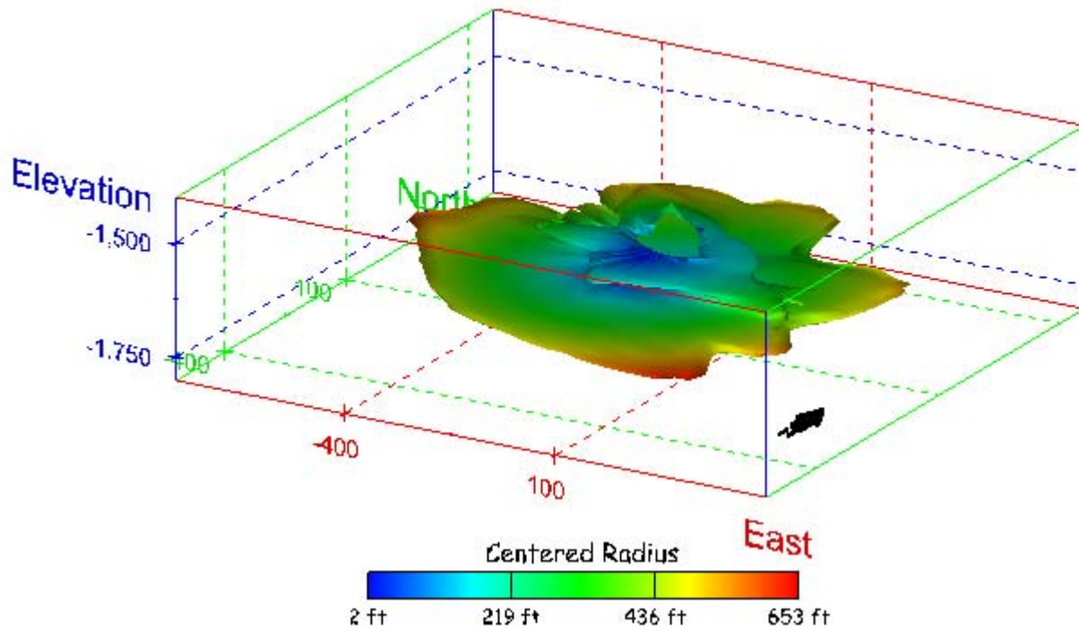
Figure 72. Sonar images of cavern BM-3, showing the geometry of the cavern colored by centered radius. View from (a) azimuth 210°, elevation 20°; (b) azimuth 150°, elevation 20°.
