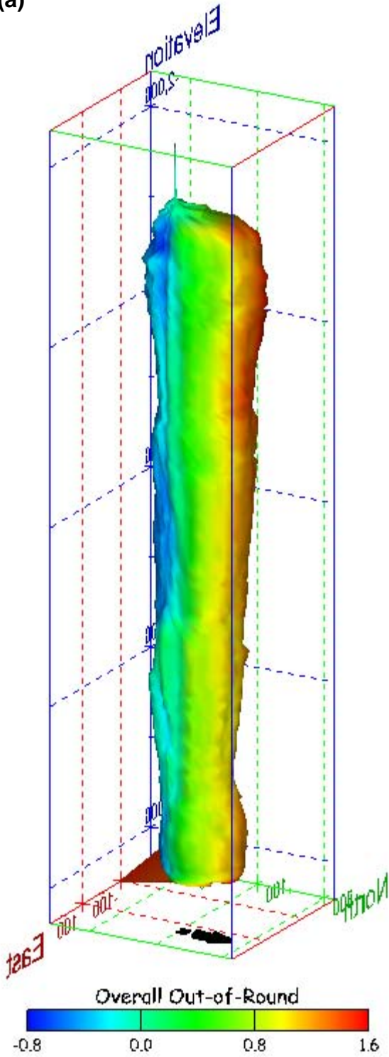
Figure 451. Sonar images of cavern BM-112, showing the geometry of the cavern colored by overall out-of-round ratio. View from (a) azimuth 60°, elevation 20°; (b) azimuth 300°, elevation 20°.
