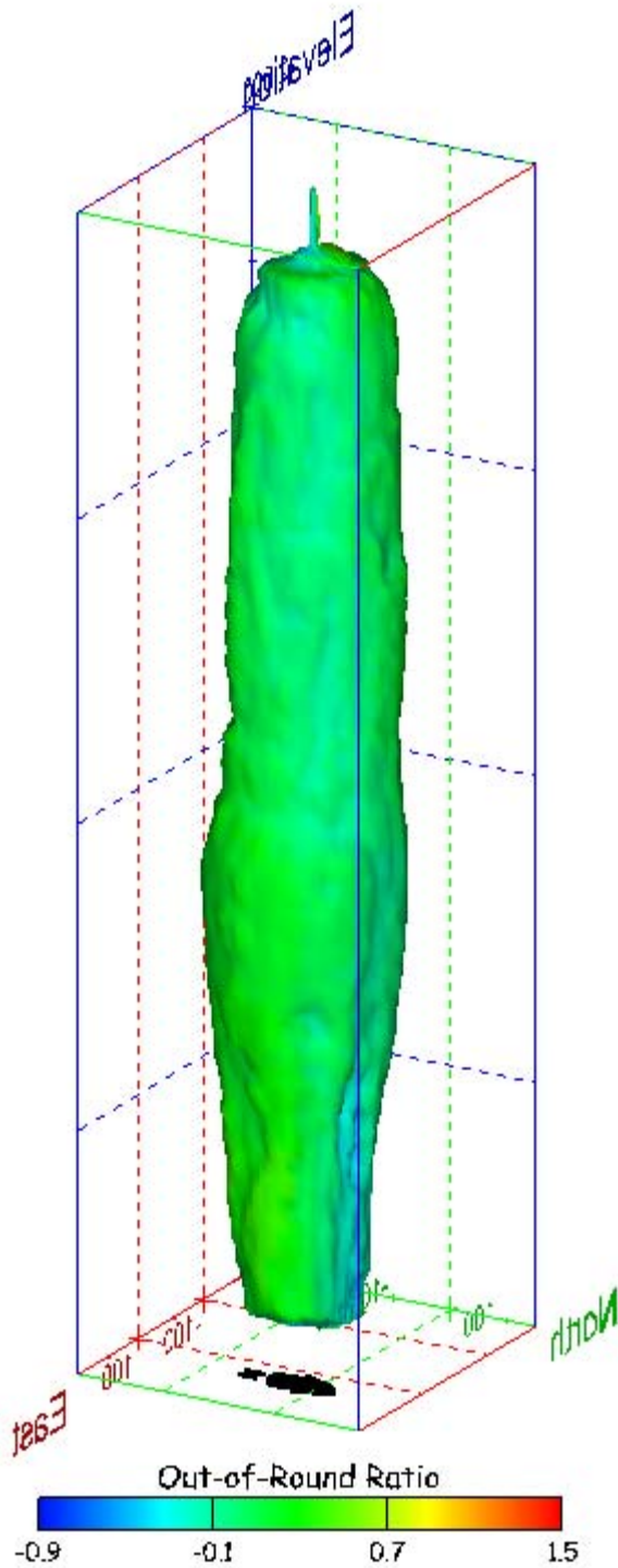
Figure 293. Sonar images of cavern BM-106, showing the geometry of the cavern colored by out-of-round ratio. View from (a) azimuth 60°, elevation 20°; (b) azimuth 300°, elevation 20°.
