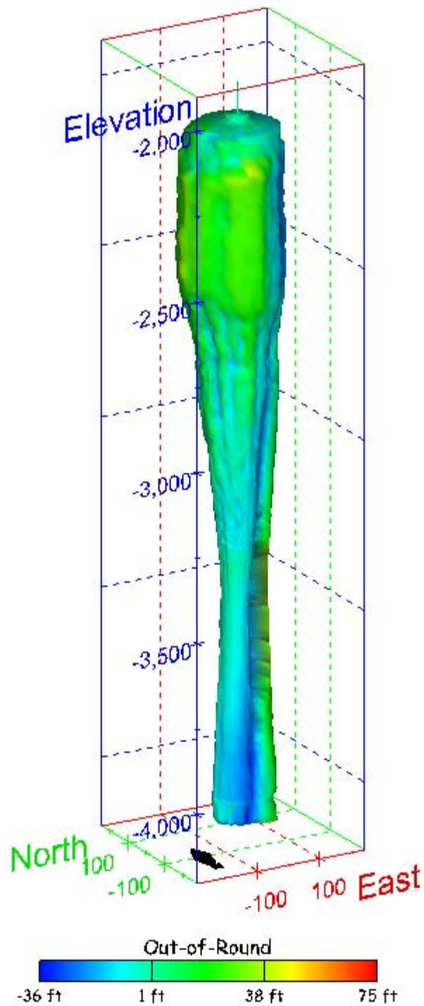
Figure 238. Sonar images of cavern BM-104, showing the geometry of the cavern colored by out-of-round distance. View from (a) azimuth 210°, elevation 20°; (b) azimuth 150°, elevation 20°.
