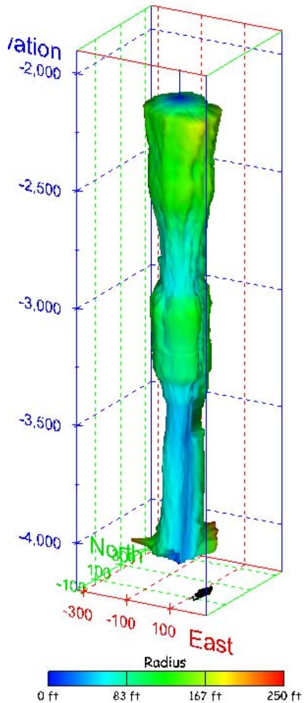
Figure 356. Sonar images of cavern BM-109, showing the geometry of the cavern colored by measured radius. View from (a) azimuth 210°, elevation 20°; (b) azimuth 150°, elevation 20°.
