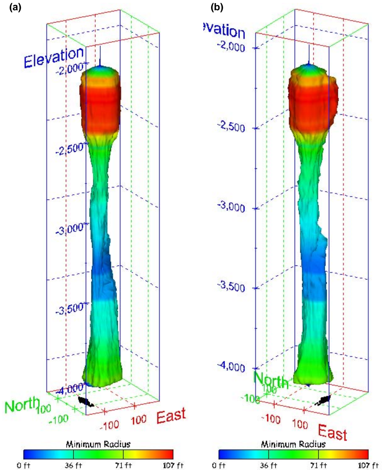
Figure 466. Sonar images of cavern BM-113, showing the geometry of the cavern colored by minimum radius. View from (a) azimuth 210°, elevation 20°; (b) azimuth 150°, elevation 20°.
