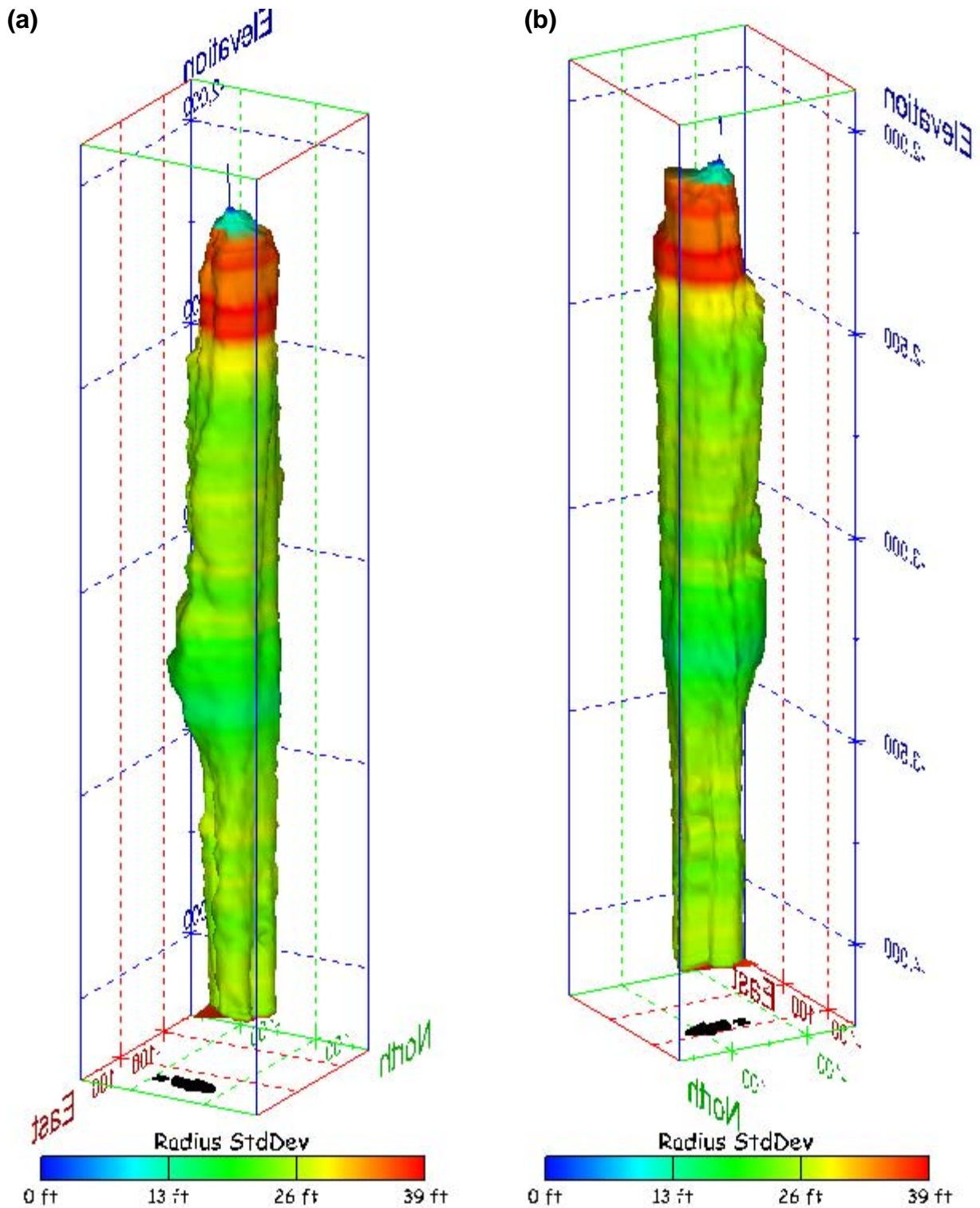
Figure 393. Sonar images of cavern BM-110, showing the geometry of the cavern colored by radius standard deviation. View from (a) azimuth 60°, elevation 20°; (b) azimuth 300°, elevation 20°.
