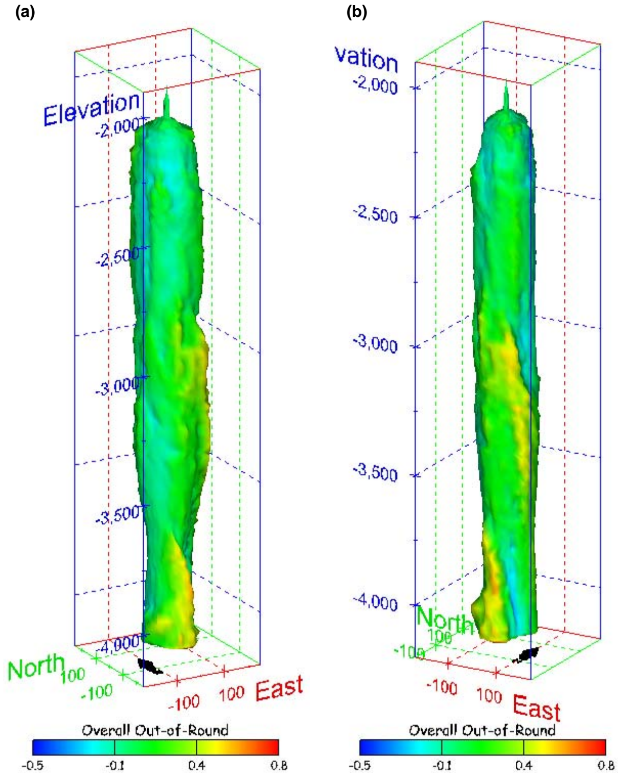
Figure 424. Sonar images of cavern BM-111, showing the geometry of the cavern colored by overall out-of-round ratio. View from (a) azimuth 210°, elevation 20°; (b) azimuth 150°, elevation 20°.
