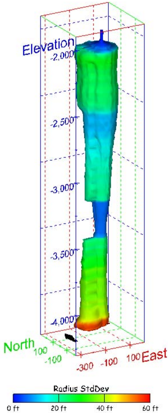
Figure 262. Sonar images of cavern BM-105, showing the geometry of the cavern colored by radius standard deviation. View from (a) azimuth 210°, elevation 20°; (b) azimuth 150°, elevation 20°.
