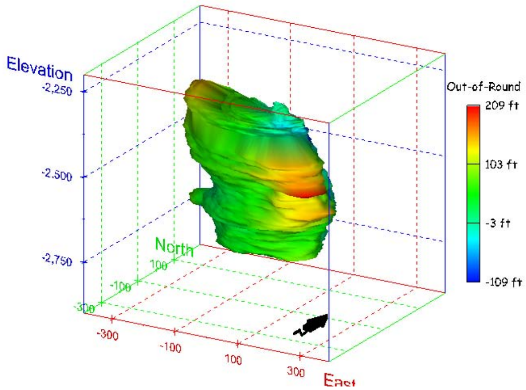
Figure 30. Sonar images of cavern BM-1, showing the geometry of the cavern colored by out-of-round distance. View from (a) azimuth 210°, elevation 20°; (b) azimuth 150°, elevation 20°.
