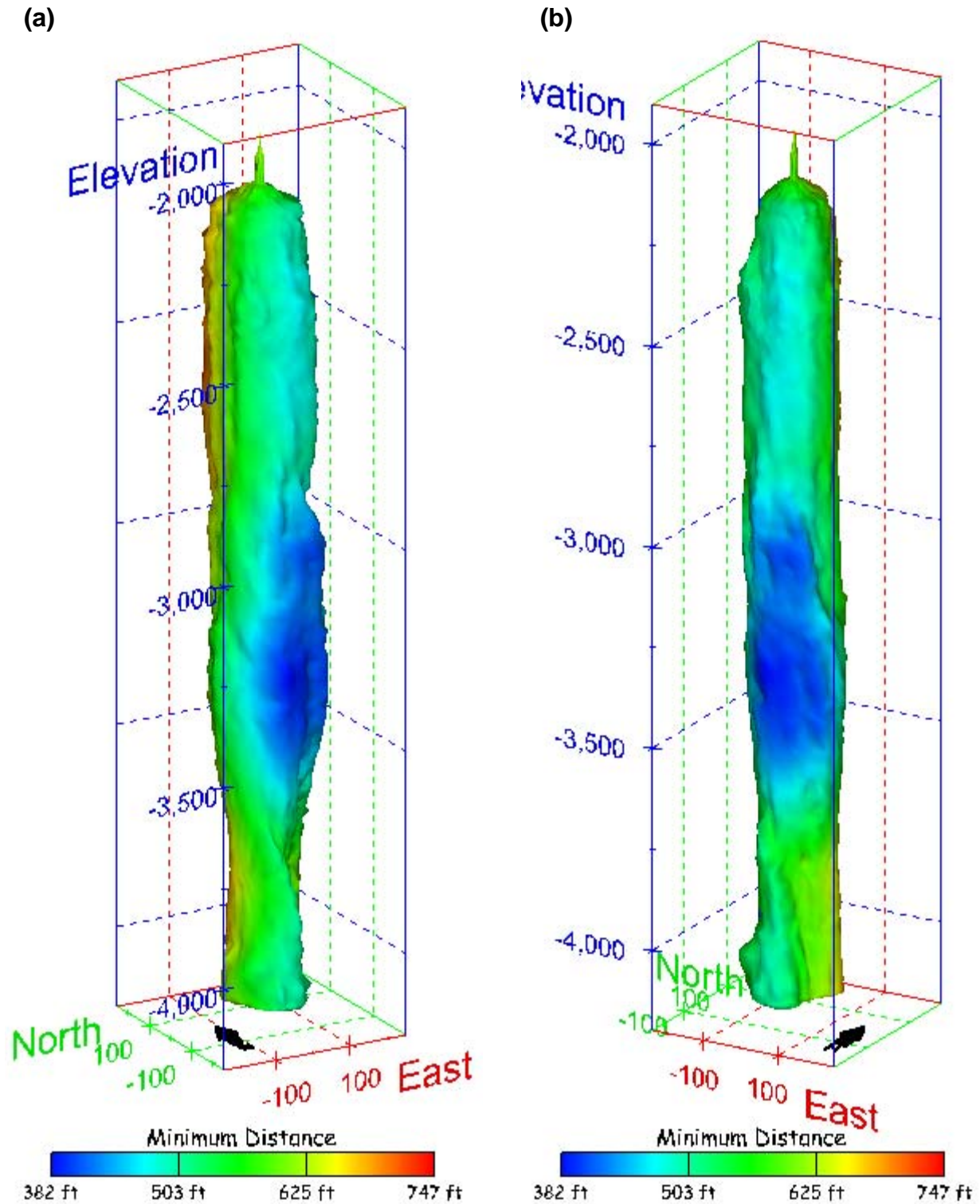
Figure 426. Sonar images of cavern BM-111, showing the geometry of the cavern colored by the minimum distance to the nearest neighboring cavern. View from (a) azimuth 210°, elevation 20°; (b) azimuth 150°, elevation 20°.
