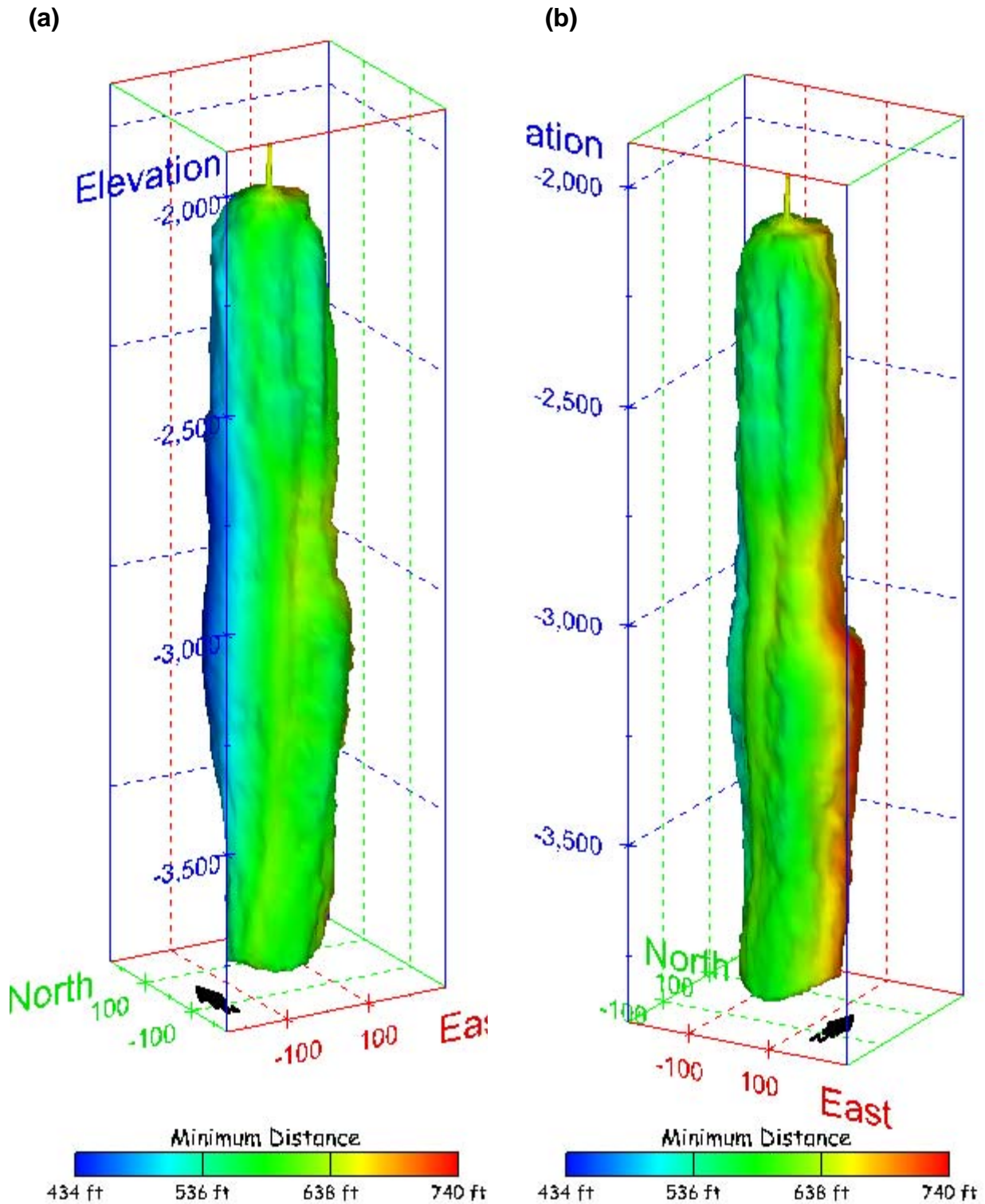
Figure 296. Sonar images of cavern BM-106, showing the geometry of the cavern colored by the minimum distance to the nearest neighboring cavern. View from (a) azimuth 210°, elevation 20°; (b) azimuth 150°, elevation 20°.
