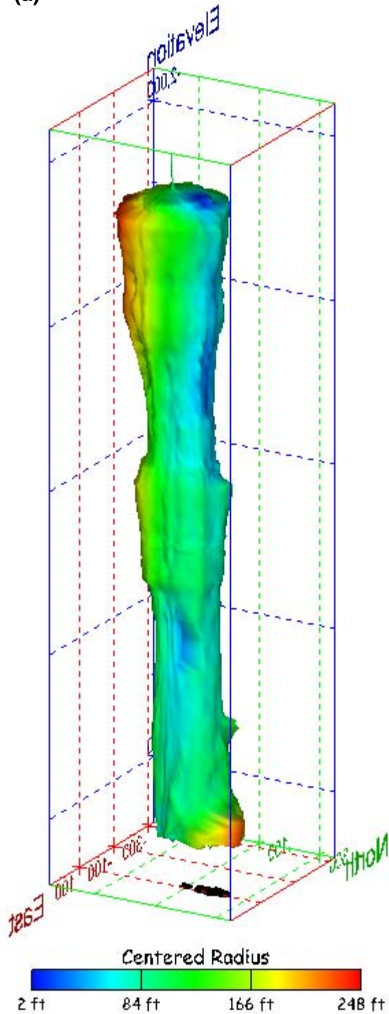
Figure 359. Sonar images of cavern BM-109, showing the geometry of the cavern colored by centered radius. View from (a) azimuth 60°, elevation 20°; (b) azimuth 300°, elevation 20°.
