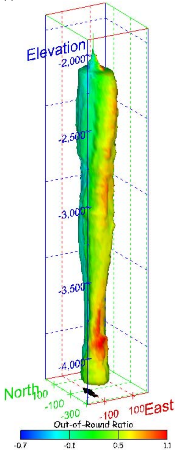
Figure 188. Sonar images of cavern BM-102, showing the geometry of the cavern colored by out-of-round ratio. View from (a) azimuth 210°, elevation 20°; (b) azimuth 150°, elevation 20°.
