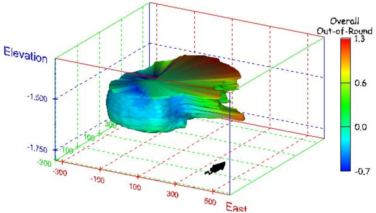
Figure 60. Sonar images of cavern BM-2, showing the geometry of the cavern colored by overall out-of-round ratio. View from (a) azimuth 210°, elevation 20°; (b) azimuth 150°, elevation 20°.
