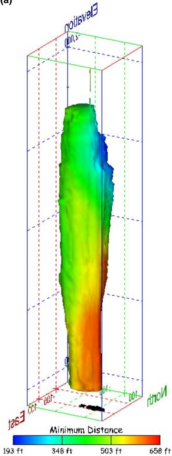
Figure 323. Sonar images of cavern BM-107, showing the geometry of the cavern colored by minimum distance to the nearest neighboring cavern. View from (a) azimuth 60°, elevation 20°; (b) azimuth 300°, elevation 20°.
