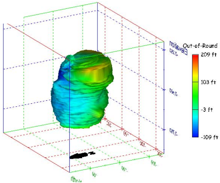
Figure 31. Sonar images of cavern BM-1, showing the geometry of the cavern colored by out-of-round distance. View from (a) azimuth 60°, elevation 20°; (b) azimuth 300°, elevation 20°.
