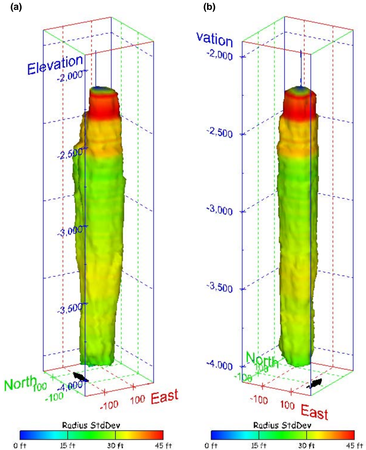
Figure 314. Sonar images of cavern BM-107, showing the geometry of the cavern colored by radius standard deviation. View from (a) azimuth 210°, elevation 20°; (b) azimuth 150°, elevation 20°.
