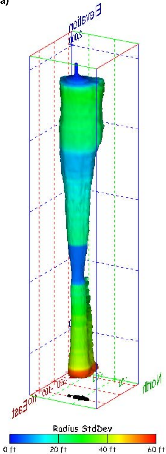
Figure 263. Sonar images of cavern BM-105, showing the geometry of the cavern colored by radius standard deviation. View from (a) azimuth 60°, elevation 20°; (b) azimuth 300°, elevation 20°.
