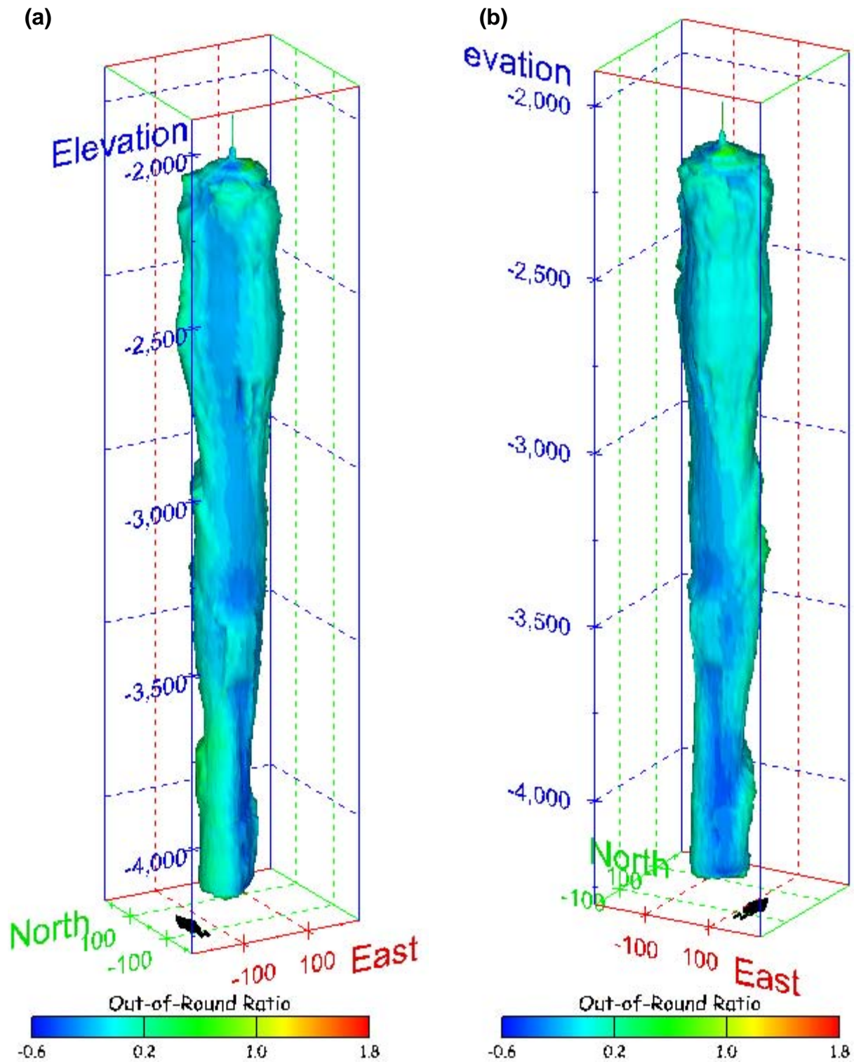
Figure 552. Sonar images of cavern BM-116, showing the geometry of the cavern colored by out-of-round ratio. View from (a) azimuth 210°, elevation 20°; (b) azimuth 150°, elevation 20°.
