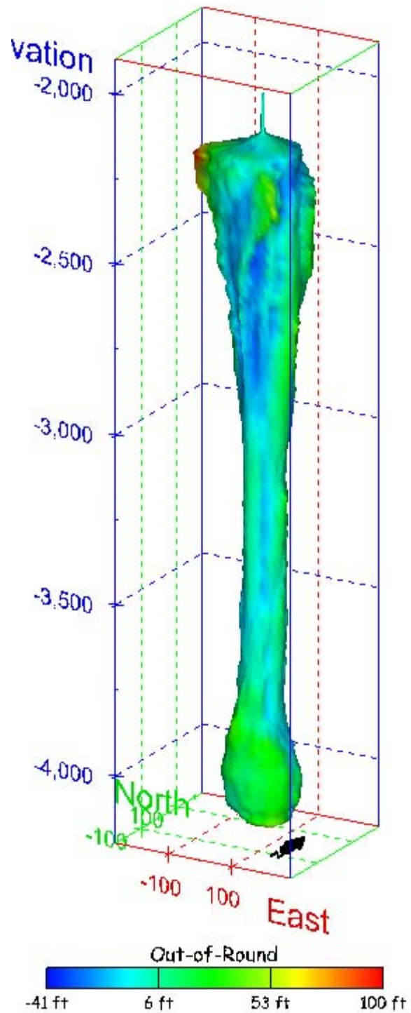
Figure 498. Sonar images of cavern BM-114, showing the geometry of the cavern colored by out-of-round distance. View from (a) azimuth 210°, elevation 20°; (b) azimuth 150°, elevation 20°.
