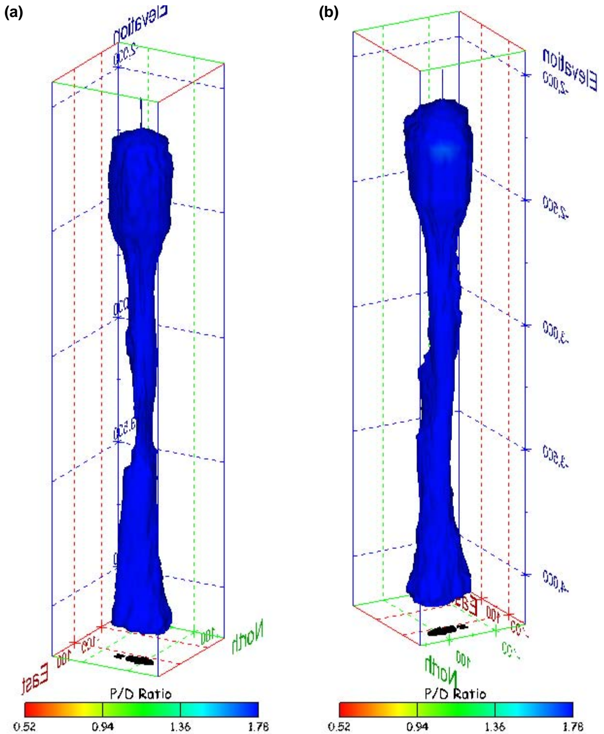
Figure 481. Sonar images of cavern BM-113, showing the geometry of the cavern colored by three-dimensional pillar-to-diameter ratio. View from (a) azimuth 60°, elevation 20°; (b) azimuth 300°, elevation 20°.
