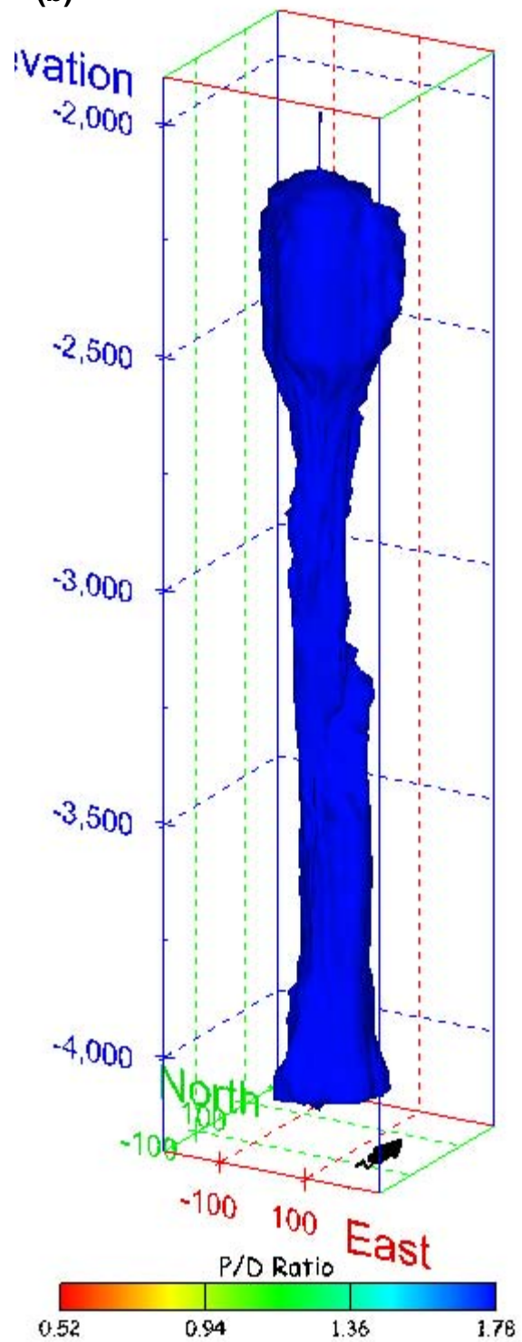
Figure 480. Sonar images of cavern BM-113, showing the geometry of the cavern colored by three-dimensional pillar-to-diameter ratio. View from (a) azimuth 210°, elevation 20°; (b) azimuth 150°, elevation 20°.
