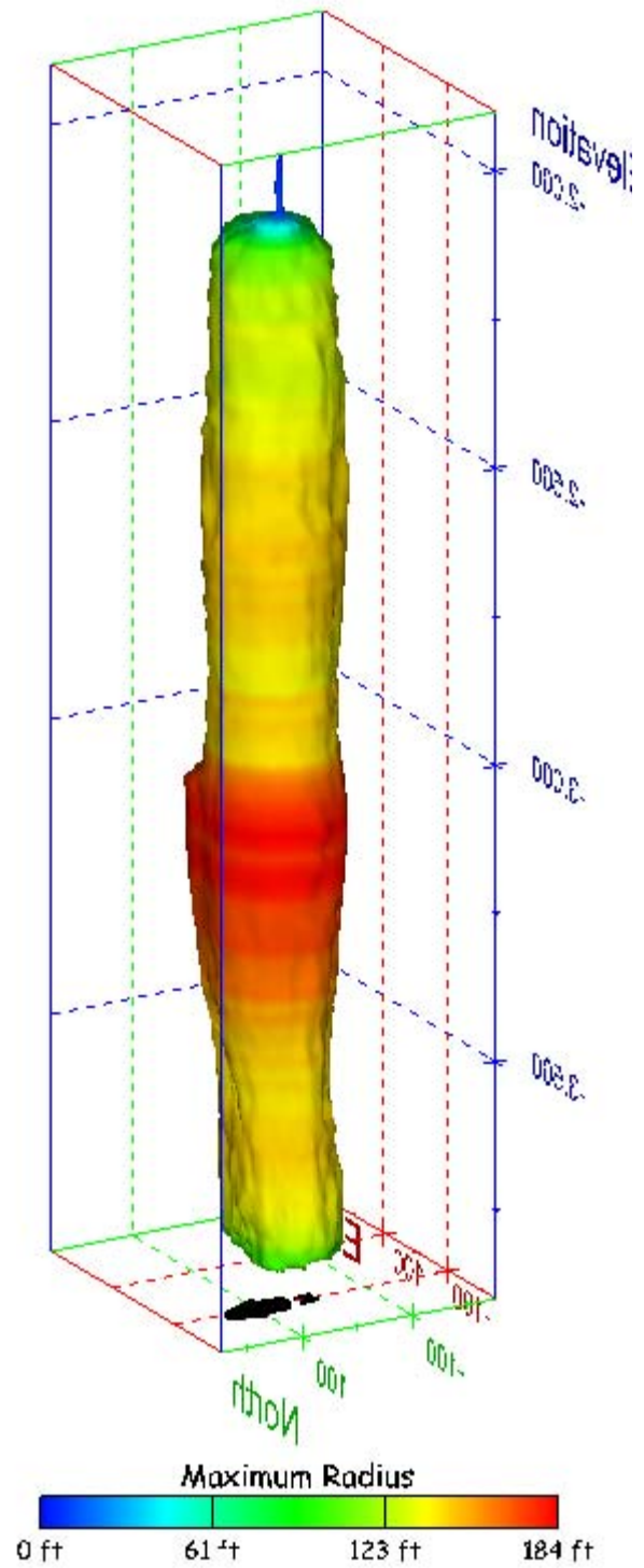
Figure 287. Sonar images of cavern BM-106, showing the geometry of the cavern colored by maximum radius. View from (a) azimuth 60°, elevation 20°; (b) azimuth 300°, elevation 20°.
