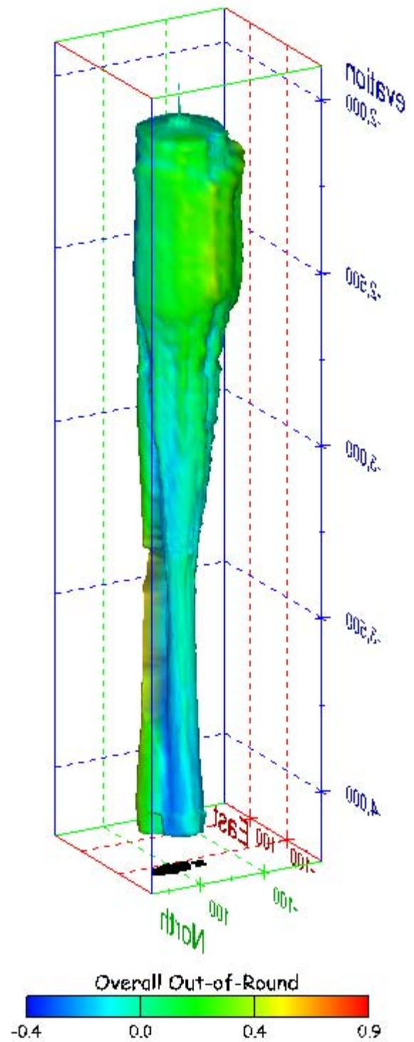
Figure 243. Sonar images of cavern BM-104, showing the geometry of the cavern colored by overall out-of-round ratio. View from (a) azimuth 60°, elevation 20°; (b) azimuth 300°, elevation 20°.
