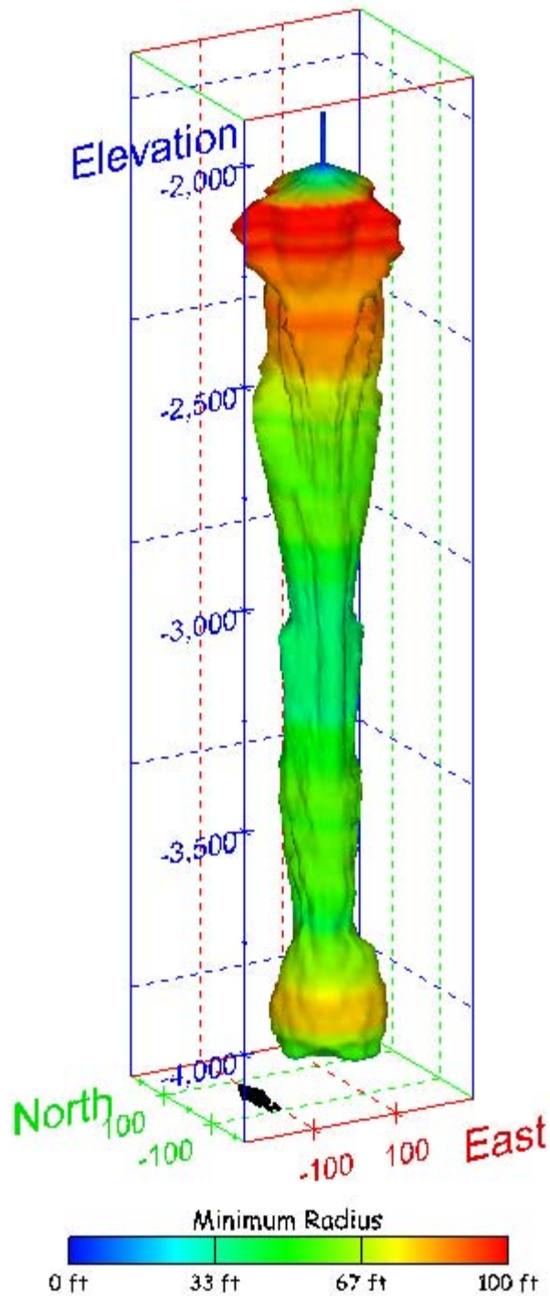
Figure 492. Sonar images of cavern BM-114, showing the geometry of the cavern colored by minimum radius. View from (a) azimuth 210°, elevation 20°; (b) azimuth 150°, elevation 20°.
