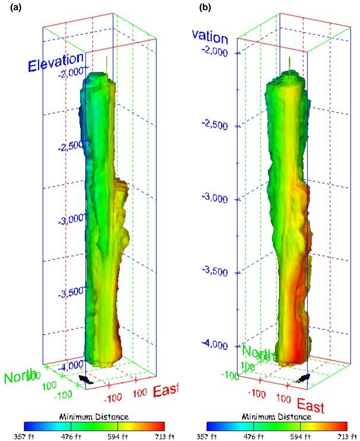
Figure 348. Sonar images of cavern BM-108, showing the geometry of the cavern colored by the minimum distance to the nearest neighboring cavern. View from (a) azimuth 210°, elevation 20°; (b) azimuth 150°, elevation 20°.
