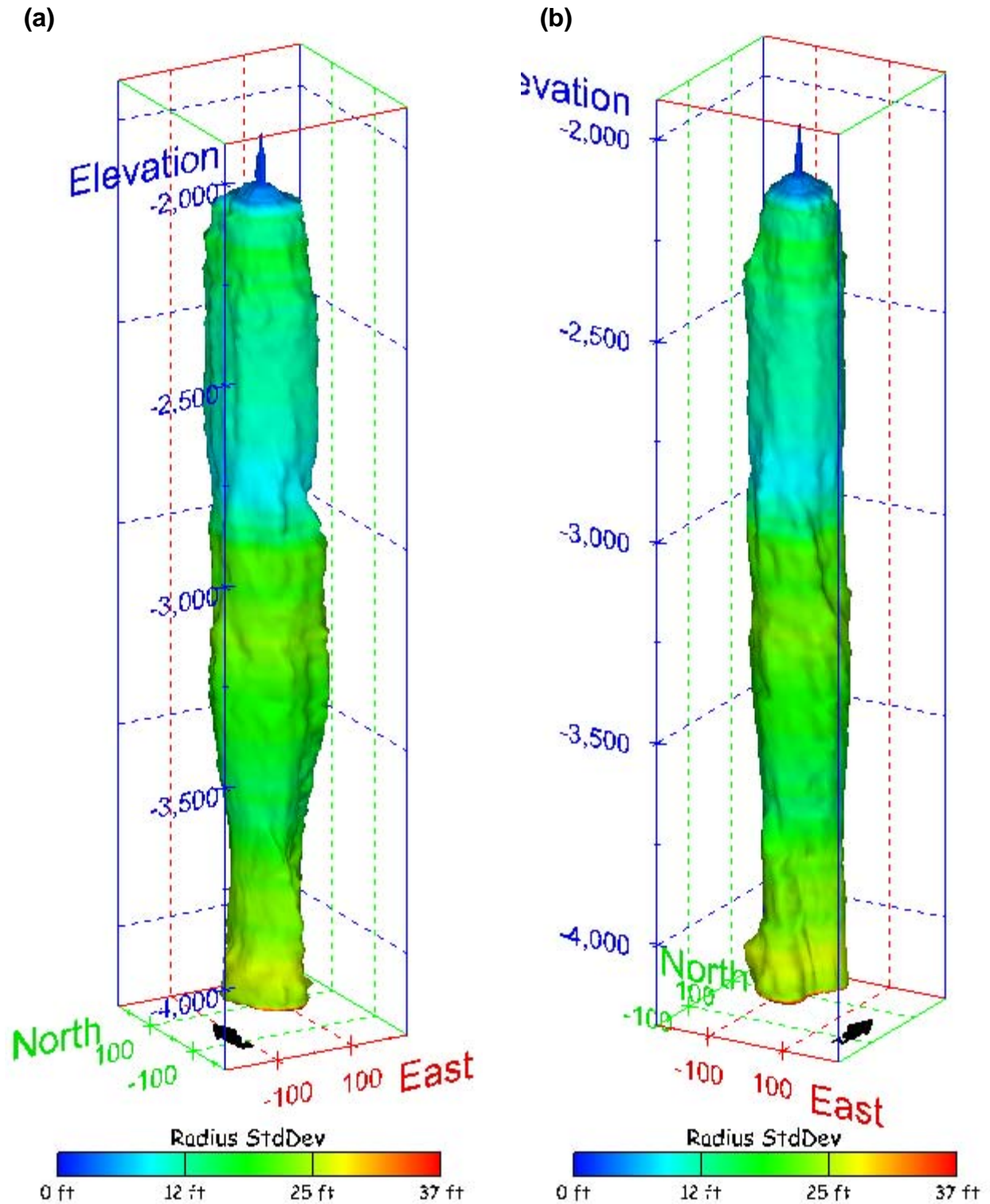
Figure 418. Sonar images of cavern BM-111, showing the geometry of the cavern colored by radius standard deviation. View from (a) azimuth 210°, elevation 20°; (b) azimuth 150°, elevation 20°.
