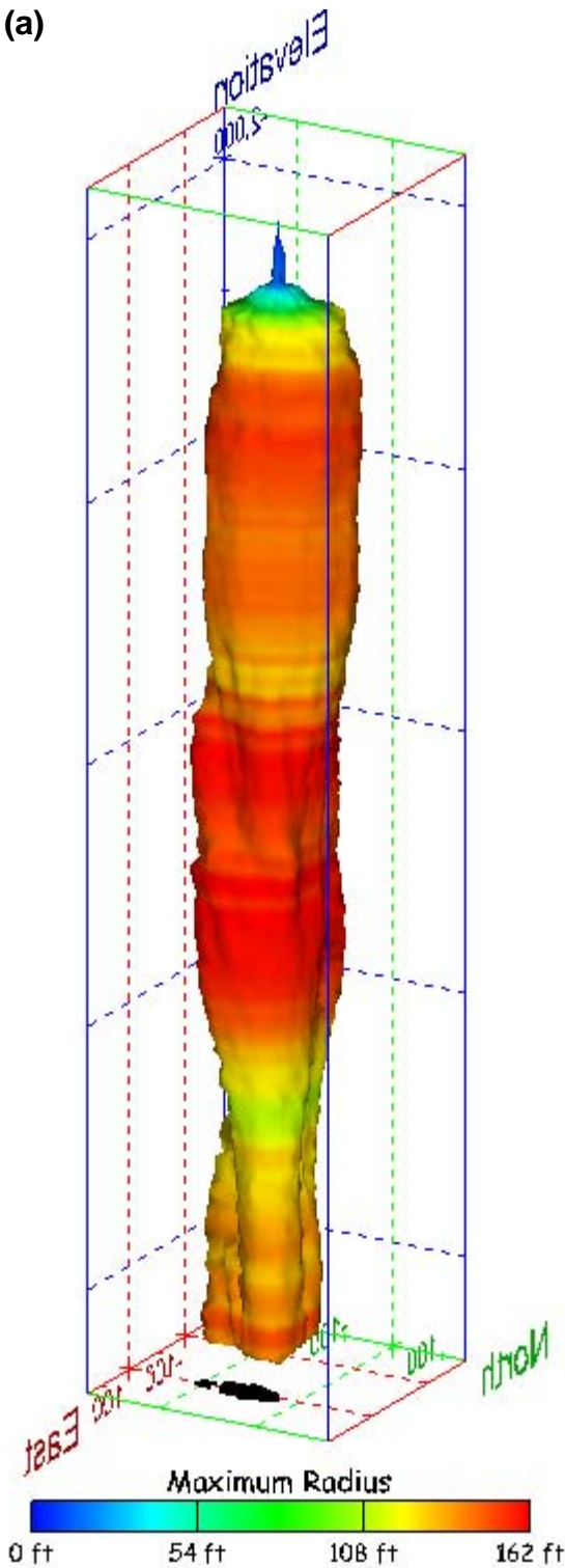
Figure 417. Sonar images of cavern BM-111, showing the geometry of the cavern colored by maximum radius. View from (a) azimuth 60°, elevation 20°; (b) azimuth 300°, elevation 20°.
