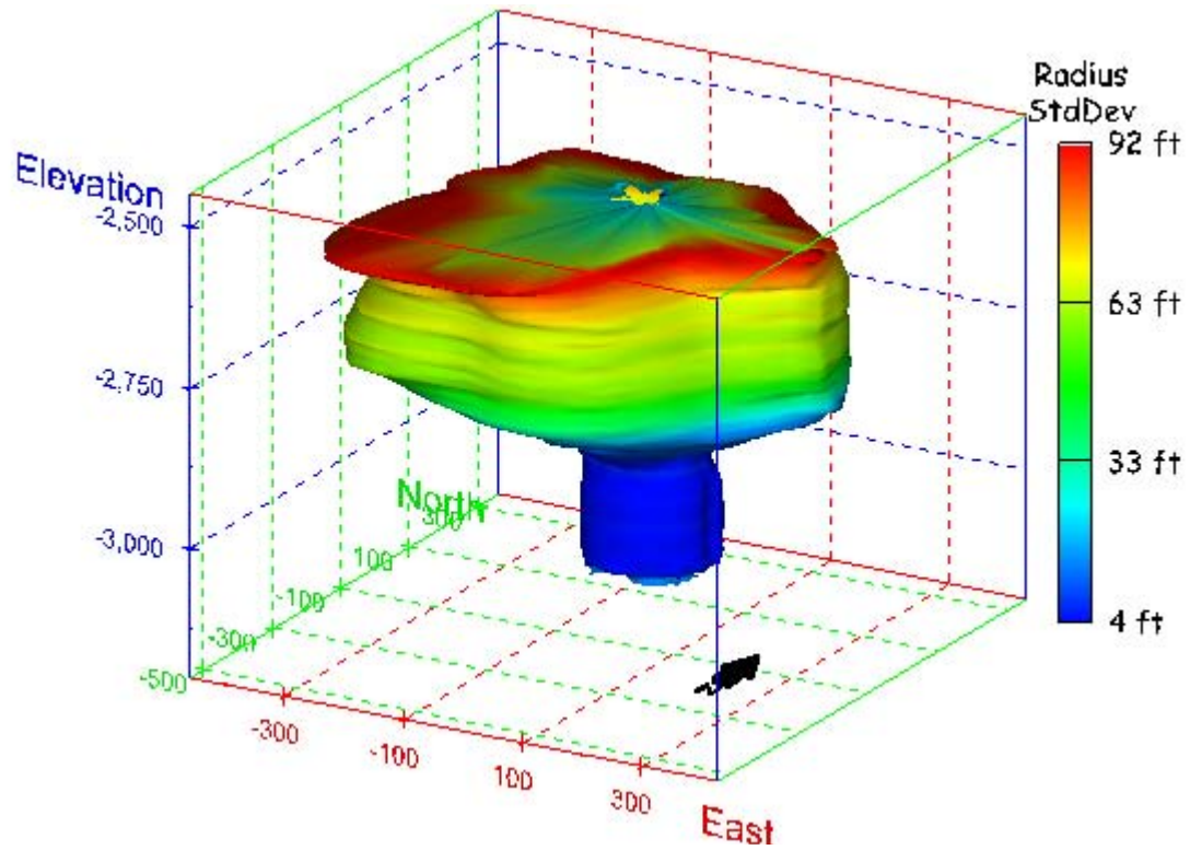
Figure 106. Sonar images of cavern BM-4, showing the geometry of the cavern colored by radius standard deviation. View from (a) azimuth 210°, elevation 20°; (b) azimuth 150°, elevation 20°.
