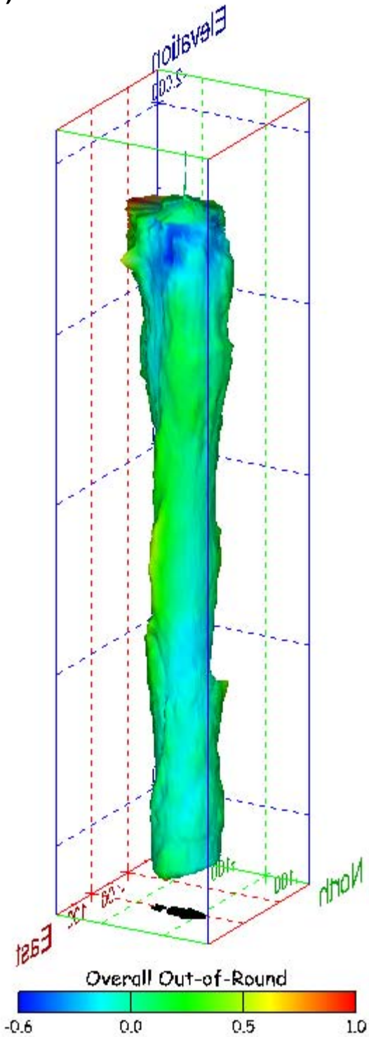
Figure 529. Sonar images of cavern BM-115, showing the geometry of the cavern colored by overall out-of-round ratio. View from (a) azimuth 60°, elevation 20°; (b) azimuth 300°, elevation 20°.
