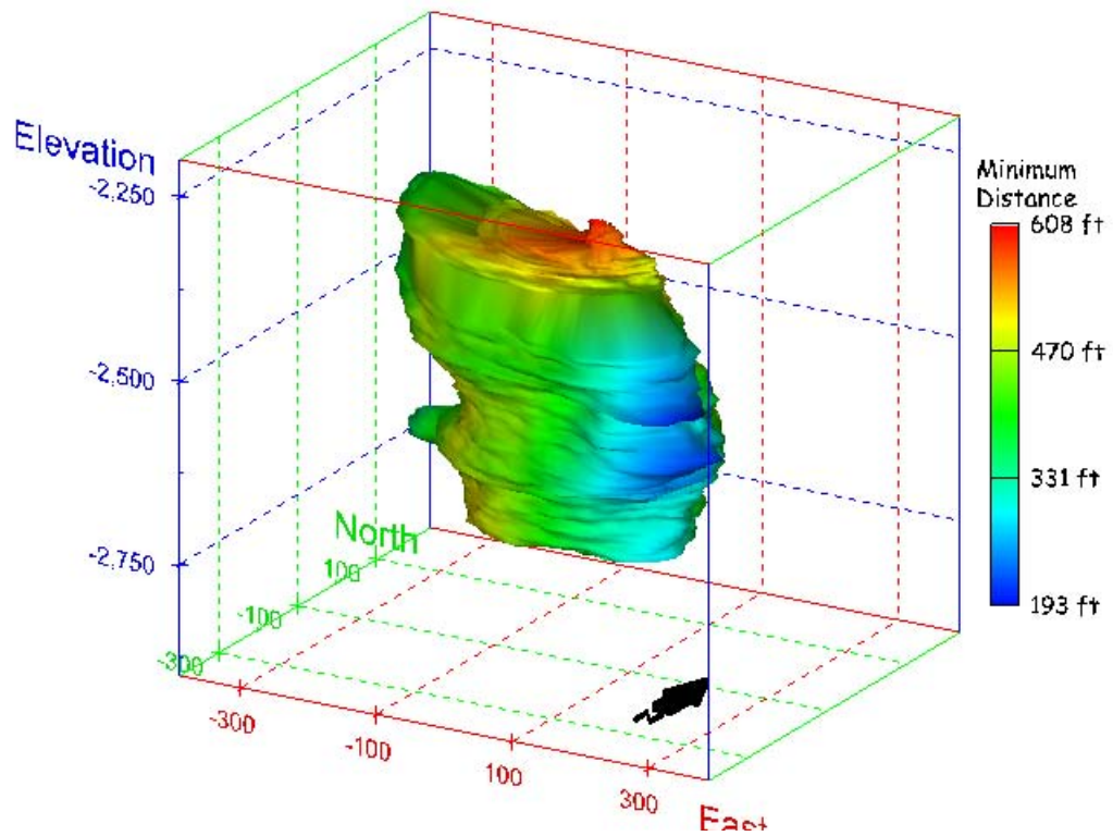
Figure 36. Sonar images of cavern BM-1, showing the geometry of the cavern colored by the minimum distance to the nearest neighboring cavern. View from (a) azimuth 210°, elevation 20°; (b) azimuth 150°, elevation 20°.
