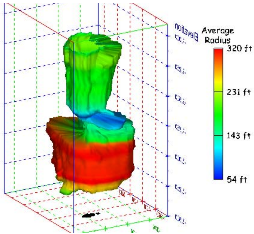
Figure 127. Sonar images of cavern BM-5, showing the geometry of the cavern colored by average radius. View from (a) azimuth 60°, elevation 20°; (b) azimuth 300°, elevation 20°.
