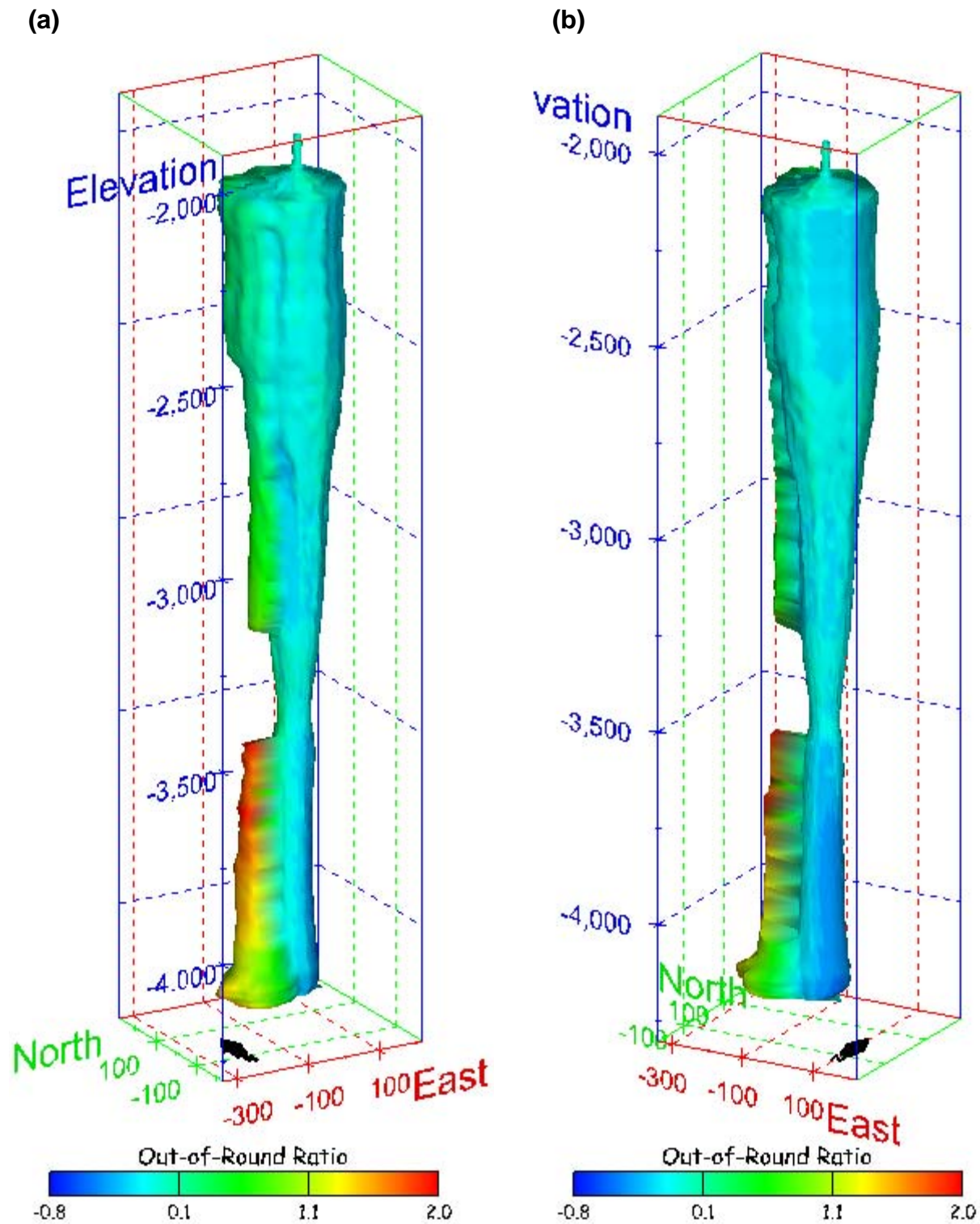
Figure 266. Sonar images of cavern BM-105, showing the geometry of the cavern colored by out-of-round ratio. View from (a) azimuth 210°, elevation 20°; (b) azimuth 150°, elevation 20°.
