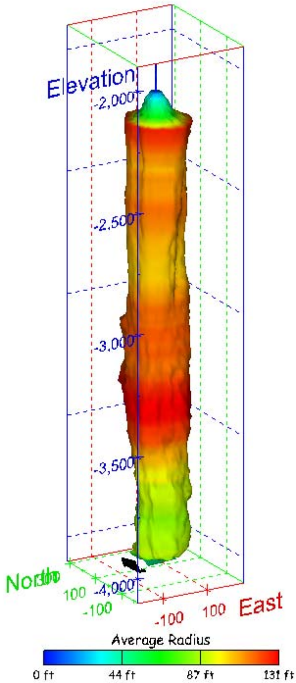
Figure 204. Sonar images of cavern BM-103, showing the geometry of the cavern colored by average radius. View from (a) azimuth 210°, elevation 20°; (b) azimuth 150°, elevation 20°.
