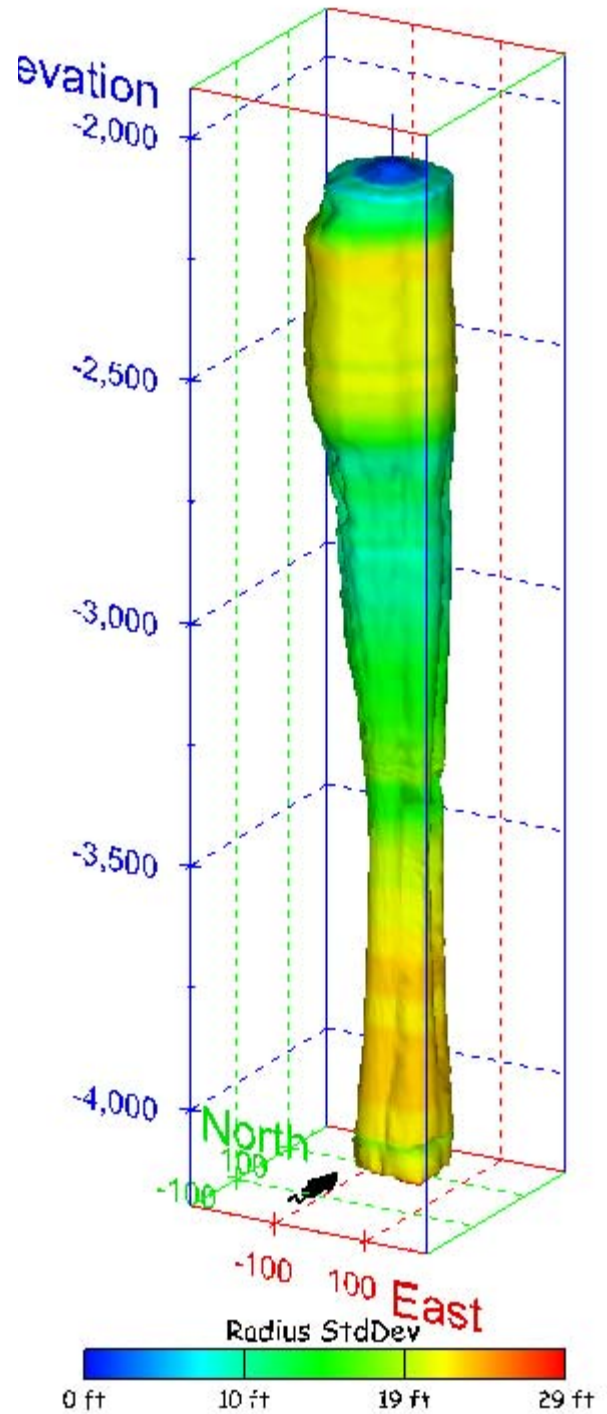
Figure 236. Sonar images of cavern BM-104, showing the geometry of the cavern colored by radius standard deviation. View from (a) azimuth 210°, elevation 20°; (b) azimuth 150°, elevation 20°.
