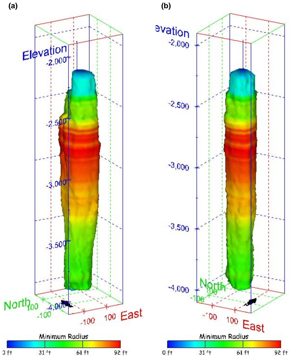
Figure 310. Sonar images of cavern BM-107, showing the geometry of the cavern colored by minimum radius. View from (a) azimuth 210°, elevation 20°; (b) azimuth 150°, elevation 20°.
