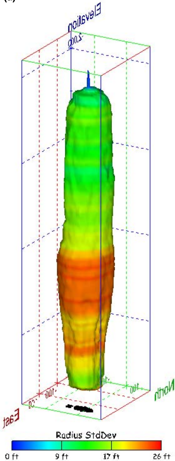
Figure 289. Sonar images of cavern BM-106, showing the geometry of the cavern colored by radius standard deviation. View from (a) azimuth 60°, elevation 20°; (b) azimuth 300°, elevation 20°.
