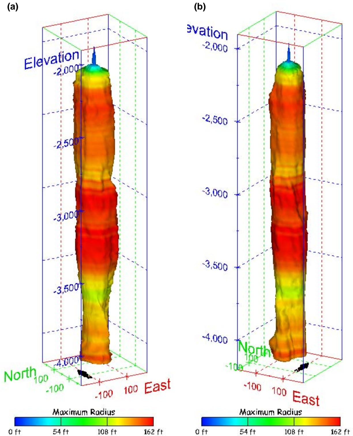
Figure 416. Sonar images of cavern BM-111, showing the geometry of the cavern colored by maximum radius. View from (a) azimuth 210°, elevation 20°; (b) azimuth 150°, elevation 20°.
