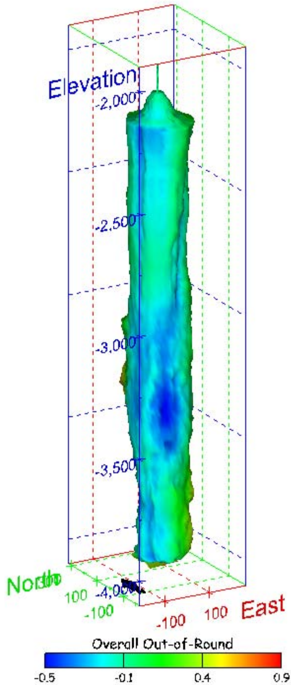
Figure 216. Sonar images of cavern BM-103, showing the geometry of the cavern colored by overall out-of-round ratio. View from (a) azimuth 210°, elevation 20°; (b) azimuth 150°, elevation 20°.
