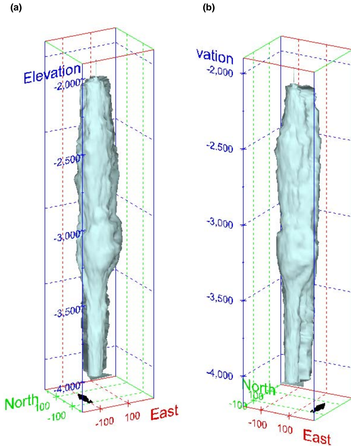
Figure 380. Sonar images of cavern BM-110, showing the basic geometric shape of the cavern. View from (a) azimuth 210°, elevation 20°; (b) azimuth 150°, elevation 20°.
