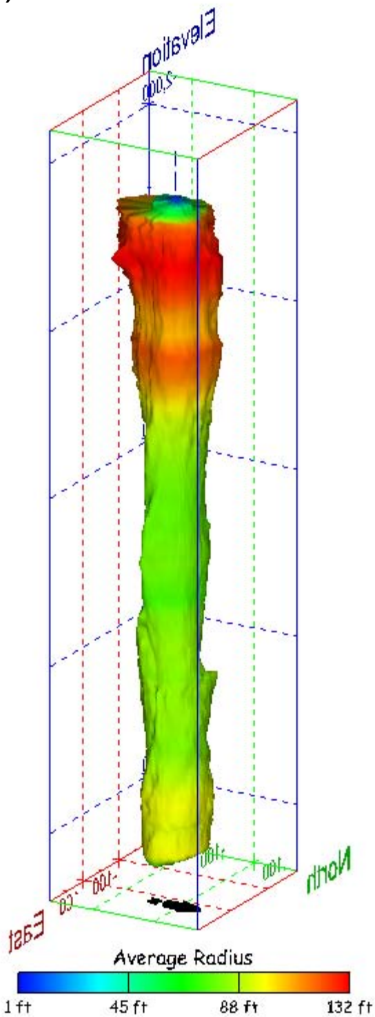
Figure 517. Sonar images of cavern BM-115, showing the geometry of the cavern colored by average radius. View from (a) azimuth 60°, elevation 20°; (b) azimuth 300°, elevation 20°.
