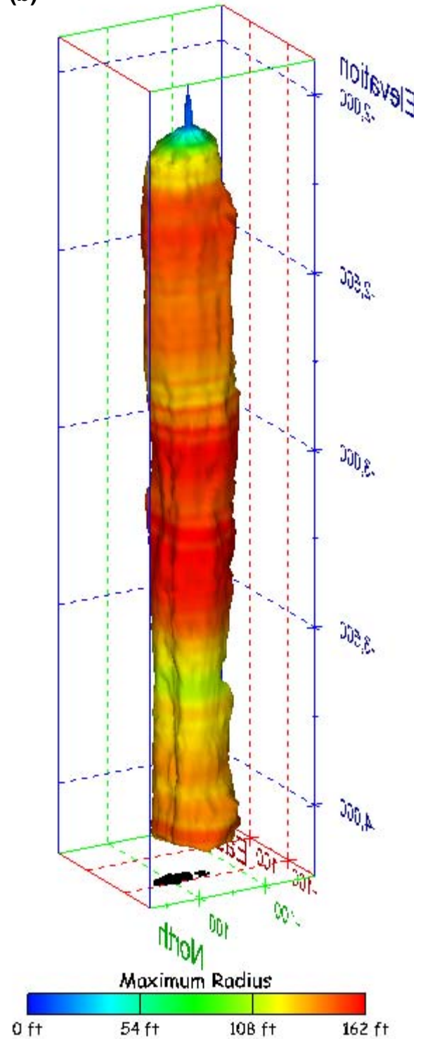
Figure 417. Sonar images of cavern BM-111, showing the geometry of the cavern colored by maximum radius. View from (a) azimuth 60°, elevation 20°; (b) azimuth 300°, elevation 20°.
