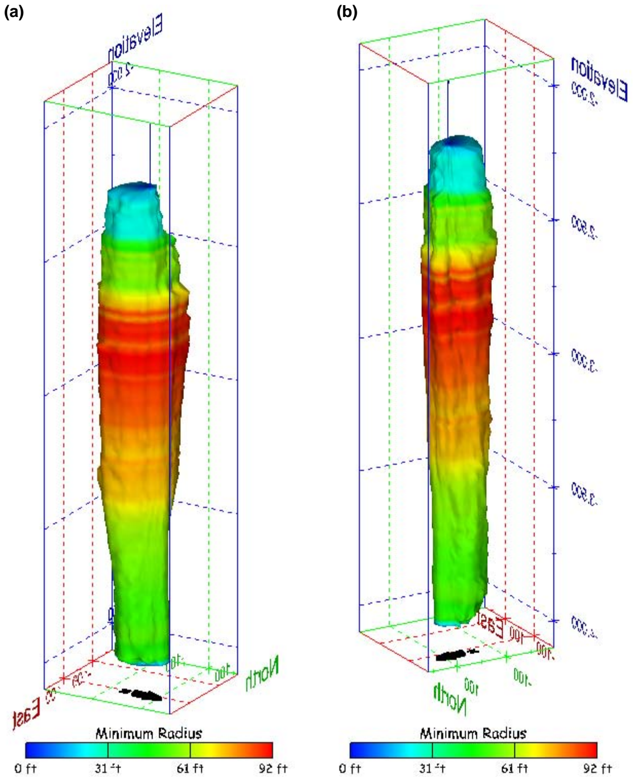
Figure 311. Sonar images of cavern BM-107, showing the geometry of the cavern colored by minimum radius. View from (a) azimuth 60°, elevation 20°; (b) azimuth 300°, elevation 20°.
