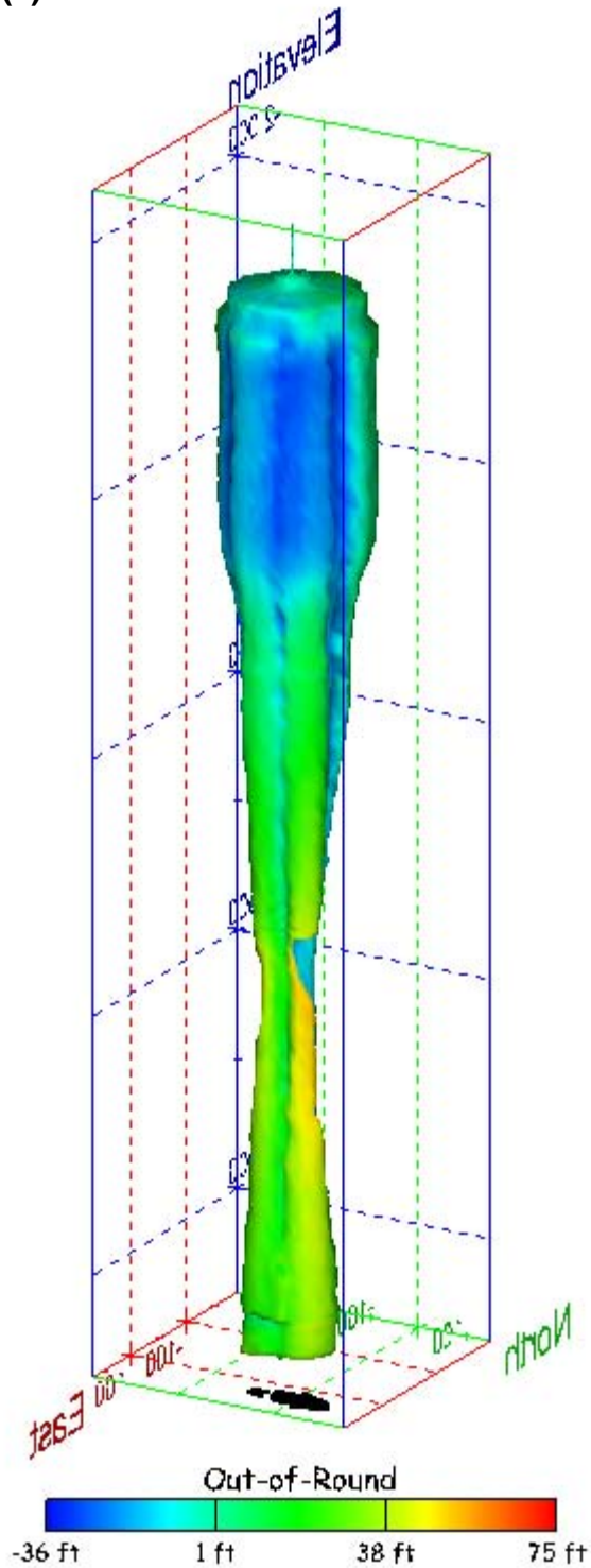
Figure 239. Sonar images of cavern BM-104, showing the geometry of the cavern colored by out-of-round distance. View from (a) azimuth 60°, elevation 20°; (b) azimuth 300°, elevation 20°.
