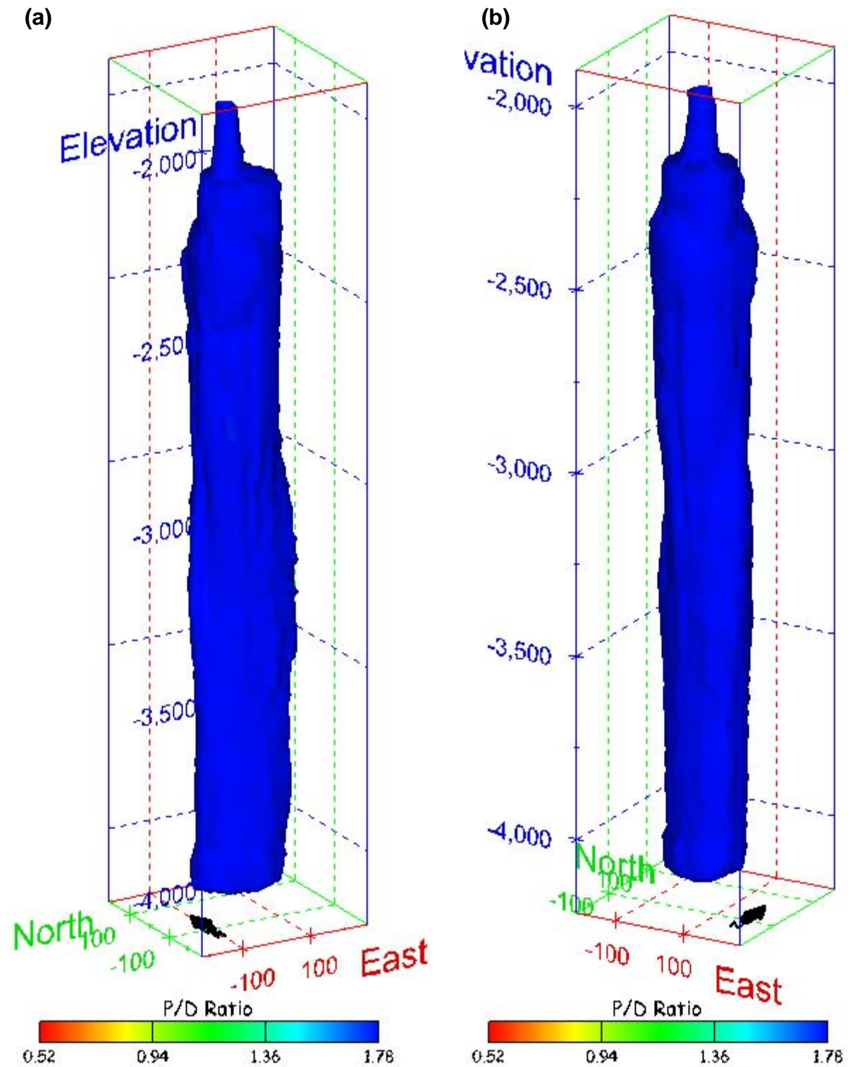
Figure 168. Sonar images of cavern BM-101, showing the geometry of the cavern colored by three-dimensional pillar-to-diameter ratio. View from (a) azimuth 210°, elevation 20°; (b) azimuth 150°, elevation 20°.
