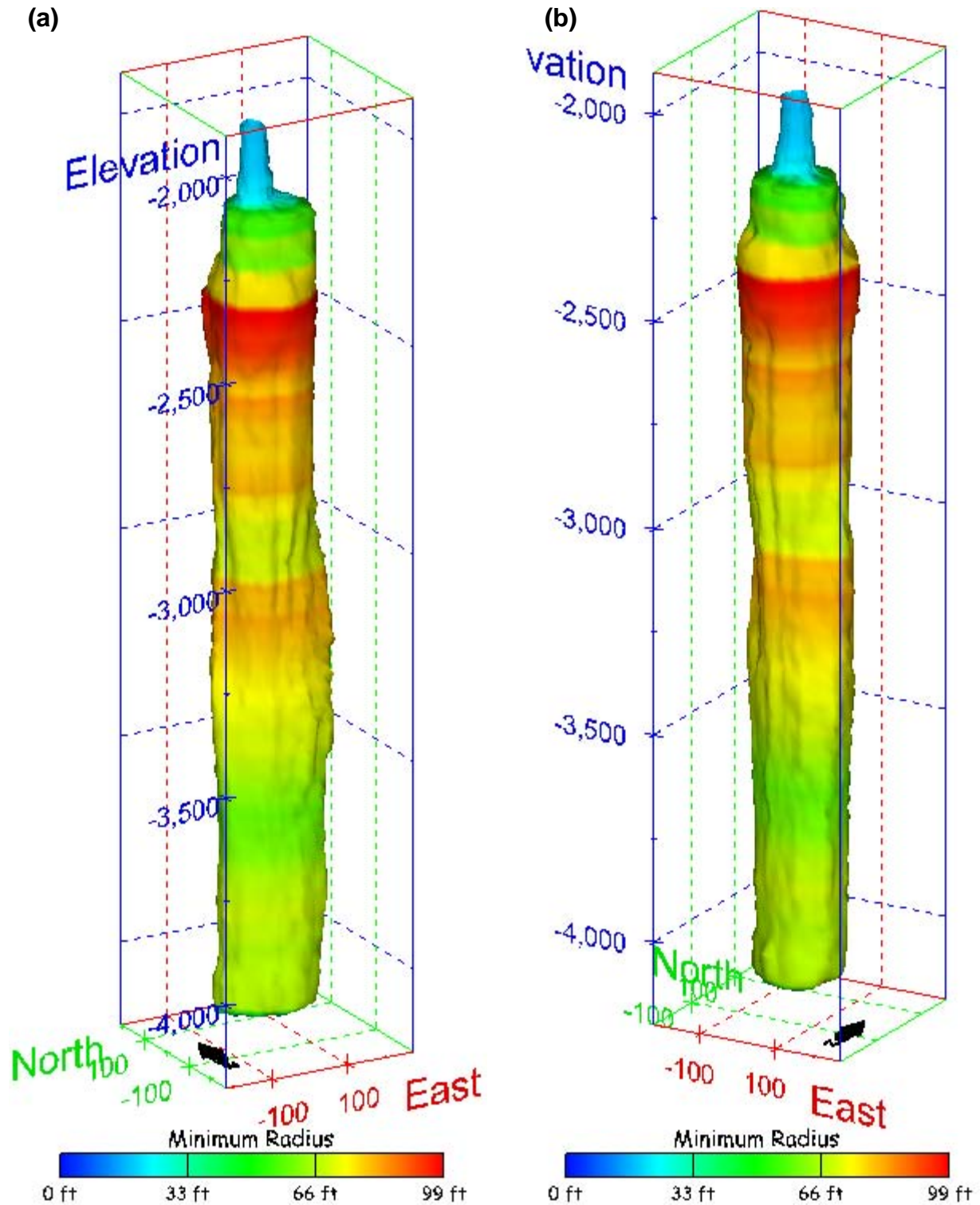
Figure 154. Sonar images of cavern BM-101, showing the geometry of the cavern colored by minimum radius. View from (a) azimuth 210°, elevation 20°; (b) azimuth 150°, elevation 20°.
