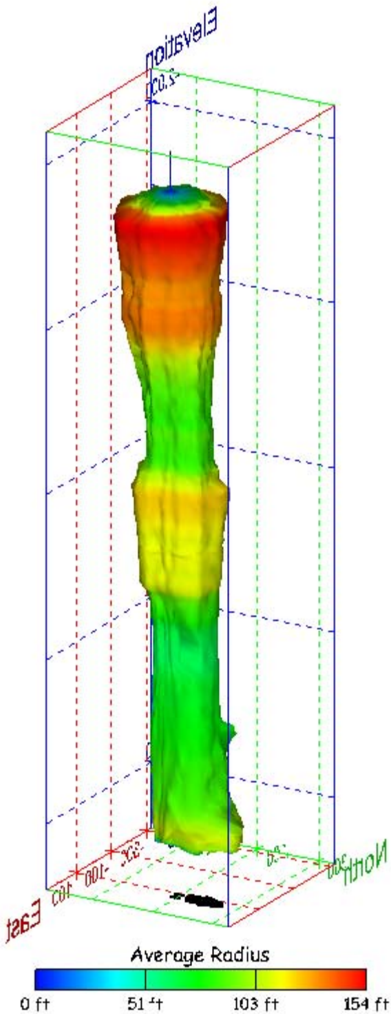
Figure 361. Sonar images of cavern BM-109, showing the geometry of the cavern colored by average radius. View from (a) azimuth 60°, elevation 20°; (b) azimuth 300°, elevation 20°.
