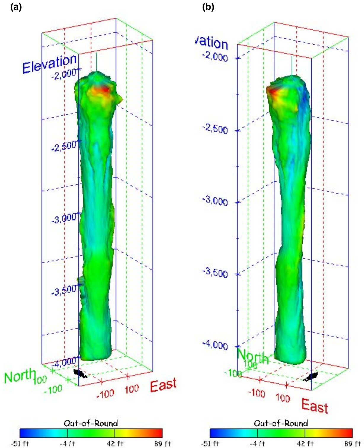
Figure 524. Sonar images of cavern BM-115, showing the geometry of the cavern colored by out-of-round distance. View from (a) azimuth 210°, elevation 20°; (b) azimuth 150°, elevation 20°.
