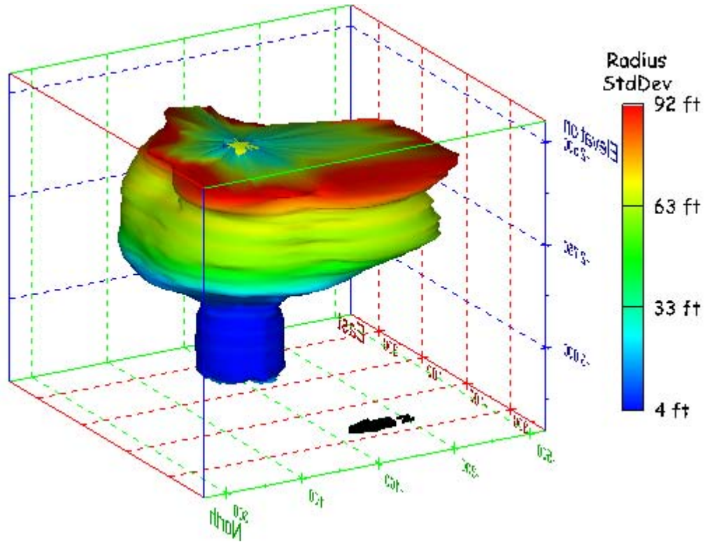
Figure 107. Sonar images of cavern BM-4, showing the geometry of the cavern colored by radius standard deviation. View from (a) azimuth 60°, elevation 20°; (b) azimuth 300°, elevation 20°.
