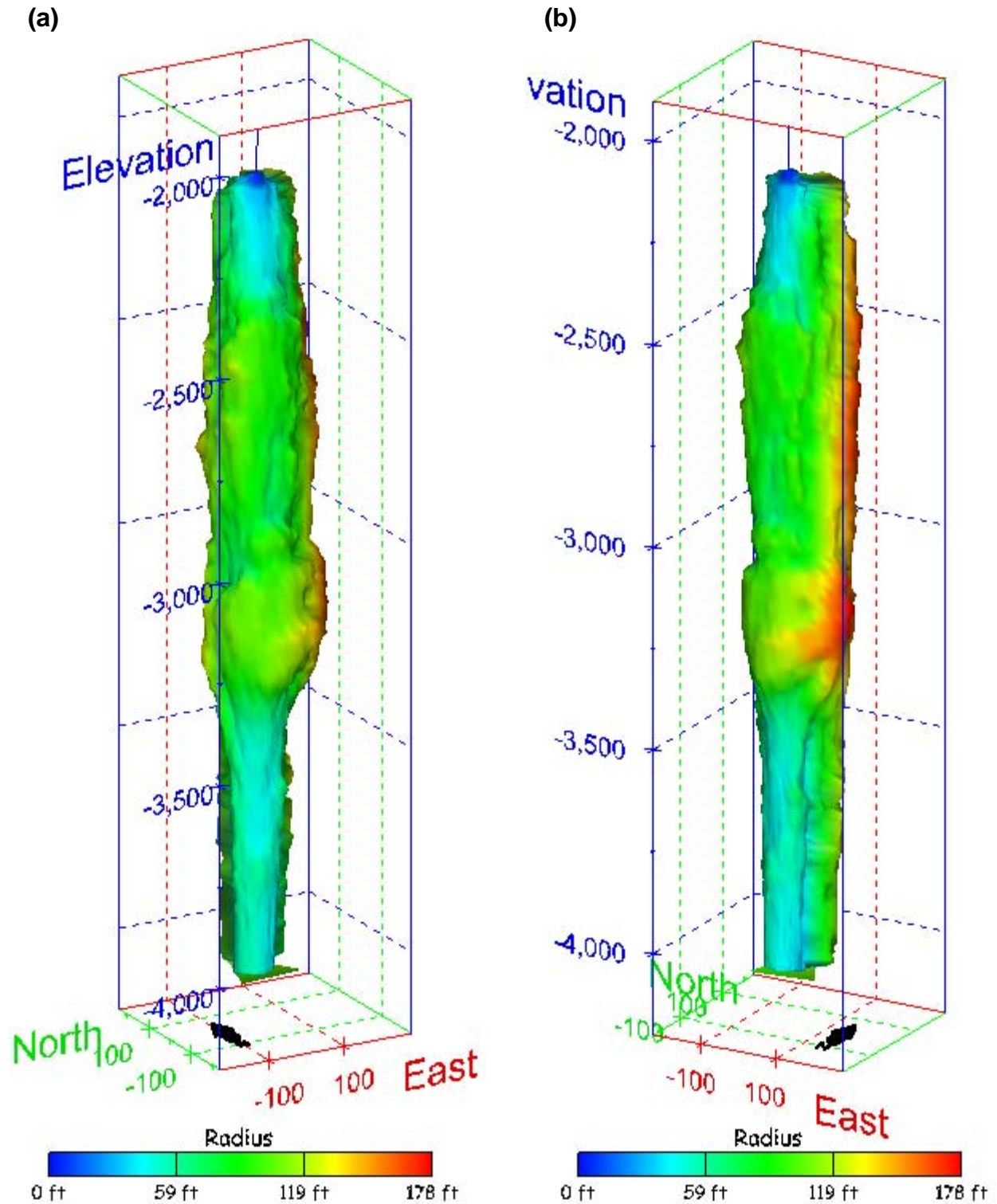
Figure 382. Sonar images of cavern BM-110, showing the geometry of the cavern colored by measured radius. View from (a) azimuth 210°, elevation 20°; (b) azimuth 150°, elevation 20°.
