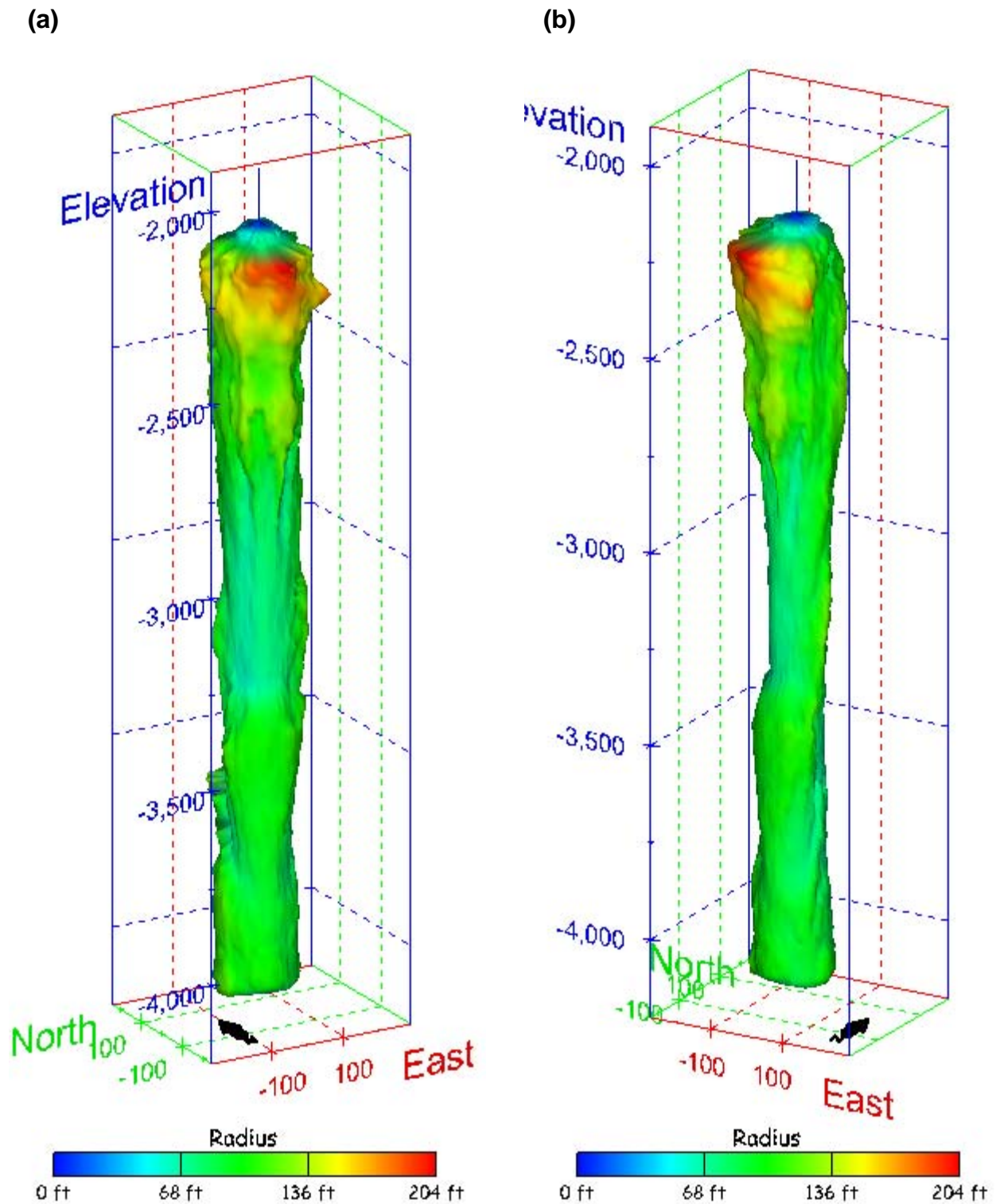
Figure 512. Sonar images of cavern BM-115, showing the geometry of the cavern colored by measured radius. View from (a) azimuth 210°, elevation 20°; (b) azimuth 150°, elevation 20°.
