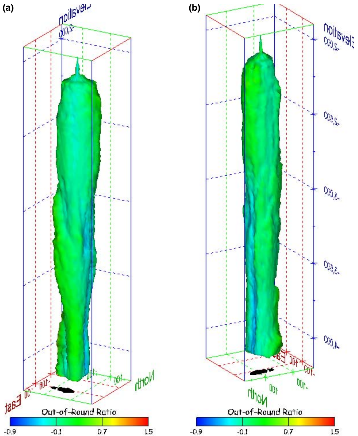
Figure 423. Sonar images of cavern BM-111, showing the geometry of the cavern colored by out-of-round ratio. View from (a) azimuth 60°, elevation 20°; (b) azimuth 300°, elevation 20°.
