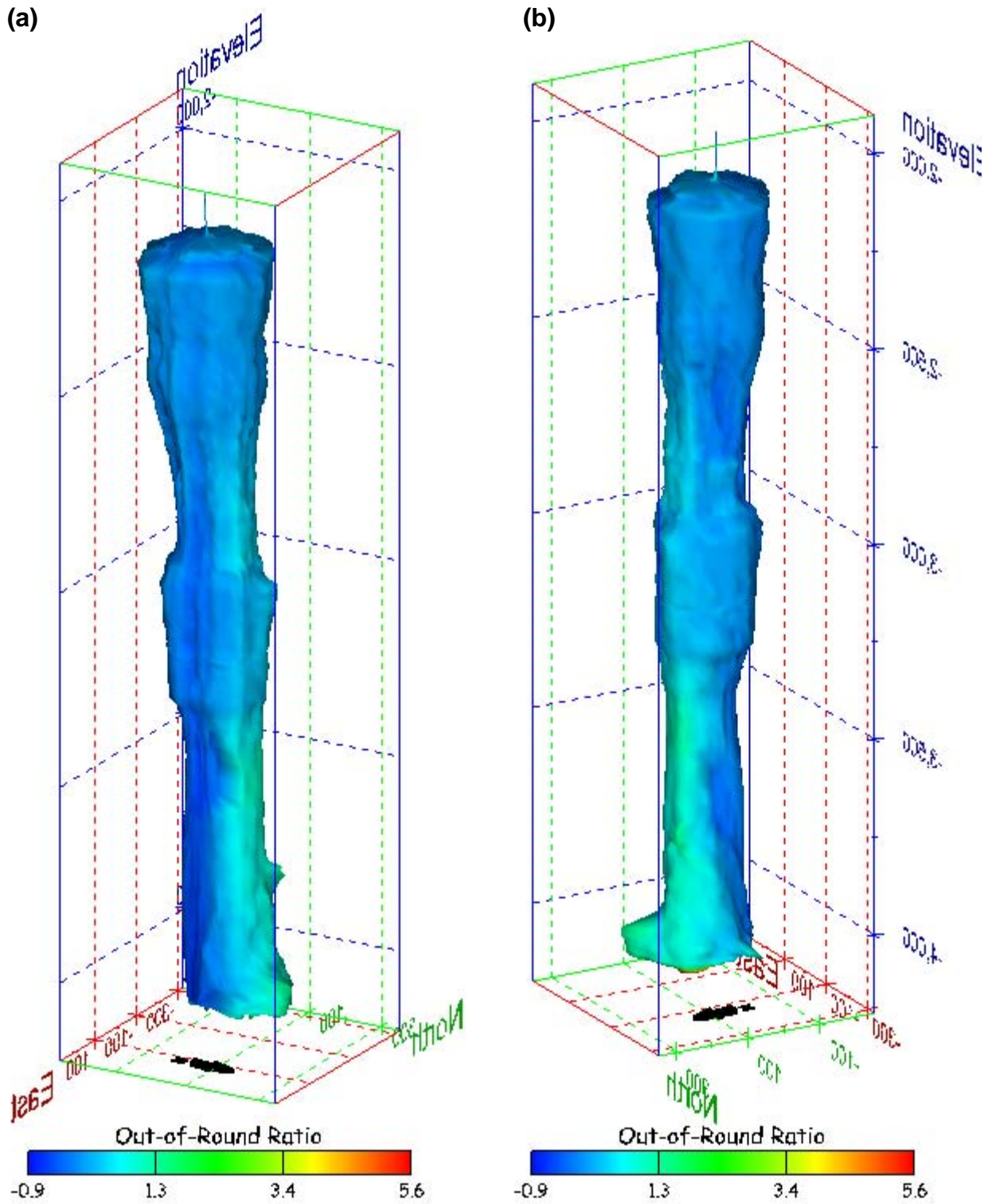
Figure 371. Sonar images of cavern BM-109, showing the geometry of the cavern colored by out-of-round ratio. View from (a) azimuth 60°, elevation 20°; (b) azimuth 300°, elevation 20°.
