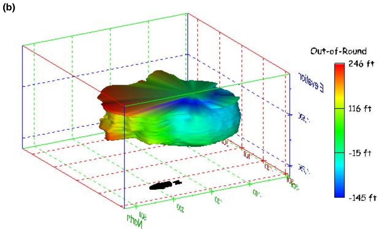
Figure 57. Sonar images of cavern BM-2, showing the geometry of the cavern colored by out-of-round distance. View from (a) azimuth 60°, elevation 20°; (b) azimuth 300°, elevation 20°.
