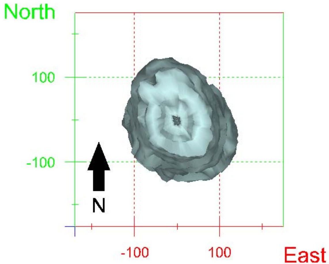
Figure 405. Map view sonar image of cavern BM-111, showing the basic geometry of the cavern. Grid squares represent 200 ft.
