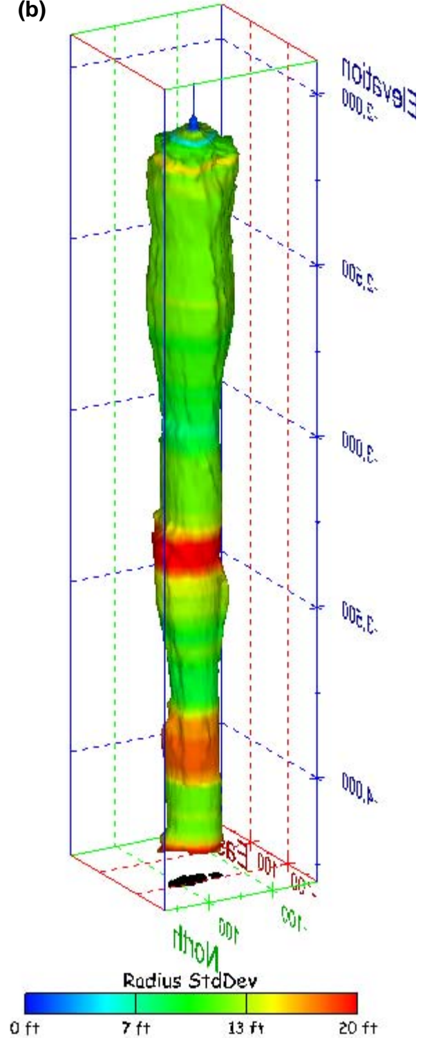
Figure 549. Sonar images of cavern BM-116, showing the geometry of the cavern colored by radius standard deviation. View from (a) azimuth 60°, elevation 20°; (b) azimuth 300°, elevation 20°.
