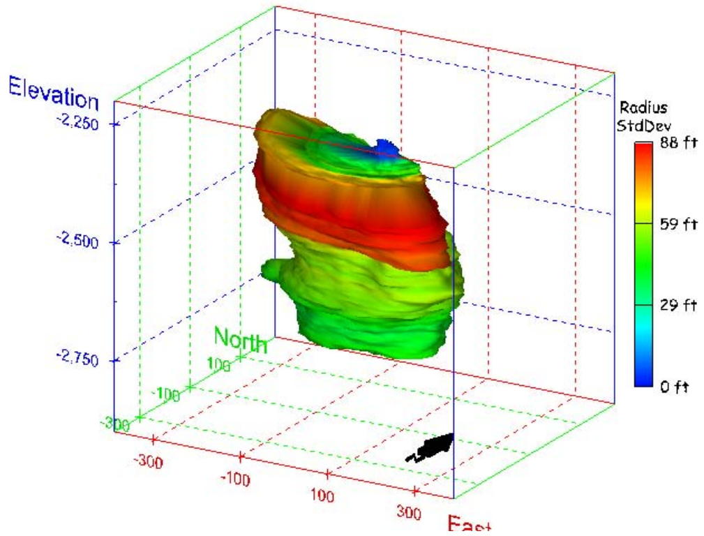
Figure 28. Sonar images of cavern BM-1, showing the geometry of the cavern colored by radius standard deviation. View from (a) azimuth 210°, elevation 20°; (b) azimuth 150°, elevation 20°.
