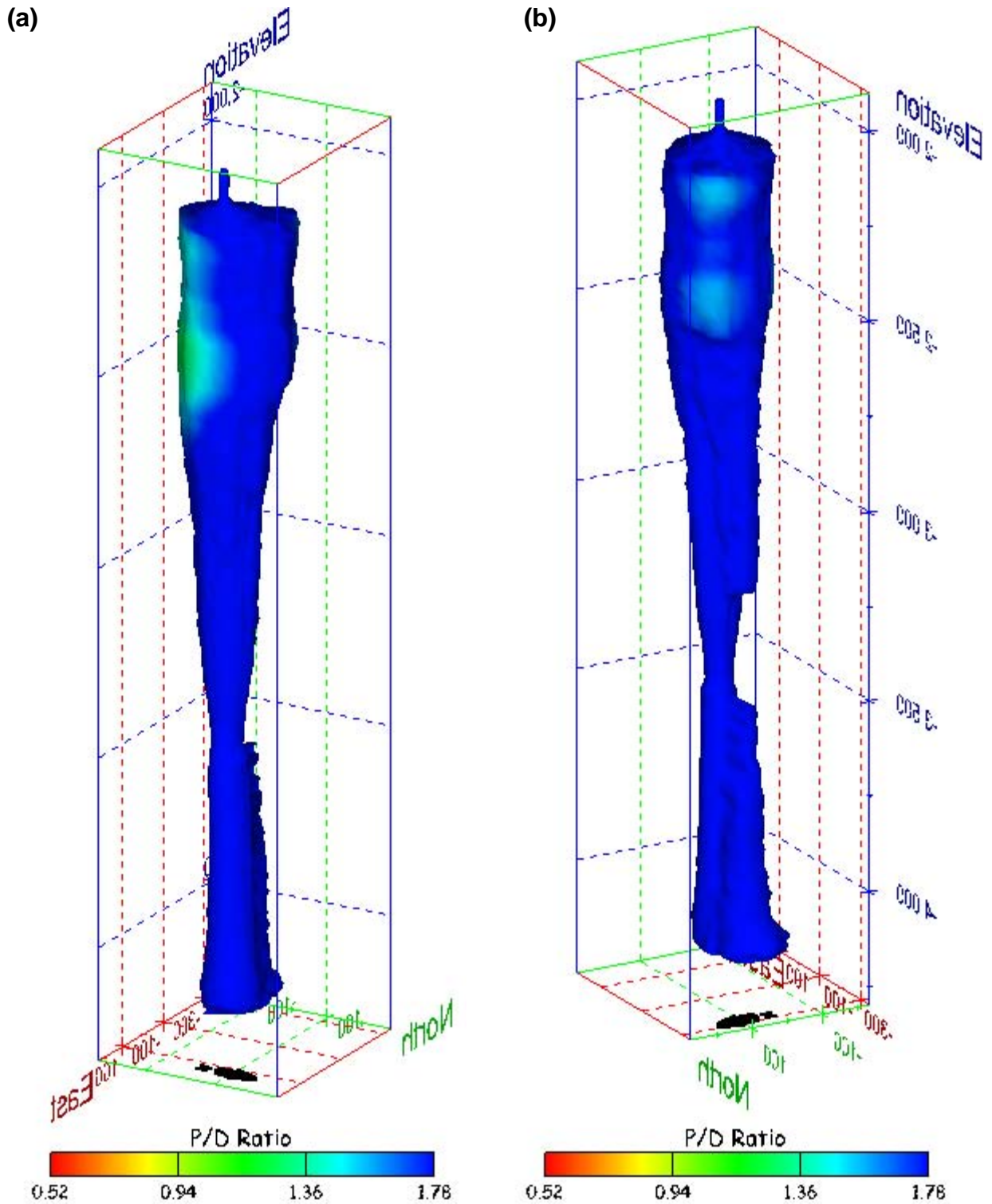
Figure 273. Sonar images of cavern BM-105, showing the geometry of the cavern colored by three-dimensional pillar-to-diameter ratio. View from (a) azimuth 60°, elevation 20°; (b) azimuth 300°, elevation 20°.
