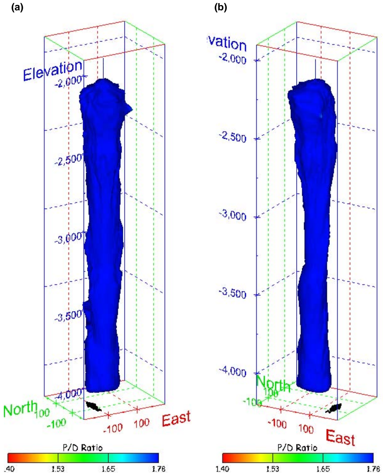
Figure 532. Sonar images of cavern BM-115, showing the geometry of the cavern colored by three-dimensional pillar-to-diameter ratio. View from (a) azimuth 210°, elevation 20°; (b) azimuth 150°, elevation 20°.
