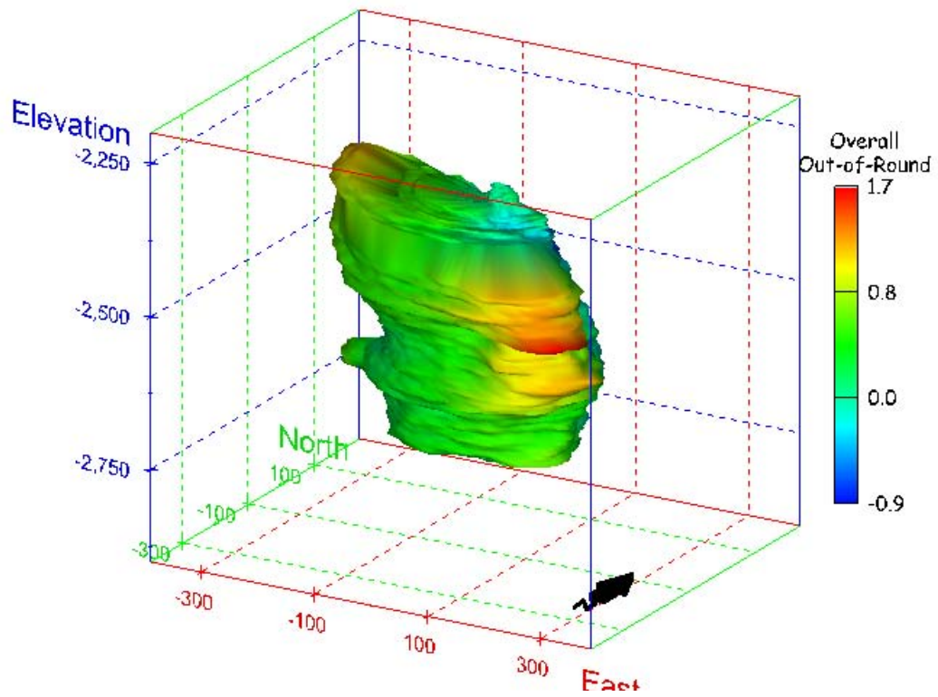
Figure 34. Sonar images of cavern BM-1, showing the geometry of the cavern colored by overall out-of-round ratio. View from (a) azimuth 210°, elevation 20°; (b) azimuth 150°, elevation 20°.
