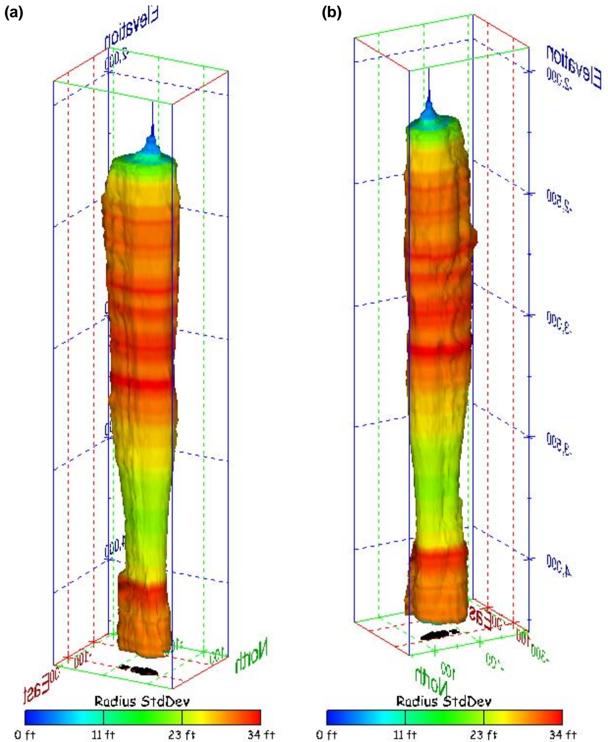
Figure 185. Sonar images of cavern BM-102, showing the geometry of the cavern colored by radius standard deviation. View from (a) azimuth 60°, elevation 20°; (b) azimuth 300°, elevation 20°.
