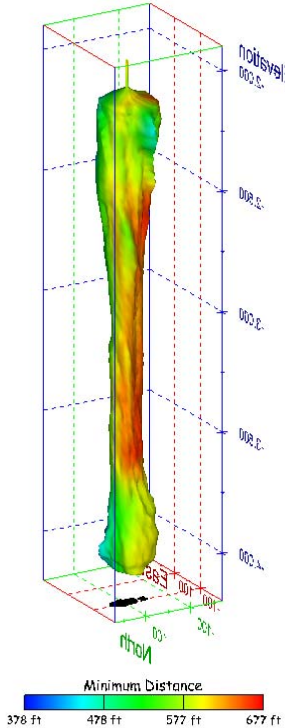
Figure 505. Sonar images of cavern BM-114, showing the geometry of the cavern colored by minimum distance to the nearest neighboring cavern. View from (a) azimuth 60°, elevation 20°; (b) azimuth 300°, elevation 20°.
