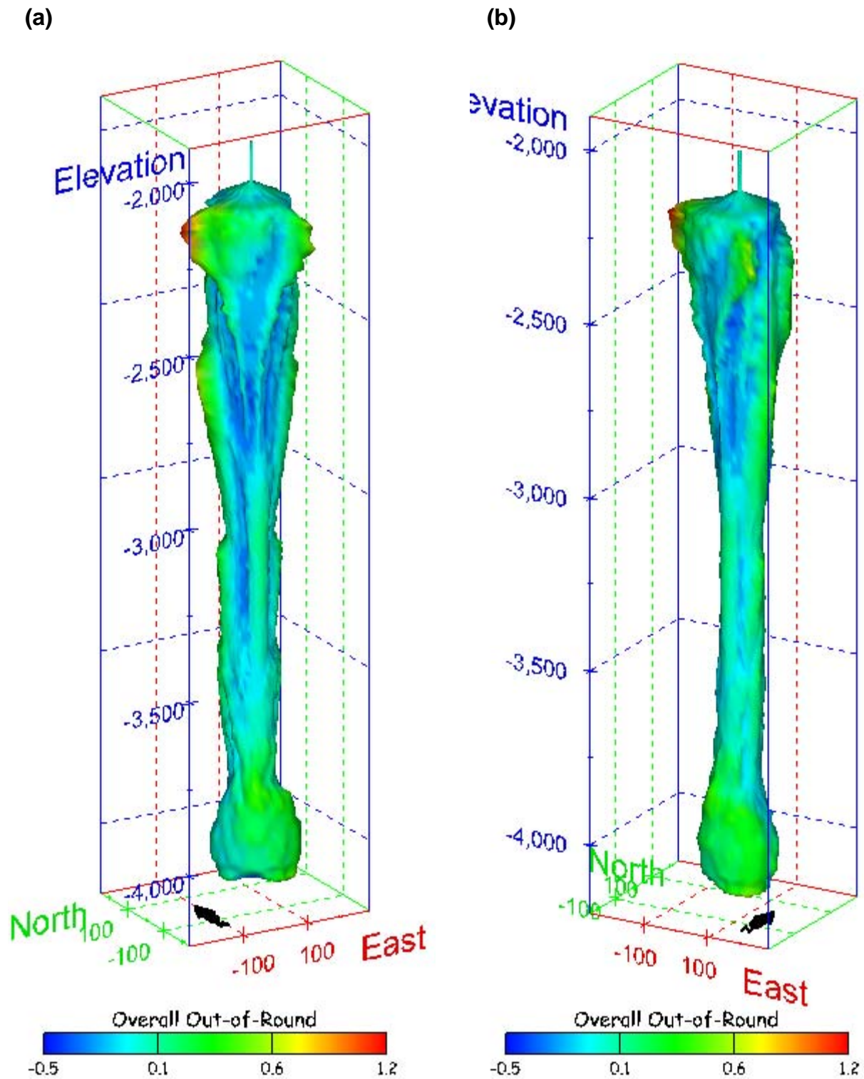
Figure 502. Sonar images of cavern BM-114, showing the geometry of the cavern colored by overall out-of-round ratio. View from (a) azimuth 210°, elevation 20°; (b) azimuth 150°, elevation 20°.
