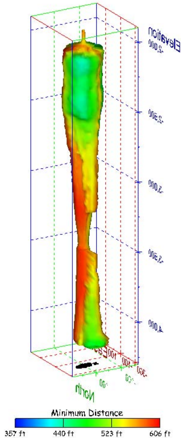
Figure 271. Sonar images of cavern BM-105, showing the geometry of the cavern colored by minimum distance to the nearest neighboring cavern. View from (a) azimuth 60°, elevation 20°; (b) azimuth 300°, elevation 20°.
