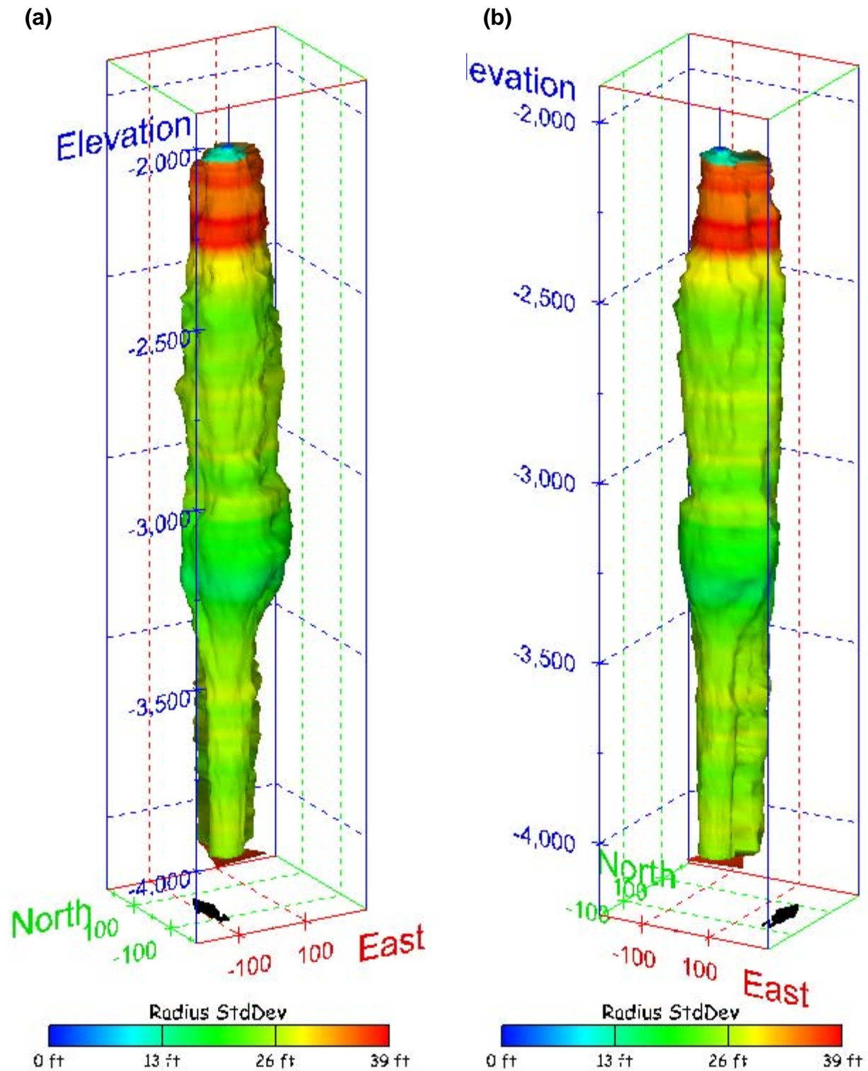
Figure 392. Sonar images of cavern BM-110, showing the geometry of the cavern colored by radius standard deviation. View from (a) azimuth 210°, elevation 20°; (b) azimuth 150°, elevation 20°.
