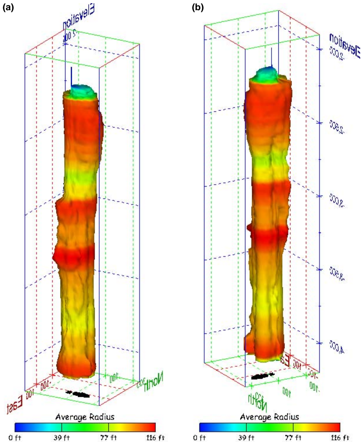
Figure 335. Sonar images of cavern BM-108, showing the geometry of the cavern colored by average radius. View from (a) azimuth 60°, elevation 20°; (b) azimuth 300°, elevation 20°.
