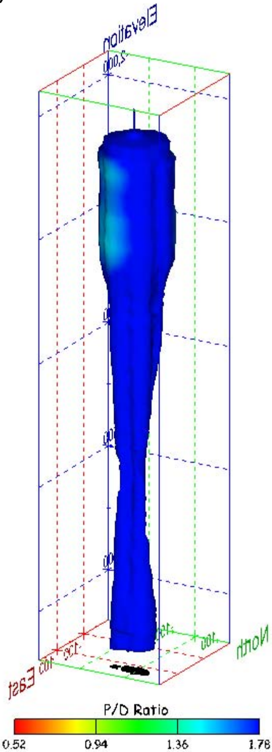
Figure 247. Sonar images of cavern BM-104, showing the geometry of the cavern colored by three-dimensional pillar-to-diameter ratio. View from (a) azimuth 60°, elevation 20°; (b) azimuth 300°, elevation 20°.
