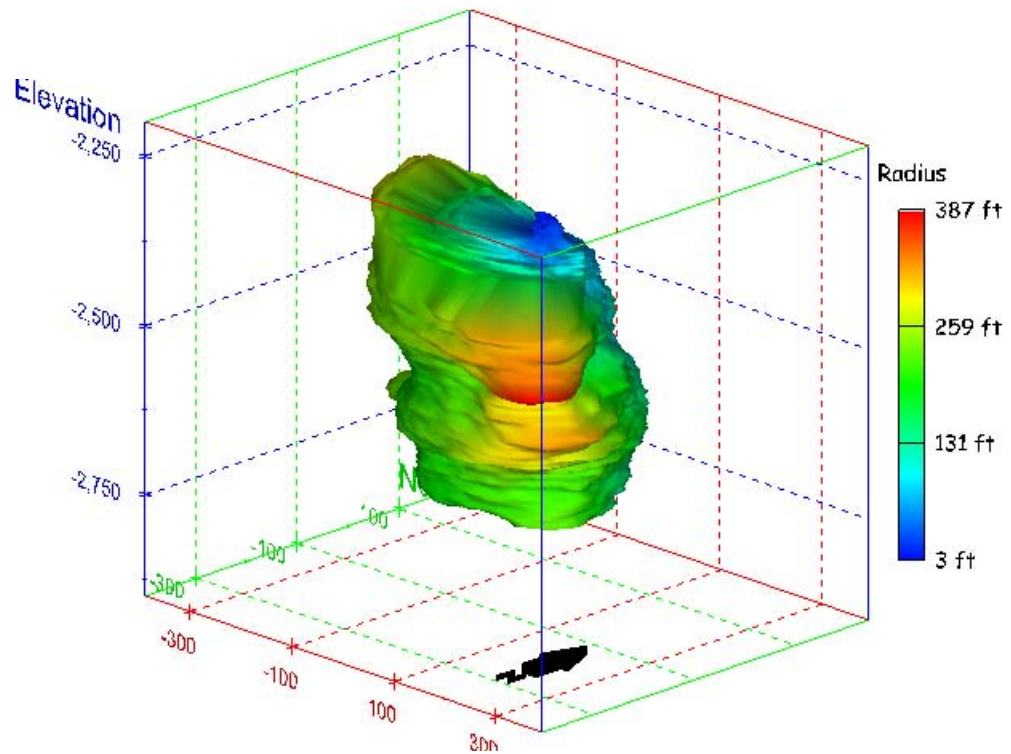
Figure 18. Sonar images of cavern BM-1, showing the geometry of the cavern colored by measured radius. View from (a) azimuth 210°, elevation 20°; (b) azimuth 150°, elevation 20°.
