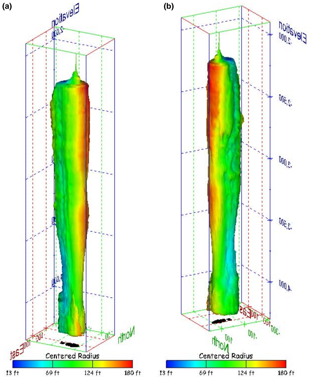
Figure 177. Sonar images of cavern BM-102, showing the geometry of the cavern colored by centered radius. View from (a) azimuth 60°, elevation 20°; (b) azimuth 300°, elevation 20°.
