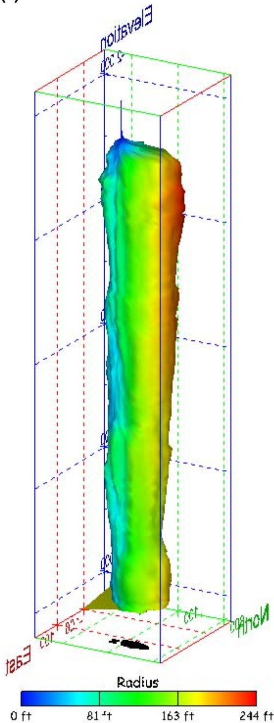
Figure 435. Sonar images of cavern BM-112, showing the geometry of the cavern colored by measured radius. View from (a) azimuth 60°, elevation 20°; (b) azimuth 300°, elevation 20°.
