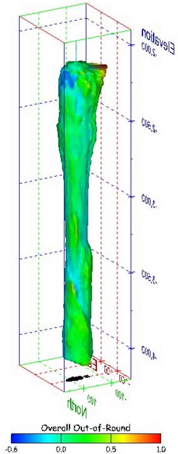
Figure 529. Sonar images of cavern BM-115, showing the geometry of the cavern colored by overall out-of-round ratio. View from (a) azimuth 60°, elevation 20°; (b) azimuth 300°, elevation 20°.
