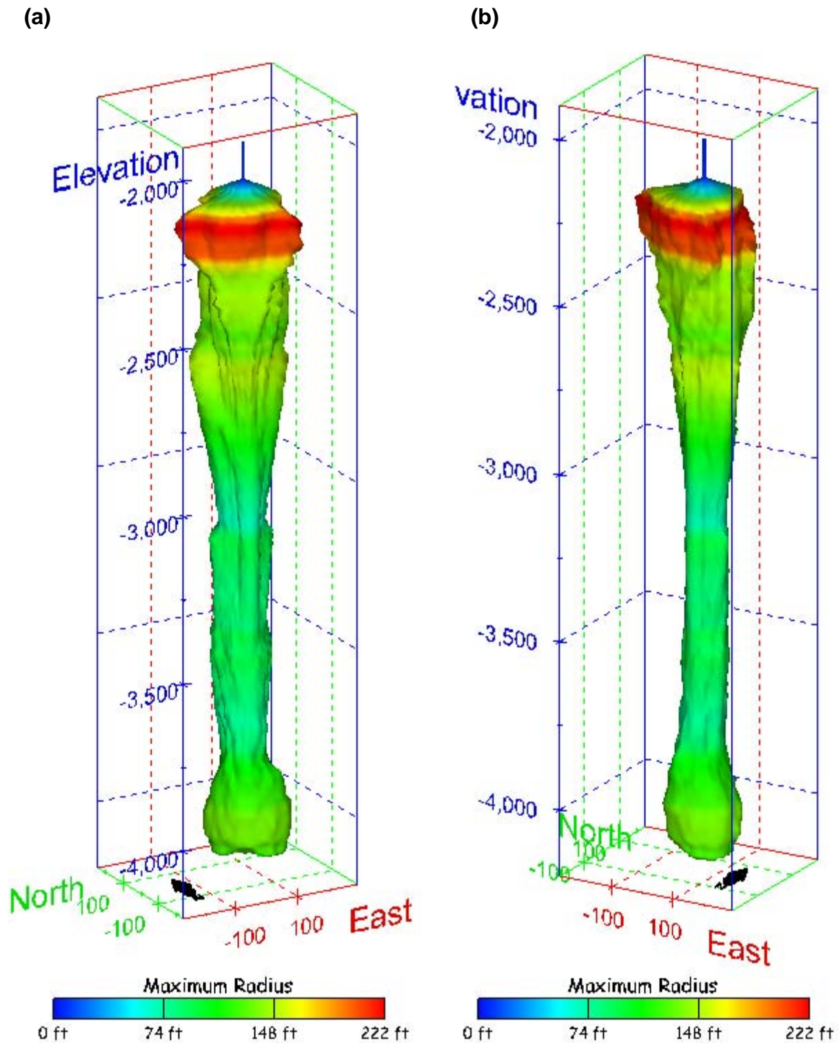
Figure 494. Sonar images of cavern BM-114, showing the geometry of the cavern colored by maximum radius. View from (a) azimuth 210°, elevation 20°; (b) azimuth 150°, elevation 20°.
