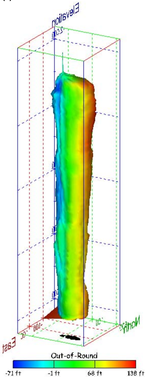
Figure 447. Sonar images of cavern BM-112, showing the geometry of the cavern colored by out-of-round distance. View from (a) azimuth 60°, elevation 20°; (b) azimuth 300°, elevation 20°.
