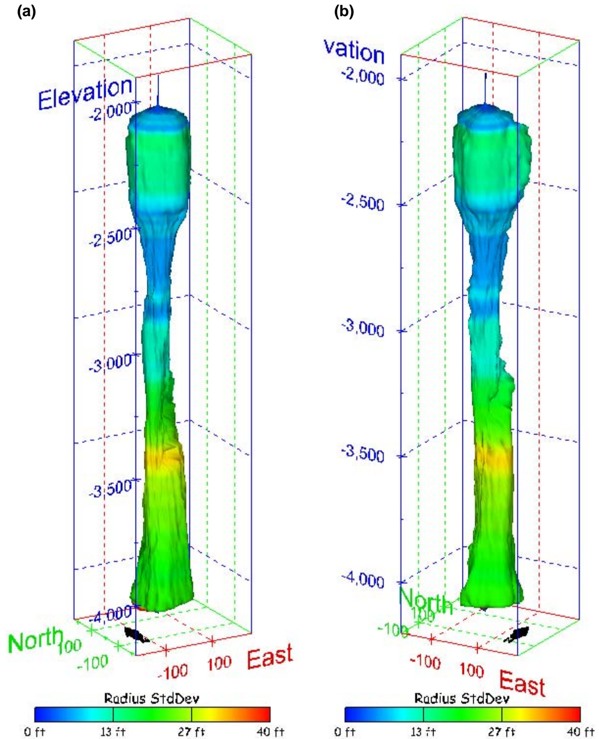
Figure 470. Sonar images of cavern BM-113, showing the geometry of the cavern colored by radius standard deviation. View from (a) azimuth 210°, elevation 20°; (b) azimuth 150°, elevation 20°.
