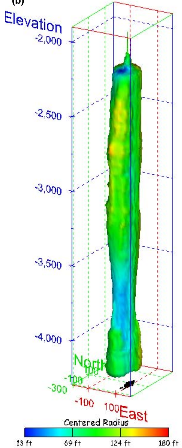
Figure 176. Sonar images of cavern BM-102, showing the geometry of the cavern colored by centered radius. View from (a) azimuth 210°, elevation 20°; (b) azimuth 150°, elevation 20°.
