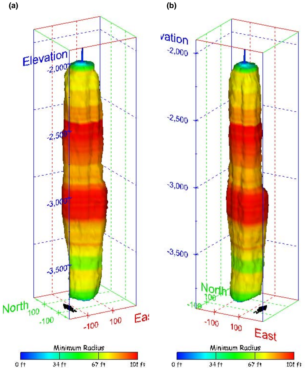
Figure 284. Sonar images of cavern BM-106, showing the geometry of the cavern colored by minimum radius. View from (a) azimuth 210°, elevation 20°; (b) azimuth 150°, elevation 20°.
