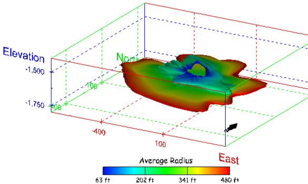
Figure 74. Sonar images of cavern BM-3, showing the geometry of the cavern colored by average radius. View from (a) azimuth 210°, elevation 20°; (b) azimuth 150°, elevation 20°.
