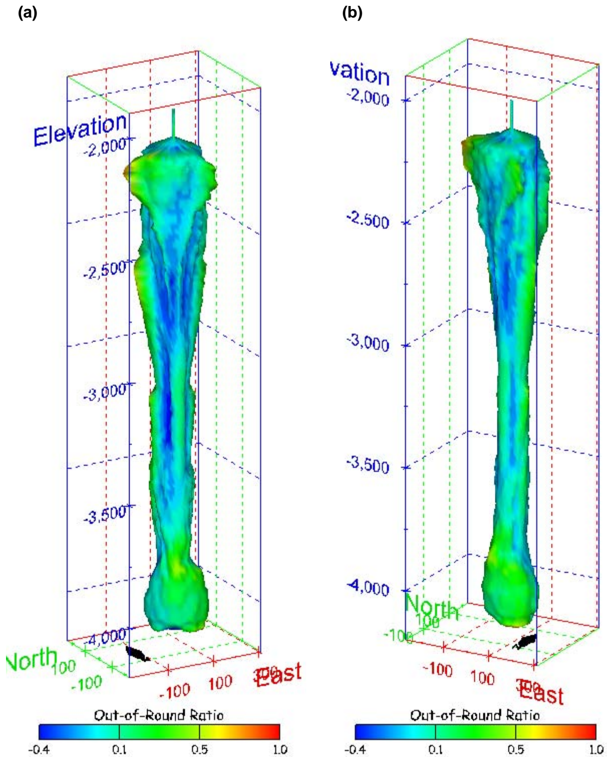
Figure 500. Sonar images of cavern BM-114, showing the geometry of the cavern colored by out-of-round ratio. View from (a) azimuth 210°, elevation 20°; (b) azimuth 150°, elevation 20°.
