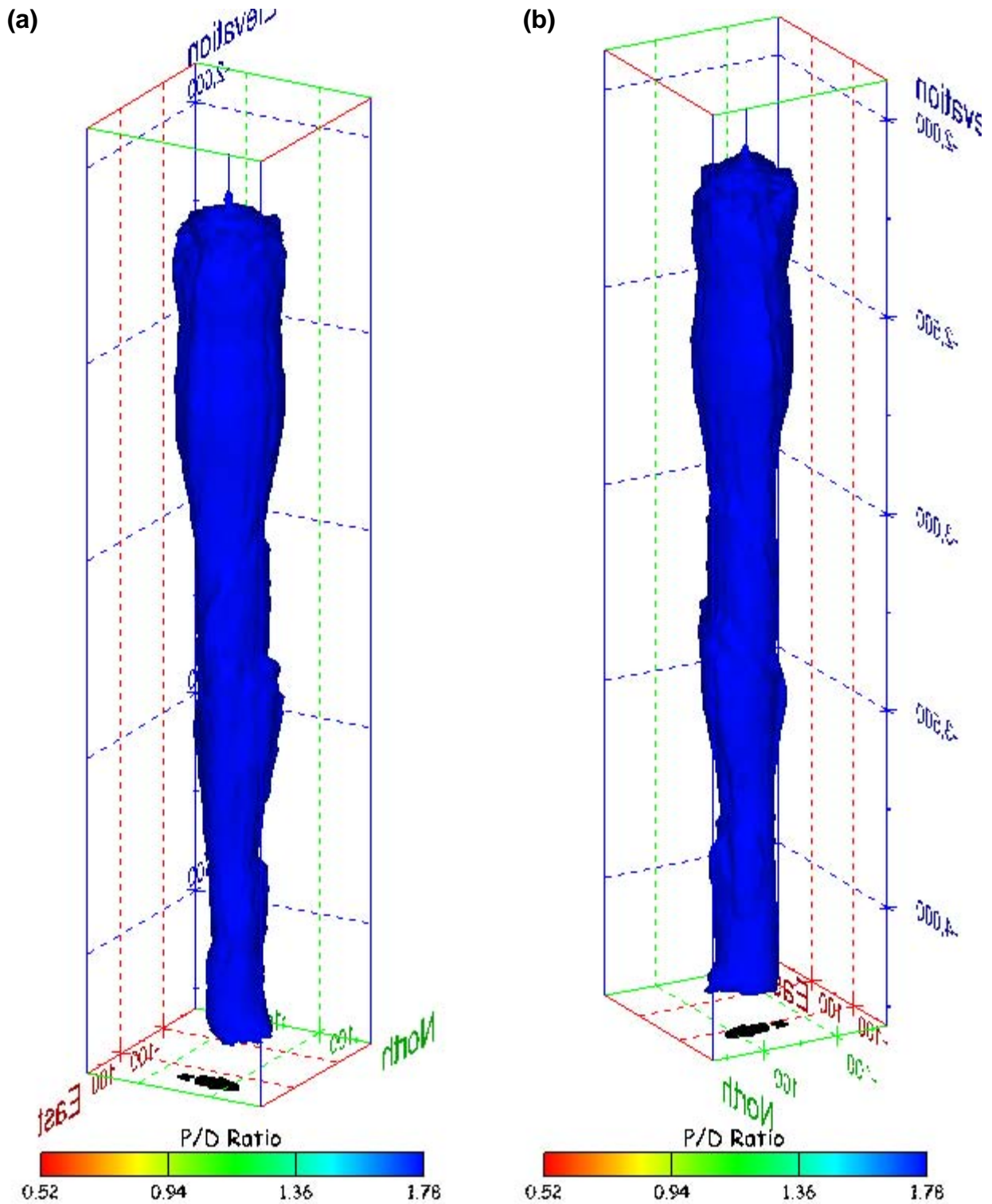
Figure 559. Sonar images of cavern BM-116, showing the geometry of the cavern colored by three-dimensional pillar-to-diameter ratio. View from (a) azimuth 60°, elevation 20°; (b) azimuth 300°, elevation 20°.
