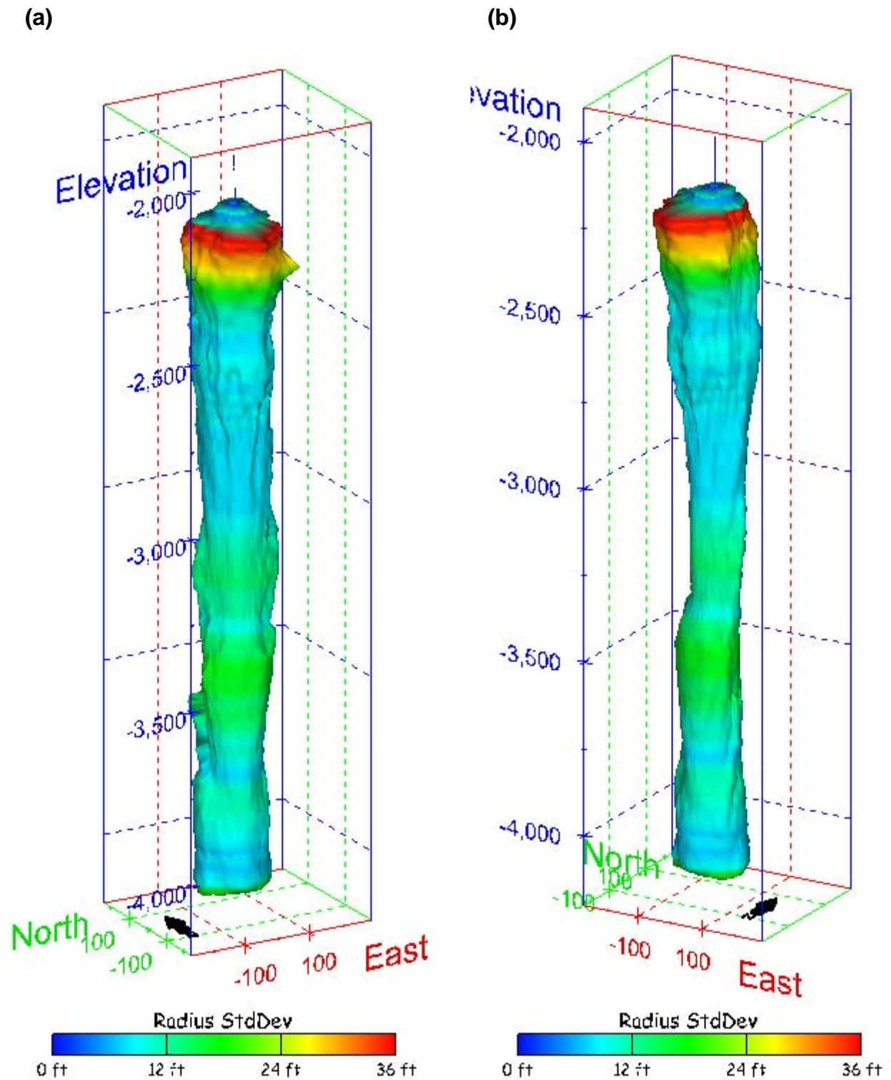
Figure 522. Sonar images of cavern BM-115, showing the geometry of the cavern colored by radius standard deviation. View from (a) azimuth 210°, elevation 20°; (b) azimuth 150°, elevation 20°.
