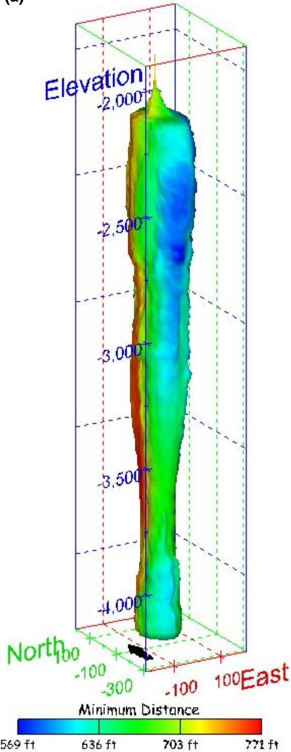
Figure 192. Sonar images of cavern BM-102, showing the geometry of the cavern colored by the minimum distance to the nearest neighboring cavern. View from (a) azimuth 210°, elevation 20°; (b) azimuth 150°, elevation 20°.
