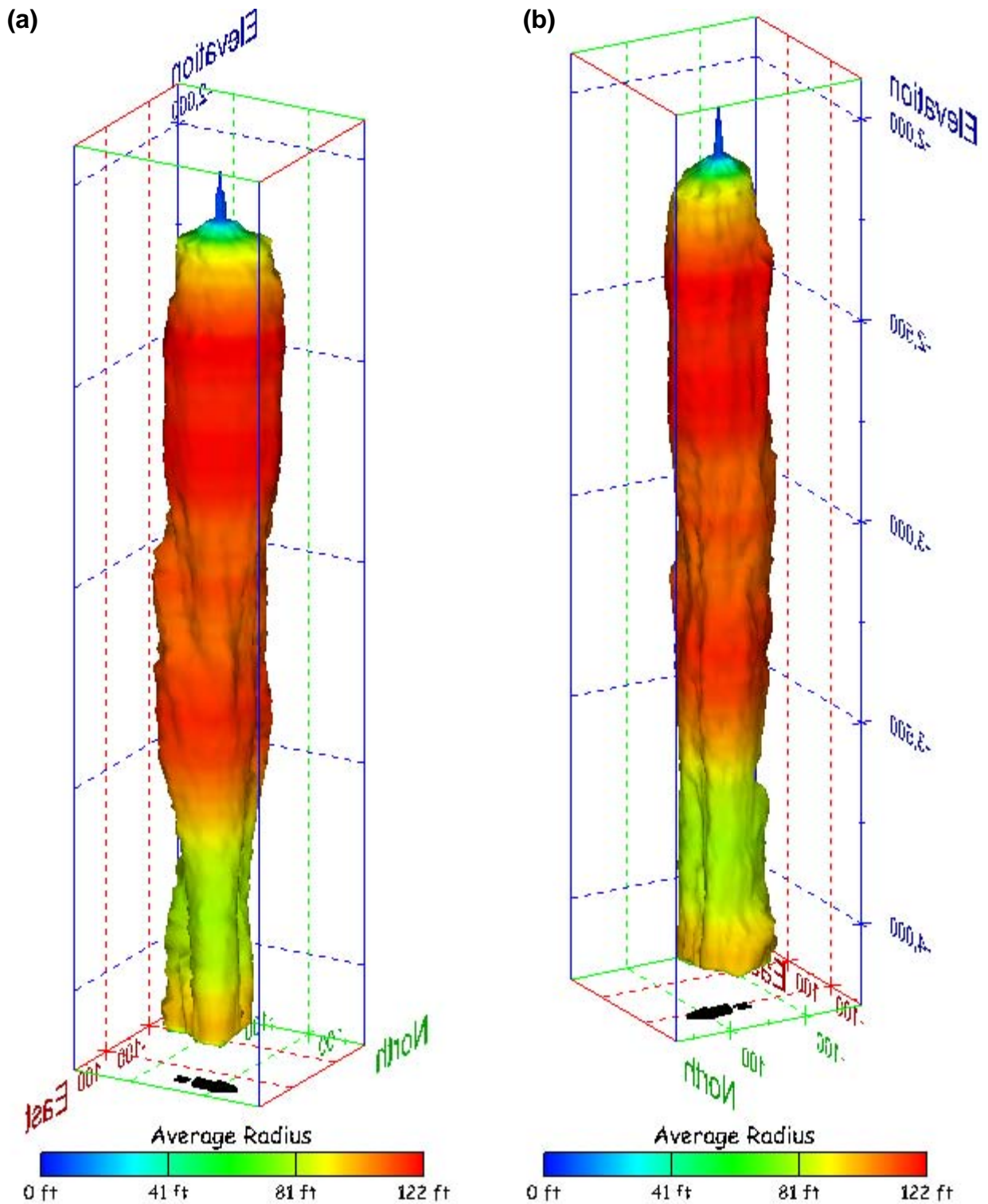
Figure 413. Sonar images of cavern BM-111, showing the geometry of the cavern colored by average radius. View from (a) azimuth 60°, elevation 20°; (b) azimuth 300°, elevation 20°.
