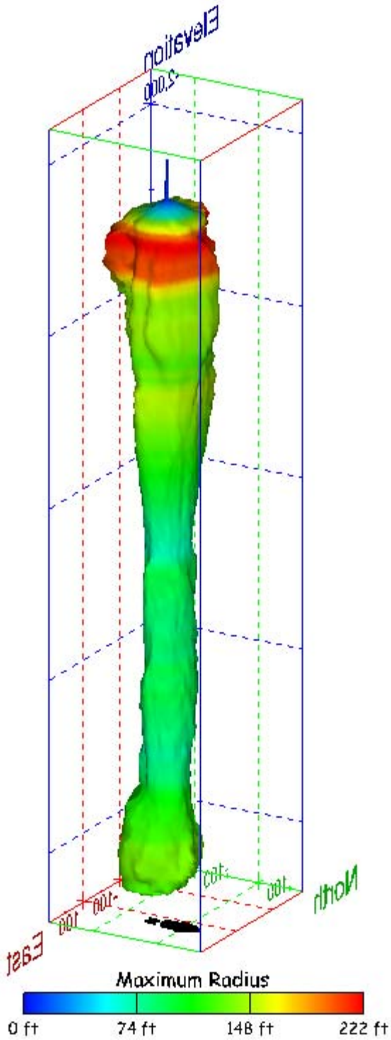
Figure 495. Sonar images of cavern BM-114, showing the geometry of the cavern colored by maximum radius. View from (a) azimuth 60°, elevation 20°; (b) azimuth 300°, elevation 20°.
