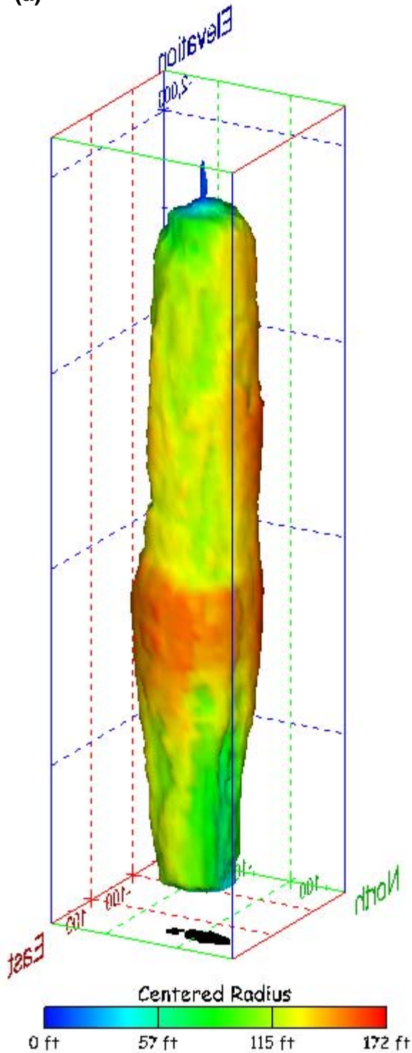
Figure 281. Sonar images of cavern BM-106, showing the geometry of the cavern colored by centered radius. View from (a) azimuth 60°, elevation 20°; (b) azimuth 300°, elevation 20°.
