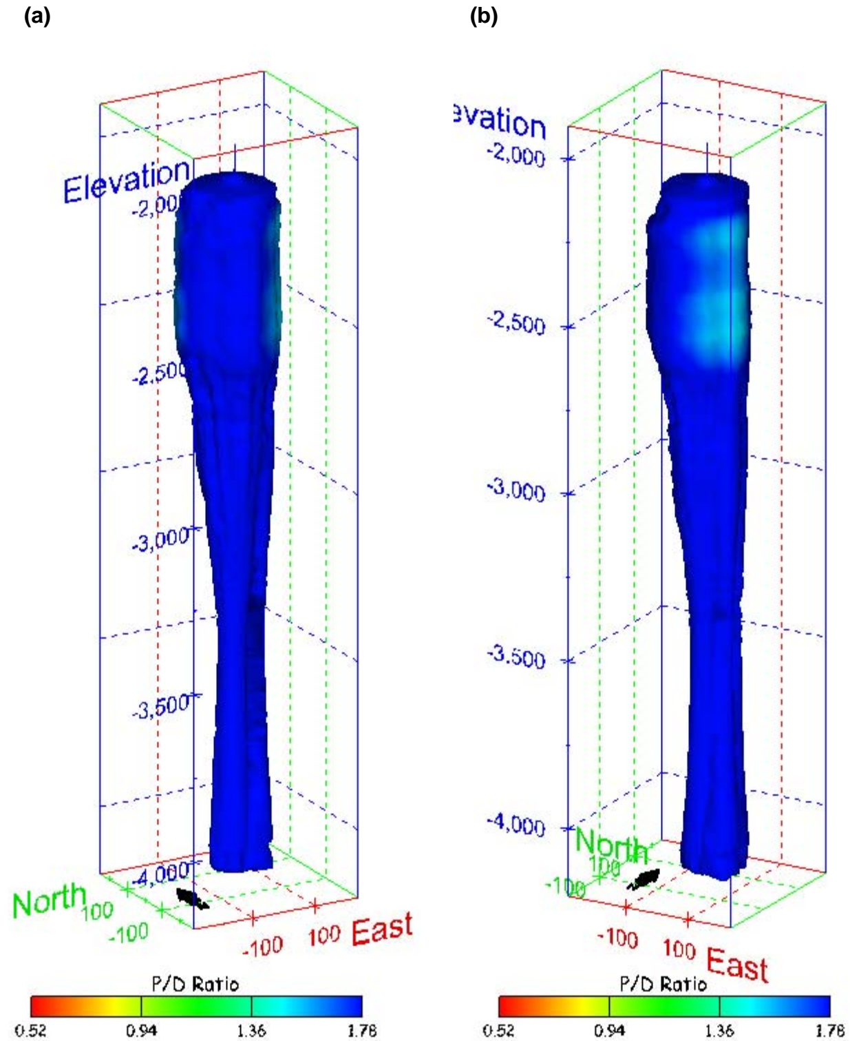
Figure 246. Sonar images of cavern BM-104, showing the geometry of the cavern colored by three-dimensional pillar-to-diameter ratio. View from (a) azimuth 210°, elevation 20°; (b) azimuth 150°, elevation 20°.
