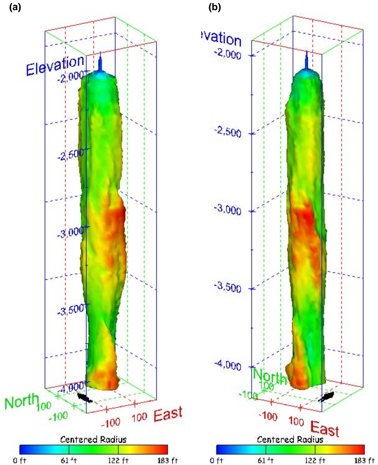
Figure 410. Sonar images of cavern BM-111, showing the geometry of the cavern colored by centered radius. View from (a) azimuth 210°, elevation 20°; (b) azimuth 150°, elevation 20°.
