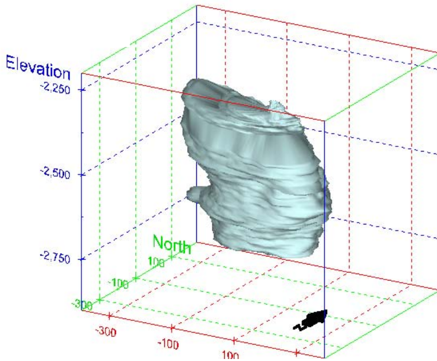
Figure 16. Sonar images of cavern BM-1, showing the basic geometric shape of the cavern. View from (a) azimuth 210°, elevation 20°; (b) azimuth 150°, elevation 20°.
