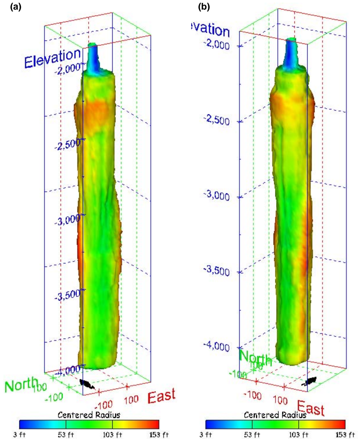
Figure 150. Sonar images of cavern BM-101, showing the geometry of the cavern colored by centered radius. View from (a) azimuth 210°, elevation 20°; (b) azimuth 150°, elevation 20°.
