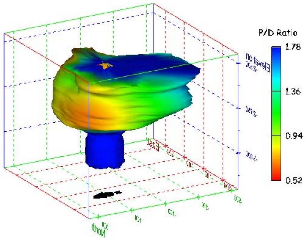
Figure 117. Sonar images of cavern BM-4, showing the geometry of the cavern colored by three-dimensional pillar-to-diameter ratio. View from (a) azimuth 60°, elevation 20°; (b) azimuth 300°, elevation 20°.
