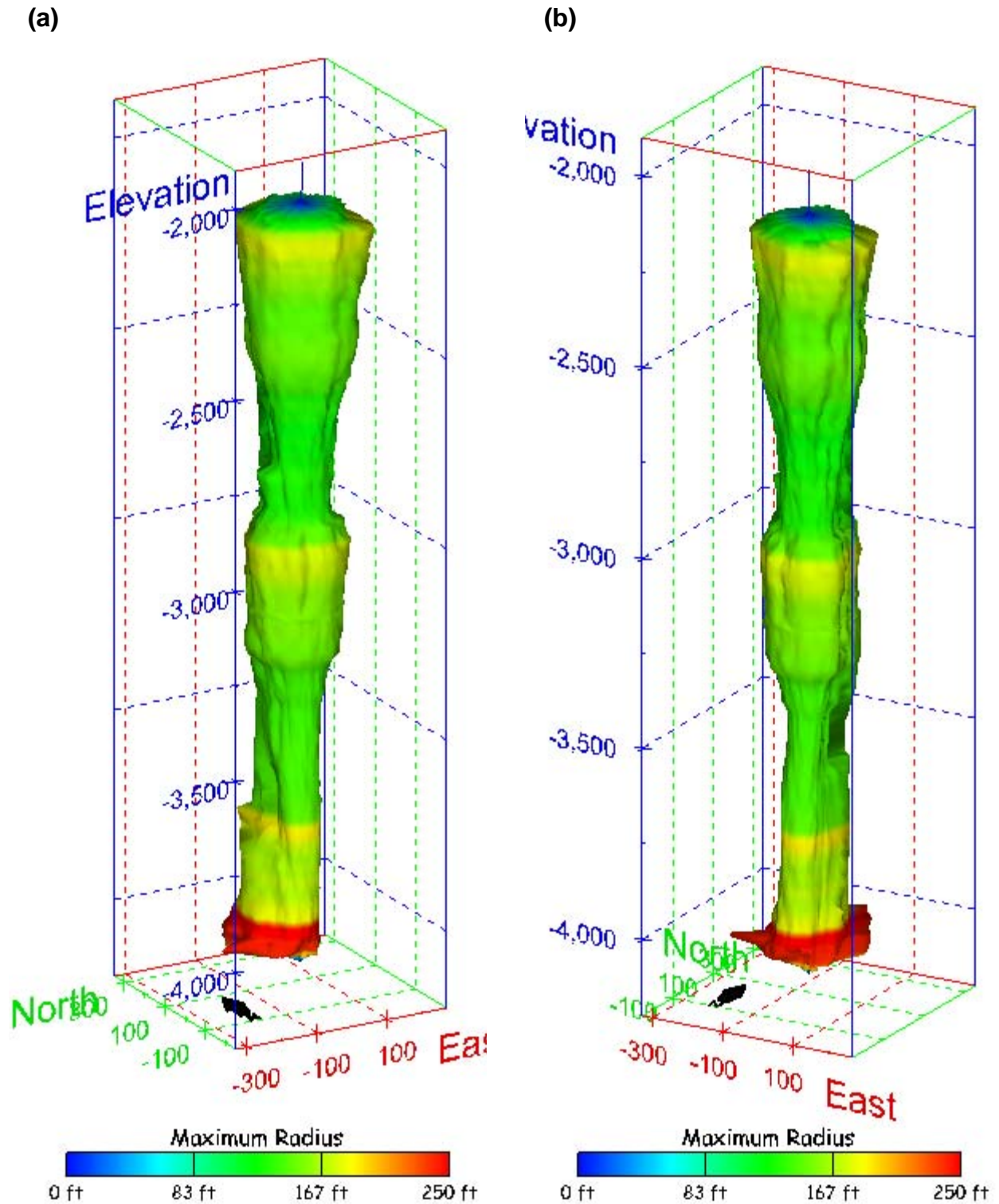
Figure 364. Sonar images of cavern BM-109, showing the geometry of the cavern colored by maximum radius. View from (a) azimuth 210°, elevation 20°; (b) azimuth 150°, elevation 20°.
