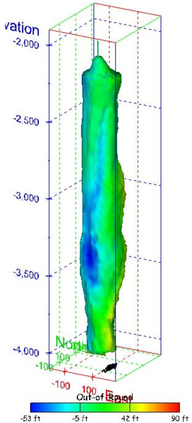
Figure 212. Sonar images of cavern BM-103, showing the geometry of the cavern colored by out-of-round distance. View from (a) azimuth 210°, elevation 20°; (b) azimuth 150°, elevation 20°.
