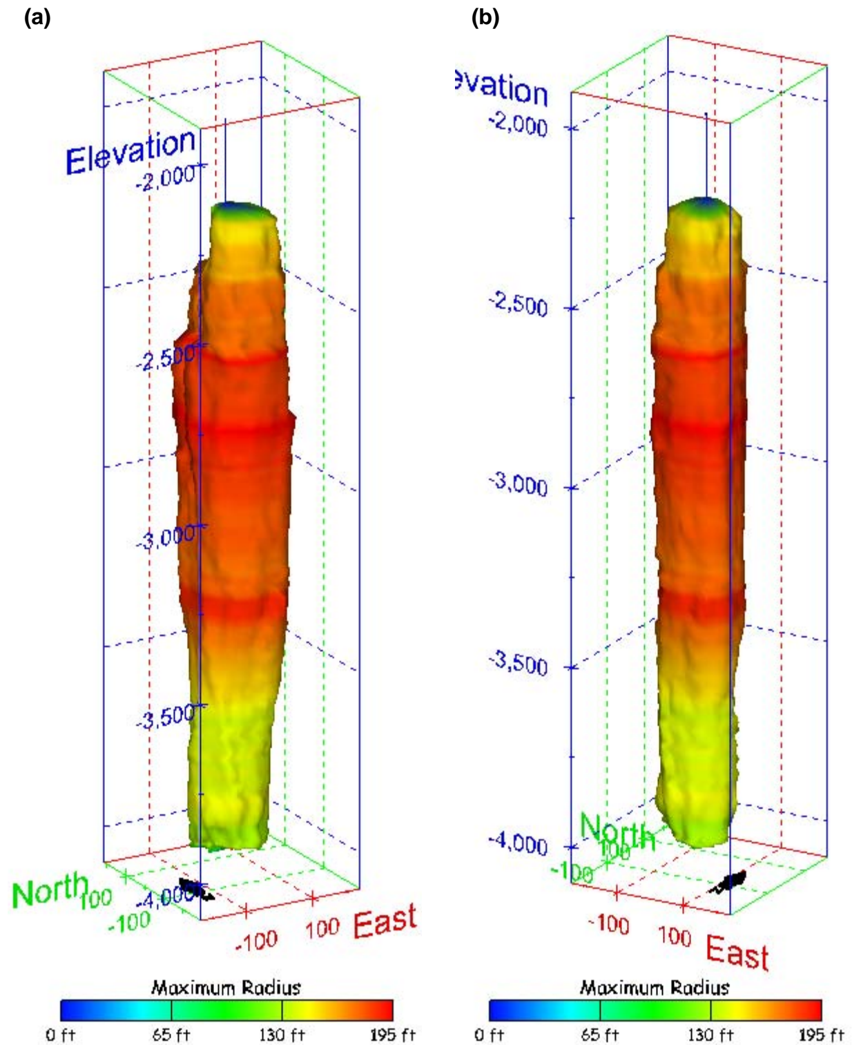
Figure 312. Sonar images of cavern BM-107, showing the geometry of the cavern colored by maximum radius. View from (a) azimuth 210°, elevation 20°; (b) azimuth 150°, elevation 20°.
