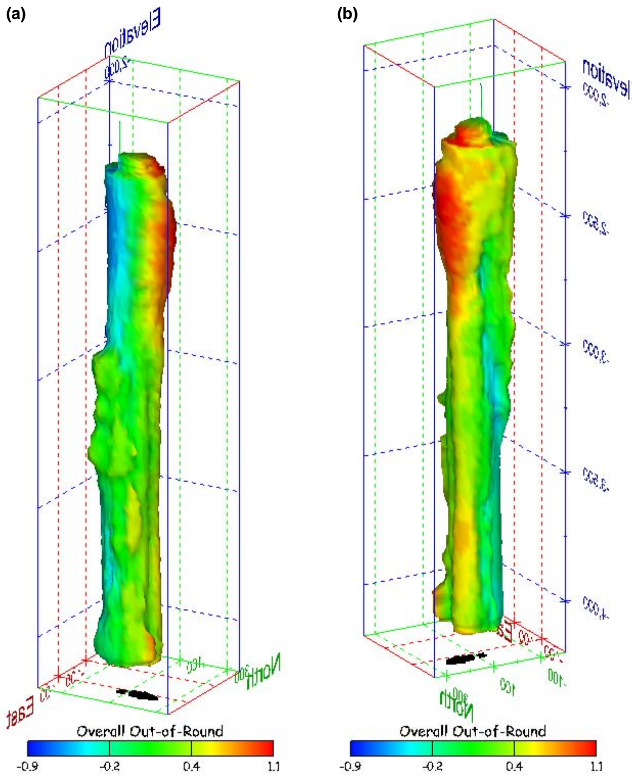
Figure 347. Sonar images of cavern BM-108, showing the geometry of the cavern colored by overall out-of-round ratio. View from (a) azimuth 60°, elevation 20°; (b) azimuth 300°, elevation 20°.
