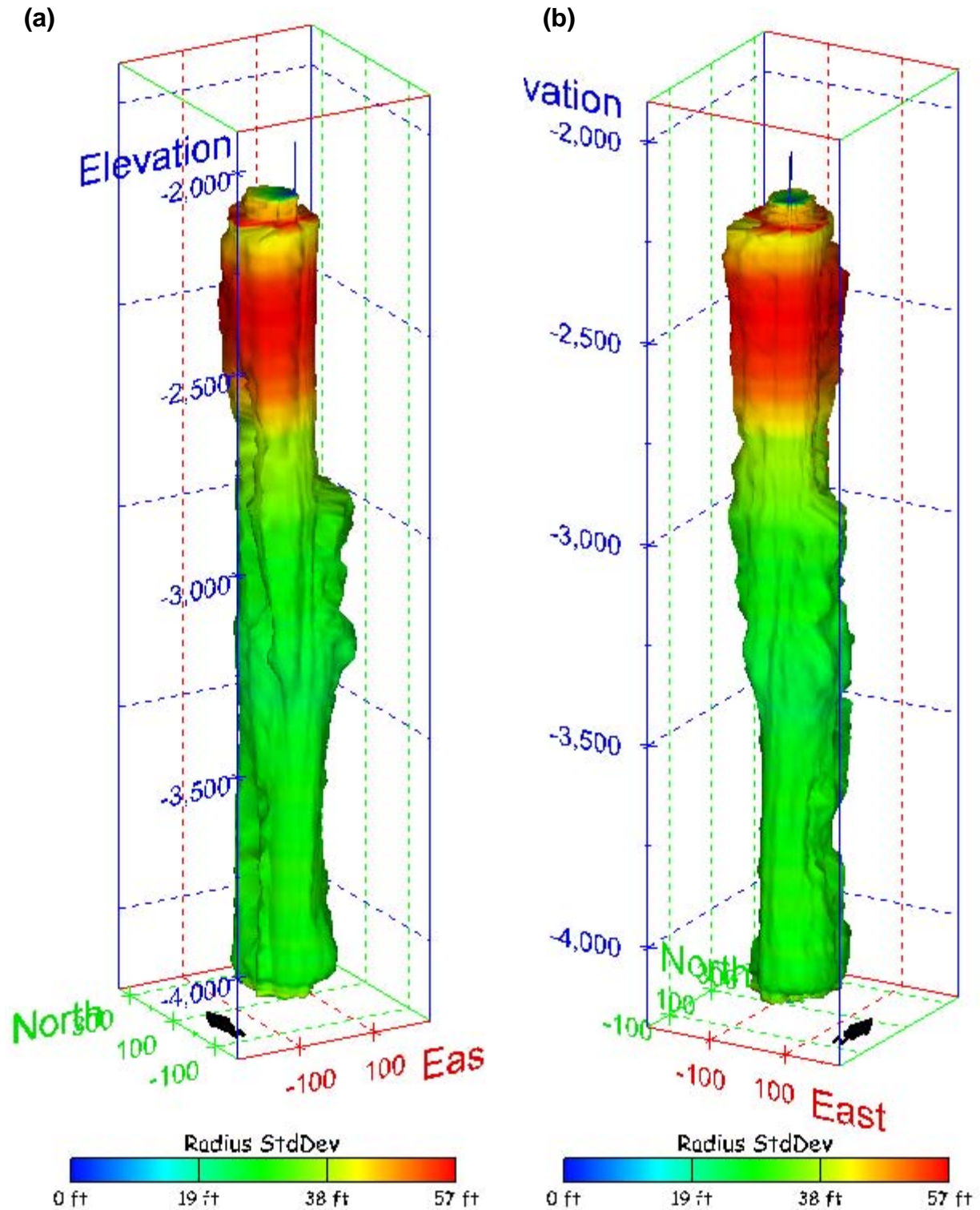
Figure 340. Sonar images of cavern BM-108, showing the geometry of the cavern colored by radius standard deviation. View from (a) azimuth 210°, elevation 20°; (b) azimuth 150°, elevation 20°.
