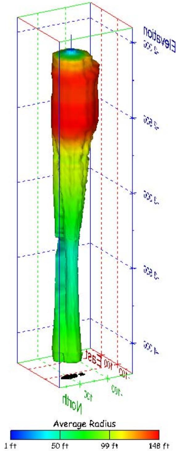
Figure 231. Sonar images of cavern BM-104, showing the geometry of the cavern colored by average radius. View from (a) azimuth 60°, elevation 20°; (b) azimuth 300°, elevation 20°.
