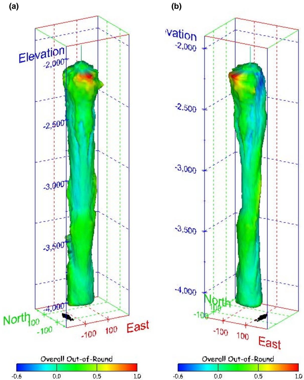
Figure 528. Sonar images of cavern BM-115, showing the geometry of the cavern colored by overall out-of-round ratio. View from (a) azimuth 210°, elevation 20°; (b) azimuth 150°, elevation 20°.
