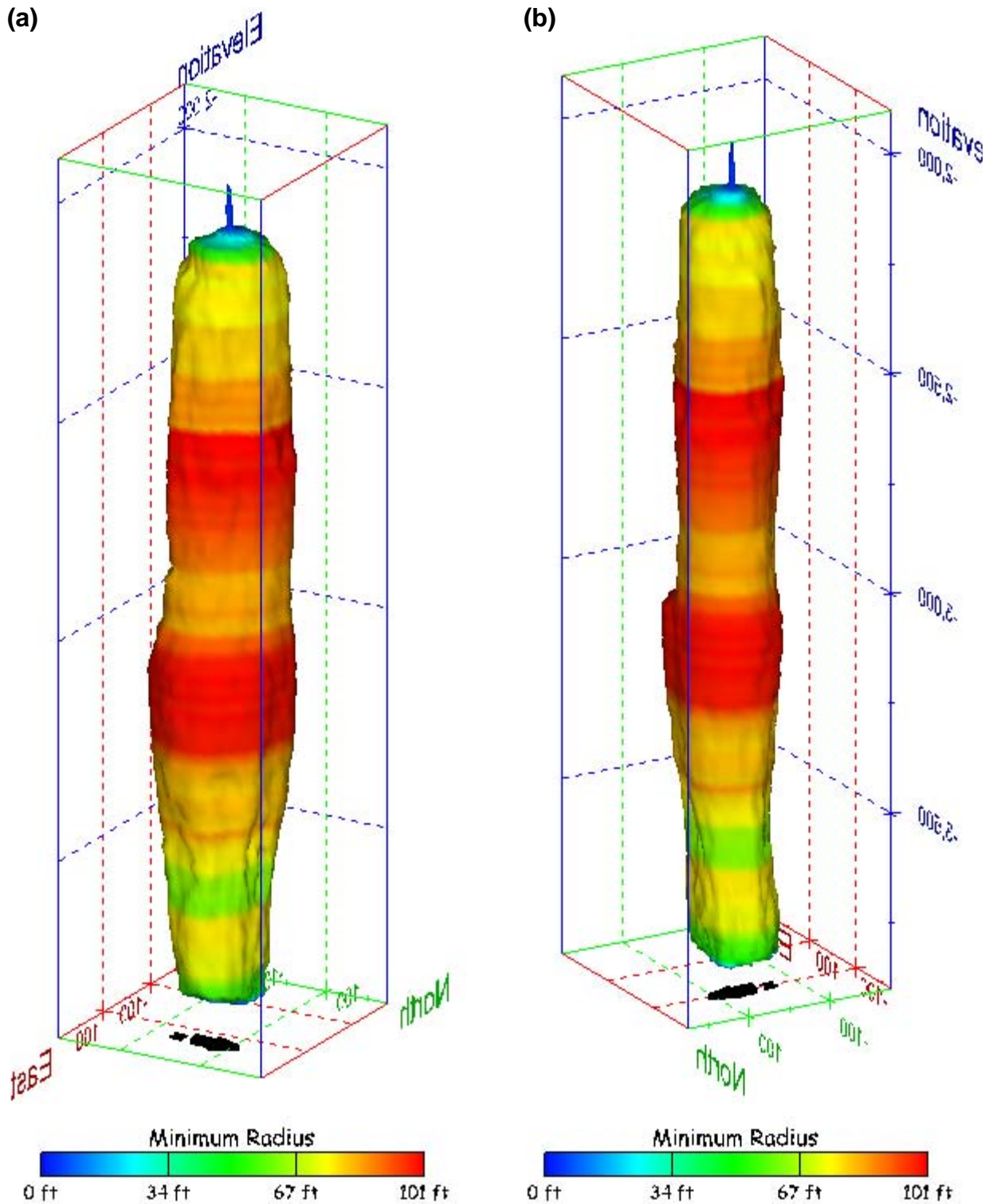
Figure 285. Sonar images of cavern BM-106, showing the geometry of the cavern colored by minimum radius. View from (a) azimuth 60°, elevation 20°; (b) azimuth 300°, elevation 20°.
