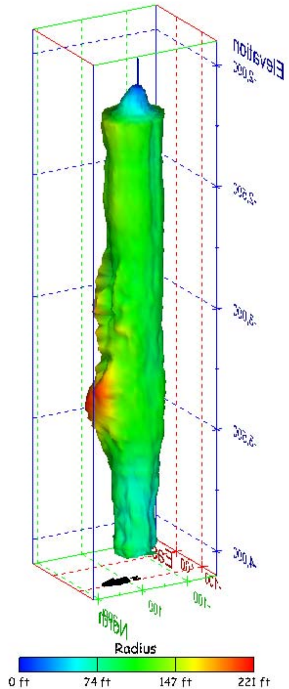
Figure 201. Sonar images of cavern BM-103, showing the geometry of the cavern colored by measured radius. View from (a) azimuth 60°, elevation 20°; (b) azimuth 300°, elevation 20°.
