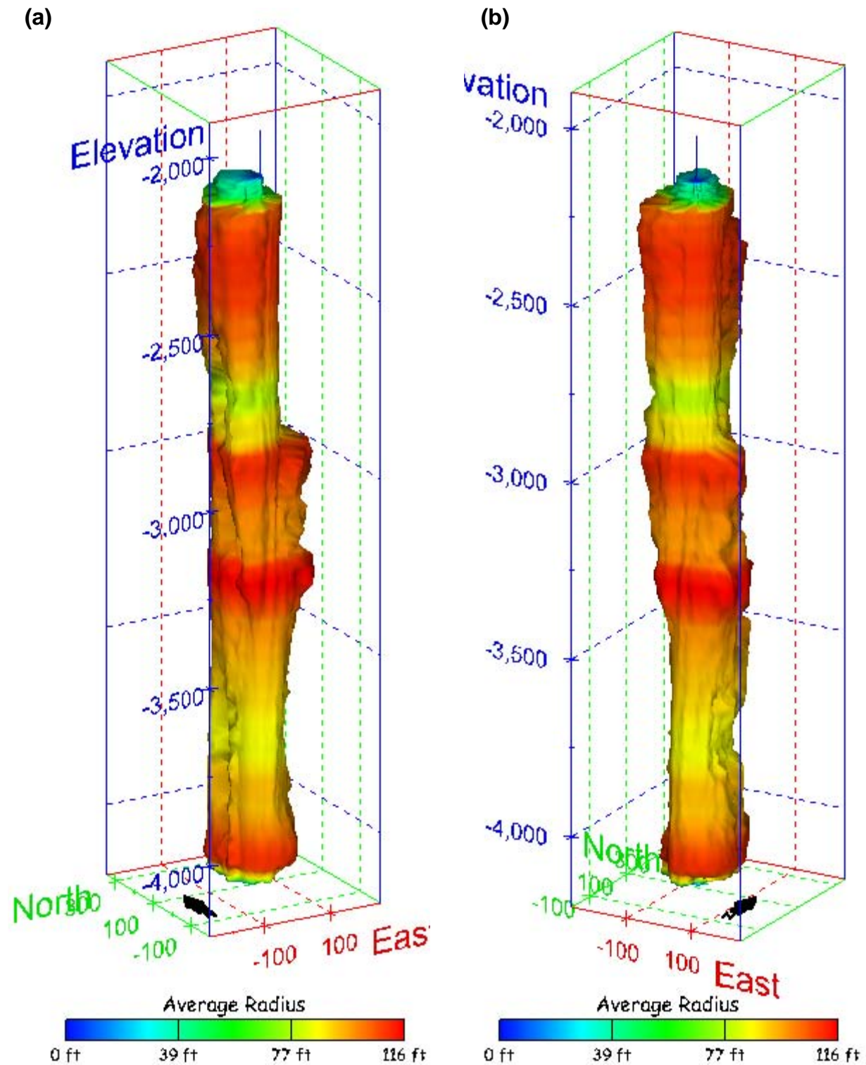
Figure 334. Sonar images of cavern BM-108, showing the geometry of the cavern colored by average radius. View from (a) azimuth 210°, elevation 20°; (b) azimuth 150°, elevation 20°.
