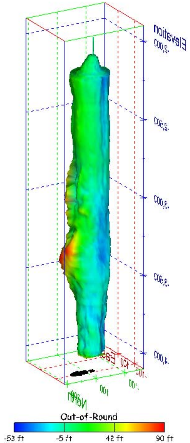
Figure 213. Sonar images of cavern BM-103, showing the geometry of the cavern colored by out-of-round distance. View from (a) azimuth 60°, elevation 20°; (b) azimuth 300°, elevation 20°.
