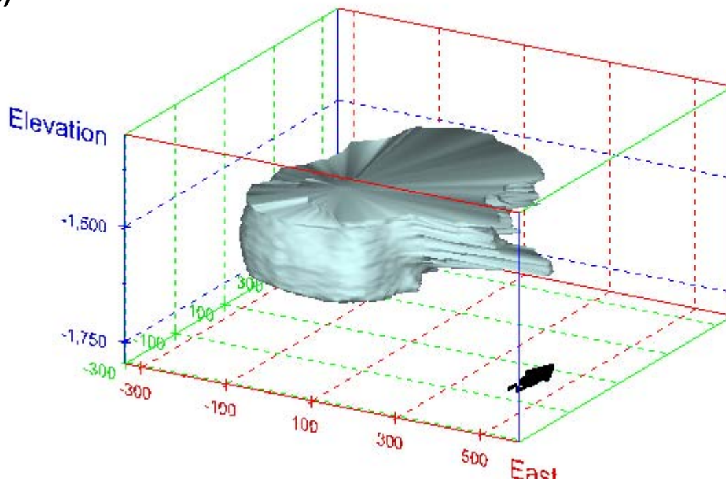
Figure 42. Sonar images of cavern BM-2, showing the basic geometric shape of the cavern. View from (a) azimuth 210°, elevation 20°; (b) azimuth 150°, elevation 20°.
