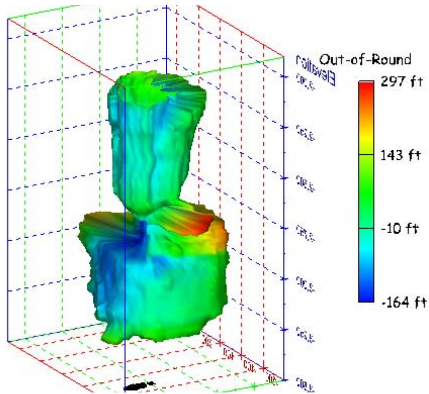
Figure 135. Sonar images of cavern BM-5, showing the geometry of the cavern colored by out-of-round distance. View from (a) azimuth 60°, elevation 20°; (b) azimuth 300°, elevation 20°.
