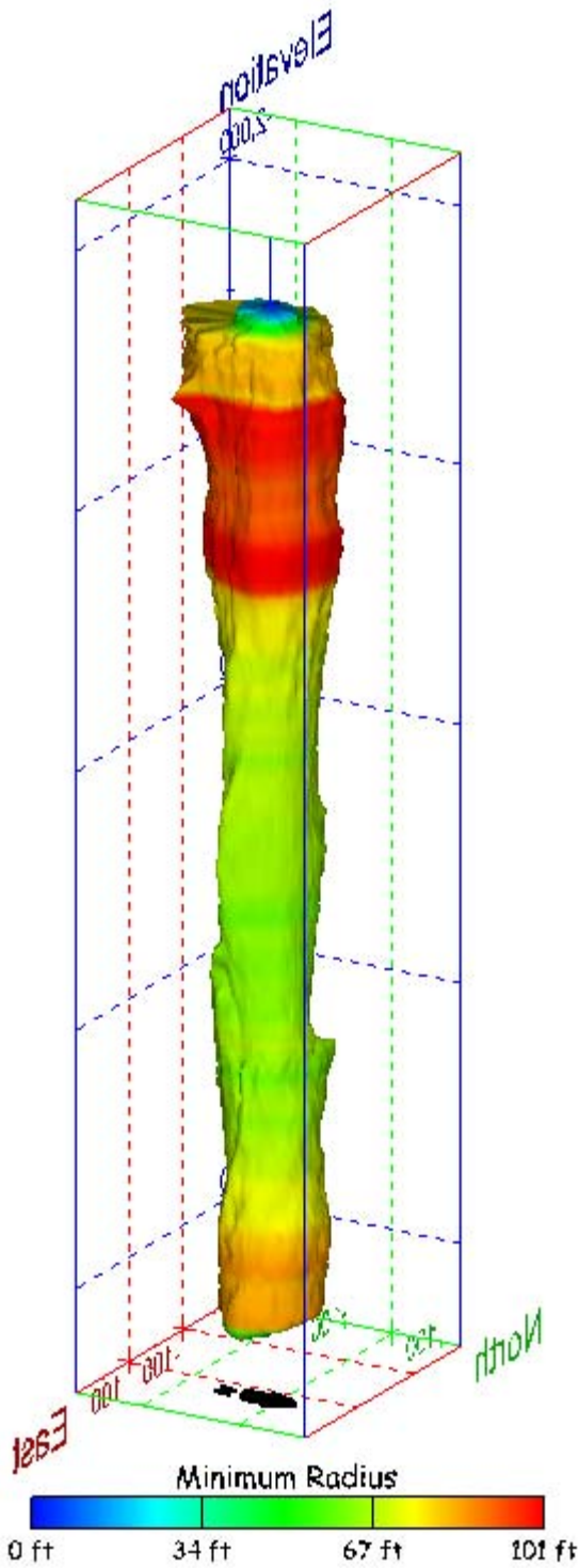
Figure 519. Sonar images of cavern BM-115, showing the geometry of the cavern colored by minimum radius. View from (a) azimuth 60°, elevation 20°; (b) azimuth 300°, elevation 20°.
