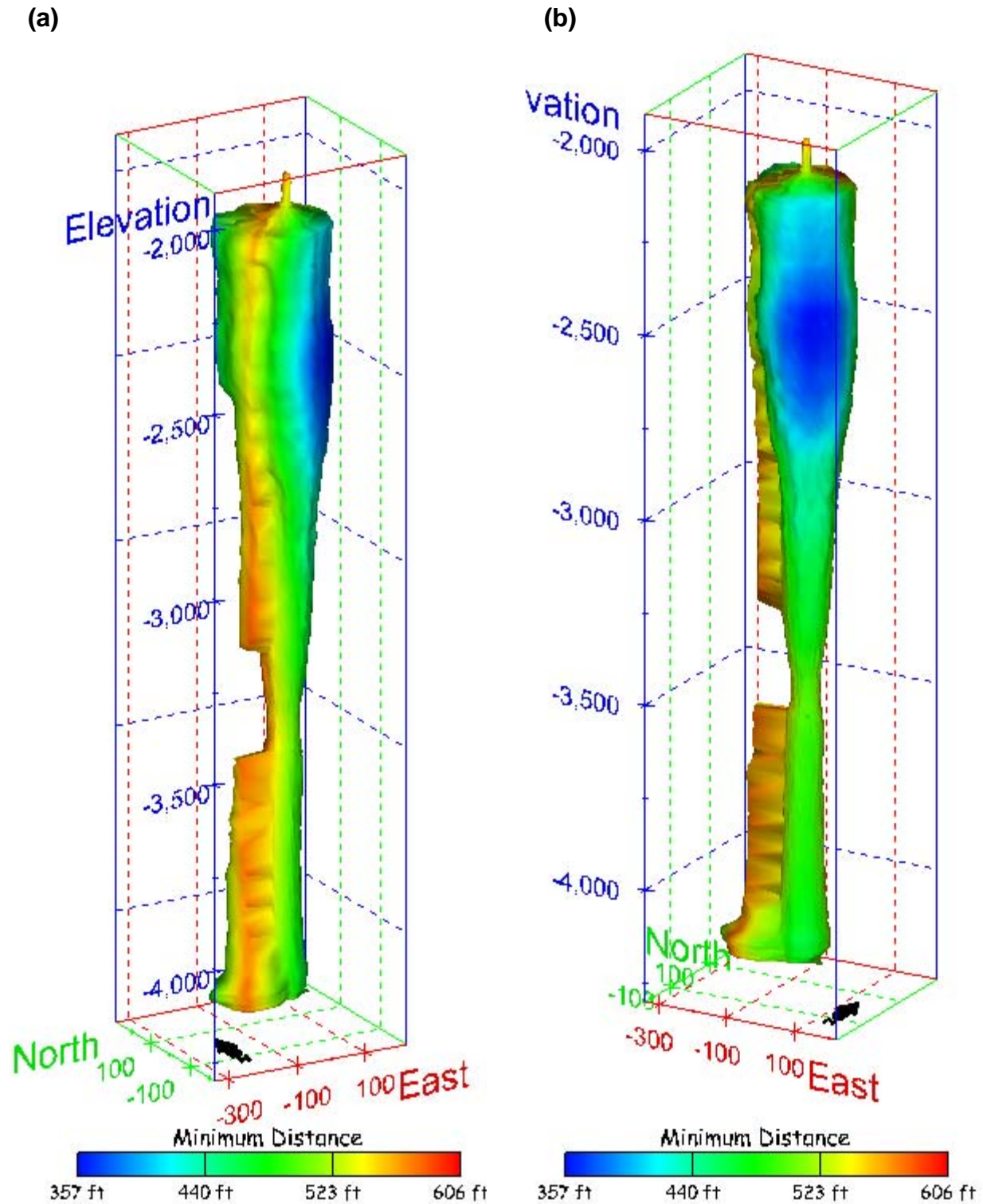
Figure 270. Sonar images of cavern BM-105, showing the geometry of the cavern colored by the minimum distance to the nearest neighboring cavern. View from (a) azimuth 210°, elevation 20°; (b) azimuth 150°, elevation 20°.
