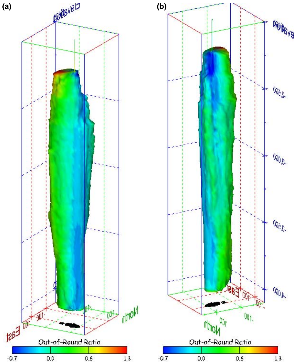
Figure 319. Sonar images of cavern BM-107, showing the geometry of the cavern colored by out-of-round ratio. View from (a) azimuth 60°, elevation 20°; (b) azimuth 300°, elevation 20°.
