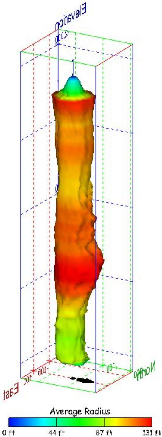
Figure 205. Sonar images of cavern BM-103, showing the geometry of the cavern colored by average radius. View from (a) azimuth 60°, elevation 20°; (b) azimuth 300°, elevation 20°.
