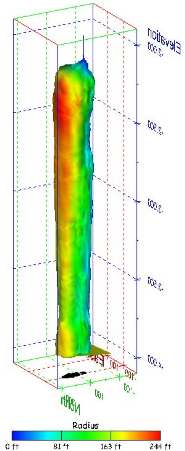
Figure 435. Sonar images of cavern BM-112, showing the geometry of the cavern colored by measured radius. View from (a) azimuth 60°, elevation 20°; (b) azimuth 300°, elevation 20°.
