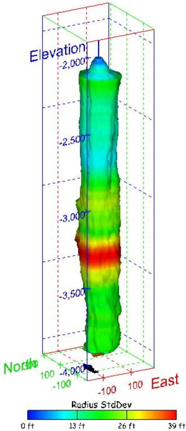
Figure 210. Sonar images of cavern BM-103, showing the geometry of the cavern colored by radius standard deviation. View from (a) azimuth 210°, elevation 20°; (b) azimuth 150°, elevation 20°.
