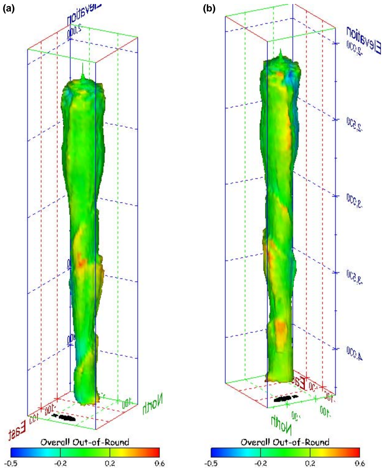
Figure 555. Sonar images of cavern BM-116, showing the geometry of the cavern colored by overall out-of-round ratio. View from (a) azimuth 60°, elevation 20°; (b) azimuth 300°, elevation 20°.
