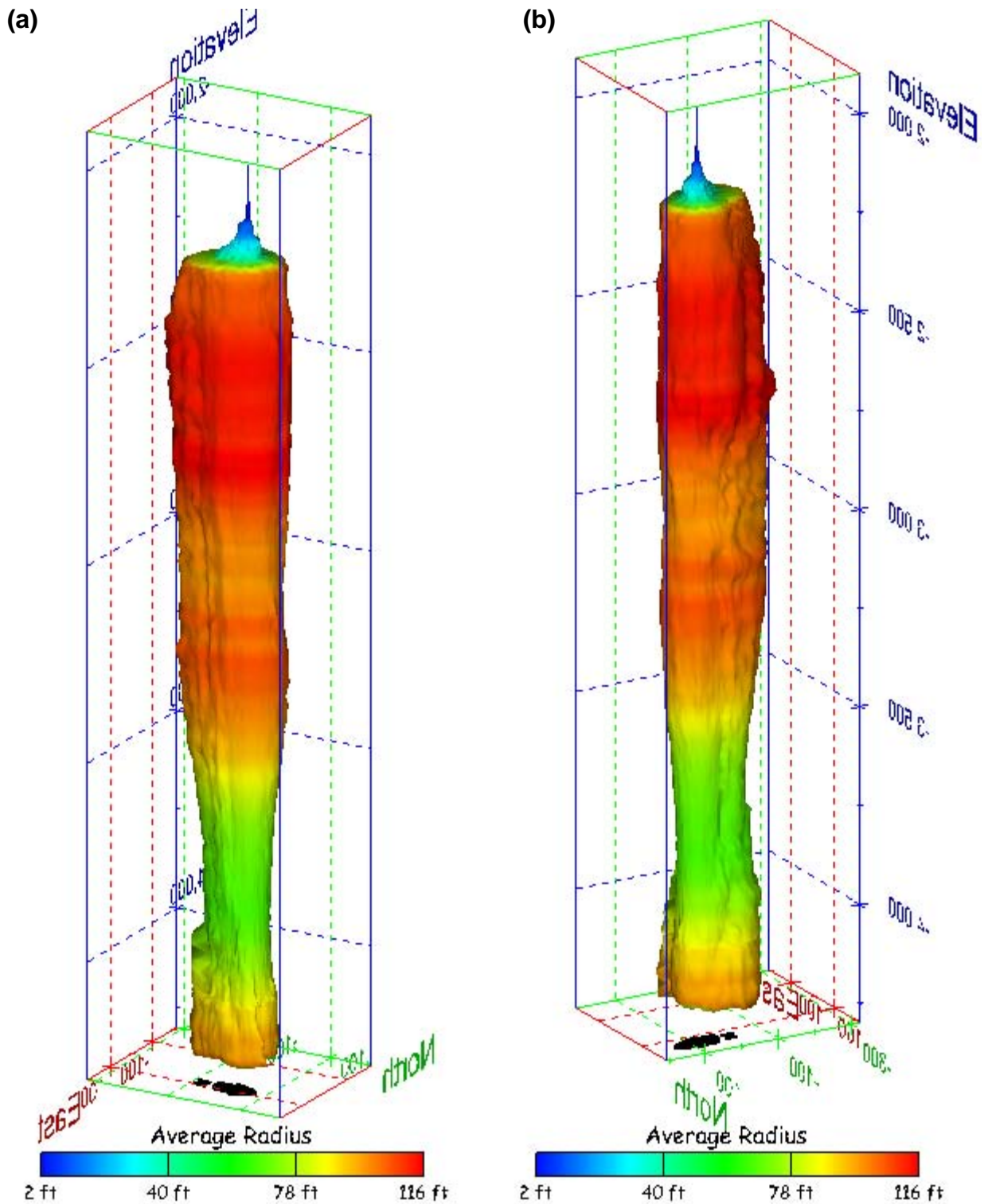
Figure 179. Sonar images of cavern BM-102, showing the geometry of the cavern colored by average radius. View from (a) azimuth 60°, elevation 20°; (b) azimuth 300°, elevation 20°.
