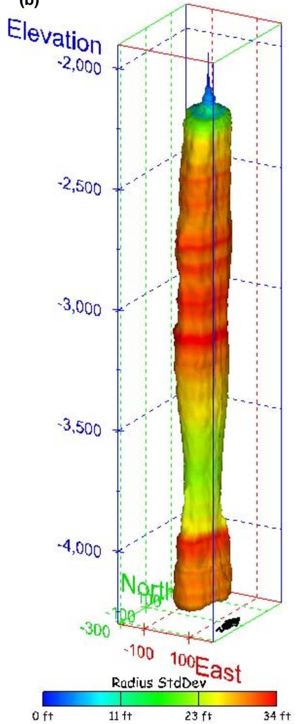
Figure 184. Sonar images of cavern BM-102, showing the geometry of the cavern colored by radius standard deviation. View from (a) azimuth 210°, elevation 20°; (b) azimuth 150°, elevation 20°.
