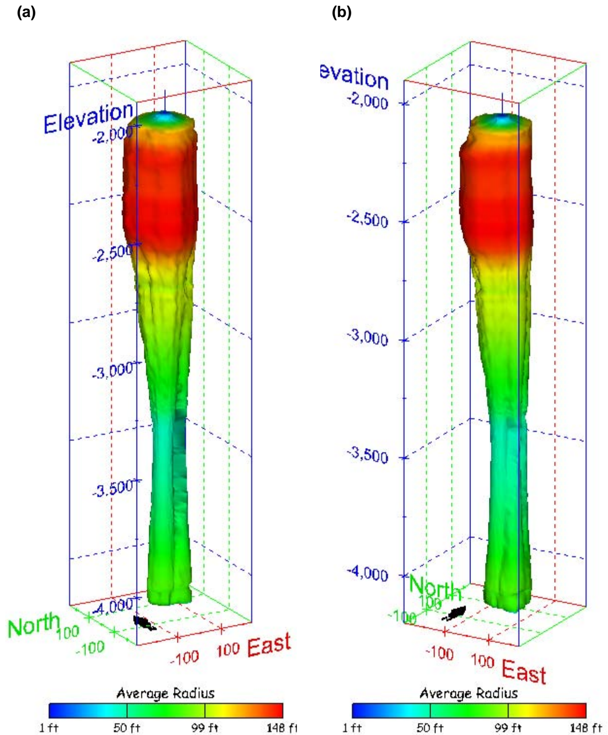
Figure 230. Sonar images of cavern BM-104, showing the geometry of the cavern colored by average radius. View from (a) azimuth 210°, elevation 20°; (b) azimuth 150°, elevation 20°.
