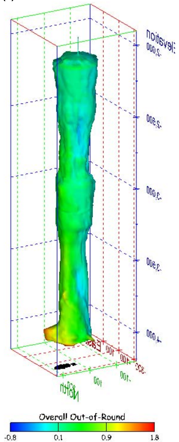
Figure 373. Sonar images of cavern BM-109, showing the geometry of the cavern colored by overall out-of-round ratio. View from (a) azimuth 60°, elevation 20°; (b) azimuth 300°, elevation 20°.
