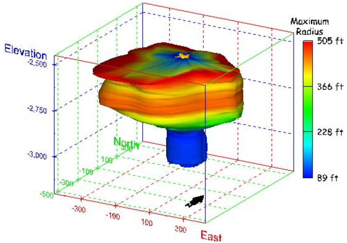
Figure 104. Sonar images of cavern BM-4, showing the geometry of the cavern colored by maximum radius. View from (a) azimuth 210°, elevation 20°; (b) azimuth 150°, elevation 20°.
