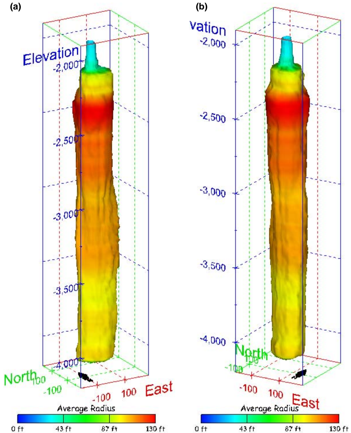
Figure 152. Sonar images of cavern BM-101, showing the geometry of the cavern colored by average radius. View from (a) azimuth 210°, elevation 20°; (b) azimuth 150°, elevation 20°.
