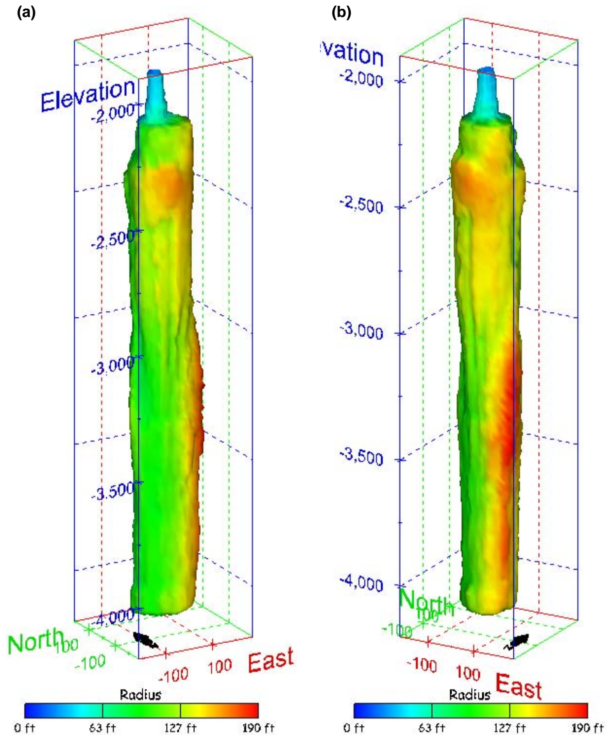
Figure 148. Sonar images of cavern BM-101, showing the geometry of the cavern colored by measured radius. View from (a) azimuth 210°, elevation 20°; (b) azimuth 150°, elevation 20°.
