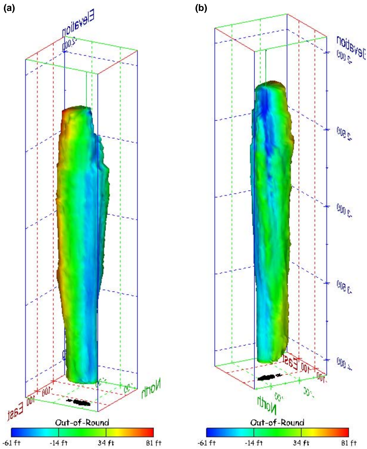
Figure 317. Sonar images of cavern BM-107, showing the geometry of the cavern colored by out-of-round distance. View from (a) azimuth 60°, elevation 20°; (b) azimuth 300°, elevation 20°.
