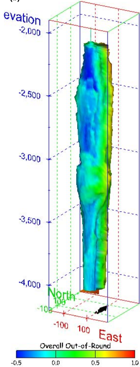
Figure 398. Sonar images of cavern BM-110, showing the geometry of the cavern colored by overall out-of-round ratio. View from (a) azimuth 210°, elevation 20°; (b) azimuth 150°, elevation 20°.
