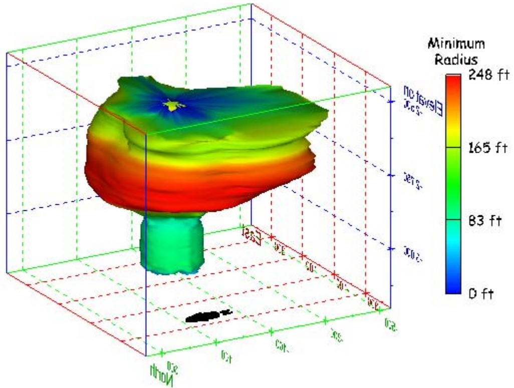
Figure 103. Sonar images of cavern BM-4, showing the geometry of the cavern colored by minimum radius. View from (a) azimuth 60°, elevation 20°; (b) azimuth 300°, elevation 20°.
