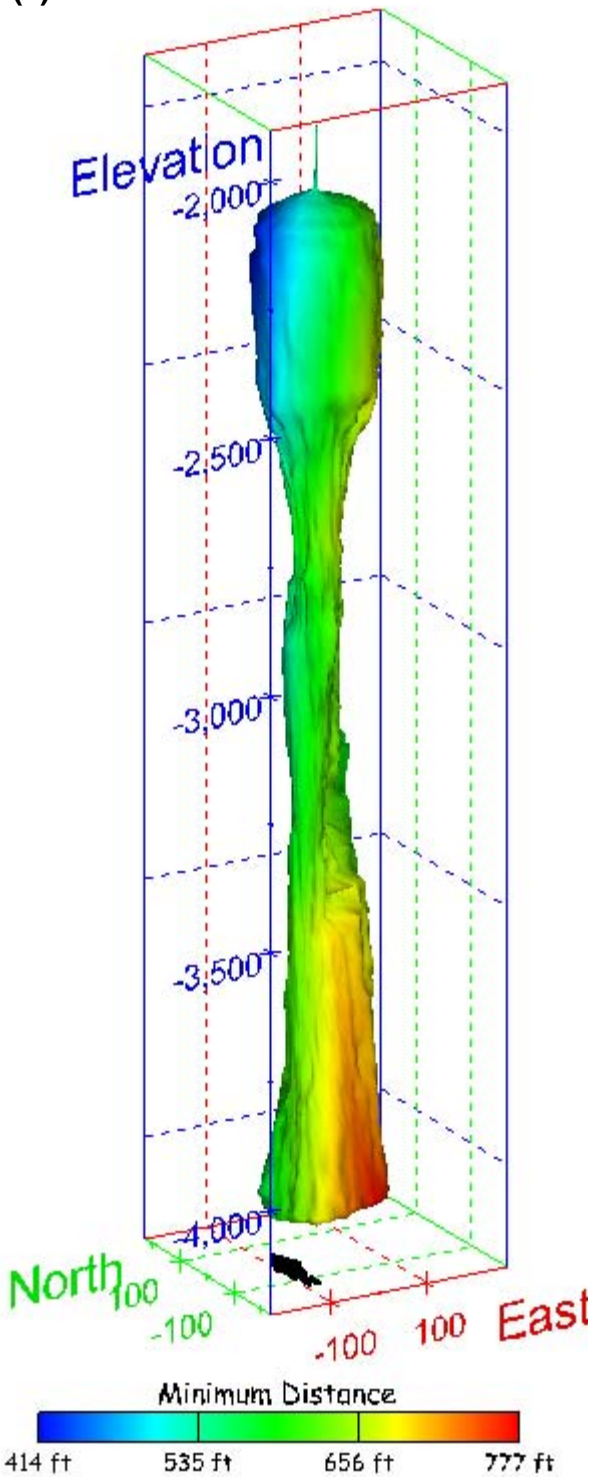
Figure 478. Sonar images of cavern BM-113, showing the geometry of the cavern colored by the minimum distance to the nearest neighboring cavern. View from (a) azimuth 210°, elevation 20°; (b) azimuth 150°, elevation 20°.
