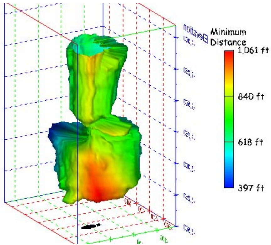
Figure 141. Sonar images of cavern BM-5, showing the geometry of the cavern colored by minimum distance to the nearest neighboring cavern. View from (a) azimuth 60°, elevation 20°; (b) azimuth 300°, elevation 20°.
