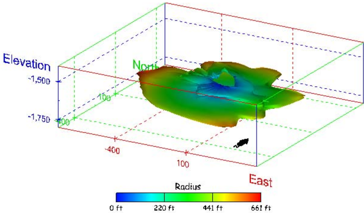
Figure 70. Sonar images of cavern BM-3, showing the geometry of the cavern colored by measured radius. View from (a) azimuth 210°, elevation 20°; (b) azimuth 150°, elevation 20°.
