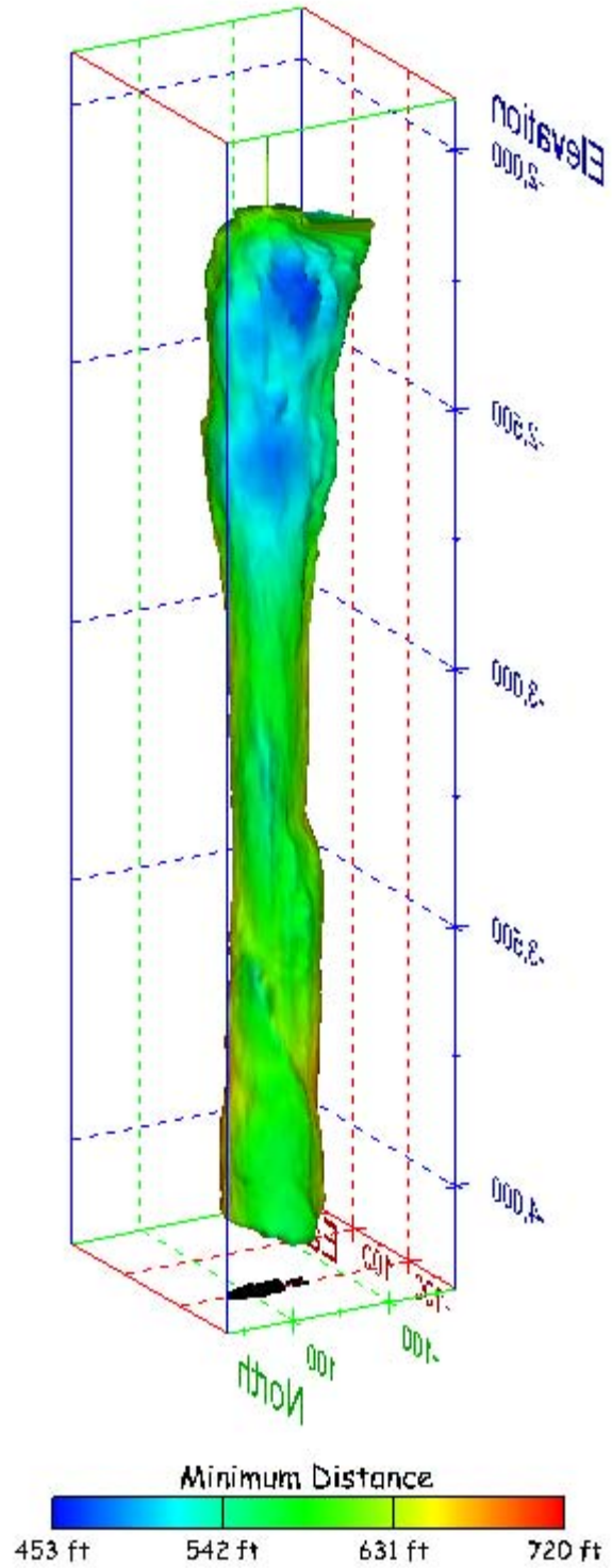
Figure 531. Sonar images of cavern BM-115, showing the geometry of the cavern colored by minimum distance to the nearest neighboring cavern. View from (a) azimuth 60°, elevation 20°; (b) azimuth 300°, elevation 20°.
