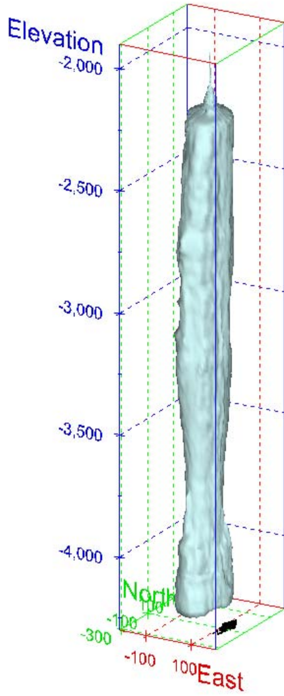
Figure 172. Sonar images of cavern BM-102, showing the basic geometric shape of the cavern. View from (a) azimuth 210°, elevation 20°; (b) azimuth 150°, elevation 20°.
