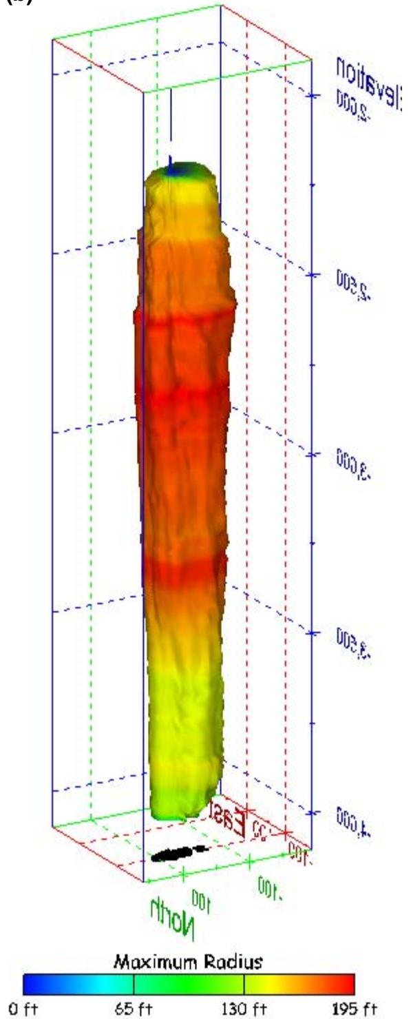
Figure 313. Sonar images of cavern BM-107, showing the geometry of the cavern colored by maximum radius. View from (a) azimuth 60°, elevation 20°; (b) azimuth 300°, elevation 20°.
