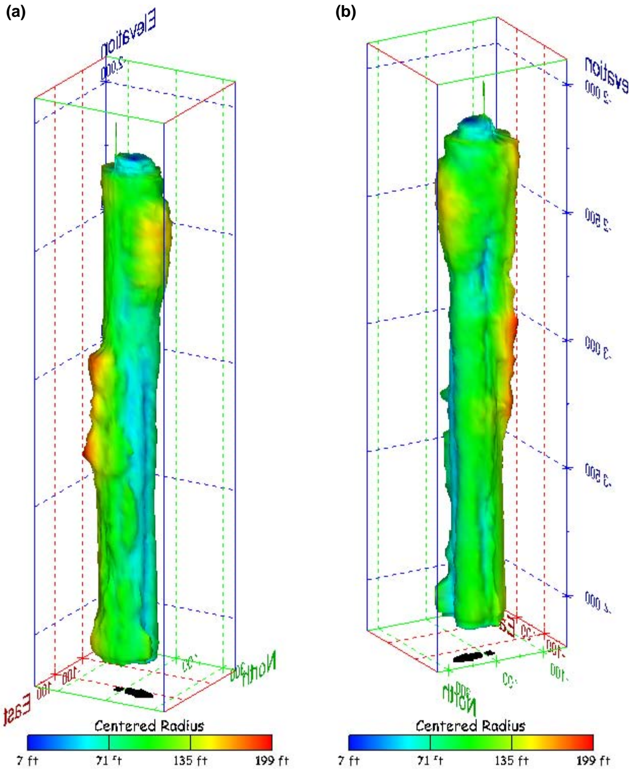
Figure 333. Sonar images of cavern BM-108, showing the geometry of the cavern colored by centered radius. View from (a) azimuth 60°, elevation 20°; (b) azimuth 300°, elevation 20°.
