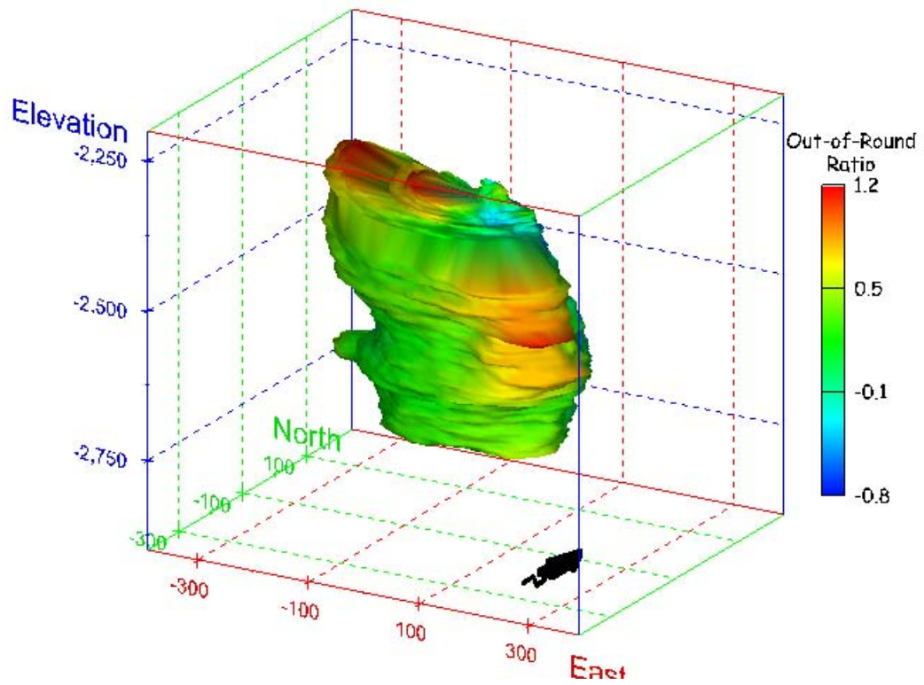
Figure 32. Sonar images of cavern BM-1, showing the geometry of the cavern colored by out-of-round ratio. View from (a) azimuth 210°, elevation 20°; (b) azimuth 150°, elevation 20°.
