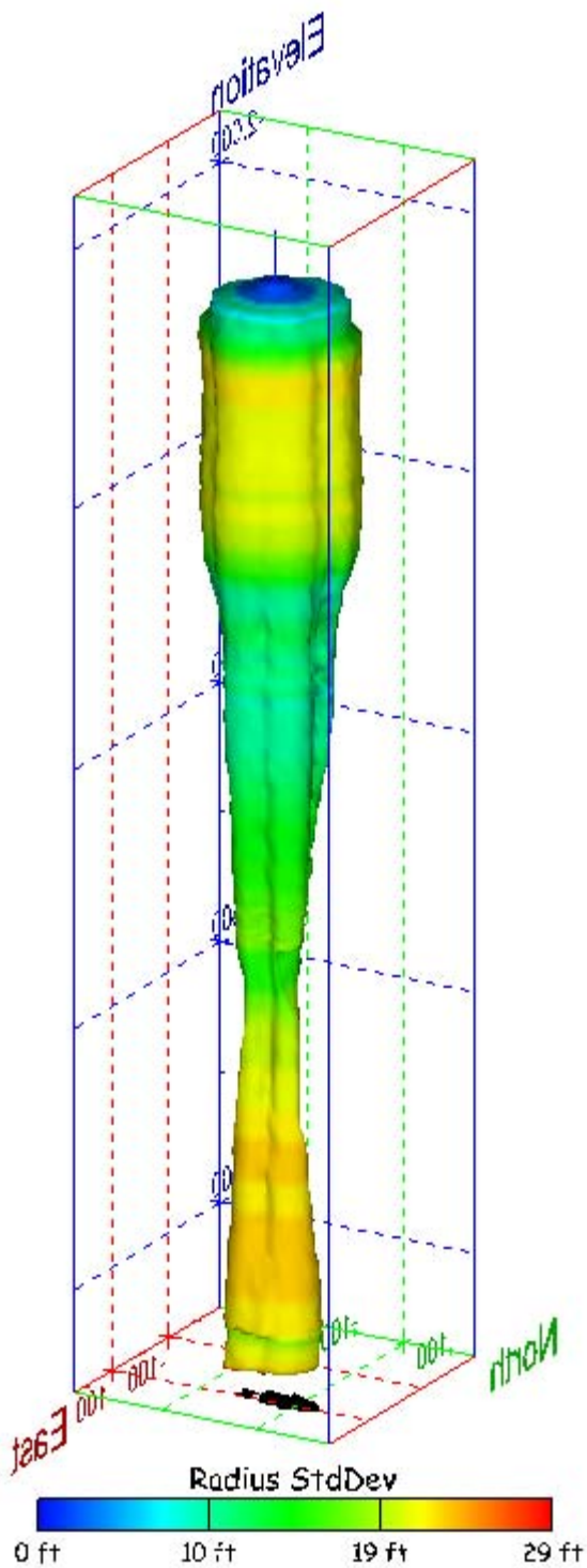
Figure 237. Sonar images of cavern BM-104, showing the geometry of the cavern colored by radius standard deviation. View from (a) azimuth 60°, elevation 20°; (b) azimuth 300°, elevation 20°.
