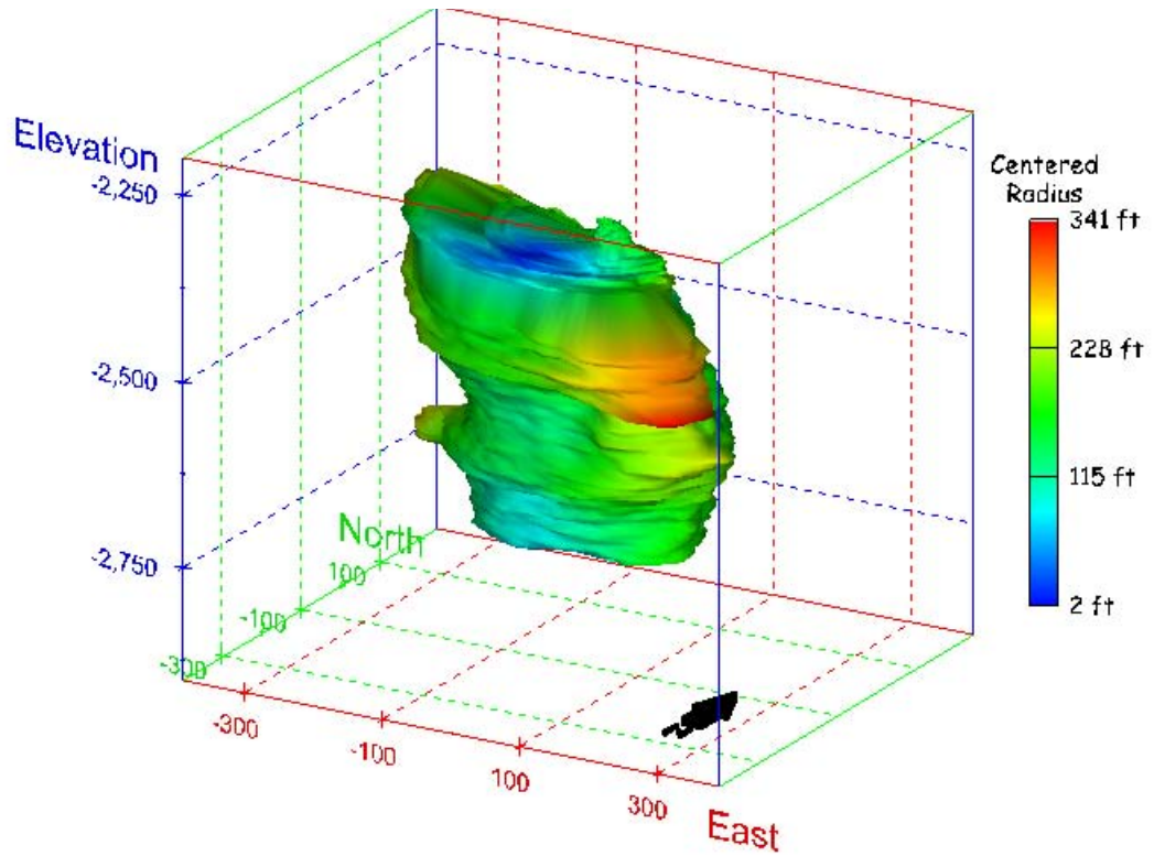
Figure 20. Sonar images of cavern BM-1, showing the geometry of the cavern colored by centered radius. View from (a) azimuth 210°, elevation 20°; (b) azimuth 150°, elevation 20°.
