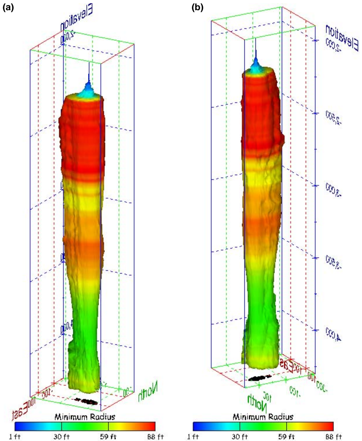
Figure 181. Sonar images of cavern BM-102, showing the geometry of the cavern colored by minimum radius. View from (a) azimuth 60°, elevation 20°; (b) azimuth 300°, elevation 20°.
