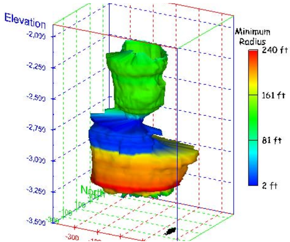
Figure 128. Sonar images of cavern BM-5, showing the geometry of the cavern colored by minimum radius. View from (a) azimuth 210°, elevation 20°; (b) azimuth 150°, elevation 20°.
