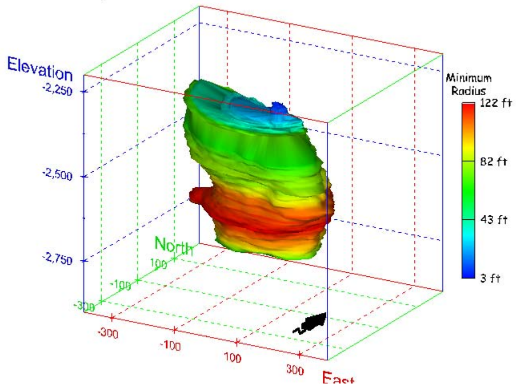
Figure 24. Sonar images of cavern BM-1, showing the geometry of the cavern colored by minimum radius. View from (a) azimuth 210°, elevation 20°; (b) azimuth 150°, elevation 20°.
