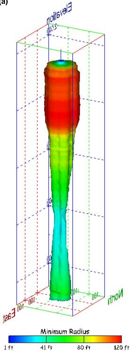
Figure 233. Sonar images of cavern BM-104, showing the geometry of the cavern colored by minimum radius. View from (a) azimuth 60°, elevation 20°; (b) azimuth 300°, elevation 20°.
