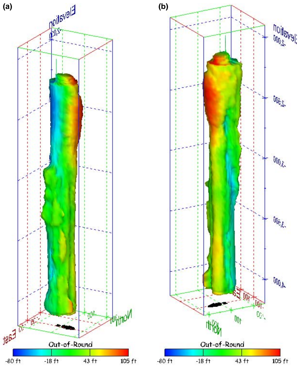
Figure 343. Sonar images of cavern BM-108, showing the geometry of the cavern colored by out-of-round distance. View from (a) azimuth 60°, elevation 20°; (b) azimuth 300°, elevation 20°.
