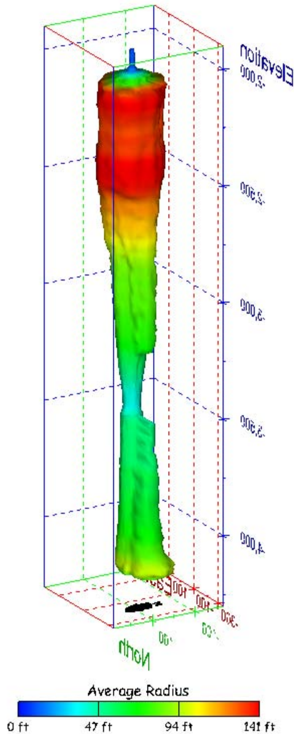
Figure 257. Sonar images of cavern BM-105, showing the geometry of the cavern colored by average radius. View from (a) azimuth 60°, elevation 20°; (b) azimuth 300°, elevation 20°.
