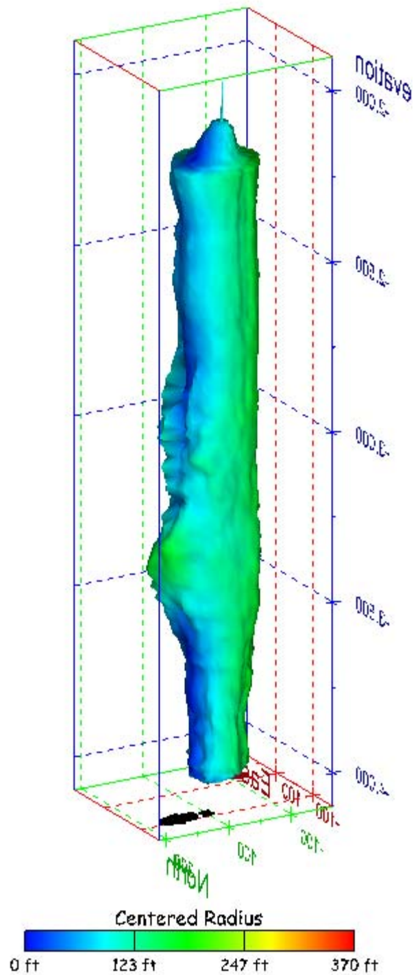
Figure 203. Sonar images of cavern BM-103, showing the geometry of the cavern colored by centered radius. View from (a) azimuth 60°, elevation 20°; (b) azimuth 300°, elevation 20°.
