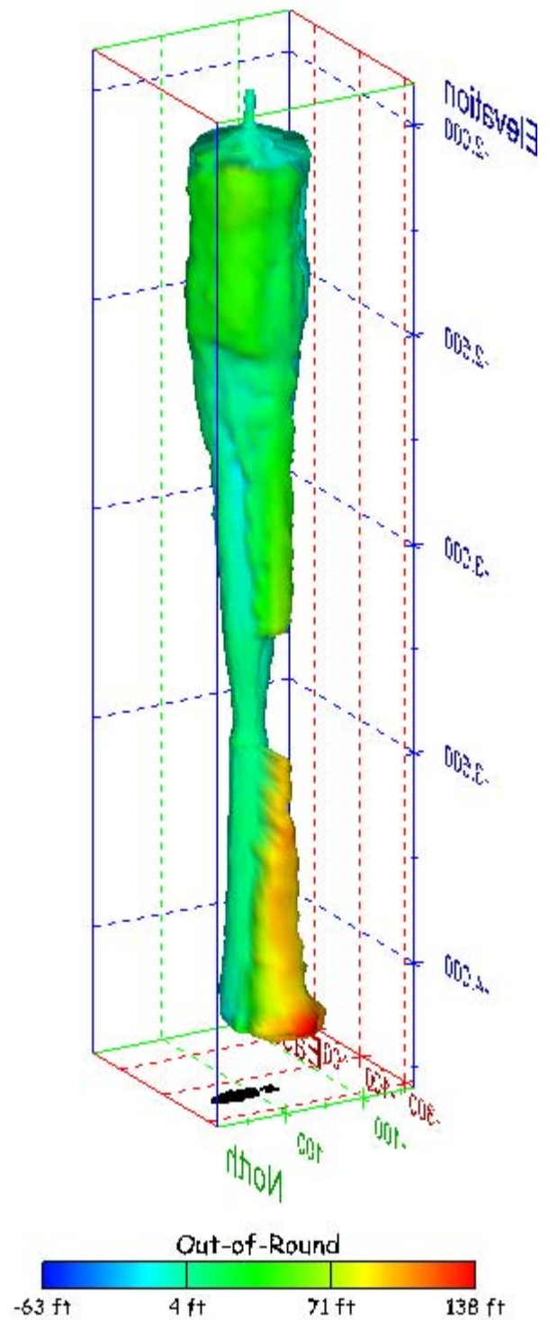
Figure 265. Sonar images of cavern BM-105, showing the geometry of the cavern colored by out-of-round distance. View from (a) azimuth 60°, elevation 20°; (b) azimuth 300°, elevation 20°.
