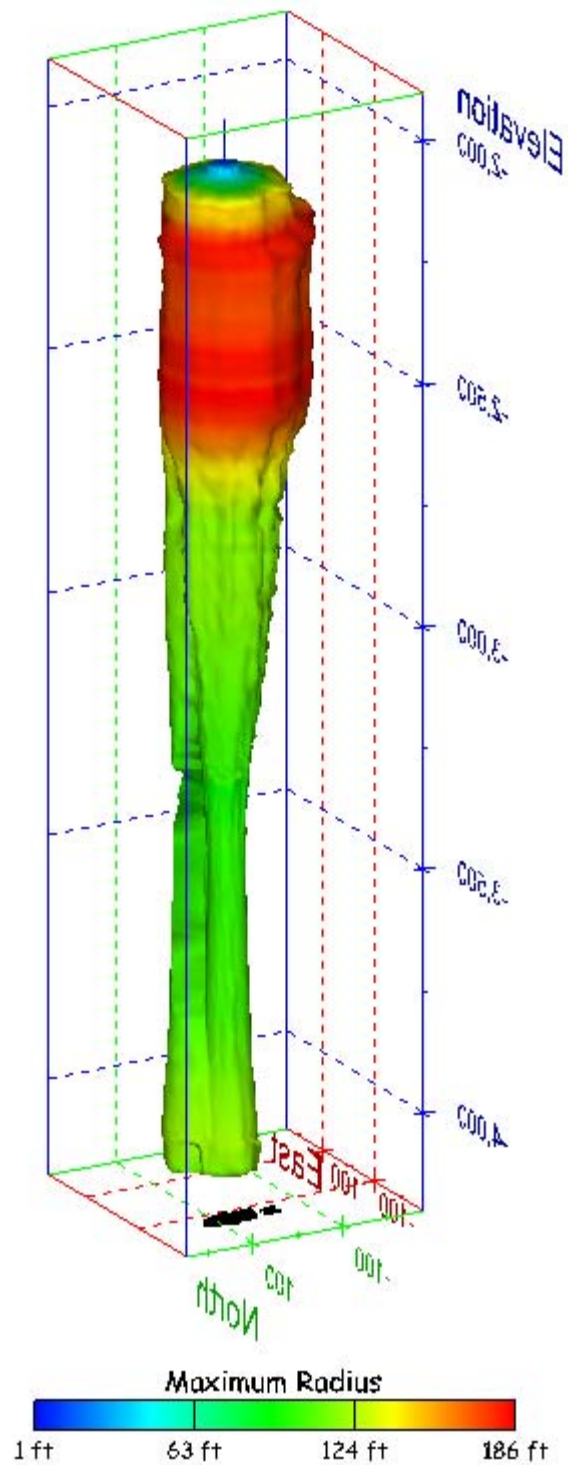
Figure 235. Sonar images of cavern BM-104, showing the geometry of the cavern colored by maximum radius. View from (a) azimuth 60°, elevation 20°; (b) azimuth 300°, elevation 20°.
