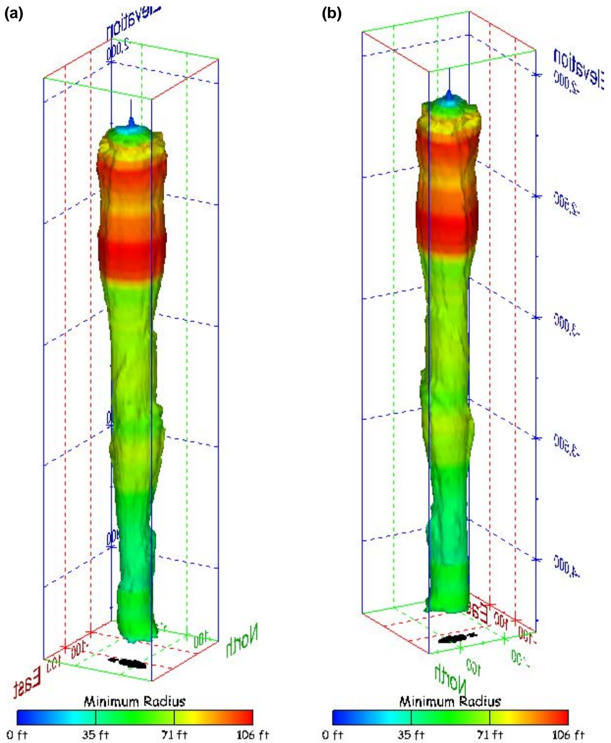
Figure 545. Sonar images of cavern BM-116, showing the geometry of the cavern colored by minimum radius. View from (a) azimuth 60°, elevation 20°; (b) azimuth 300°, elevation 20°.
