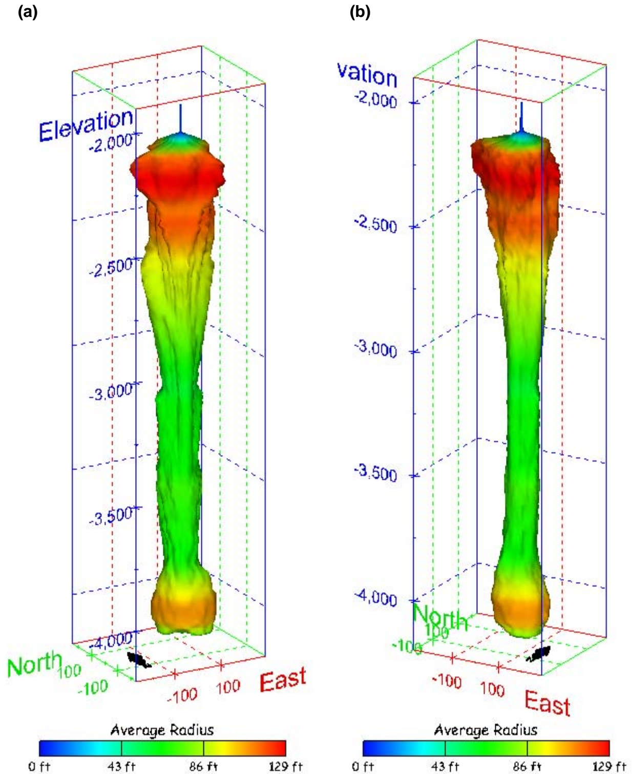
Figure 490. Sonar images of cavern BM-114, showing the geometry of the cavern colored by average radius. View from (a) azimuth 210°, elevation 20°; (b) azimuth 150°, elevation 20°.
