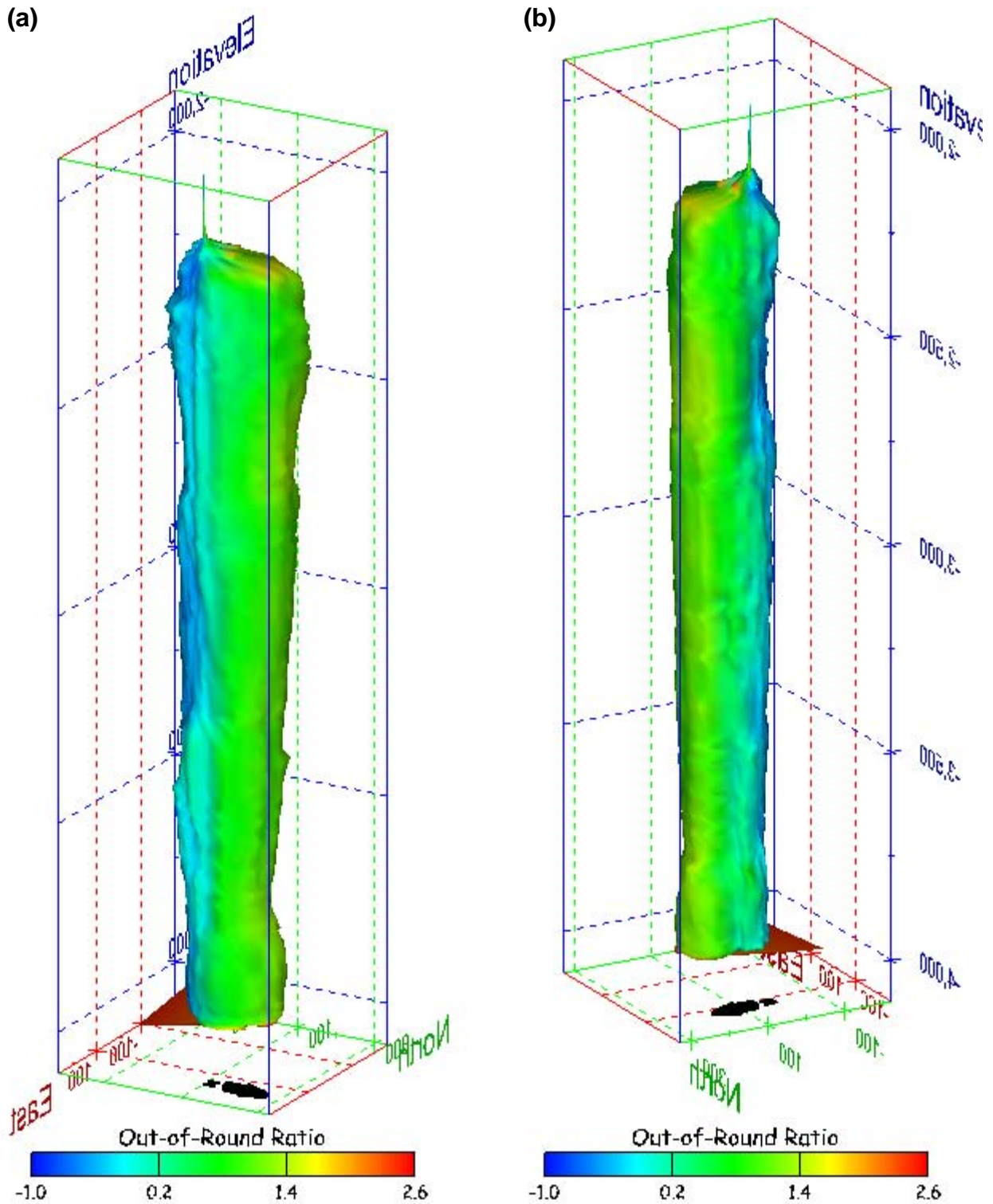
Figure 449. Sonar images of cavern BM-112, showing the geometry of the cavern colored by out-of-round ratio. View from (a) azimuth 60°, elevation 20°; (b) azimuth 300°, elevation 20°.
