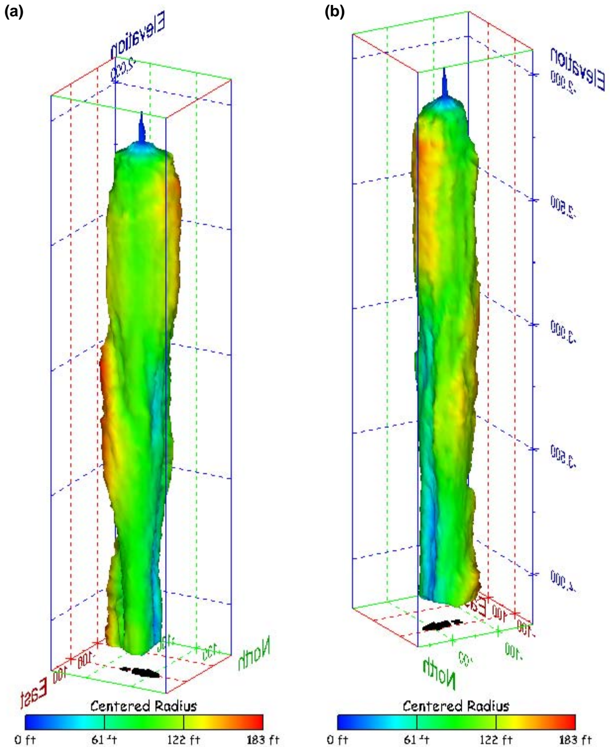
Figure 411. Sonar images of cavern BM-111, showing the geometry of the cavern colored by centered radius. View from (a) azimuth 60°, elevation 20°; (b) azimuth 300°, elevation 20°.
