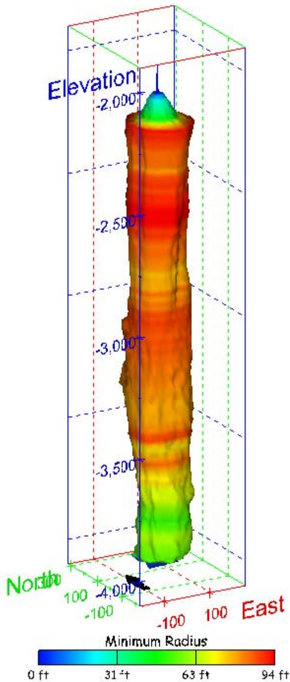
Figure 206. Sonar images of cavern BM-103, showing the geometry of the cavern colored by minimum radius. View from (a) azimuth 210°, elevation 20°; (b) azimuth 150°, elevation 20°.
