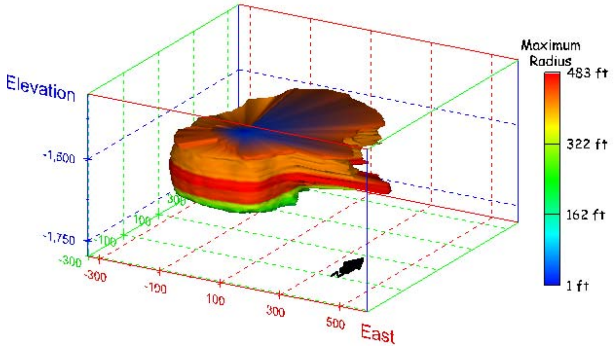
Figure 52. Sonar images of cavern BM-2, showing the geometry of the cavern colored by maximum radius. View from (a) azimuth 210°, elevation 20°; (b) azimuth 150°, elevation 20°.
