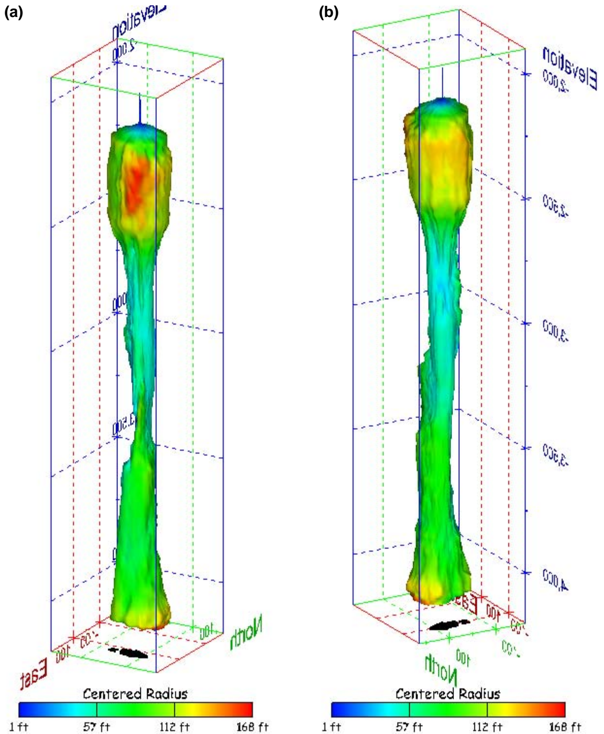
Figure 463. Sonar images of cavern BM-113, showing the geometry of the cavern colored by centered radius. View from (a) azimuth 60°, elevation 20°; (b) azimuth 300°, elevation 20°.
