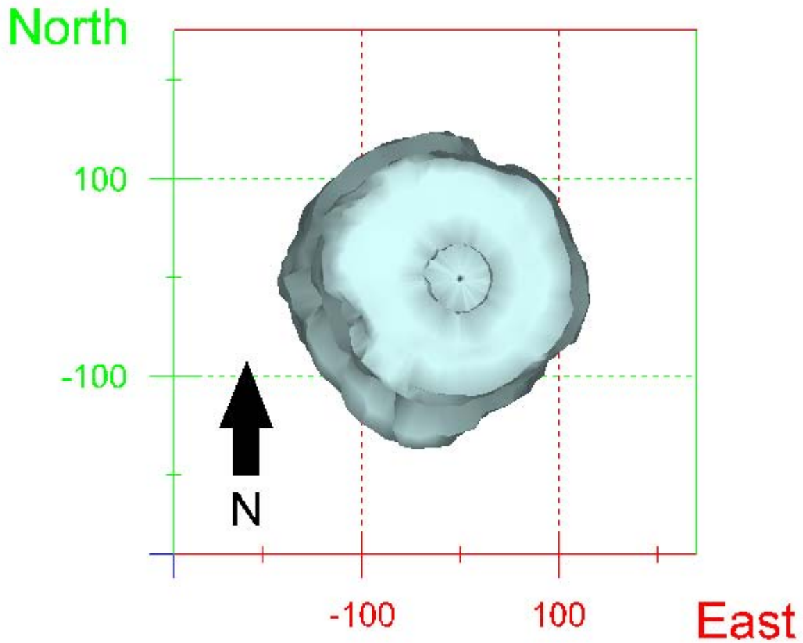
Figure 249. Map view sonar image of cavern BM-105, showing the basic geometry of the cavern. Grid squares represent 200 ft.
