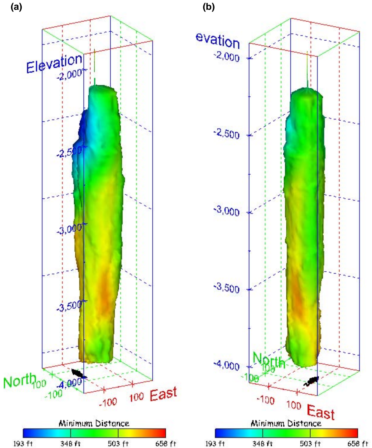
Figure 322. Sonar images of cavern BM-107, showing the geometry of the cavern colored by the minimum distance to the nearest neighboring cavern. View from (a) azimuth 210°, elevation 20°; (b) azimuth 150°, elevation 20°.
