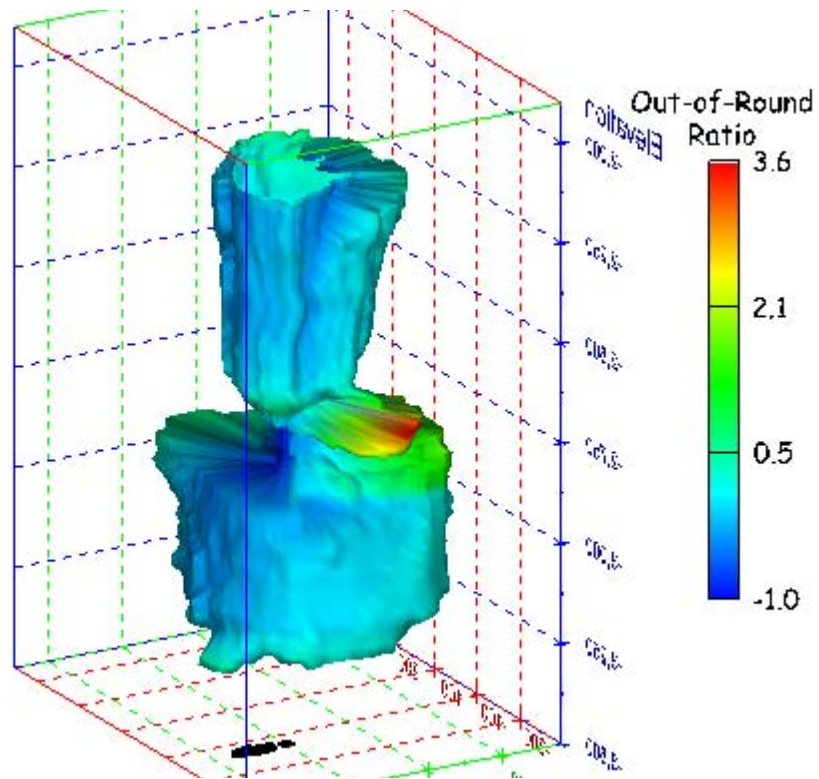
Figure 137. Sonar images of cavern BM-5, showing the geometry of the cavern colored by out-of-round ratio. View from (a) azimuth 60°, elevation 20°; (b) azimuth 300°, elevation 20°.
