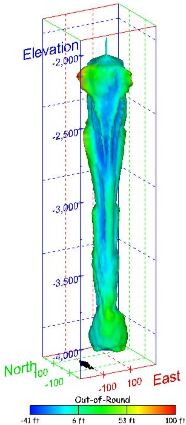
Figure 498. Sonar images of cavern BM-114, showing the geometry of the cavern colored by out-of-round distance. View from (a) azimuth 210°, elevation 20°; (b) azimuth 150°, elevation 20°.
