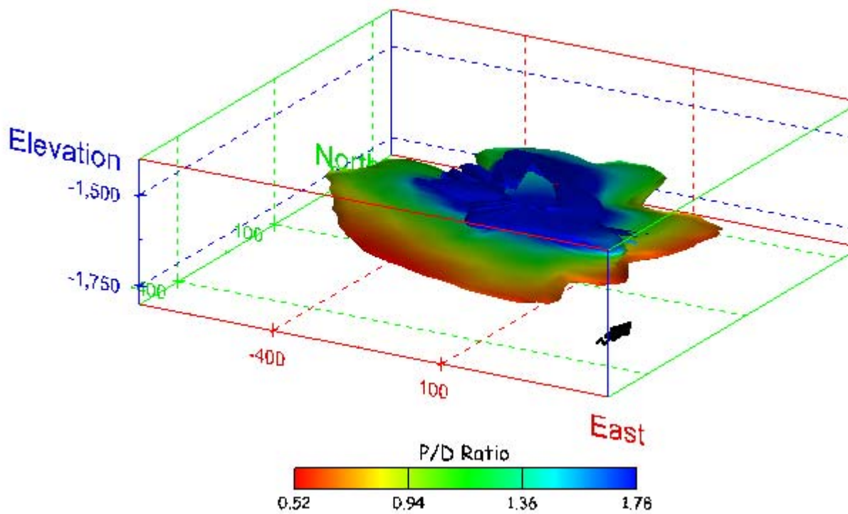
Figure 90. Sonar images of cavern BM-3, showing the geometry of the cavern colored by three-dimensional pillar-to-diameter ratio. View from (a) azimuth 210°, elevation 20°; (b) azimuth 150°, elevation 20°.
