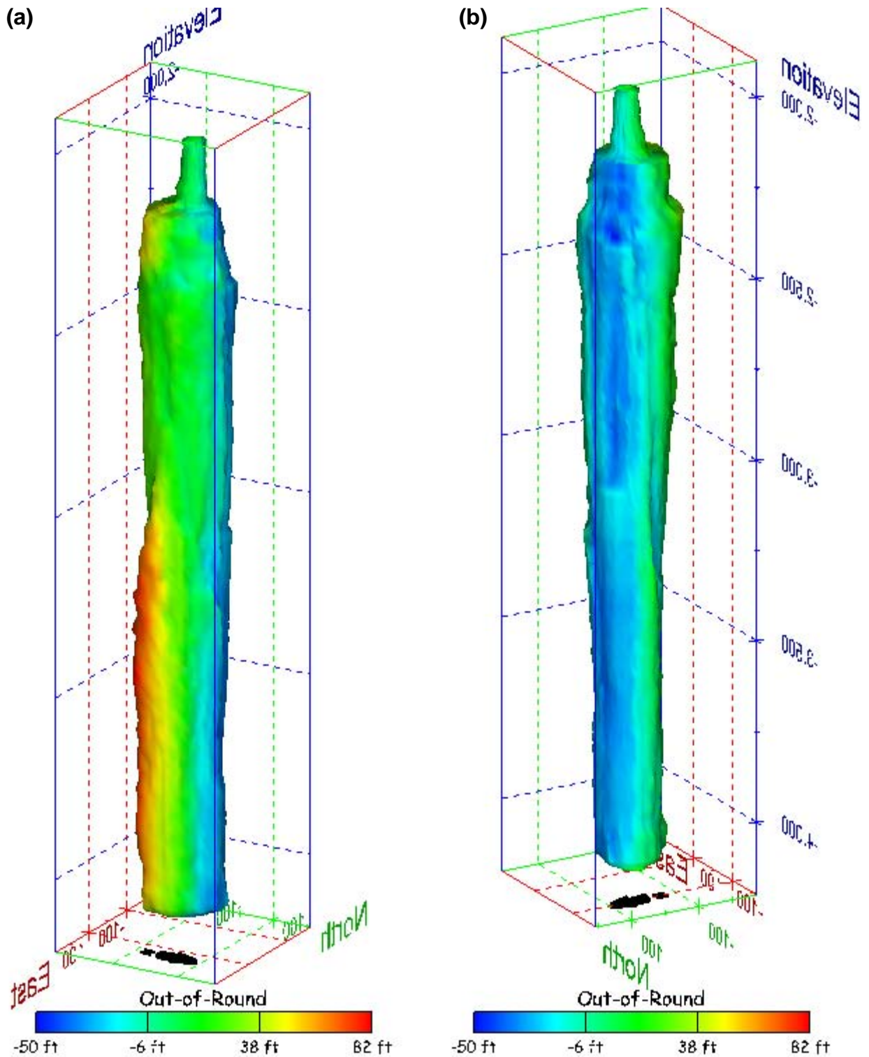
Figure 161. Sonar images of cavern BM-101, showing the geometry of the cavern colored by out-of-round distance. View from (a) azimuth 60°, elevation 20°; (b) azimuth 300°, elevation 20°.
