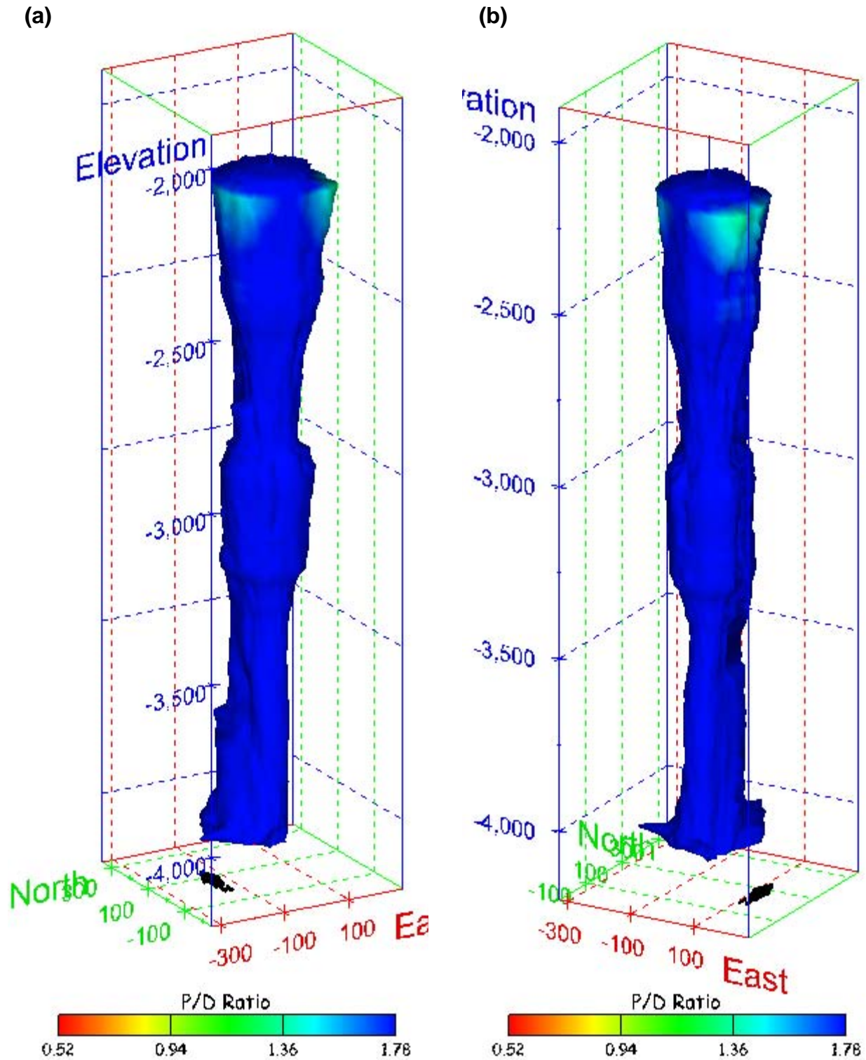
Figure 376. Sonar images of cavern BM-109, showing the geometry of the cavern colored by three-dimensional pillar-to-diameter ratio. View from (a) azimuth 210°, elevation 20°; (b) azimuth 150°, elevation 20°.
