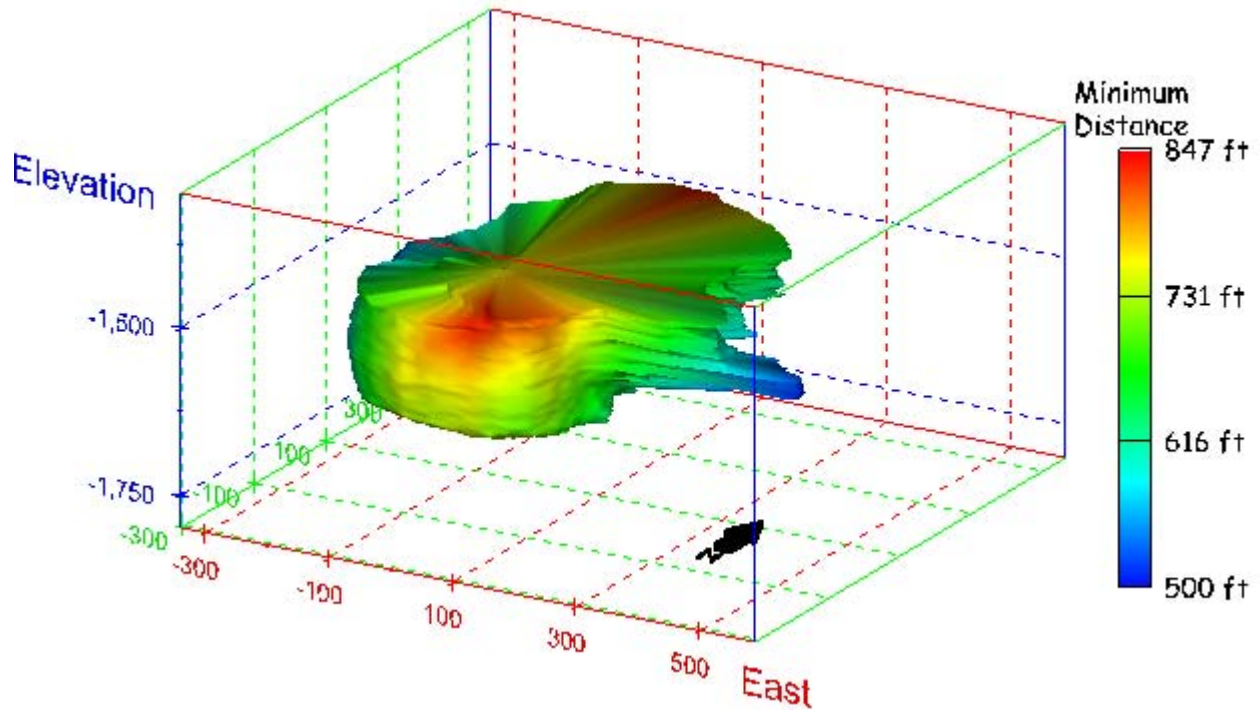
Figure 62. Sonar images of cavern BM-2, showing the geometry of the cavern colored by the minimum distance to the nearest neighboring cavern. View from (a) azimuth 210°, elevation 20°; (b) azimuth 150°, elevation 20°.
