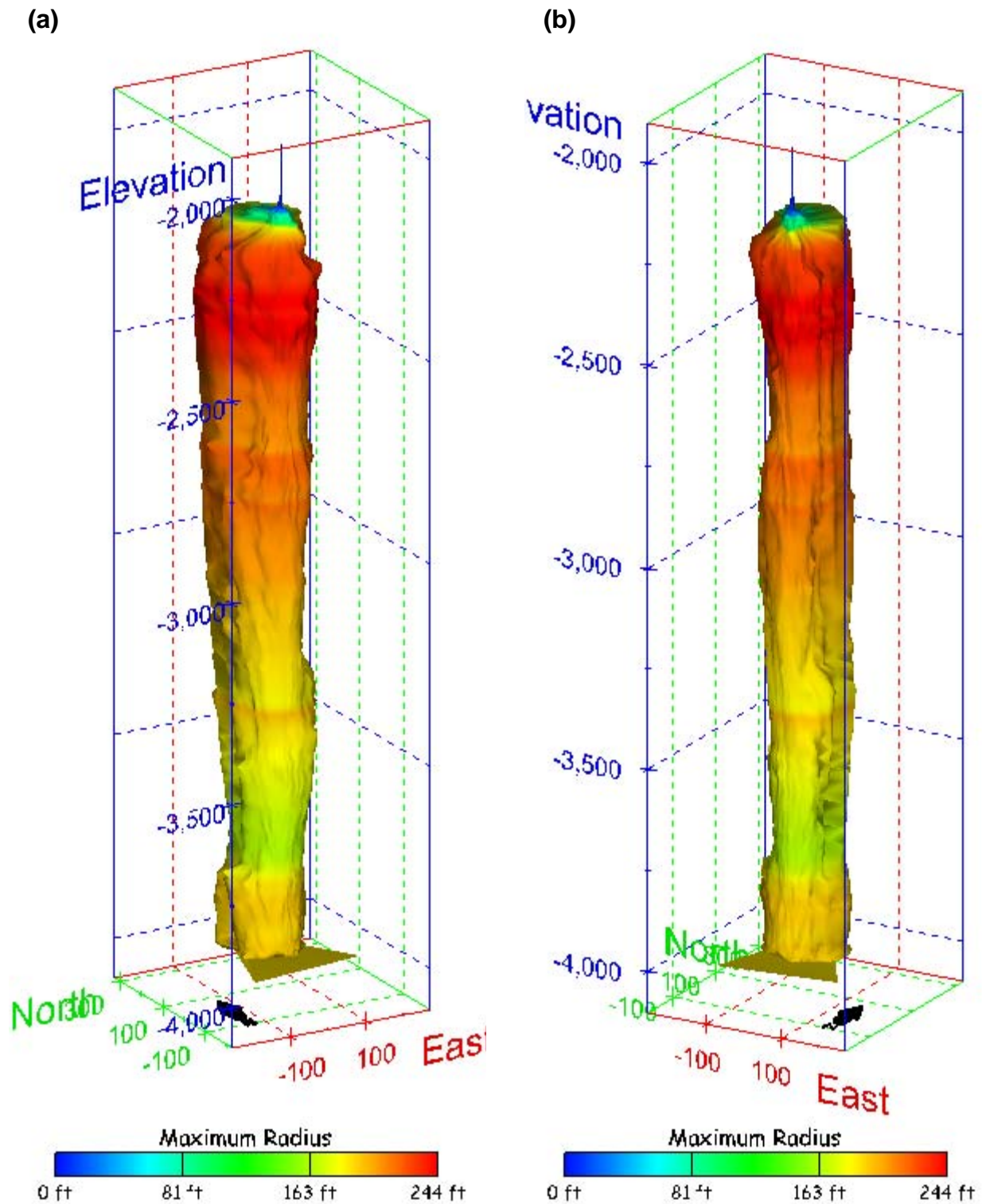
Figure 442. Sonar images of cavern BM-112, showing the geometry of the cavern colored by maximum radius. View from (a) azimuth 210°, elevation 20°; (b) azimuth 150°, elevation 20°.
