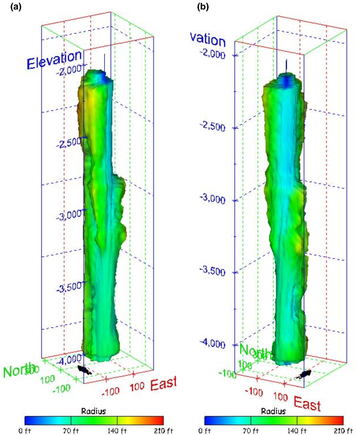
Figure 330. Sonar images of cavern BM-108, showing the geometry of the cavern colored by measured radius. View from (a) azimuth 210°, elevation 20°; (b) azimuth 150°, elevation 20°.
