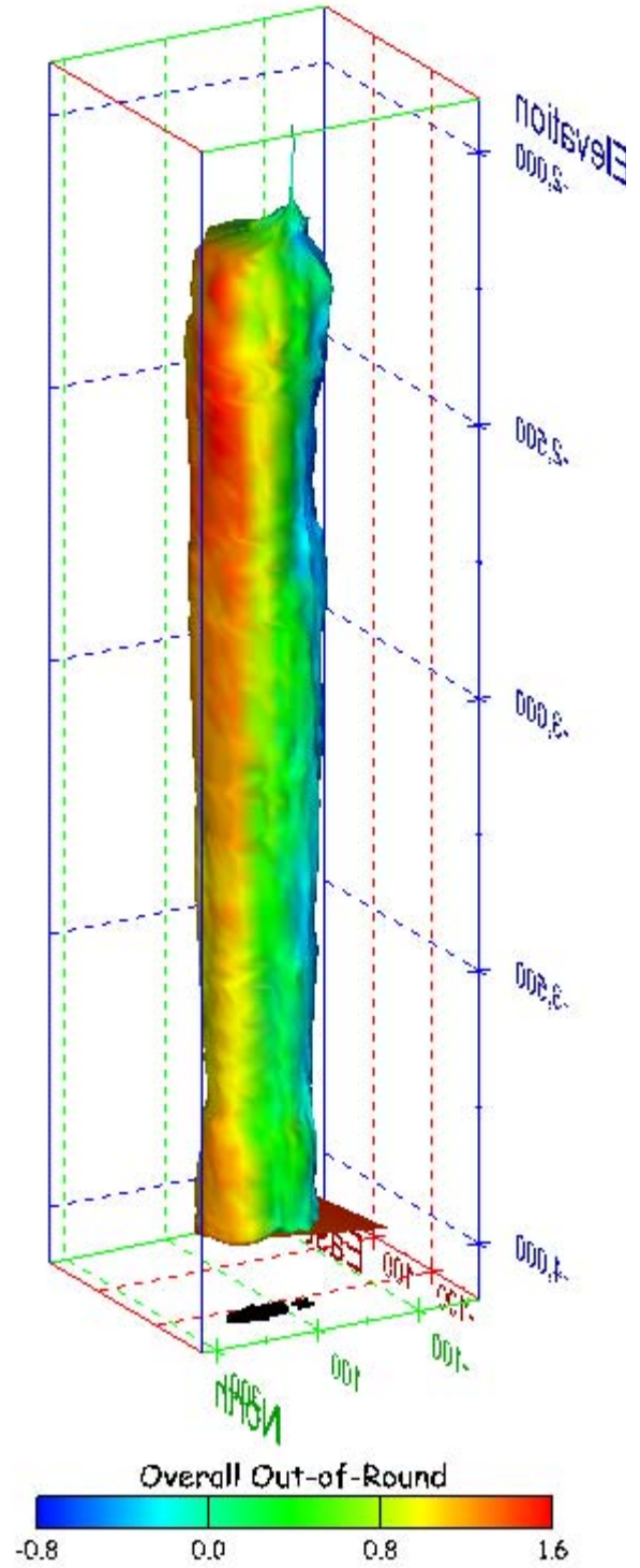
Figure 451. Sonar images of cavern BM-112, showing the geometry of the cavern colored by overall out-of-round ratio. View from (a) azimuth 60°, elevation 20°; (b) azimuth 300°, elevation 20°.
