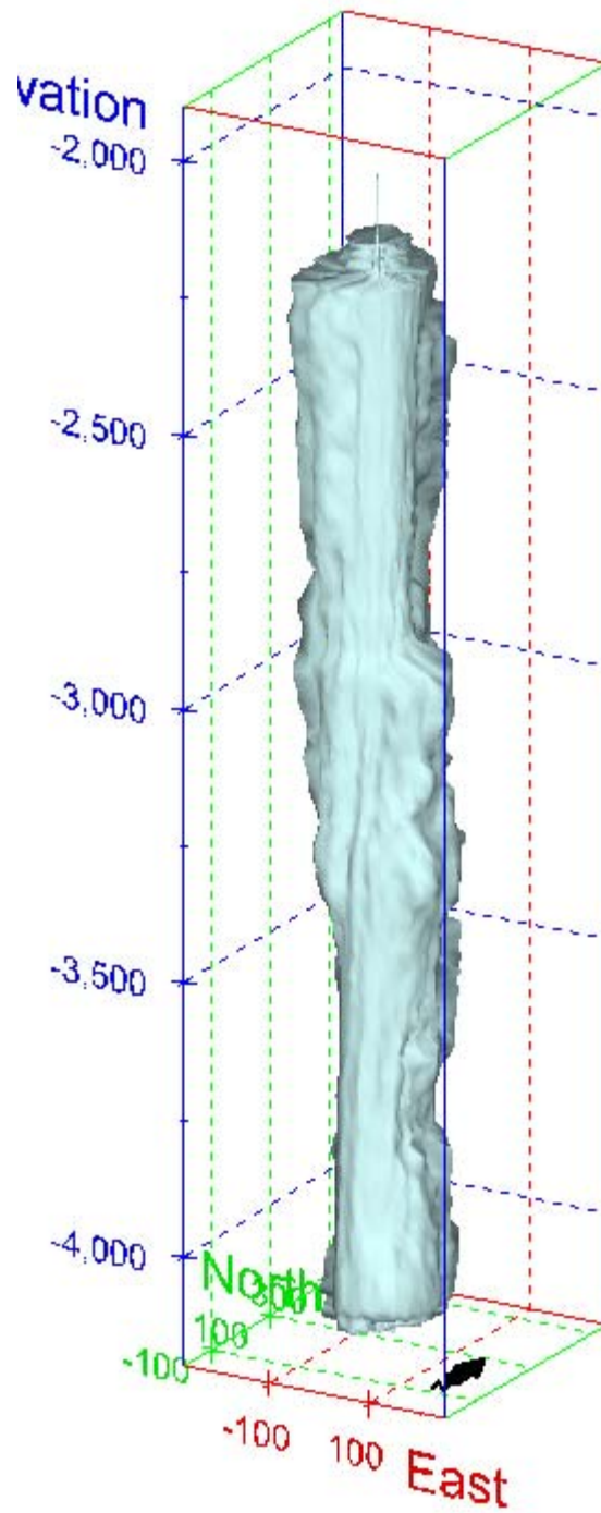
Figure 328. Sonar images of cavern BM-108, showing the basic geometric shape of the cavern. View from (a) azimuth 210°, elevation 20°; (b) azimuth 150°, elevation 20°.
