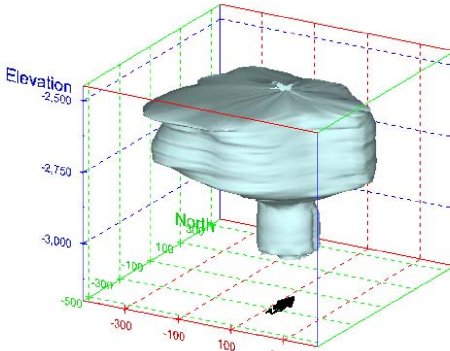
Figure 94. Sonar images of cavern BM-4, showing the basic geometric shape of the cavern. View from (a) azimuth 210°, elevation 20°; (b) azimuth 150°, elevation 20°.
