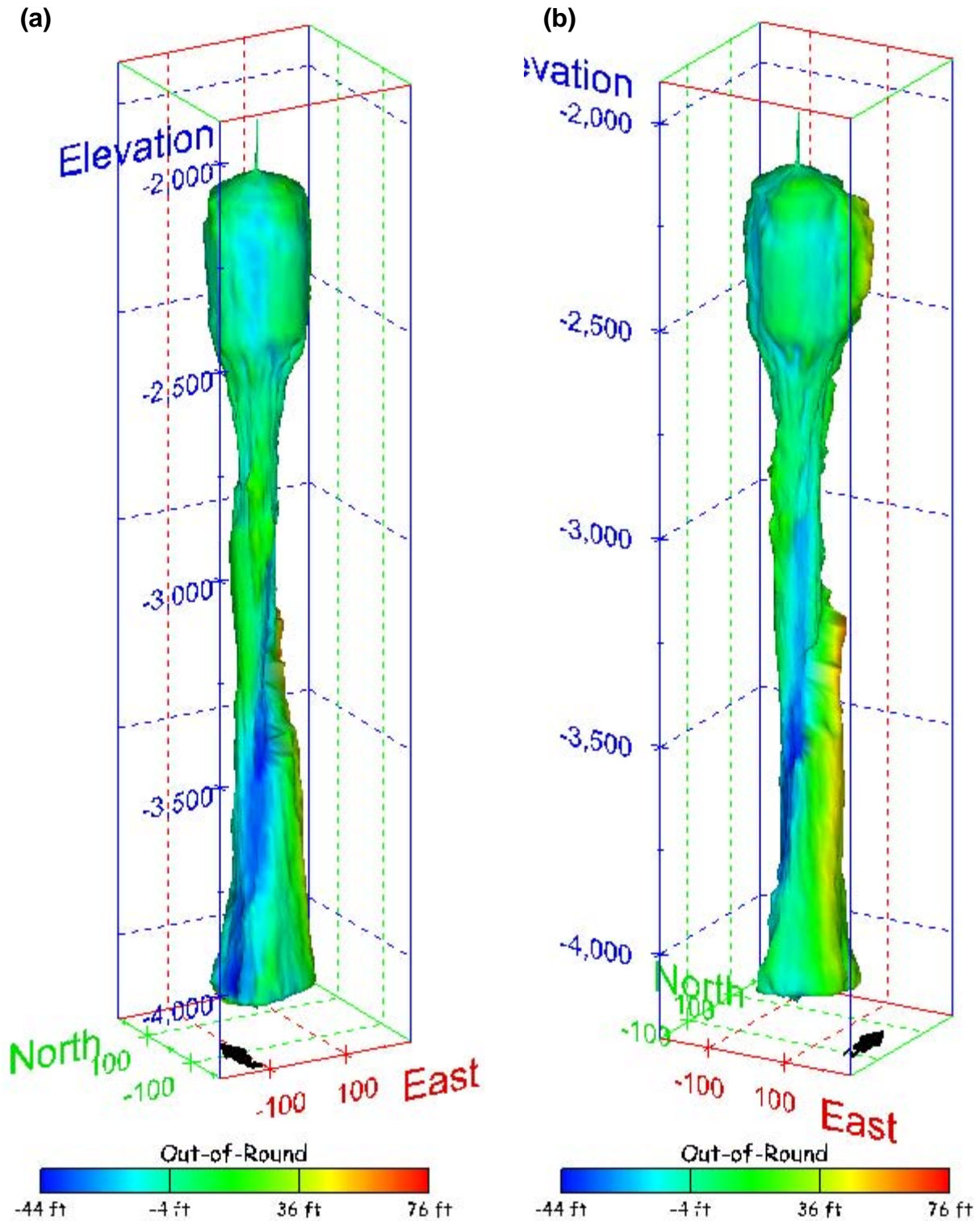
Figure 472. Sonar images of cavern BM-113, showing the geometry of the cavern colored by out-of-round distance. View from (a) azimuth 210°, elevation 20°; (b) azimuth 150°, elevation 20°.
