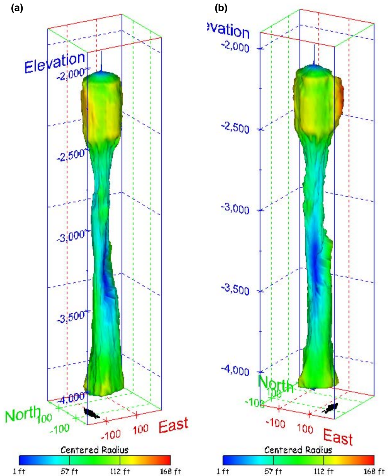
Figure 462. Sonar images of cavern BM-113, showing the geometry of the cavern colored by centered radius. View from (a) azimuth 210°, elevation 20°; (b) azimuth 150°, elevation 20°.
