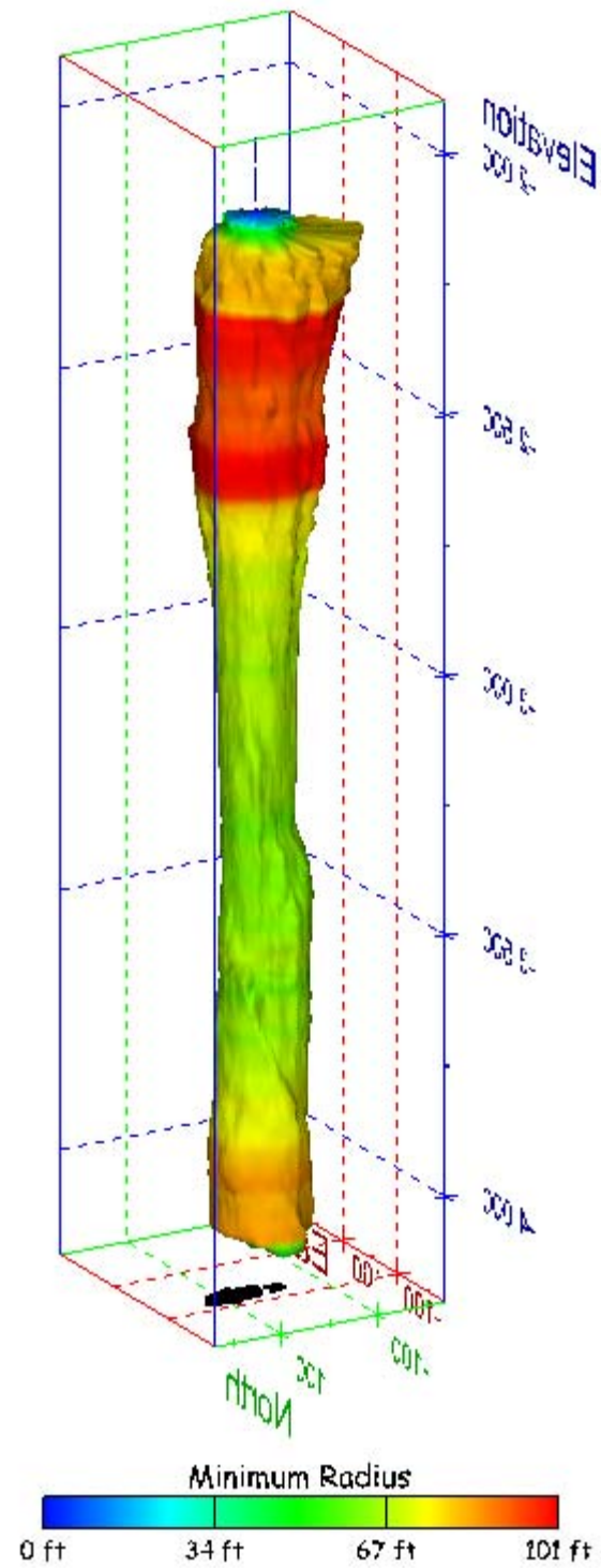
Figure 519. Sonar images of cavern BM-115, showing the geometry of the cavern colored by minimum radius. View from (a) azimuth 60°, elevation 20°; (b) azimuth 300°, elevation 20°.
