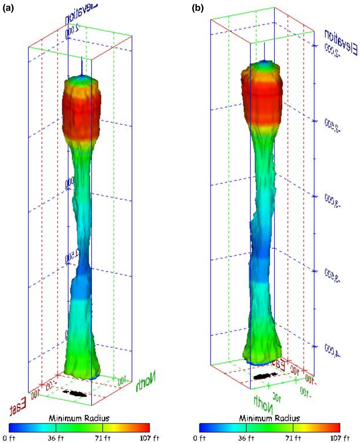
Figure 467. Sonar images of cavern BM-113, showing the geometry of the cavern colored by minimum radius. View from (a) azimuth 60°, elevation 20°; (b) azimuth 300°, elevation 20°.
