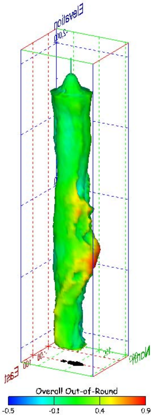
Figure 217. Sonar images of cavern BM-103, showing the geometry of the cavern colored by overall out-of-round ratio. View from (a) azimuth 60°, elevation 20°; (b) azimuth 300°, elevation 20°.
