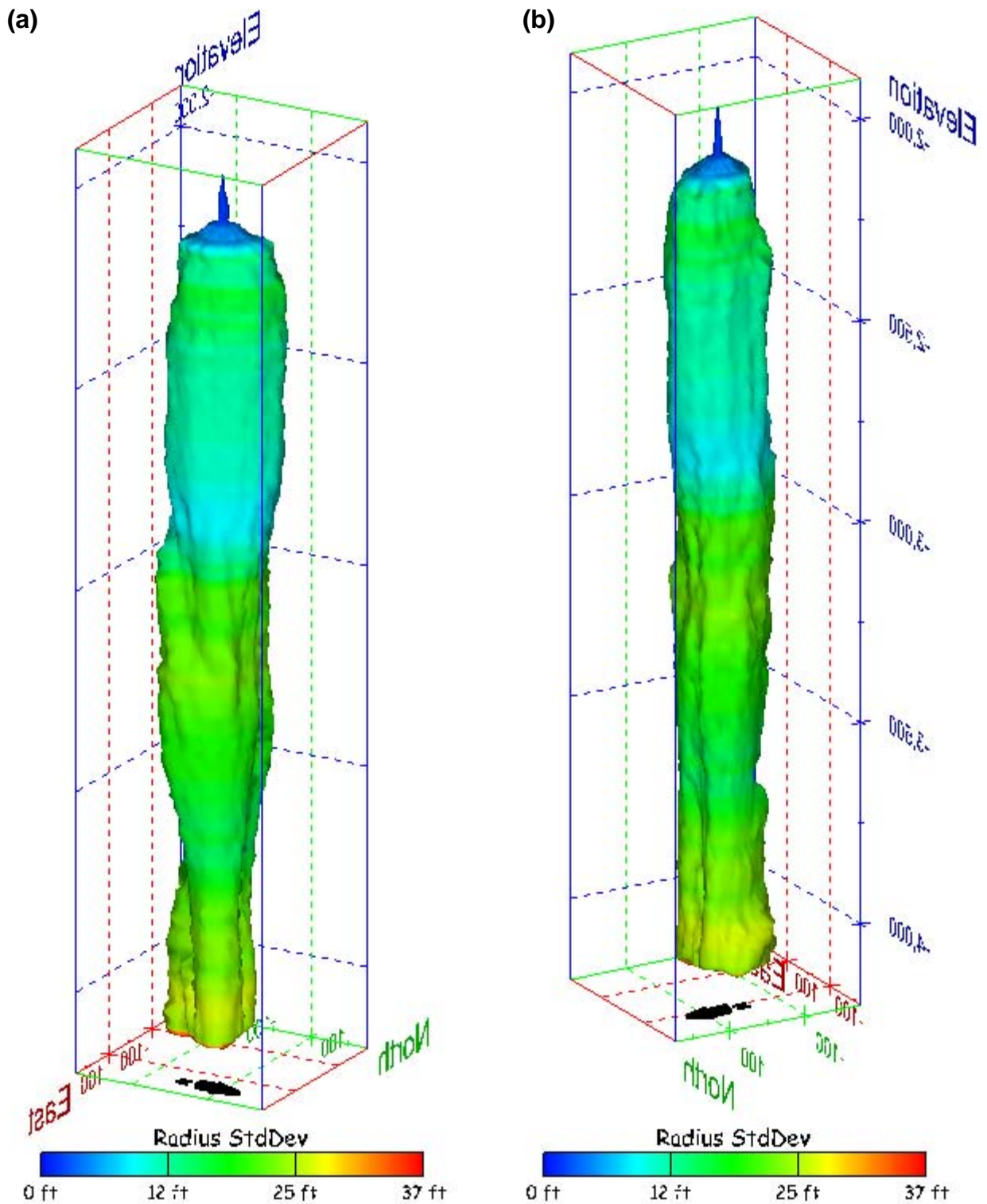
Figure 419. Sonar images of cavern BM-111, showing the geometry of the cavern colored by radius standard deviation. View from (a) azimuth 60°, elevation 20°; (b) azimuth 300°, elevation 20°.
