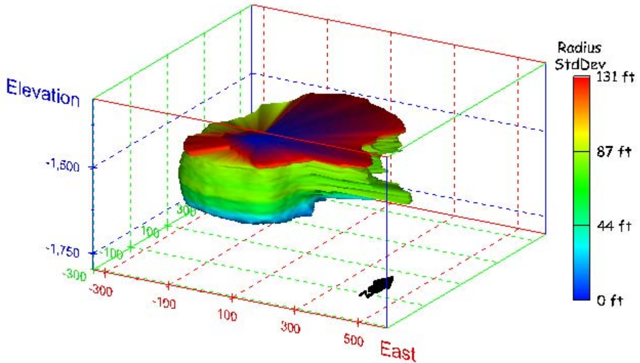
Figure 54. Sonar images of cavern BM-2, showing the geometry of the cavern colored by radius standard deviation. View from (a) azimuth 210°, elevation 20°; (b) azimuth 150°, elevation 20°.
