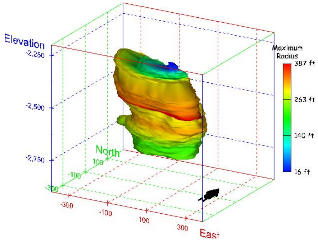
Figure 26. Sonar images of cavern BM-1, showing the geometry of the cavern colored by maximum radius. View from (a) azimuth 210°, elevation 20°; (b) azimuth 150°, elevation 20°.
