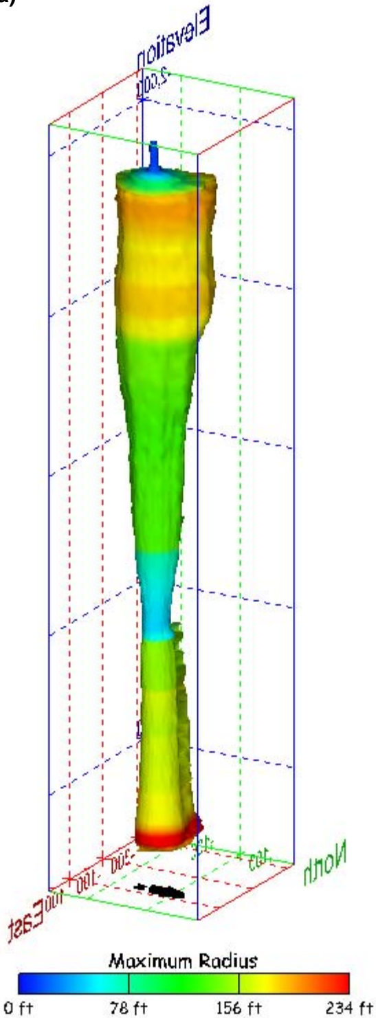
Figure 261. Sonar images of cavern BM-105, showing the geometry of the cavern colored by maximum radius. View from (a) azimuth 60°, elevation 20°; (b) azimuth 300°, elevation 20°.
