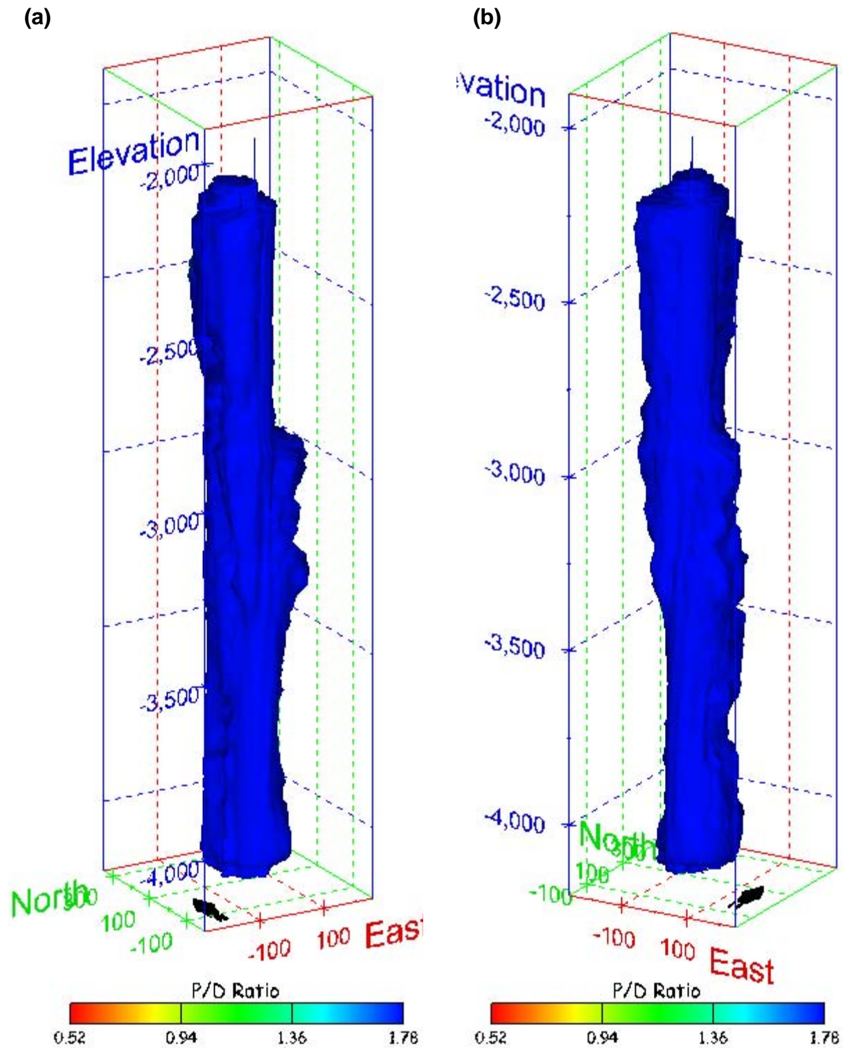
Figure 350. Sonar images of cavern BM-108, showing the geometry of the cavern colored by three-dimensional pillar-to-diameter ratio. View from (a) azimuth 210°, elevation 20°; (b) azimuth 150°, elevation 20°.
