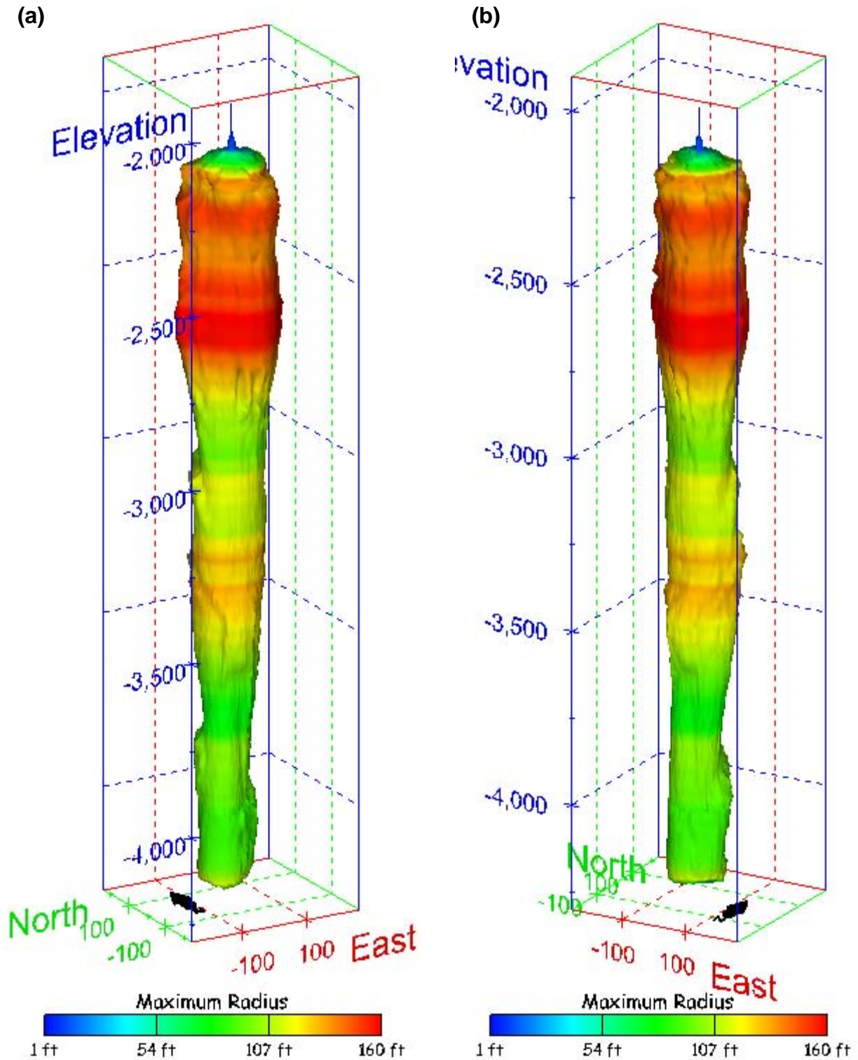
Figure 546. Sonar images of cavern BM-116, showing the geometry of the cavern colored by maximum radius. View from (a) azimuth 210°, elevation 20°; (b) azimuth 150°, elevation 20°.
