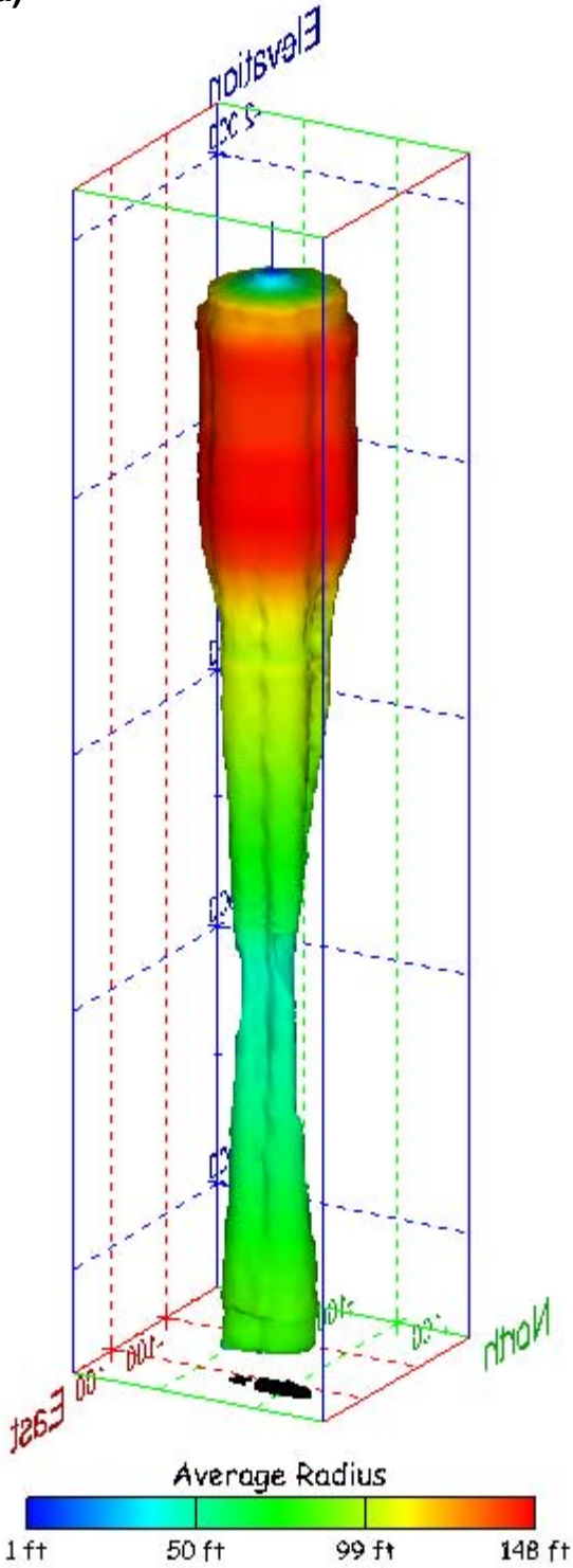
Figure 231. Sonar images of cavern BM-104, showing the geometry of the cavern colored by average radius. View from (a) azimuth 60°, elevation 20°; (b) azimuth 300°, elevation 20°.
