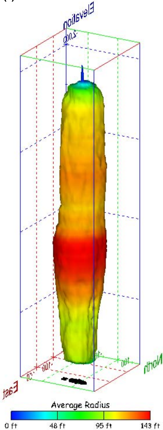
Figure 283. Sonar images of cavern BM-106, showing the geometry of the cavern colored by average radius. View from (a) azimuth 60°, elevation 20°; (b) azimuth 300°, elevation 20°.
