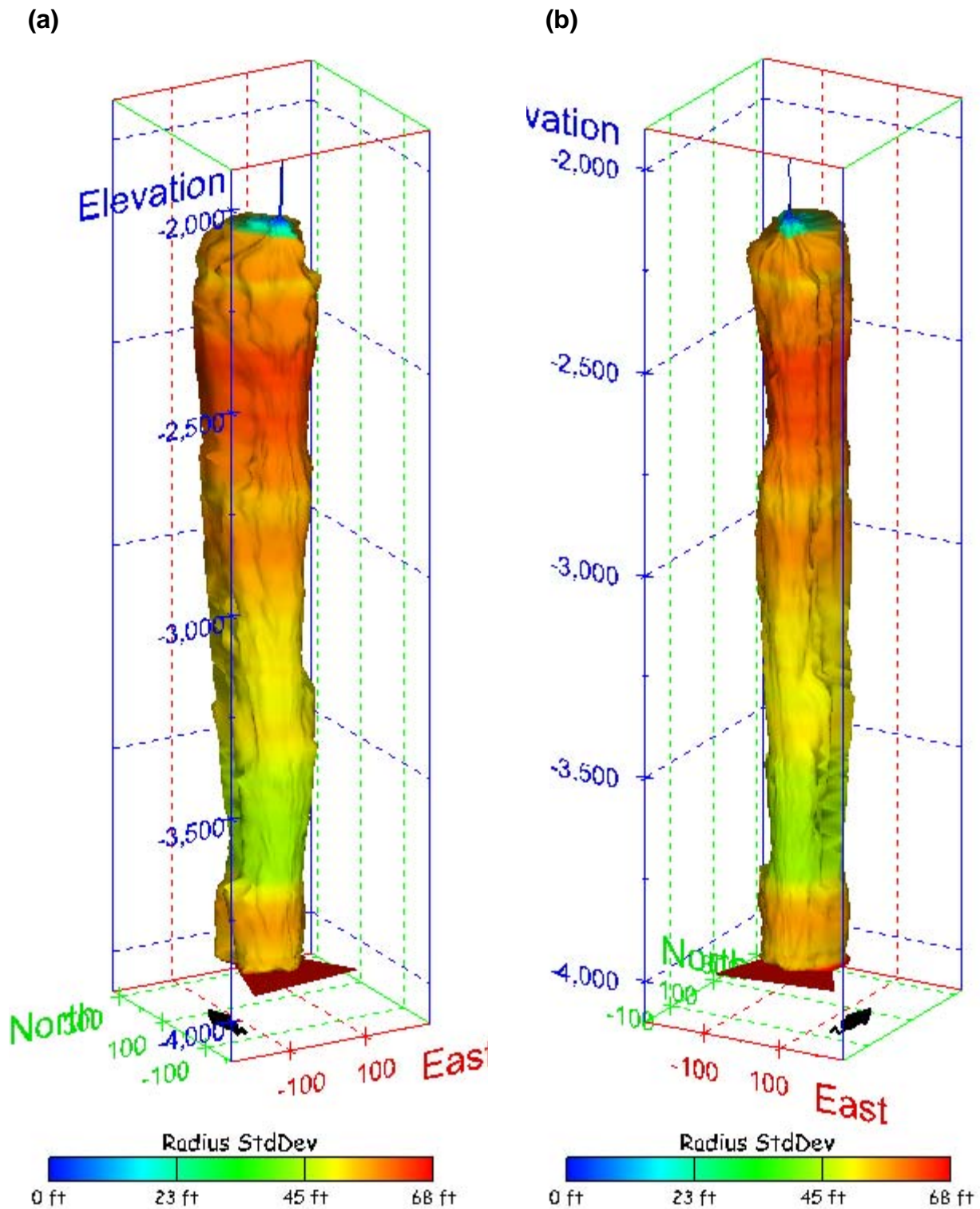
Figure 444. Sonar images of cavern BM-112, showing the geometry of the cavern colored by radius standard deviation. View from (a) azimuth 210°, elevation 20°; (b) azimuth 150°, elevation 20°.
