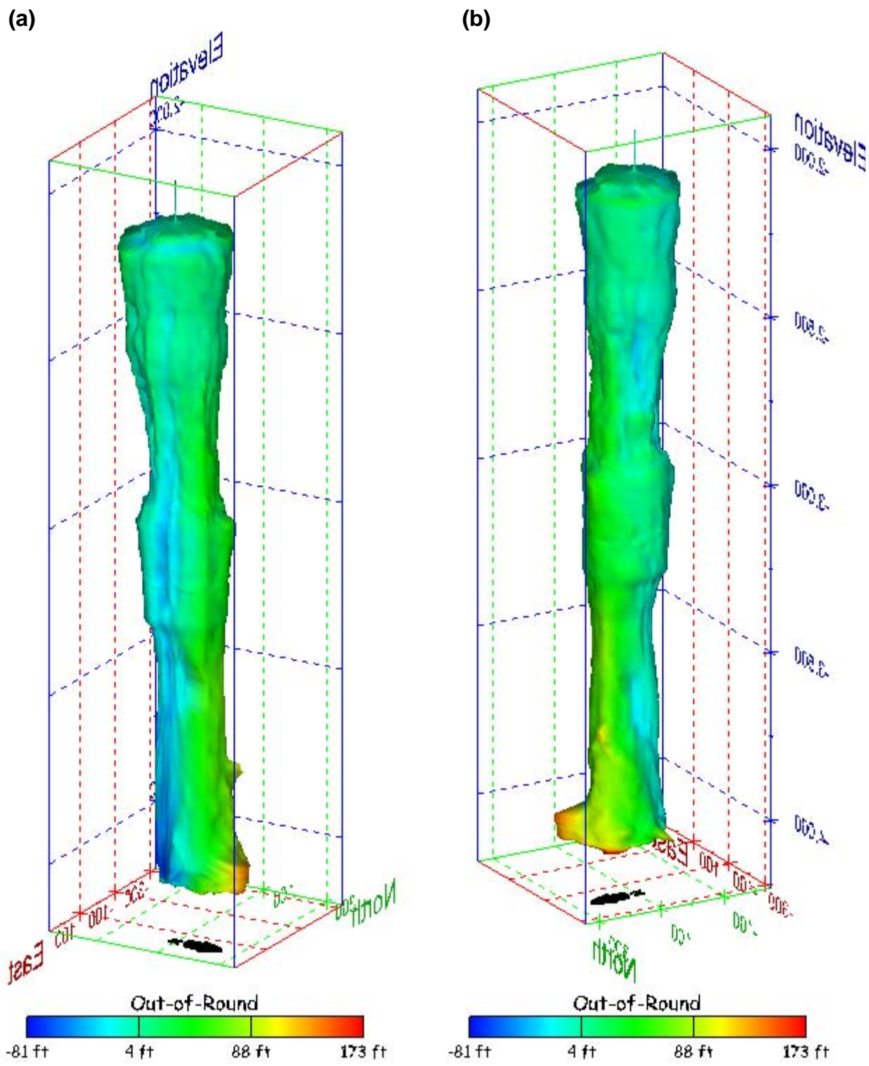
Figure 369. Sonar images of cavern BM-109, showing the geometry of the cavern colored by out-of-round distance. View from (a) azimuth 60°, elevation 20°; (b) azimuth 300°, elevation 20°.
