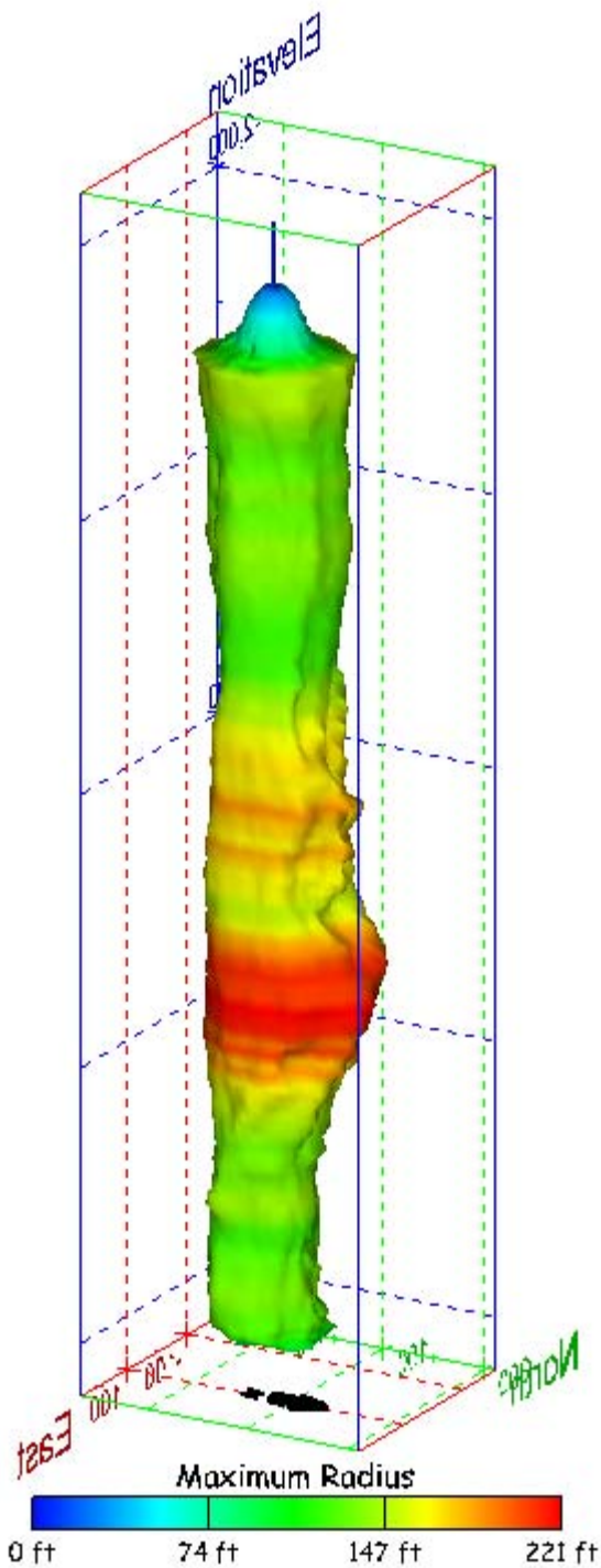
Figure 209. Sonar images of cavern BM-103, showing the geometry of the cavern colored by maximum radius. View from (a) azimuth 60°, elevation 20°; (b) azimuth 300°, elevation 20°.
