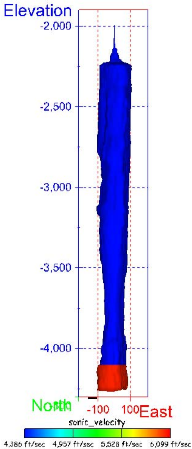
Figure 196. Sonar image of cavern BM-102, showing the geometry of the cavern colored by the reported velocity of sound on the survey date of May 2003. View from (a) due south, elevation zero.
