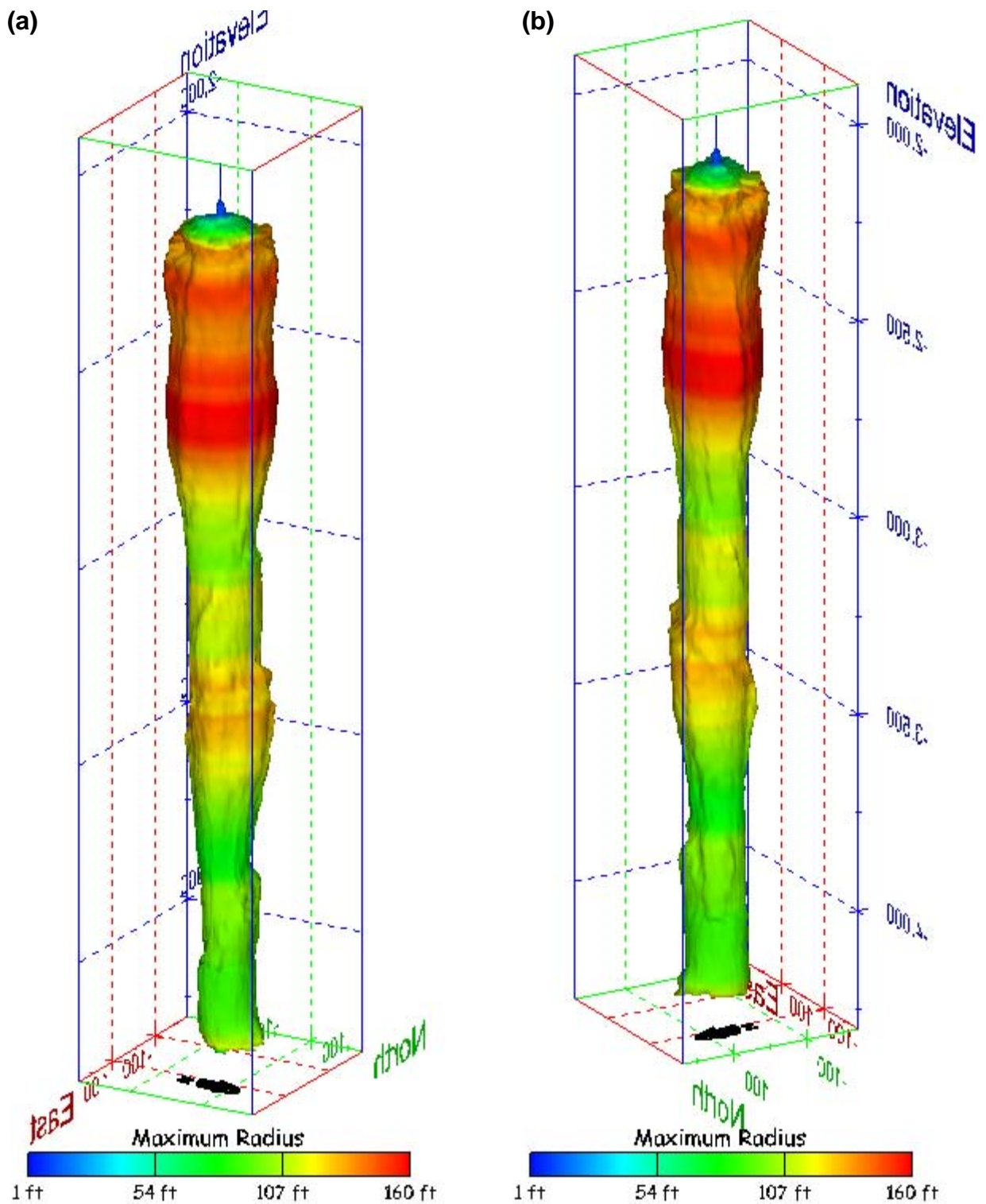
Figure 547. Sonar images of cavern BM-116, showing the geometry of the cavern colored by maximum radius. View from (a) azimuth 60°, elevation 20°; (b) azimuth 300°, elevation 20°.
