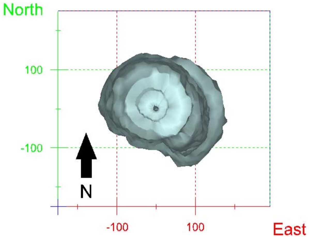
Figure 275. Map view sonar image of cavern BM-106, showing the basic geometry of the cavern. Grid squares represent 200 ft.
