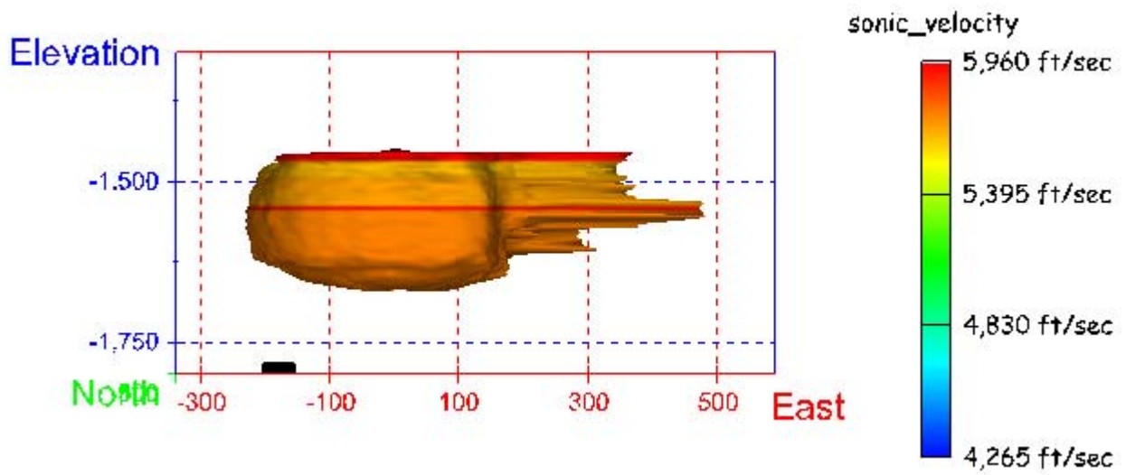
Figure 66. Sonar image of cavern BM-2, showing the geometry of the cavern colored by the reported velocity of sound on the survey date of December 1995. View from (a) due south, elevation zero.
