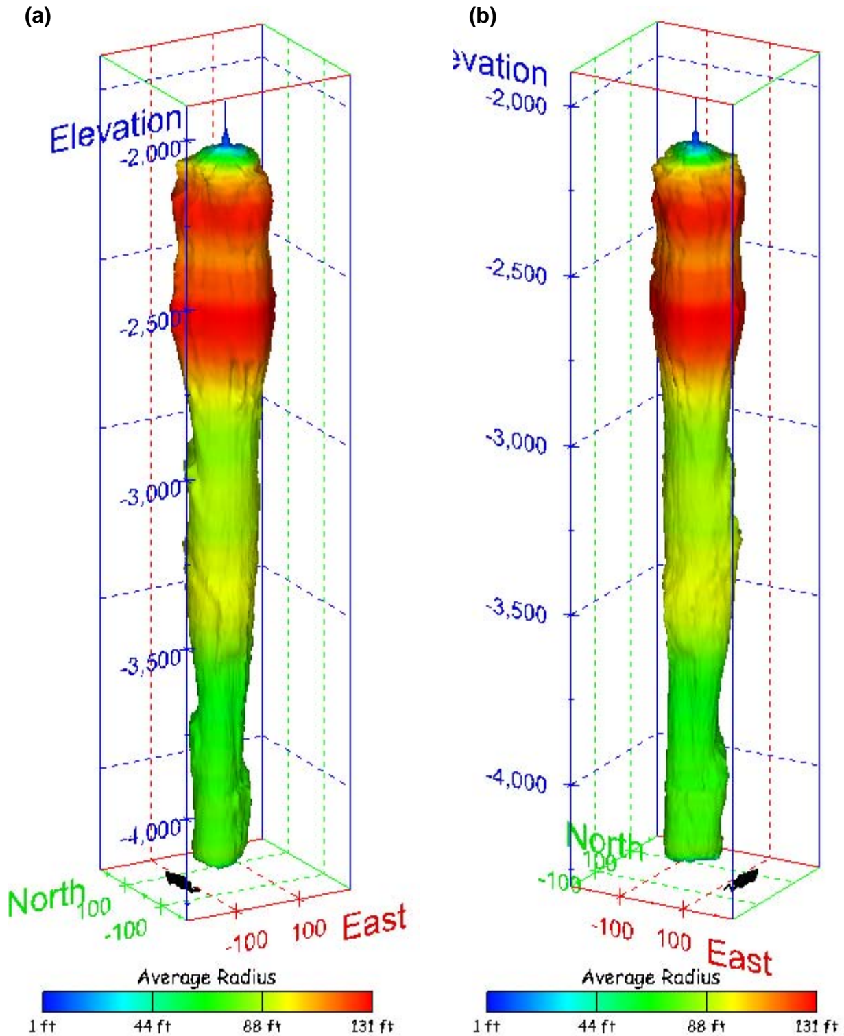
Figure 542. Sonar images of cavern BM-116, showing the geometry of the cavern colored by average radius. View from (a) azimuth 210°, elevation 20°; (b) azimuth 150°, elevation 20°.
