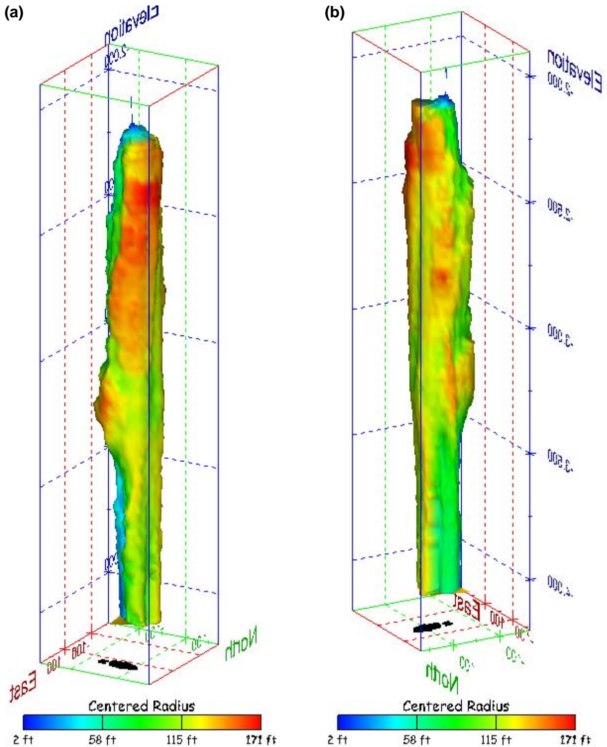
Figure 385. Sonar images of cavern BM-110, showing the geometry of the cavern colored by centered radius. View from (a) azimuth 60°, elevation 20°; (b) azimuth 300°, elevation 20°.
