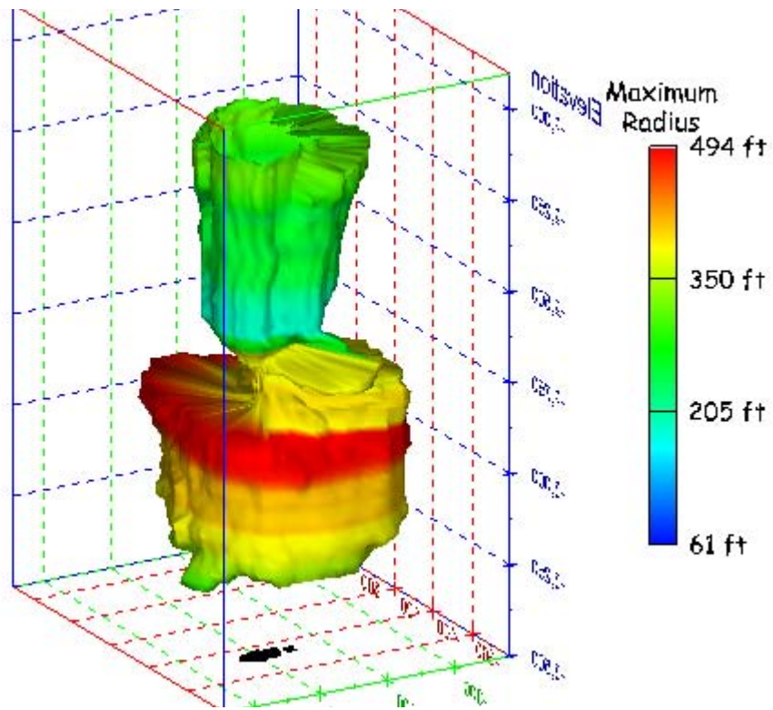
Figure 131. Sonar images of cavern BM-5, showing the geometry of the cavern colored by maximum radius. View from (a) azimuth 60°, elevation 20°; (b) azimuth 300°, elevation 20°.
