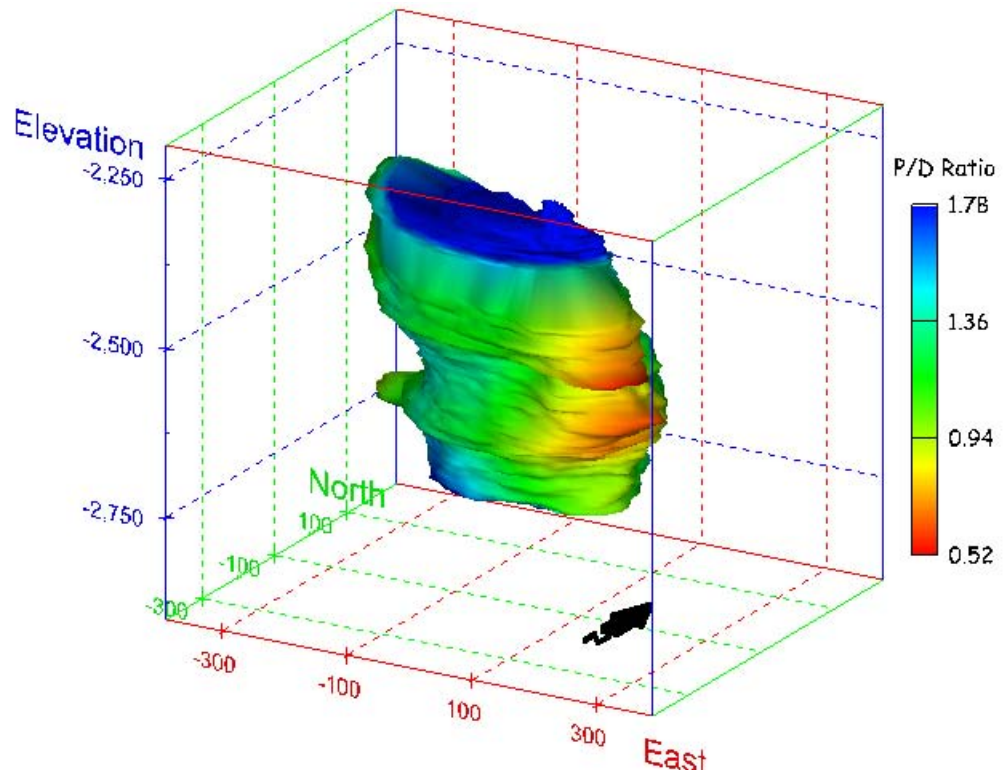
Figure 38. Sonar images of cavern BM-1, showing the geometry of the cavern colored by three-dimensional pillar-to-diameter ratio. View from (a) azimuth 210°, elevation 20°; (b) azimuth 150°, elevation 20°.
