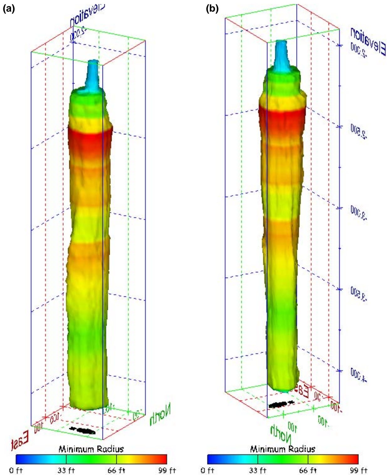
Figure 155. Sonar images of cavern BM-101, showing the geometry of the cavern colored by minimum radius. View from (a) azimuth 60°, elevation 20°; (b) azimuth 300°, elevation 20°.
