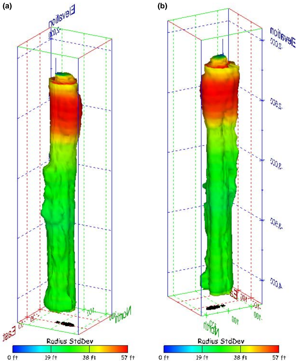
Figure 341. Sonar images of cavern BM-108, showing the geometry of the cavern colored by radius standard deviation. View from (a) azimuth 60°, elevation 20°; (b) azimuth 300°, elevation 20°.
