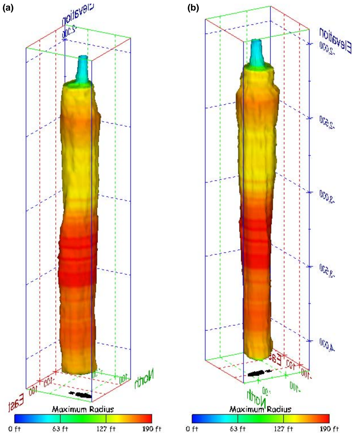
Figure 157. Sonar images of cavern BM-101, showing the geometry of the cavern colored by maximum radius. View from (a) azimuth 60°, elevation 20°; (b) azimuth 300°, elevation 20°.
