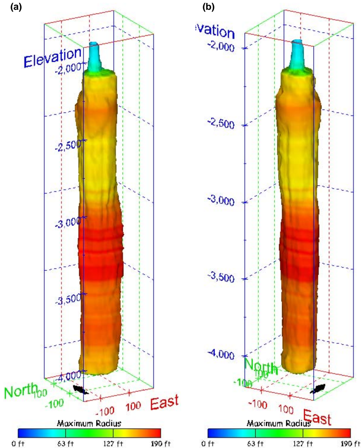
Figure 156. Sonar images of cavern BM-101, showing the geometry of the cavern colored by maximum radius. View from (a) azimuth 210°, elevation 20°; (b) azimuth 150°, elevation 20°.
