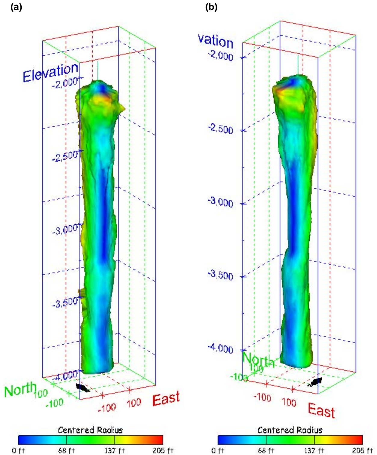
Figure 514. Sonar images of cavern BM-115, showing the geometry of the cavern colored by centered radius. View from (a) azimuth 210°, elevation 20°; (b) azimuth 150°, elevation 20°.
