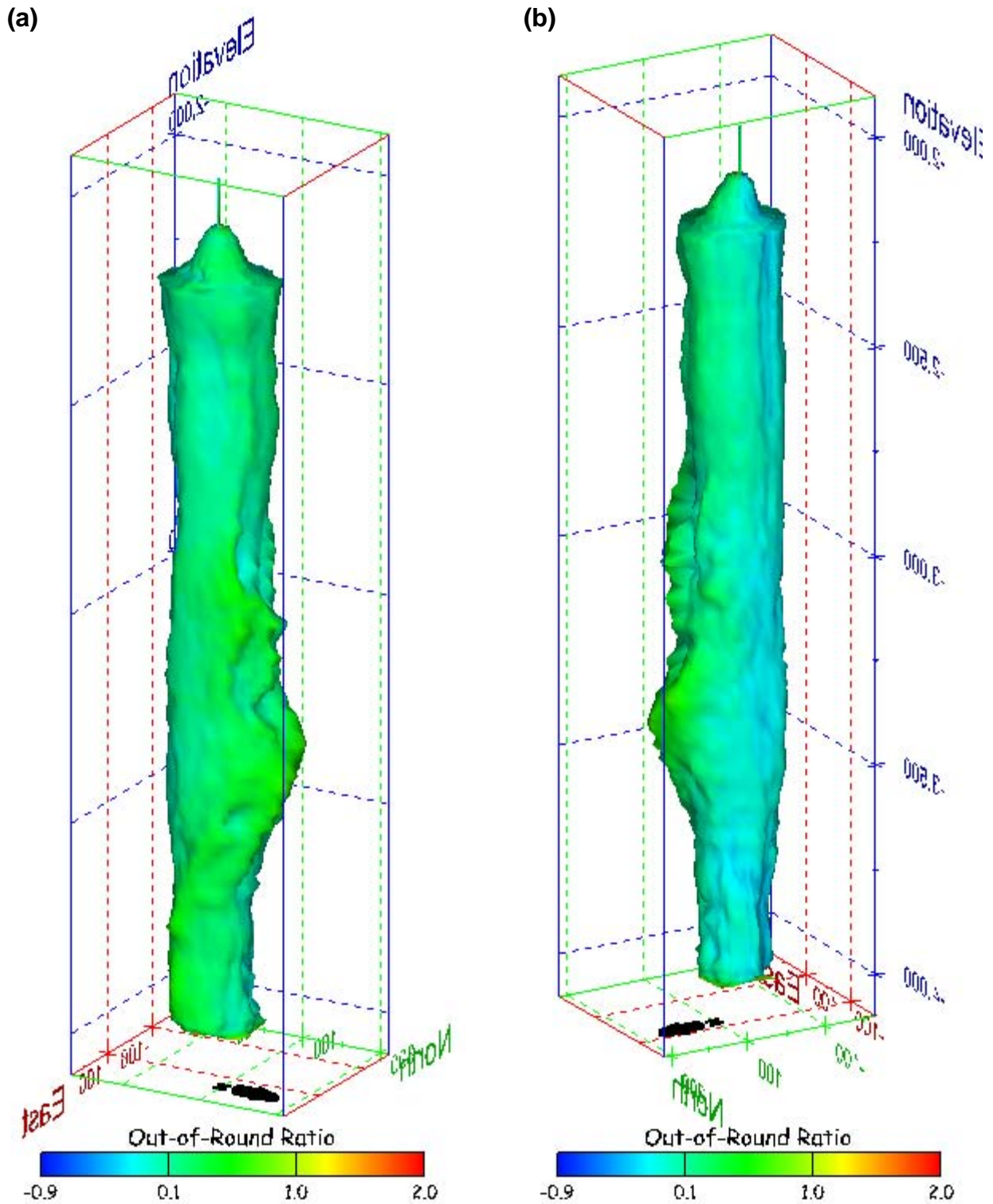
Figure 215. Sonar images of cavern BM-103, showing the geometry of the cavern colored by out-of-round ratio. View from (a) azimuth 60°, elevation 20°; (b) azimuth 300°, elevation 20°.
