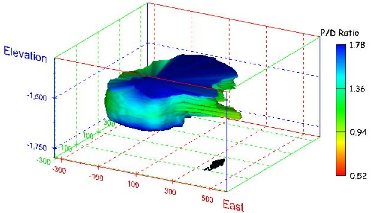
Figure 64. Sonar images of cavern BM-2, showing the geometry of the cavern colored by three-dimensional pillar-to-diameter ratio. View from (a) azimuth 210°, elevation 20°; (b) azimuth 150°, elevation 20°.
