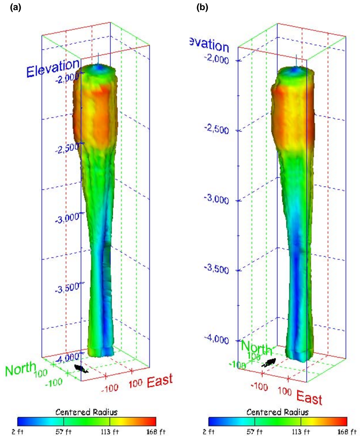
Figure 228. Sonar images of cavern BM-104, showing the geometry of the cavern colored by centered radius. View from (a) azimuth 210°, elevation 20°; (b) azimuth 150°, elevation 20°.
