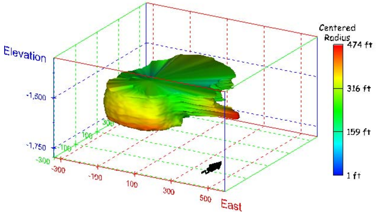
Figure 46. Sonar images of cavern BM-2, showing the geometry of the cavern colored by centered radius. View from (a) azimuth 210°, elevation 20°; (b) azimuth 150°, elevation 20°.
