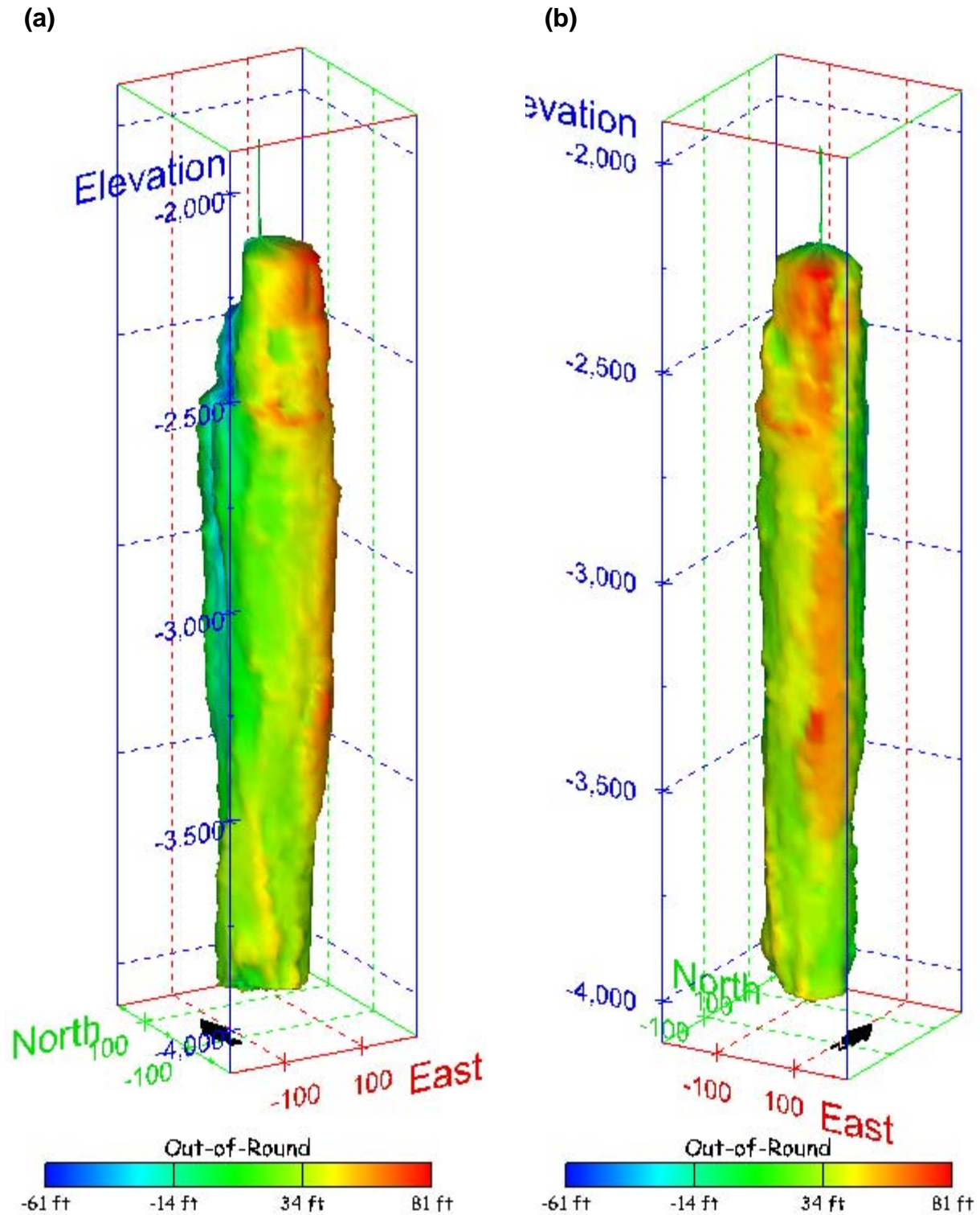
Figure 316. Sonar images of cavern BM-107, showing the geometry of the cavern colored by out-of-round distance. View from (a) azimuth 210°, elevation 20°; (b) azimuth 150°, elevation 20°.
