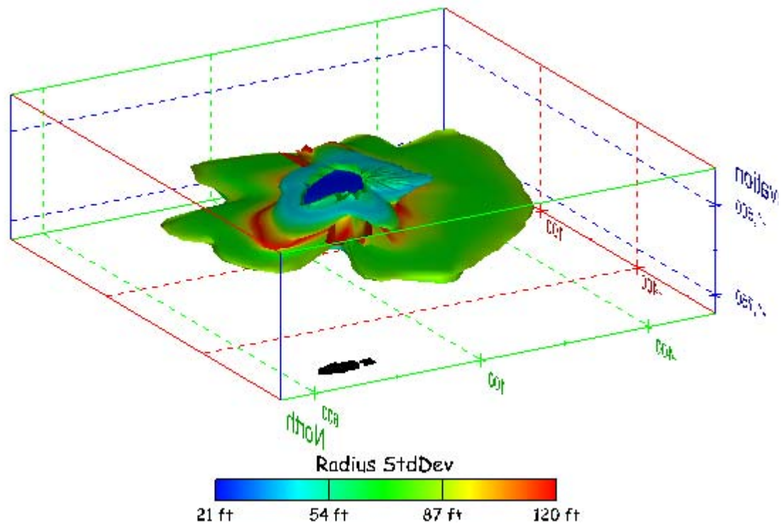
Figure 81. Sonar images of cavern BM-3, showing the geometry of the cavern colored by radius standard deviation. View from (a) azimuth 60°, elevation 20°; (b) azimuth 300°, elevation 20°.
