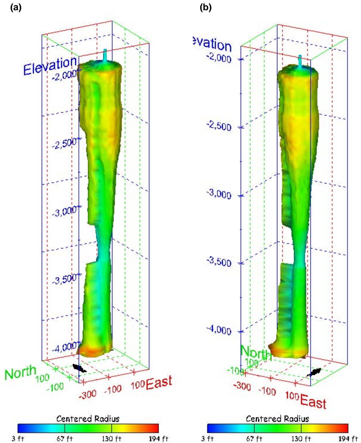
Figure 254. Sonar images of cavern BM-105, showing the geometry of the cavern colored by centered radius. View from (a) azimuth 210°, elevation 20°; (b) azimuth 150°, elevation 20°.
