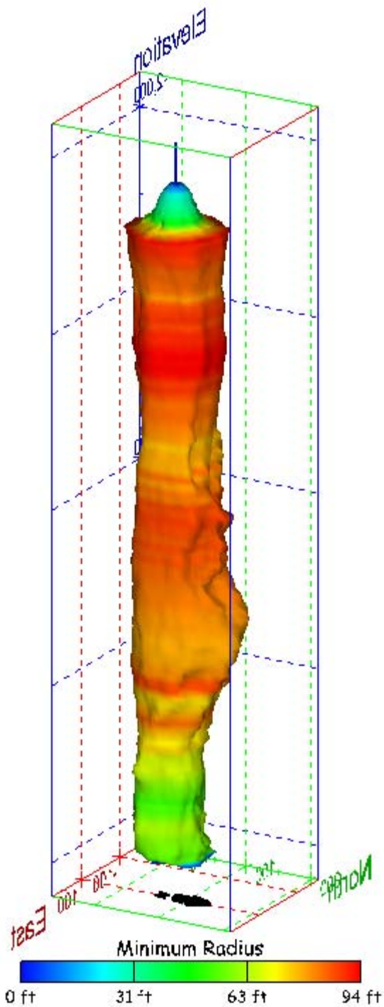
Figure 207. Sonar images of cavern BM-103, showing the geometry of the cavern colored by minimum radius. View from (a) azimuth 60°, elevation 20°; (b) azimuth 300°, elevation 20°.
