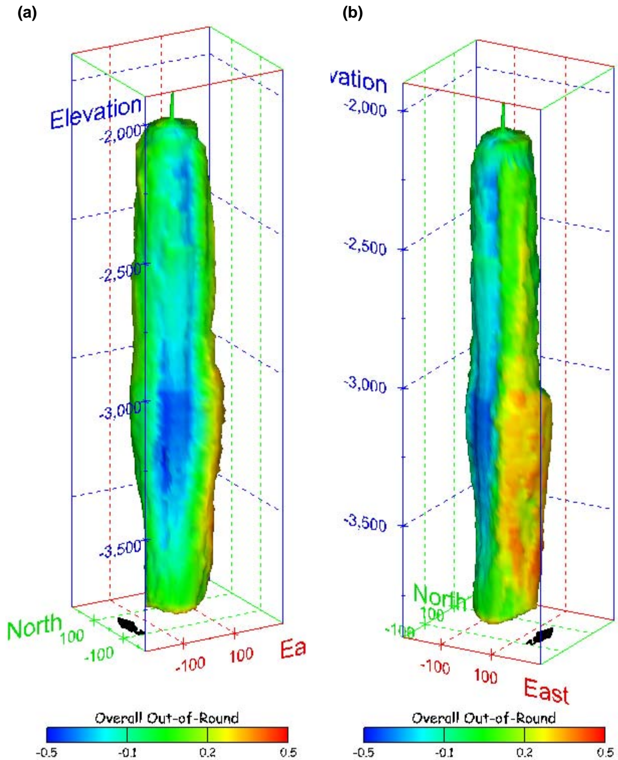
Figure 294. Sonar images of cavern BM-106, showing the geometry of the cavern colored by overall out-of-round ratio. View from (a) azimuth 210°, elevation 20°; (b) azimuth 150°, elevation 20°.
