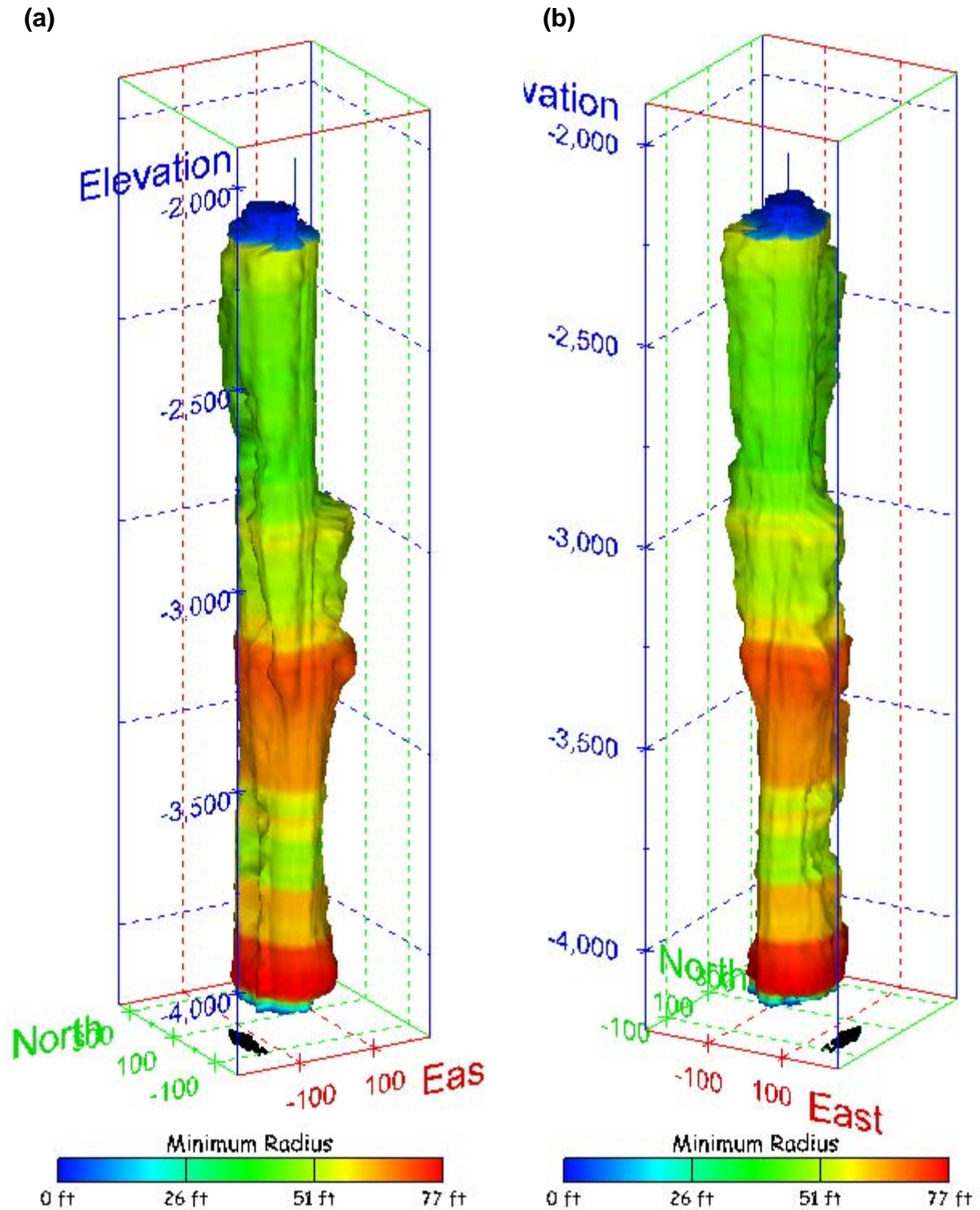
Figure 336. Sonar images of cavern BM-108, showing the geometry of the cavern colored by minimum radius. View from (a) azimuth 210°, elevation 20°; (b) azimuth 150°, elevation 20°.
