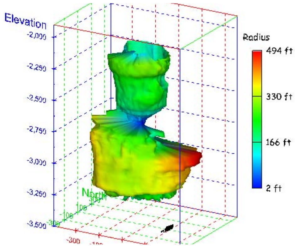
Figure 122. Sonar images of cavern BM-5, showing the geometry of the cavern colored by measured radius. View from (a) azimuth 210°, elevation 20°; (b) azimuth 150°, elevation 20°.
