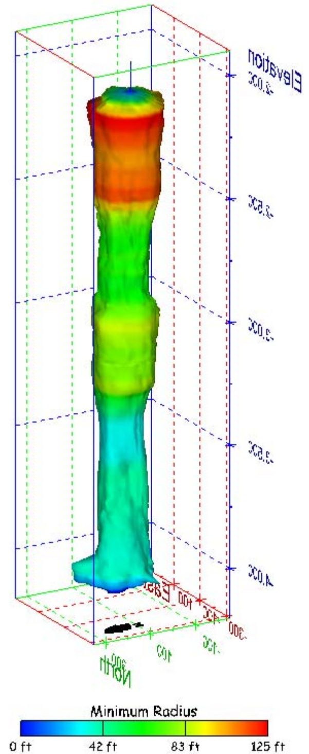
Figure 363. Sonar images of cavern BM-109, showing the geometry of the cavern colored by minimum radius. View from (a) azimuth 60°, elevation 20°; (b) azimuth 300°, elevation 20°.
