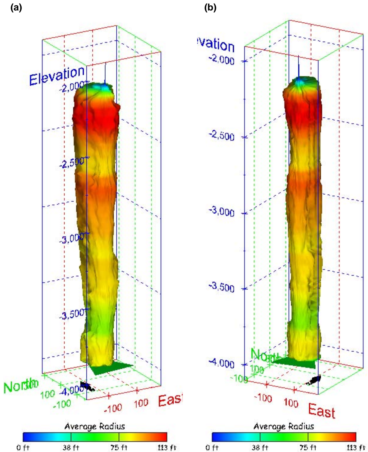
Figure 438. Sonar images of cavern BM-112, showing the geometry of the cavern colored by average radius. View from (a) azimuth 210°, elevation 20°; (b) azimuth 150°, elevation 20°.
