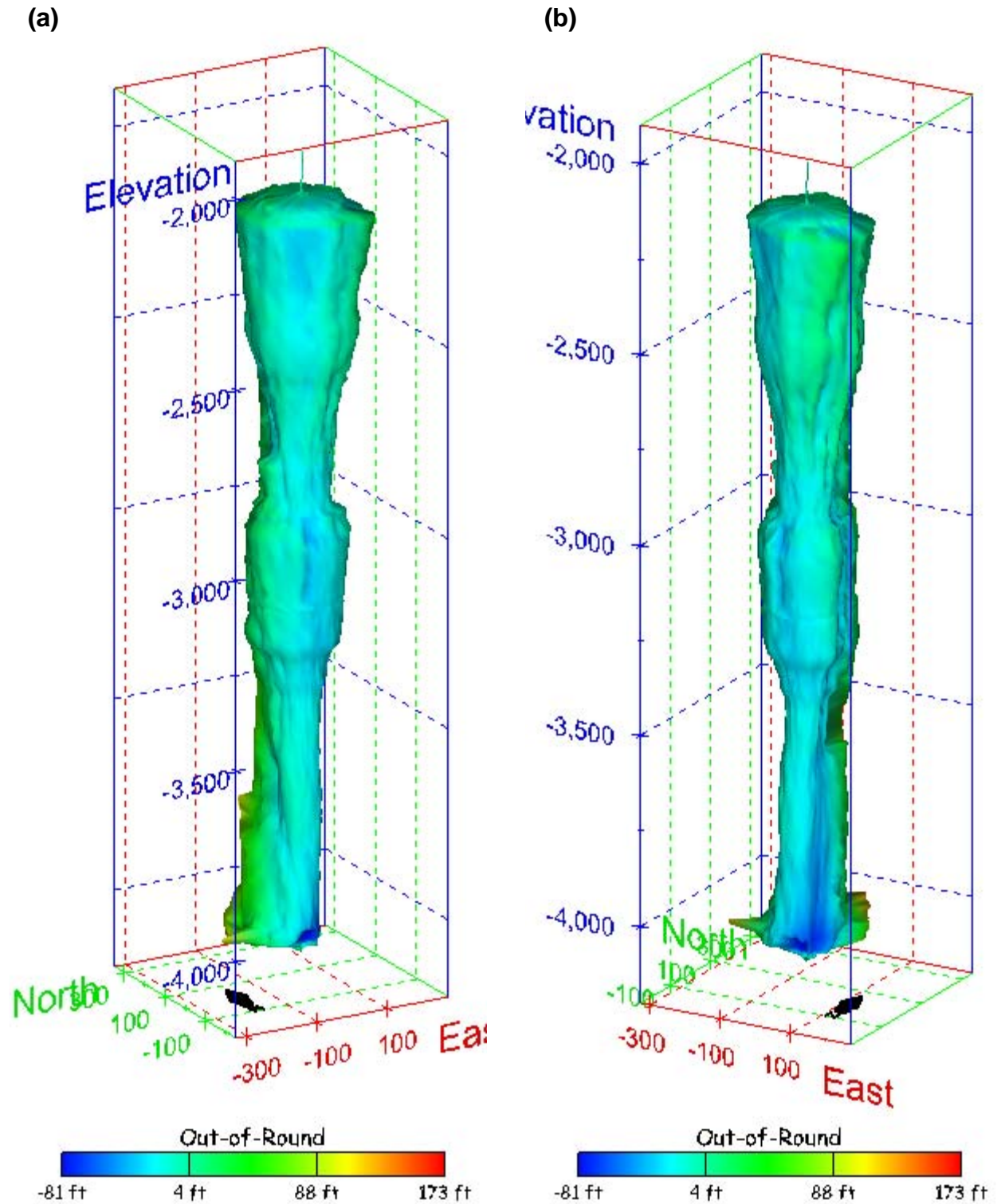
Figure 368. Sonar images of cavern BM-109, showing the geometry of the cavern colored by out-of-round distance. View from (a) azimuth 210°, elevation 20°; (b) azimuth 150°, elevation 20°.
