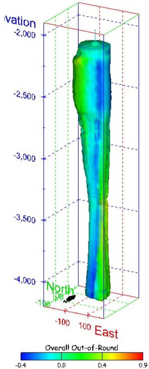
Figure 242. Sonar images of cavern BM-104, showing the geometry of the cavern colored by overall out-of-round ratio. View from (a) azimuth 210°, elevation 20°; (b) azimuth 150°, elevation 20°.
