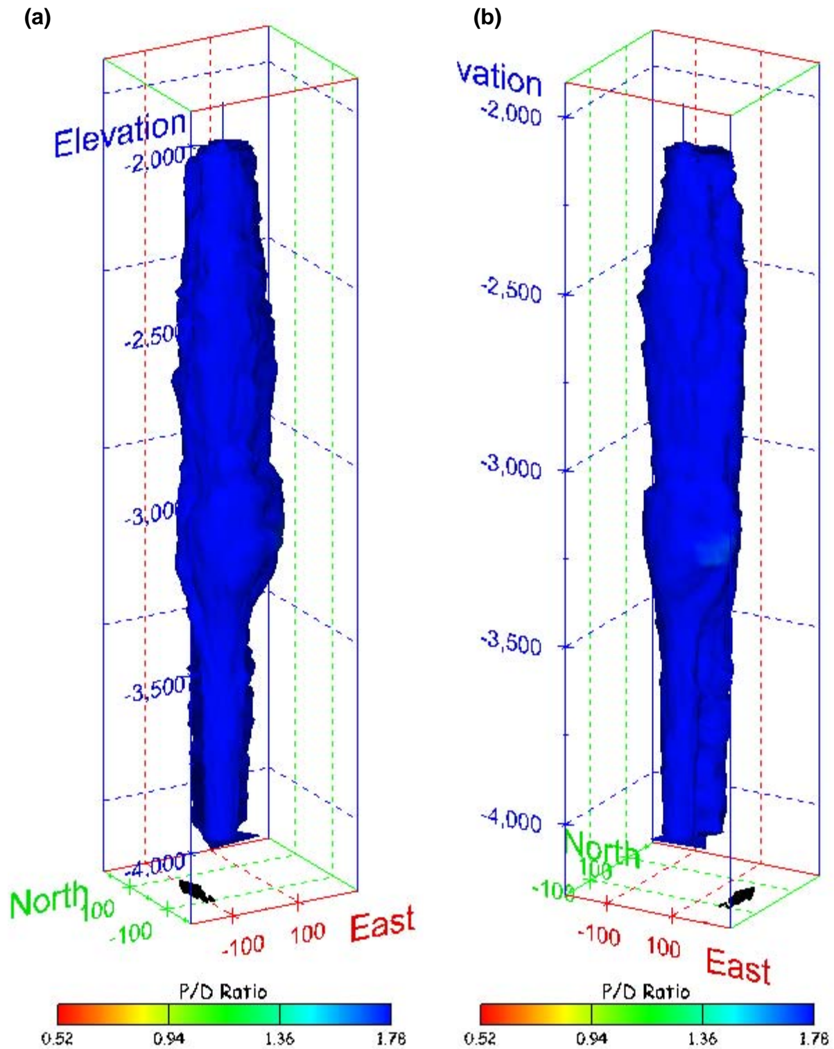
Figure 402. Sonar images of cavern BM-110, showing the geometry of the cavern colored by three-dimensional pillar-to-diameter ratio. View from (a) azimuth 210°, elevation 20°; (b) azimuth 150°, elevation 20°.
