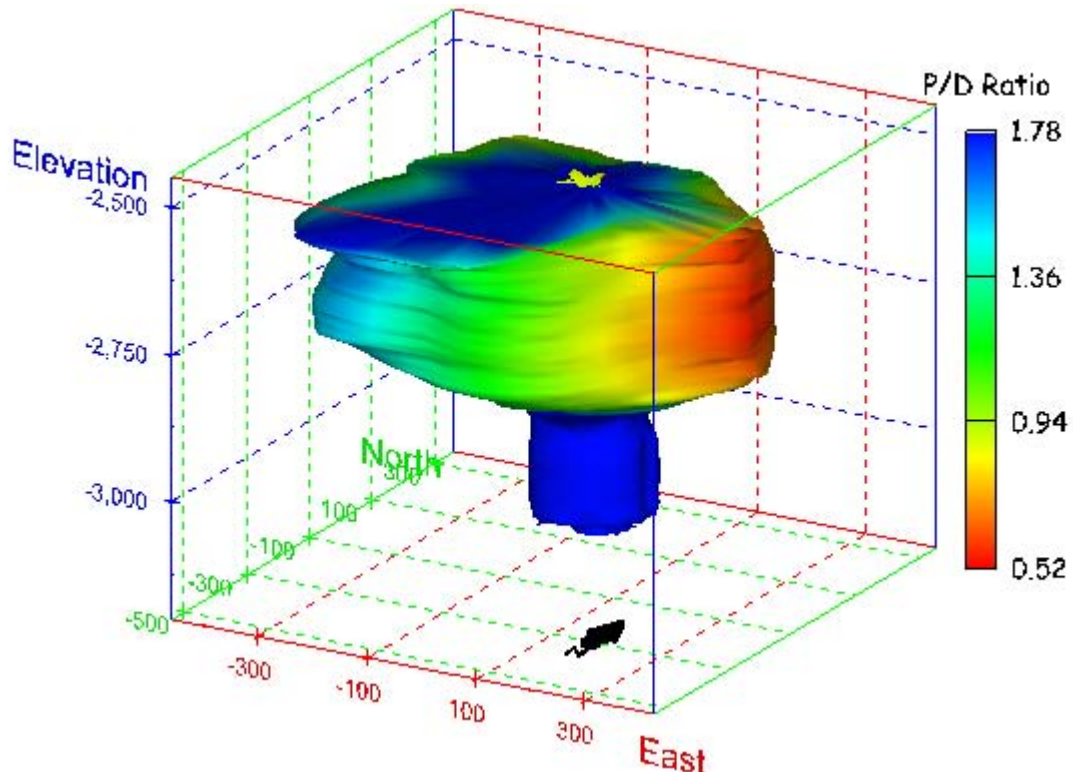
Figure 116. Sonar images of cavern BM-4, showing the geometry of the cavern colored by three-dimensional pillar-to-diameter ratio. View from (a) azimuth 210°, elevation 20°; (b) azimuth 150°, elevation 20°.
