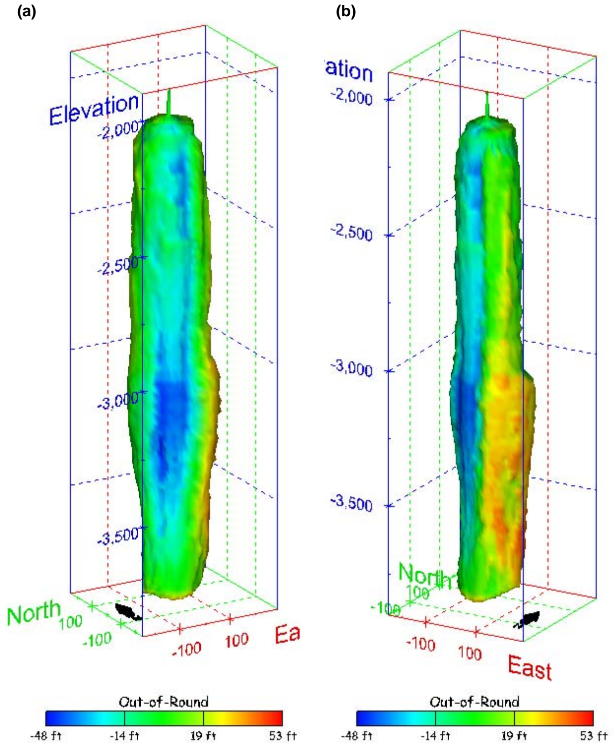
Figure 290. Sonar images of cavern BM-106, showing the geometry of the cavern colored by out-of-round distance. View from (a) azimuth 210°, elevation 20°; (b) azimuth 150°, elevation 20°.
