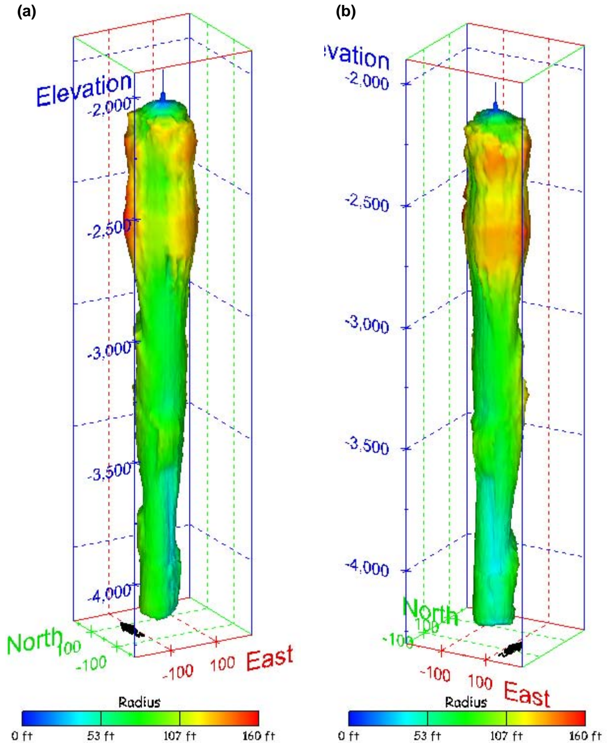
Figure 538. Sonar images of cavern BM-116, showing the geometry of the cavern colored by measured radius. View from (a) azimuth 210°, elevation 20°; (b) azimuth 150°, elevation 20°.
