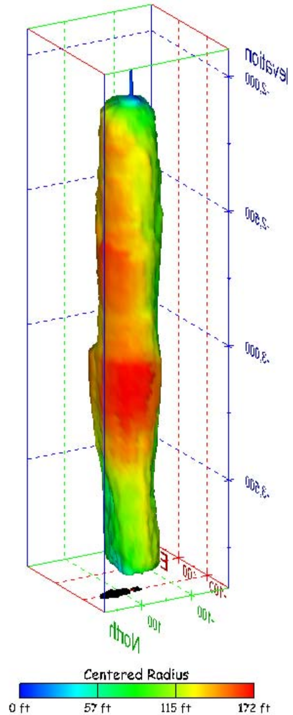
Figure 281. Sonar images of cavern BM-106, showing the geometry of the cavern colored by centered radius. View from (a) azimuth 60°, elevation 20°; (b) azimuth 300°, elevation 20°.
