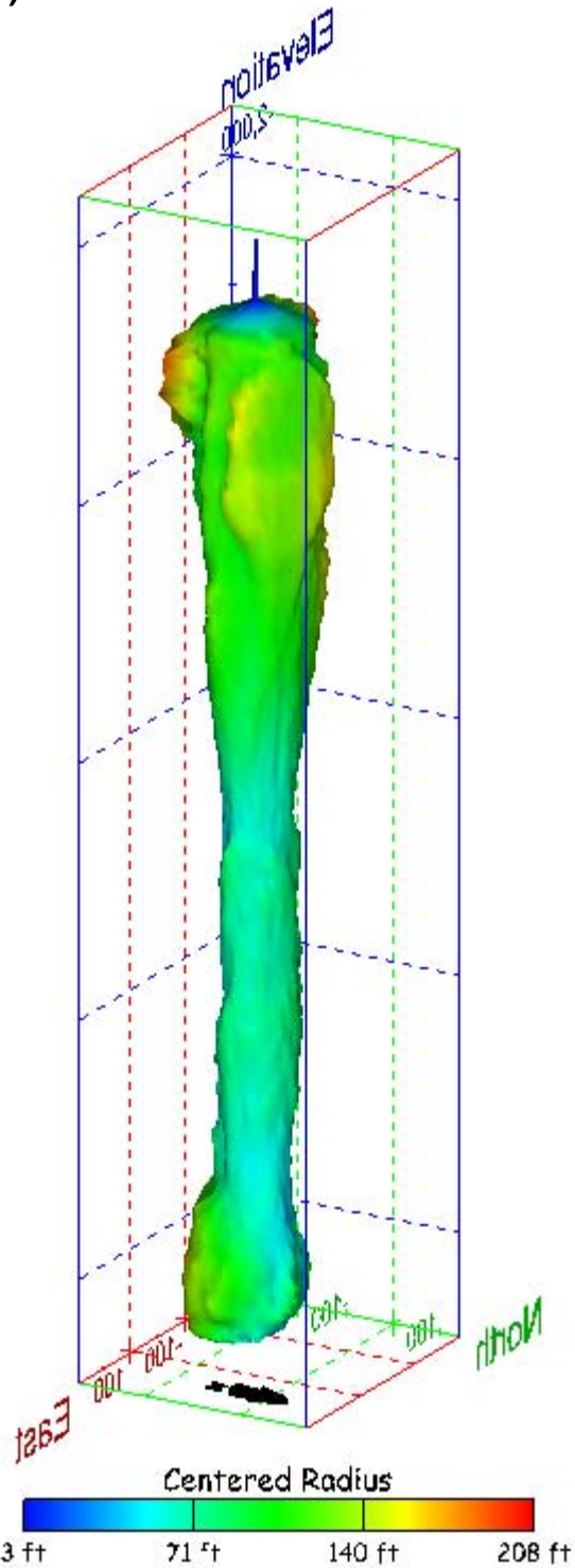
Figure 489. Sonar images of cavern BM-114, showing the geometry of the cavern colored by centered radius. View from (a) azimuth 60°, elevation 20°; (b) azimuth 300°, elevation 20°.
