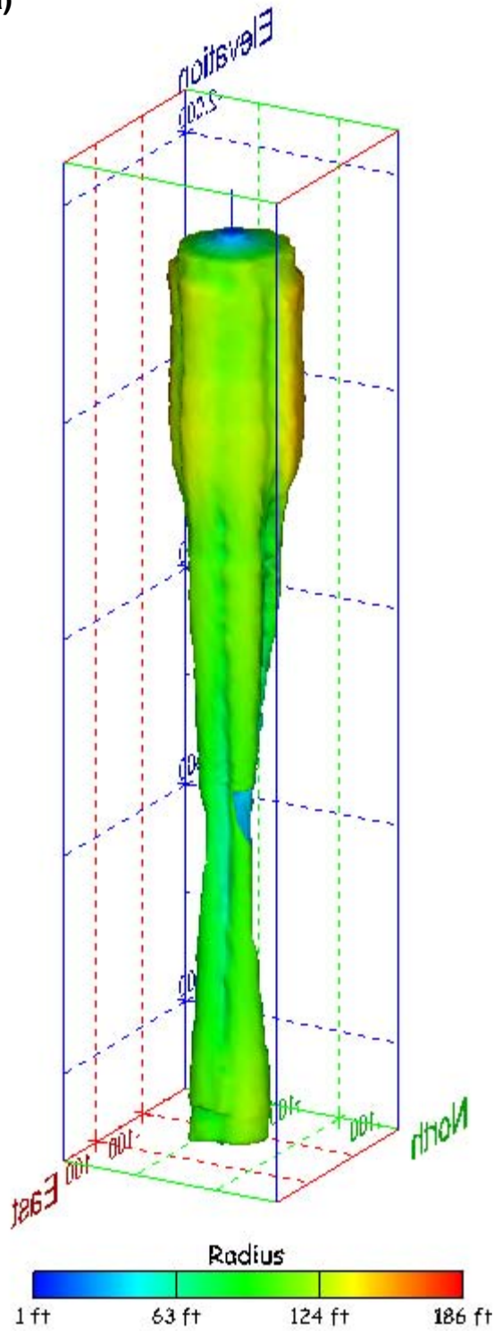
Figure 227. Sonar images of cavern BM-104, showing the geometry of the cavern colored by measured radius. View from (a) azimuth 60°, elevation 20°; (b) azimuth 300°, elevation 20°.
