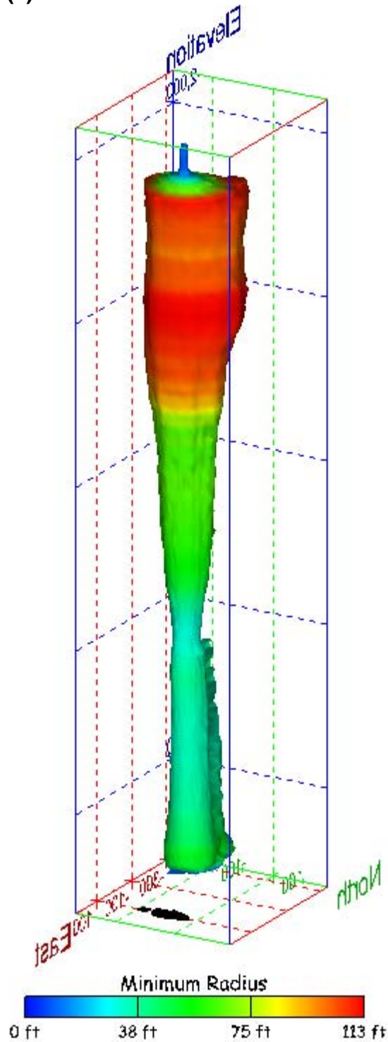
Figure 259. Sonar images of cavern BM-105, showing the geometry of the cavern colored by minimum radius. View from (a) azimuth 60°, elevation 20°; (b) azimuth 300°, elevation 20°.
