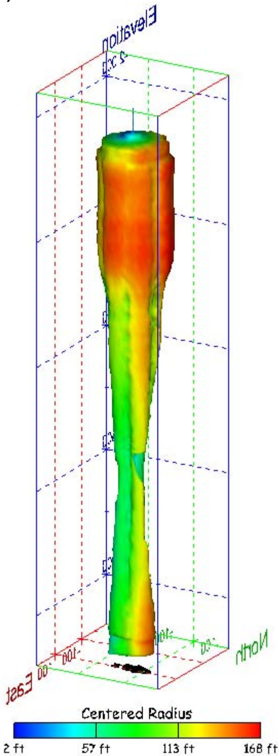
Figure 229. Sonar images of cavern BM-104, showing the geometry of the cavern colored by centered radius. View from (a) azimuth 60°, elevation 20°; (b) azimuth 300°, elevation 20°.
