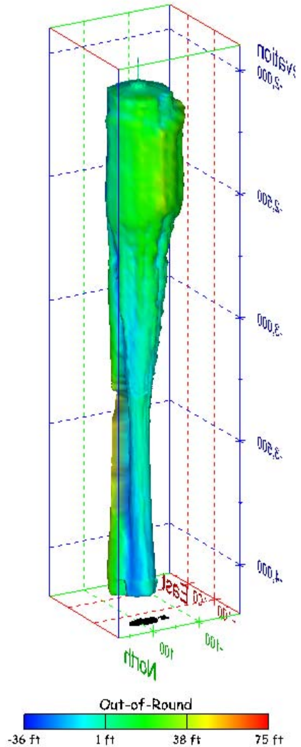
Figure 239. Sonar images of cavern BM-104, showing the geometry of the cavern colored by out-of-round distance. View from (a) azimuth 60°, elevation 20°; (b) azimuth 300°, elevation 20°.
