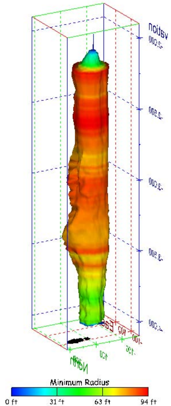
Figure 207. Sonar images of cavern BM-103, showing the geometry of the cavern colored by minimum radius. View from (a) azimuth 60°, elevation 20°; (b) azimuth 300°, elevation 20°.
