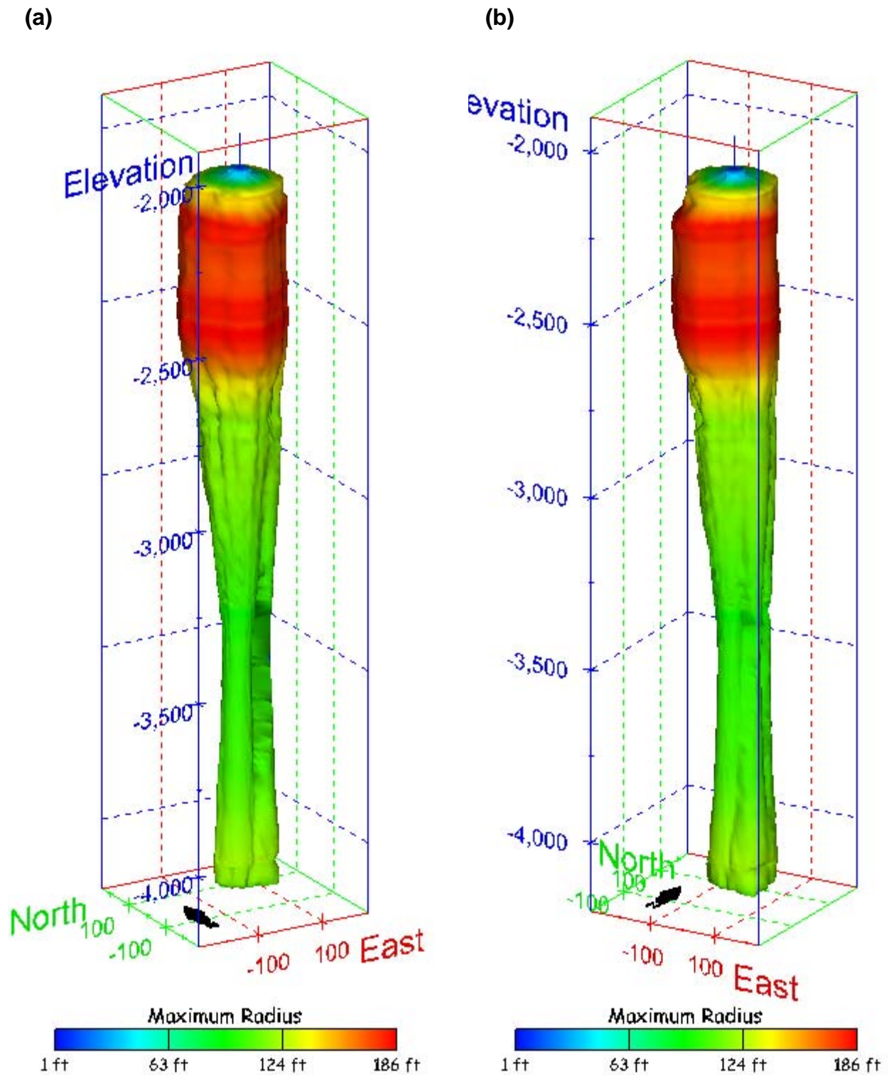
Figure 234. Sonar images of cavern BM-104, showing the geometry of the cavern colored by maximum radius. View from (a) azimuth 210°, elevation 20°; (b) azimuth 150°, elevation 20°.
