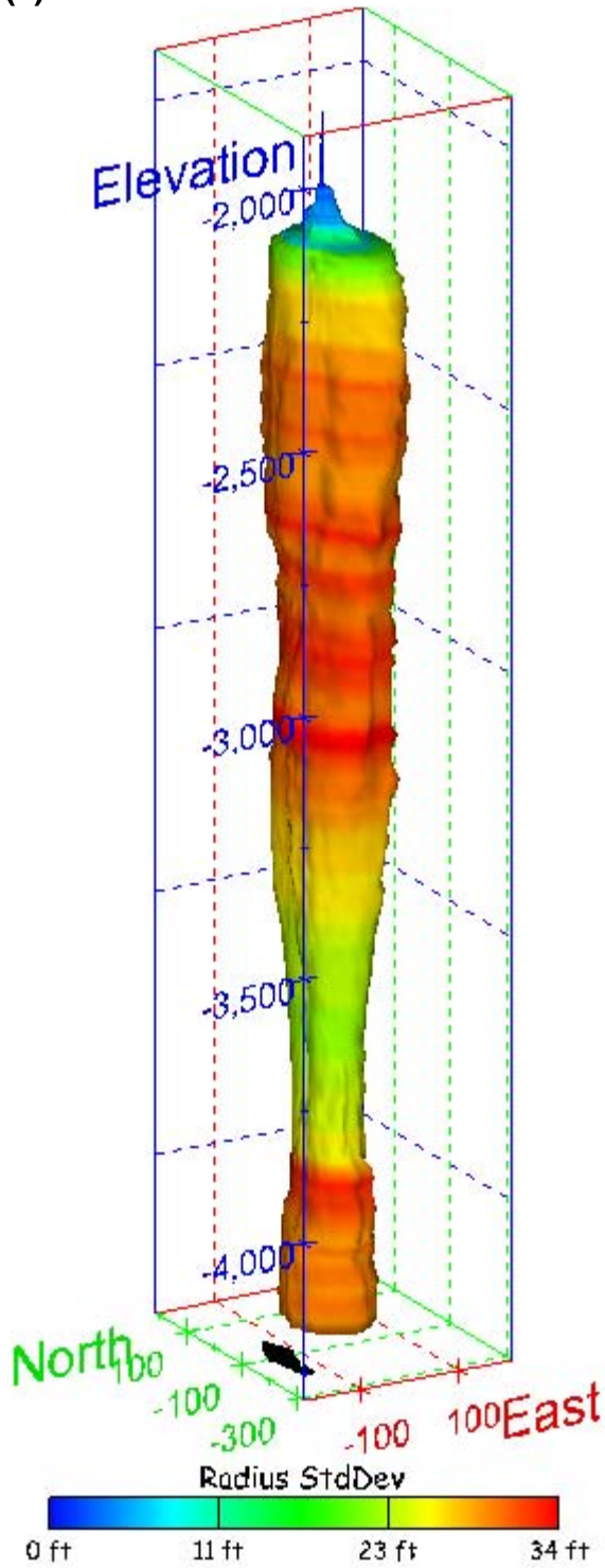
Figure 184. Sonar images of cavern BM-102, showing the geometry of the cavern colored by radius standard deviation. View from (a) azimuth 210°, elevation 20°; (b) azimuth 150°, elevation 20°.
