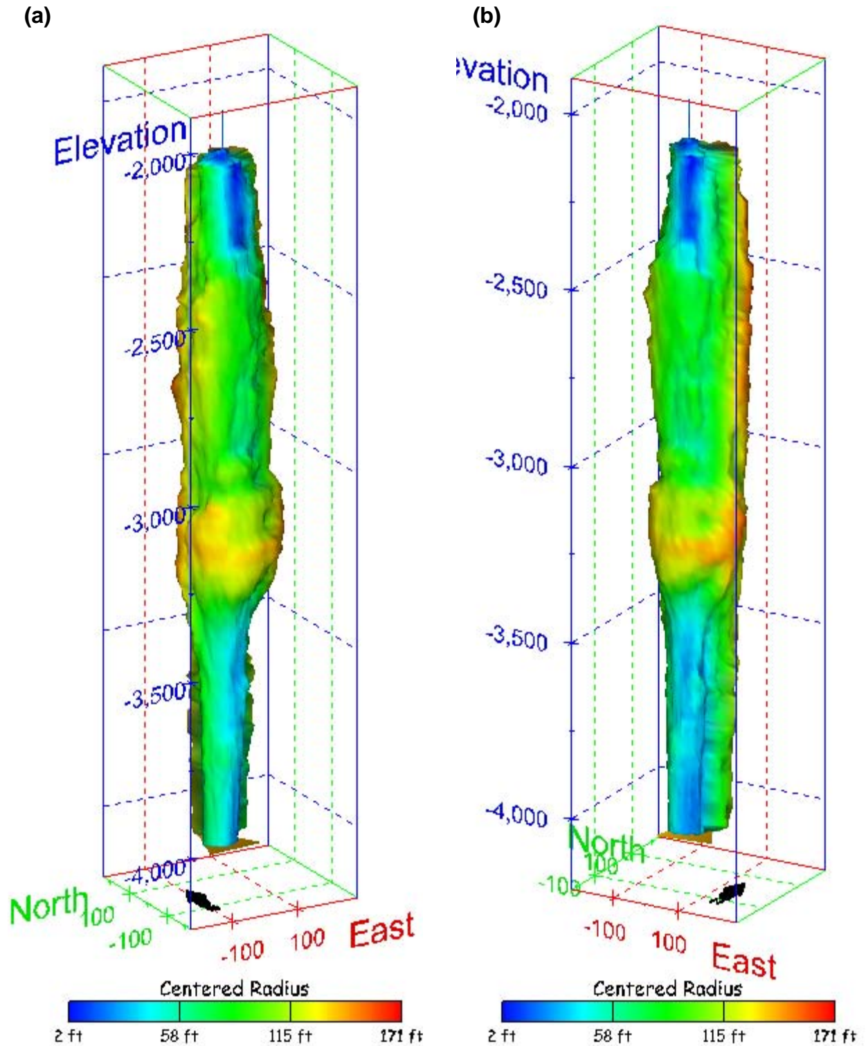
Figure 384. Sonar images of cavern BM-110, showing the geometry of the cavern colored by centered radius. View from (a) azimuth 210°, elevation 20°; (b) azimuth 150°, elevation 20°.
