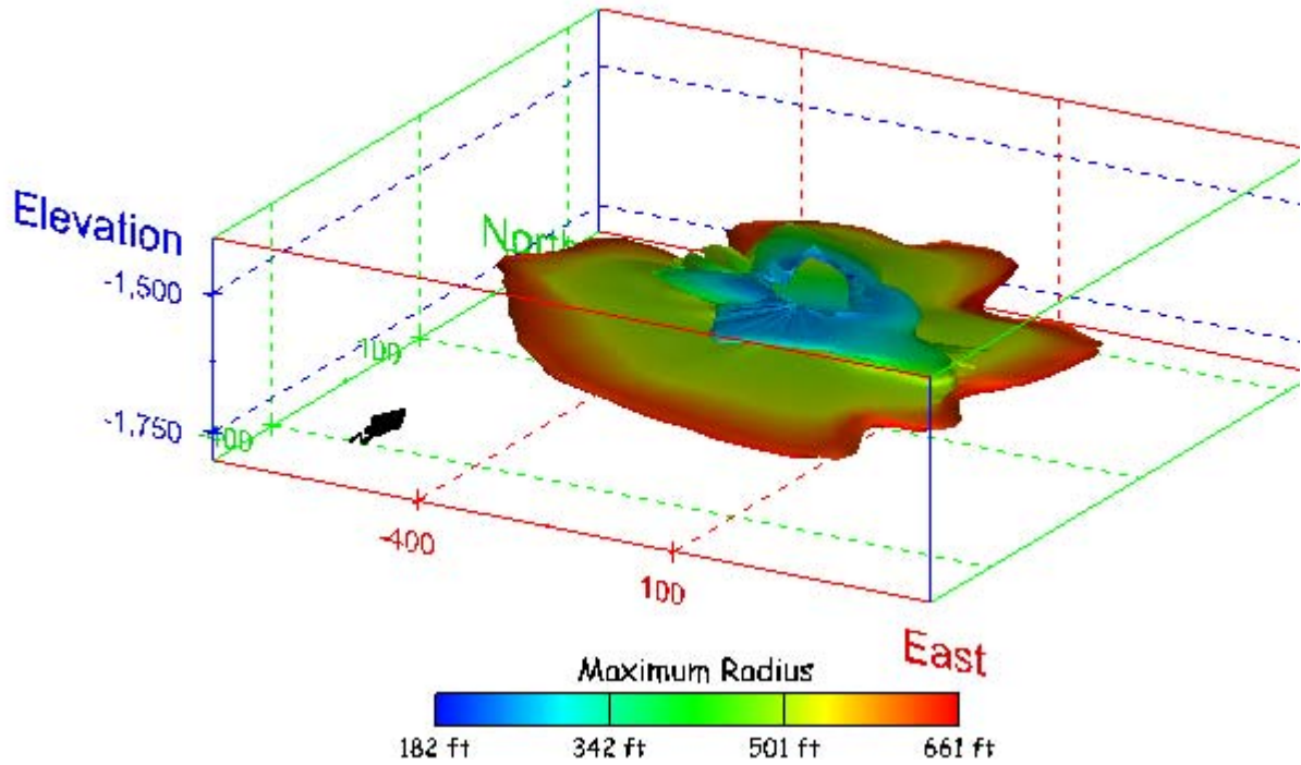
Figure 78. Sonar images of cavern BM-3, showing the geometry of the cavern colored by maximum radius. View from (a) azimuth 210°, elevation 20°; (b) azimuth 150°, elevation 20°.
