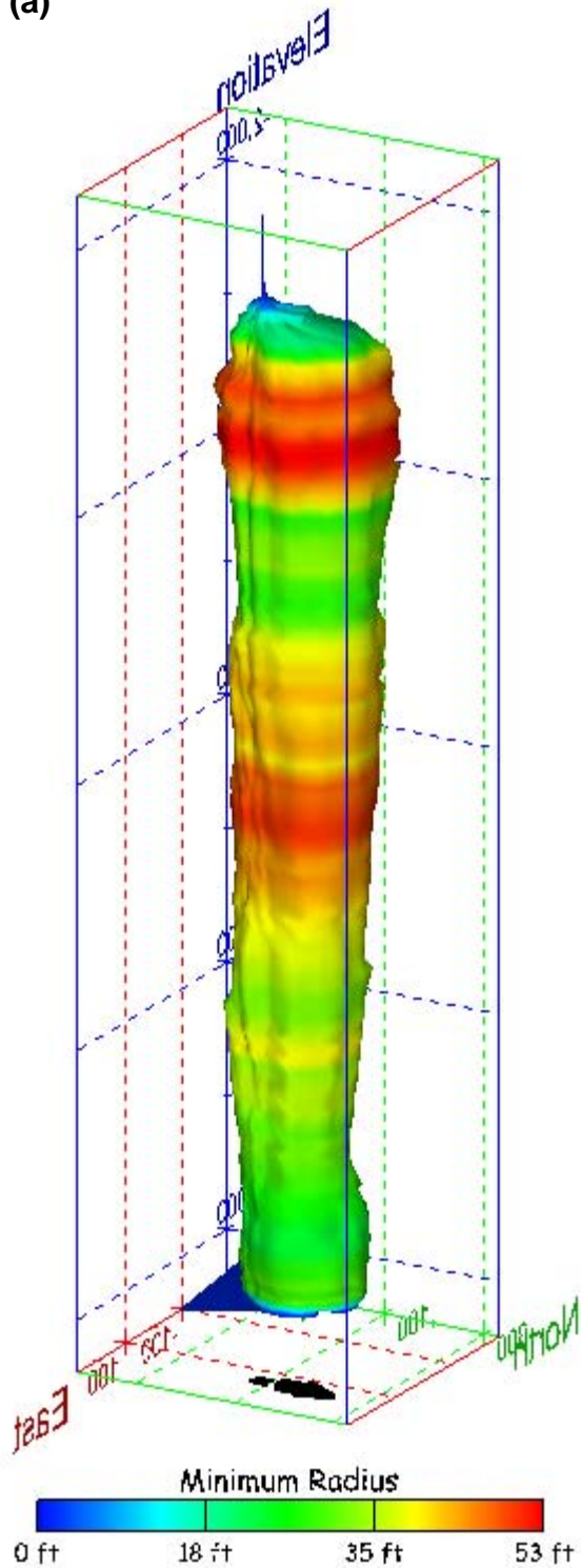
Figure 441. Sonar images of cavern BM-112, showing the geometry of the cavern colored by minimum radius. View from (a) azimuth 60°, elevation 20°; (b) azimuth 300°, elevation 20°.
