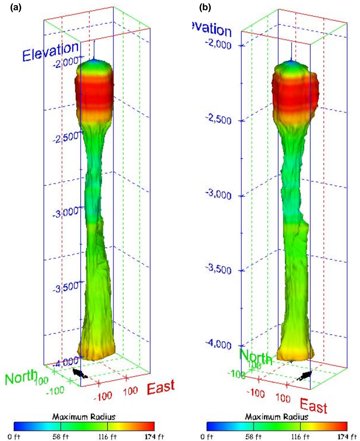
Figure 468. Sonar images of cavern BM-113, showing the geometry of the cavern colored by maximum radius. View from (a) azimuth 210°, elevation 20°; (b) azimuth 150°, elevation 20°.
