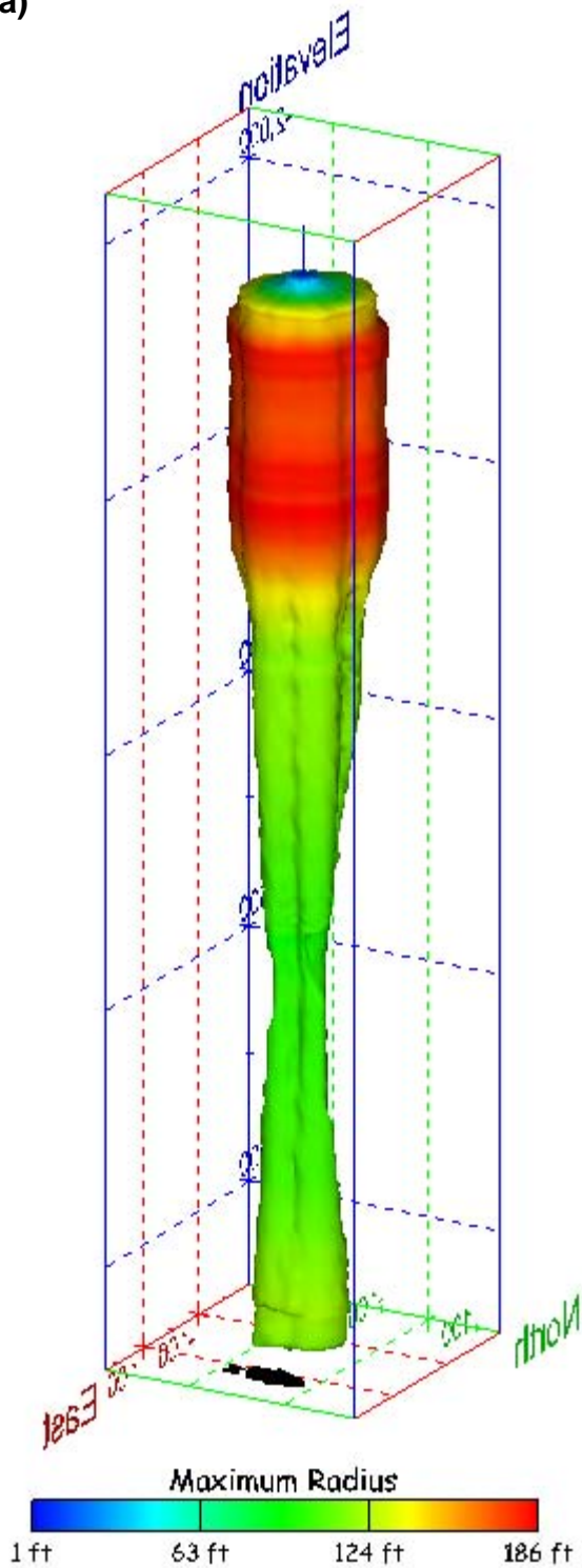
Figure 235. Sonar images of cavern BM-104, showing the geometry of the cavern colored by maximum radius. View from (a) azimuth 60°, elevation 20°; (b) azimuth 300°, elevation 20°.
