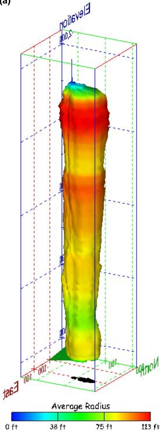
Figure 439. Sonar images of cavern BM-112, showing the geometry of the cavern colored by average radius. View from (a) azimuth 60°, elevation 20°; (b) azimuth 300°, elevation 20°.
