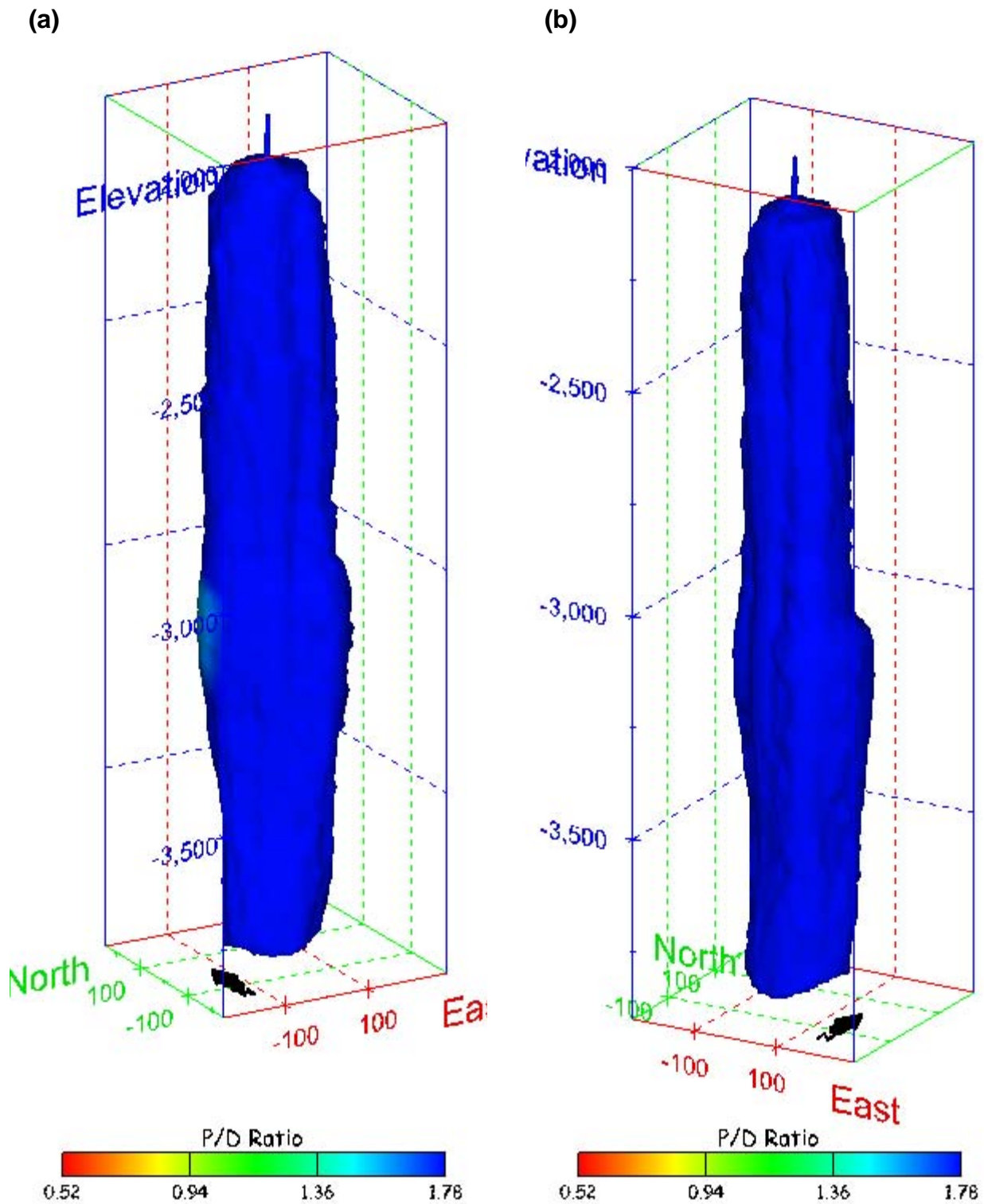
Figure 298. Sonar images of cavern BM-106, showing the geometry of the cavern colored by three-dimensional pillar-to-diameter ratio. View from (a) azimuth 210°, elevation 20°; (b) azimuth 150°, elevation 20°.
