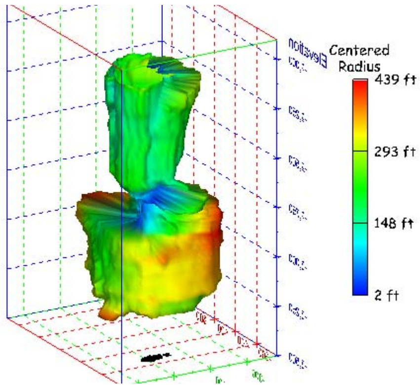
Figure 125. Sonar images of cavern BM-5, showing the geometry of the cavern colored by centered radius. View from (a) azimuth 60°, elevation 20°; (b) azimuth 300°, elevation 20°.
