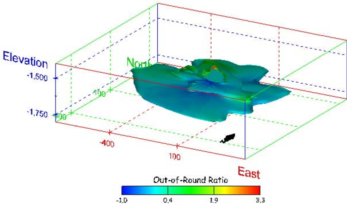
Figure 84. Sonar images of cavern BM-3, showing the geometry of the cavern colored by out-of-round ratio. View from (a) azimuth 210°, elevation 20°; (b) azimuth 150°, elevation 20°.
