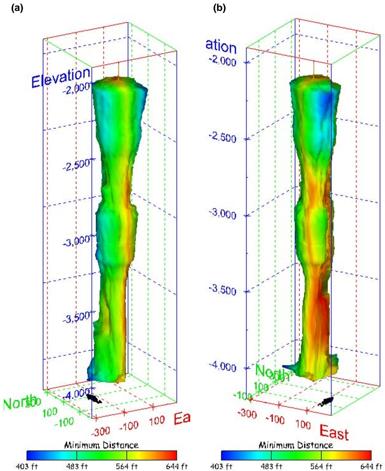
Figure 374. Sonar images of cavern BM-109, showing the geometry of the cavern colored by the minimum distance to the nearest neighboring cavern. View from (a) azimuth 210°, elevation 20°; (b) azimuth 150°, elevation 20°.
