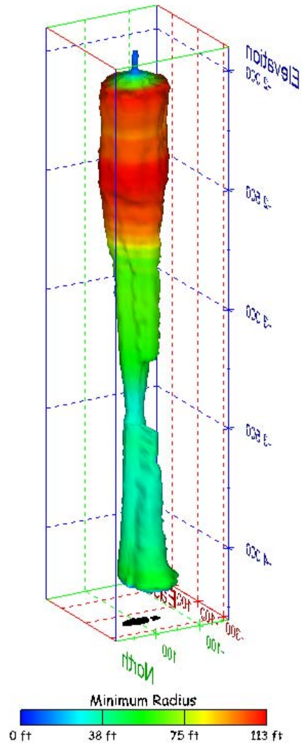
Figure 259. Sonar images of cavern BM-105, showing the geometry of the cavern colored by minimum radius. View from (a) azimuth 60°, elevation 20°; (b) azimuth 300°, elevation 20°.
