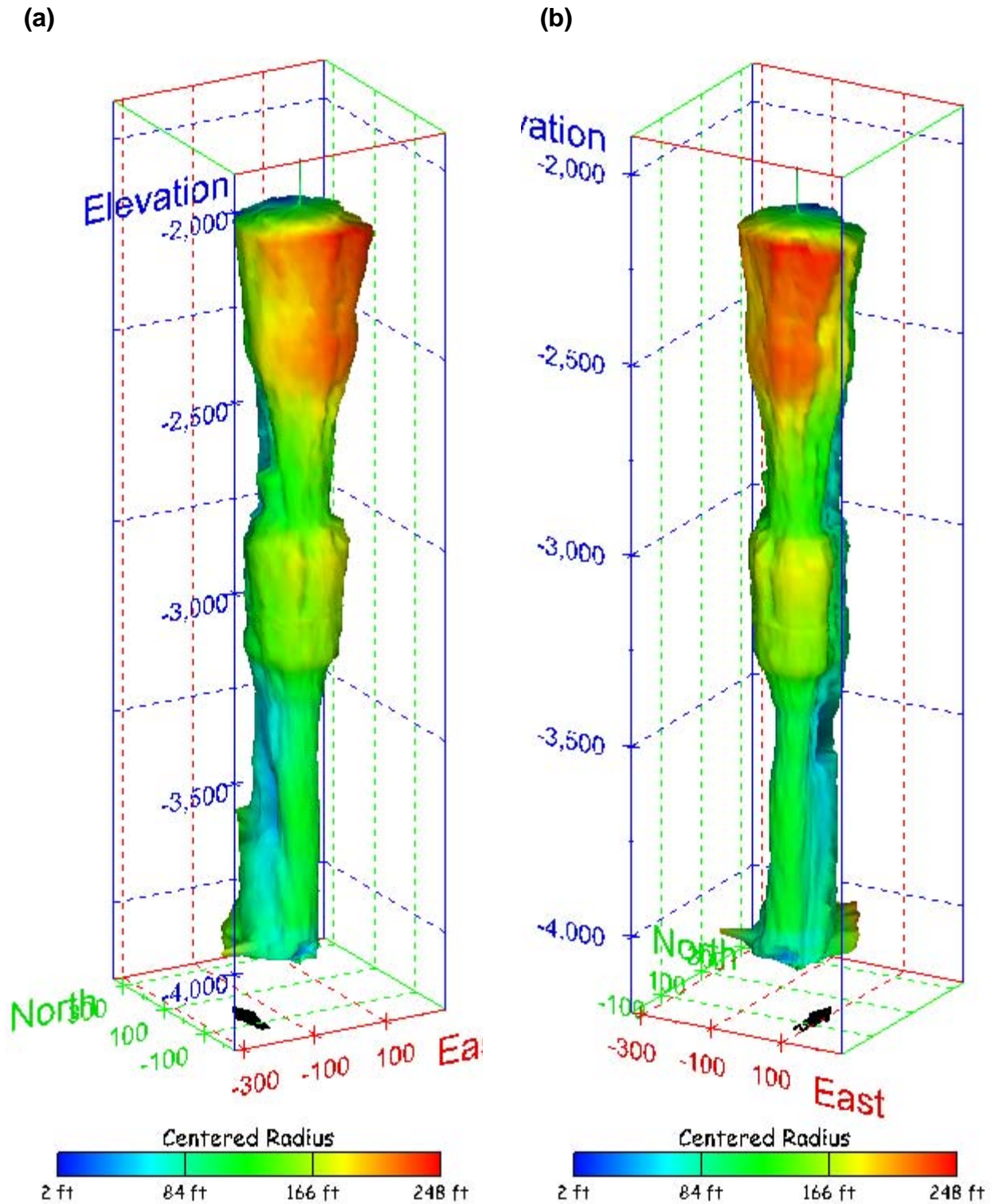
Figure 358. Sonar images of cavern BM-109, showing the geometry of the cavern colored by centered radius. View from (a) azimuth 210°, elevation 20°; (b) azimuth 150°, elevation 20°.
