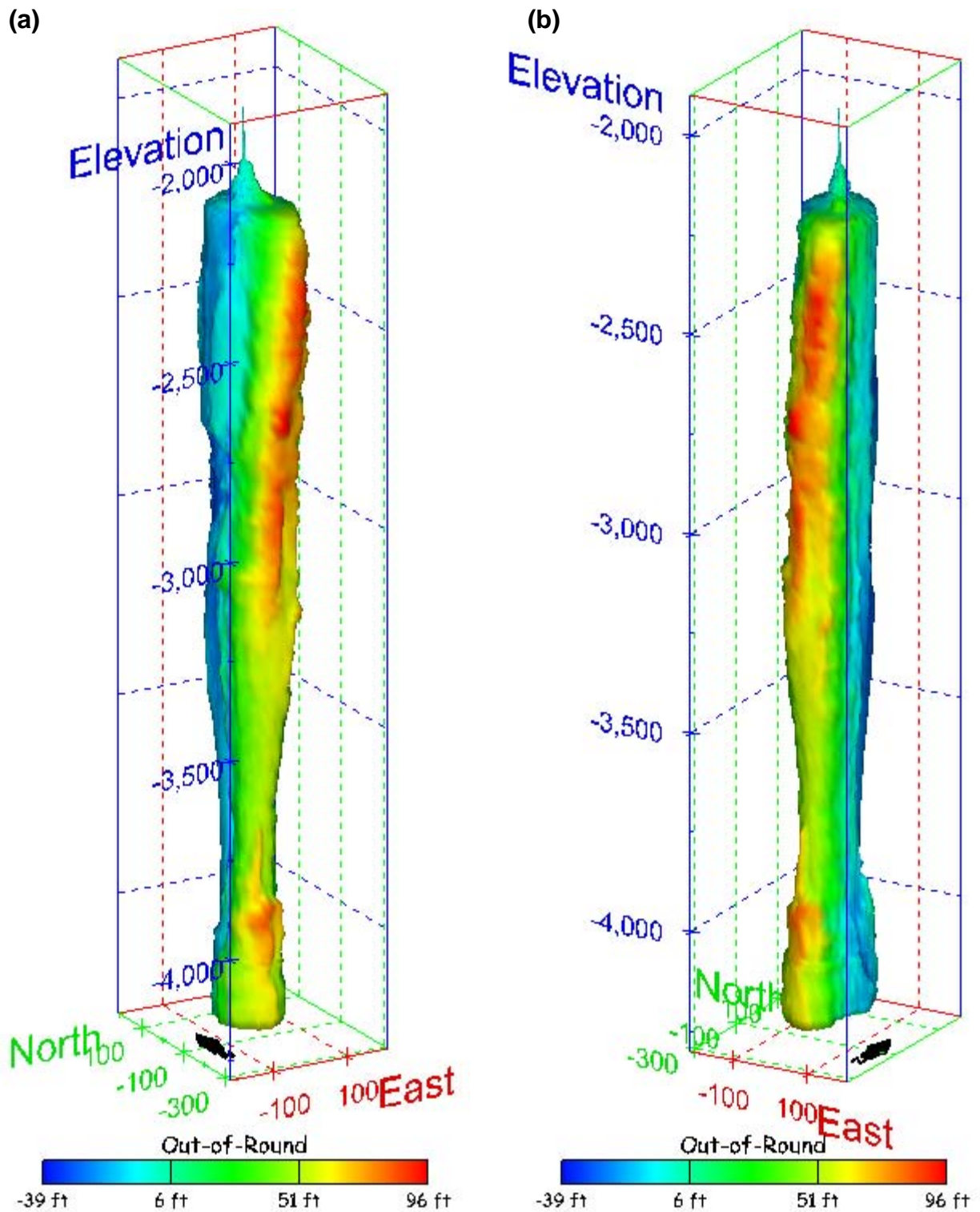
Figure 186. Sonar images of cavern BM-102, showing the geometry of the cavern colored by out-of-round distance. View from (a) azimuth 210°, elevation 20°; (b) azimuth 150°, elevation 20°.
