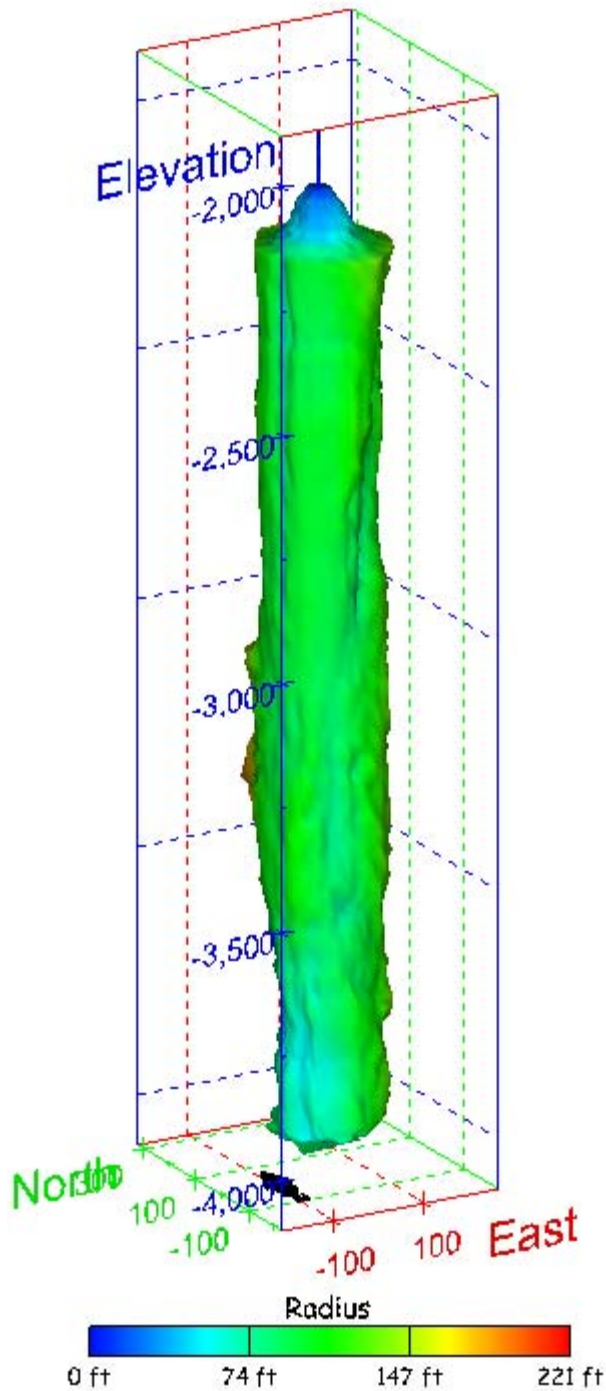
Figure 200. Sonar images of cavern BM-103, showing the geometry of the cavern colored by measured radius. View from (a) azimuth 210°, elevation 20°; (b) azimuth 150°, elevation 20°.
