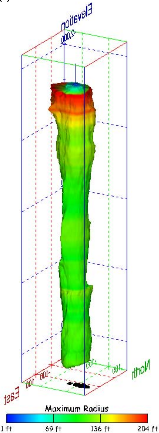
Figure 521. Sonar images of cavern BM-115, showing the geometry of the cavern colored by maximum radius. View from (a) azimuth 60°, elevation 20°; (b) azimuth 300°, elevation 20°.
