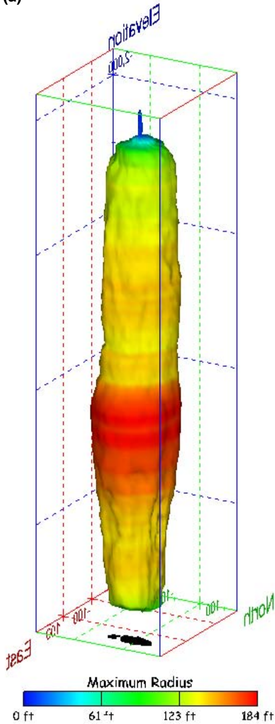
Figure 287. Sonar images of cavern BM-106, showing the geometry of the cavern colored by maximum radius. View from (a) azimuth 60°, elevation 20°; (b) azimuth 300°, elevation 20°.
