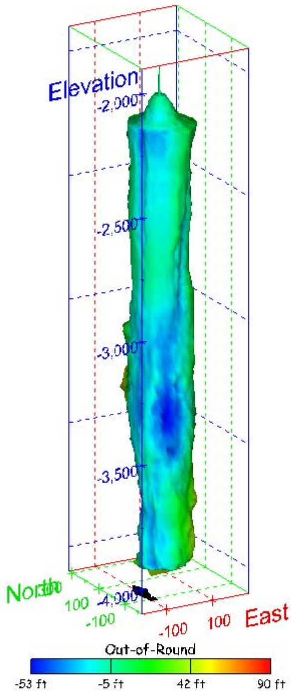
Figure 212. Sonar images of cavern BM-103, showing the geometry of the cavern colored by out-of-round distance. View from (a) azimuth 210°, elevation 20°; (b) azimuth 150°, elevation 20°.
