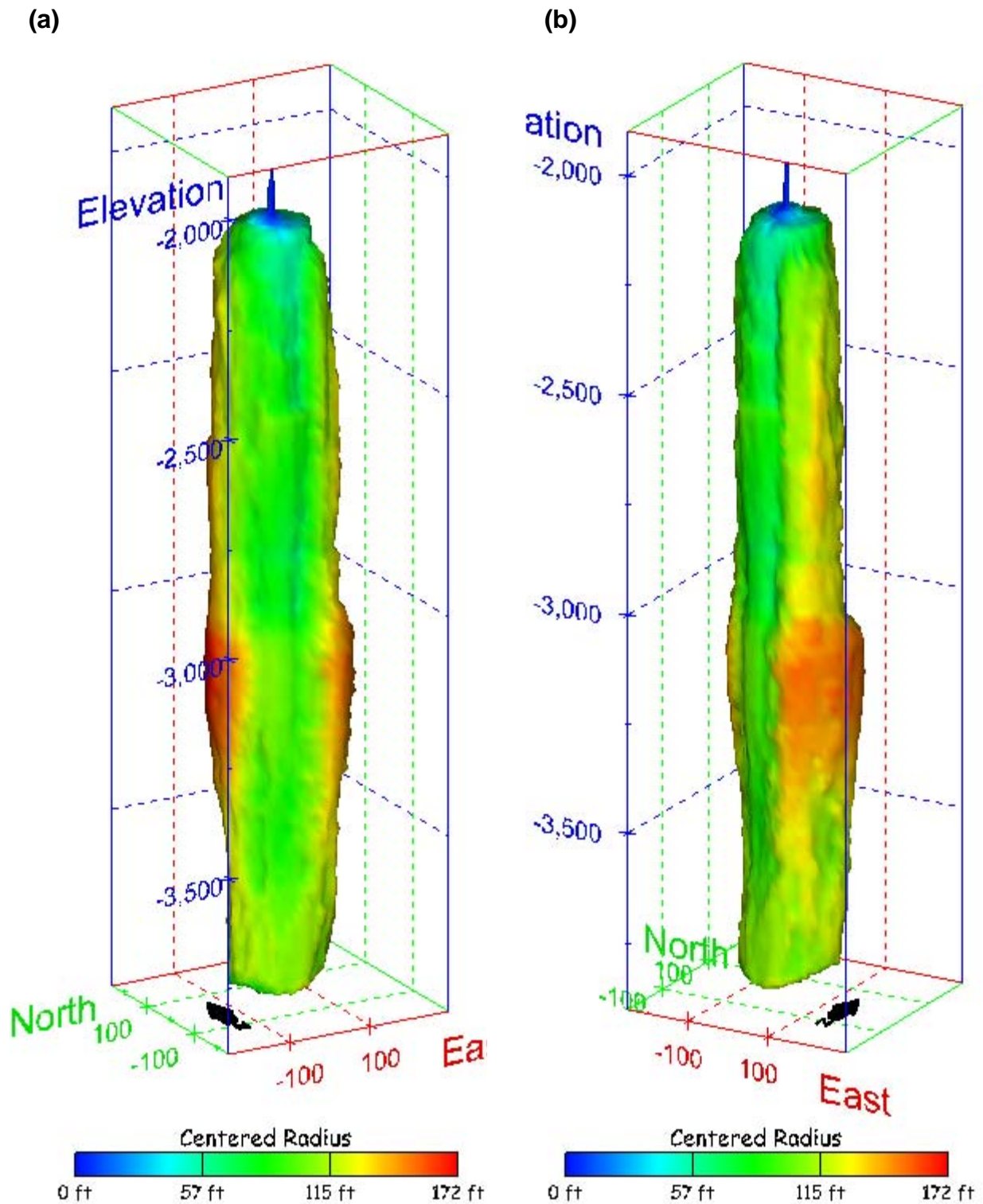
Figure 280. Sonar images of cavern BM-106, showing the geometry of the cavern colored by centered radius. View from (a) azimuth 210°, elevation 20°; (b) azimuth 150°, elevation 20°.
