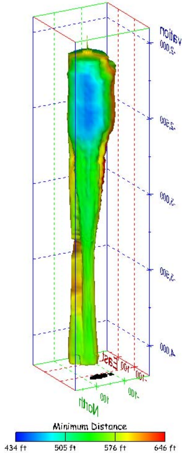
Figure 245. Sonar images of cavern BM-104, showing the geometry of the cavern colored by minimum distance to the nearest neighboring cavern. View from (a) azimuth 60°, elevation 20°; (b) azimuth 300°, elevation 20°.
