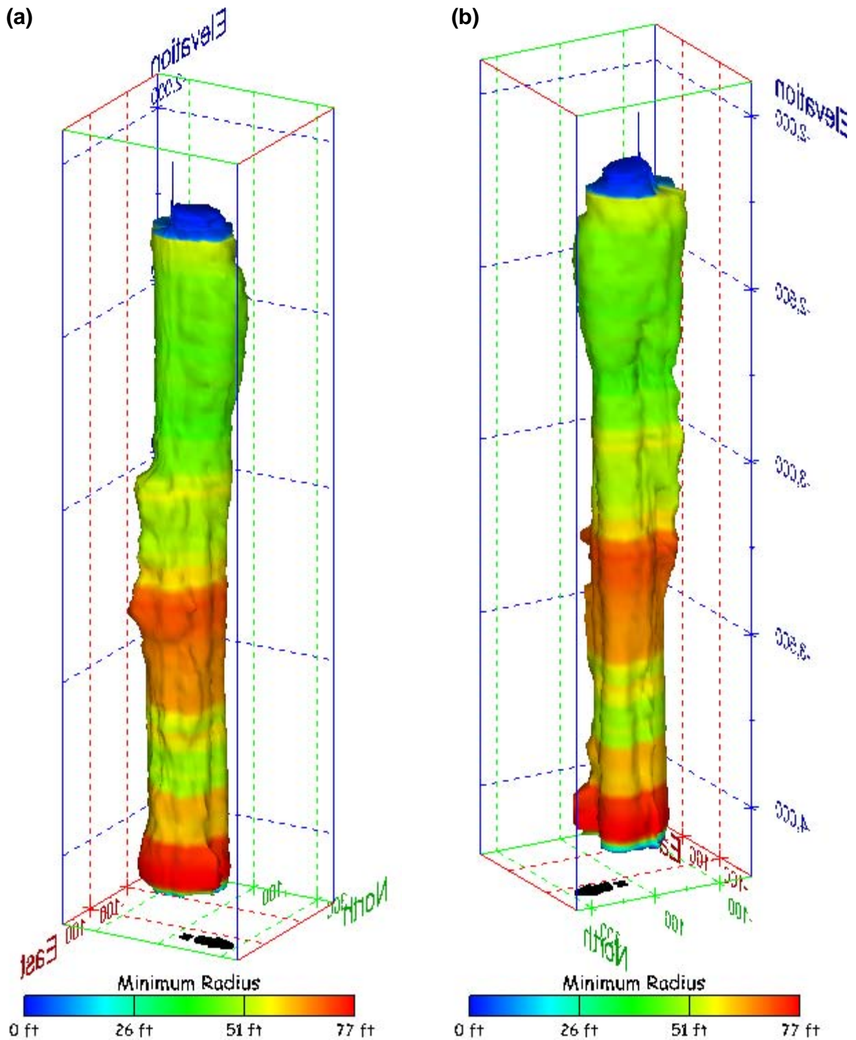
Figure 337. Sonar images of cavern BM-108, showing the geometry of the cavern colored by minimum radius. View from (a) azimuth 60°, elevation 20°; (b) azimuth 300°, elevation 20°.
