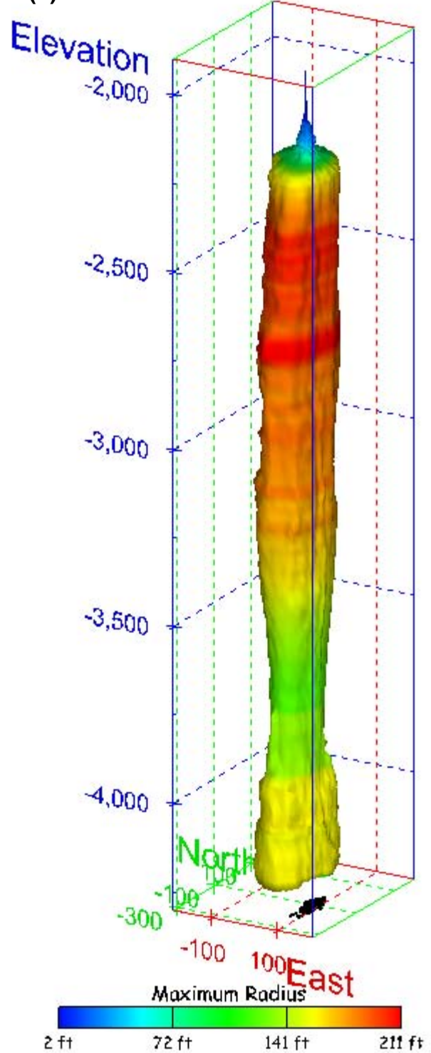
Figure 182. Sonar images of cavern BM-102, showing the geometry of the cavern colored by maximum radius. View from (a) azimuth 210°, elevation 20°; (b) azimuth 150°, elevation 20°.
