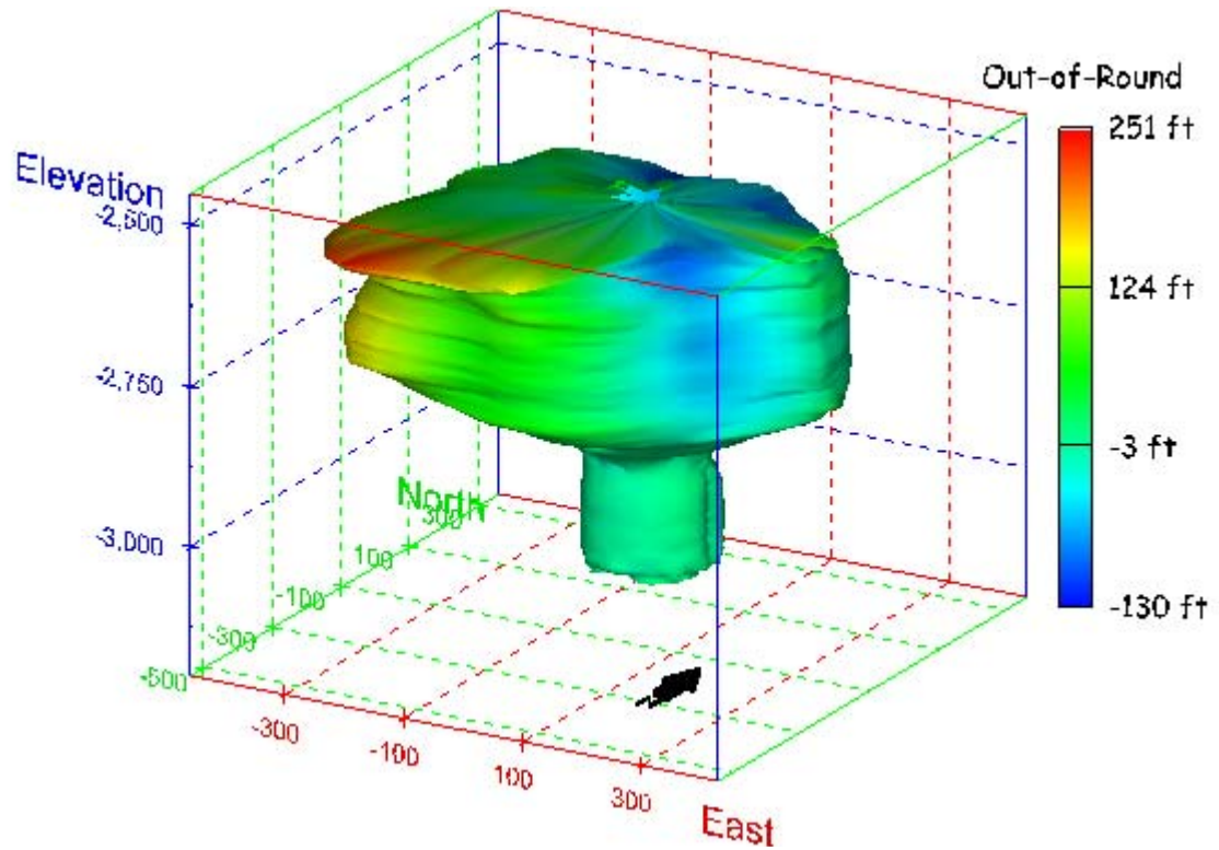
Figure 108. Sonar images of cavern BM-4, showing the geometry of the cavern colored by out-of-round distance. View from (a) azimuth 210°, elevation 20°; (b) azimuth 150°, elevation 20°.
