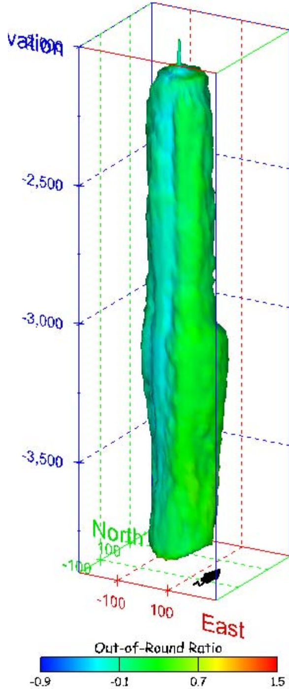
Figure 292. Sonar images of cavern BM-106, showing the geometry of the cavern colored by out-of-round ratio. View from (a) azimuth 210°, elevation 20°; (b) azimuth 150°, elevation 20°.
