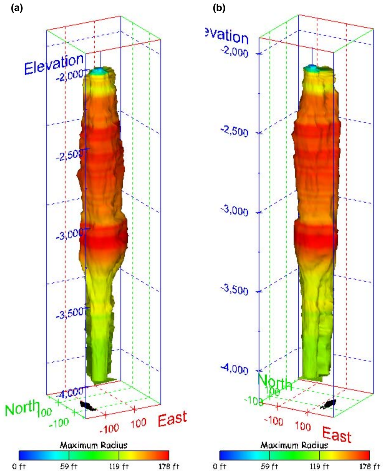
Figure 390. Sonar images of cavern BM-110, showing the geometry of the cavern colored by maximum radius. View from (a) azimuth 210°, elevation 20°; (b) azimuth 150°, elevation 20°.
