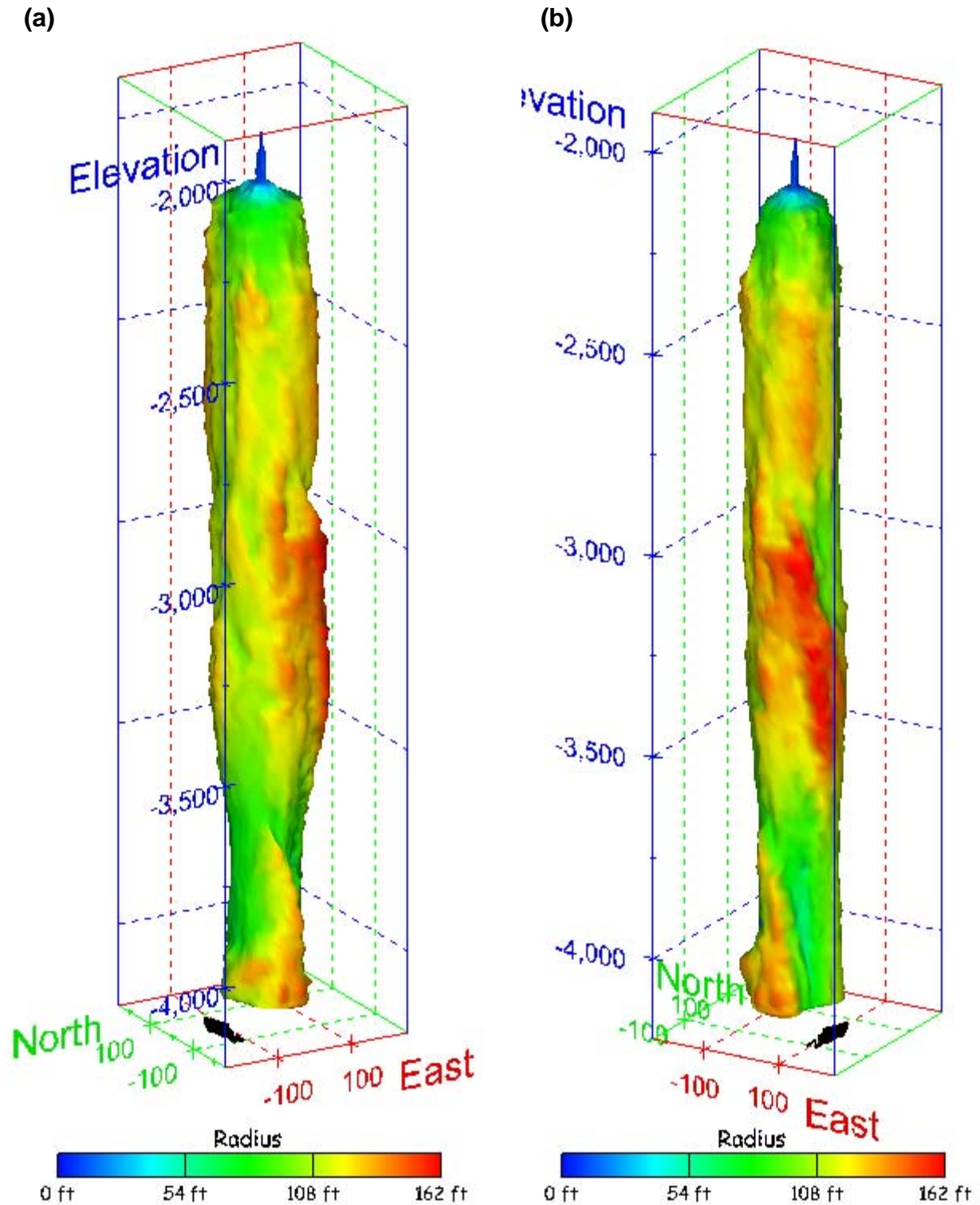
Figure 408. Sonar images of cavern BM-111, showing the geometry of the cavern colored by measured radius. View from (a) azimuth 210°, elevation 20°; (b) azimuth 150°, elevation 20°.
