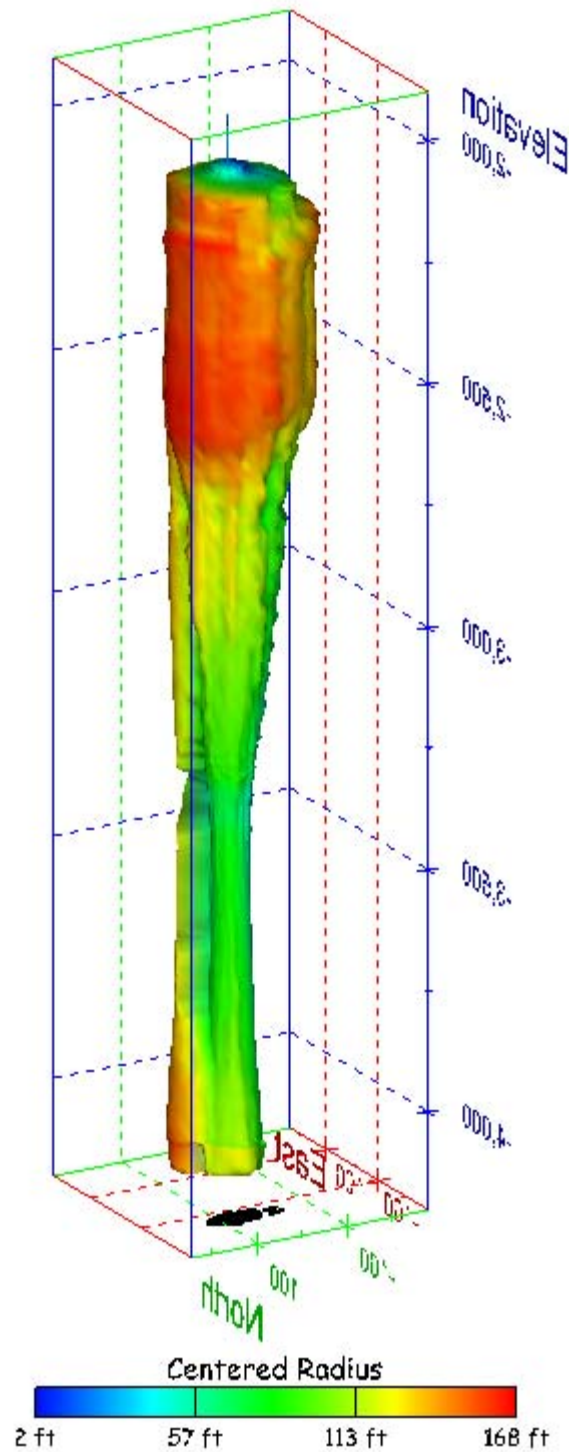
Figure 229. Sonar images of cavern BM-104, showing the geometry of the cavern colored by centered radius. View from (a) azimuth 60°, elevation 20°; (b) azimuth 300°, elevation 20°.
