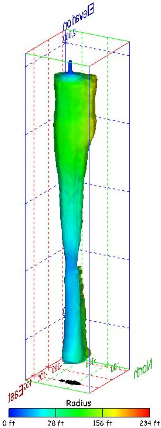
Figure 253. Sonar images of cavern BM-105, showing the geometry of the cavern colored by measured radius. View from (a) azimuth 60°, elevation 20°; (b) azimuth 300°, elevation 20°.
