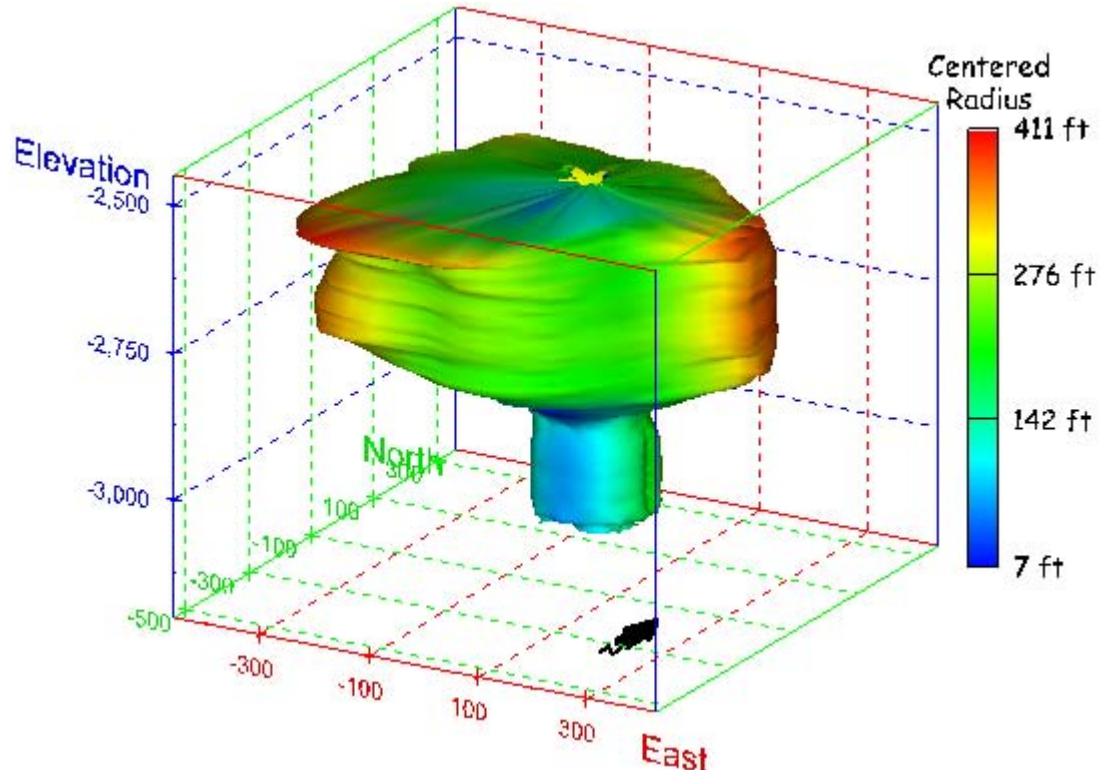
Figure 98. Sonar images of cavern BM-4, showing the geometry of the cavern colored by centered radius. View from (a) azimuth 210°, elevation 20°; (b) azimuth 150°, elevation 20°.
