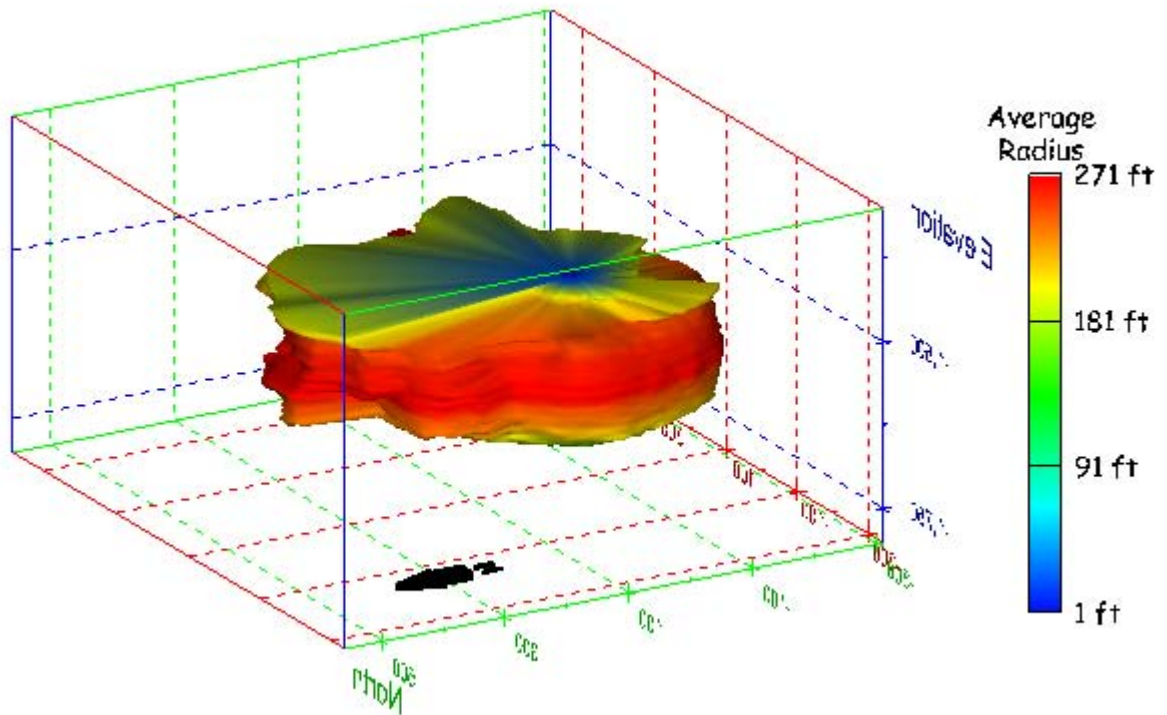
Figure 49. Sonar images of cavern BM-2, showing the geometry of the cavern colored by average radius. View from (a) azimuth 60°, elevation 20°; (b) azimuth 300°, elevation 20°.
