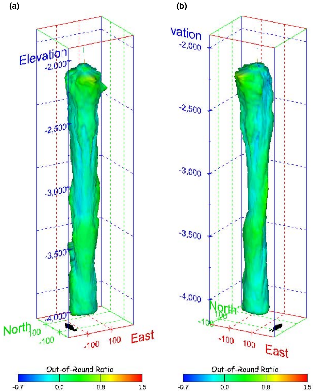
Figure 526. Sonar images of cavern BM-115, showing the geometry of the cavern colored by out-of-round ratio. View from (a) azimuth 210°, elevation 20°; (b) azimuth 150°, elevation 20°.
