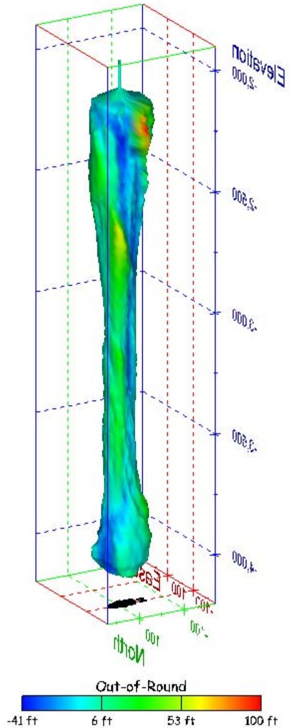
Figure 499. Sonar images of cavern BM-114, showing the geometry of the cavern colored by out-of-round distance. View from (a) azimuth 60°, elevation 20°; (b) azimuth 300°, elevation 20°.
