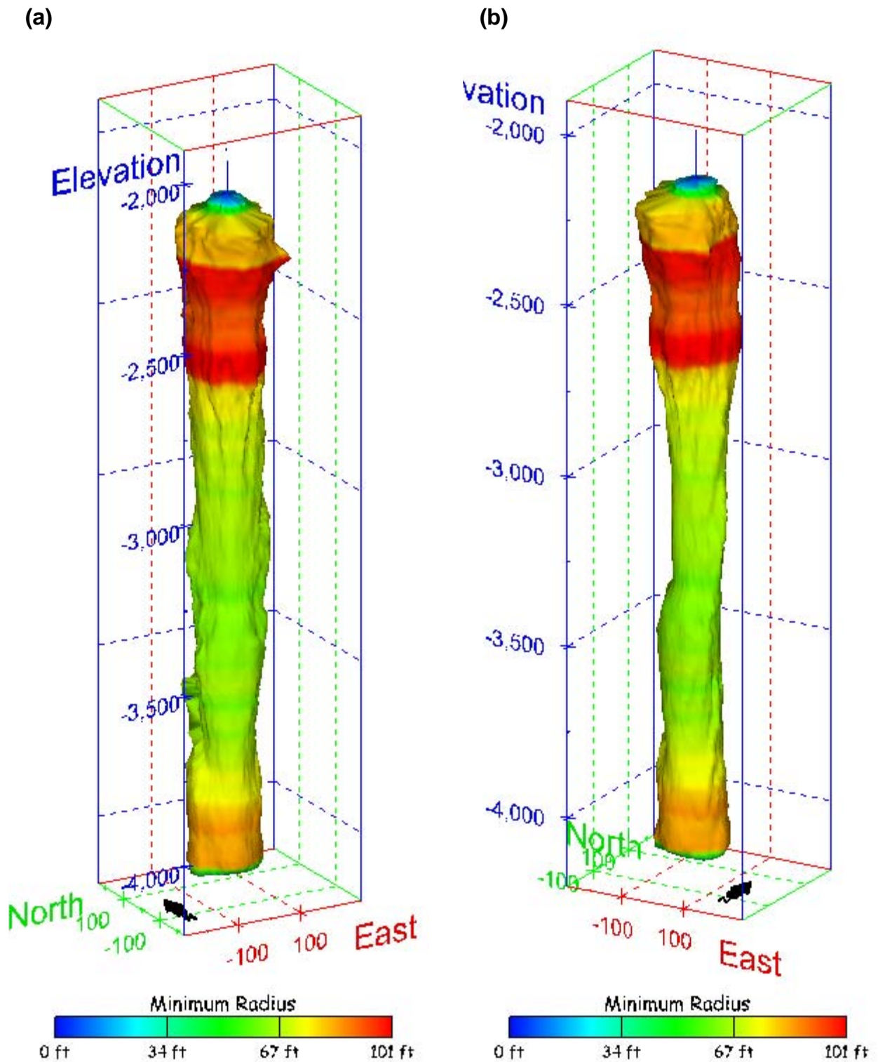
Figure 518. Sonar images of cavern BM-115, showing the geometry of the cavern colored by minimum radius. View from (a) azimuth 210°, elevation 20°; (b) azimuth 150°, elevation 20°.
