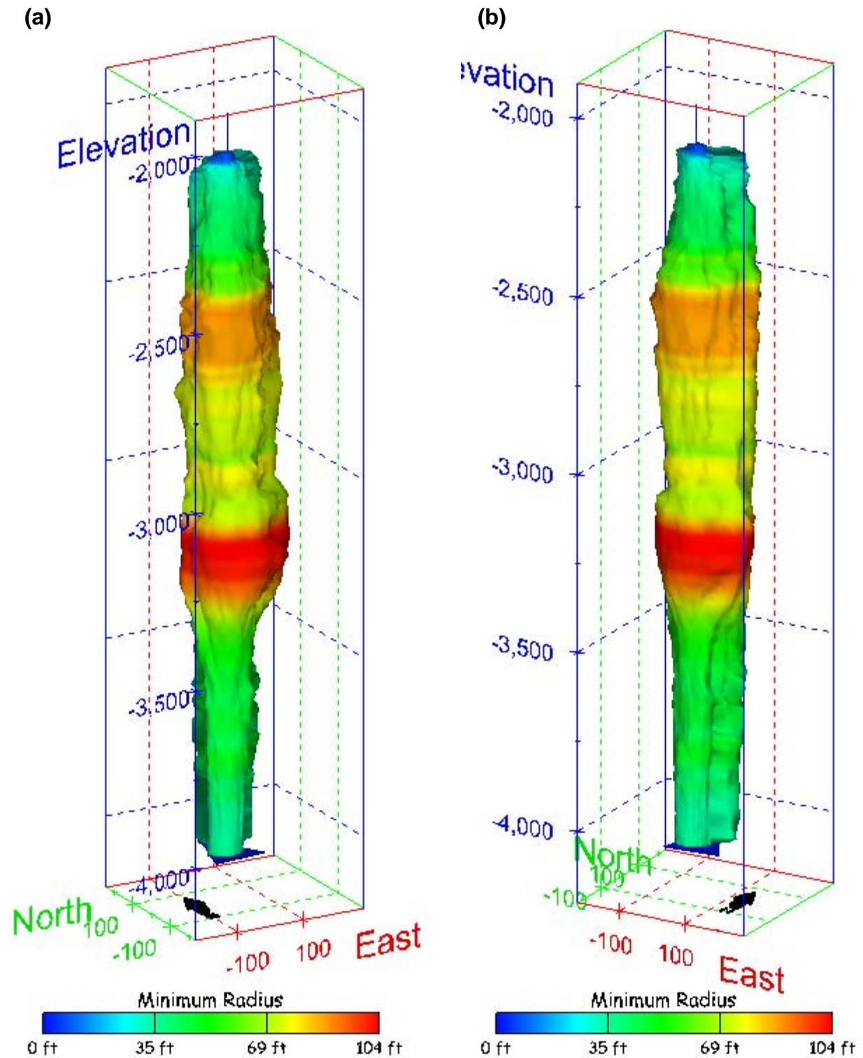
Figure 388. Sonar images of cavern BM-110, showing the geometry of the cavern colored by minimum radius. View from (a) azimuth 210°, elevation 20°; (b) azimuth 150°, elevation 20°.
