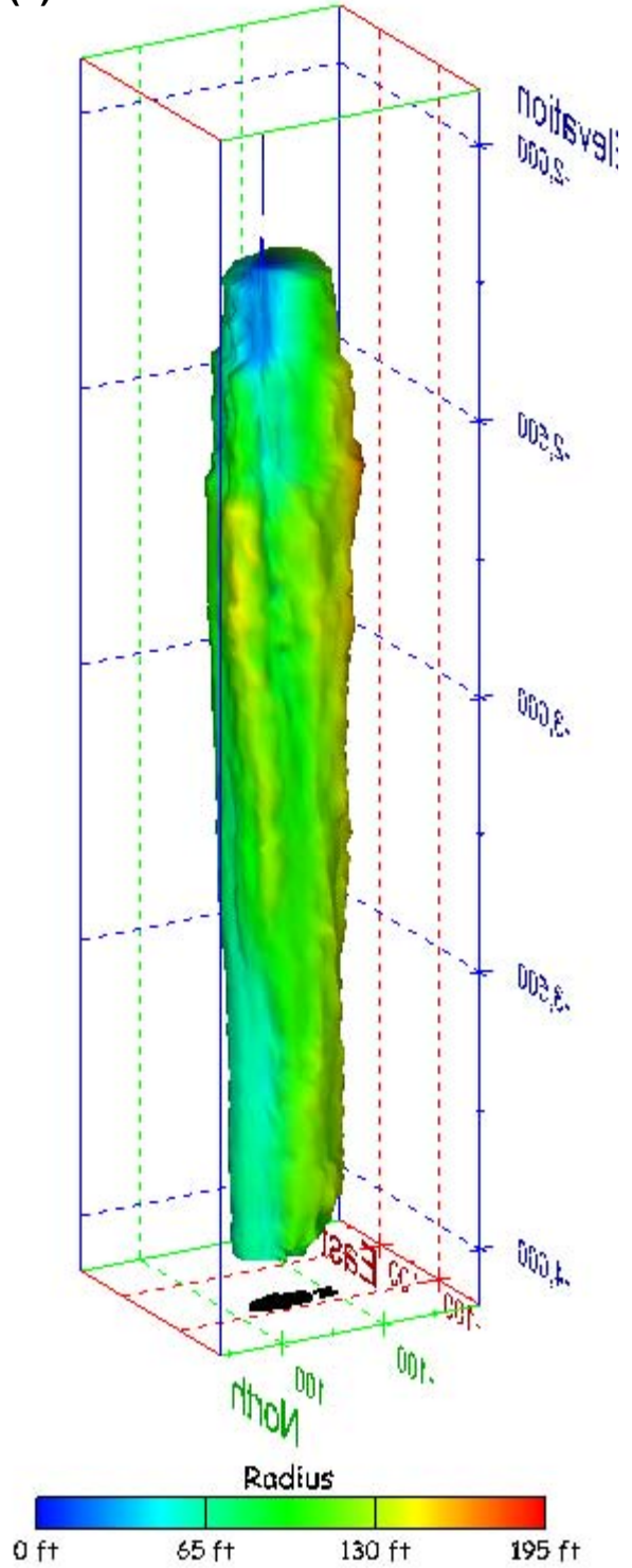
Figure 305. Sonar images of cavern BM-107, showing the geometry of the cavern colored by measured radius. View from (a) azimuth 60°, elevation 20°; (b) azimuth 300°, elevation 20°.
