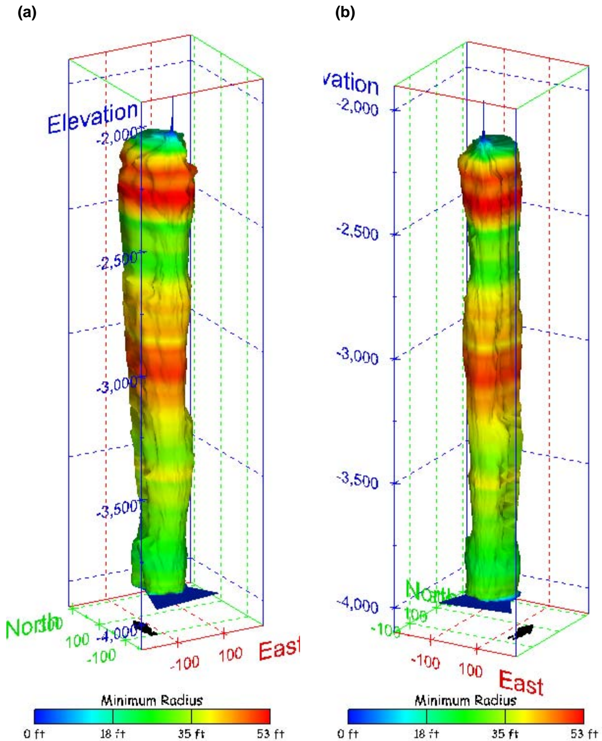
Figure 440. Sonar images of cavern BM-112, showing the geometry of the cavern colored by minimum radius. View from (a) azimuth 210°, elevation 20°; (b) azimuth 150°, elevation 20°.
