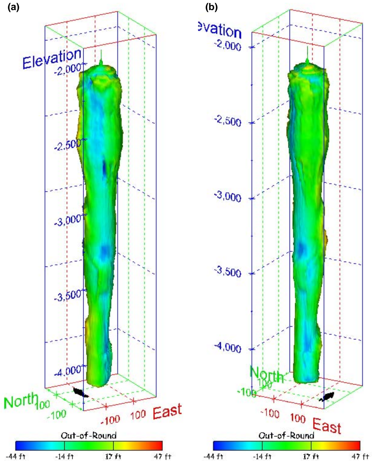
Figure 550. Sonar images of cavern BM-116, showing the geometry of the cavern colored by out-of-round distance. View from (a) azimuth 210°, elevation 20°; (b) azimuth 150°, elevation 20°.
