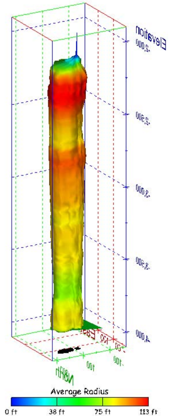
Figure 439. Sonar images of cavern BM-112, showing the geometry of the cavern colored by average radius. View from (a) azimuth 60°, elevation 20°; (b) azimuth 300°, elevation 20°.
