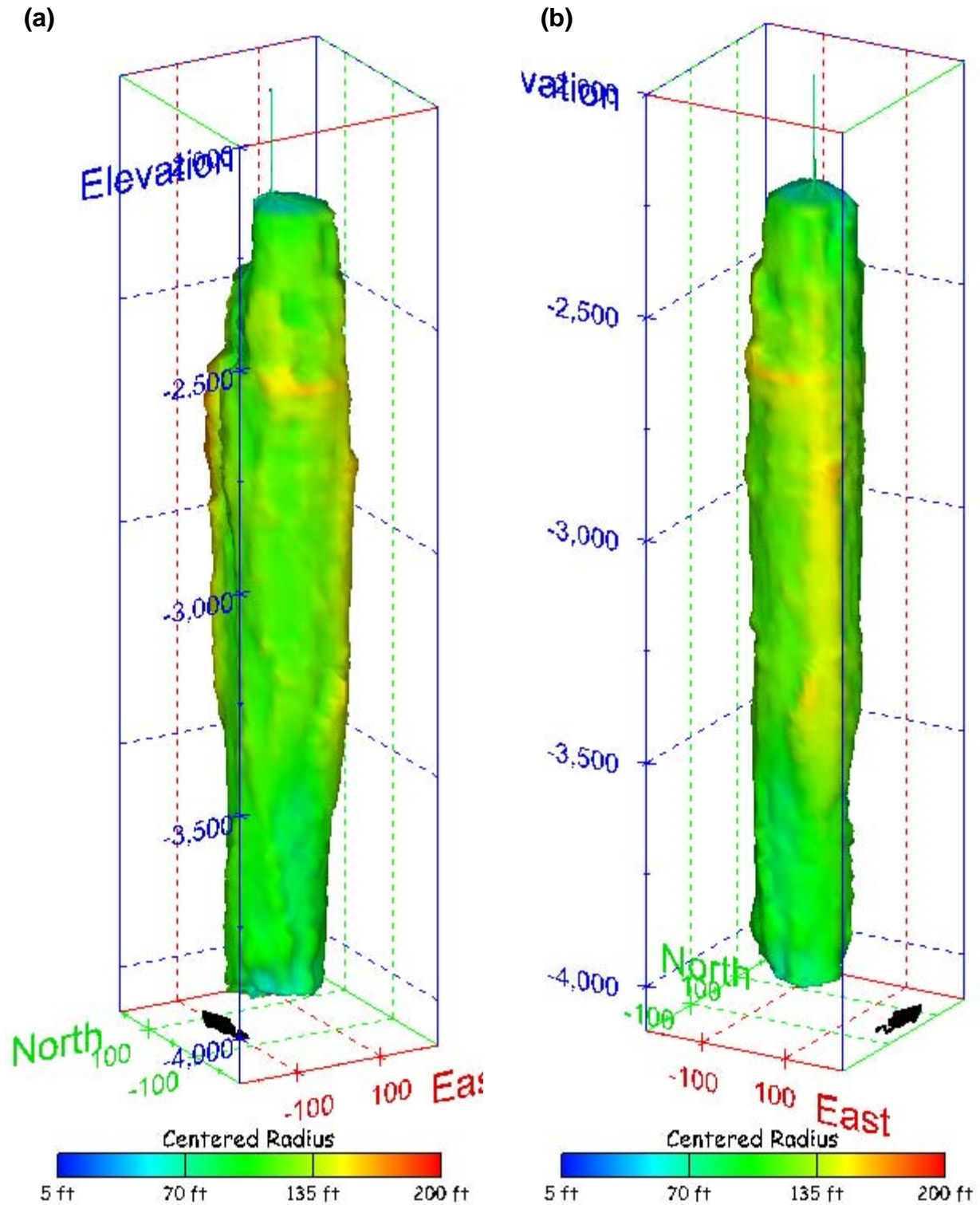
Figure 306. Sonar images of cavern BM-107, showing the geometry of the cavern colored by centered radius. View from (a) azimuth 210°, elevation 20°; (b) azimuth 150°, elevation 20°.
