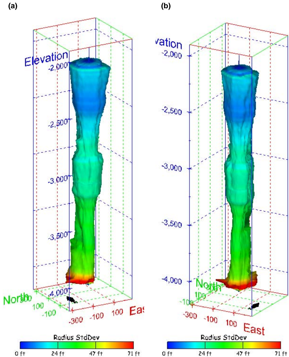
Figure 366. Sonar images of cavern BM-109, showing the geometry of the cavern colored by radius standard deviation. View from (a) azimuth 210°, elevation 20°; (b) azimuth 150°, elevation 20°.
