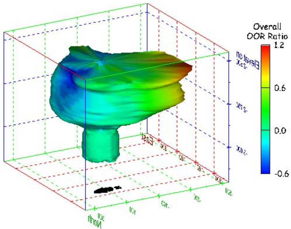
Figure 113. Sonar images of cavern BM-4, showing the geometry of the cavern colored by overall out-of-round ratio. View from (a) azimuth 60°, elevation 20°; (b) azimuth 300°, elevation 20°.
