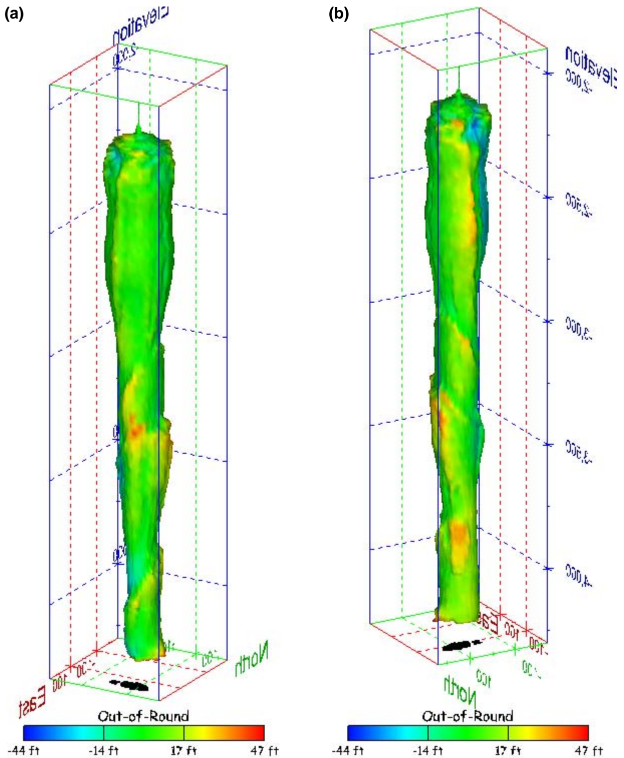
Figure 551. Sonar images of cavern BM-116, showing the geometry of the cavern colored by out-of-round distance. View from (a) azimuth 60°, elevation 20°; (b) azimuth 300°, elevation 20°.
