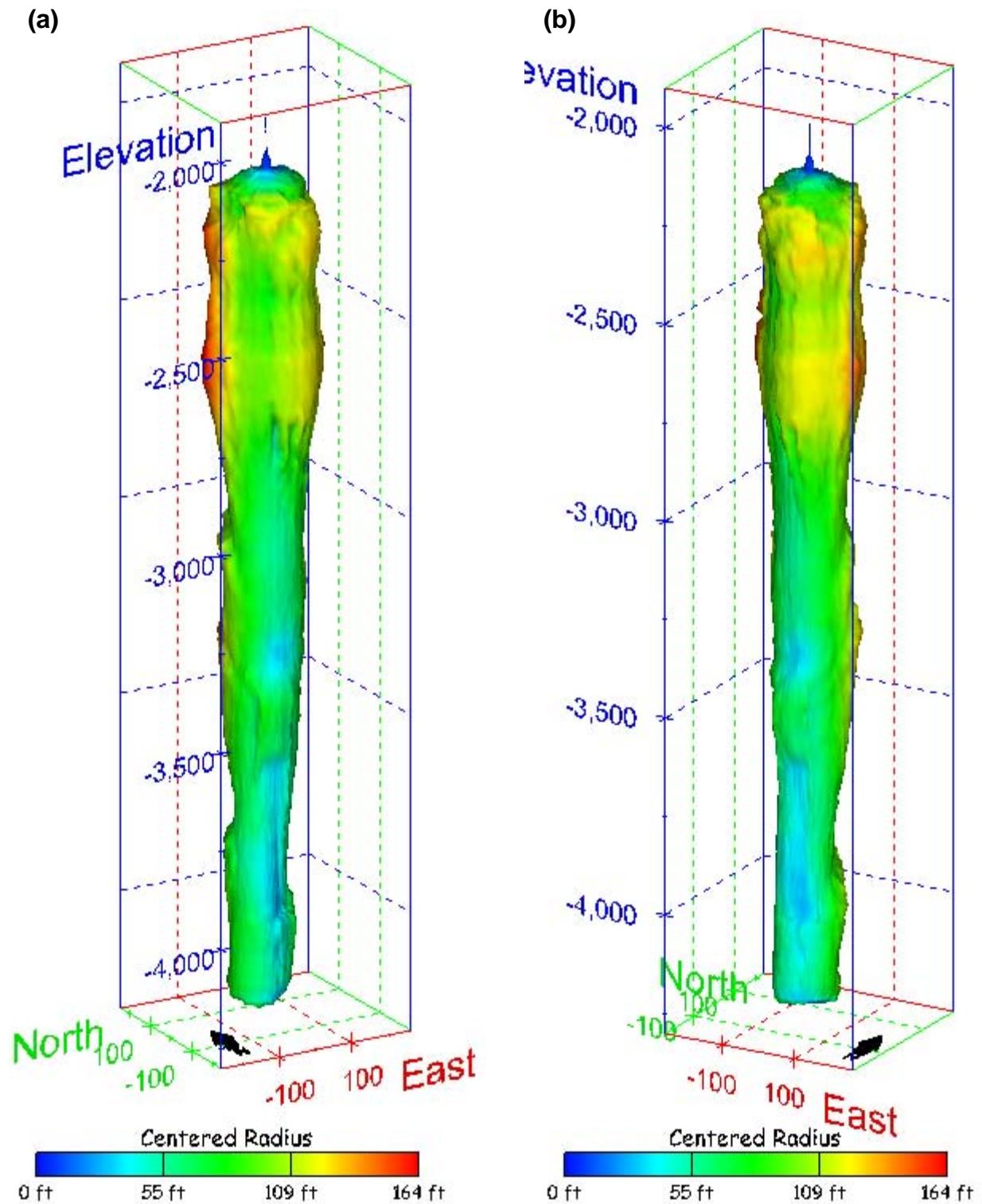
Figure 540. Sonar images of cavern BM-116, showing the geometry of the cavern colored by centered radius. View from (a) azimuth 210°, elevation 20°; (b) azimuth 150°, elevation 20°.
