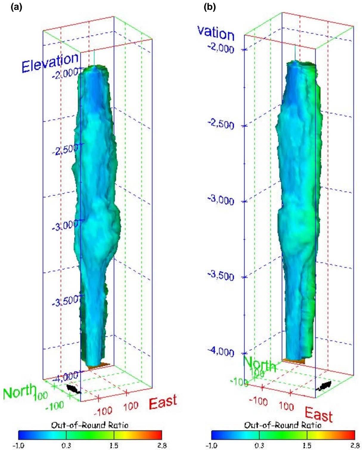
Figure 396. Sonar images of cavern BM-110, showing the geometry of the cavern colored by out-of-round ratio. View from (a) azimuth 210°, elevation 20°; (b) azimuth 150°, elevation 20°.
