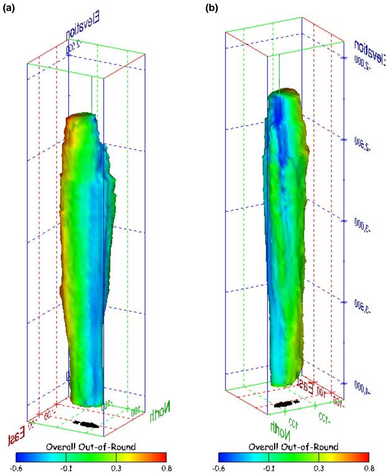
Figure 321. Sonar images of cavern BM-107, showing the geometry of the cavern colored by overall out-of-round ratio. View from (a) azimuth 60°, elevation 20°; (b) azimuth 300°, elevation 20°.
