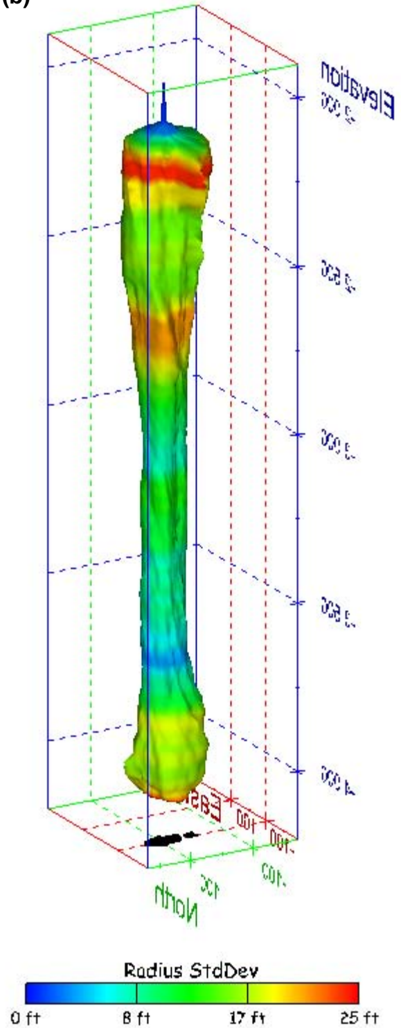
Figure 497. Sonar images of cavern BM-114, showing the geometry of the cavern colored by radius standard deviation. View from (a) azimuth 60°, elevation 20°; (b) azimuth 300°, elevation 20°.
