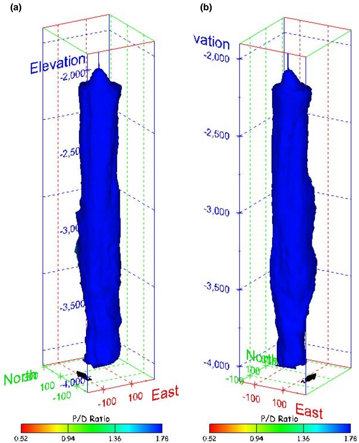
Figure 220. Sonar images of cavern BM-103, showing the geometry of the cavern colored by three-dimensional pillar-to-diameter ratio. View from (a) azimuth 210°, elevation 20°; (b) azimuth 150°, elevation 20°.
