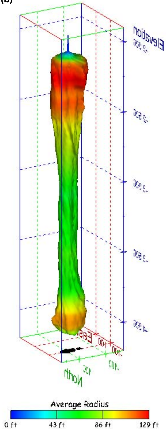
Figure 491. Sonar images of cavern BM-114, showing the geometry of the cavern colored by average radius. View from (a) azimuth 60°, elevation 20°; (b) azimuth 300°, elevation 20°.
