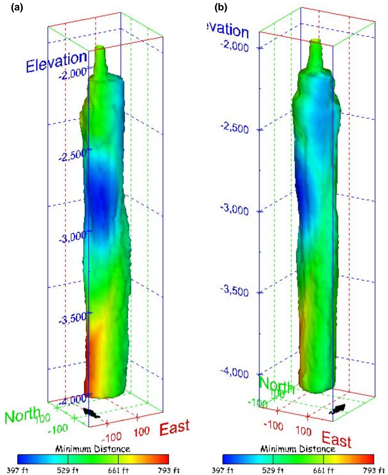
Figure 166. Sonar images of cavern BM-101, showing the geometry of the cavern colored by the minimum distance to the nearest neighboring cavern. View from (a) azimuth 210°, elevation 20°; (b) azimuth 150°, elevation 20°.
