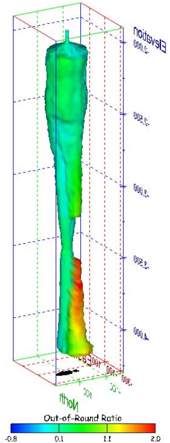
Figure 267. Sonar images of cavern BM-105, showing the geometry of the cavern colored by out-of-round ratio. View from (a) azimuth 60°, elevation 20°; (b) azimuth 300°, elevation 20°.
