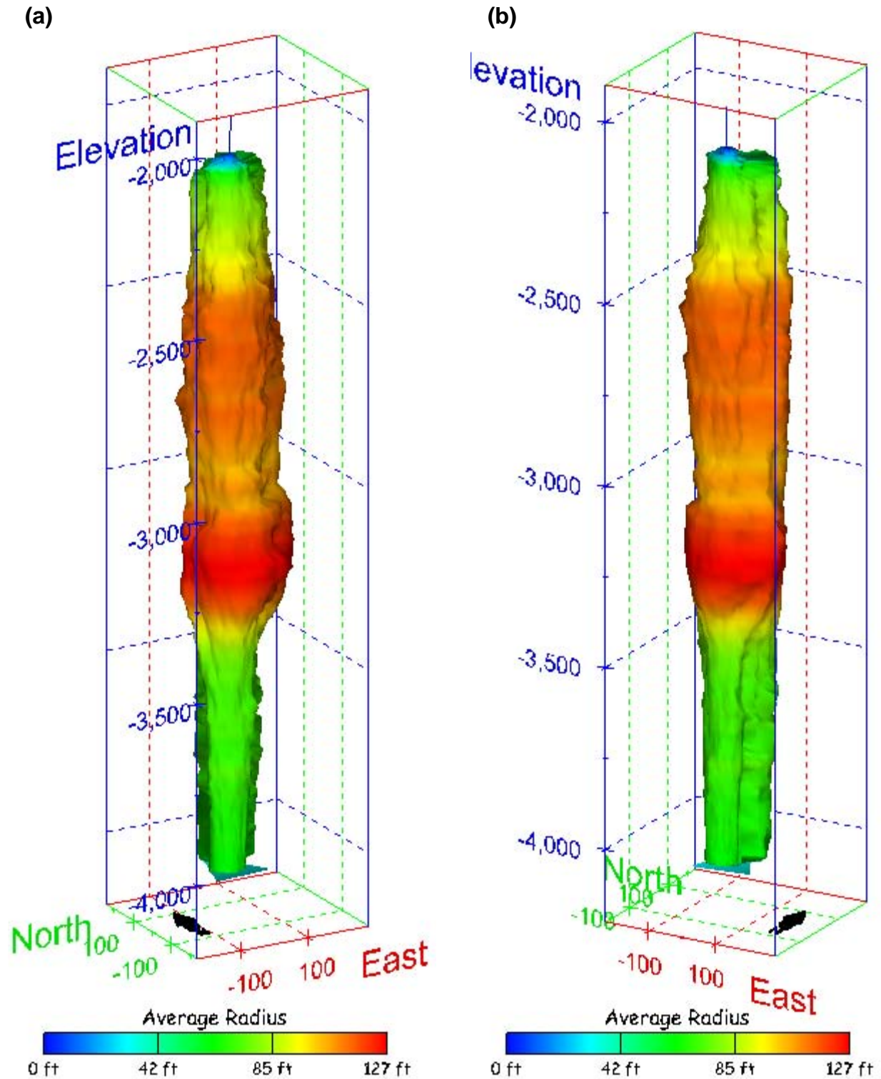
Figure 386. Sonar images of cavern BM-110, showing the geometry of the cavern colored by average radius. View from (a) azimuth 210°, elevation 20°; (b) azimuth 150°, elevation 20°.
