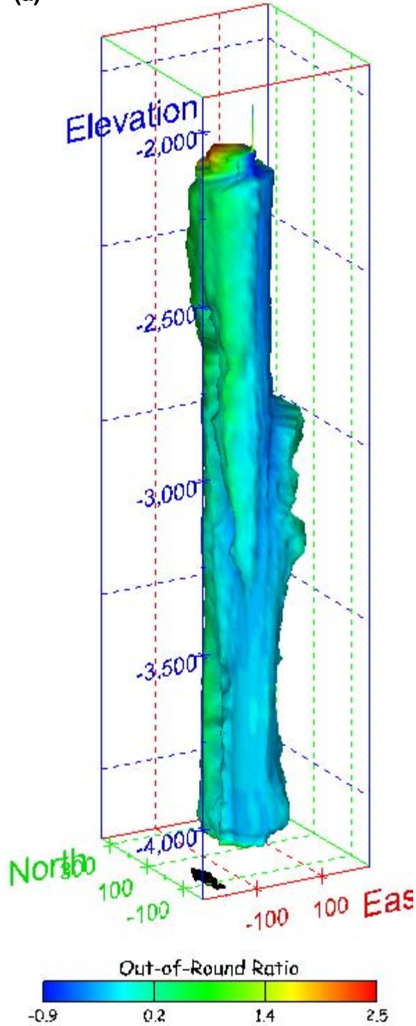
Figure 344. Sonar images of cavern BM-108, showing the geometry of the cavern colored by out-of-round ratio. View from (a) azimuth 210°, elevation 20°; (b) azimuth 150°, elevation 20°.
