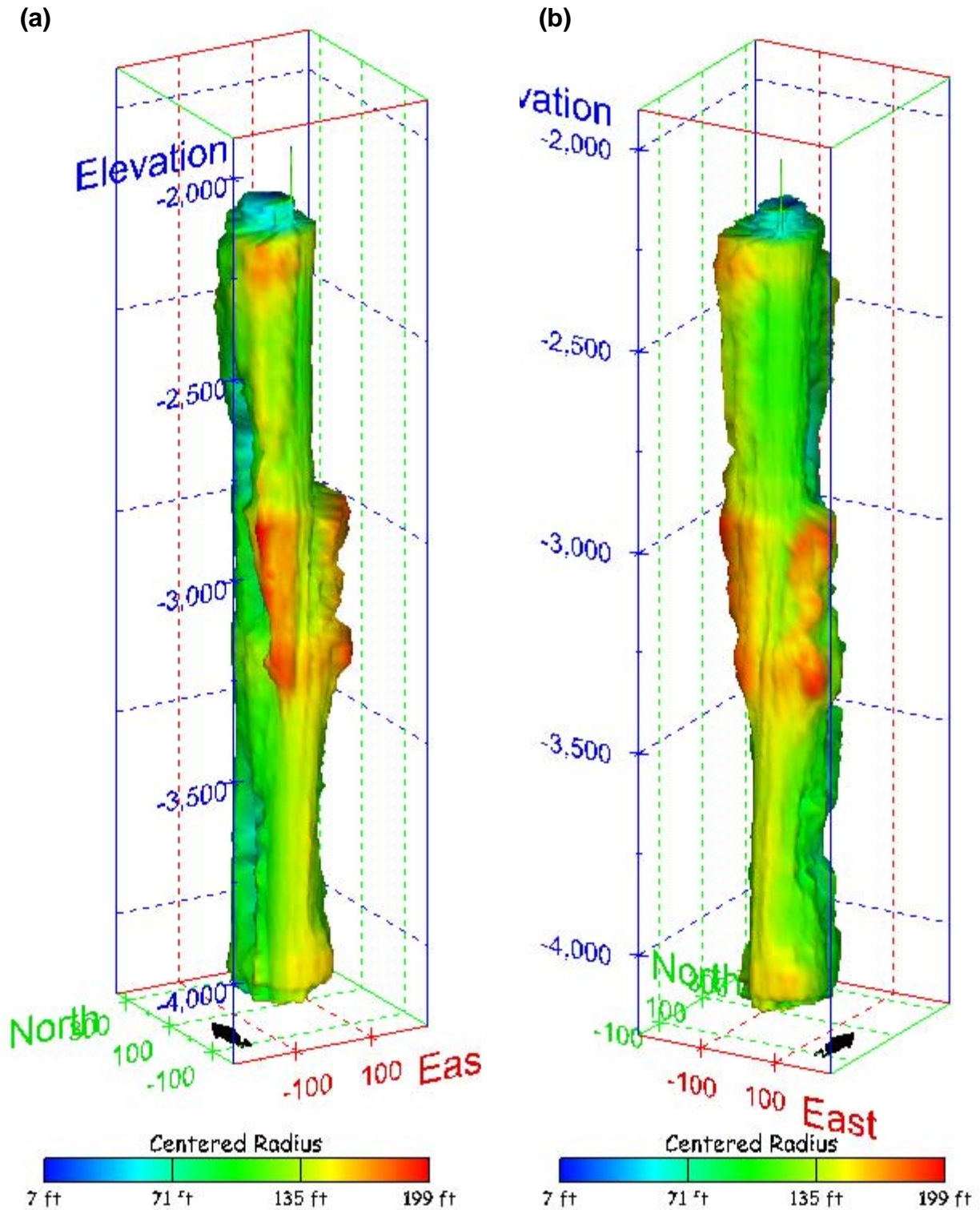
Figure 332. Sonar images of cavern BM-108, showing the geometry of the cavern colored by centered radius. View from (a) azimuth 210°, elevation 20°; (b) azimuth 150°, elevation 20°.
