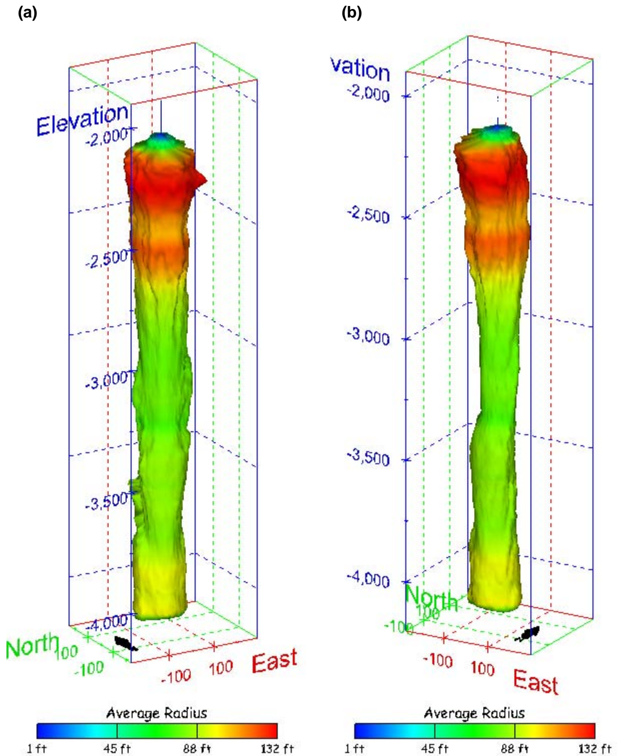
Figure 516. Sonar images of cavern BM-115, showing the geometry of the cavern colored by average radius. View from (a) azimuth 210°, elevation 20°; (b) azimuth 150°, elevation 20°.
