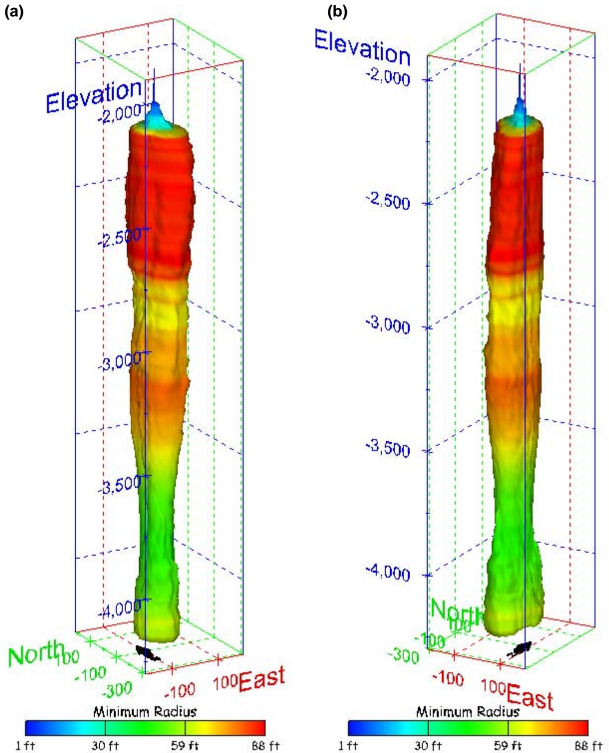
Figure 180. Sonar images of cavern BM-102, showing the geometry of the cavern colored by minimum radius. View from (a) azimuth 210°, elevation 20°; (b) azimuth 150°, elevation 20°.
