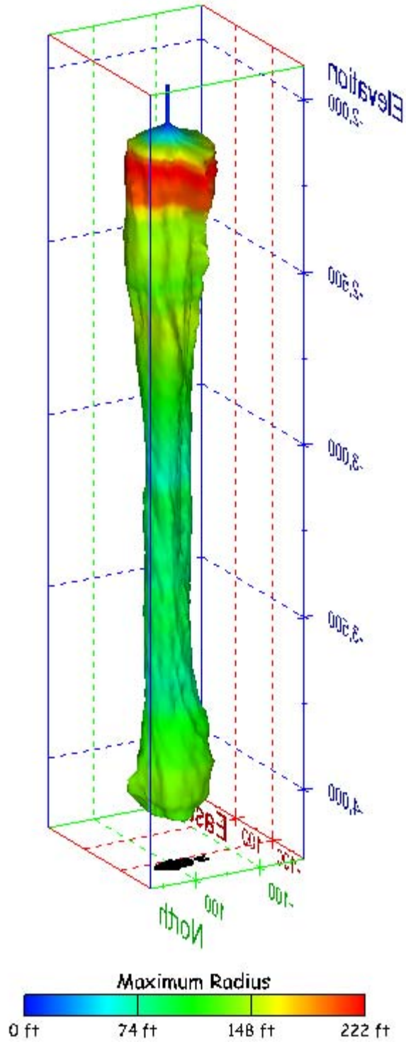
Figure 495. Sonar images of cavern BM-114, showing the geometry of the cavern colored by maximum radius. View from (a) azimuth 60°, elevation 20°; (b) azimuth 300°, elevation 20°.
