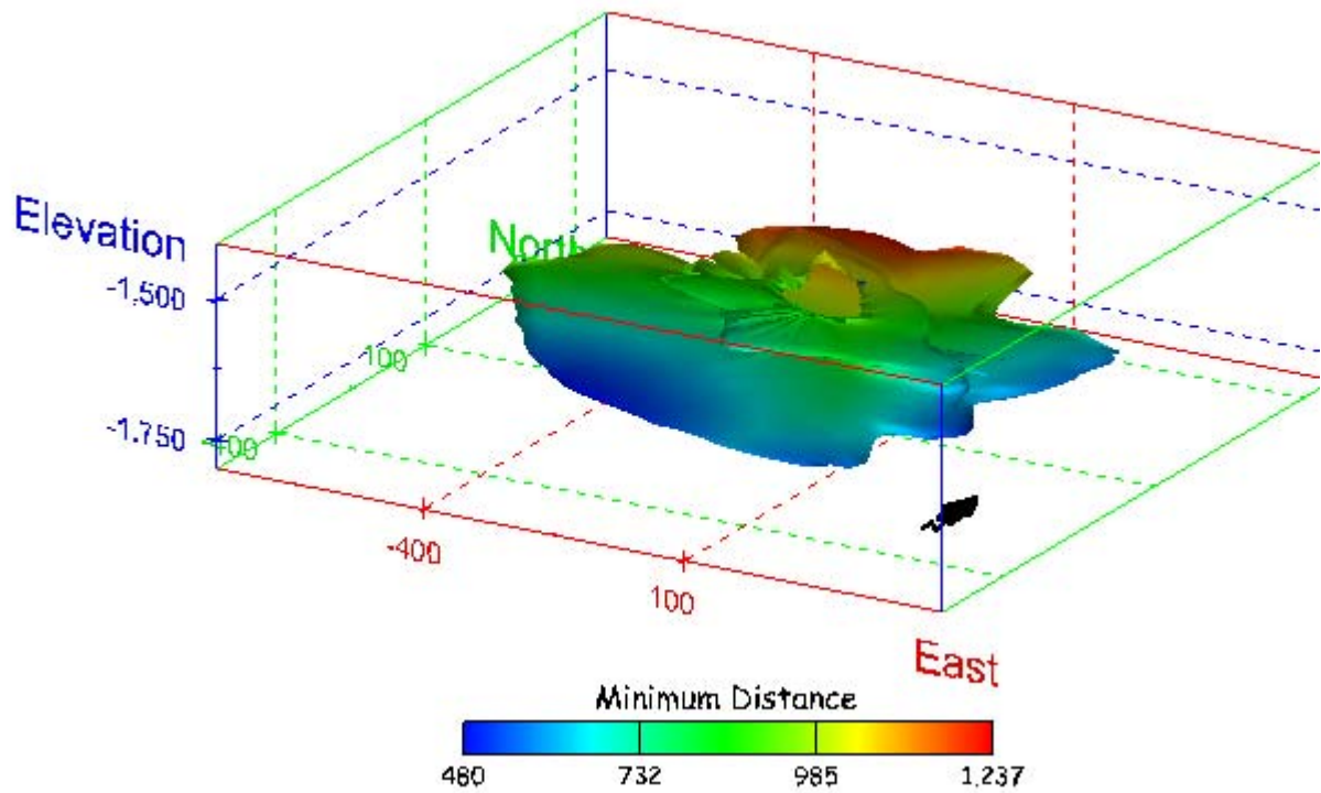
Figure 88. Sonar images of cavern BM-3, showing the geometry of the cavern colored by the minimum distance to the nearest neighboring cavern. View from (a) azimuth 210°, elevation 20°; (b) azimuth 150°, elevation 20°.
