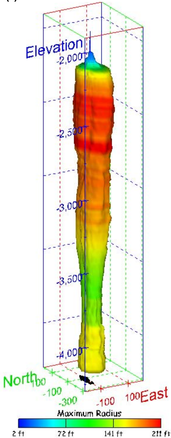
Figure 182. Sonar images of cavern BM-102, showing the geometry of the cavern colored by maximum radius. View from (a) azimuth 210°, elevation 20°; (b) azimuth 150°, elevation 20°.
