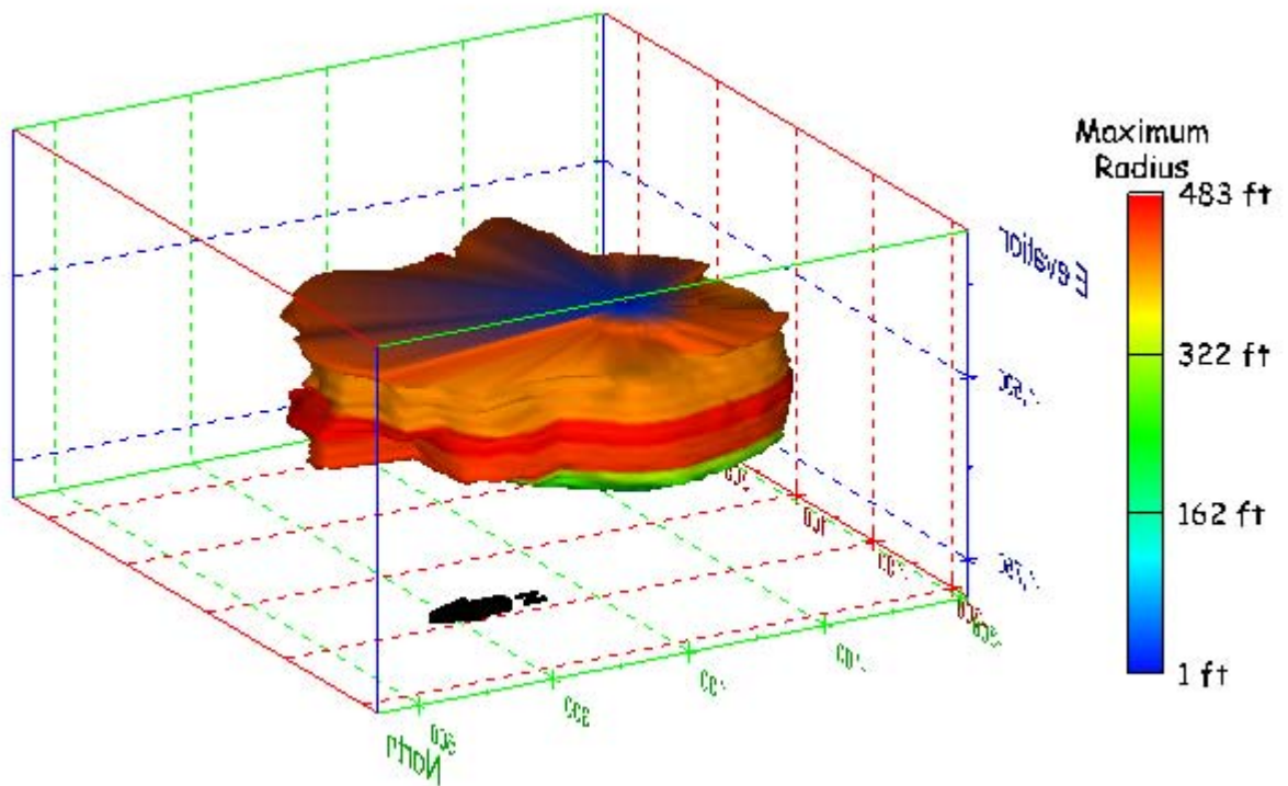
Figure 53. Sonar images of cavern BM-2, showing the geometry of the cavern colored by maximum radius. View from (a) azimuth 60°, elevation 20°; (b) azimuth 300°, elevation 20°.
