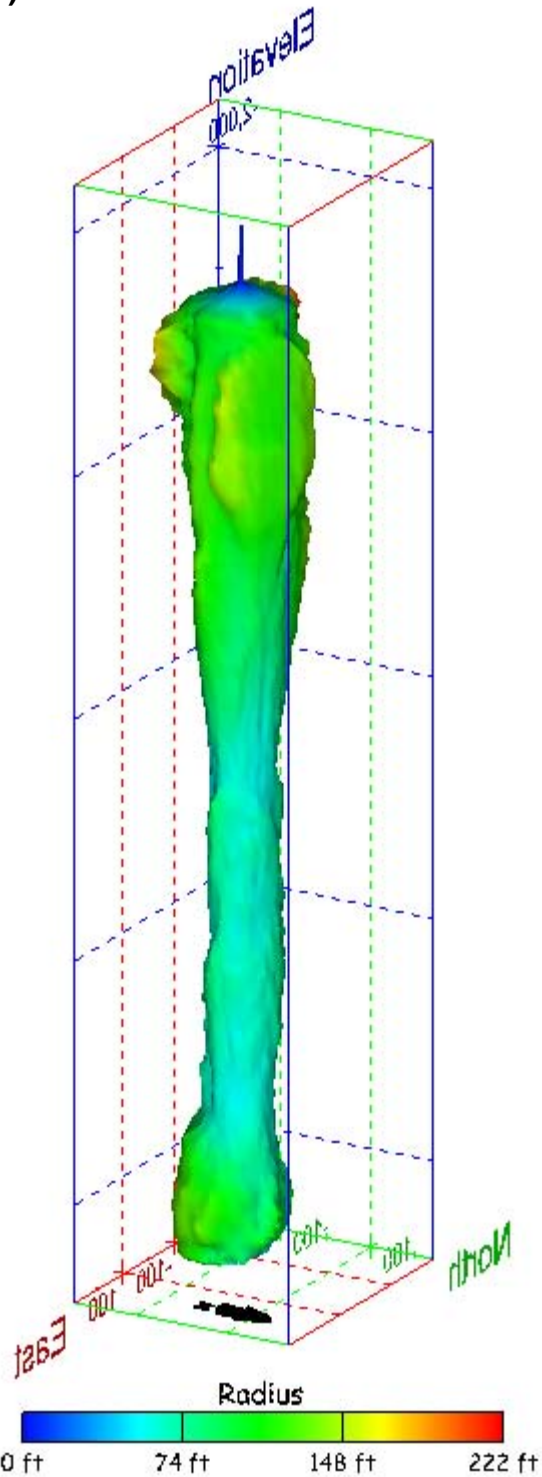
Figure 487. Sonar images of cavern BM-114, showing the geometry of the cavern colored by measured radius. View from (a) azimuth 60°, elevation 20°; (b) azimuth 300°, elevation 20°.
