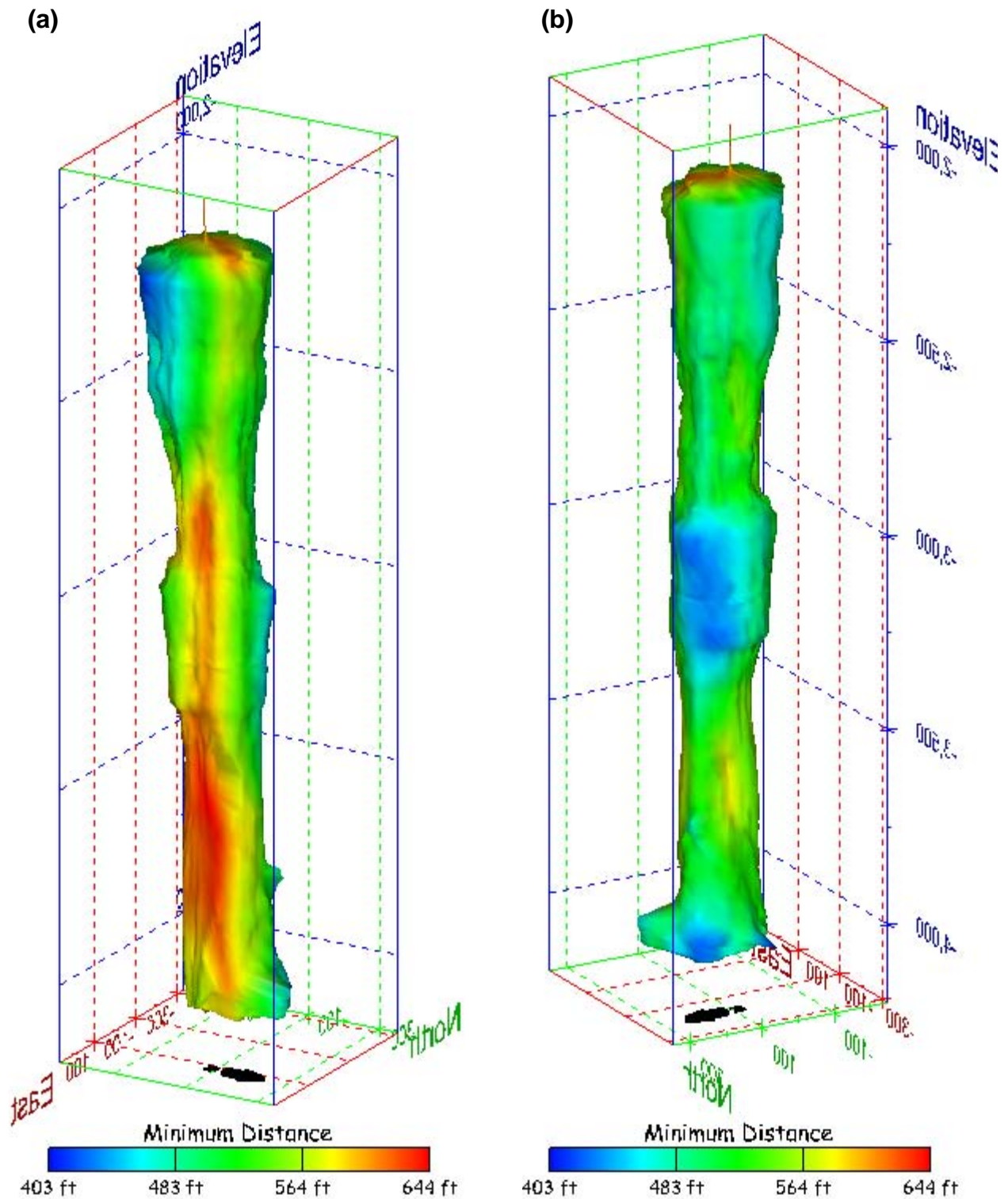
Figure 375. Sonar images of cavern BM-109, showing the geometry of the cavern colored by minimum distance to the nearest neighboring cavern. View from (a) azimuth 60°, elevation 20°; (b) azimuth 300°, elevation 20°.
