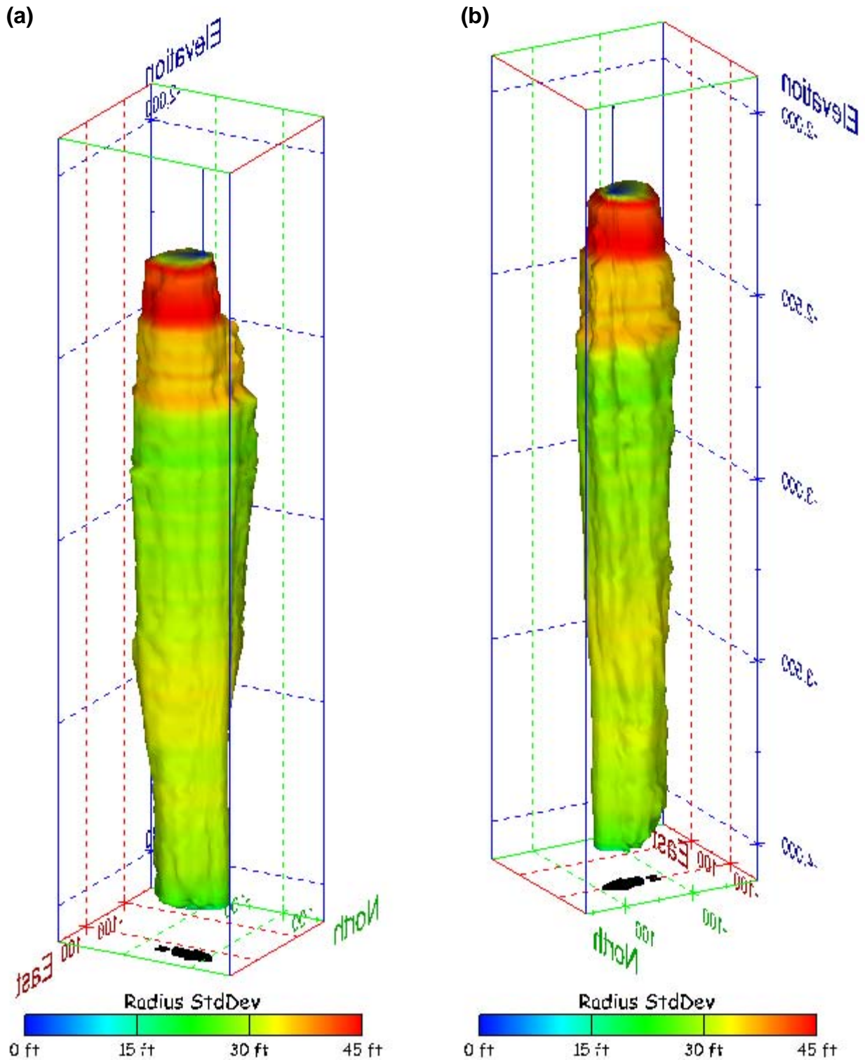
Figure 315. Sonar images of cavern BM-107, showing the geometry of the cavern colored by radius standard deviation. View from (a) azimuth 60°, elevation 20°; (b) azimuth 300°, elevation 20°.
