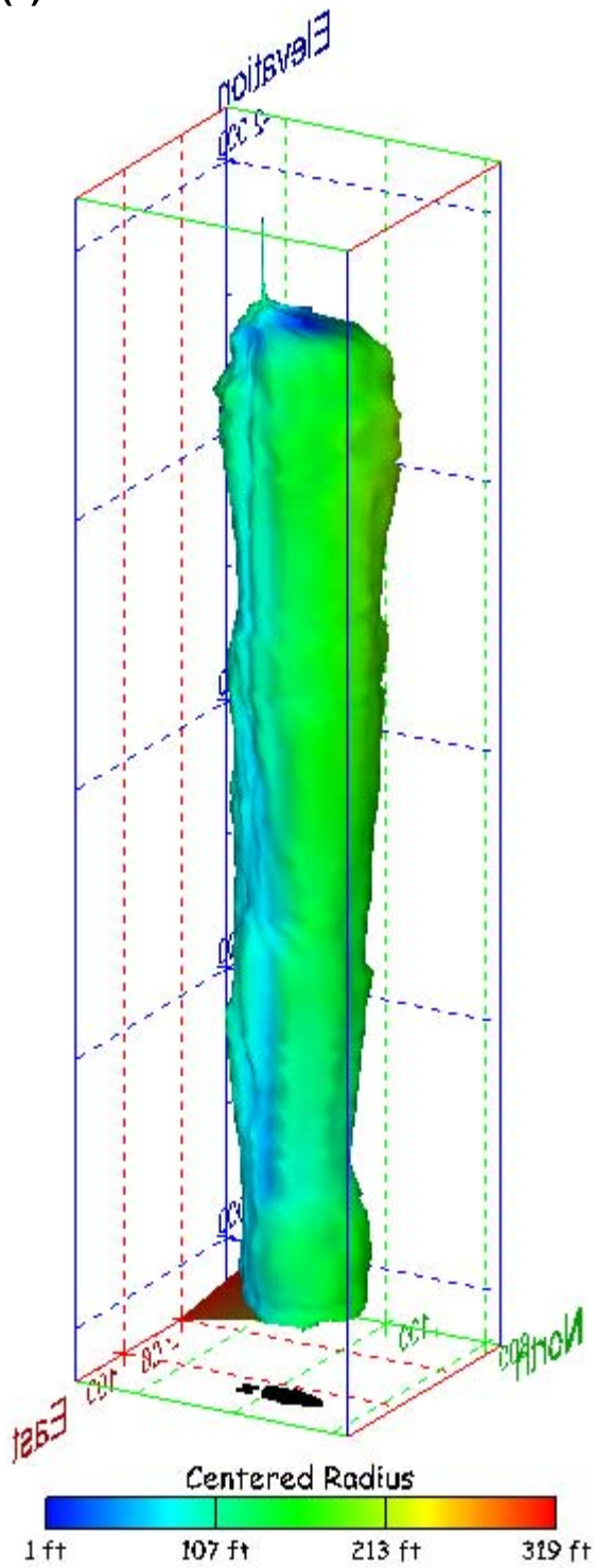
Figure 437. Sonar images of cavern BM-112, showing the geometry of the cavern colored by centered radius. View from (a) azimuth 60°, elevation 20°; (b) azimuth 300°, elevation 20°.
