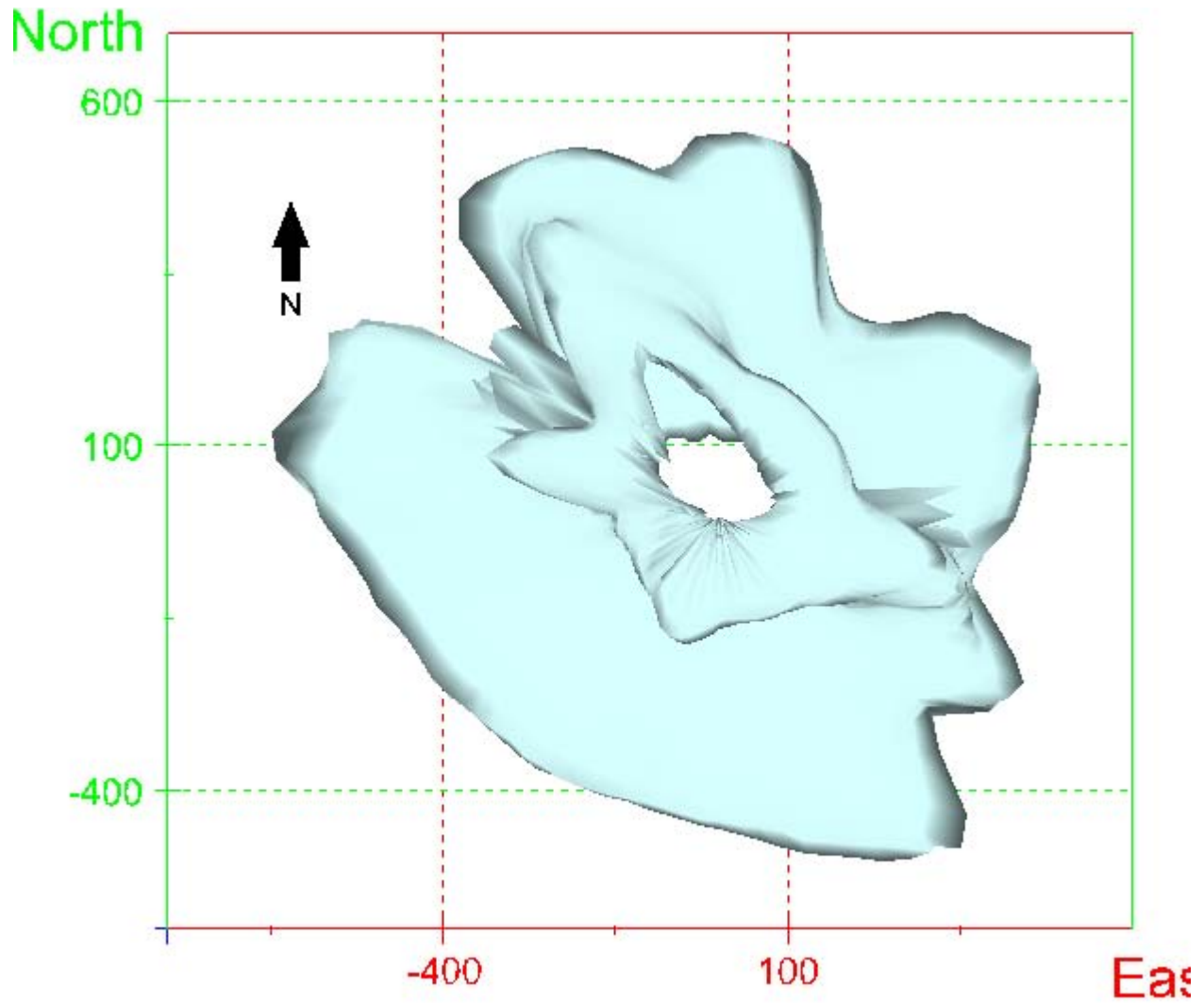
Figure 67. Map view sonar image of cavern BM-3, showing the basic geometry of the cavern. Grid squares represent 500 ft. The open “center” of the image is an artifact of the particular sonar survey used.
