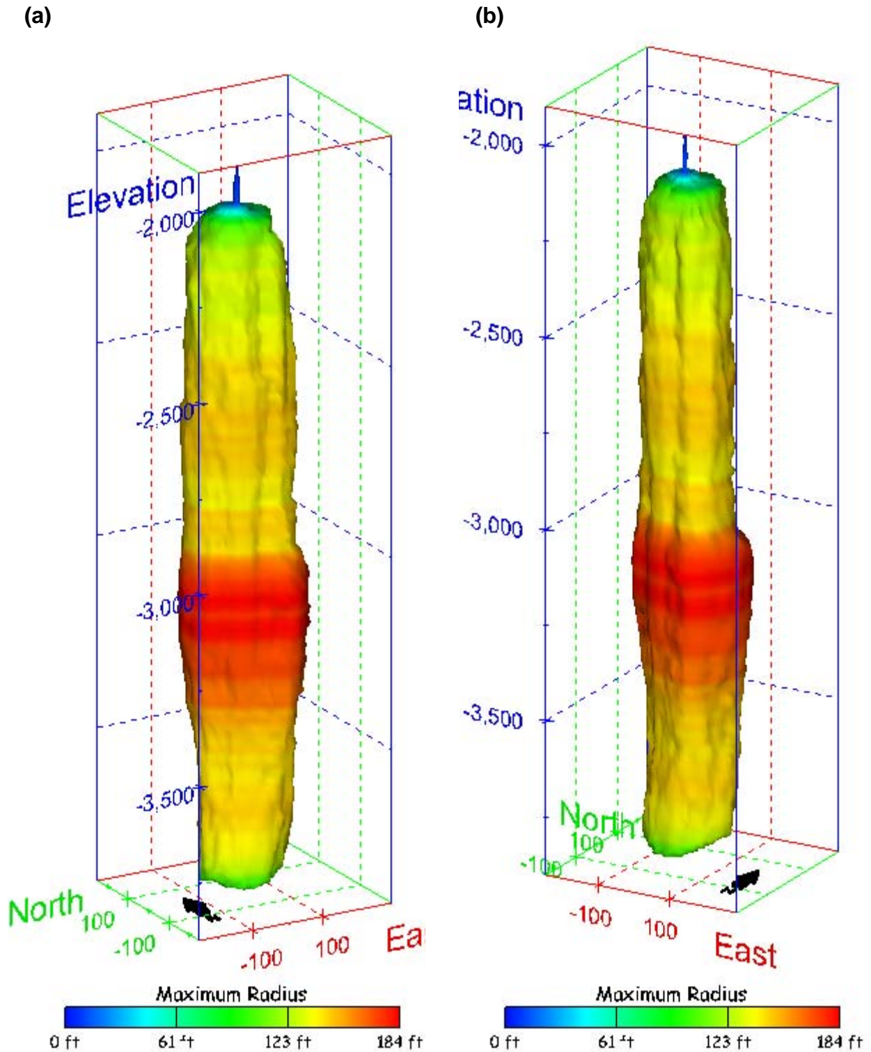
Figure 286. Sonar images of cavern BM-106, showing the geometry of the cavern colored by maximum radius. View from (a) azimuth 210°, elevation 20°; (b) azimuth 150°, elevation 20°.
