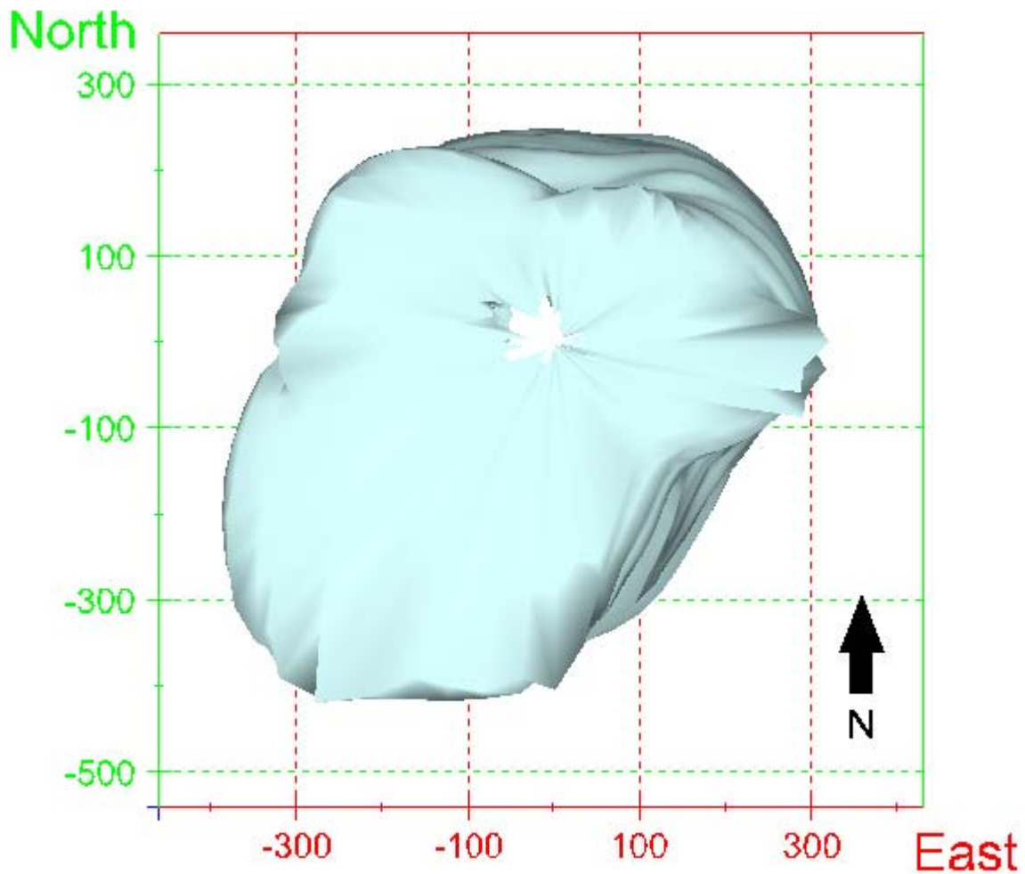
Figure 93. Map view sonar image of cavern BM-4, showing the basic geometry of the cavern. Grid squares represent 200 ft. The open “center” of the image is an artifact of the particular sonar survey used.
