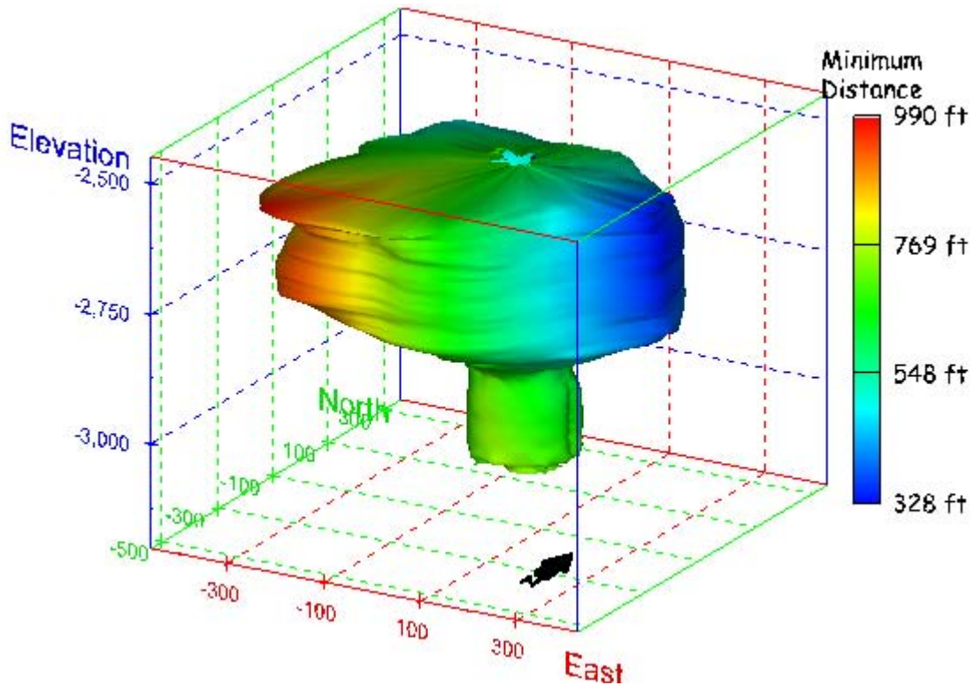
Figure 114. Sonar images of cavern BM-4, showing the geometry of the cavern colored by the minimum distance to the nearest neighboring cavern. View from (a) azimuth 210°, elevation 20°; (b) azimuth 150°, elevation 20°.
