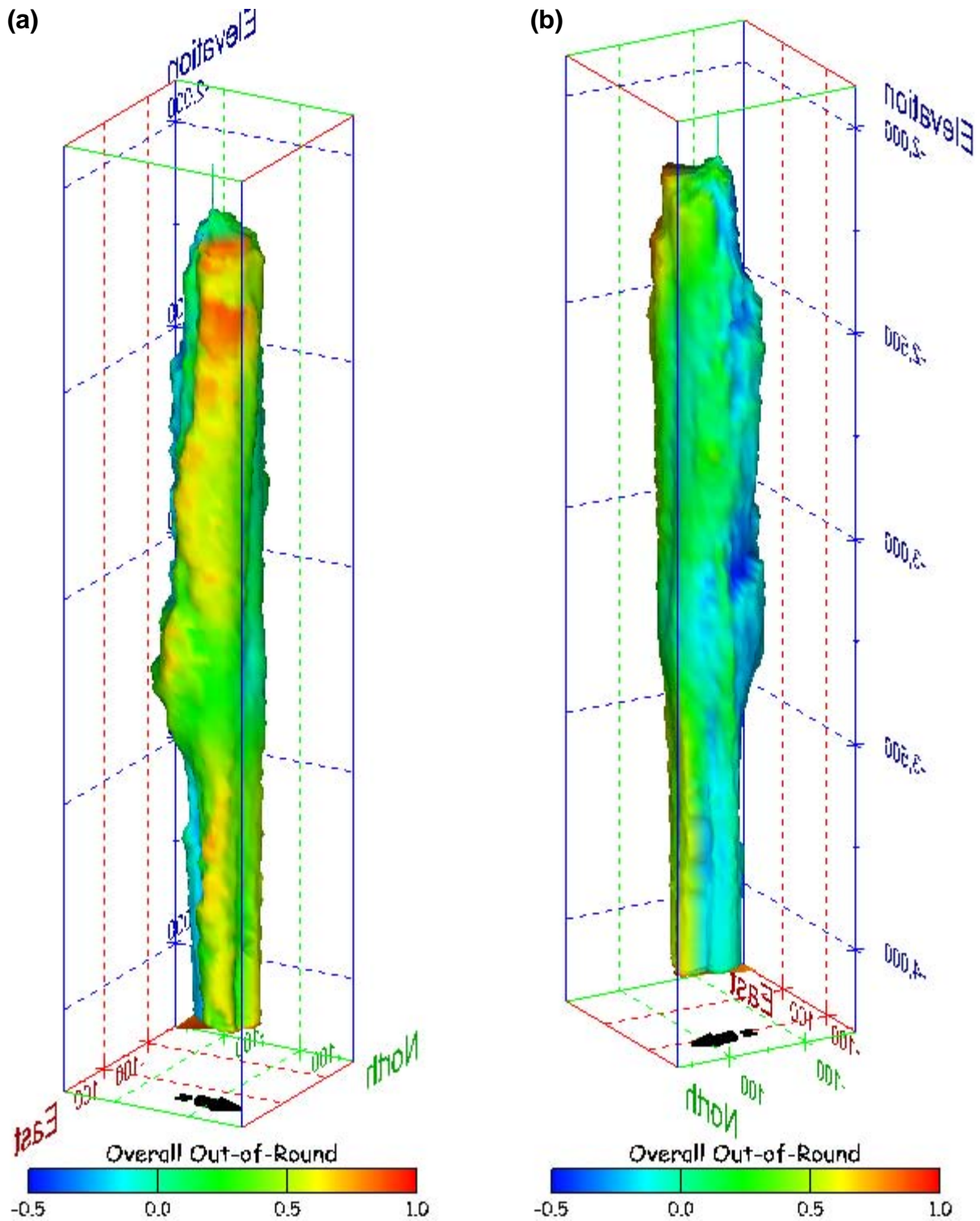
Figure 399. Sonar images of cavern BM-110, showing the geometry of the cavern colored by overall out-of-round ratio. View from (a) azimuth 60°, elevation 20°; (b) azimuth 300°, elevation 20°.
