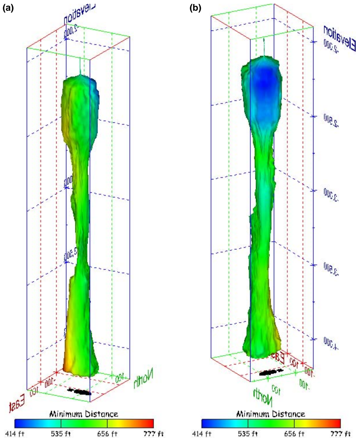
Figure 479. Sonar images of cavern BM-113, showing the geometry of the cavern colored by minimum distance to the nearest neighboring cavern. View from (a) azimuth 60°, elevation 20°; (b) azimuth 300°, elevation 20°.
