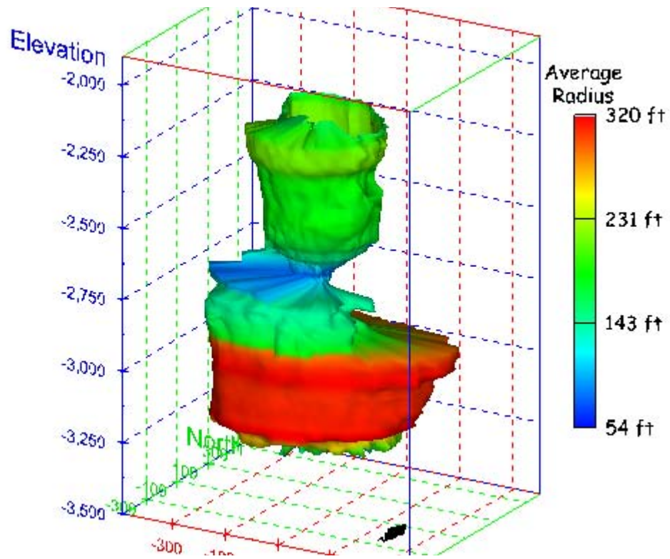
Figure 126. Sonar images of cavern BM-5, showing the geometry of the cavern colored by average radius. View from (a) azimuth 210°, elevation 20°; (b) azimuth 150°, elevation 20°.
