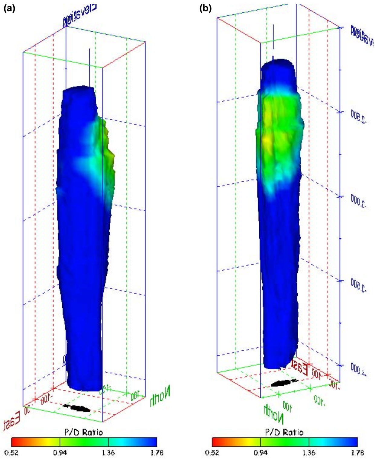
Figure 325. Sonar images of cavern BM-107, showing the geometry of the cavern colored by three-dimensional pillar-to-diameter ratio. View from (a) azimuth 60°, elevation 20°; (b) azimuth 300°, elevation 20°.
