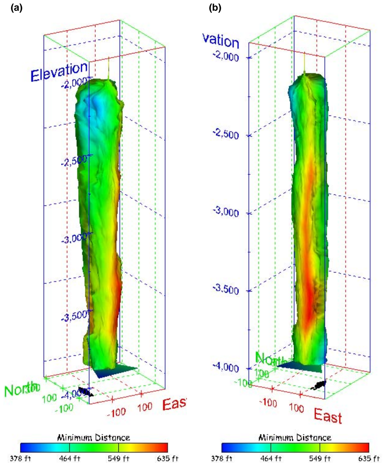
Figure 452. Sonar images of cavern BM-112, showing the geometry of the cavern colored by the minimum distance to the nearest neighboring cavern. View from (a) azimuth 210°, elevation 20°; (b) azimuth 150°, elevation 20°.
