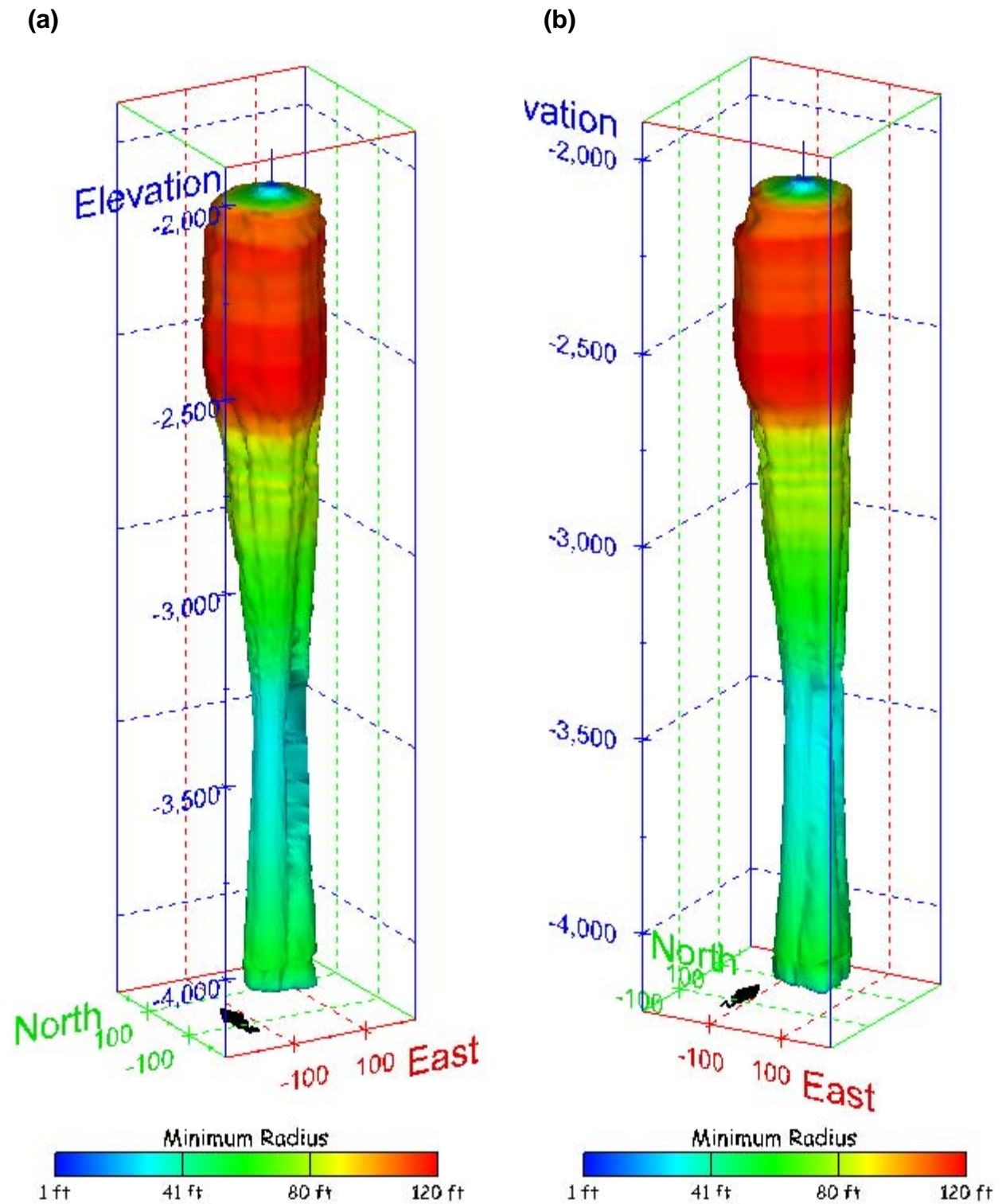
Figure 232. Sonar images of cavern BM-104, showing the geometry of the cavern colored by minimum radius. View from (a) azimuth 210°, elevation 20°; (b) azimuth 150°, elevation 20°.
