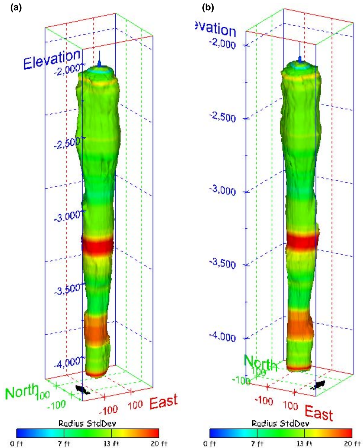
Figure 548. Sonar images of cavern BM-116, showing the geometry of the cavern colored by radius standard deviation. View from (a) azimuth 210°, elevation 20°; (b) azimuth 150°, elevation 20°.
