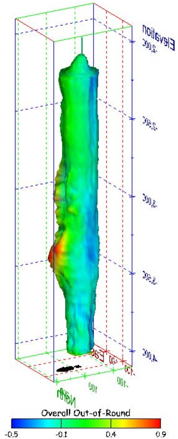
Figure 217. Sonar images of cavern BM-103, showing the geometry of the cavern colored by overall out-of-round ratio. View from (a) azimuth 60°, elevation 20°; (b) azimuth 300°, elevation 20°.
