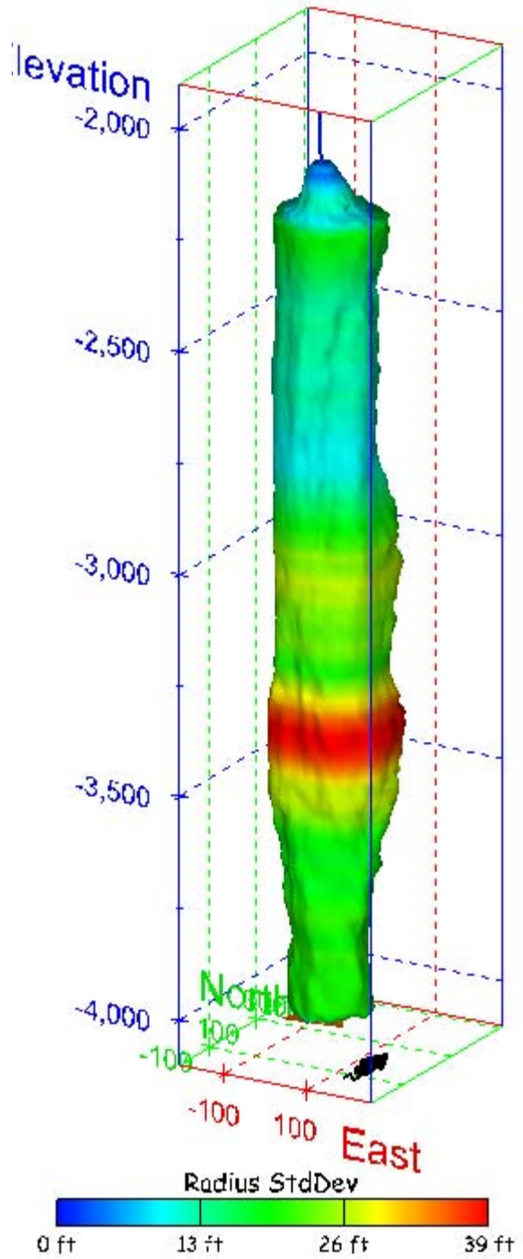
Figure 210. Sonar images of cavern BM-103, showing the geometry of the cavern colored by radius standard deviation. View from (a) azimuth 210°, elevation 20°; (b) azimuth 150°, elevation 20°.
