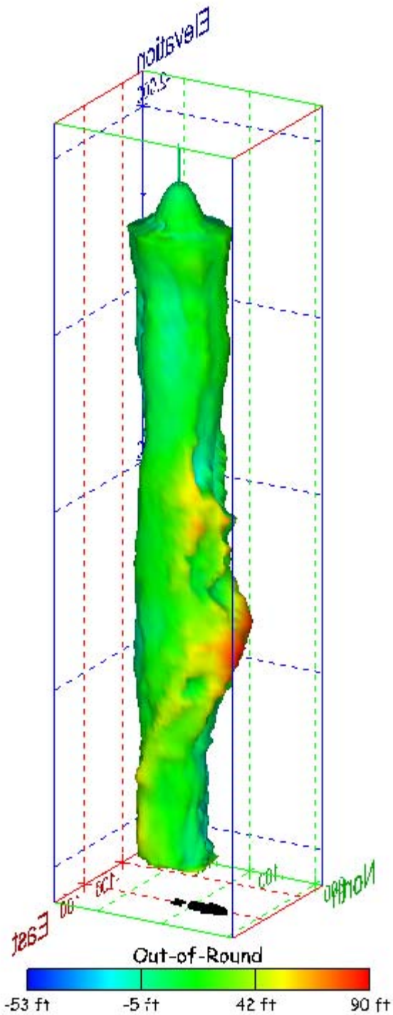
Figure 213. Sonar images of cavern BM-103, showing the geometry of the cavern colored by out-of-round distance. View from (a) azimuth 60°, elevation 20°; (b) azimuth 300°, elevation 20°.
