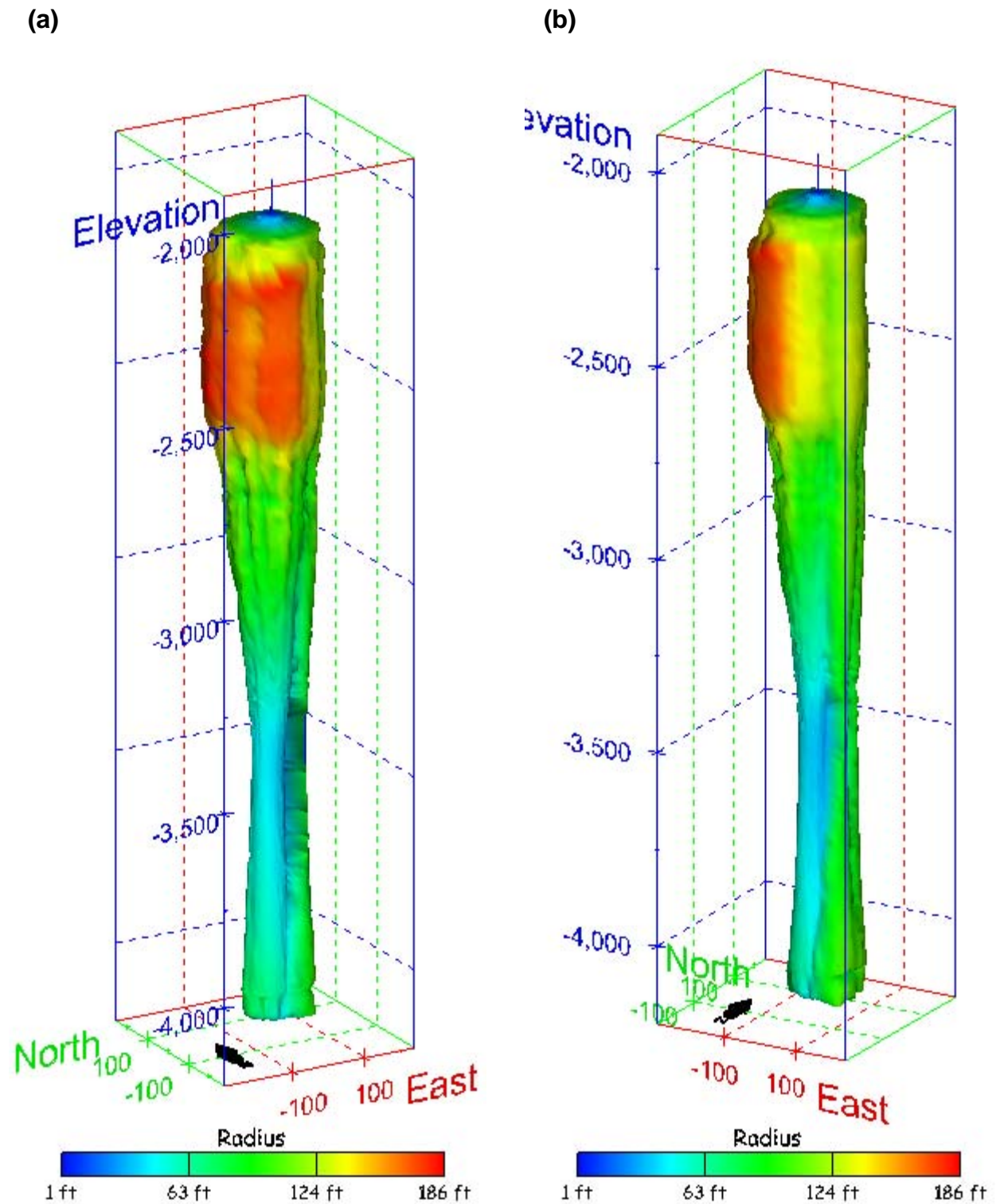
Figure 226. Sonar images of cavern BM-104, showing the geometry of the cavern colored by measured radius. View from (a) azimuth 210°, elevation 20°; (b) azimuth 150°, elevation 20°.
