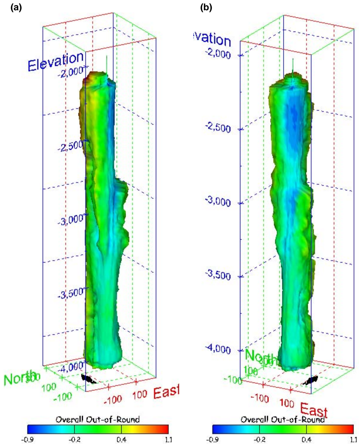
Figure 346. Sonar images of cavern BM-108, showing the geometry of the cavern colored by overall out-of-round ratio. View from (a) azimuth 210°, elevation 20°; (b) azimuth 150°, elevation 20°.
