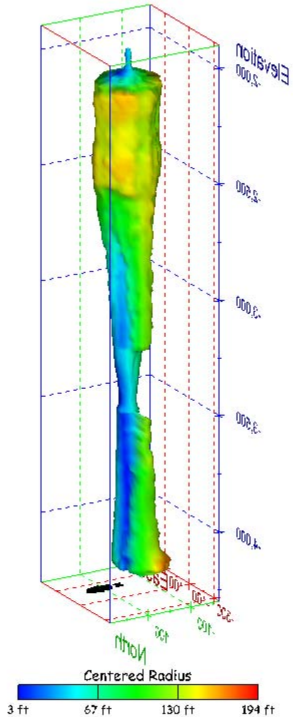
Figure 255. Sonar images of cavern BM-105, showing the geometry of the cavern colored by centered radius. View from (a) azimuth 60°, elevation 20°; (b) azimuth 300°, elevation 20°.
