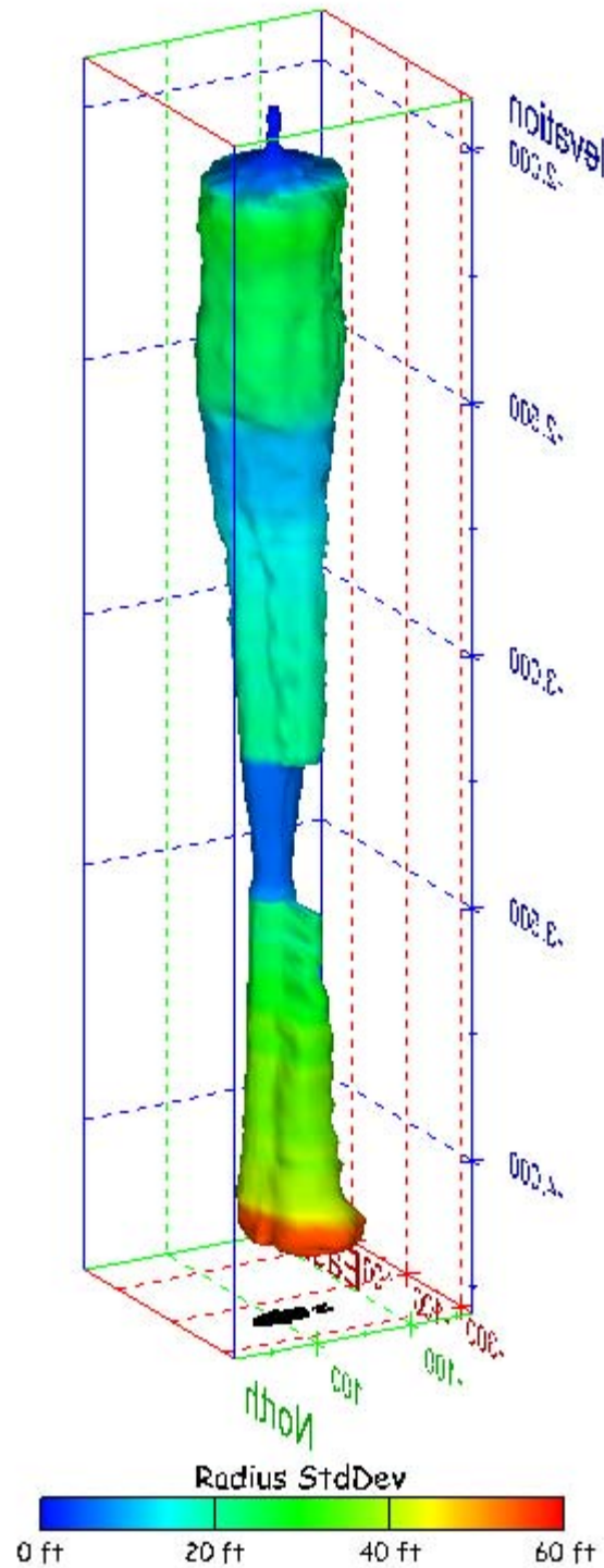
Figure 263. Sonar images of cavern BM-105, showing the geometry of the cavern colored by radius standard deviation. View from (a) azimuth 60°, elevation 20°; (b) azimuth 300°, elevation 20°.
