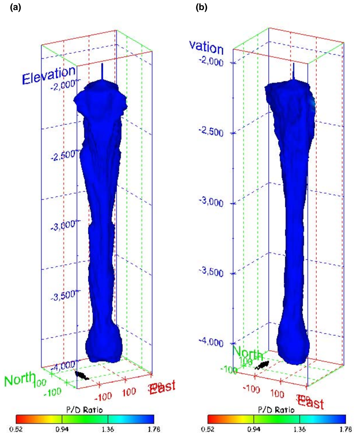
Figure 506. Sonar images of cavern BM-114, showing the geometry of the cavern colored by three-dimensional pillar-to-diameter ratio. View from (a) azimuth 210°, elevation 20°; (b) azimuth 150°, elevation 20°.
