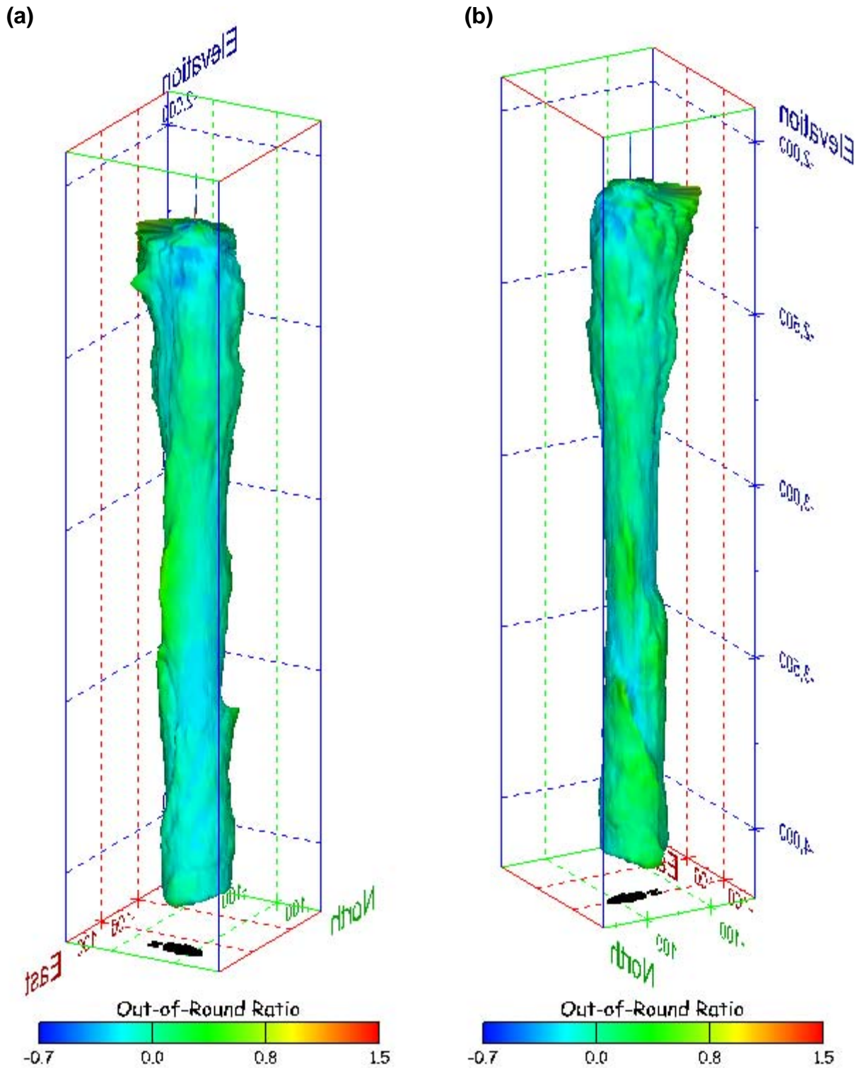
Figure 527. Sonar images of cavern BM-115, showing the geometry of the cavern colored by out-of-round ratio. View from (a) azimuth 60°, elevation 20°; (b) azimuth 300°, elevation 20°.
