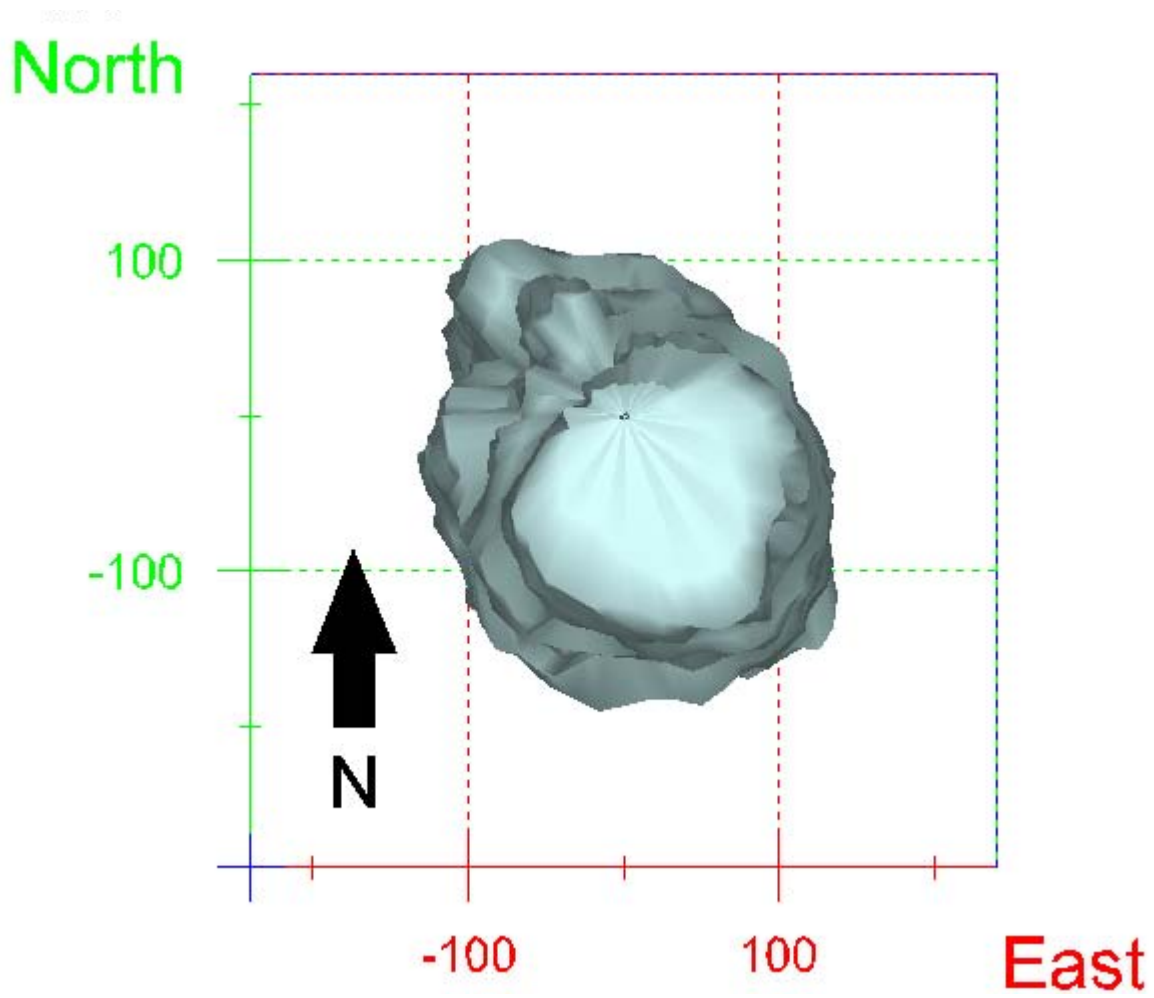
Figure 301. Map view sonar image of cavern BM-107, showing the basic geometry of the cavern. Grid squares represent 200 ft.
