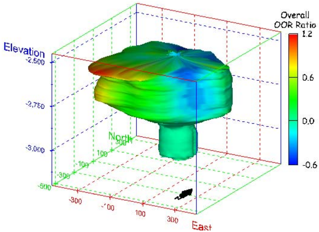
Figure 112. Sonar images of cavern BM-4, showing the geometry of the cavern colored by overall out-of-round ratio. View from (a) azimuth 210°, elevation 20°; (b) azimuth 150°, elevation 20°.
