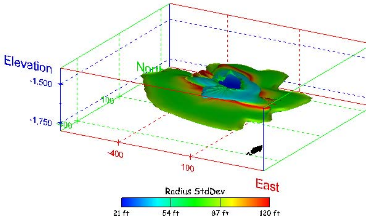
Figure 80. Sonar images of cavern BM-3, showing the geometry of the cavern colored by radius standard deviation. View from (a) azimuth 210°, elevation 20°; (b) azimuth 150°, elevation 20°.
