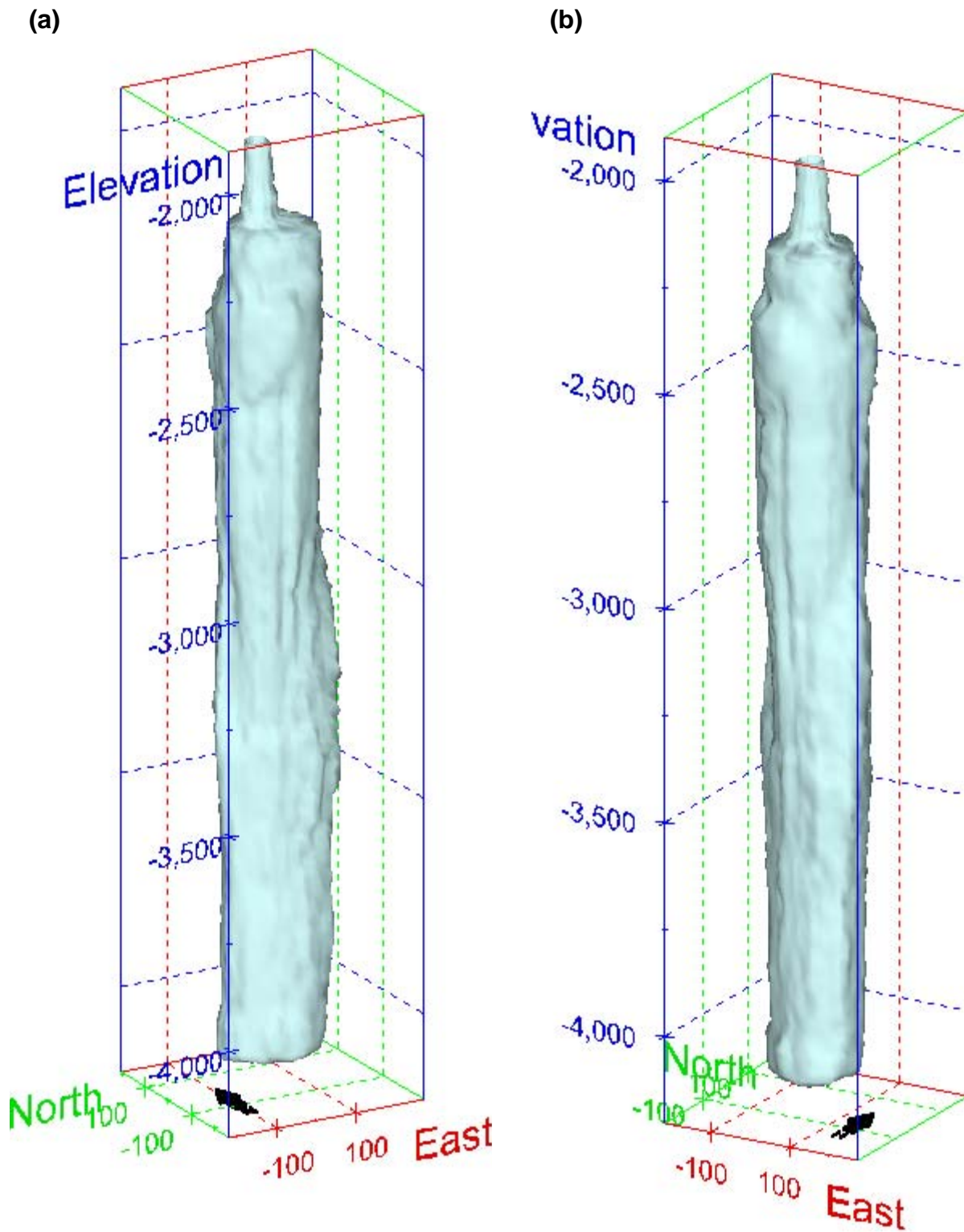
Figure 146. Sonar images of cavern BM-101, showing the basic geometric shape of the cavern. View from (a) azimuth 210°, elevation 20°; (b) azimuth 150°, elevation 20°.
