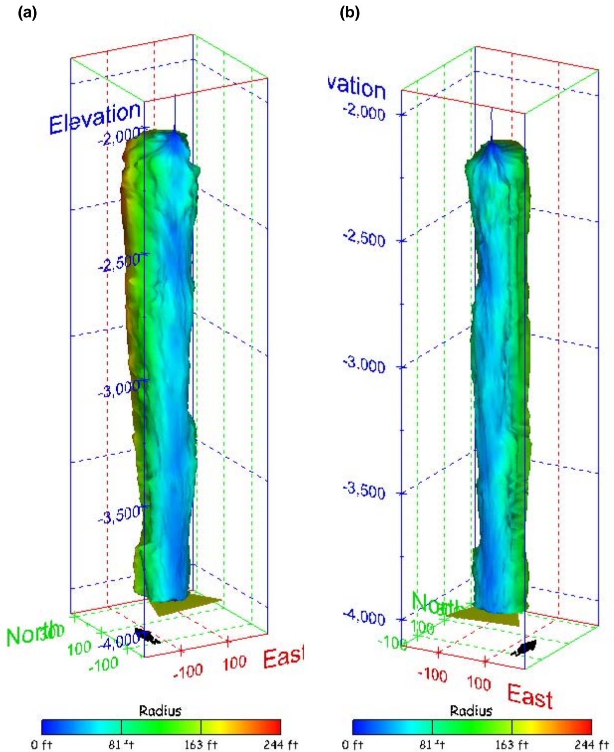
Figure 434. Sonar images of cavern BM-112, showing the geometry of the cavern colored by measured radius. View from (a) azimuth 210°, elevation 20°; (b) azimuth 150°, elevation 20°.
