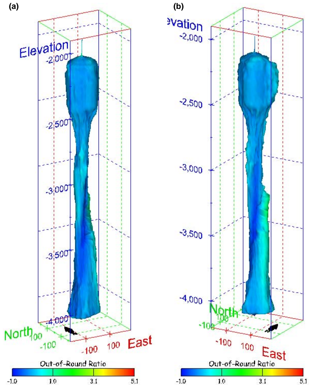
Figure 474. Sonar images of cavern BM-113, showing the geometry of the cavern colored by out-of-round ratio. View from (a) azimuth 210°, elevation 20°; (b) azimuth 150°, elevation 20°.
