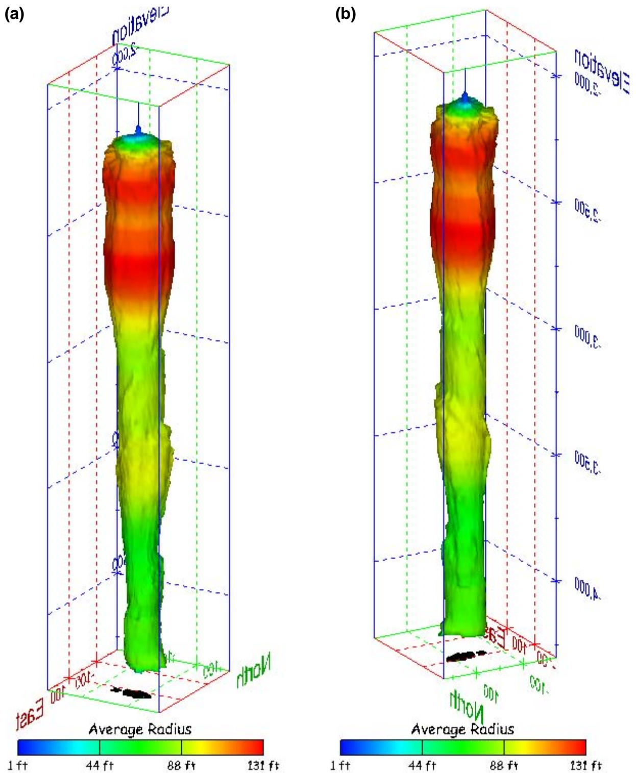
Figure 543. Sonar images of cavern BM-116, showing the geometry of the cavern colored by average radius. View from (a) azimuth 60°, elevation 20°; (b) azimuth 300°, elevation 20°.
