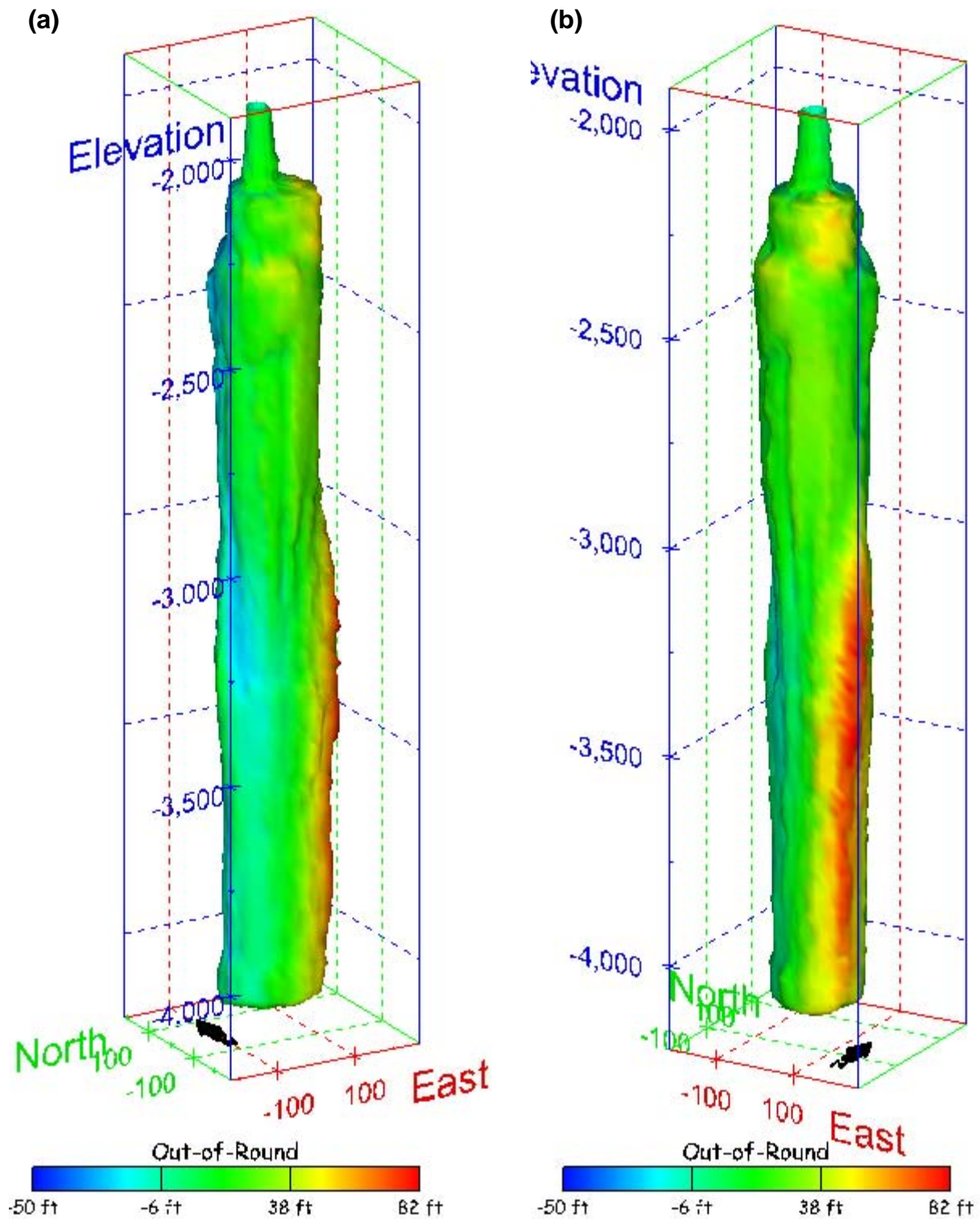
Figure 160. Sonar images of cavern BM-101, showing the geometry of the cavern colored by out-of-round distance. View from (a) azimuth 210°, elevation 20°; (b) azimuth 150°, elevation 20°.
