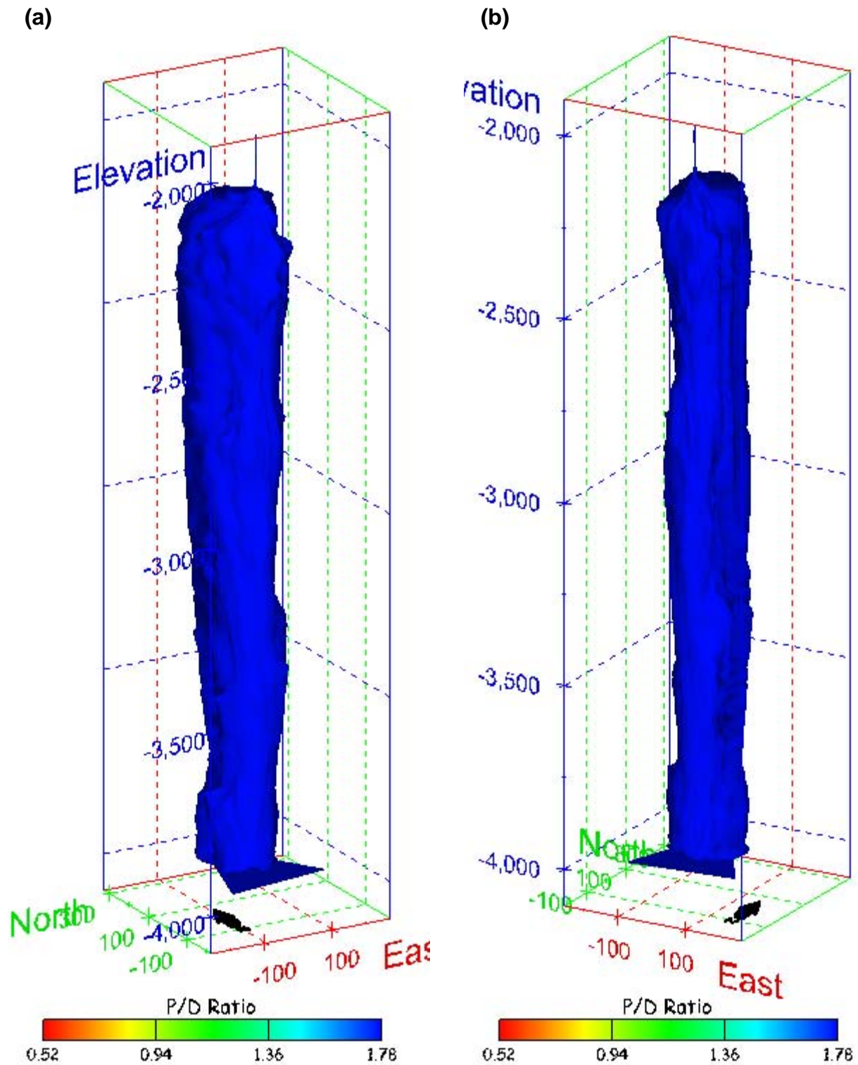
Figure 454. Sonar images of cavern BM-112, showing the geometry of the cavern colored by three-dimensional pillar-to-diameter ratio. View from (a) azimuth 210°, elevation 20°; (b) azimuth 150°, elevation 20°.
