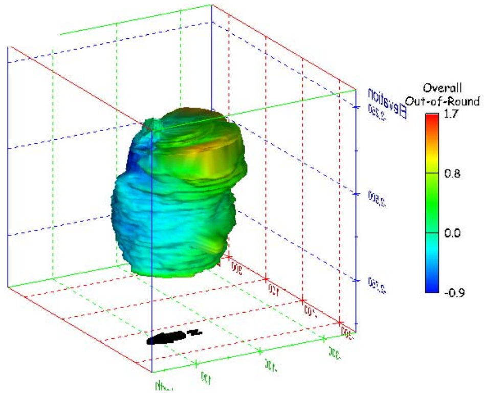
Figure 35. Sonar images of cavern BM-1, showing the geometry of the cavern colored by overall out-of-round ratio. View from (a) azimuth 60°, elevation 20°; (b) azimuth 300°, elevation 20°.
