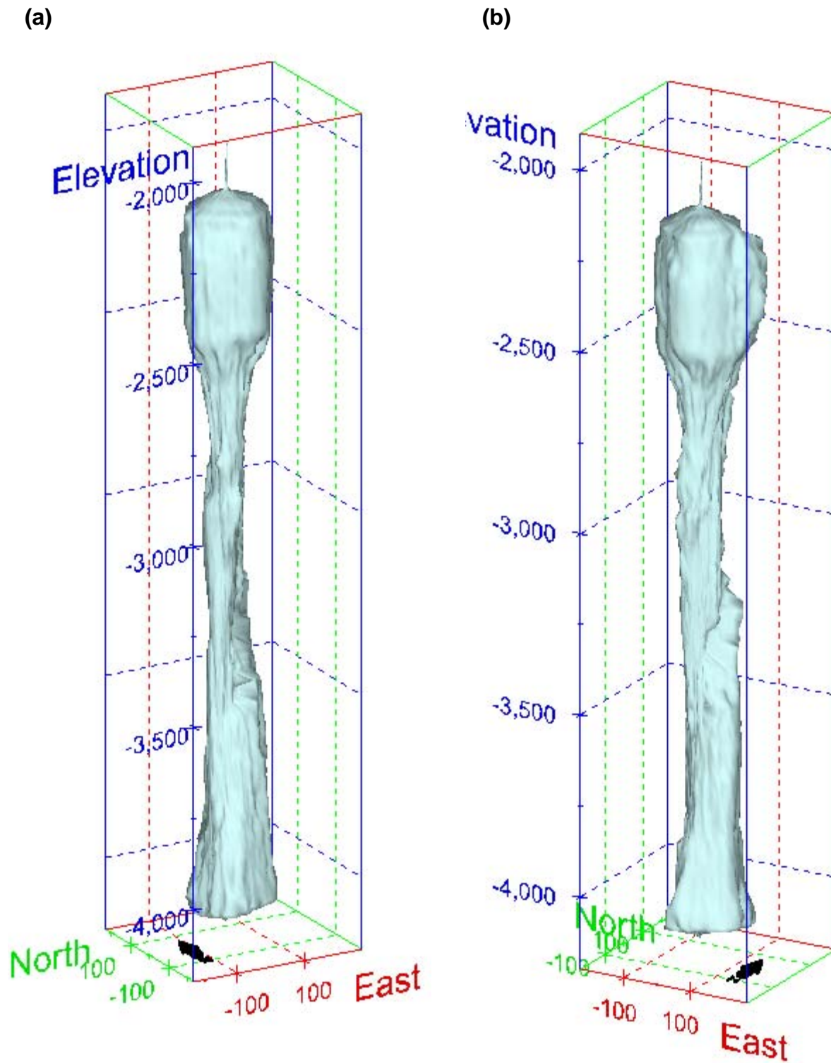
Figure 458. Sonar images of cavern BM-113, showing the basic geometric shape of the cavern. View from (a) azimuth 210°, elevation 20°; (b) azimuth 150°, elevation 20°.
