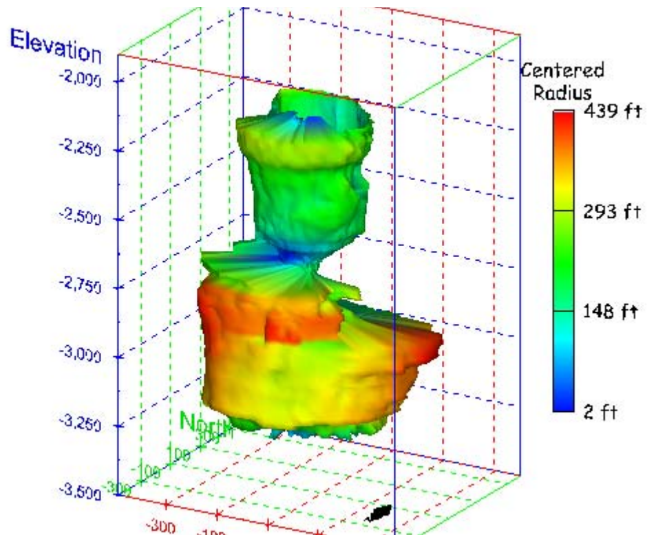
Figure 124. Sonar images of cavern BM-5, showing the geometry of the cavern colored by centered radius. View from (a) azimuth 210°, elevation 20°; (b) azimuth 150°, elevation 20°.
