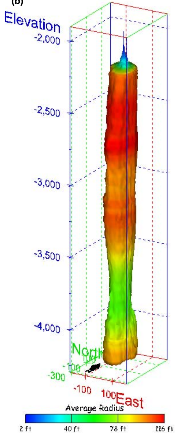
Figure 178. Sonar images of cavern BM-102, showing the geometry of the cavern colored by average radius. View from (a) azimuth 210°, elevation 20°; (b) azimuth 150°, elevation 20°.
