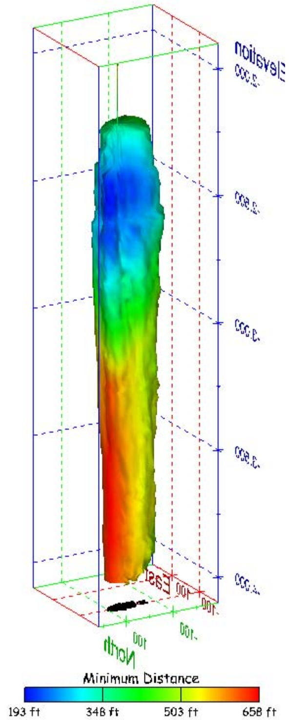
Figure 323. Sonar images of cavern BM-107, showing the geometry of the cavern colored by minimum distance to the nearest neighboring cavern. View from (a) azimuth 60°, elevation 20°; (b) azimuth 300°, elevation 20°.
