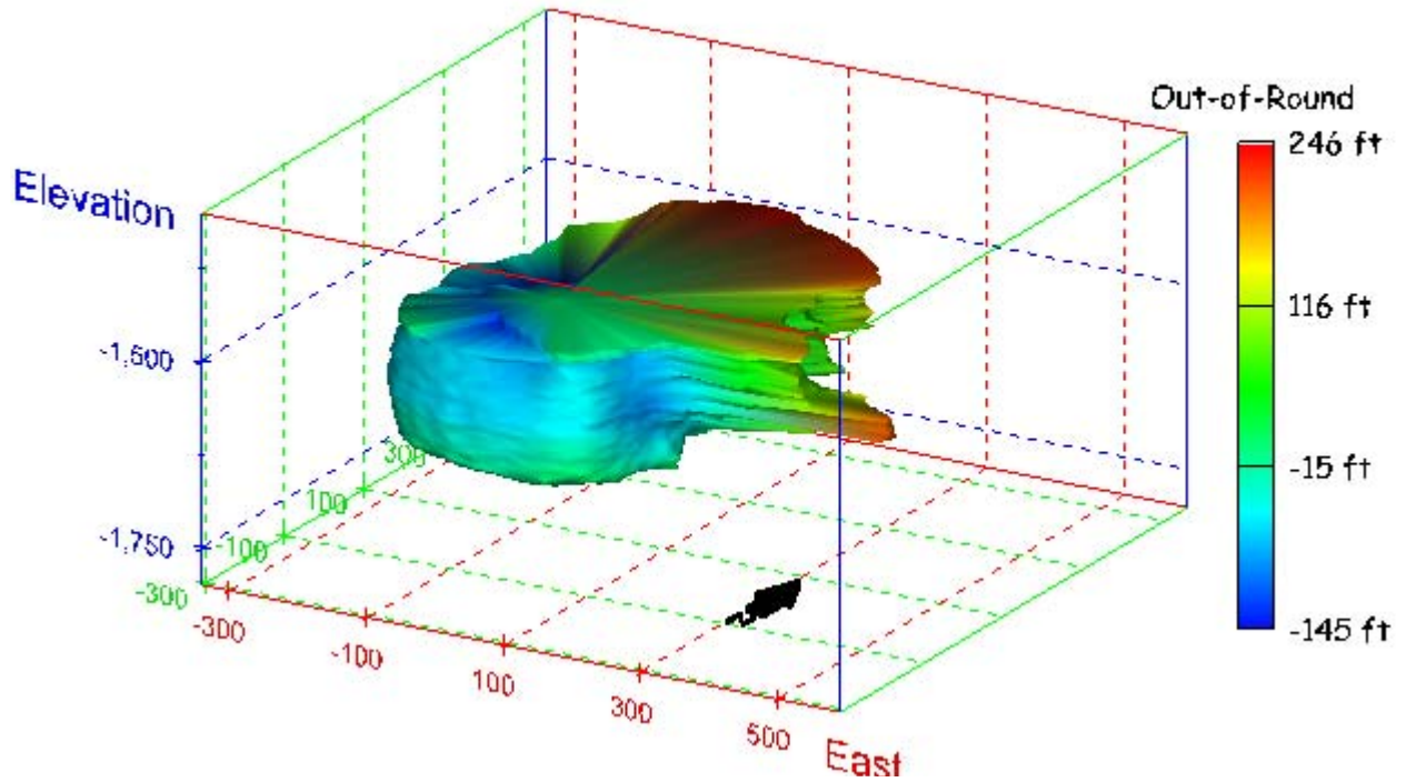
Figure 56. Sonar images of cavern BM-2, showing the geometry of the cavern colored by out-of-round distance. View from (a) azimuth 210°, elevation 20°; (b) azimuth 150°, elevation 20°.
