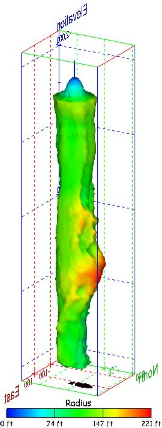
Figure 201. Sonar images of cavern BM-103, showing the geometry of the cavern colored by measured radius. View from (a) azimuth 60°, elevation 20°; (b) azimuth 300°, elevation 20°.
