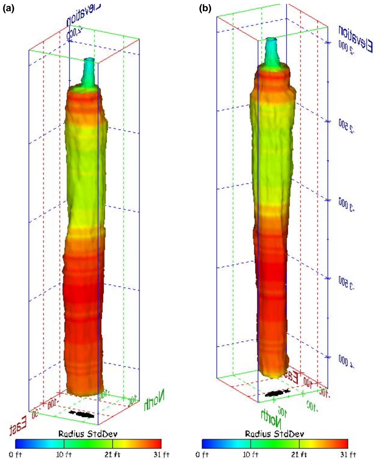
Figure 159. Sonar images of cavern BM-101, showing the geometry of the cavern colored by radius standard deviation. View from (a) azimuth 60°, elevation 20°; (b) azimuth 300°, elevation 20°.
