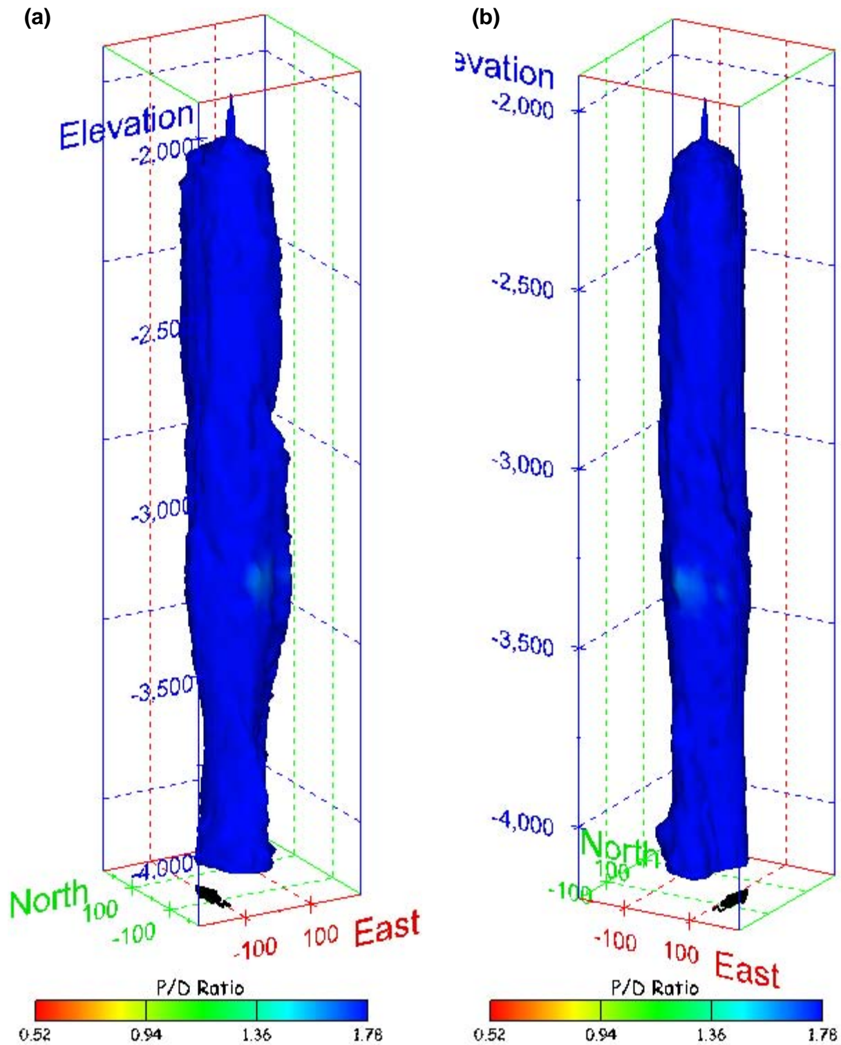
Figure 428. Sonar images of cavern BM-111, showing the geometry of the cavern colored by three-dimensional pillar-to-diameter ratio. View from (a) azimuth 210°, elevation 20°; (b) azimuth 150°, elevation 20°.
