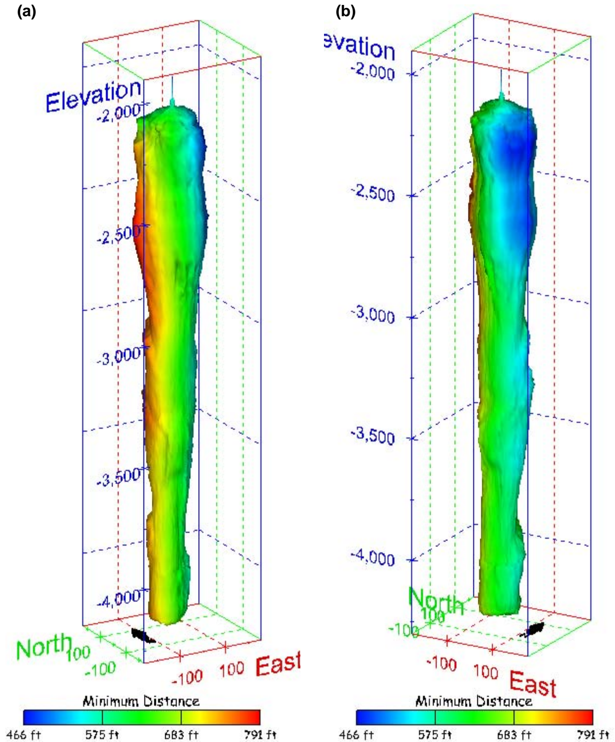
Figure 556. Sonar images of cavern BM-116, showing the geometry of the cavern colored by the minimum distance to the nearest neighboring cavern. View from (a) azimuth 210°, elevation 20°; (b) azimuth 150°, elevation 20°.
