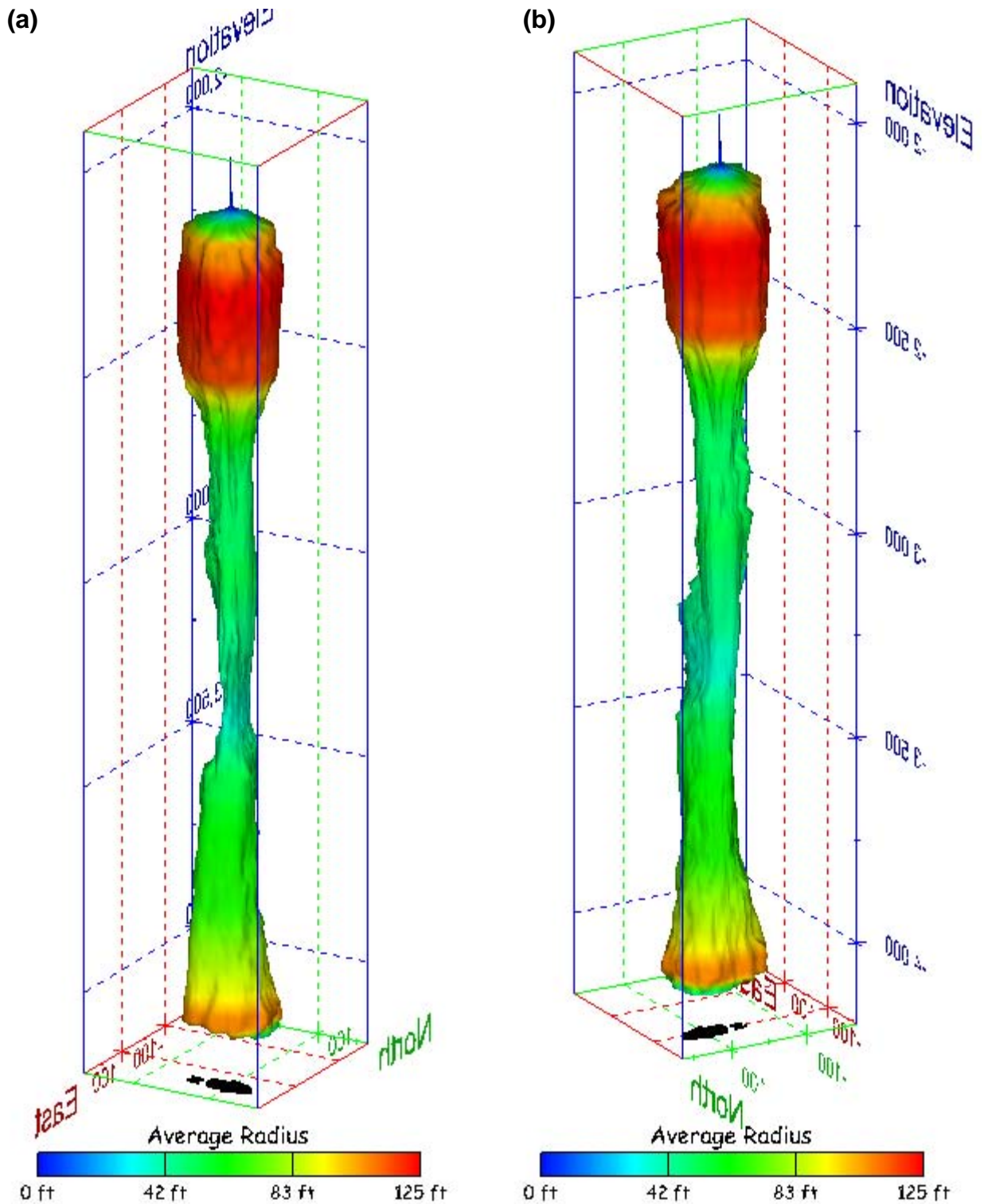
Figure 465. Sonar images of cavern BM-113, showing the geometry of the cavern colored by average radius. View from (a) azimuth 60°, elevation 20°; (b) azimuth 300°, elevation 20°.
