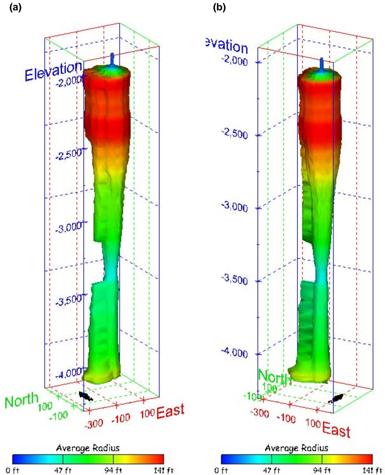
Figure 256. Sonar images of cavern BM-105, showing the geometry of the cavern colored by average radius. View from (a) azimuth 210°, elevation 20°; (b) azimuth 150°, elevation 20°.
