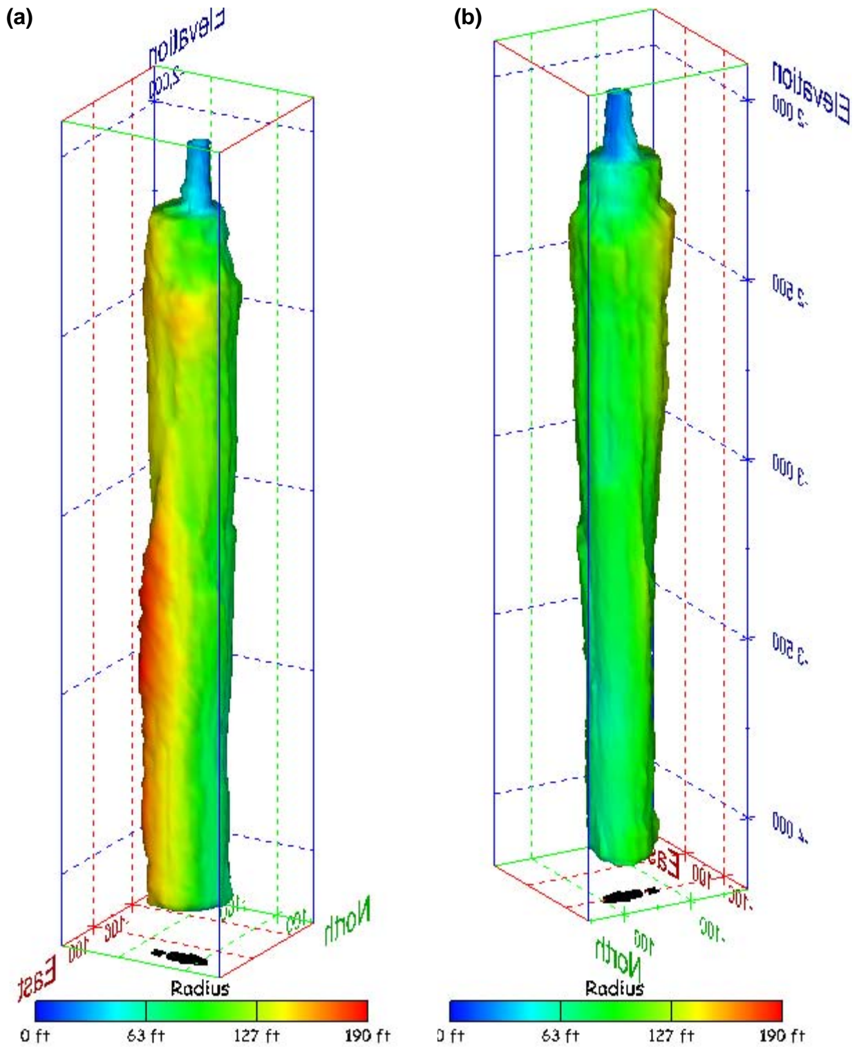
Figure 149. Sonar images of cavern BM-101, showing the geometry of the cavern colored by measured radius. View from (a) azimuth 60°, elevation 20°; (b) azimuth 300°, elevation 20°.
