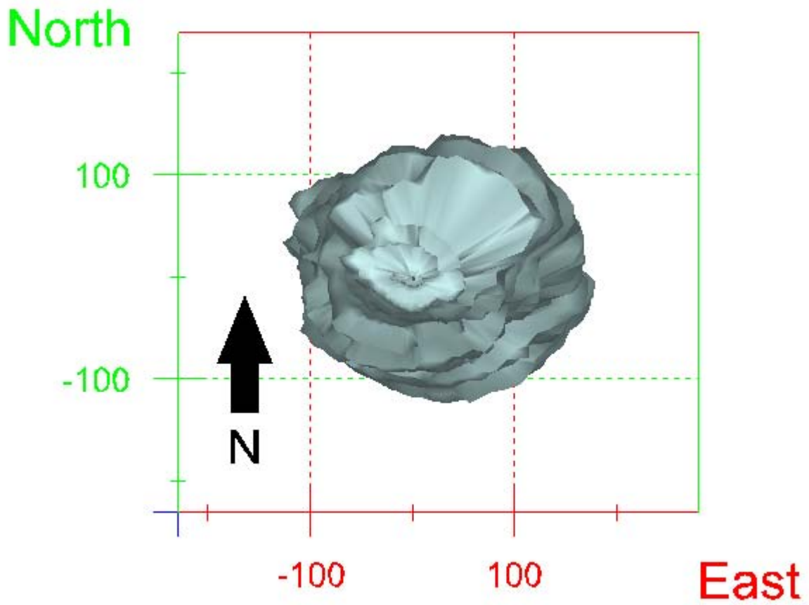
Figure 379. Map view sonar image of cavern BM-110, showing the basic geometry of the cavern. Grid squares represent 200 ft.
