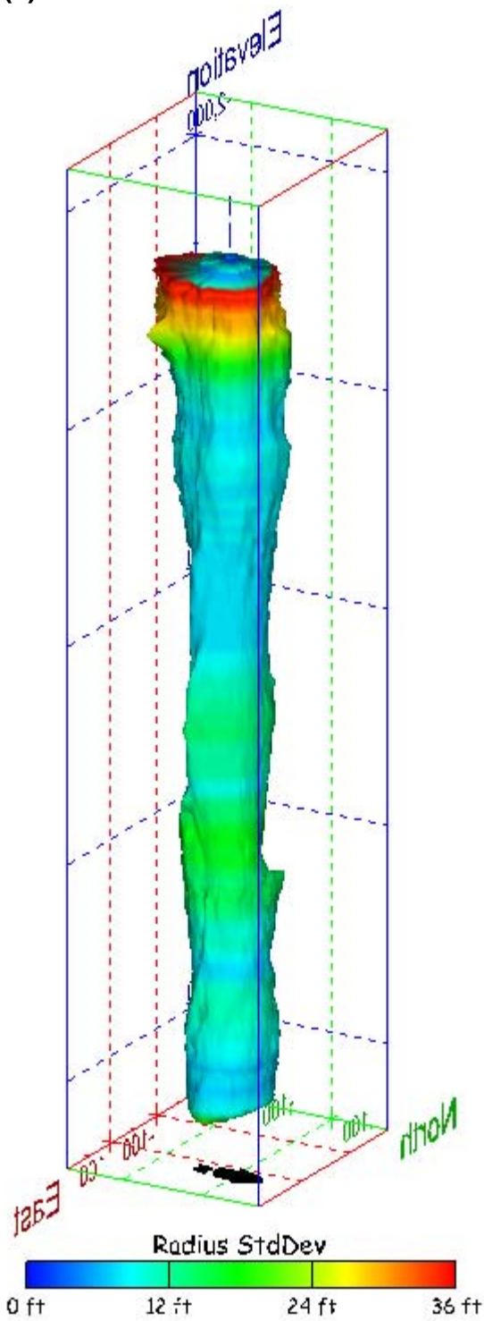
Figure 523. Sonar images of cavern BM-115, showing the geometry of the cavern colored by radius standard deviation. View from (a) azimuth 60°, elevation 20°; (b) azimuth 300°, elevation 20°.
