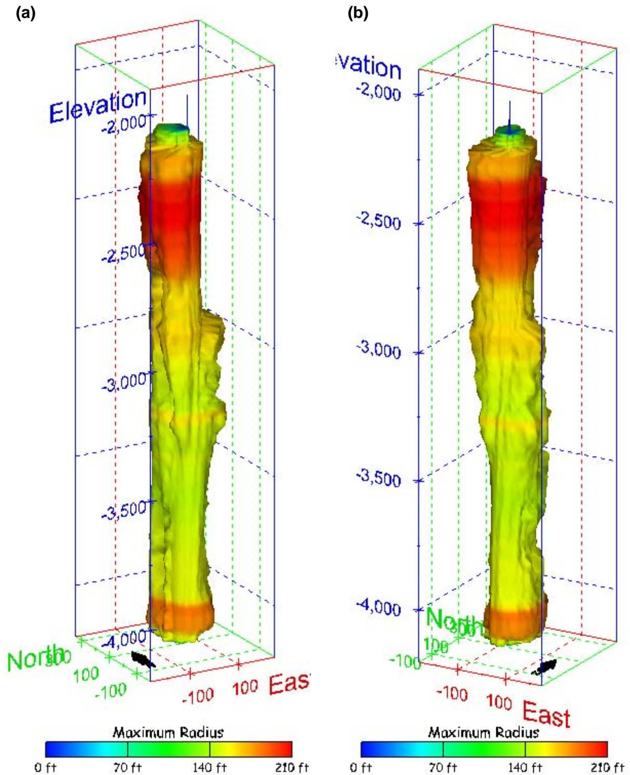
Figure 338. Sonar images of cavern BM-108, showing the geometry of the cavern colored by maximum radius. View from (a) azimuth 210°, elevation 20°; (b) azimuth 150°, elevation 20°.
