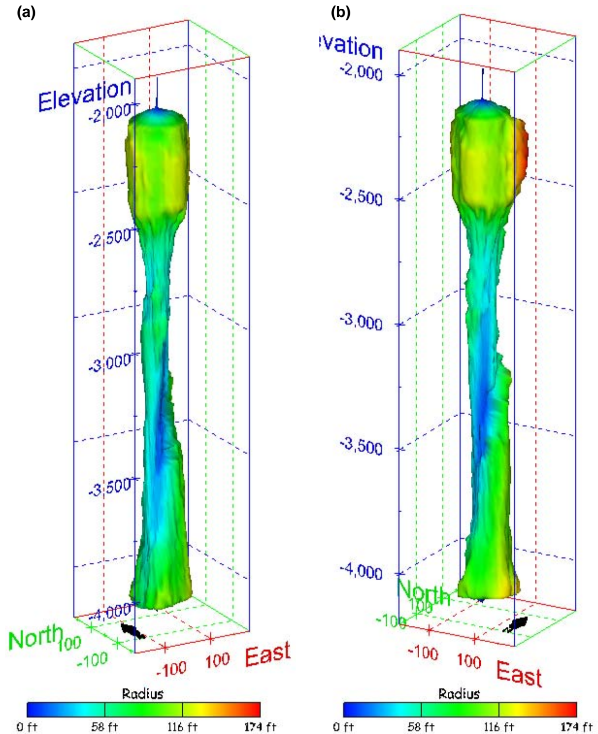
Figure 460. Sonar images of cavern BM-113, showing the geometry of the cavern colored by measured radius. View from (a) azimuth 210°, elevation 20°; (b) azimuth 150°, elevation 20°.
