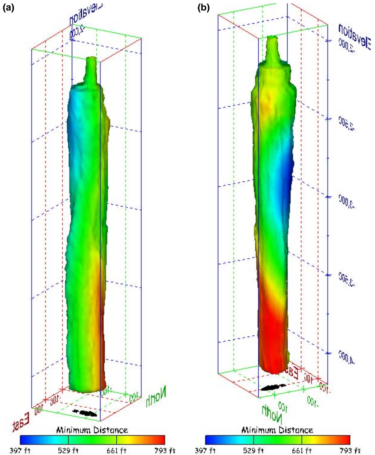
Figure 167. Sonar images of cavern BM-101, showing the geometry of the cavern colored by minimum distance to the nearest neighboring cavern. View from (a) azimuth 60°, elevation 20°; (b) azimuth 300°, elevation 20°.
