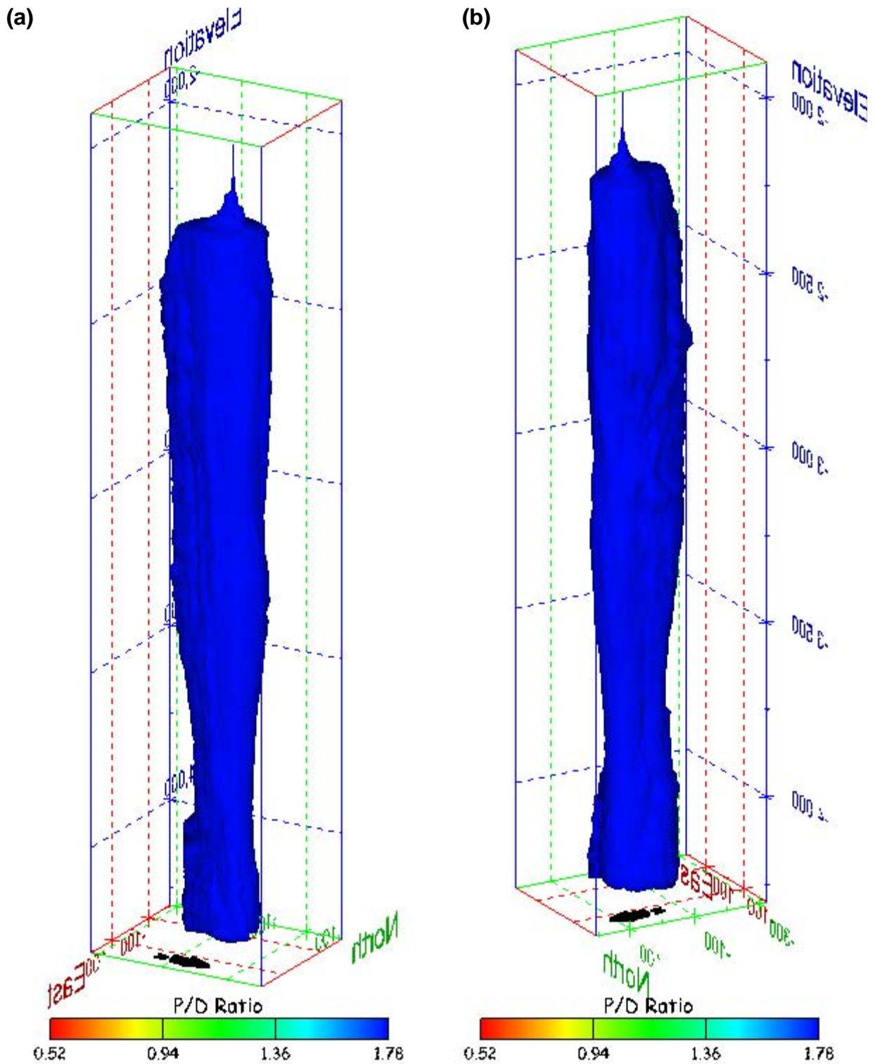
Figure 195. Sonar images of cavern BM-102, showing the geometry of the cavern colored by three-dimensional pillar-to-diameter ratio. View from (a) azimuth 60°, elevation 20°; (b) azimuth 300°, elevation 20°.
