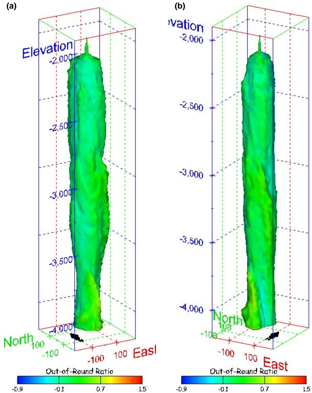
Figure 422. Sonar images of cavern BM-111, showing the geometry of the cavern colored by out-of-round ratio. View from (a) azimuth 210°, elevation 20°; (b) azimuth 150°, elevation 20°.
