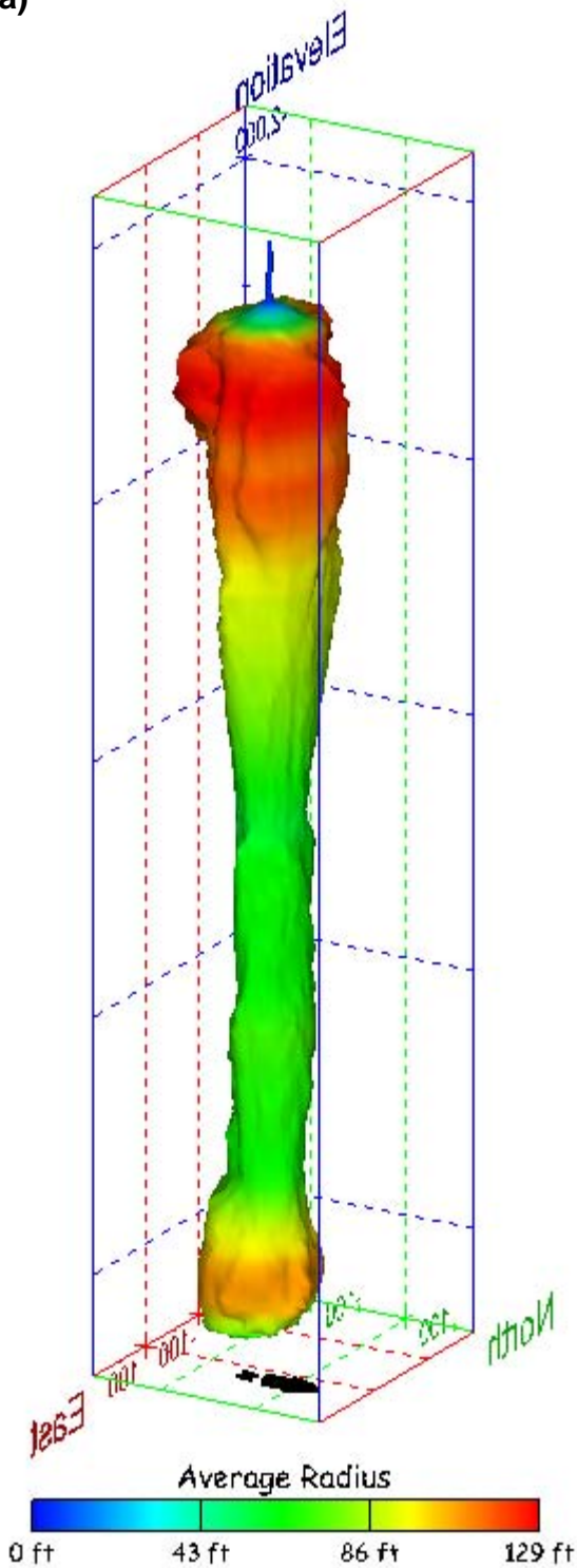
Figure 491. Sonar images of cavern BM-114, showing the geometry of the cavern colored by average radius. View from (a) azimuth 60°, elevation 20°; (b) azimuth 300°, elevation 20°.
