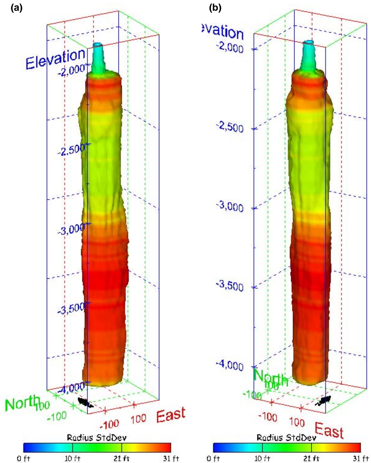
Figure 158. Sonar images of cavern BM-101, showing the geometry of the cavern colored by radius standard deviation. View from (a) azimuth 210°, elevation 20°; (b) azimuth 150°, elevation 20°.
