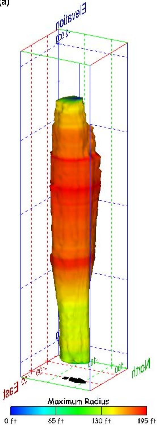
Figure 313. Sonar images of cavern BM-107, showing the geometry of the cavern colored by maximum radius. View from (a) azimuth 60°, elevation 20°; (b) azimuth 300°, elevation 20°.
