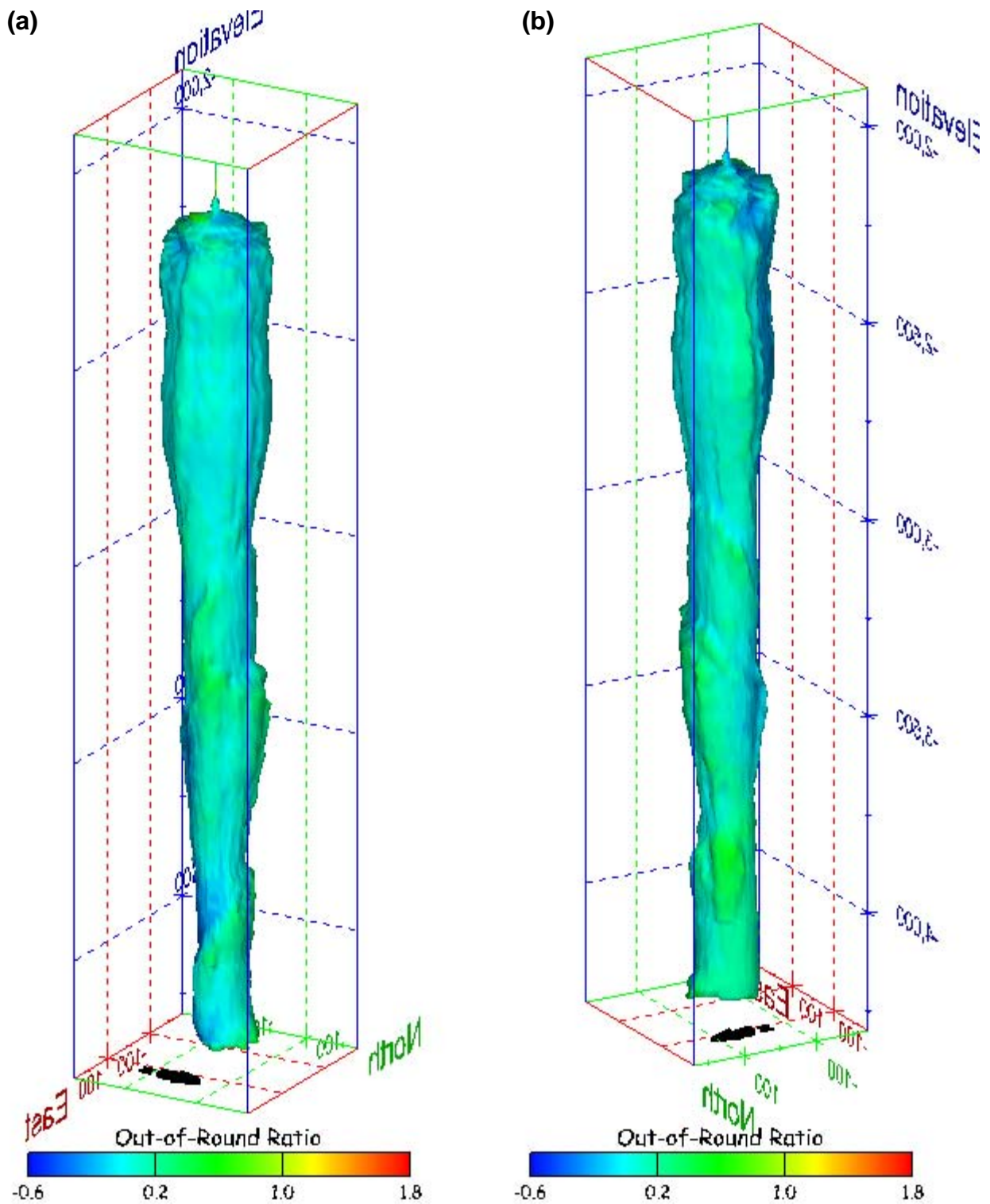
Figure 553. Sonar images of cavern BM-116, showing the geometry of the cavern colored by out-of-round ratio. View from (a) azimuth 60°, elevation 20°; (b) azimuth 300°, elevation 20°.
