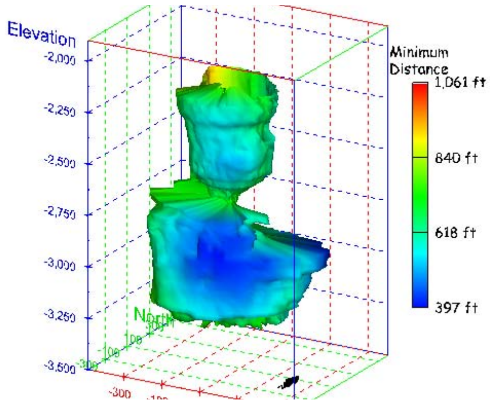
Figure 140. Sonar images of cavern BM-5, showing the geometry of the cavern colored by the minimum distance to the nearest neighboring cavern. View from (a) azimuth 210°, elevation 20°; (b) azimuth 150°, elevation 20°.
