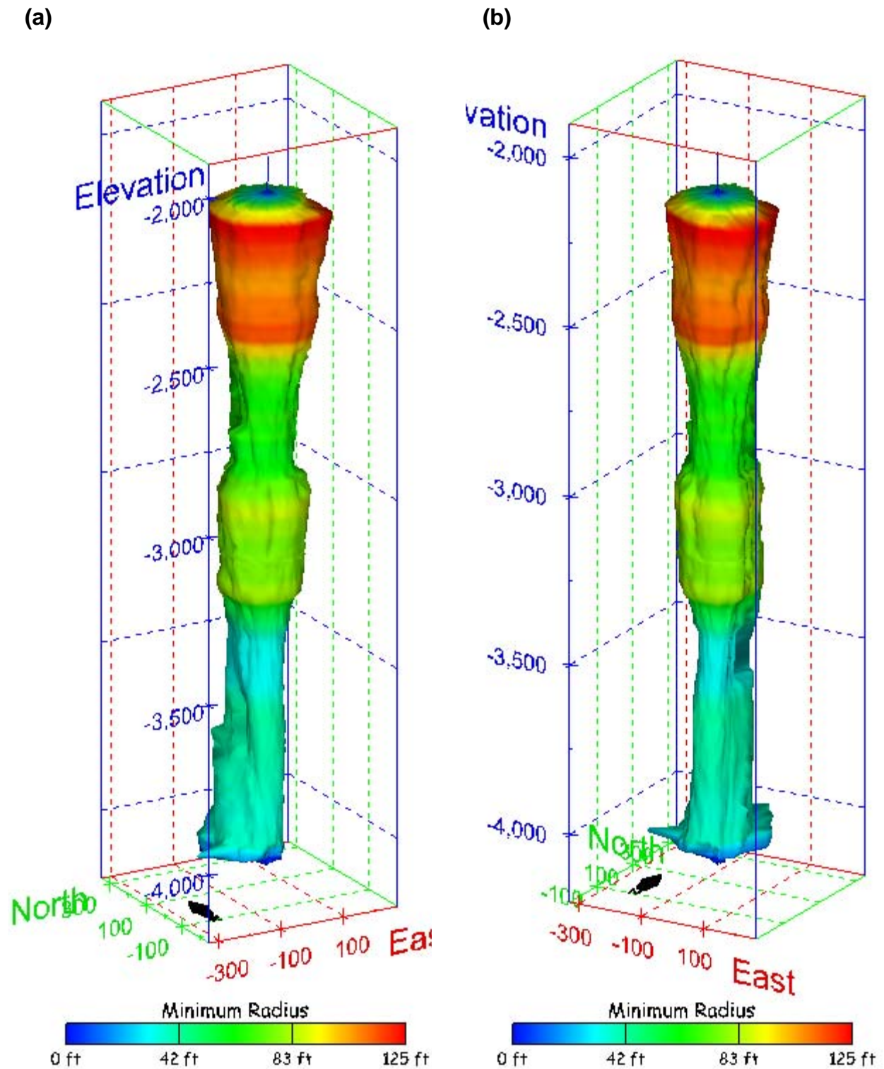
Figure 362. Sonar images of cavern BM-109, showing the geometry of the cavern colored by minimum radius. View from (a) azimuth 210°, elevation 20°; (b) azimuth 150°, elevation 20°.
