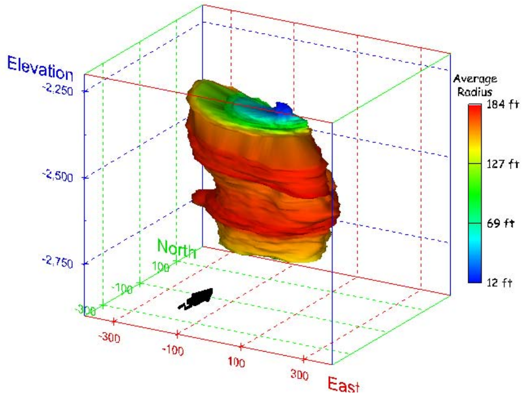
Figure 22. Sonar images of cavern BM-1, showing the geometry of the cavern colored by average radius. View from (a) azimuth 210°, elevation 20°; (b) azimuth 150°, elevation 20°.
