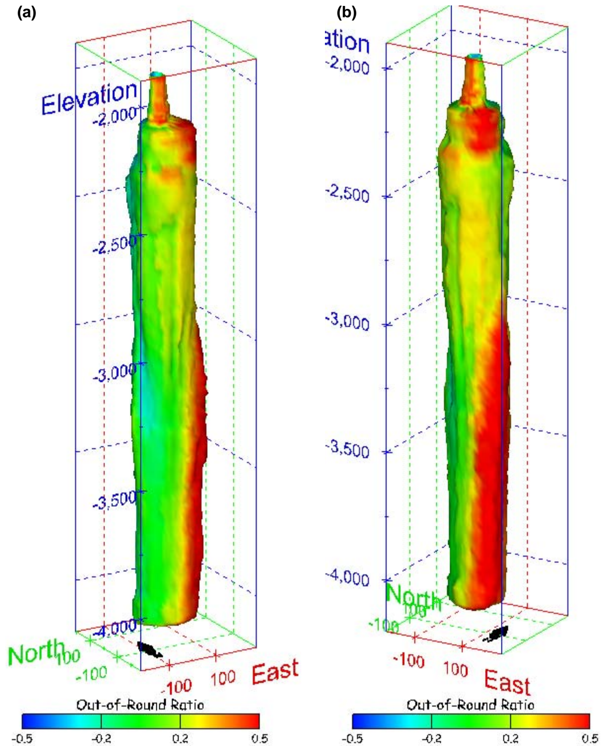
Figure 162. Sonar images of cavern BM-101, showing the geometry of the cavern colored by out-of-round ratio. View from (a) azimuth 210°, elevation 20°; (b) azimuth 150°, elevation 20°.
