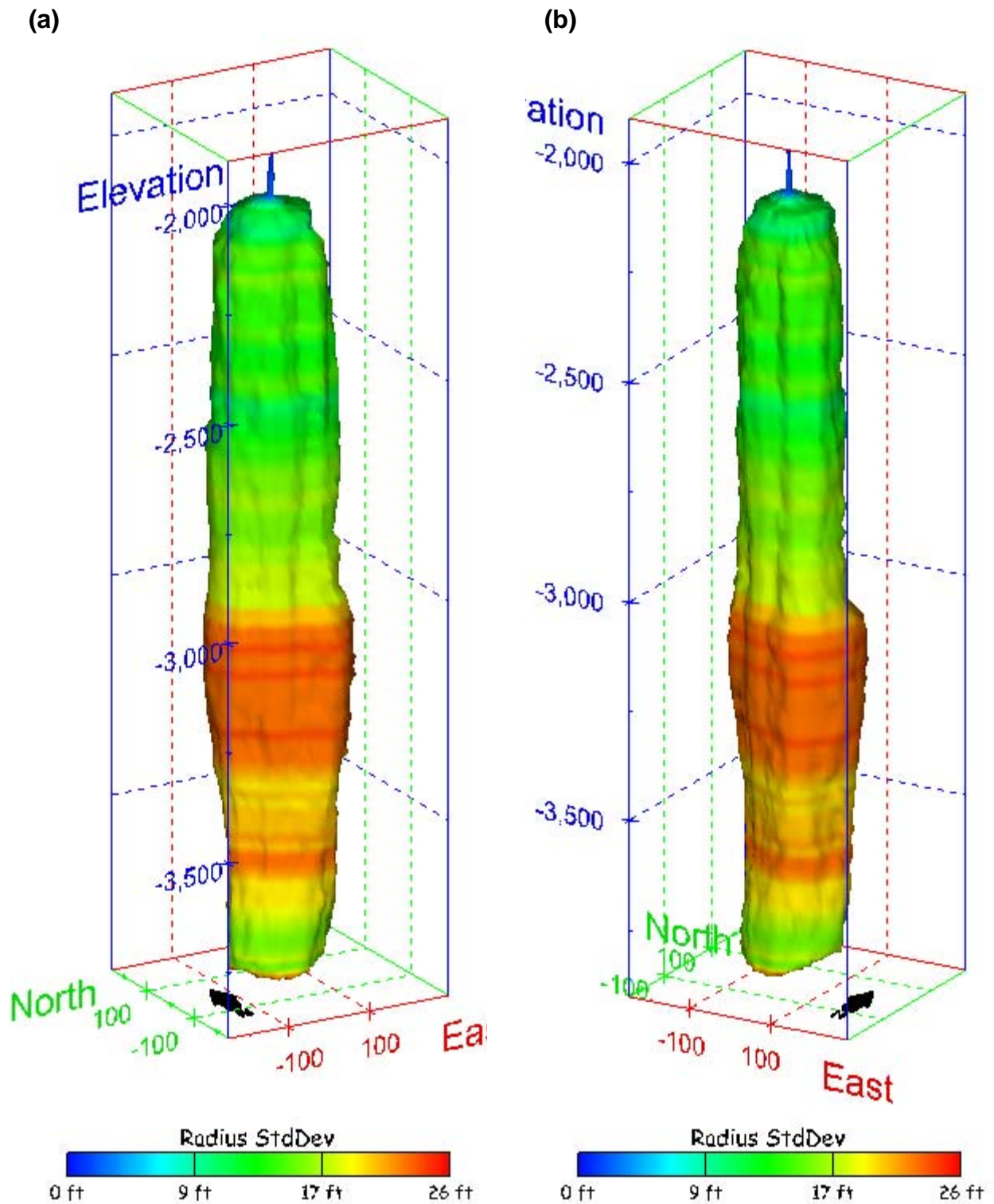
Figure 288. Sonar images of cavern BM-106, showing the geometry of the cavern colored by radius standard deviation. View from (a) azimuth 210°, elevation 20°; (b) azimuth 150°, elevation 20°.
