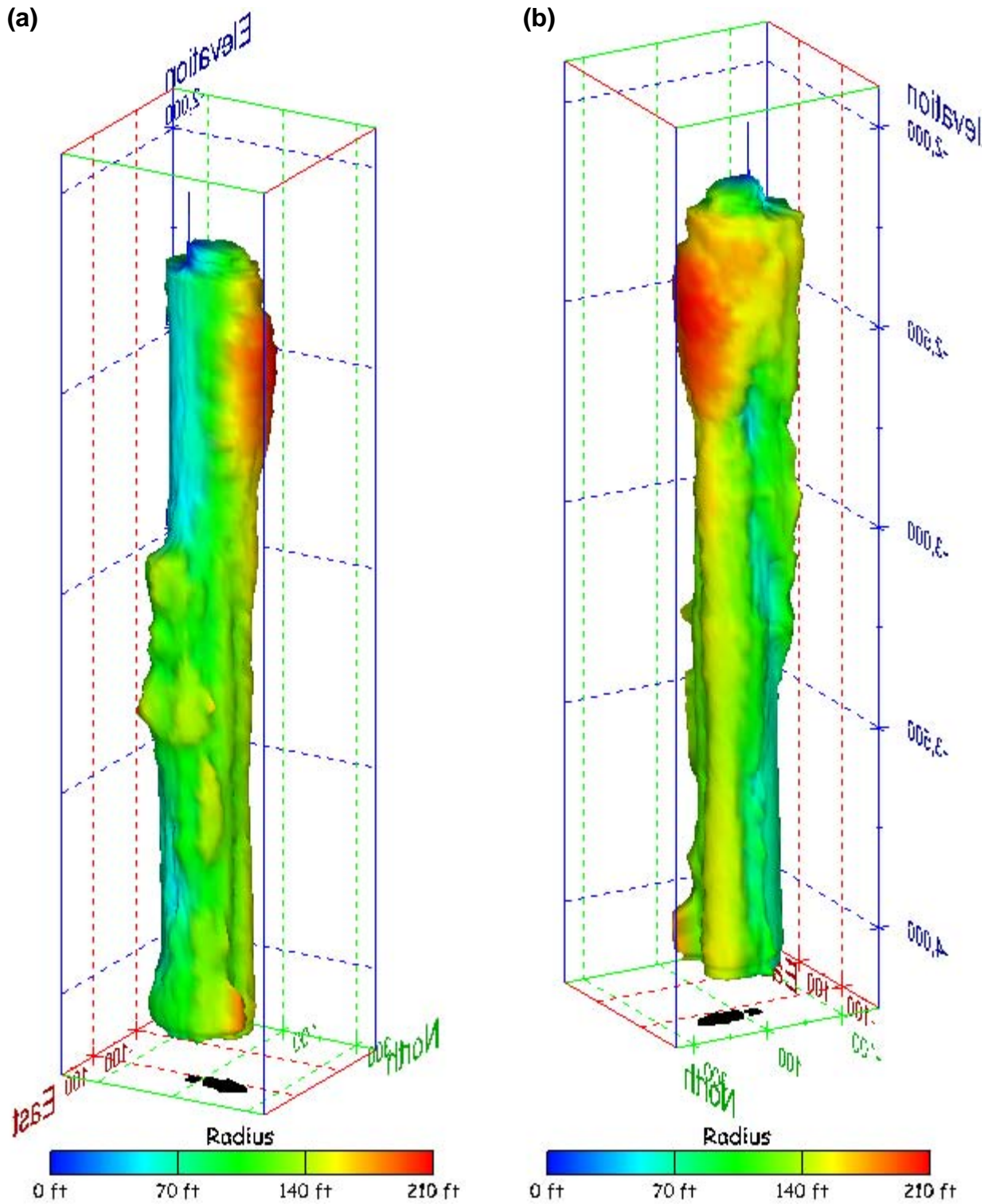
Figure 331. Sonar images of cavern BM-108, showing the geometry of the cavern colored by measured radius. View from (a) azimuth 60°, elevation 20°; (b) azimuth 300°, elevation 20°.
