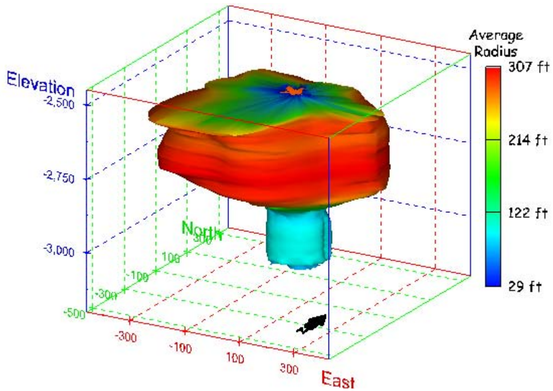
Figure 100. Sonar images of cavern BM-4, showing the geometry of the cavern colored by average radius. View from (a) azimuth 210°, elevation 20°; (b) azimuth 150°, elevation 20°.
