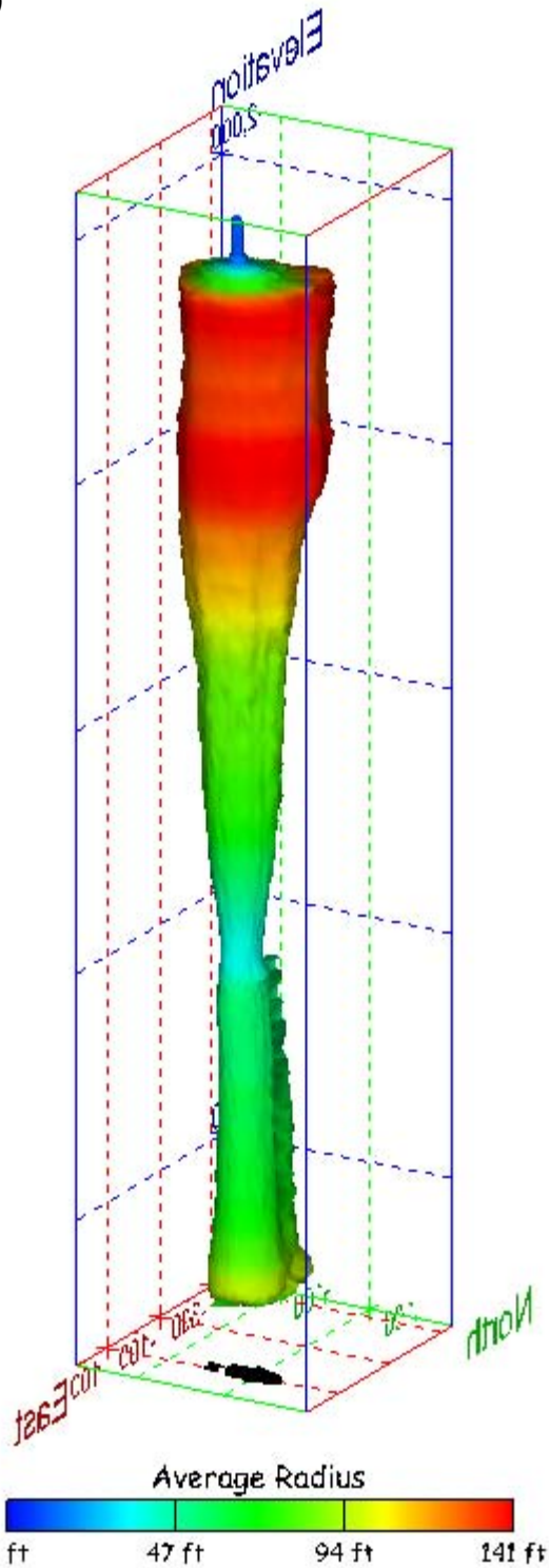
Figure 257. Sonar images of cavern BM-105, showing the geometry of the cavern colored by average radius. View from (a) azimuth 60°, elevation 20°; (b) azimuth 300°, elevation 20°.
