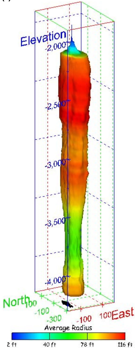
Figure 178. Sonar images of cavern BM-102, showing the geometry of the cavern colored by average radius. View from (a) azimuth 210°, elevation 20°; (b) azimuth 150°, elevation 20°.
