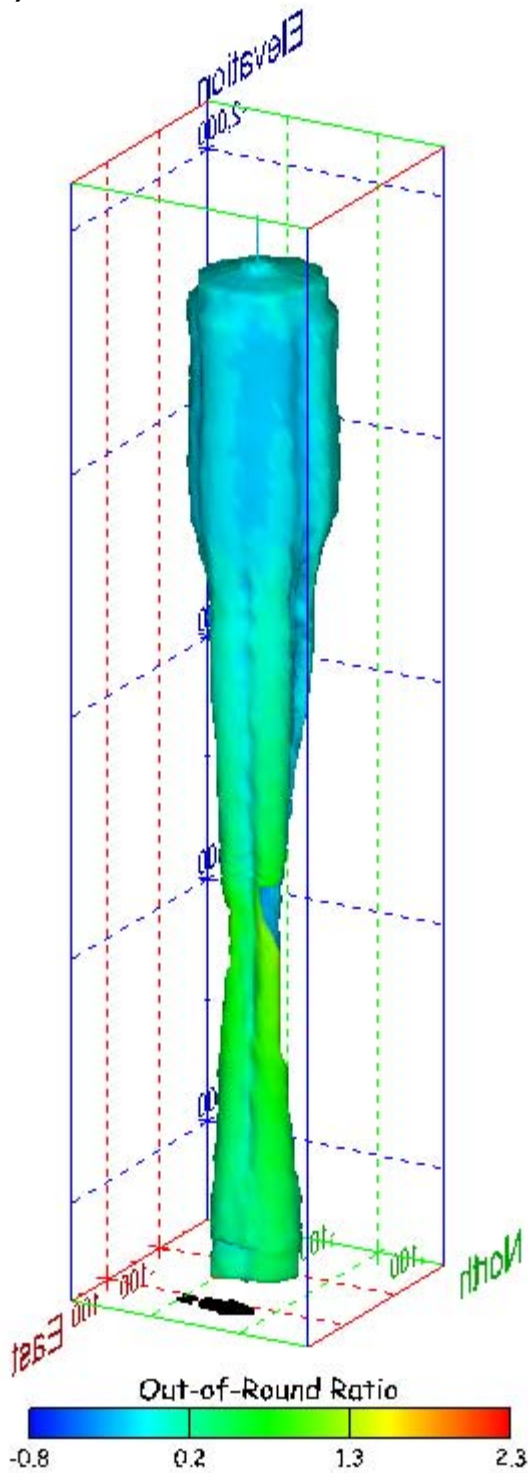
Figure 241. Sonar images of cavern BM-104, showing the geometry of the cavern colored by out-of-round ratio. View from (a) azimuth 60°, elevation 20°; (b) azimuth 300°, elevation 20°.
