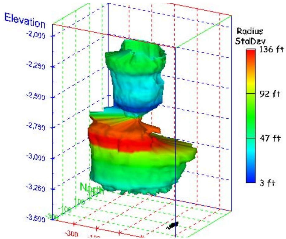
Figure 132. Sonar images of cavern BM-5, showing the geometry of the cavern colored by radius standard deviation. View from (a) azimuth 210°, elevation 20°; (b) azimuth 150°, elevation 20°.
