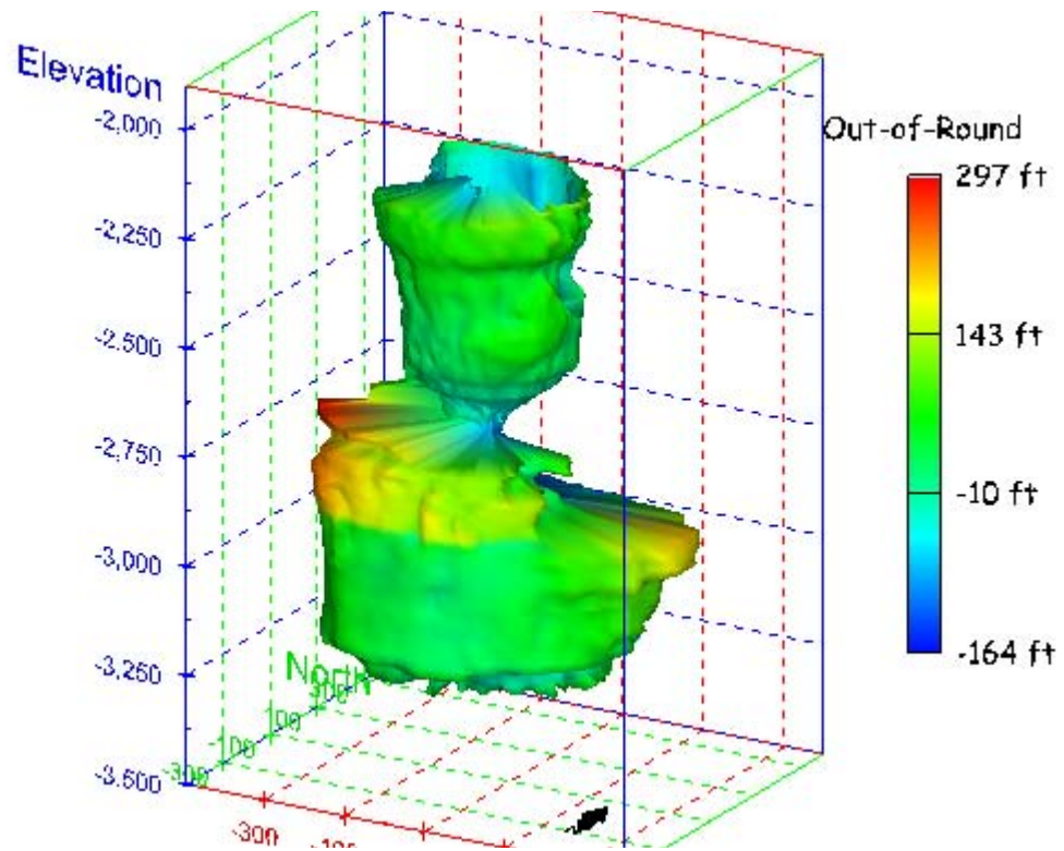
Figure 134. Sonar images of cavern BM-5, showing the geometry of the cavern colored by out-of-round distance. View from (a) azimuth 210°, elevation 20°; (b) azimuth 150°, elevation 20°.
