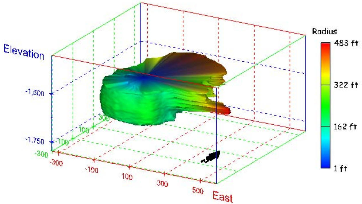
Figure 44. Sonar images of cavern BM-2, showing the geometry of the cavern colored by measured radius. View from (a) azimuth 210°, elevation 20°; (b) azimuth 150°, elevation 20°.
