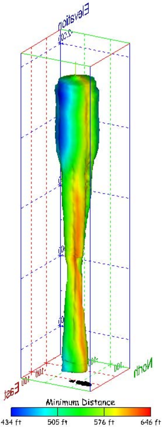
Figure 245. Sonar images of cavern BM-104, showing the geometry of the cavern colored by minimum distance to the nearest neighboring cavern. View from (a) azimuth 60°, elevation 20°; (b) azimuth 300°, elevation 20°.
