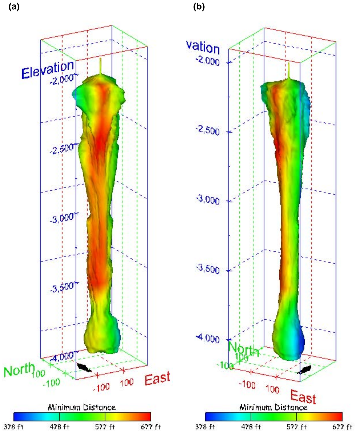
Figure 504. Sonar images of cavern BM-114, showing the geometry of the cavern colored by the minimum distance to the nearest neighboring cavern. View from (a) azimuth 210°, elevation 20°; (b) azimuth 150°, elevation 20°.
