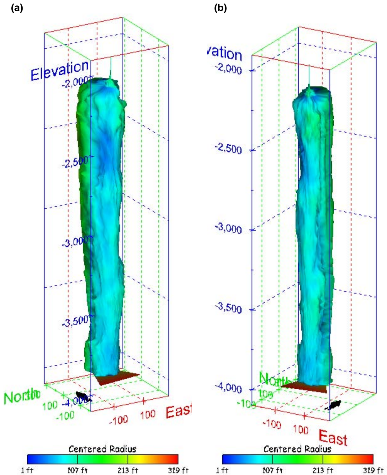
Figure 436. Sonar images of cavern BM-112, showing the geometry of the cavern colored by centered radius. View from (a) azimuth 210°, elevation 20°; (b) azimuth 150°, elevation 20°.
