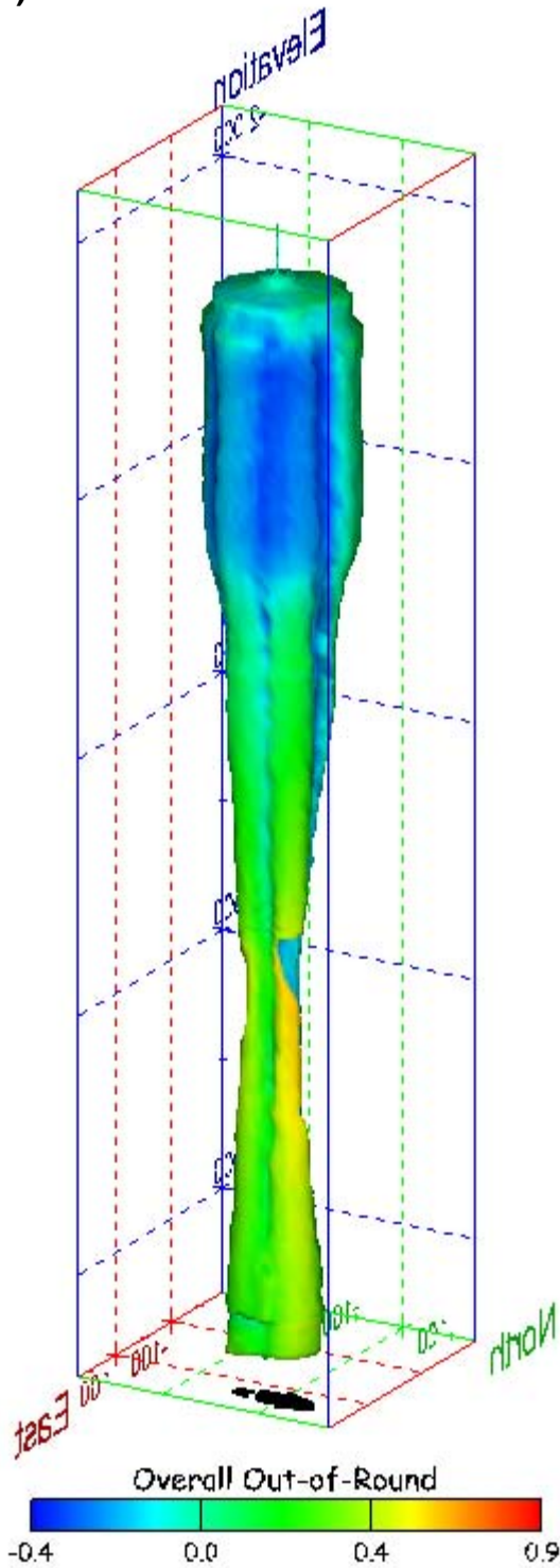
Figure 243. Sonar images of cavern BM-104, showing the geometry of the cavern colored by overall out-of-round ratio. View from (a) azimuth 60°, elevation 20°; (b) azimuth 300°, elevation 20°.
