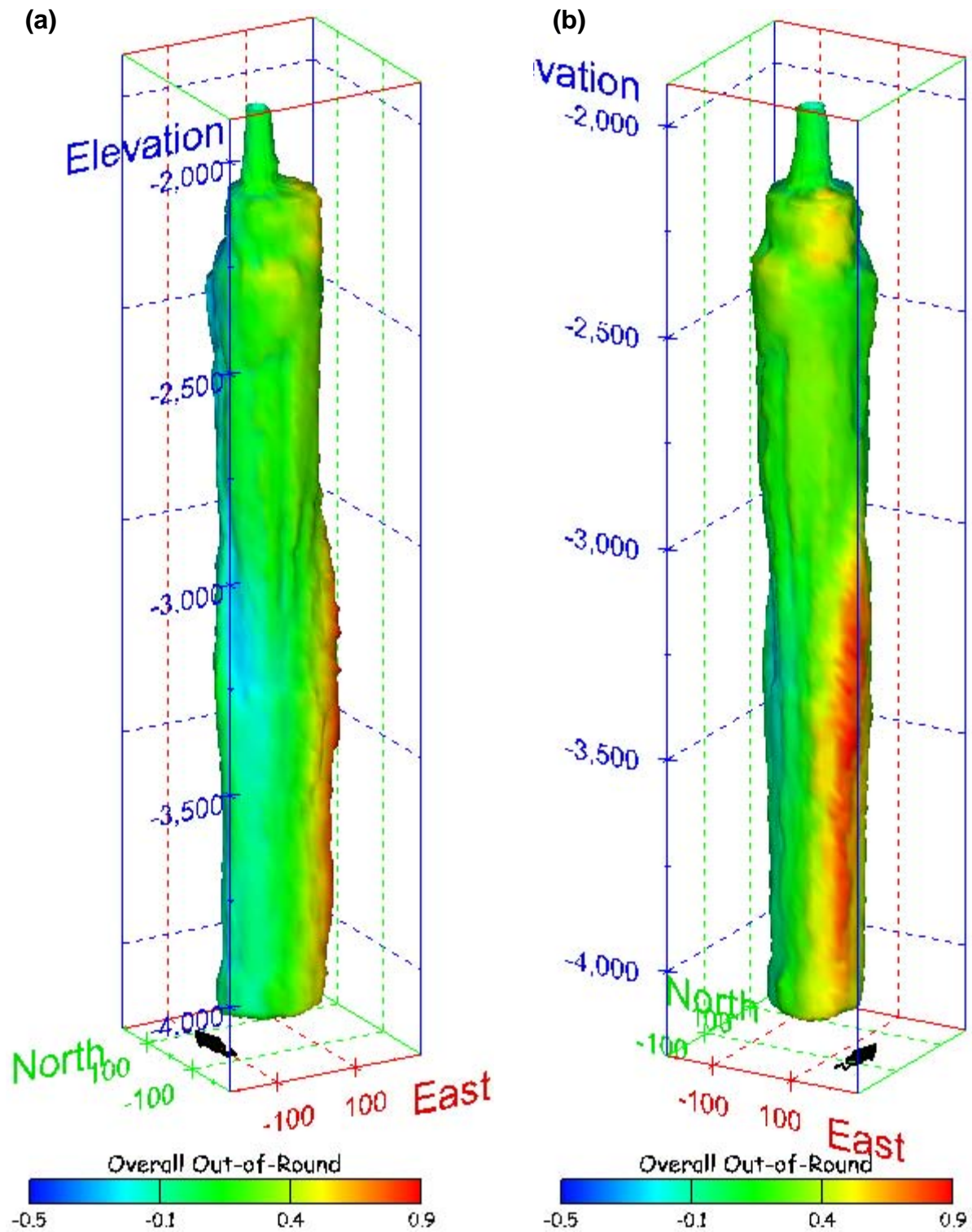
Figure 164. Sonar images of cavern BM-101, showing the geometry of the cavern colored by overall out-of-round ratio. View from (a) azimuth 210°, elevation 20°; (b) azimuth 150°, elevation 20°.
