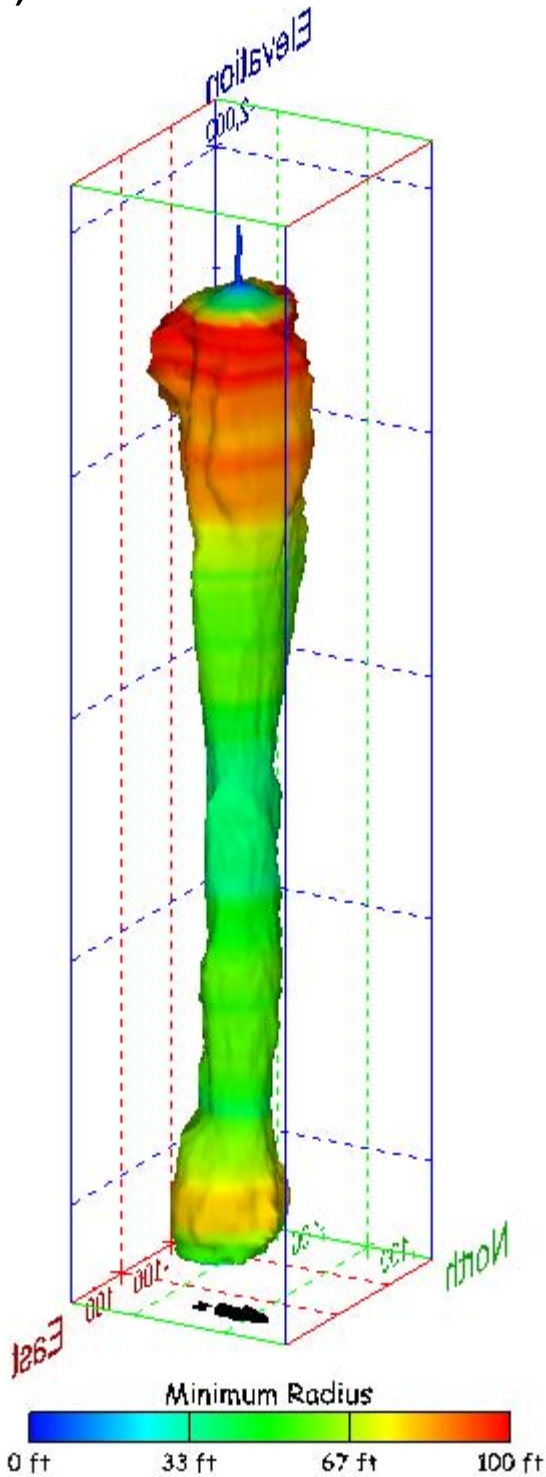
Figure 493. Sonar images of cavern BM-114, showing the geometry of the cavern colored by minimum radius. View from (a) azimuth 60°, elevation 20°; (b) azimuth 300°, elevation 20°.
