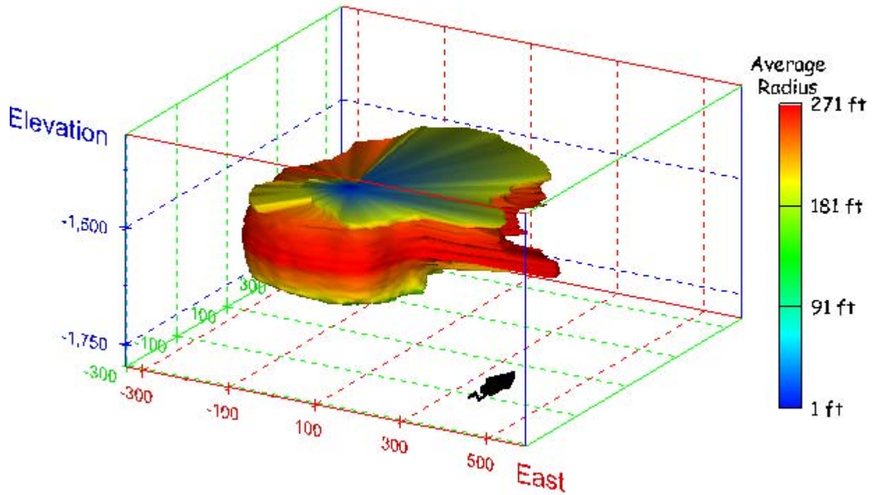
Figure 48. Sonar images of cavern BM-2, showing the geometry of the cavern colored by average radius. View from (a) azimuth 210°, elevation 20°; (b) azimuth 150°, elevation 20°.
