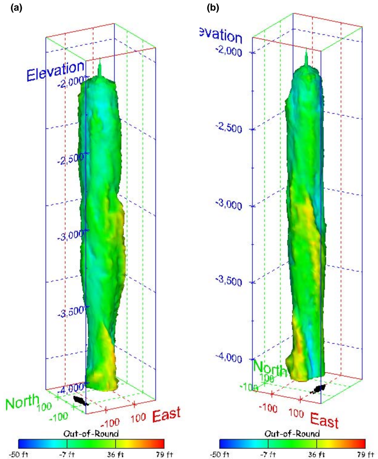
Figure 420. Sonar images of cavern BM-111, showing the geometry of the cavern colored by out-of-round distance. View from (a) azimuth 210°, elevation 20°; (b) azimuth 150°, elevation 20°.
