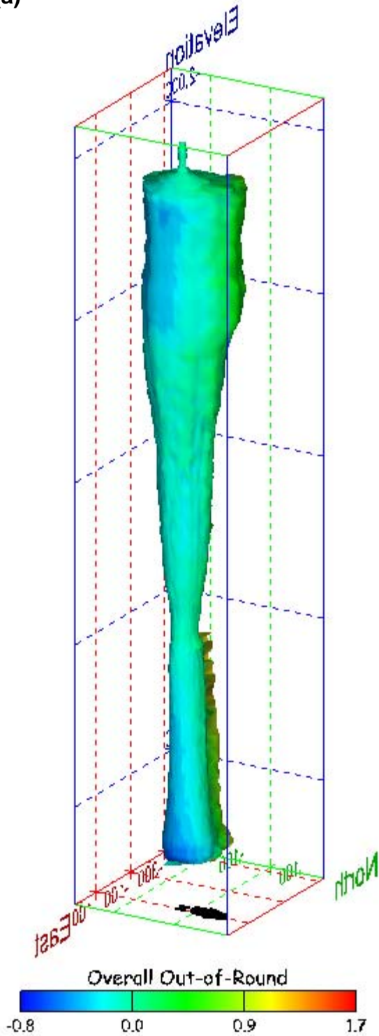
Figure 269. Sonar images of cavern BM-105, showing the geometry of the cavern colored by overall out-of-round ratio. View from (a) azimuth 60°, elevation 20°; (b) azimuth 300°, elevation 20°.
