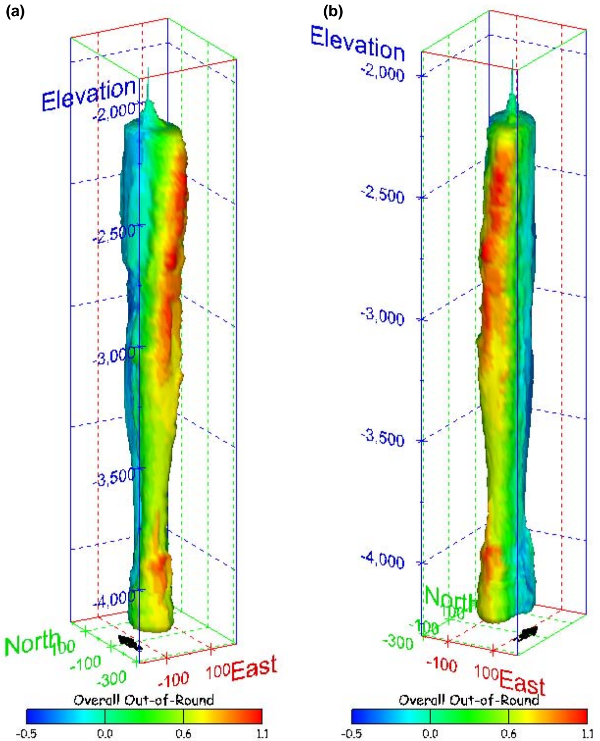
Figure 190. Sonar images of cavern BM-102, showing the geometry of the cavern colored by overall out-of-round ratio. View from (a) azimuth 210°, elevation 20°; (b) azimuth 150°, elevation 20°.
