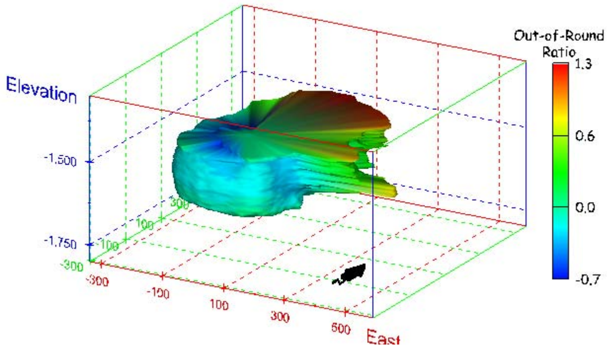
Figure 58. Sonar images of cavern BM-2, showing the geometry of the cavern colored by out-of-round ratio. View from (a) azimuth 210°, elevation 20°; (b) azimuth 150°, elevation 20°.
