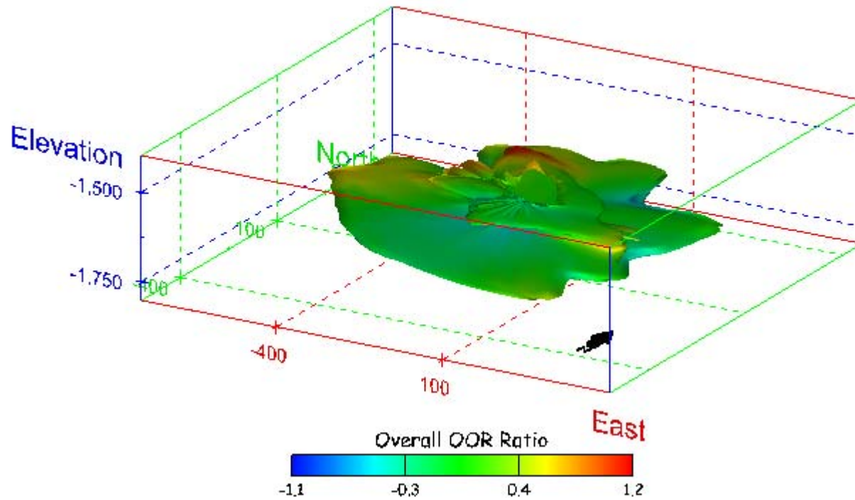
Figure 86. Sonar images of cavern BM-3, showing the geometry of the cavern colored by overall out-of-round ratio. View from (a) azimuth 210°, elevation 20°; (b) azimuth 150°, elevation 20°.
