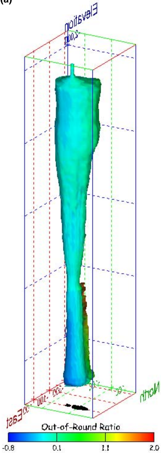
Figure 267. Sonar images of cavern BM-105, showing the geometry of the cavern colored by out-of-round ratio. View from (a) azimuth 60°, elevation 20°; (b) azimuth 300°, elevation 20°.
