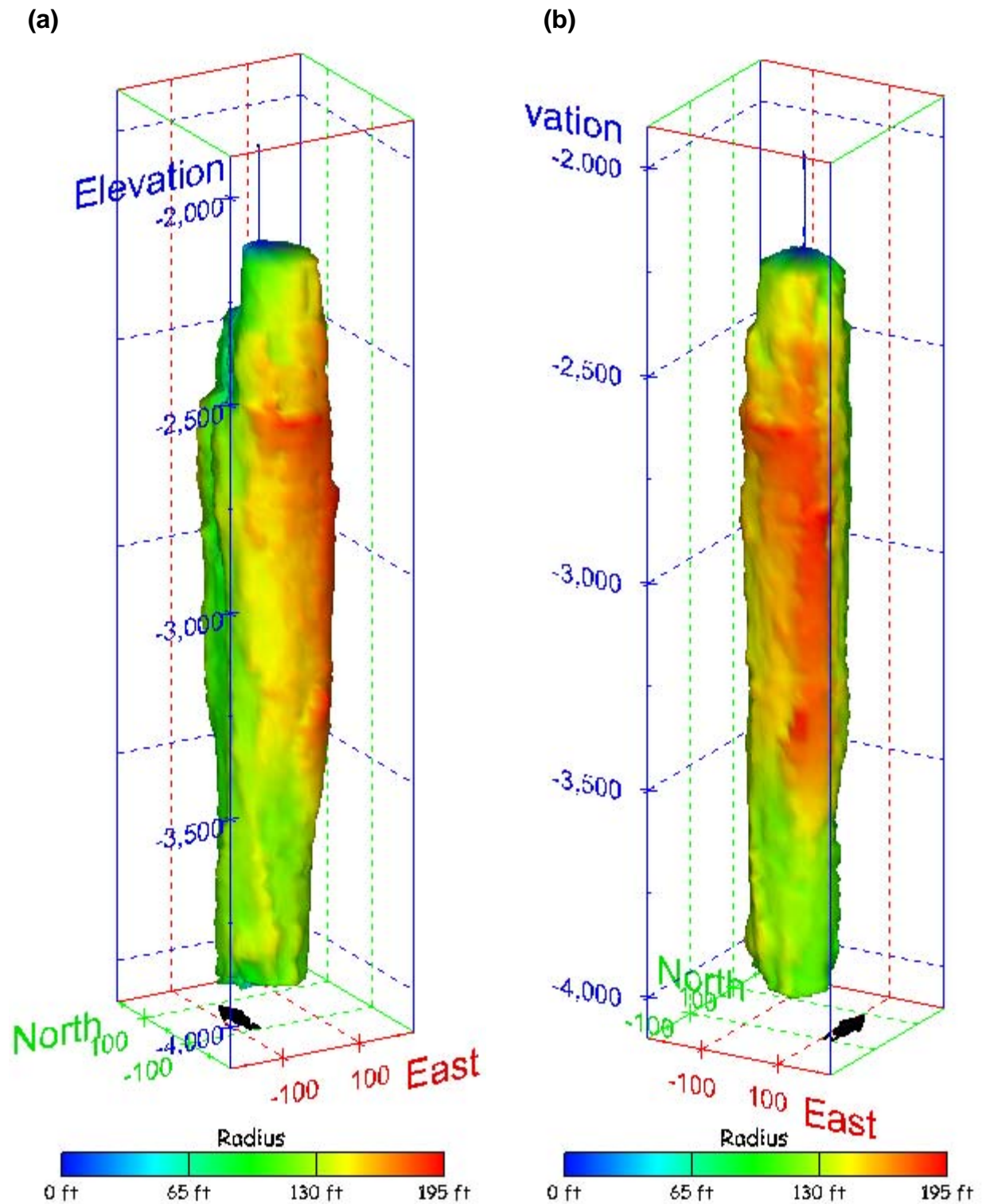
Figure 304. Sonar images of cavern BM-107, showing the geometry of the cavern colored by measured radius. View from (a) azimuth 210°, elevation 20°; (b) azimuth 150°, elevation 20°.
