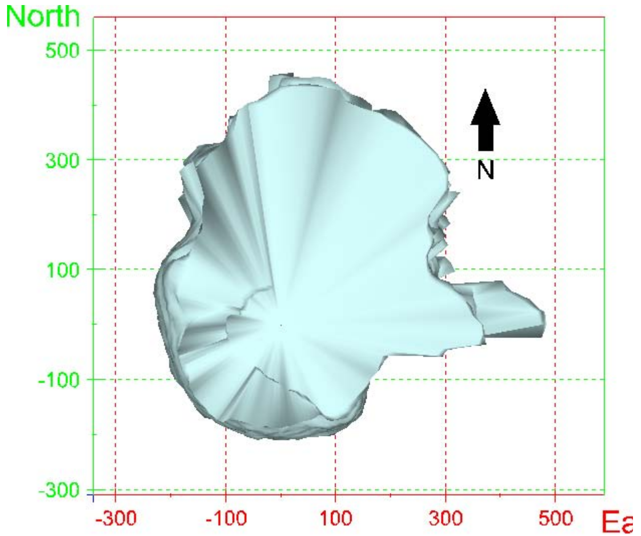
Figure 41. Map view sonar image of cavern BM-2, showing the basic geometry of the cavern. Grid squares represent 200 ft.
