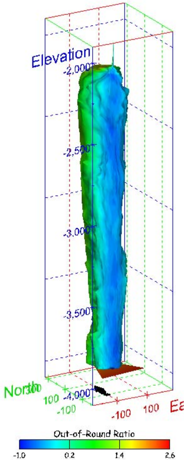
Figure 448. Sonar images of cavern BM-112, showing the geometry of the cavern colored by out-of-round ratio. View from (a) azimuth 210°, elevation 20°; (b) azimuth 150°, elevation 20°.
