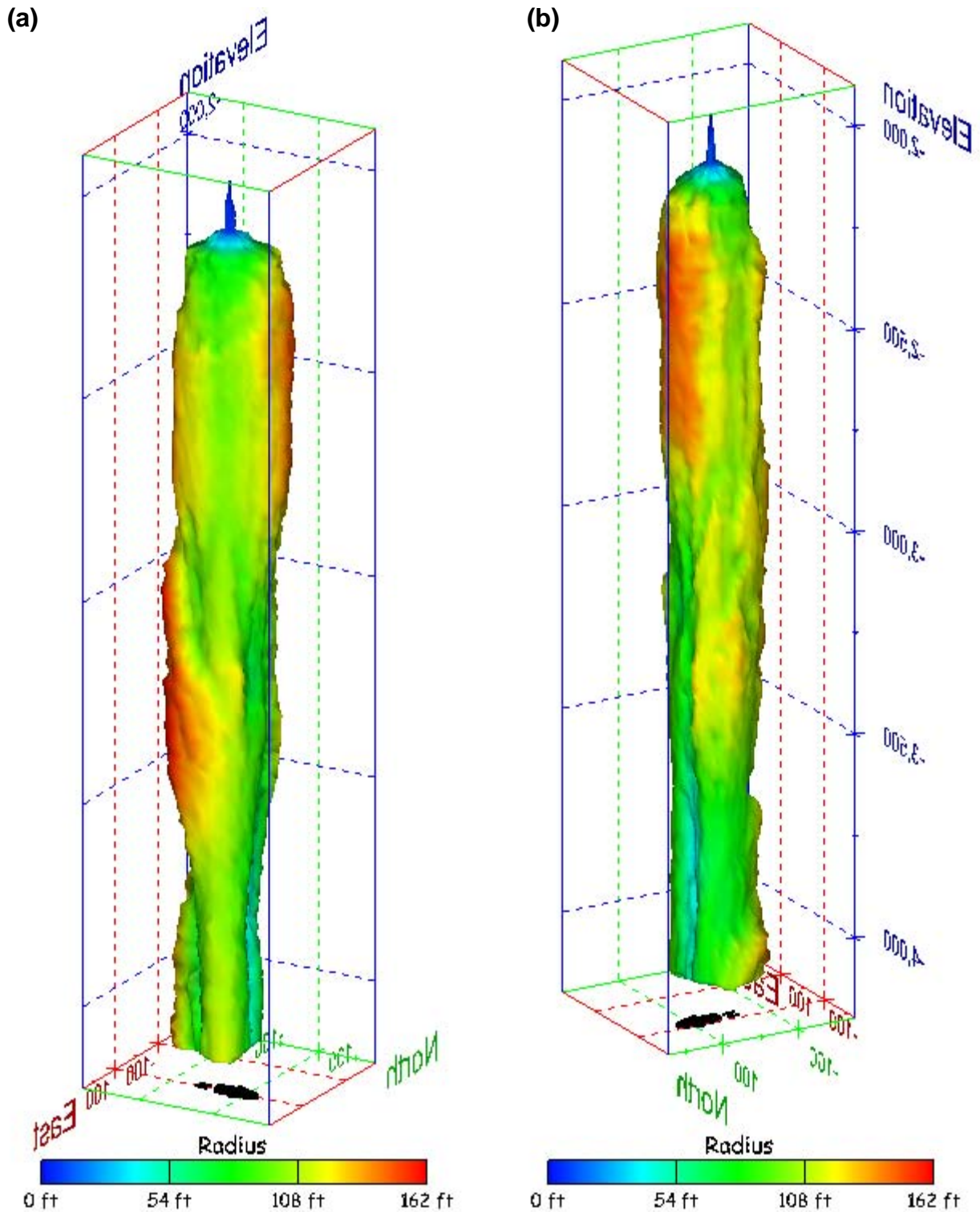
Figure 409. Sonar images of cavern BM-111, showing the geometry of the cavern colored by measured radius. View from (a) azimuth 60°, elevation 20°; (b) azimuth 300°, elevation 20°.
