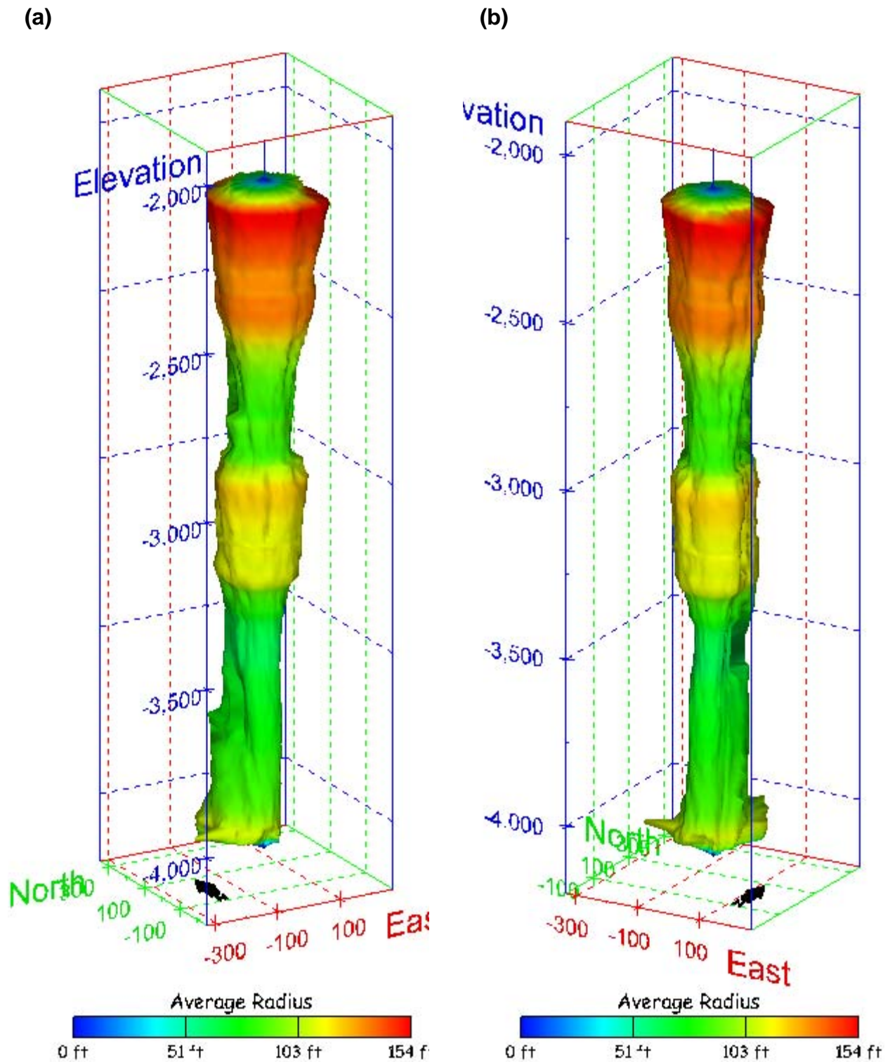
Figure 360. Sonar images of cavern BM-109, showing the geometry of the cavern colored by average radius. View from (a) azimuth 210°, elevation 20°; (b) azimuth 150°, elevation 20°.
