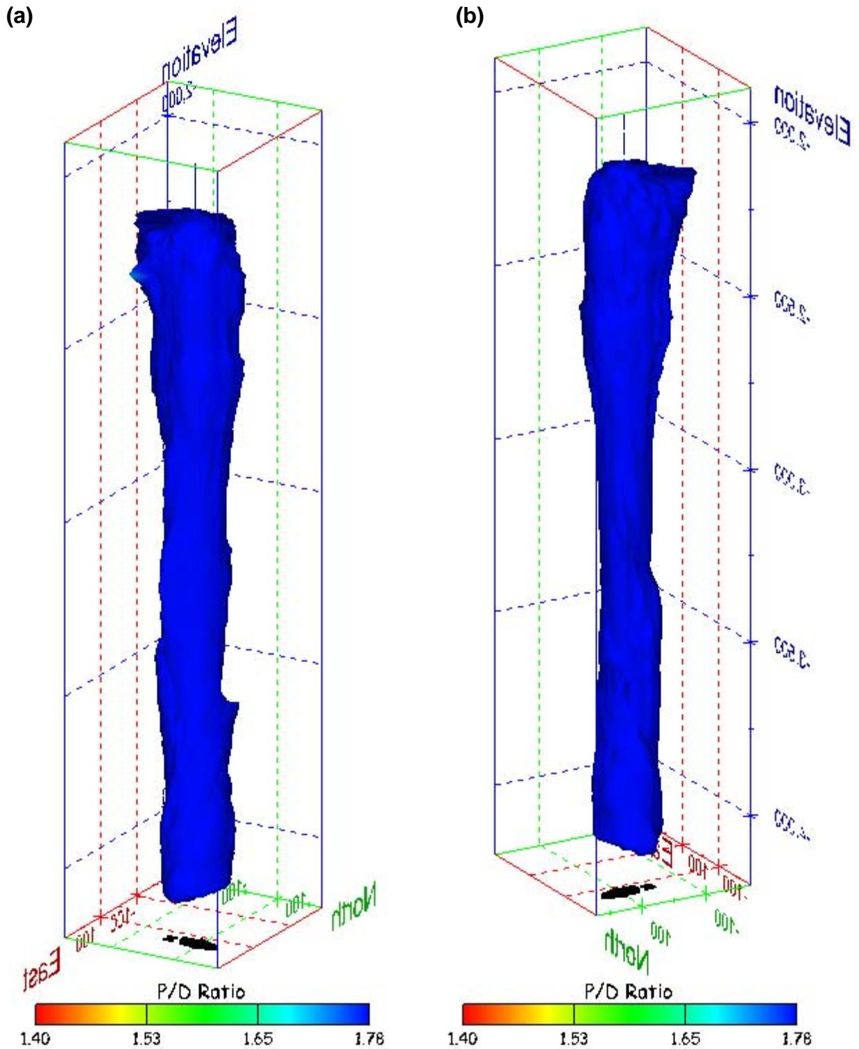
Figure 533. Sonar images of cavern BM-115, showing the geometry of the cavern colored by three-dimensional pillar-to-diameter ratio. View from (a) azimuth 60°, elevation 20°; (b) azimuth 300°, elevation 20°.
