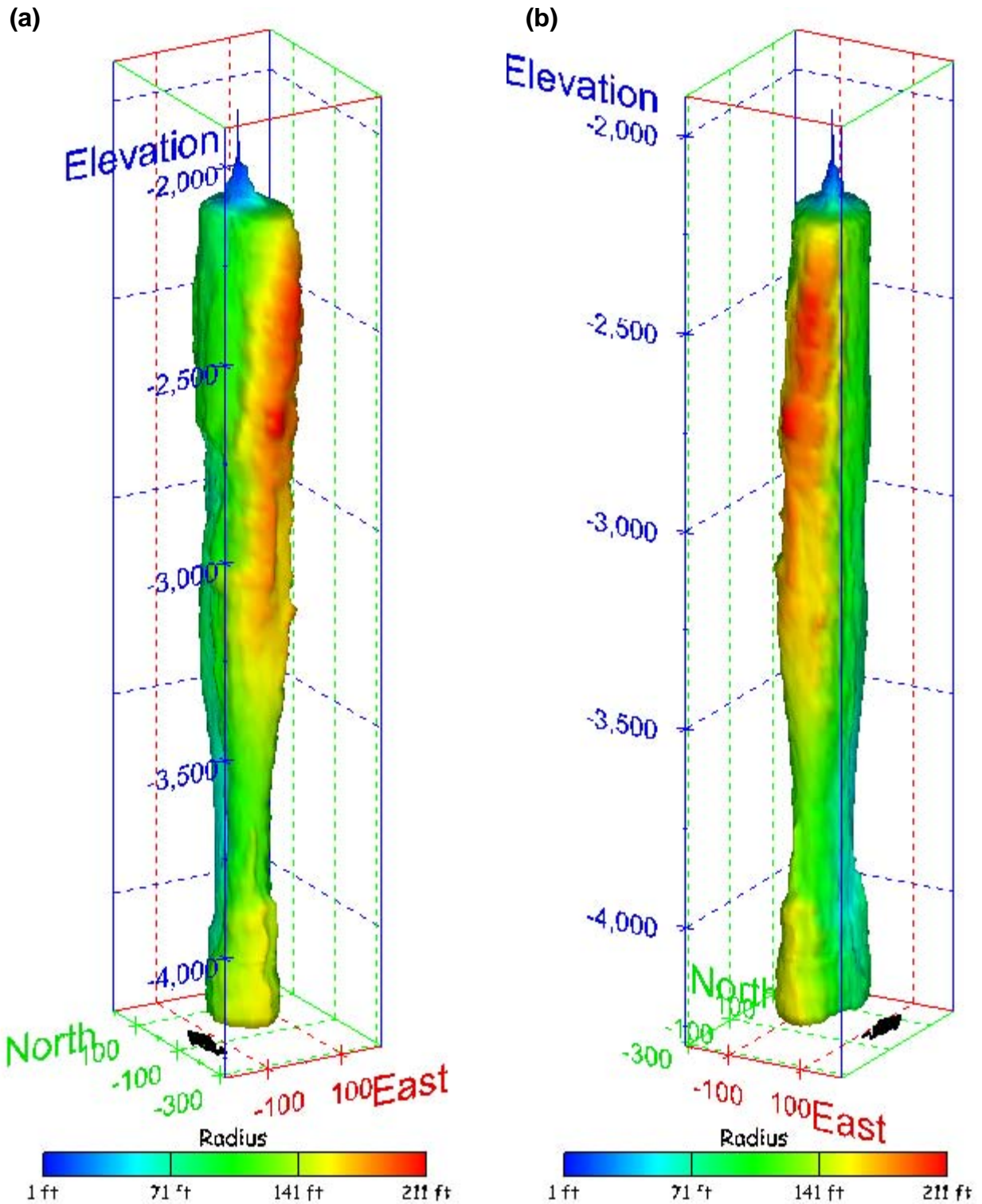
Figure 174. Sonar images of cavern BM-102, showing the geometry of the cavern colored by measured radius. View from (a) azimuth 210°, elevation 20°; (b) azimuth 150°, elevation 20°.
