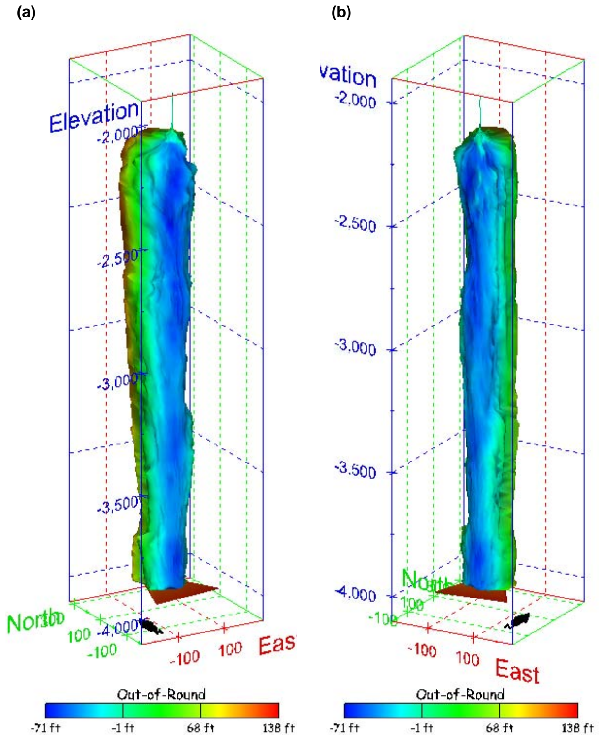
Figure 446. Sonar images of cavern BM-112, showing the geometry of the cavern colored by out-of-round distance. View from (a) azimuth 210°, elevation 20°; (b) azimuth 150°, elevation 20°.
