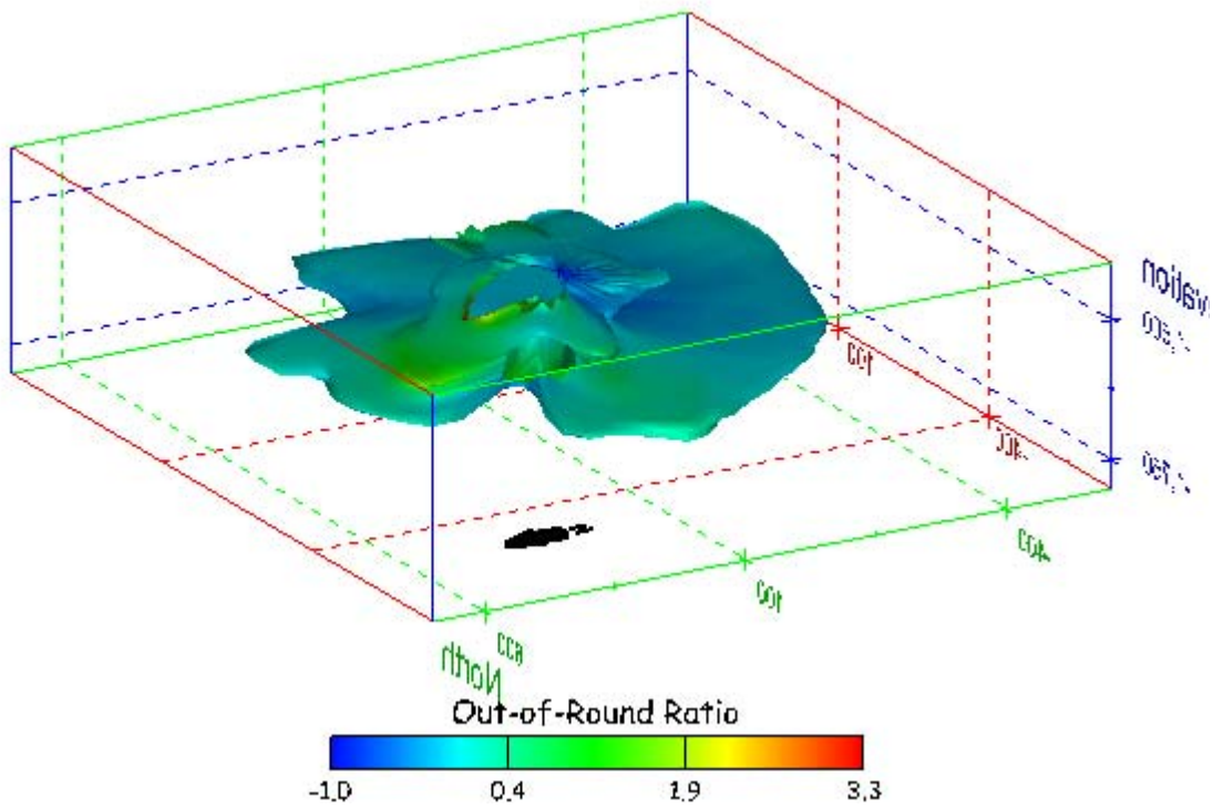
Figure 85. Sonar images of cavern BM-3, showing the geometry of the cavern colored by out-of-round ratio. View from (a) azimuth 60°, elevation 20°; (b) azimuth 300°, elevation 20°.
