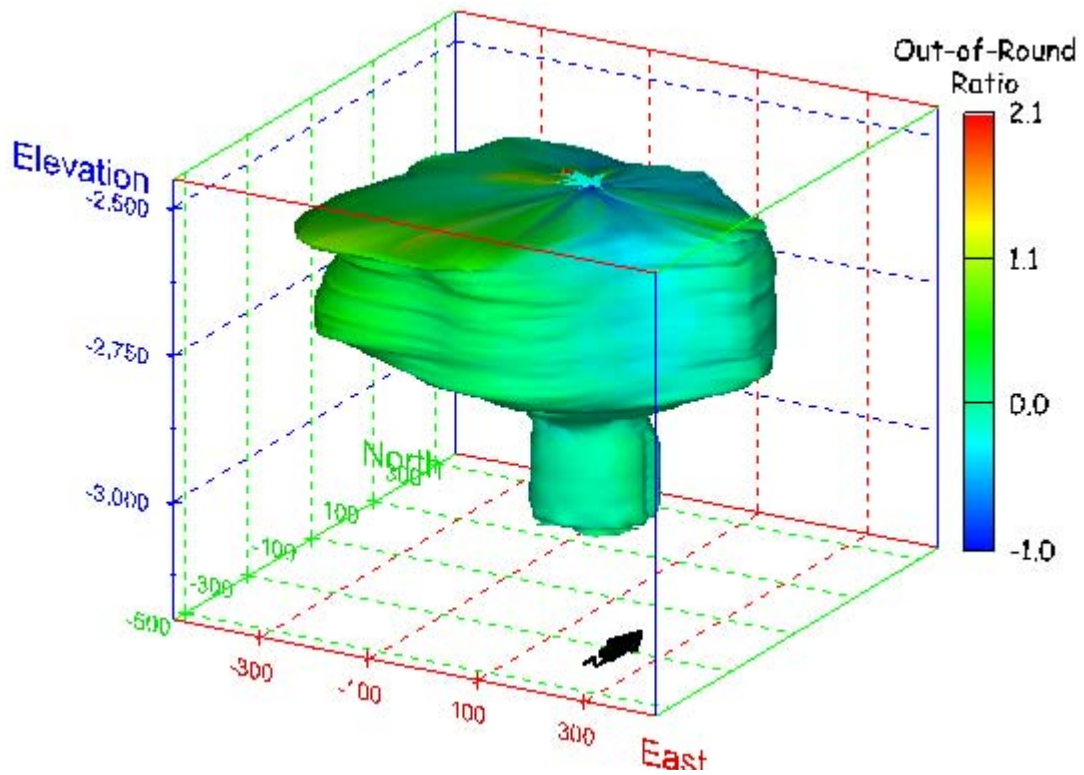
Figure 110. Sonar images of cavern BM-4, showing the geometry of the cavern colored by out-of-round ratio. View from (a) azimuth 210°, elevation 20°; (b) azimuth 150°, elevation 20°.
