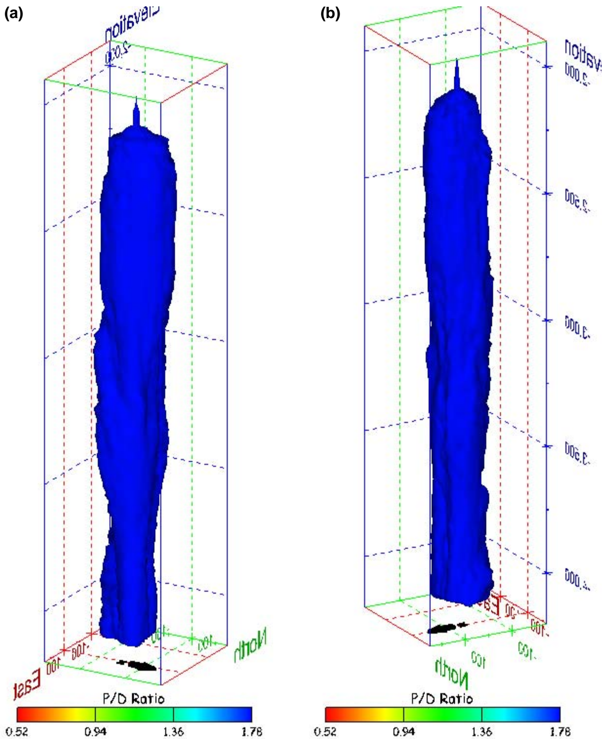
Figure 429. Sonar images of cavern BM-111, showing the geometry of the cavern colored by three-dimensional pillar-to-diameter ratio. View from (a) azimuth 60°, elevation 20°; (b) azimuth 300°, elevation 20°.
