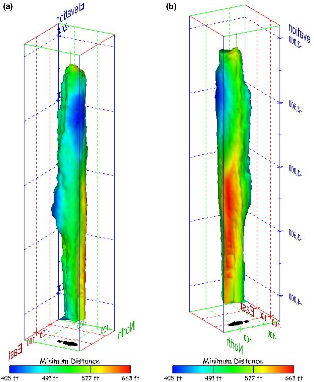
Figure 401. Sonar images of cavern BM-110, showing the geometry of the cavern colored by minimum distance to the nearest neighboring cavern. View from (a) azimuth 60°, elevation 20°; (b) azimuth 300°, elevation 20°.
