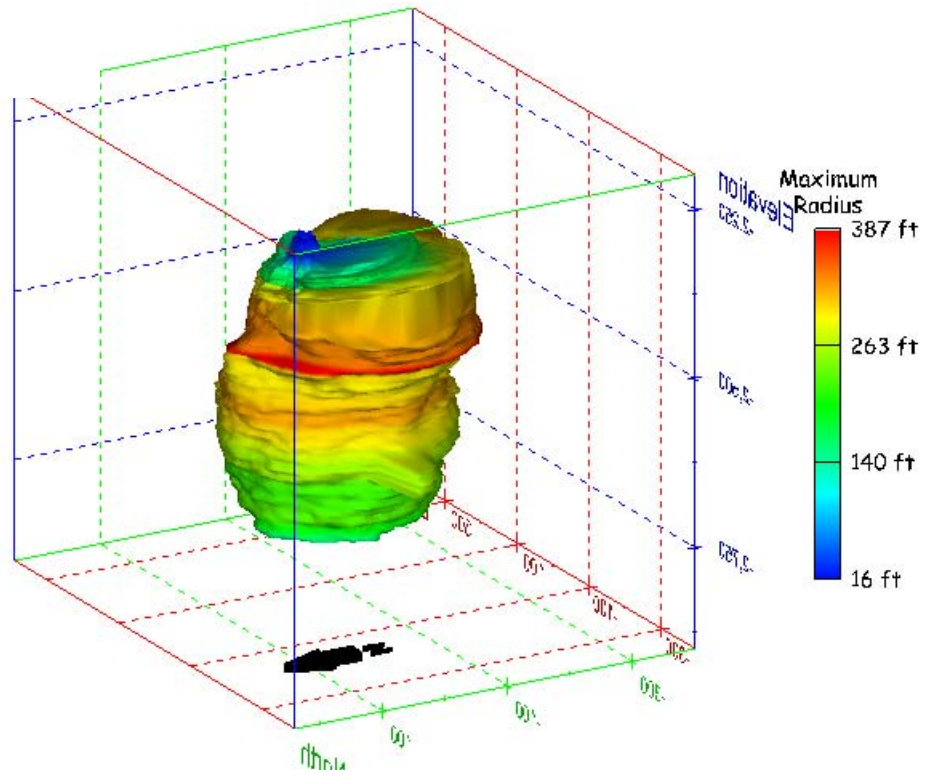
Figure 27. Sonar images of cavern BM-1, showing the geometry of the cavern colored by maximum radius. View from (a) azimuth 60°, elevation 20°; (b) azimuth 300°, elevation 20°.
