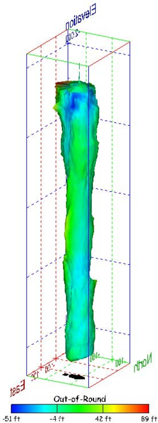
Figure 525. Sonar images of cavern BM-115, showing the geometry of the cavern colored by out-of-round distance. View from (a) azimuth 60°, elevation 20°; (b) azimuth 300°, elevation 20°.
