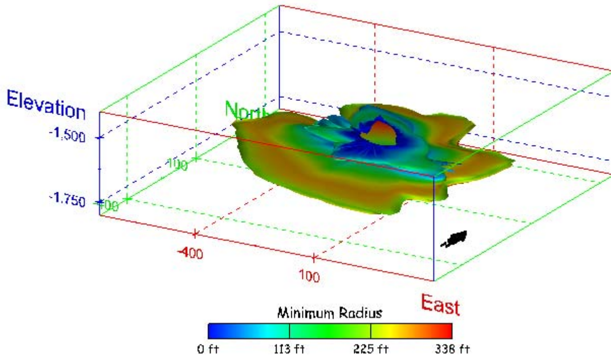
Figure 76. Sonar images of cavern BM-3, showing the geometry of the cavern colored by minimum radius. View from (a) azimuth 210°, elevation 20°; (b) azimuth 150°, elevation 20°.
