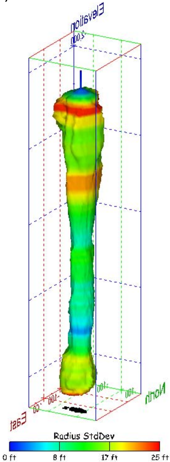
Figure 497. Sonar images of cavern BM-114, showing the geometry of the cavern colored by radius standard deviation. View from (a) azimuth 60°, elevation 20°; (b) azimuth 300°, elevation 20°.
