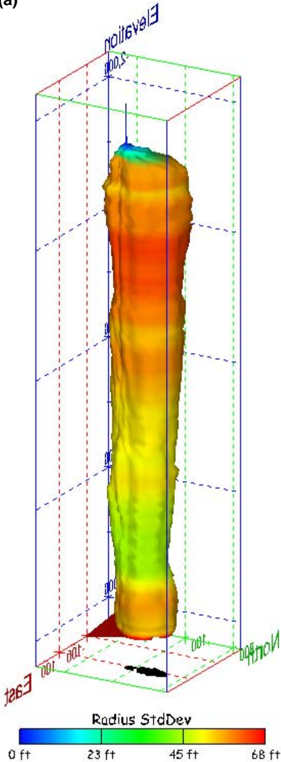
Figure 445. Sonar images of cavern BM-112, showing the geometry of the cavern colored by radius standard deviation. View from (a) azimuth 60°, elevation 20°; (b) azimuth 300°, elevation 20°.
