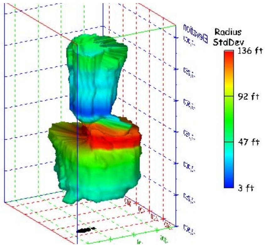
Figure 133. Sonar images of cavern BM-5, showing the geometry of the cavern colored by radius standard deviation. View from (a) azimuth 60°, elevation 20°; (b) azimuth 300°, elevation 20°.
