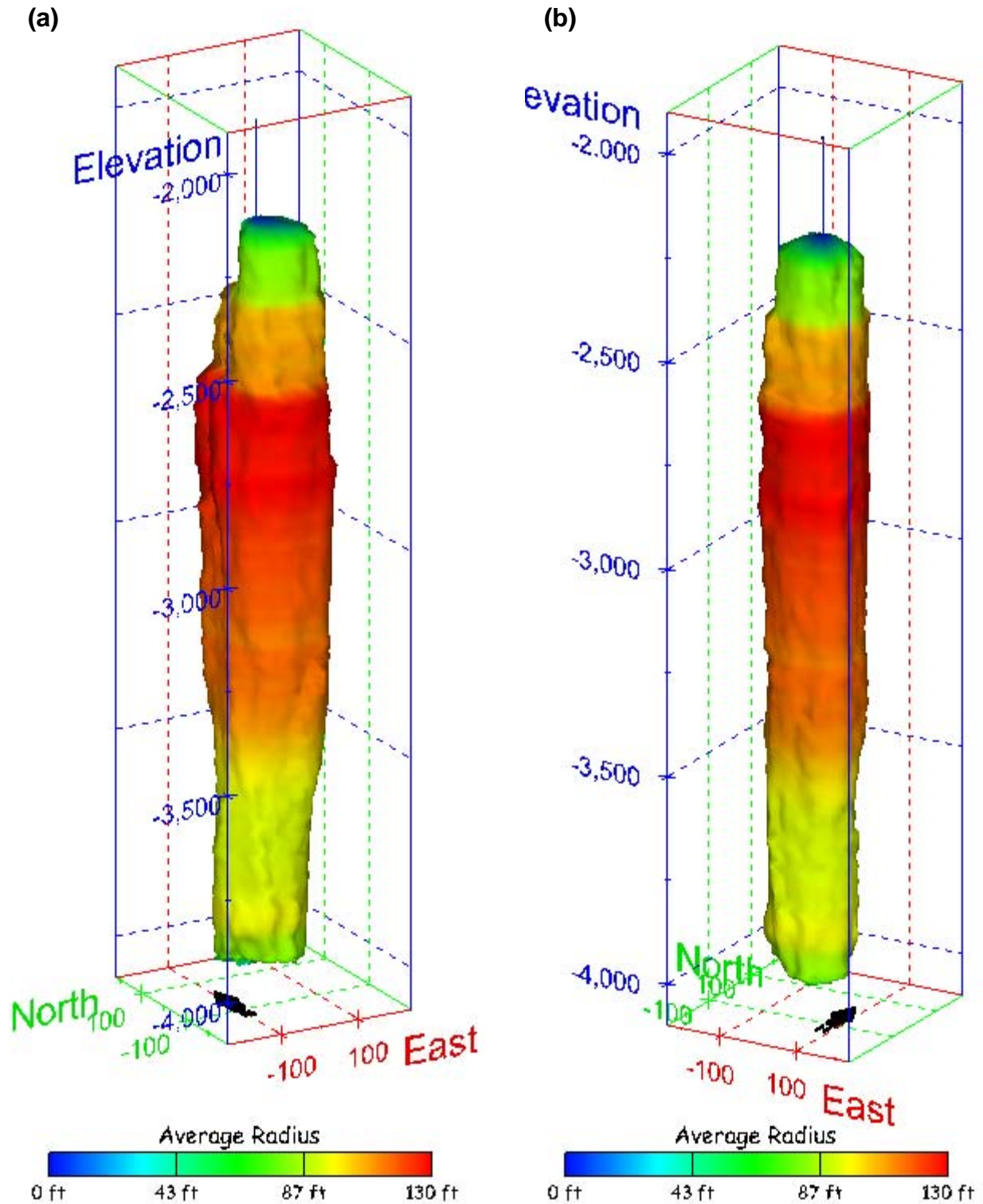
Figure 308. Sonar images of cavern BM-107, showing the geometry of the cavern colored by average radius. View from (a) azimuth 210°, elevation 20°; (b) azimuth 150°, elevation 20°.
