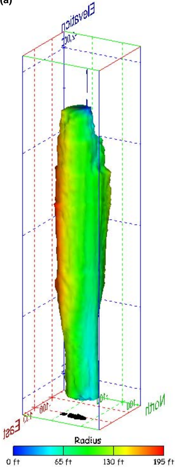
Figure 305. Sonar images of cavern BM-107, showing the geometry of the cavern colored by measured radius. View from (a) azimuth 60°, elevation 20°; (b) azimuth 300°, elevation 20°.
