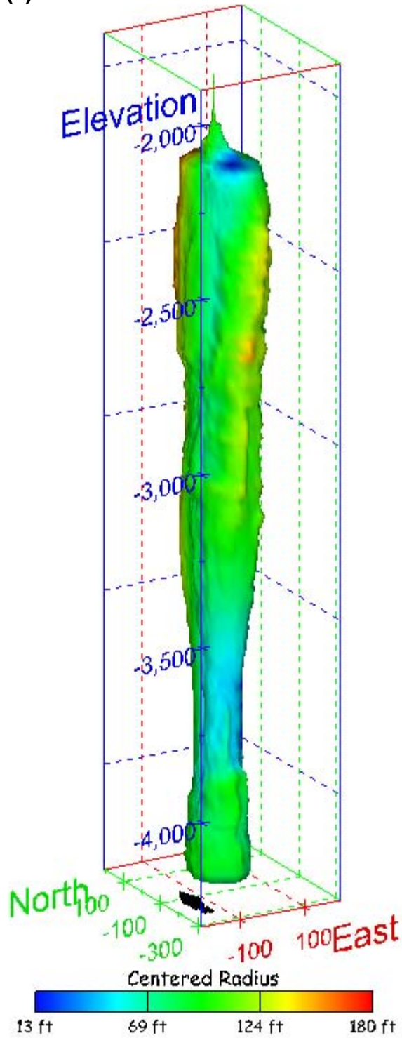
Figure 176. Sonar images of cavern BM-102, showing the geometry of the cavern colored by centered radius. View from (a) azimuth 210°, elevation 20°; (b) azimuth 150°, elevation 20°.
