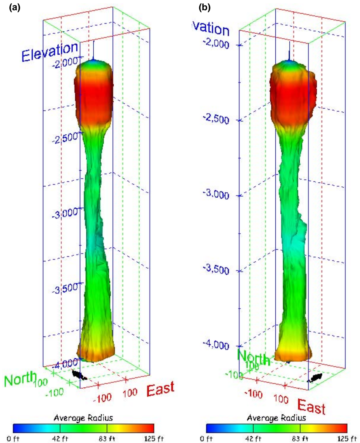
Figure 464. Sonar images of cavern BM-113, showing the geometry of the cavern colored by average radius. View from (a) azimuth 210°, elevation 20°; (b) azimuth 150°, elevation 20°.
