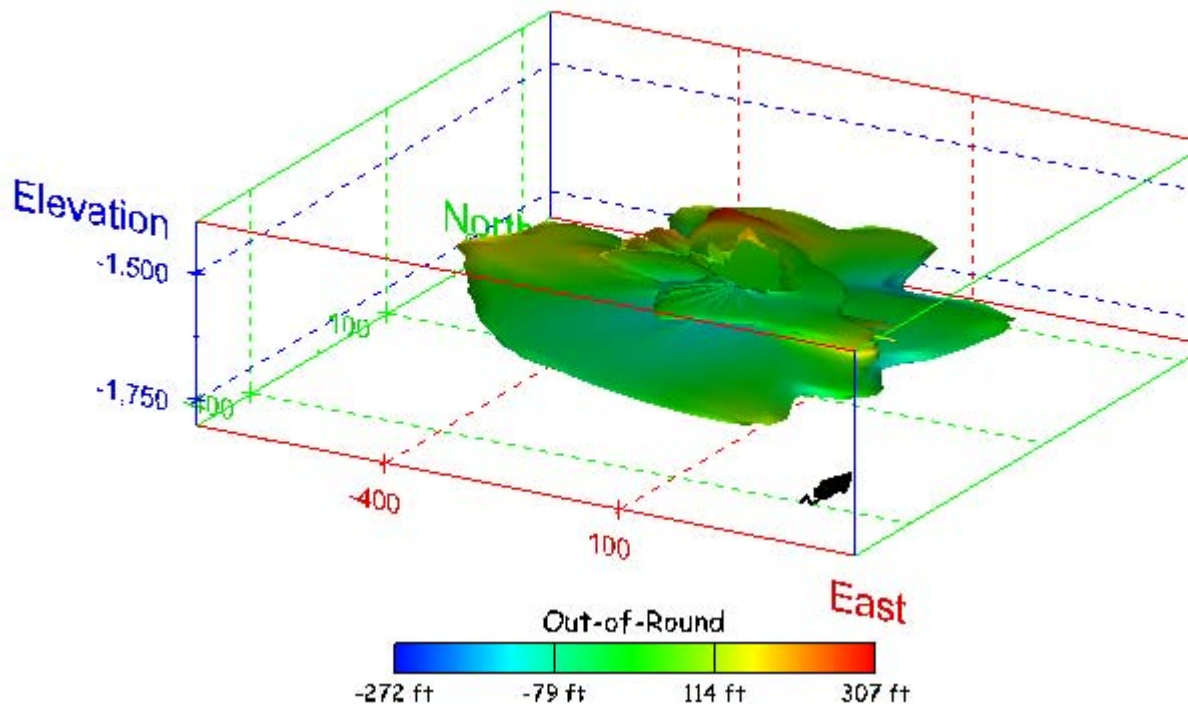
Figure 82. Sonar images of cavern BM-3, showing the geometry of the cavern colored by out-of-round distance. View from (a) azimuth 210°, elevation 20°; (b) azimuth 150°, elevation 20°.
