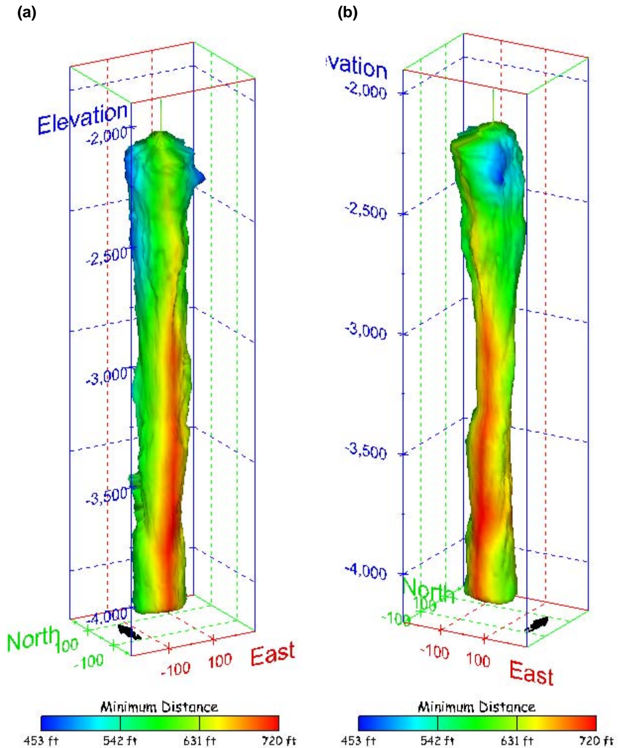
Figure 530. Sonar images of cavern BM-115, showing the geometry of the cavern colored by the minimum distance to the nearest neighboring cavern. View from (a) azimuth 210°, elevation 20°; (b) azimuth 150°, elevation 20°.
