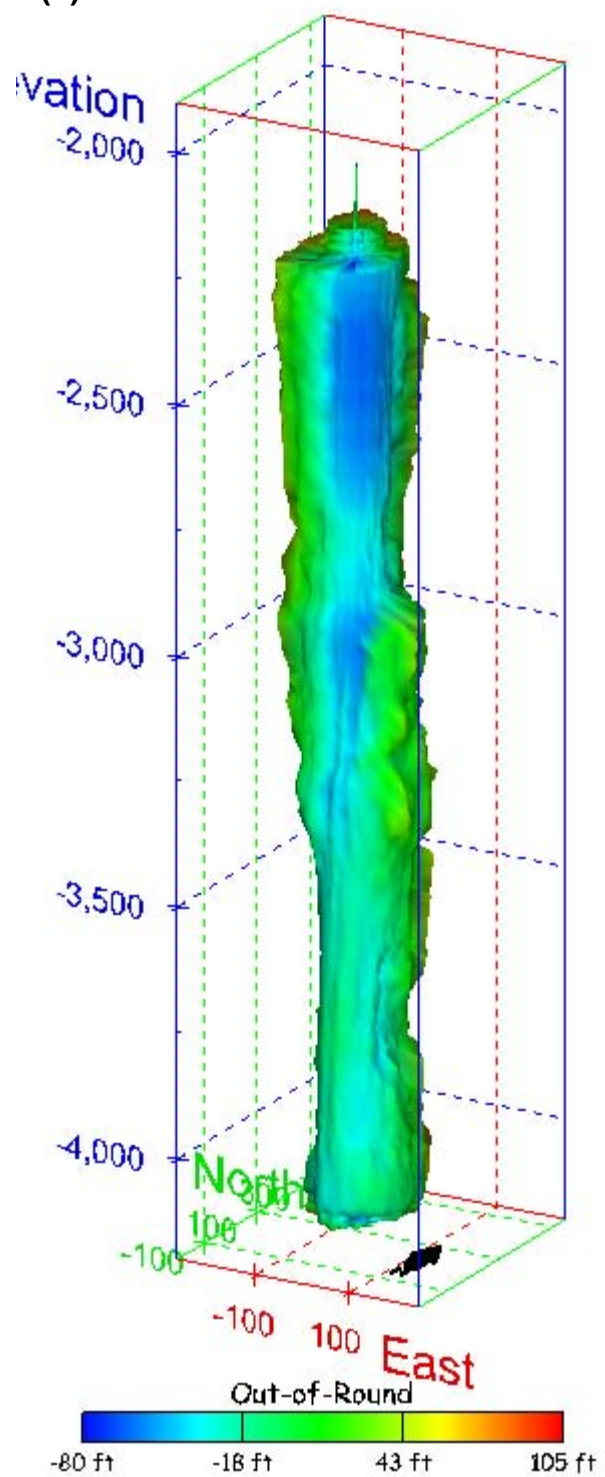
Figure 342. Sonar images of cavern BM-108, showing the geometry of the cavern colored by out-of-round distance. View from (a) azimuth 210°, elevation 20°; (b) azimuth 150°, elevation 20°.
