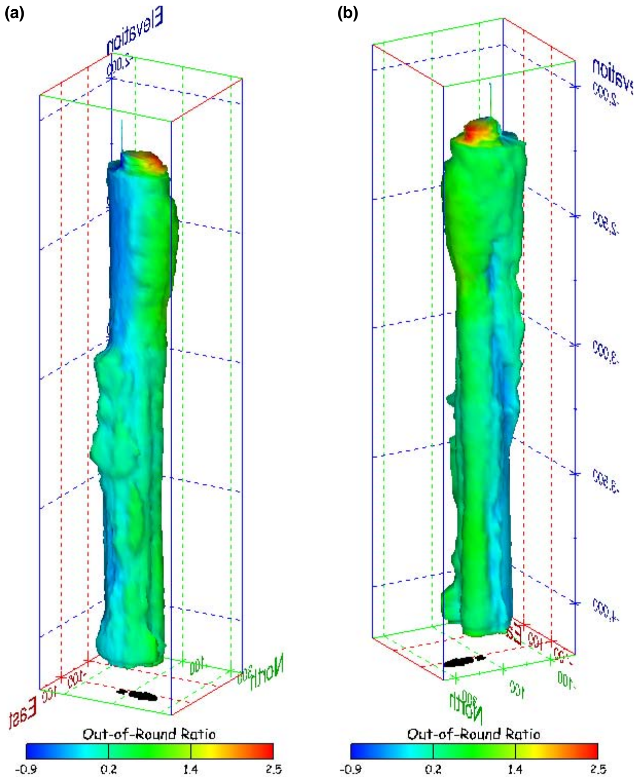
Figure 345. Sonar images of cavern BM-108, showing the geometry of the cavern colored by out-of-round ratio. View from (a) azimuth 60°, elevation 20°; (b) azimuth 300°, elevation 20°.
