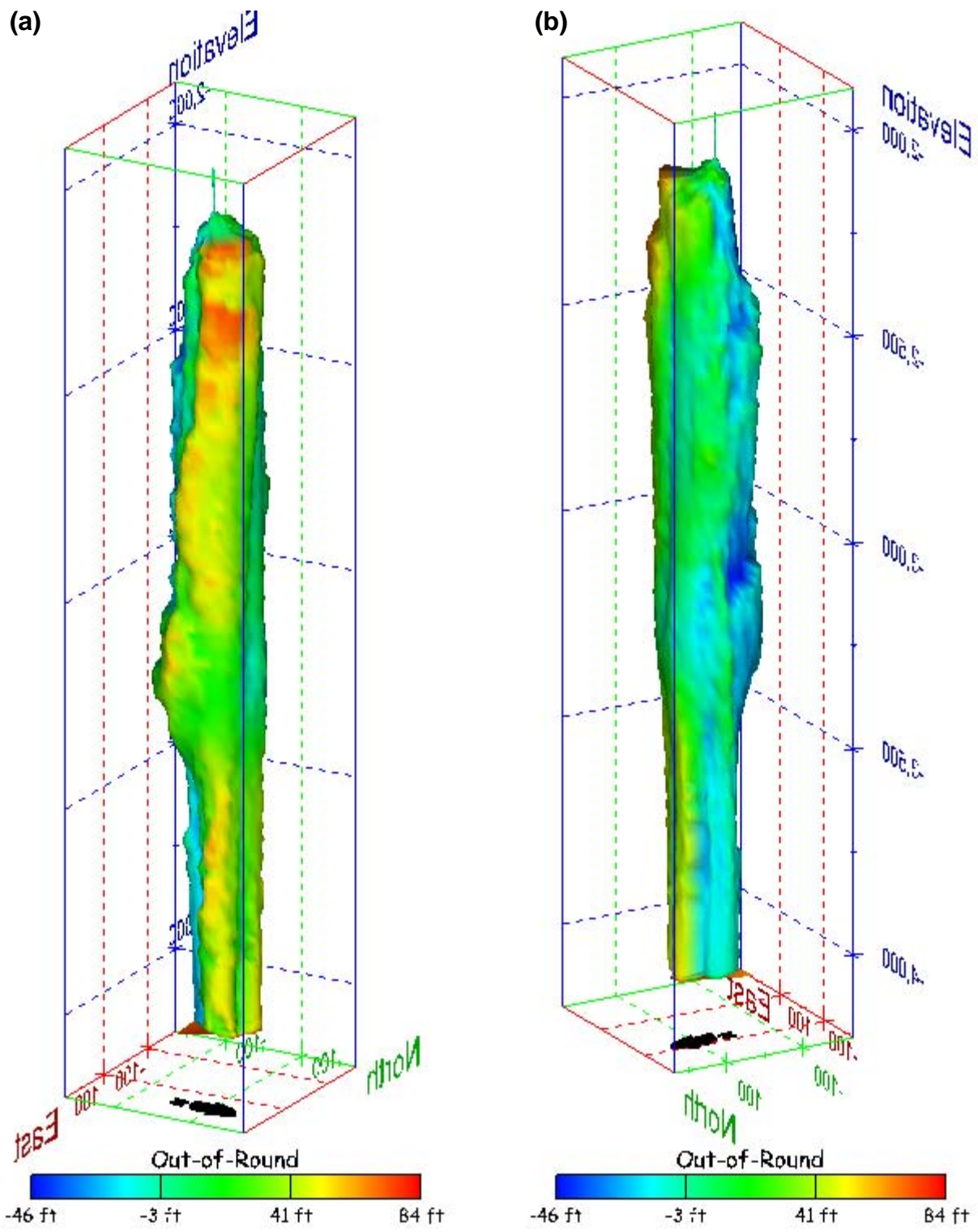
Figure 395. Sonar images of cavern BM-110, showing the geometry of the cavern colored by out-of-round distance. View from (a) azimuth 60°, elevation 20°; (b) azimuth 300°, elevation 20°.
