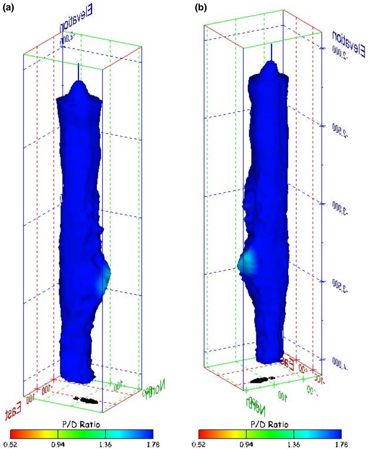
Figure 221. Sonar images of cavern BM-103, showing the geometry of the cavern colored by three-dimensional pillar-to-diameter ratio. View from (a) azimuth 60°, elevation 20°; (b) azimuth 300°, elevation 20°.
