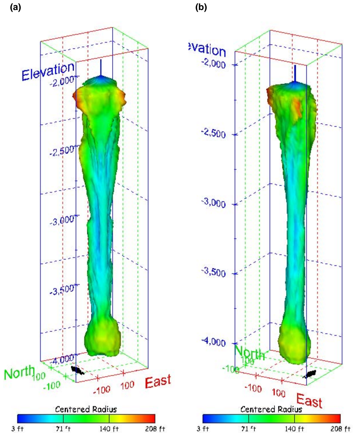
Figure 488. Sonar images of cavern BM-114, showing the geometry of the cavern colored by centered radius. View from (a) azimuth 210°, elevation 20°; (b) azimuth 150°, elevation 20°.
