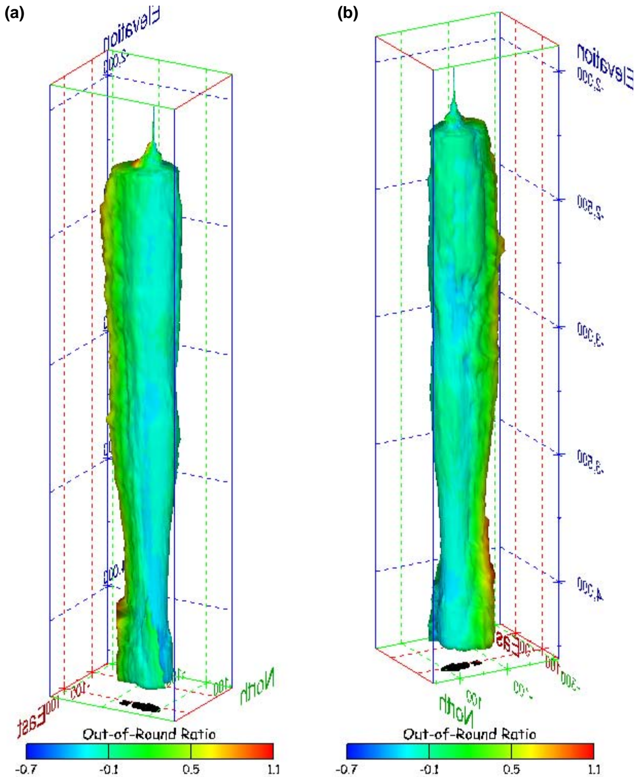
Figure 189. Sonar images of cavern BM-102, showing the geometry of the cavern colored by out-of-round ratio. View from (a) azimuth 60°, elevation 20°; (b) azimuth 300°, elevation 20°.
