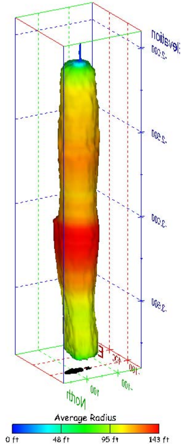
Figure 283. Sonar images of cavern BM-106, showing the geometry of the cavern colored by average radius. View from (a) azimuth 60°, elevation 20°; (b) azimuth 300°, elevation 20°.
