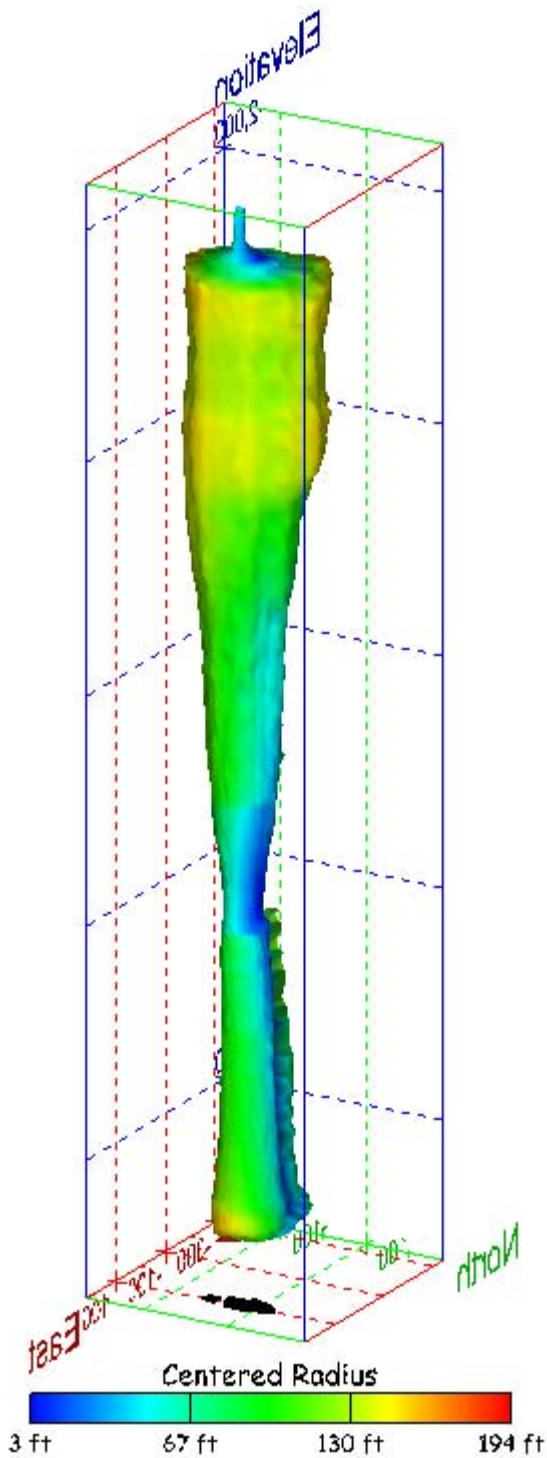
Figure 255. Sonar images of cavern BM-105, showing the geometry of the cavern colored by centered radius. View from (a) azimuth 60°, elevation 20°; (b) azimuth 300°, elevation 20°.
