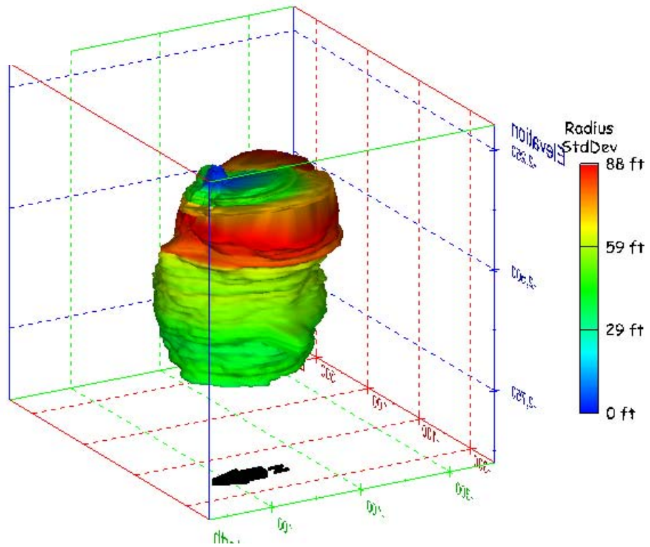
Figure 29. Sonar images of cavern BM-1, showing the geometry of the cavern colored by radius standard deviation. View from (a) azimuth 60°, elevation 20°; (b) azimuth 300°, elevation 20°.
