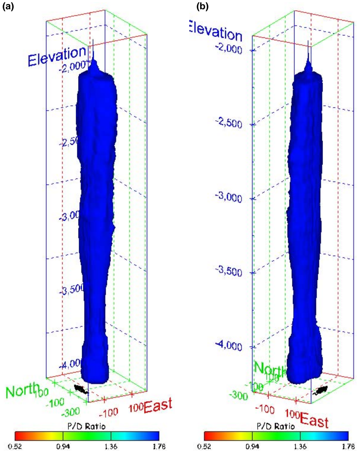
Figure 194. Sonar images of cavern BM-102, showing the geometry of the cavern colored by three-dimensional pillar-to-diameter ratio. View from (a) azimuth 210°, elevation 20°; (b) azimuth 150°, elevation 20°.
