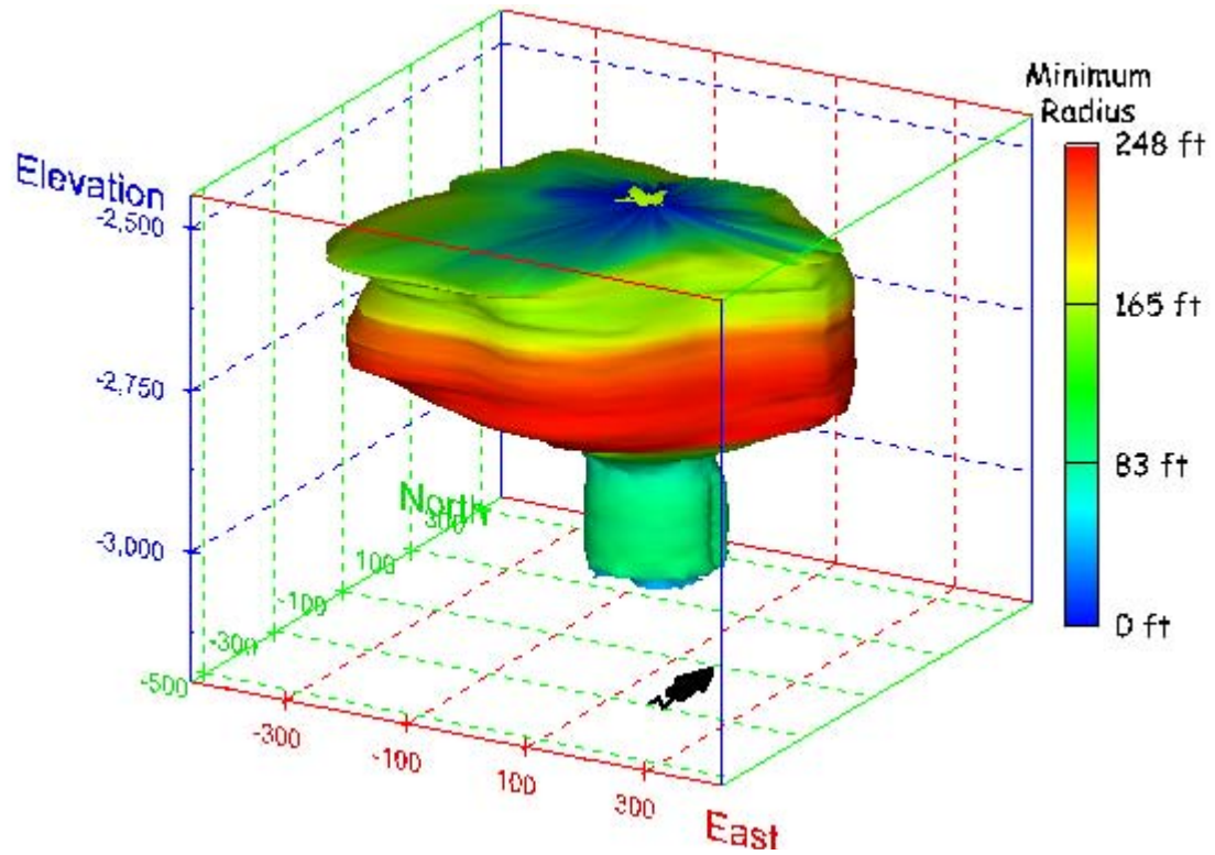
Figure 102. Sonar images of cavern BM-4, showing the geometry of the cavern colored by minimum radius. View from (a) azimuth 210°, elevation 20°; (b) azimuth 150°, elevation 20°.
