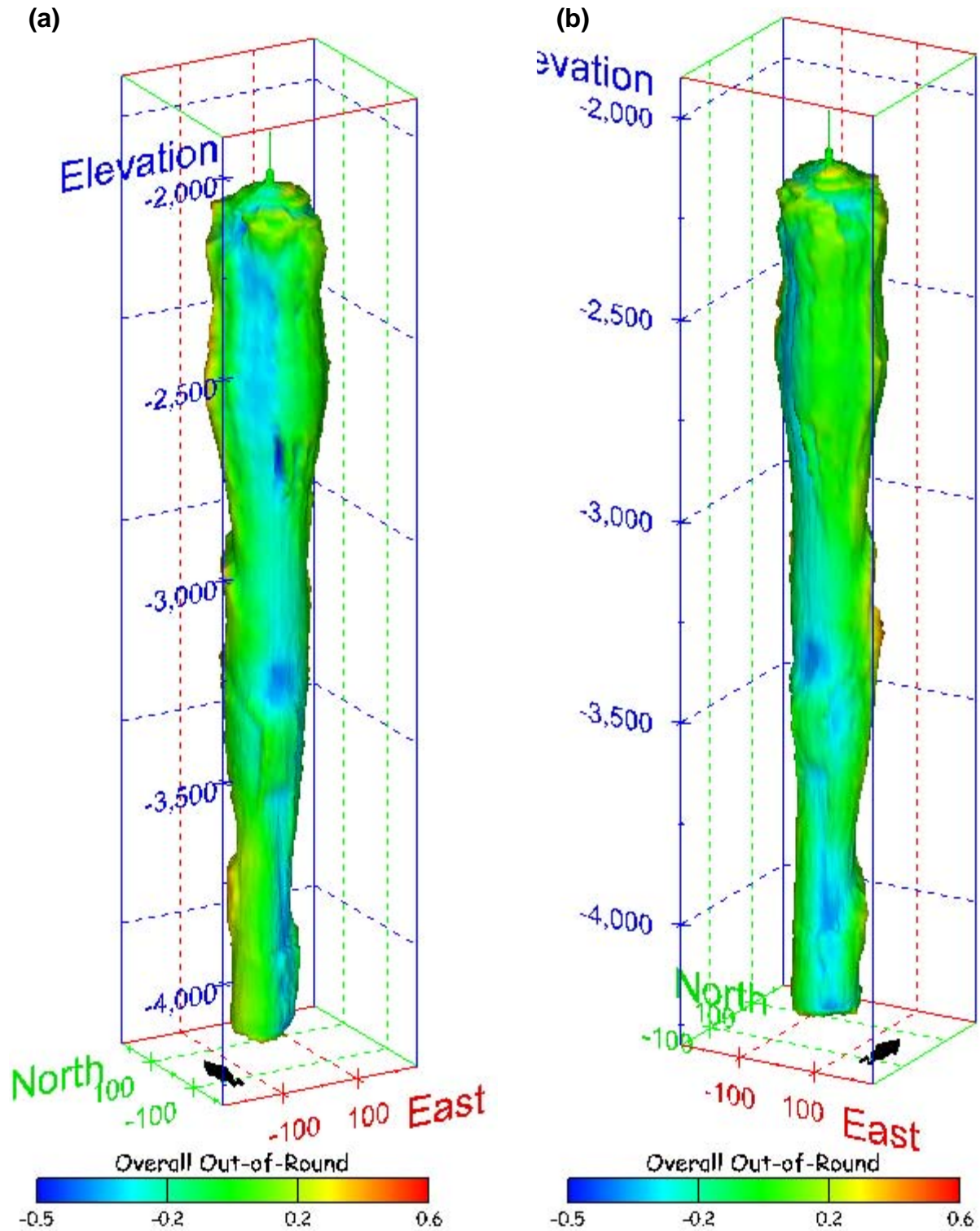
Figure 554. Sonar images of cavern BM-116, showing the geometry of the cavern colored by overall out-of-round ratio. View from (a) azimuth 210°, elevation 20°; (b) azimuth 150°, elevation 20°.
