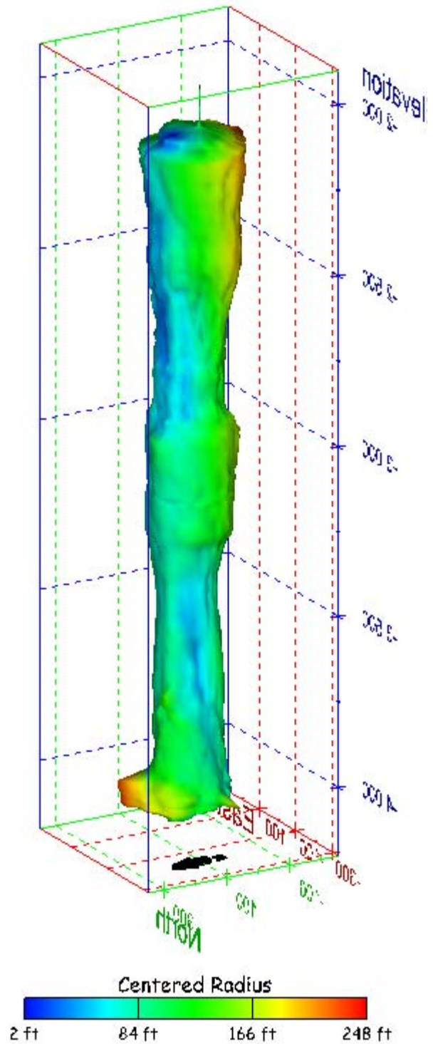
Figure 359. Sonar images of cavern BM-109, showing the geometry of the cavern colored by centered radius. View from (a) azimuth 60°, elevation 20°; (b) azimuth 300°, elevation 20°.
