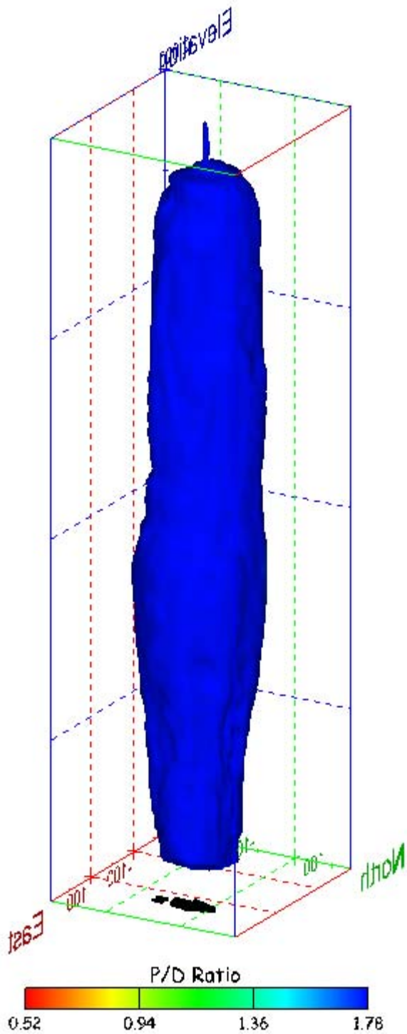
Figure 299. Sonar images of cavern BM-106, showing the geometry of the cavern colored by three-dimensional pillar-to-diameter ratio. View from (a) azimuth 60°, elevation 20°; (b) azimuth 300°, elevation 20°.
