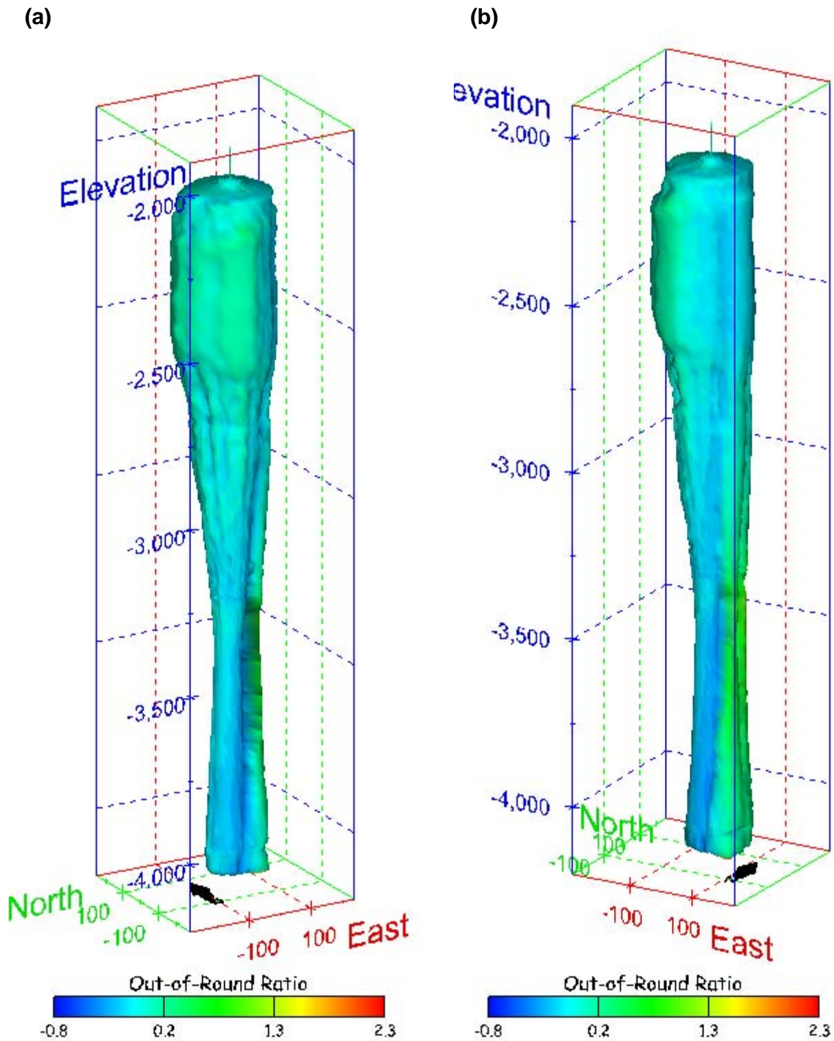
Figure 240. Sonar images of cavern BM-104, showing the geometry of the cavern colored by out-of-round ratio. View from (a) azimuth 210°, elevation 20°; (b) azimuth 150°, elevation 20°.
