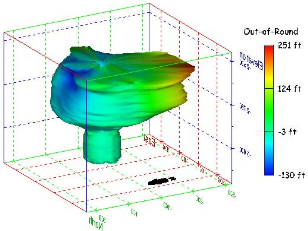
Figure 109. Sonar images of cavern BM-4, showing the geometry of the cavern colored by out-of-round distance. View from (a) azimuth 60°, elevation 20°; (b) azimuth 300°, elevation 20°.
