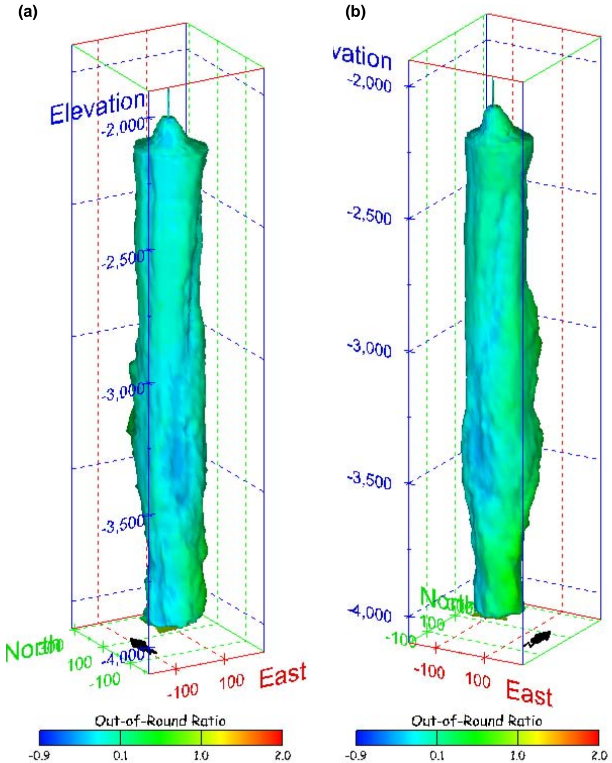
Figure 214. Sonar images of cavern BM-103, showing the geometry of the cavern colored by out-of-round ratio. View from (a) azimuth 210°, elevation 20°; (b) azimuth 150°, elevation 20°.
