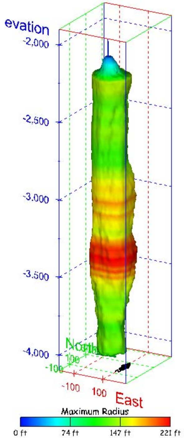
Figure 208. Sonar images of cavern BM-103, showing the geometry of the cavern colored by maximum radius. View from (a) azimuth 210°, elevation 20°; (b) azimuth 150°, elevation 20°.
