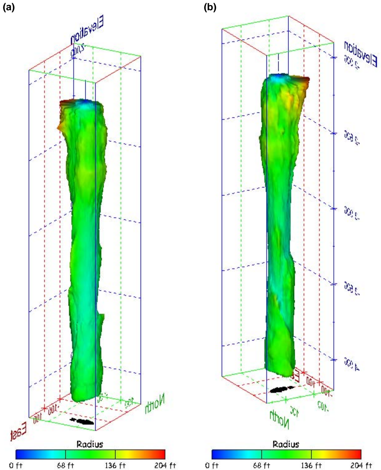
Figure 513. Sonar images of cavern BM-115, showing the geometry of the cavern colored by measured radius. View from (a) azimuth 60°, elevation 20°; (b) azimuth 300°, elevation 20°.
