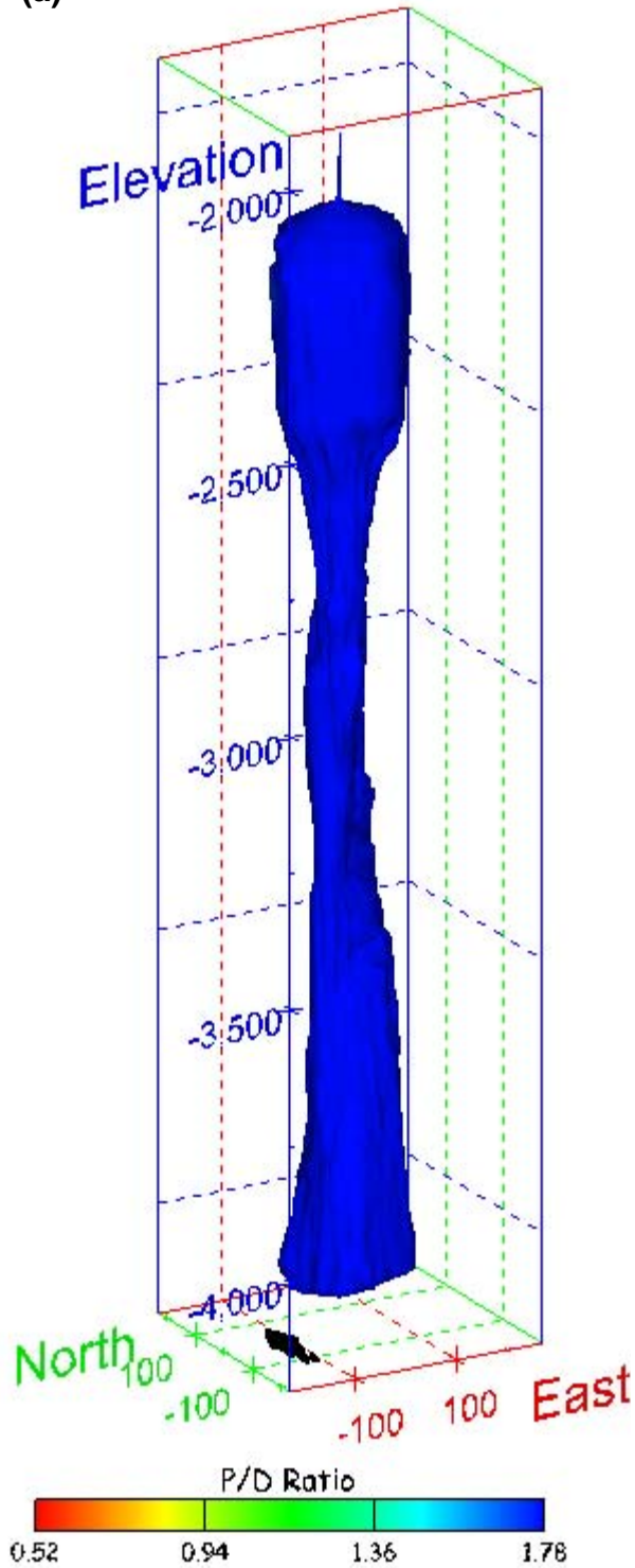
Figure 480. Sonar images of cavern BM-113, showing the geometry of the cavern colored by three-dimensional pillar-to-diameter ratio. View from (a) azimuth 210°, elevation 20°; (b) azimuth 150°, elevation 20°.
