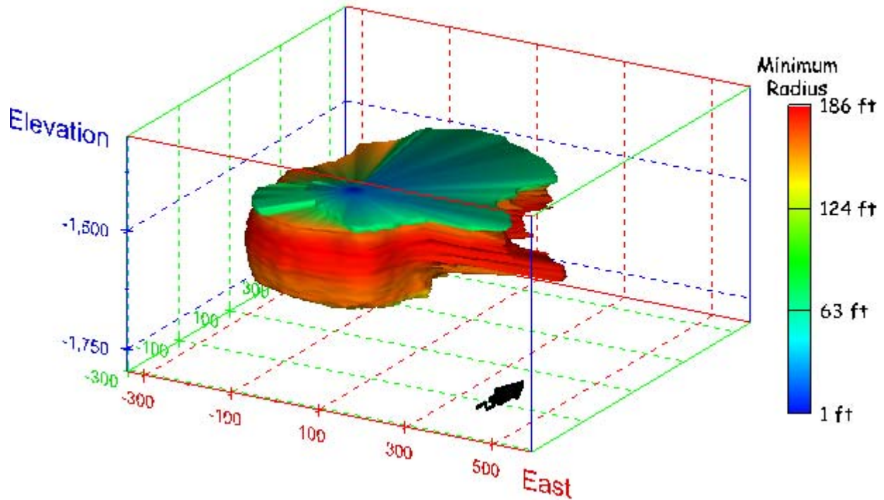
Figure 50. Sonar images of cavern BM-2, showing the geometry of the cavern colored by minimum radius. View from (a) azimuth 210°, elevation 20°; (b) azimuth 150°, elevation 20°.
