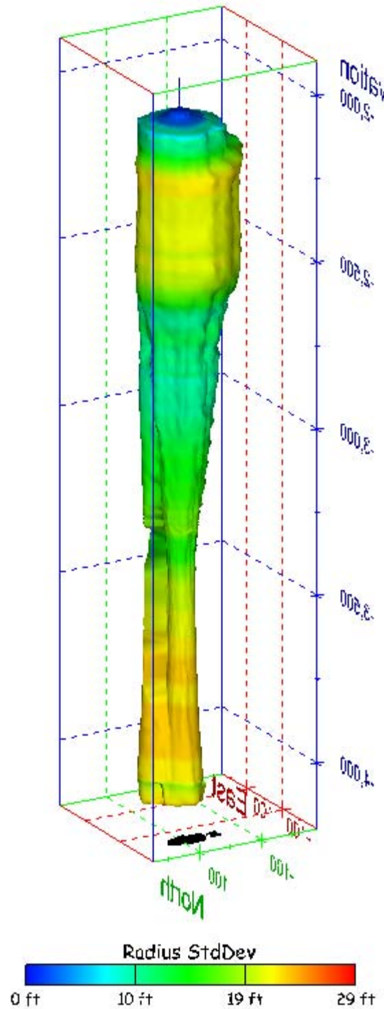
Figure 237. Sonar images of cavern BM-104, showing the geometry of the cavern colored by radius standard deviation. View from (a) azimuth 60°, elevation 20°; (b) azimuth 300°, elevation 20°.
