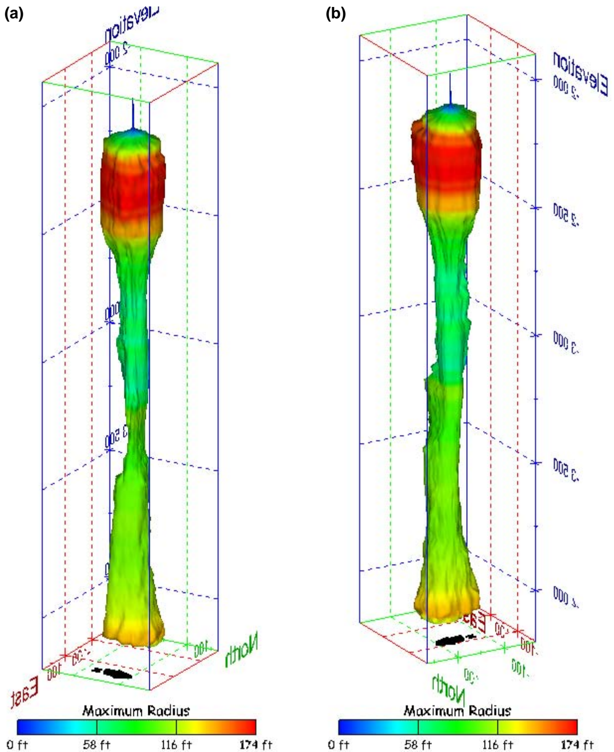
Figure 469. Sonar images of cavern BM-113, showing the geometry of the cavern colored by maximum radius. View from (a) azimuth 60°, elevation 20°; (b) azimuth 300°, elevation 20°.
