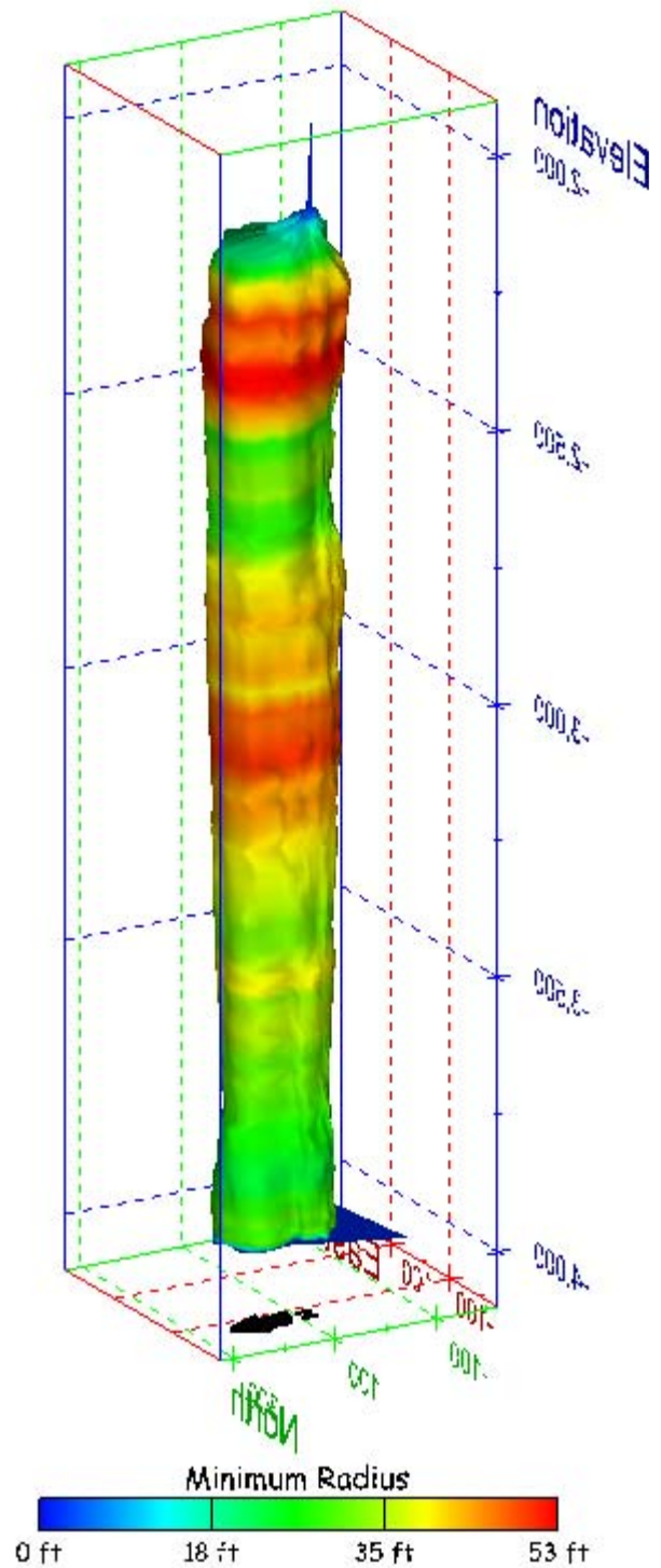
Figure 441. Sonar images of cavern BM-112, showing the geometry of the cavern colored by minimum radius. View from (a) azimuth 60°, elevation 20°; (b) azimuth 300°, elevation 20°.
