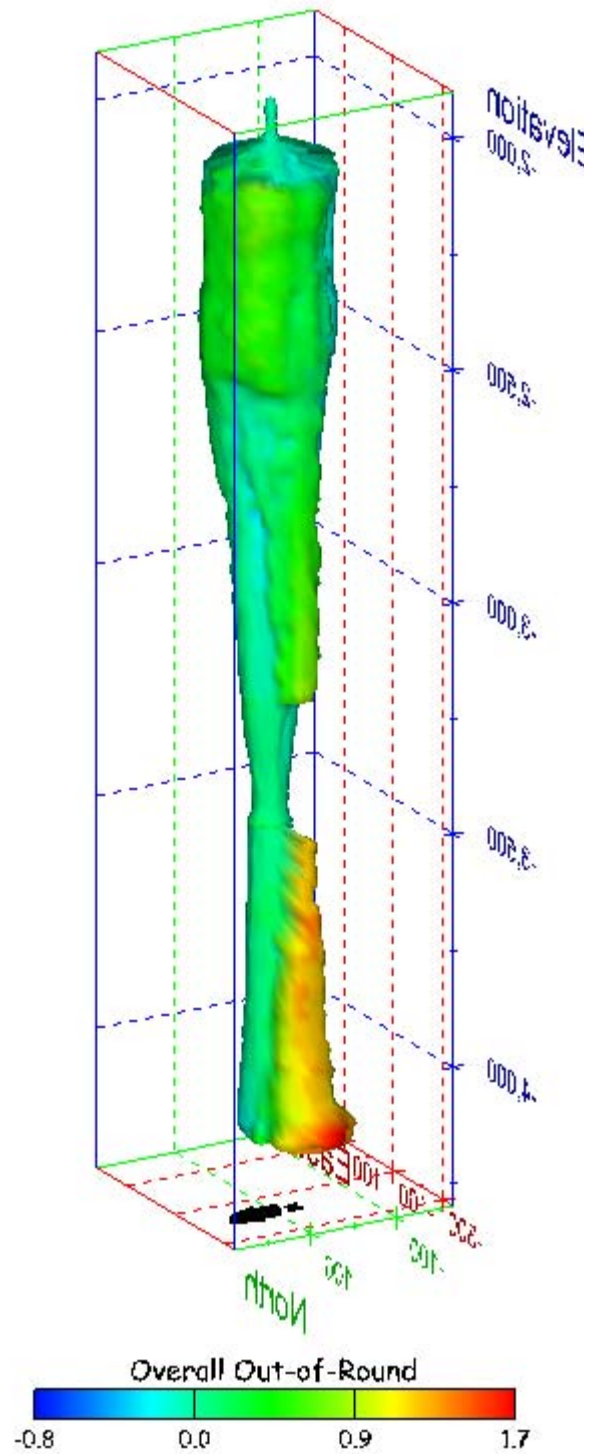
Figure 269. Sonar images of cavern BM-105, showing the geometry of the cavern colored by overall out-of-round ratio. View from (a) azimuth 60°, elevation 20°; (b) azimuth 300°, elevation 20°.
