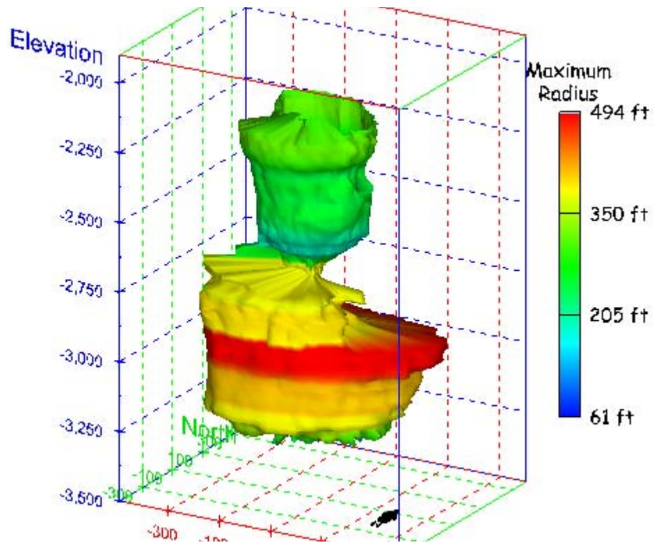
Figure 130. Sonar images of cavern BM-5, showing the geometry of the cavern colored by maximum radius. View from (a) azimuth 210°, elevation 20°; (b) azimuth 150°, elevation 20°.
