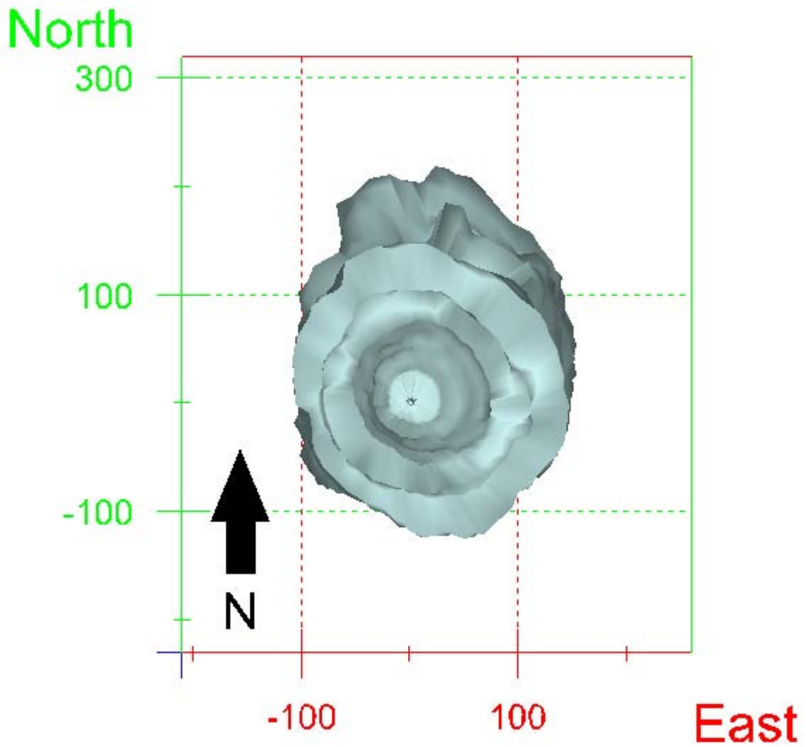
Figure 197. Map view sonar image of cavern BM-103, showing the basic geometry of the cavern. Grid squares represent 200 ft.
