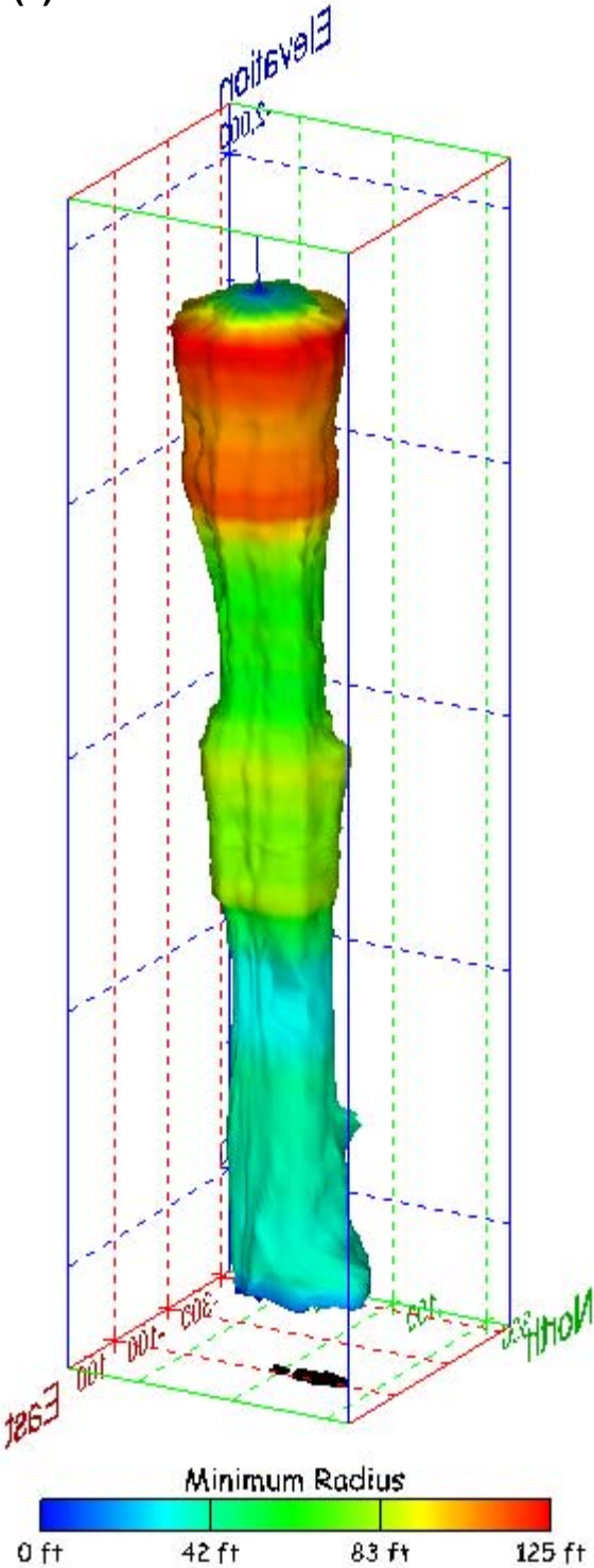
Figure 363. Sonar images of cavern BM-109, showing the geometry of the cavern colored by minimum radius. View from (a) azimuth 60°, elevation 20°; (b) azimuth 300°, elevation 20°.
