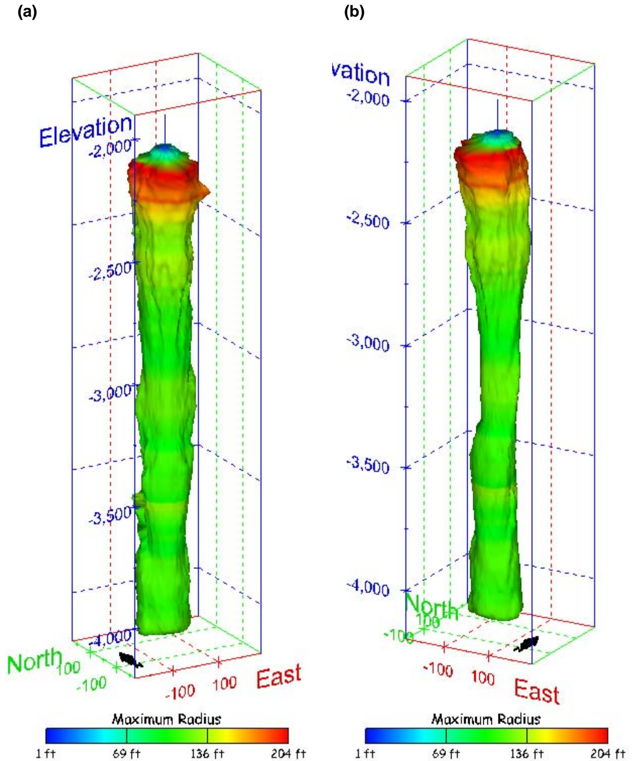
Figure 520. Sonar images of cavern BM-115, showing the geometry of the cavern colored by maximum radius. View from (a) azimuth 210°, elevation 20°; (b) azimuth 150°, elevation 20°.
