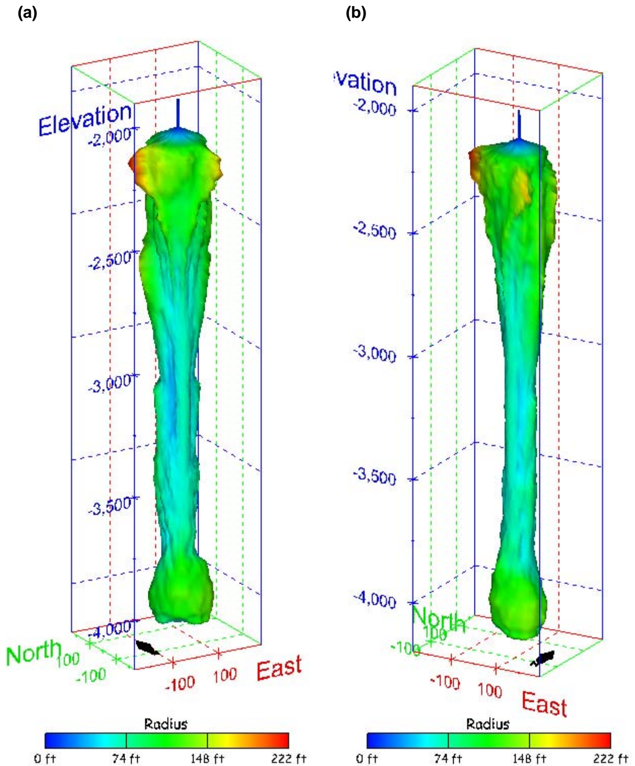
Figure 486. Sonar images of cavern BM-114, showing the geometry of the cavern colored by measured radius. View from (a) azimuth 210°, elevation 20°; (b) azimuth 150°, elevation 20°.
