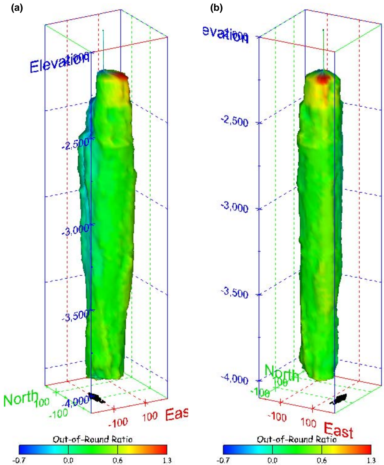
Figure 318. Sonar images of cavern BM-107, showing the geometry of the cavern colored by out-of-round ratio. View from (a) azimuth 210°, elevation 20°; (b) azimuth 150°, elevation 20°.
