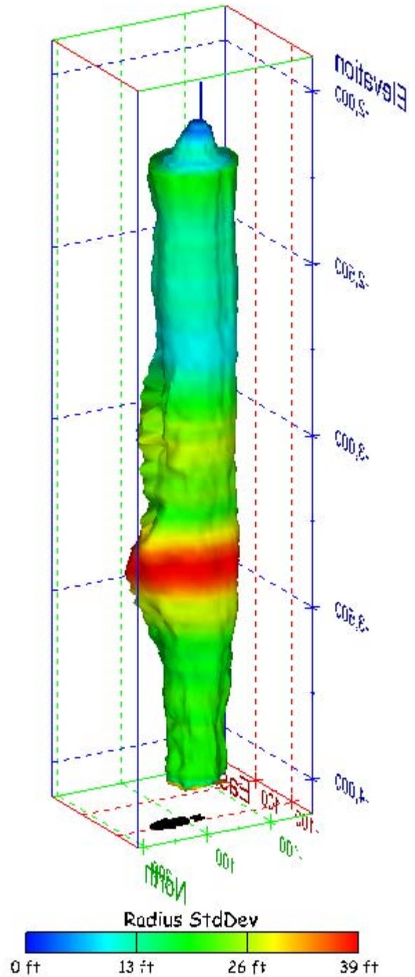
Figure 211. Sonar images of cavern BM-103, showing the geometry of the cavern colored by radius standard deviation. View from (a) azimuth 60°, elevation 20°; (b) azimuth 300°, elevation 20°.
