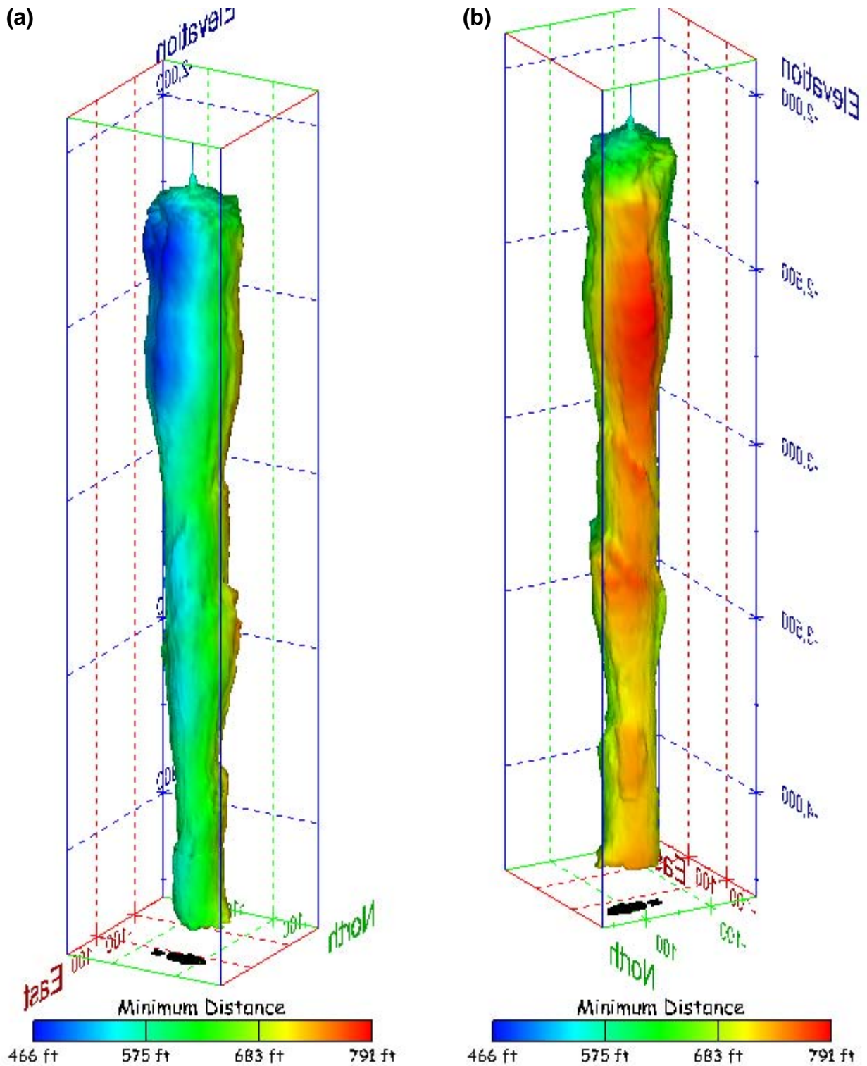
Figure 557. Sonar images of cavern BM-116, showing the geometry of the cavern colored by minimum distance to the nearest neighboring cavern. View from (a) azimuth 60°, elevation 20°; (b) azimuth 300°, elevation 20°.
