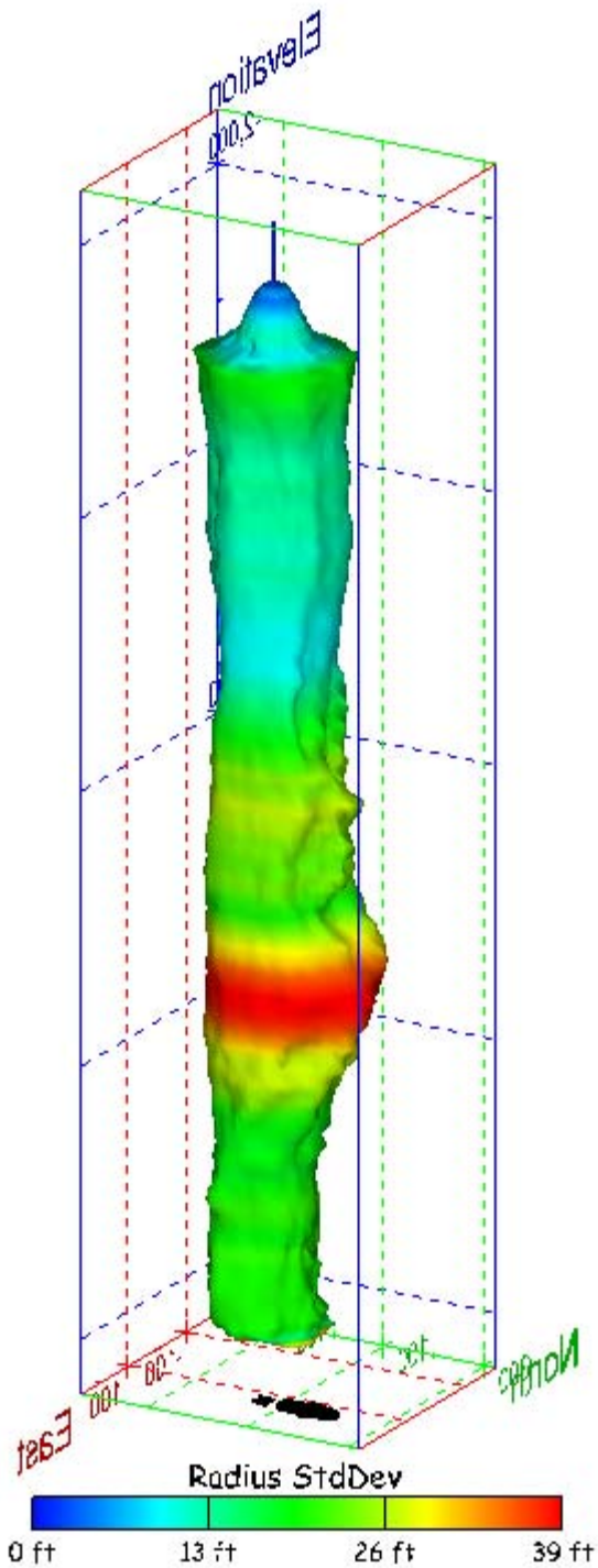
Figure 211. Sonar images of cavern BM-103, showing the geometry of the cavern colored by radius standard deviation. View from (a) azimuth 60°, elevation 20°; (b) azimuth 300°, elevation 20°.
