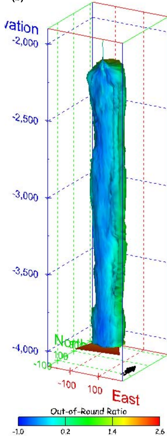
Figure 448. Sonar images of cavern BM-112, showing the geometry of the cavern colored by out-of-round ratio. View from (a) azimuth 210°, elevation 20°; (b) azimuth 150°, elevation 20°.
