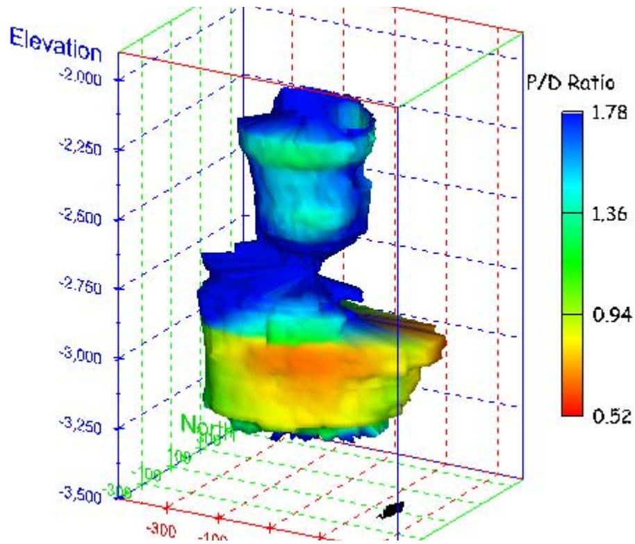
Figure 142. Sonar images of cavern BM-5, showing the geometry of the cavern colored by three-dimensional pillar-to-diameter ratio. View from (a) azimuth 210°, elevation 20°; (b) azimuth 150°, elevation 20°.
