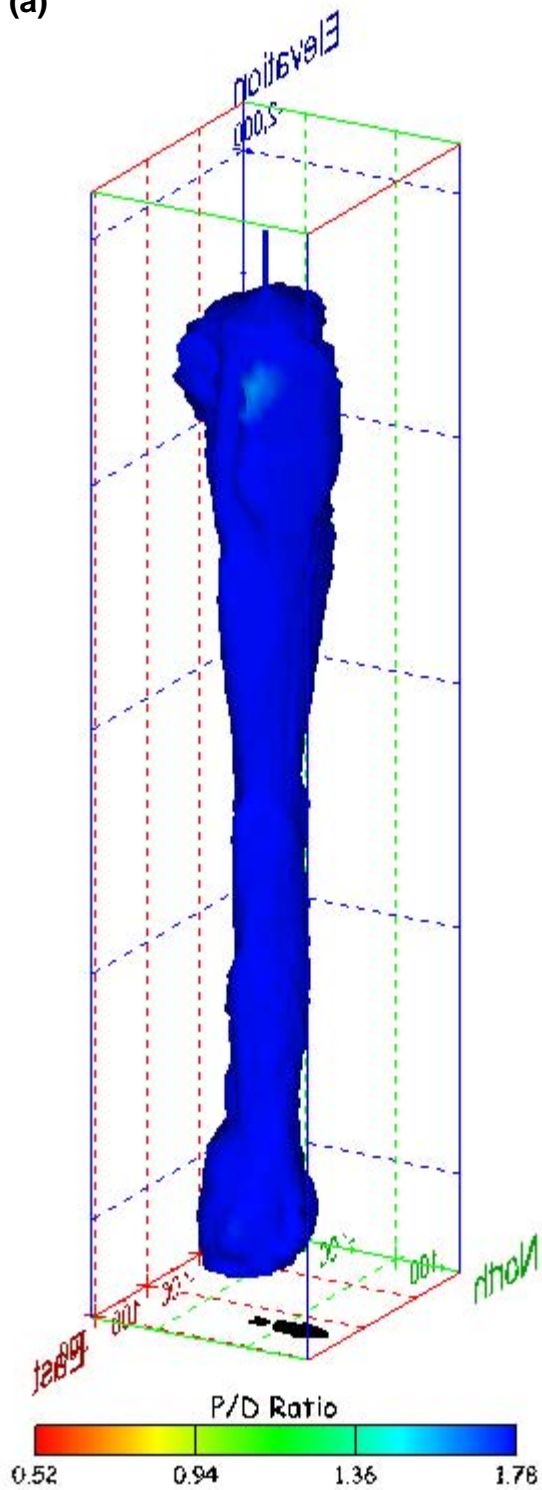
Figure 507. Sonar images of cavern BM-114, showing the geometry of the cavern colored by three-dimensional pillar-to-diameter ratio. View from (a) azimuth 60°, elevation 20°; (b) azimuth 300°, elevation 20°.
