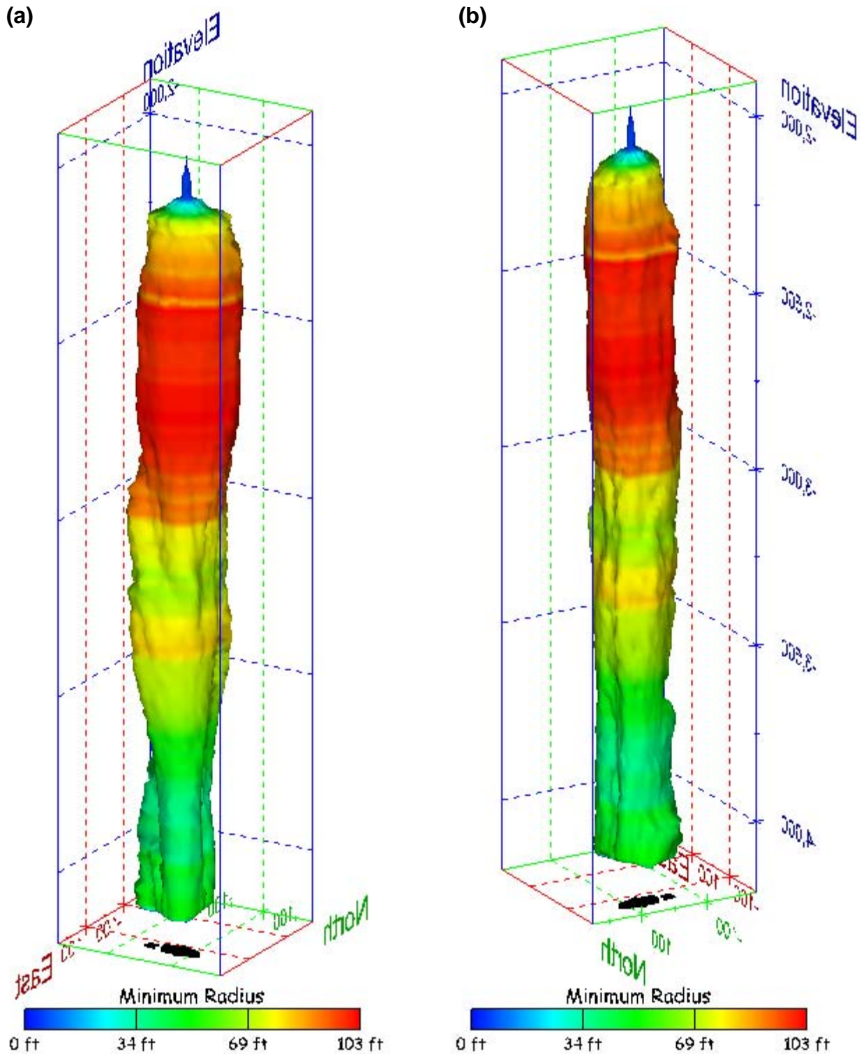
Figure 415. Sonar images of cavern BM-111, showing the geometry of the cavern colored by minimum radius. View from (a) azimuth 60°, elevation 20°; (b) azimuth 300°, elevation 20°.
