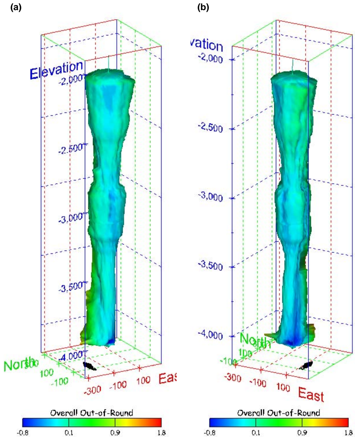
Figure 372. Sonar images of cavern BM-109, showing the geometry of the cavern colored by overall out-of-round ratio. View from (a) azimuth 210°, elevation 20°; (b) azimuth 150°, elevation 20°.
