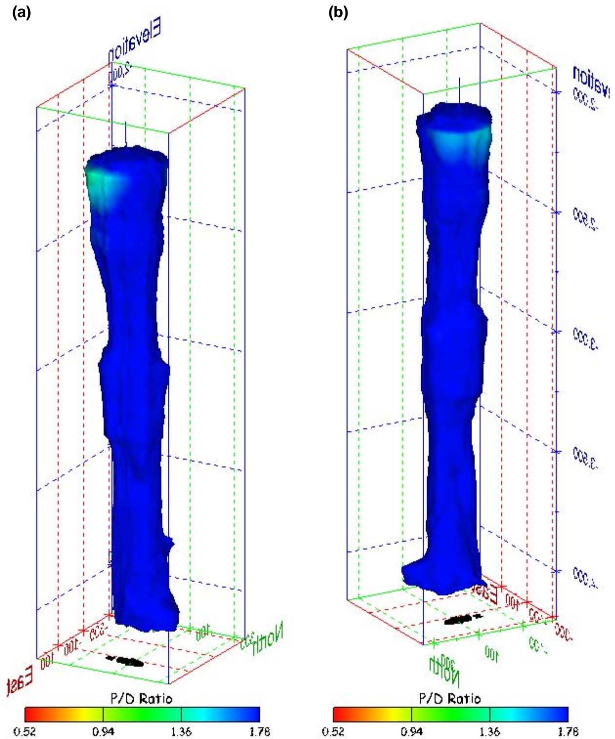
Figure 377. Sonar images of cavern BM-109, showing the geometry of the cavern colored by three-dimensional pillar-to-diameter ratio. View from (a) azimuth 60°, elevation 20°; (b) azimuth 300°, elevation 20°.
