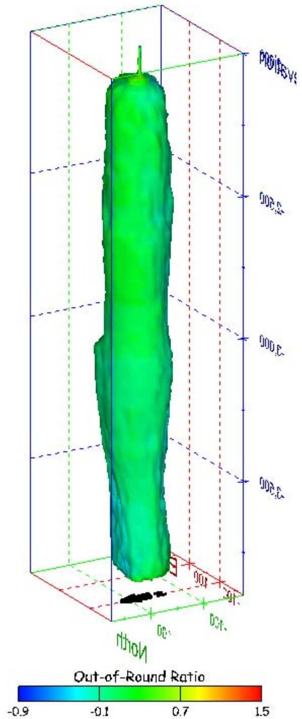
Figure 293. Sonar images of cavern BM-106, showing the geometry of the cavern colored by out-of-round ratio. View from (a) azimuth 60°, elevation 20°; (b) azimuth 300°, elevation 20°.
