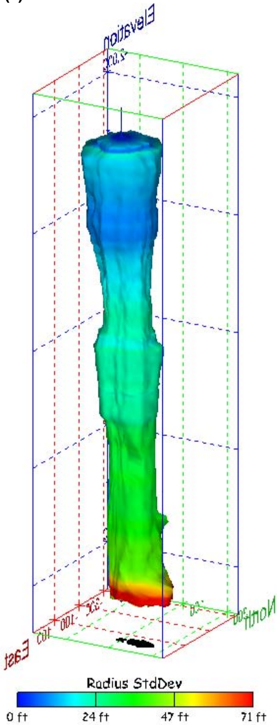
Figure 367. Sonar images of cavern BM-109, showing the geometry of the cavern colored by radius standard deviation. View from (a) azimuth 60°, elevation 20°; (b) azimuth 300°, elevation 20°.
