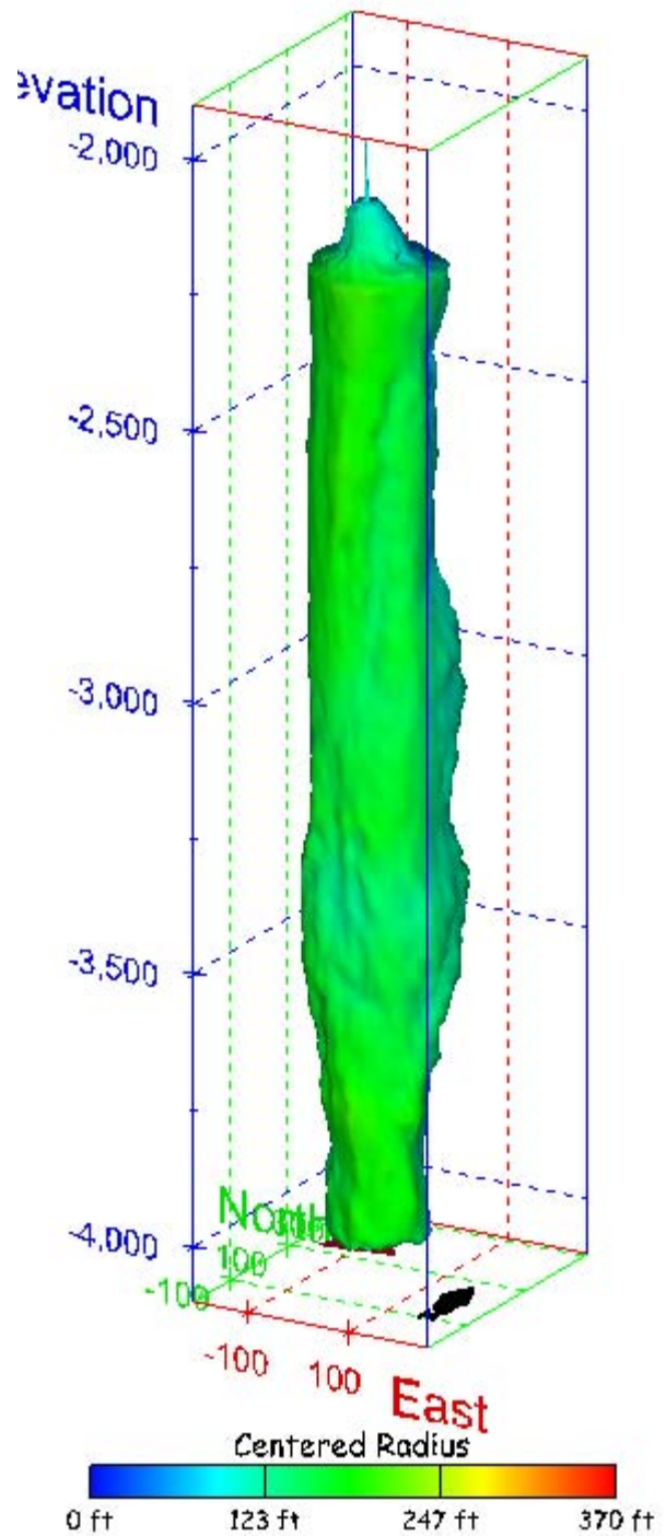
Figure 202. Sonar images of cavern BM-103, showing the geometry of the cavern colored by centered radius. View from (a) azimuth 210°, elevation 20°; (b) azimuth 150°, elevation 20°.
