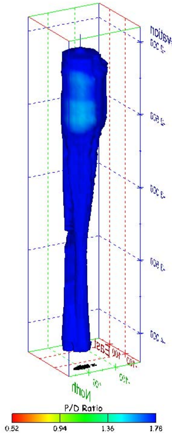
Figure 247. Sonar images of cavern BM-104, showing the geometry of the cavern colored by three-dimensional pillar-to-diameter ratio. View from (a) azimuth 60°, elevation 20°; (b) azimuth 300°, elevation 20°.
