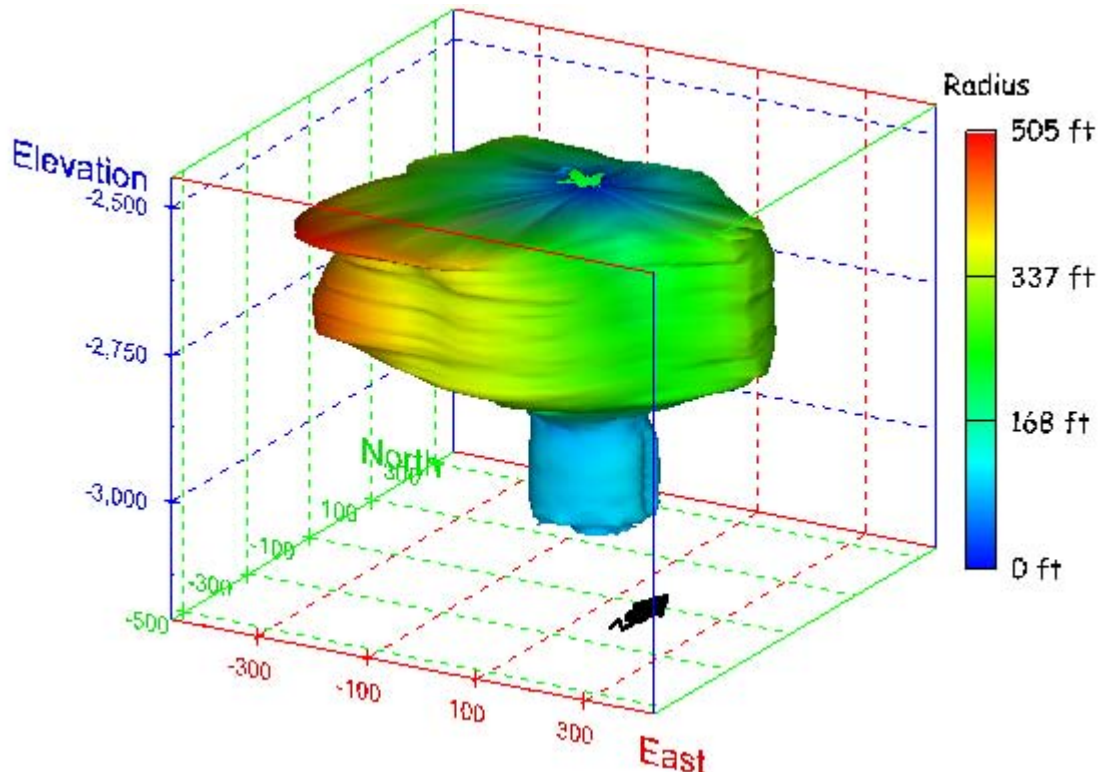
Figure 96. Sonar images of cavern BM-4, showing the geometry of the cavern colored by measured radius. View from (a) azimuth 210°, elevation 20°; (b) azimuth 150°, elevation 20°.
