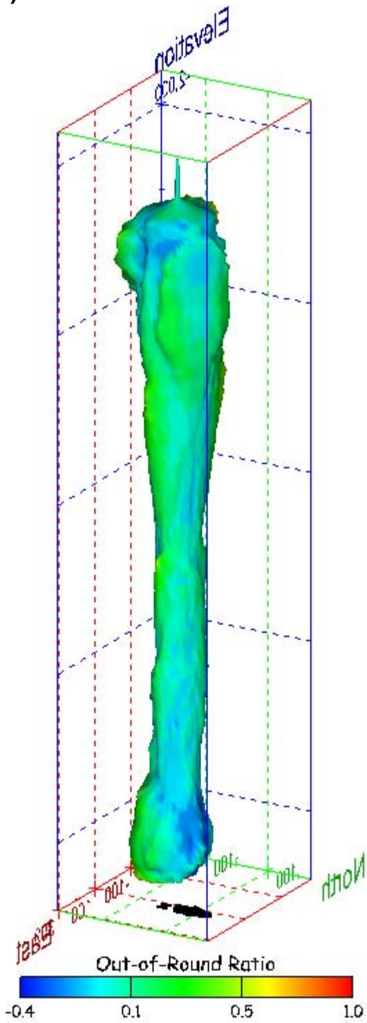
Figure 501. Sonar images of cavern BM-114, showing the geometry of the cavern colored by out-of-round ratio. View from (a) azimuth 60°, elevation 20°; (b) azimuth 300°, elevation 20°.
