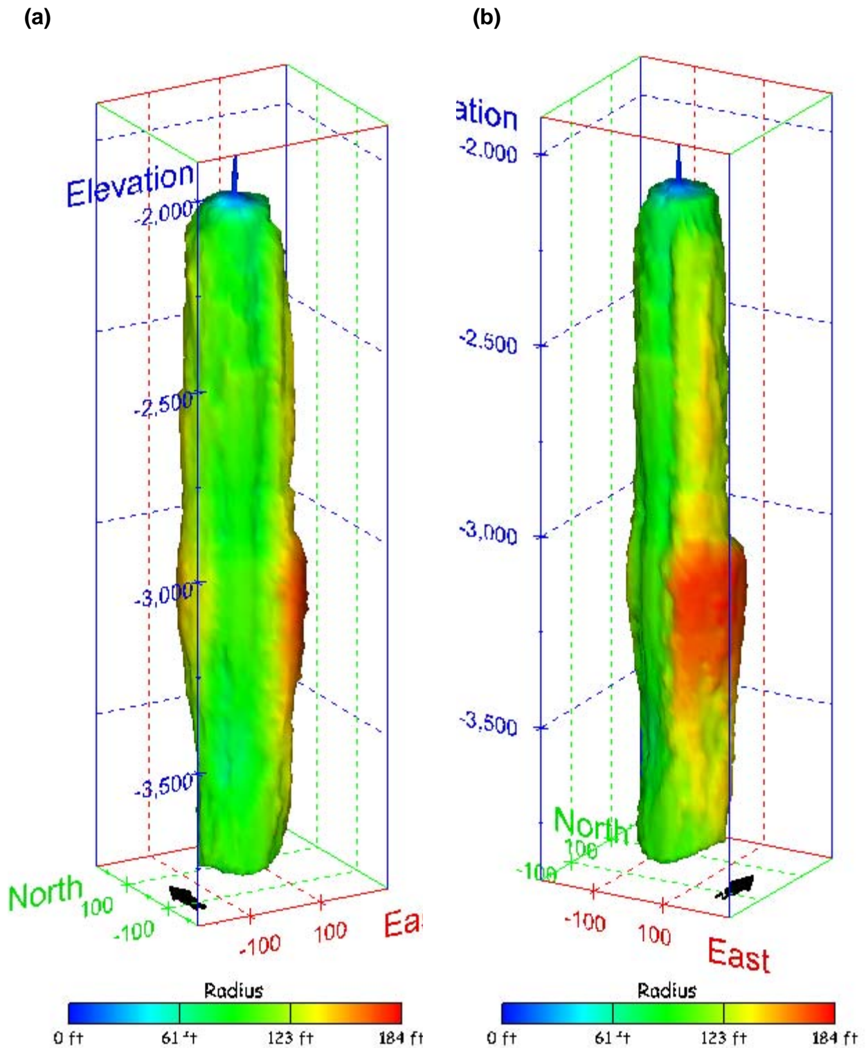
Figure 278. Sonar images of cavern BM-106, showing the geometry of the cavern colored by measured radius. View from (a) azimuth 210°, elevation 20°; (b) azimuth 150°, elevation 20°.
