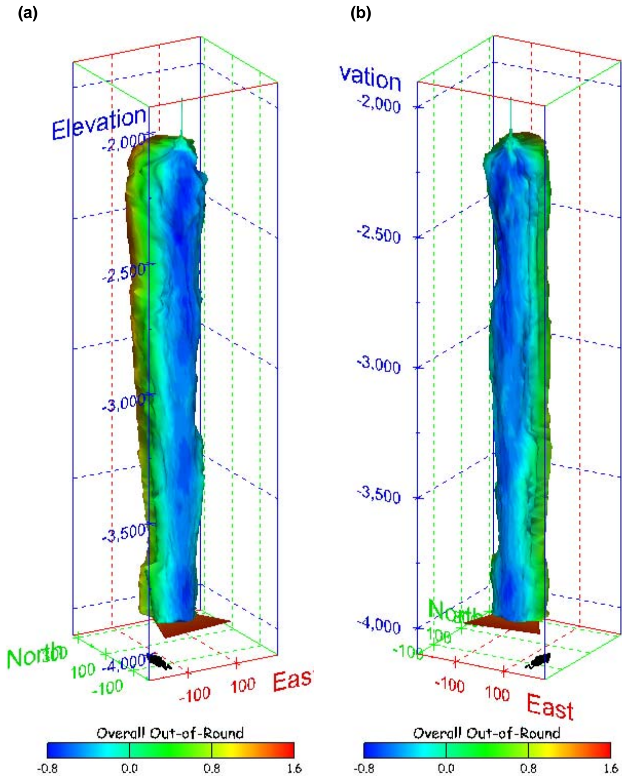
Figure 450. Sonar images of cavern BM-112, showing the geometry of the cavern colored by overall out-of-round ratio. View from (a) azimuth 210°, elevation 20°; (b) azimuth 150°, elevation 20°.
