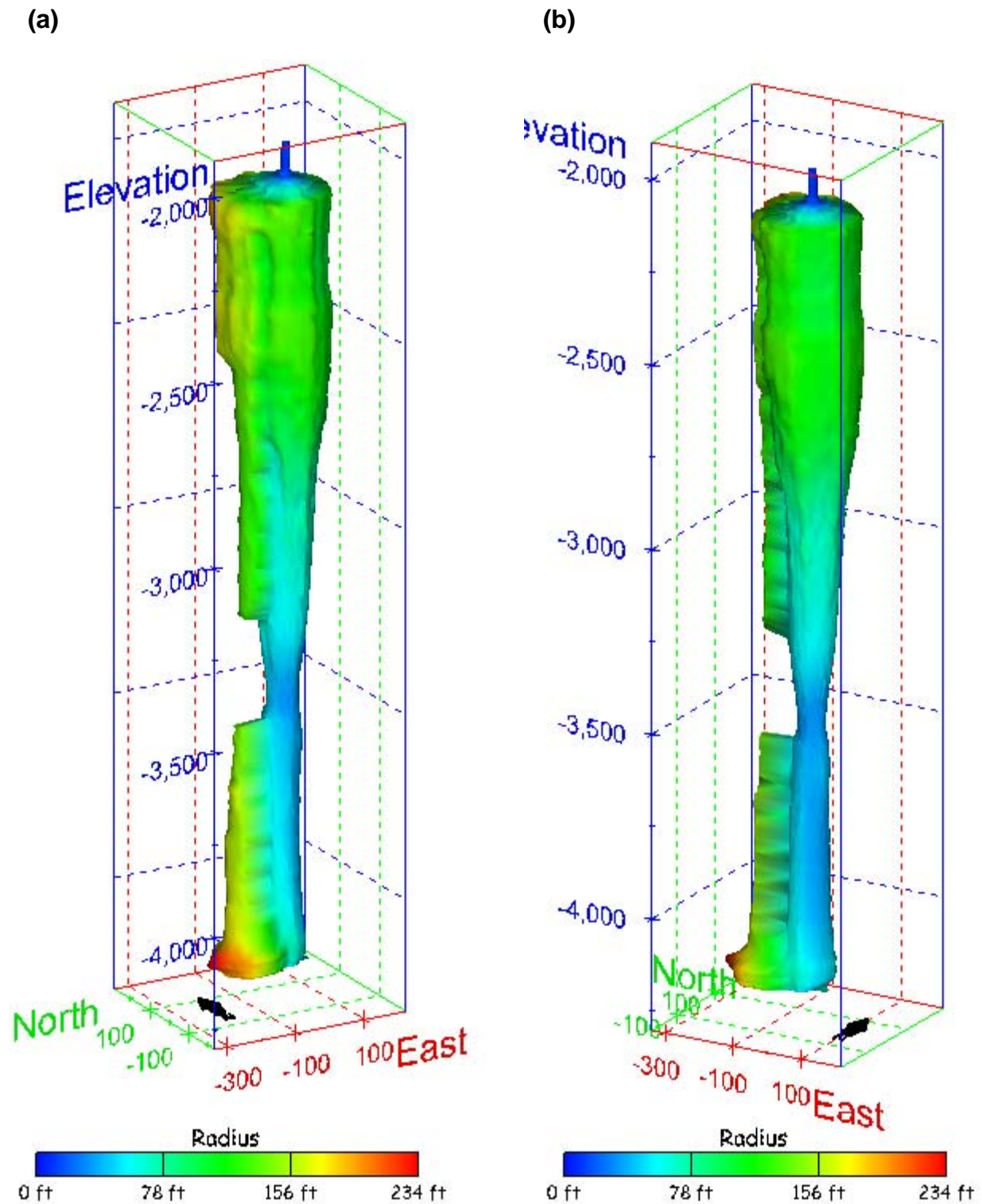
Figure 252. Sonar images of cavern BM-105, showing the geometry of the cavern colored by measured radius. View from (a) azimuth 210°, elevation 20°; (b) azimuth 150°, elevation 20°.
