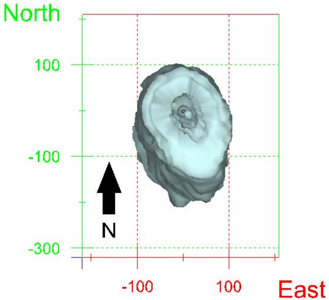
Figure 171. Map view sonar image of cavern BM-102, showing the basic geometry of the cavern. Grid squares represent 200 ft.
