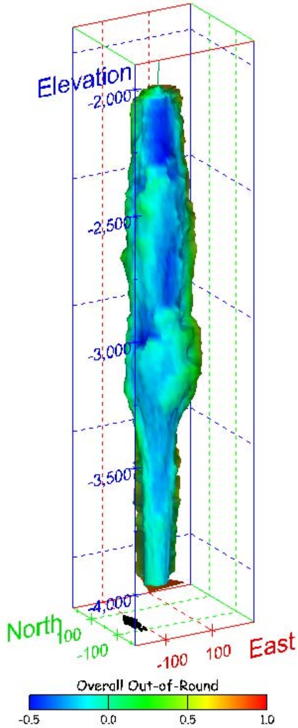
Figure 398. Sonar images of cavern BM-110, showing the geometry of the cavern colored by overall out-of-round ratio. View from (a) azimuth 210°, elevation 20°; (b) azimuth 150°, elevation 20°.
