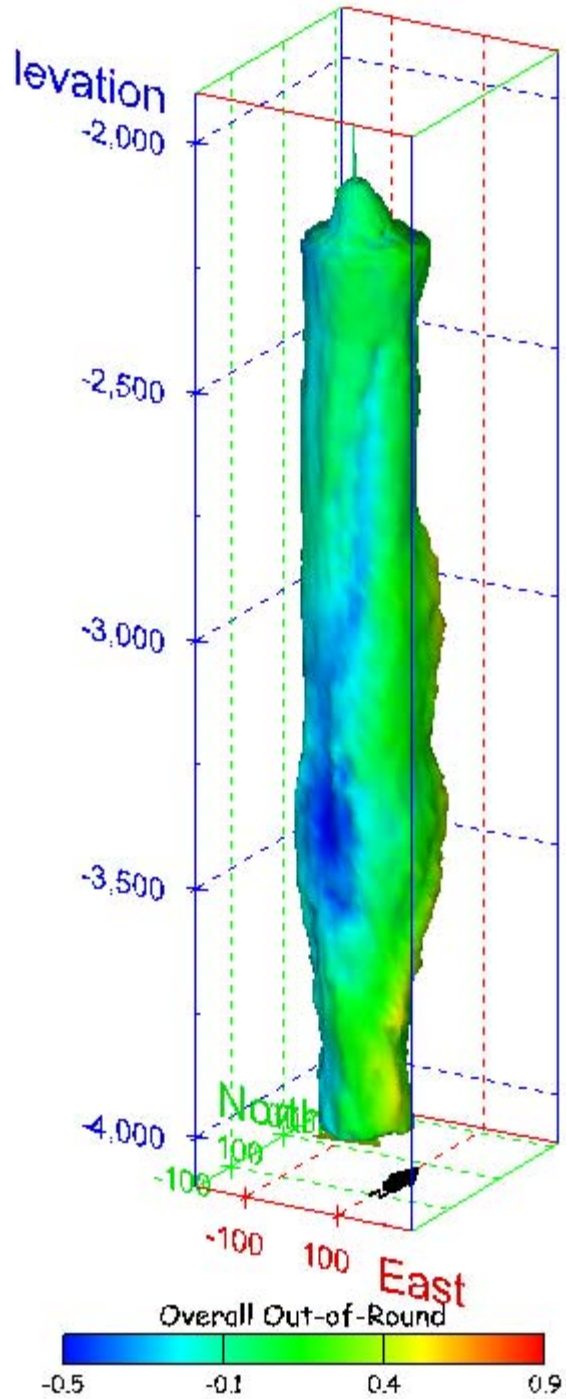
Figure 216. Sonar images of cavern BM-103, showing the geometry of the cavern colored by overall out-of-round ratio. View from (a) azimuth 210°, elevation 20°; (b) azimuth 150°, elevation 20°.
