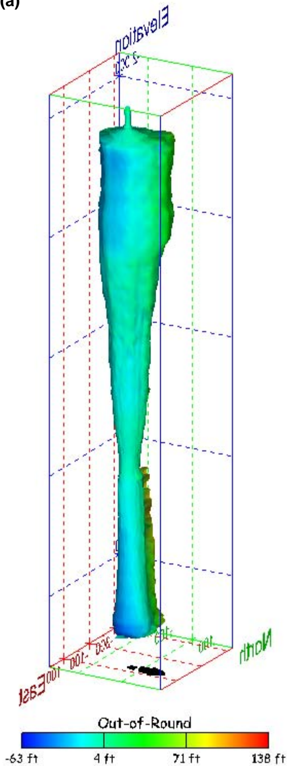
Figure 265. Sonar images of cavern BM-105, showing the geometry of the cavern colored by out-of-round distance. View from (a) azimuth 60°, elevation 20°; (b) azimuth 300°, elevation 20°.
