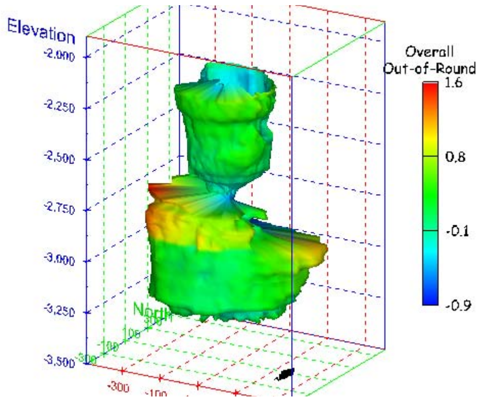
Figure 138. Sonar images of cavern BM-5, showing the geometry of the cavern colored by overall out-of-round ratio. View from (a) azimuth 210°, elevation 20°; (b) azimuth 150°, elevation 20°.
