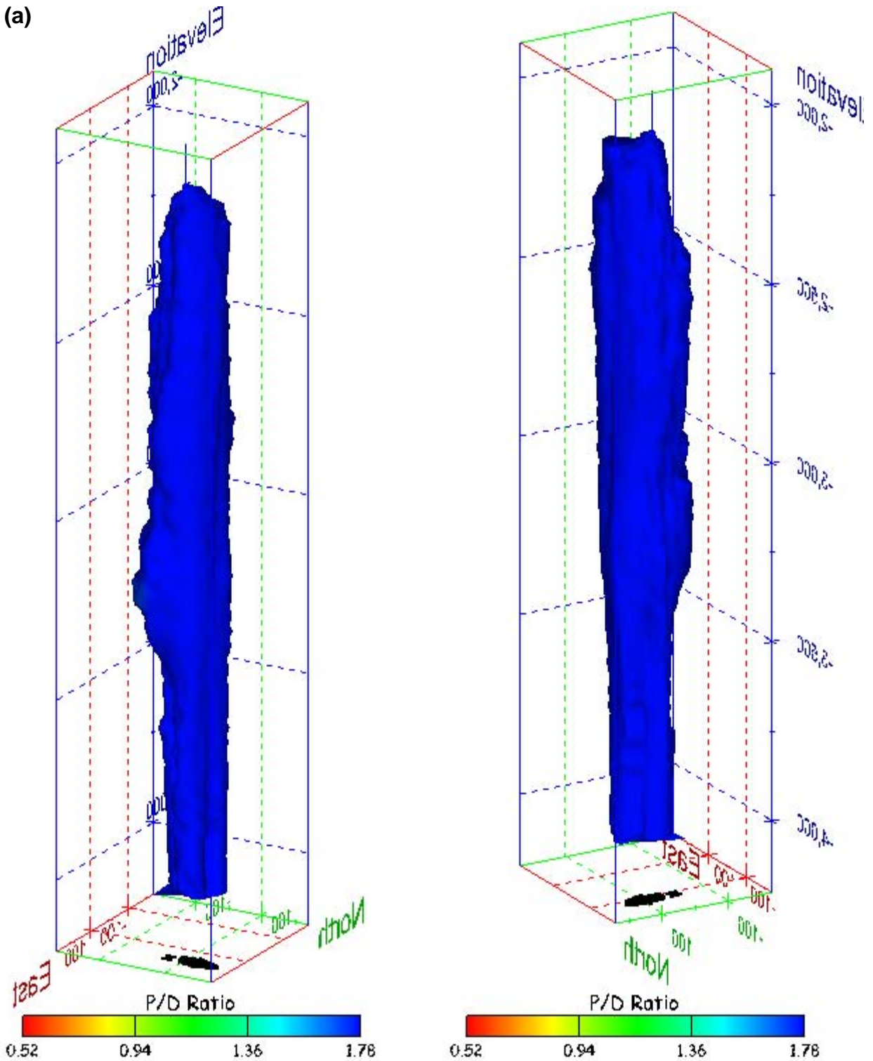
Figure 403. Sonar images of cavern BM-110, showing the geometry of the cavern colored by three-dimensional pillar-to-diameter ratio. View from (a) azimuth 60°, elevation 20°; (b) azimuth 300°, elevation 20°.
