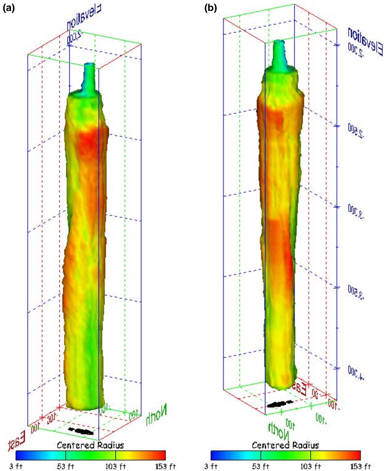
Figure 151. Sonar images of cavern BM-101, showing the geometry of the cavern colored by centered radius. View from (a) azimuth 60°, elevation 20°; (b) azimuth 300°, elevation 20°.
