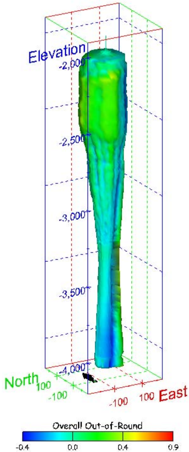
Figure 242. Sonar images of cavern BM-104, showing the geometry of the cavern colored by overall out-of-round ratio. View from (a) azimuth 210°, elevation 20°; (b) azimuth 150°, elevation 20°.
