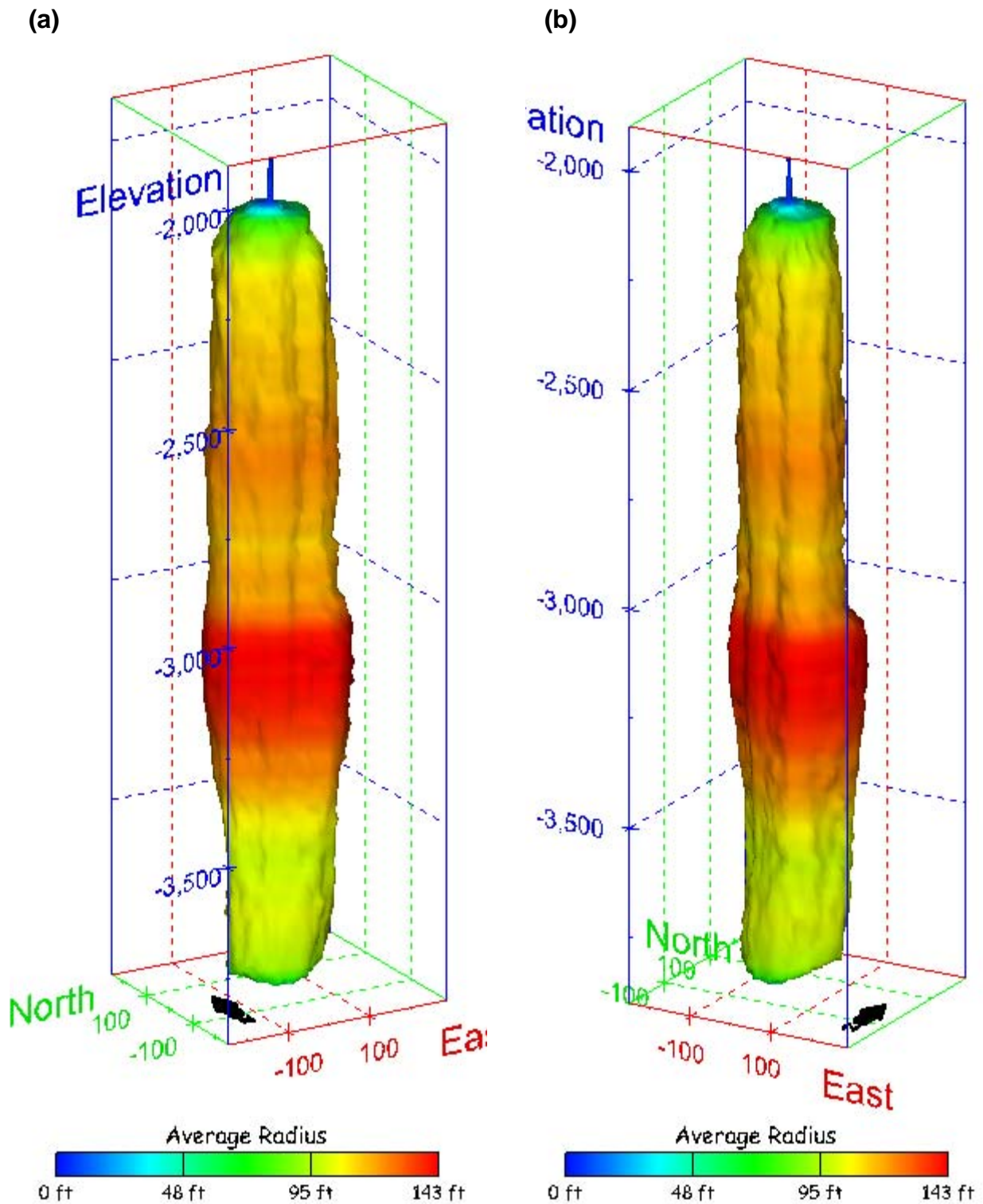
Figure 282. Sonar images of cavern BM-106, showing the geometry of the cavern colored by average radius. View from (a) azimuth 210°, elevation 20°; (b) azimuth 150°, elevation 20°.
