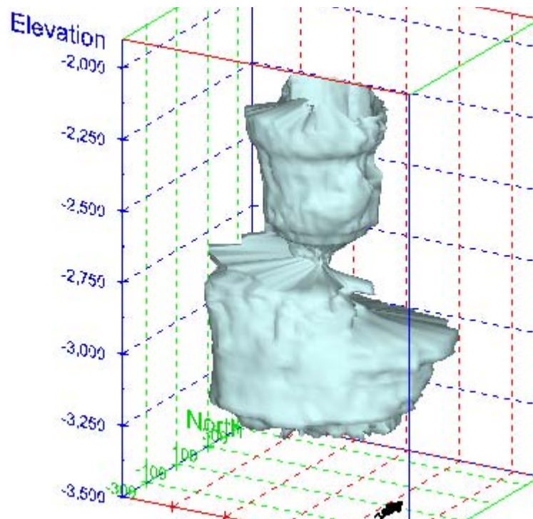
Figure 120. Sonar images of cavern BM-5, showing the basic geometric shape of the cavern. View from (a) azimuth 210°, elevation 20°; (b) azimuth 150°, elevation 20°.
