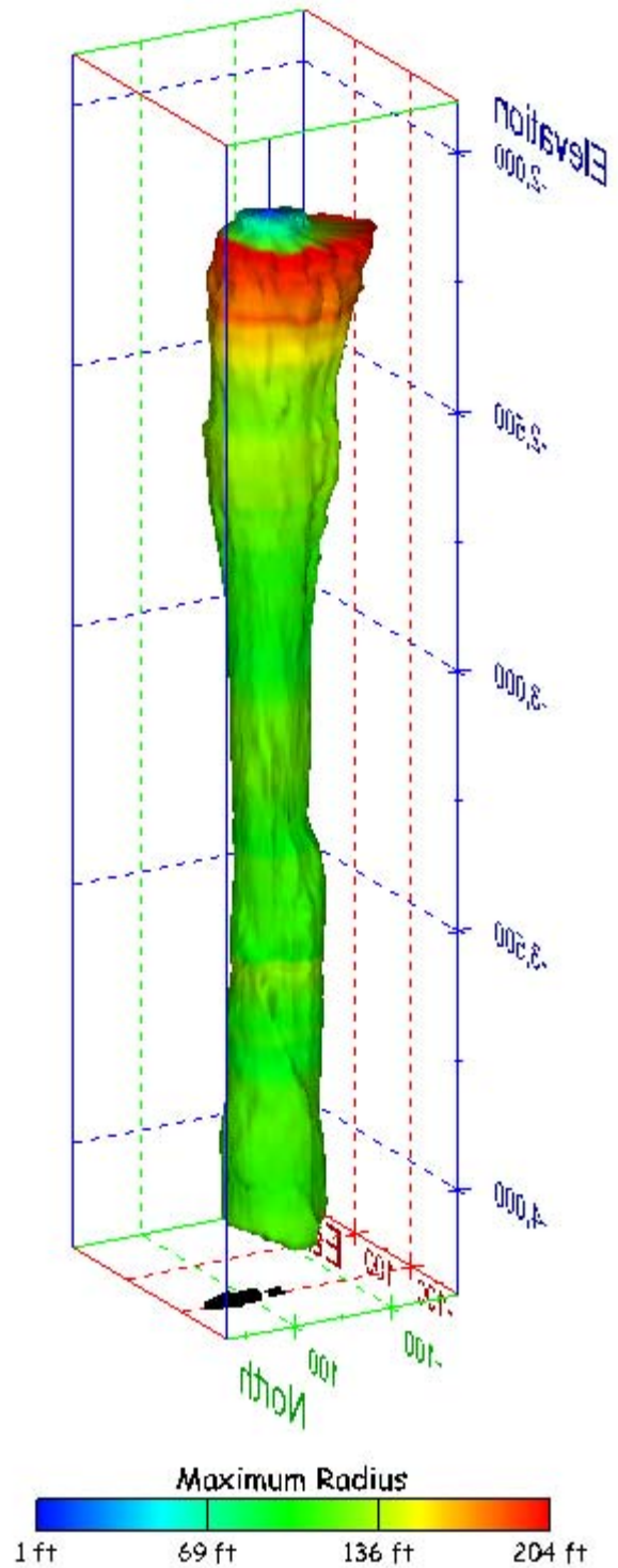
Figure 521. Sonar images of cavern BM-115, showing the geometry of the cavern colored by maximum radius. View from (a) azimuth 60°, elevation 20°; (b) azimuth 300°, elevation 20°.
