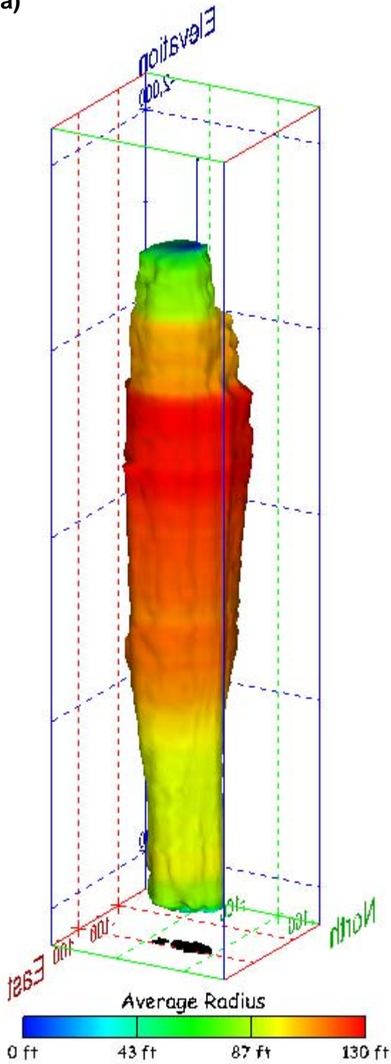
Figure 309. Sonar images of cavern BM-107, showing the geometry of the cavern colored by average radius. View from (a) azimuth 60°, elevation 20°; (b) azimuth 300°, elevation 20°.
