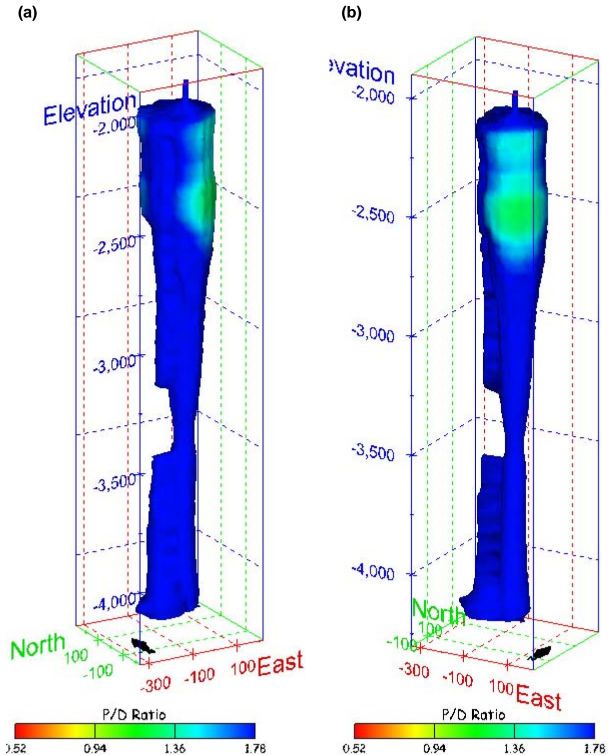
Figure 272. Sonar images of cavern BM-105, showing the geometry of the cavern colored by three-dimensional pillar-to-diameter ratio. View from (a) azimuth 210°, elevation 20°; (b) azimuth 150°, elevation 20°.
