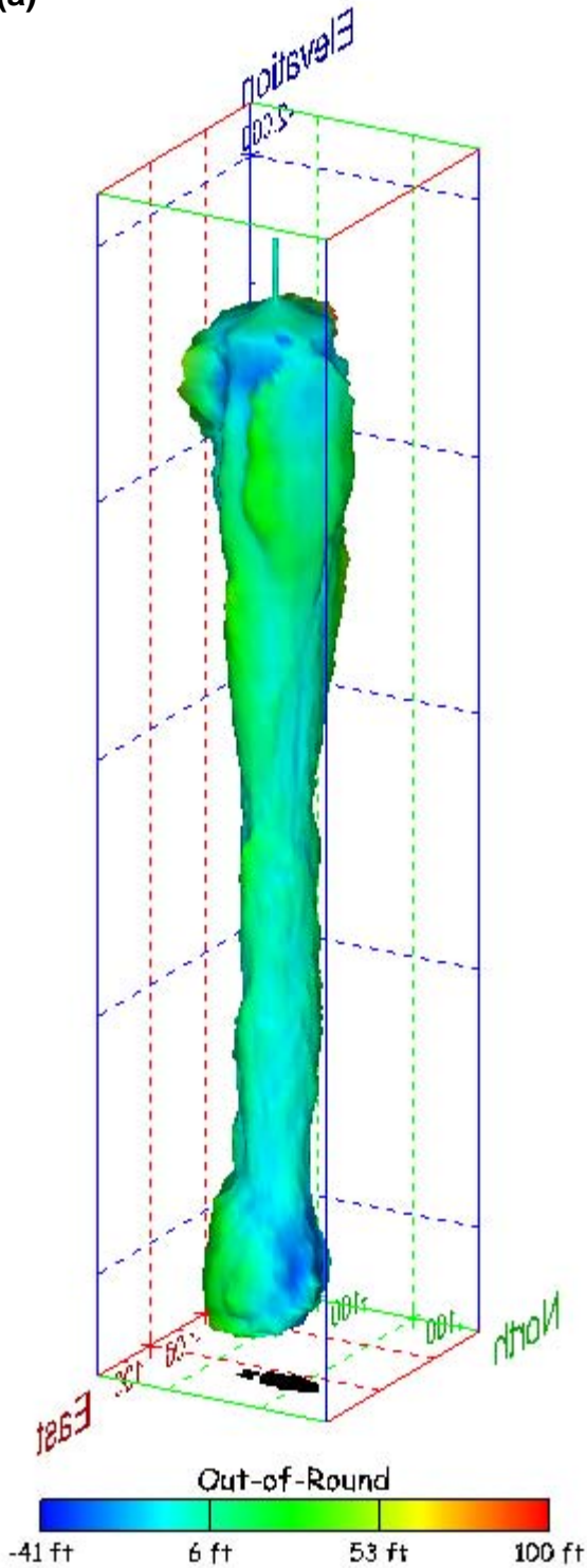
Figure 499. Sonar images of cavern BM-114, showing the geometry of the cavern colored by out-of-round distance. View from (a) azimuth 60°, elevation 20°; (b) azimuth 300°, elevation 20°.
