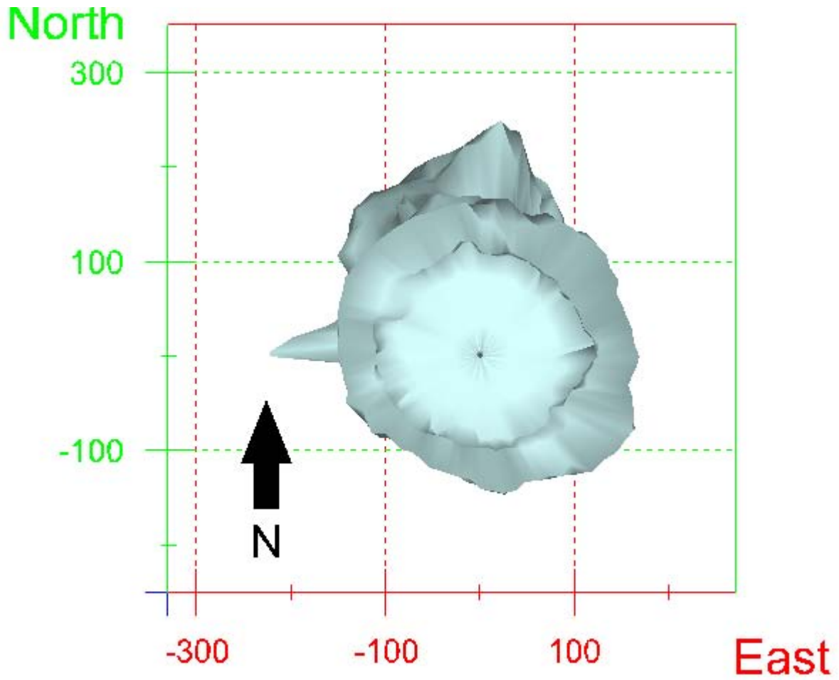
Figure 353. Map view sonar image of cavern BM-109, showing the basic geometry of the cavern. Grid squares represent 200 ft.
