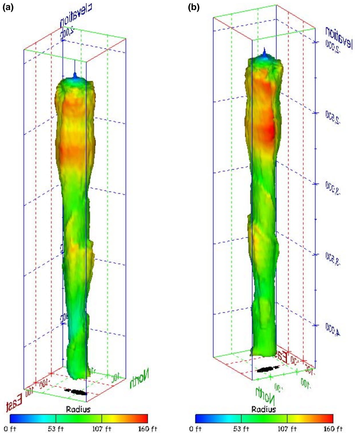
Figure 539. Sonar images of cavern BM-116, showing the geometry of the cavern colored by measured radius. View from (a) azimuth 60°, elevation 20°; (b) azimuth 300°, elevation 20°.
