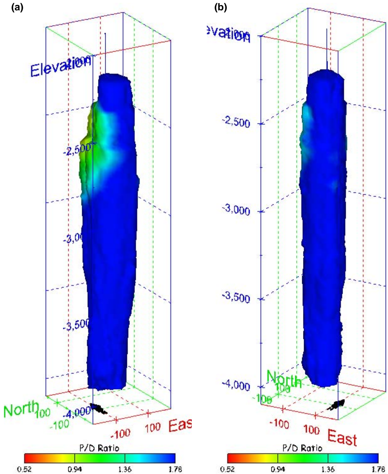
Figure 324. Sonar images of cavern BM-107, showing the geometry of the cavern colored by three-dimensional pillar-to-diameter ratio. View from (a) azimuth 210°, elevation 20°; (b) azimuth 150°, elevation 20°.
