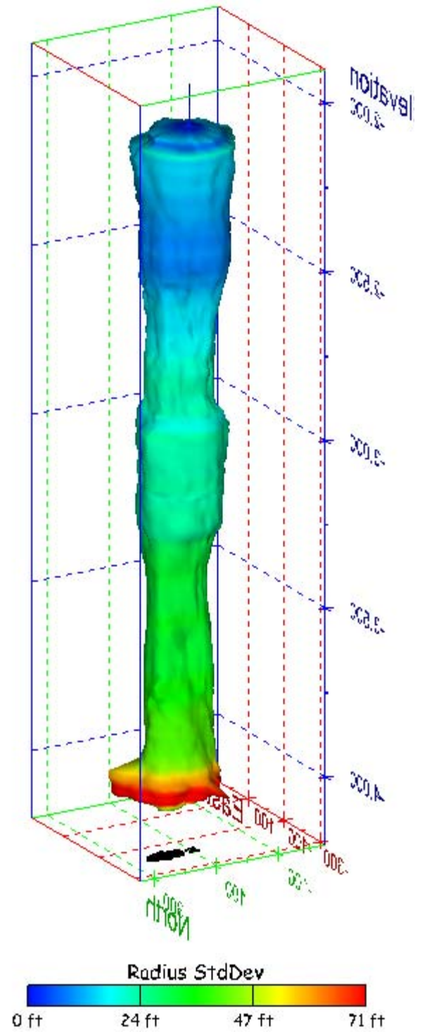
Figure 367. Sonar images of cavern BM-109, showing the geometry of the cavern colored by radius standard deviation. View from (a) azimuth 60°, elevation 20°; (b) azimuth 300°, elevation 20°.
