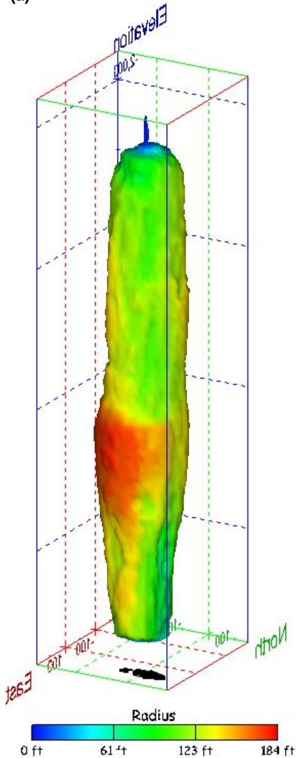
Figure 279. Sonar images of cavern BM-106, showing the geometry of the cavern colored by measured radius. View from (a) azimuth 60°, elevation 20°; (b) azimuth 300°, elevation 20°.
