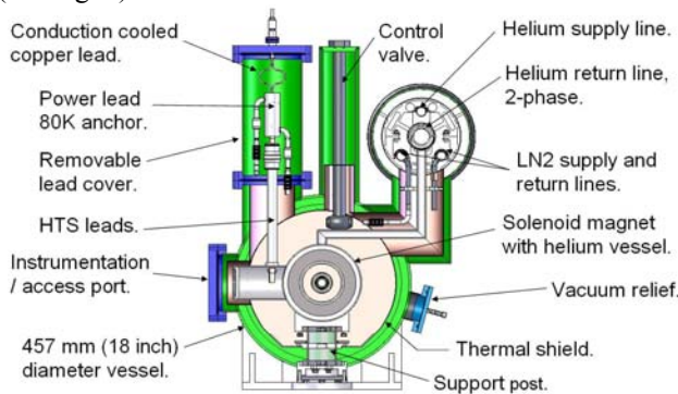
Figure 2: Cross section through CH solenoid cryostat
