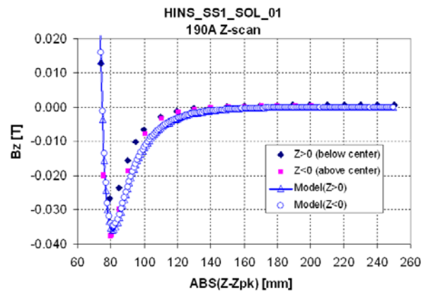
Figure 3: Predicted and measured axial magnetic field in the fringe region at 190A for SS1 prototype solenoid
