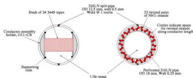
Fig. 1 Conceptual designs of HTS and LTS conductors
