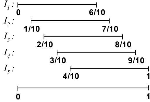
Fig. 9. Graphical illustration of sets I_1, I_2, I_3, I_4, I_5 defined in Eq. (6.1) with the interval [a, b] normalized to [0, 1] for notational convenience.
