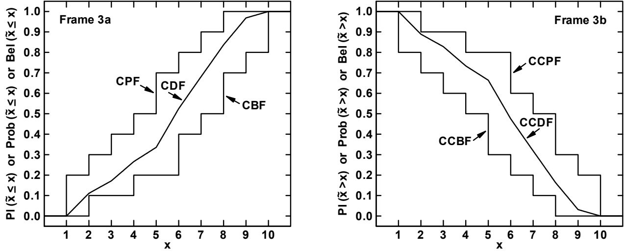
Fig. 3. Plots of (a) CBF, CCBF, CPF and CCPF for evidence space (\mathcal{X}, \Xi, m) with (i) \mathcal{X} = \{x: 1 \leq x \leq 10\} , (ii) \Xi = \{\mathcal{U}_1, \mathcal{U}_2, \dots, \mathcal{U}_{10}\} with \mathcal{U}_i = [i, 2i] for i = 1, 2, 3, 4, 5 , \mathcal{U}_i = [i-1, i] for i = 6, 7, 8, 9 , and \mathcal{U} = [1, 10] , and (iii) m(\mathcal{U}) = 1/10 if \mathcal{U} \in \Xi and m(\mathcal{U}) = 0 otherwise, and (iv) PI(\tilde{x} \leq x) , Bel(\tilde{x} \leq x) , PI(\tilde{x} > x) and Bel(\tilde{x} > x) used as abbreviated notations for PI_i(\mathcal{U}_x) , Bel_i(\mathcal{U}_x) , PI_i(\mathcal{U}_x^c) and Bel_i(\mathcal{U}_x^c) in Eqs. (2.25) and (2.26), and (b) CDF and CCDF for probability space (\mathcal{X}, \Xi, p) with density function d defined as indicated in Eq. (2.40) with Prob(\tilde{x} \leq x) and Prob(\tilde{x} > x) used as abbreviated notations for p_i(\mathcal{U}_x) and p_i(\mathcal{U}_x^c) in Eqs. (2.37) and (2.38).
