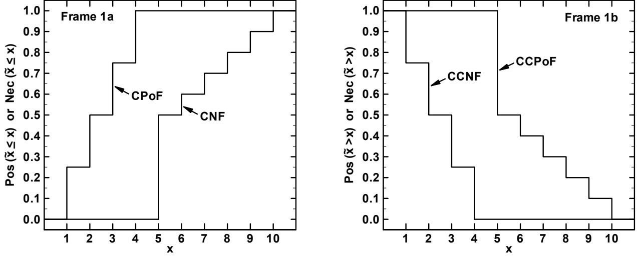
Fig. 1. Plots of CNF, CCNF, CPoF and CCPoF for possibility space (X, r) with (i) X = \{x: 1 \leq x \leq 10\} , (ii) r(x) = i/4 for i \leq x \leq i + 1 and i = 1, 2, 3, 4 , (iii) r(x) = (10 - i)/10 for i \leq x \leq i + 1 and i = 5, 6, 7, 8, 9 , and (iv) Pos(\tilde{x} \leq x) , Nec(\tilde{x} \leq x) , Pos(\tilde{x} > x) and Nec(\tilde{x} > x) used as abbreviated notations for the expressions Pos_i(\mathcal{U}_x) , Nec_i(\mathcal{U}_x) , Pos_i(\mathcal{U}_x^c) and Nec_i(\mathcal{U}_x^c) in Eqs. (2.11) and (2.12): (a) CNF and CPoF, and (b) CCNF and CCPoF.
