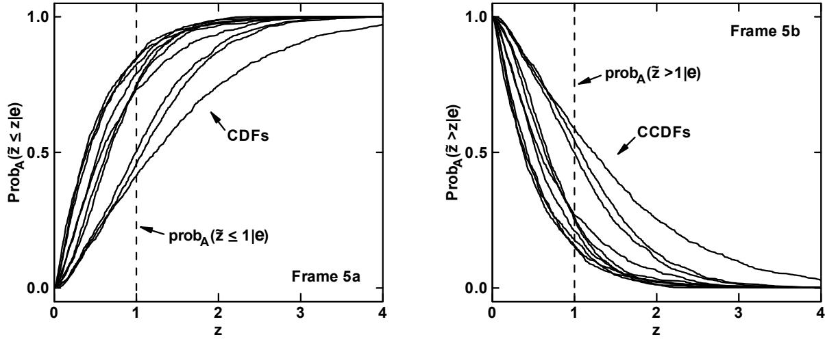
Fig. 5. Example CDFs and CCDFs that result for different values of the vector \mathbf{e} = [\mathbf{e}_M, \mathbf{e}_D] of epistemically uncertain analysis inputs: (a) CDFs, and (b) CCDFs.
