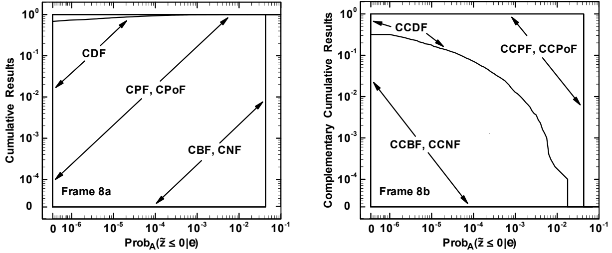
Fig. 8. Illustration of (i) CNF, CCNF, CPoF and CCPoF for unstructured possibility space (\mathcal{P}, r_p) defined in Sect. 5 (see Eqs. (5.1) and (5.5)), (ii) CBF, CCBF, CPF and CCPF for unstructured evidence space (\mathcal{P}, \Pi, m_p) defined in Sect. 5 (see Eqs. (5.2) and (5.6)), and (iii) CDF and CCDF for uniform probability space (\mathcal{P}, \Pi, p_p) defined in Sect. 5 (see Eqs. (5.3) and (5.7)): (a) CDF, CPF, CPoF, CBF and CNF, and (b) CCDF, CCPF, CCPoF, CCBF and CCNF.
