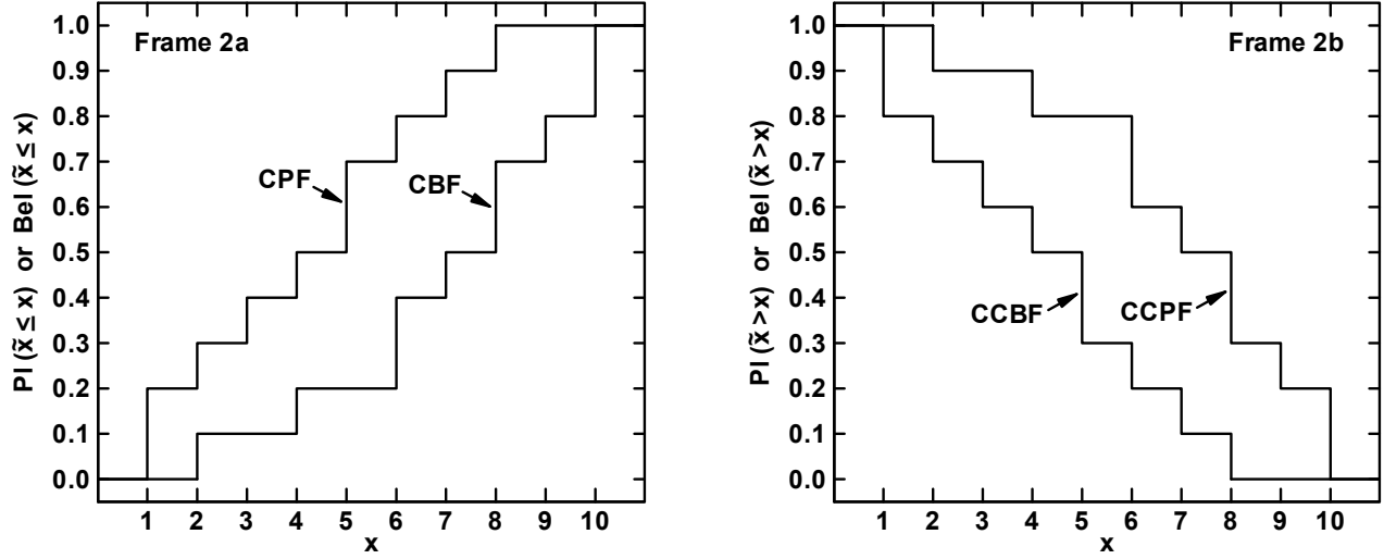
Fig. 2. Plots of CBF, CCBF, CPF and CCPF for evidence space (\mathcal{X}, \Xi, m) with (i) \mathcal{X} = \{x: 1 \leq x \leq 10\} , (ii) \Xi = \{\mathcal{U}_1, \mathcal{U}_2, \dots, \mathcal{U}_{10}\} with \mathcal{U}_i = [i, 2i] for i = 1, 2, 3, 4, 5 and \mathcal{U}_i = [i-1, i] for i = 6, 7, 8, 9, 10 , (iii) m(\mathcal{U}) = 1/10 if \mathcal{U} \in \Xi and m(\mathcal{U}) = 0 otherwise, and (iv) Pl(\tilde{x} \leq x) , Bel(\tilde{x} \leq x) , Pl(\tilde{x} > x) and Bel(\tilde{x} > x) used as abbreviated notations for Pl_i(\mathcal{U}_x) , Bel_i(\mathcal{U}_x) , Pl_i(\mathcal{U}_x^c) and Bel_i(\mathcal{U}_x^c) in Eqs. (2.25) and (2.26): (a) CBF and CPF, and (b) CCBF and CCPF.
