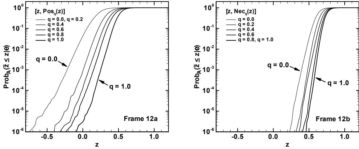
Fig. 12. Illustration of possibility curves and necessity curves defined by [z, Pos_q(z)] and [z, Nec_q(z)] , respectively, for z_{mn} \leq z \leq z_{mx} and q = 0.0, 0.2, 0.4, 0.6, 0.8 and 1.0 : (a) Possibility curves, and (b) Necessity curves.
