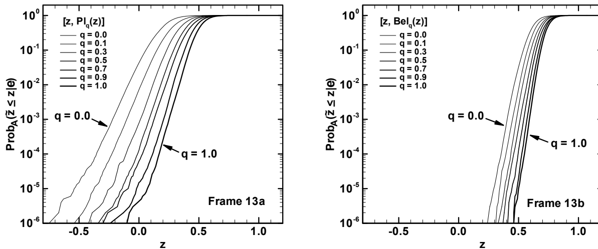
Fig. 13. Illustration of plausibility curves and belief curves defined by [z, Pl_q(z)] and [z, Bel_q(z)] , respectively, for z_{mn} \leq z \leq z_{mx} and q = 0.0, 0.1, 0.3, 0.5, 0.7, 0.9 and 1.0 : (a) Plausibility curves, and (b) Belief curves.
