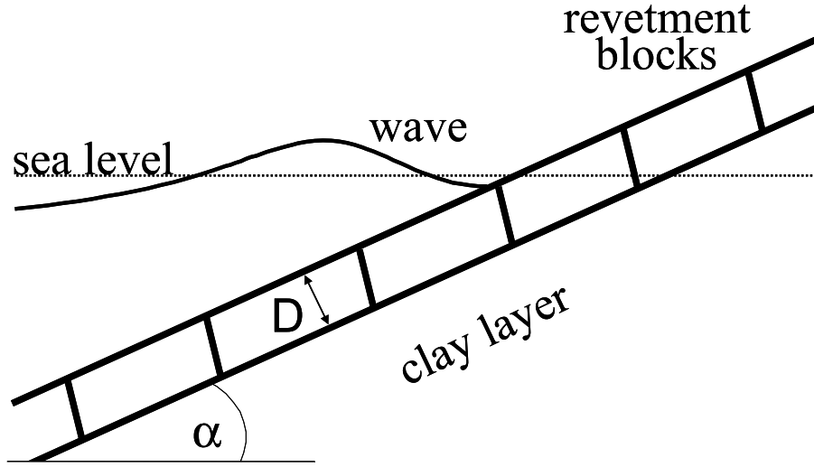
Fig. 6. Dike revetment (Fig. 12 in Ferson and Tucker [147] as redrawn from Husaarts et al. [145]).
