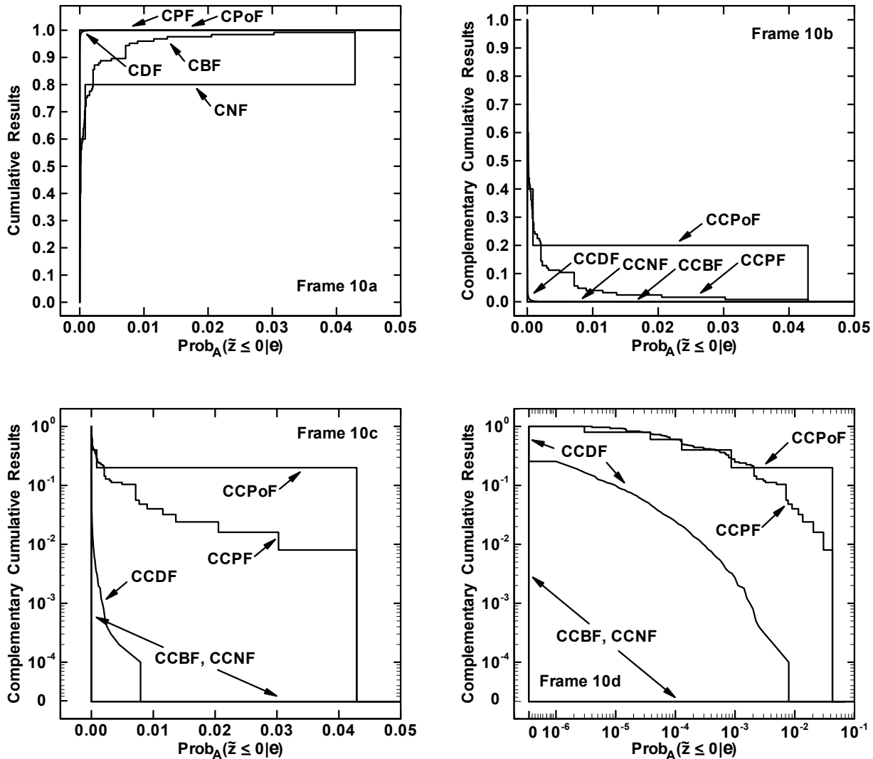
Fig. 10. Illustration of (i) CNF, CCNF, CPoF and CCPoF for structured possibility space (\mathcal{P}, r_p) defined in Sect. 6 (see Eq. (6.2) and resultant definition for r_E ), (ii) CBF, CCBF, CPF and CCPF for structured evidence space (\mathcal{P}, \Pi, m_p) defined in Sect. 6 (see Eq. (6.3) and resultant definition for m_E ), and (iii) CDF and CCDF for nonuniform probability space (\mathcal{P}, \Pi, p_p) defined in Sect. 6 (see Eq. (6.4) and resultant definition for density function d_E corresponding to p_E ): (a) CPoF, CNF, CPF, CBF and CDF with linear scales on abscissa and ordinate, (b) CCPoF, CCNF, CCPF, CCBF and CCDF with linear scales on abscissa and ordinate, (c) same as (b) but with log scale on ordinate, and (d) same as (b) but with log scales on abscissa and ordinate.
