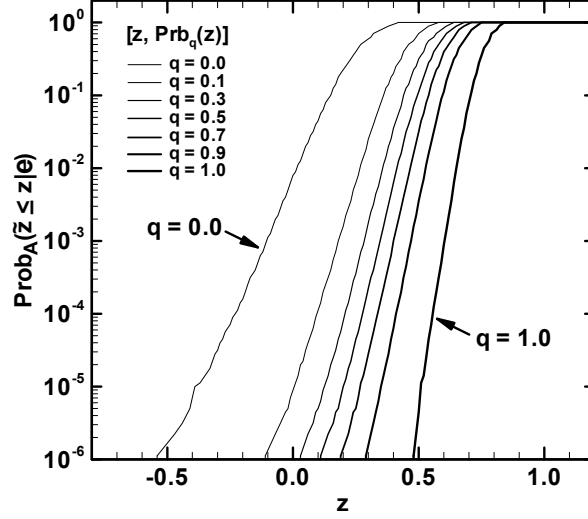
Fig. 11. Illustration of quantile (probability) curves defined by [z, Prb_q(z)] for z_{mn} \leq z \leq z_{mx} and q = 0.0, 0.1, 0.3, 0.5, 0.7, 0.9 and 1.0 .
