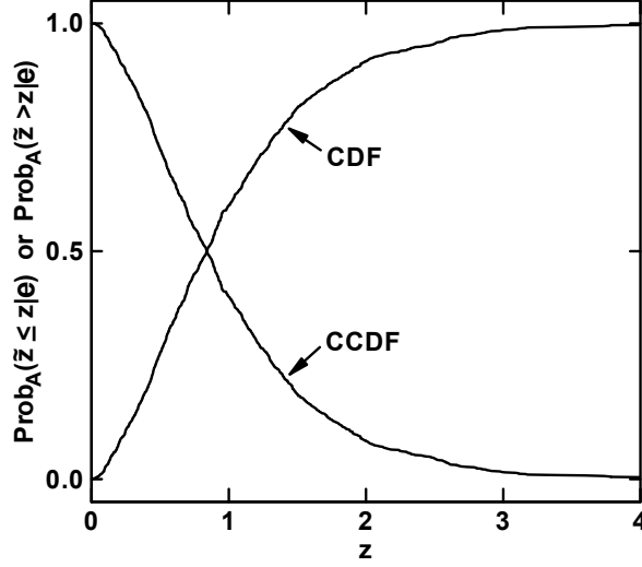
Fig. 4. Example CDF and CCDF defined by points [z, Prob_A(\bar{z} \leq z | \mathbf{e})] and [z, Prob_A(\bar{z} > z | \mathbf{e})] , respectively.
