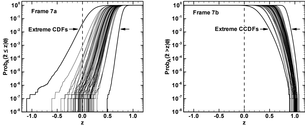
Fig. 7. Illustration of 50 of the nSE = 10,256 CDFs and CCDFs generated for the sample in Eq. (5.15): (a) CDFs, and (b) CCDFs.
