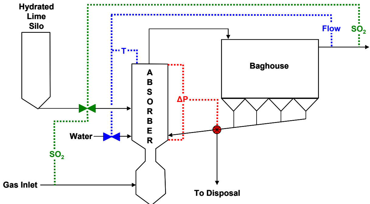
Figure 9. Process control schematic showing major control loops for the Turbosorp® circulating fluidized bed dry scrubber at AES Greenidge. Lime injection control is shown in green; water injection control is shown in blue, and solid product recycle control is shown in red.
