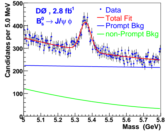
Figure 4: The invariant mass distribution of B_s^0 candidates from D0
