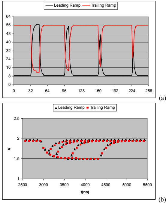
Fig. 5. (a) Raw data from TDC (b) Digitized waveform It should be pointed out that the TDC values represent not only the voltage levels at the sampling points, but also the sampling times. In high precision applications, the differences of the sampling times should be taken into account but it is not too difficult to do so.
