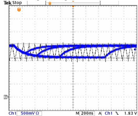
Fig. 4. The input to ADC (blue) and the reference voltage (black)
