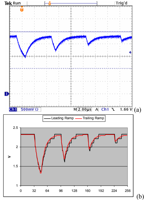
Fig. 7. (a) Input waveform (b) Digitized waveform Passive components are chosen for the ramping reference voltage generation network primarily for simplicity. The ramping voltage from passive RC network is intrinsically non-linear which sometimes is viewed as a disadvantage. In FPGA, however, correcting nonlinearity is merely a transform via a look-up table. In our example here, the exponential voltage ramp can be further used to increase measurement dynamic range, which becomes an advantage.
