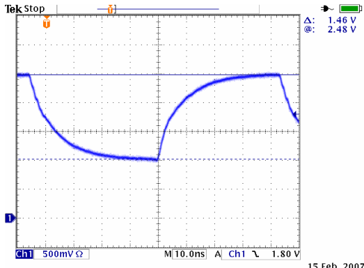
Fig. 6. The reference voltage with exponential discharge property The exponential reference voltage samples the input waveform shown in Fig. 7(a). (Note that the oscilloscope time scales for Fig. 6 and 7(a) are different but the voltage scales
