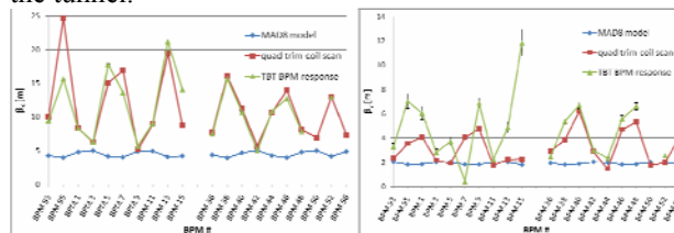
Figure 11: Comparison of measured and theoretical \beta -functions.
