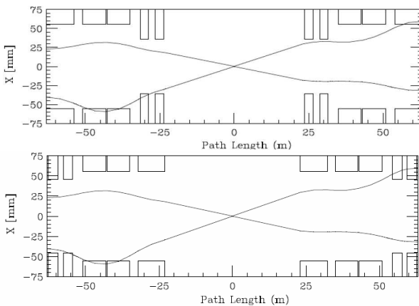
Figure 4. Magnet apertures and 9\sigma beam envelopes in the crossing plane for SYM with a 90 mm Nb3Sn Q1 (top), and 110mm Nb3Sn Q3 (bottom).
