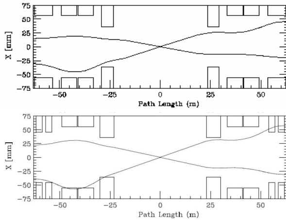
Figure 3. Magnet apertures and 9\sigma beam envelopes in the crossing plane for LBM with a 90mm Nb3Sn Q1 (top), and 110mm Nb3Sn Q3 (bottom).
