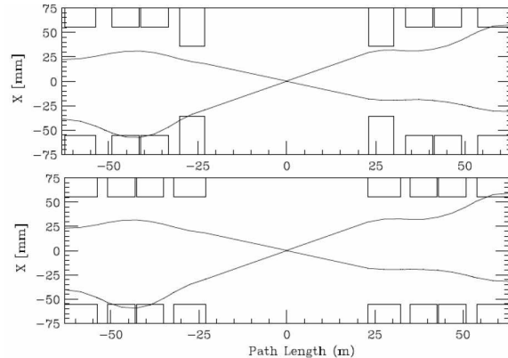
Figure 2. Magnet apertures and 9\sigma beam envelopes for LBM (top) and SYM (bottom) in the crossing plane, with a 225 \mu\text{rad} half-crossing angle.
