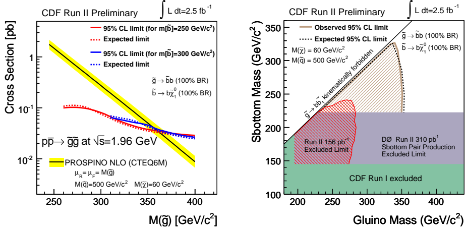
Figure 4: Left: Upper limit on \sigma(p\bar{p} \rightarrow \tilde{g}\tilde{g}, \tilde{g} \rightarrow \tilde{b}b_1 (100\%)) at 95% C.L. as a function of M(\tilde{g}) for two different M(\tilde{b}_1) = 250, 300 GeV/c 2 . Right: M(\tilde{b}_1) vs M(\tilde{g}) exclusion plot showing observed and expected limits at 95% C.L. with R-parity conserved. Please see the details in [11].
