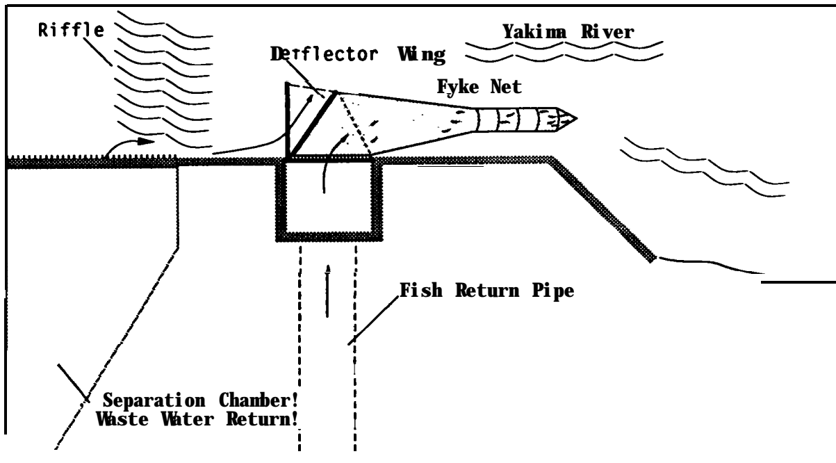
FIGURE. Fyke Net Used in Pipe Tests at the Wapato Screens, Spring 1989
