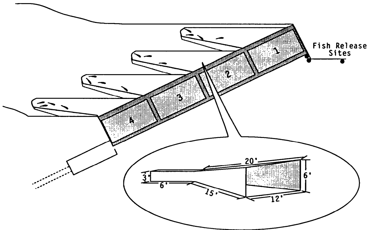
FIGURE 7. Fyke Nets Used in Integrity Tests at the Uestside Ditch Screens, Spring 1989
