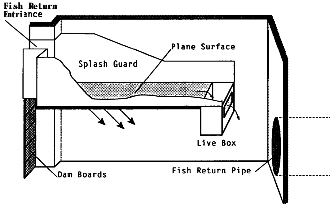
FIGURE. Inclined Plane Used at the Westside Ditch Canal Fish Screening Facility, Spring 1989
