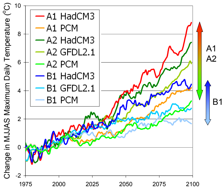
Figure 1. Projected increase in summer (May–Sept) daily maximum temperatures relative to 1971–2000 mean for the HadCM3, GFDL2.1, and PCM models as simulated for the A1fi (higher), A2 (mid-high), and B1 (lower) scenarios. A 10-year running mean is shown.
