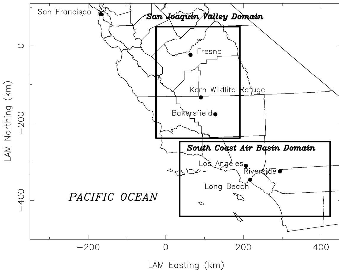
Figure 3-1: Modeling domains used for sensitivity studies in the San Joaquin Valley and the South Coast Air Basin [14].
