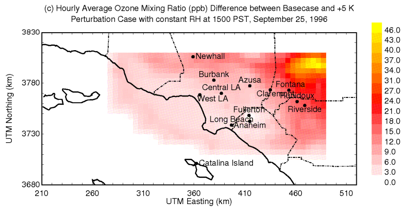
Figure 5-3: Hourly average ozone mixing ratio (panel a) and ozone mixing ratio difference in response to uniform temperature perturbations with constant relative humidity (panels b,c) at 1500 PST on September 25, 1996. Units are ppb.
