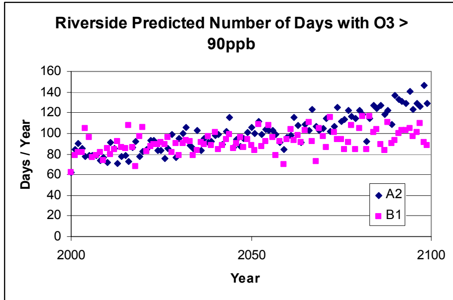
Figure 6. GFDL projected monthly mean 850 millibar temperatures in the SoCAB converted to estimates of the number of days each year with ozone greater than 90 ppb at Riverside. Global emissions scenario A2 has higher global CO 2 emissions than scenario B1.
