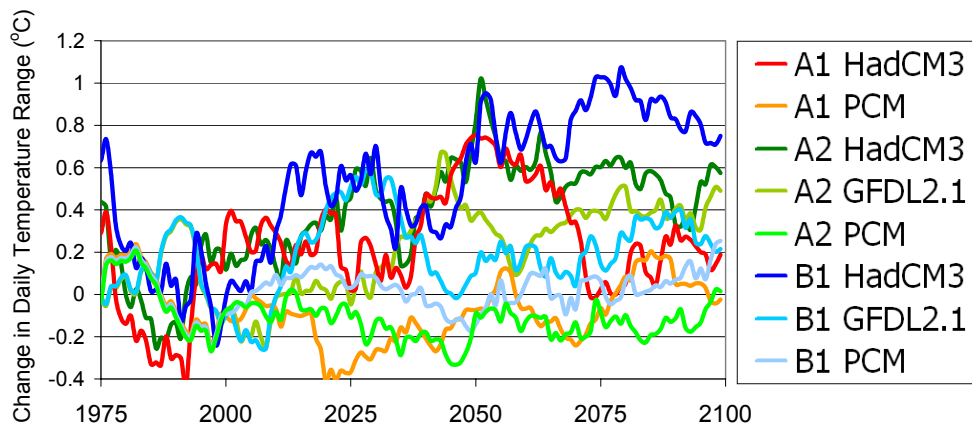
Figure 2. Projected change in summer (May–Sept) daily temperature range relative to 1971–2000 for the HadCM3, GFDL2.1, and PCM models as simulated for the A1fi (higher), A2 (mid-high), and B1 (lower) scenarios. 15-year running mean is shown.
