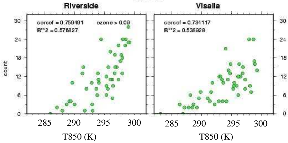
Figure 7-1: Number of days each month with 1-hr average ozone greater than 90ppb vs. monthly average T850 at Riverside (SoCAB) and Visalia (SJV) for May – October during the years 1996-2003.
