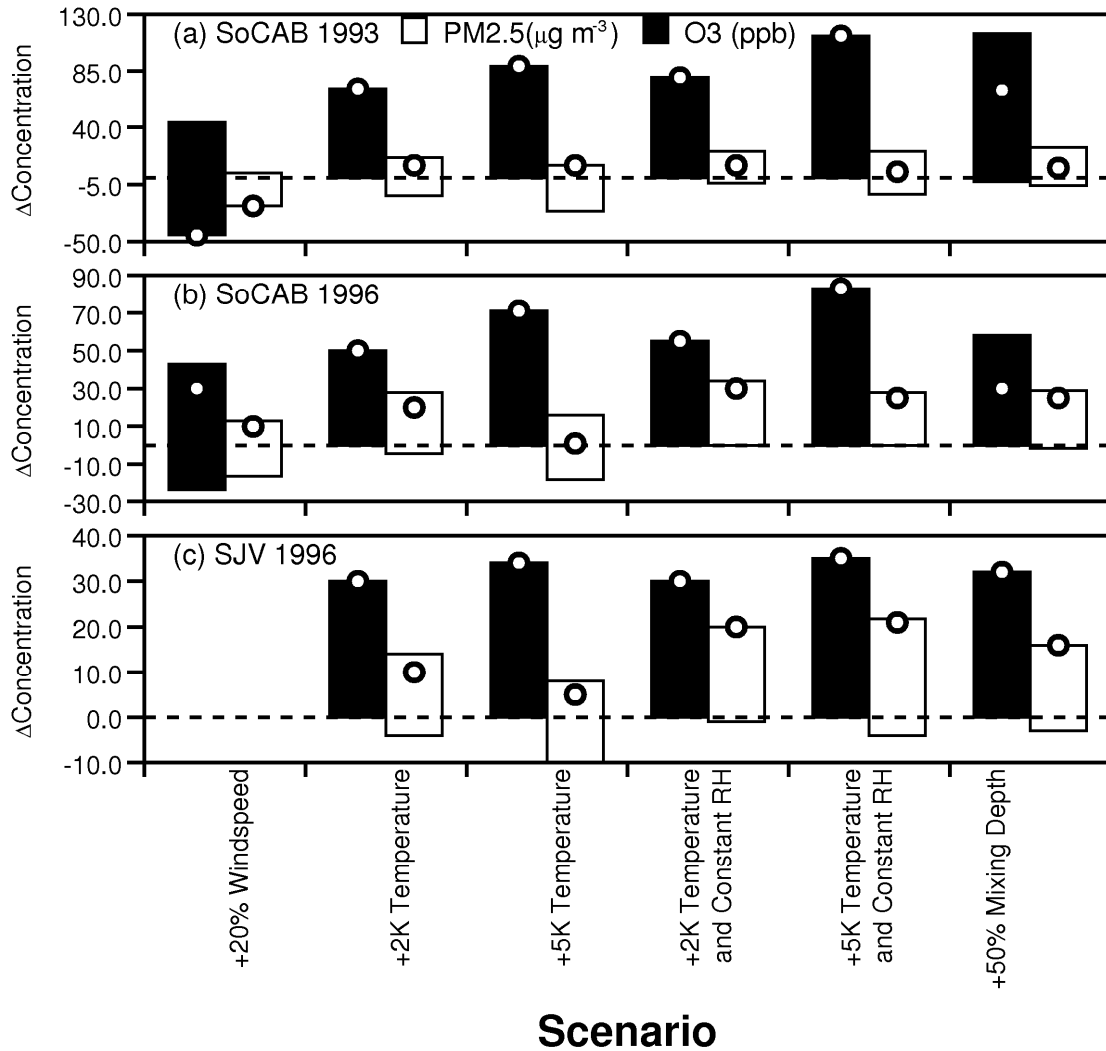
Figure 9. Summary of pollutant response to meteorological perturbations when background ozone concentrations are 60 ppb during pollution episodes that occurred in: (a) Southern California September 9, 1993, (b) Southern California September 25, 1996, and (c) the San Joaquin Valley January 6, 1996. The bars represent the range of concentration change at any location in the modeling domain in response to the indicated perturbation. The circles represent the concentration change at the location of the maximum concentration for each pollutant.
