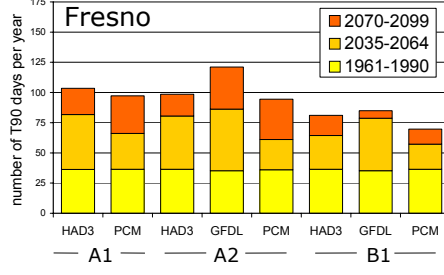
Figure 4. Projected change in number of T90 days for five urban centers in California as simulated by the HadCM3, GFDL2.1, and PCM models for the A1fi (higher), A2 (mid-high), and B1 (lower) emission scenarios. Yellow denotes the number of 90th percentile exceedance days during historical reference period (~36 days), orange the number of days by mid-century, and red the number of days by end-of-century.
