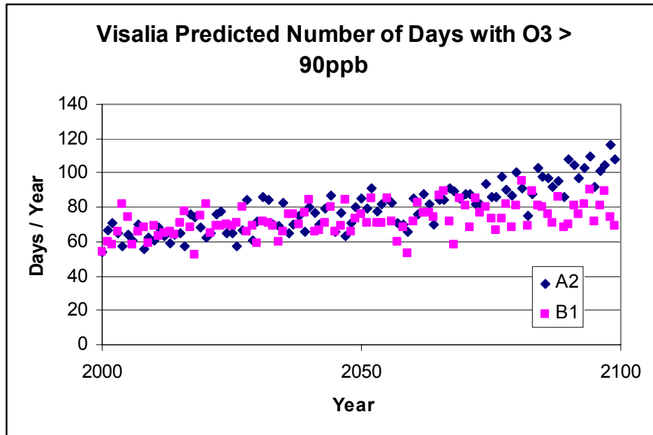
Figure 7. GFDL projected monthly mean 850 millibar temperatures in the SJV converted to estimates of the number of days each year with ozone greater than 90 ppb at Visalia (Note: Trends are based on historical data with no change in emissions).
