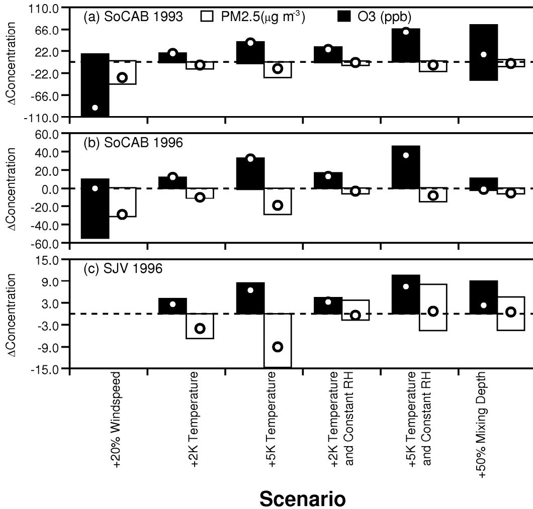
Figure 8. Summary of pollutant response to meteorological perturbations during pollution episodes that occurred in: (a) Southern California September 9, 1993, (b) Southern California September 25, 1996, and (c) the San Joaquin Valley January 6, 1996. The bars represent the range of concentration change at any location in the modeling domain in response to the indicated perturbation. The circles represent the concentration change at the location of the maximum concentration for each pollutant.
