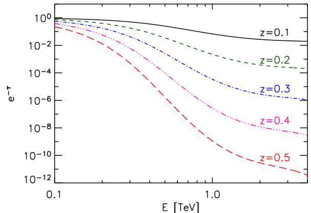
FIG. 2: Suppression of the gamma-ray spectrum due to pair production for sources at redshifts of z = 0.1, 0.2, 0.3, 0.4, and 0.5 , from top to bottom.
