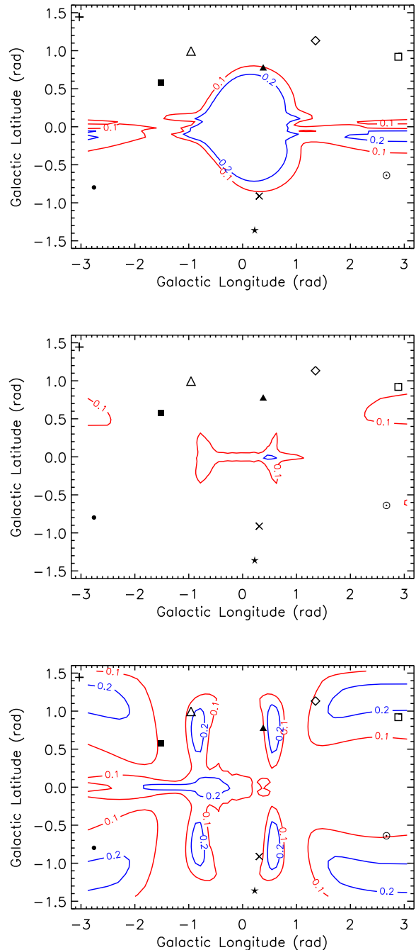
FIG. 1: The probability of ALP-photon conversion in three different models of the Galactic Magnetic Field (PS, TT, HMR from top to bottom), for g_{11} = 5 and assuming that the conditions of Eq. (3) are satisfied. Also shown are the locations of the known very high energy gamma-ray sources at redshift greater than 0.1, labeled according to the symbols found in table I.
