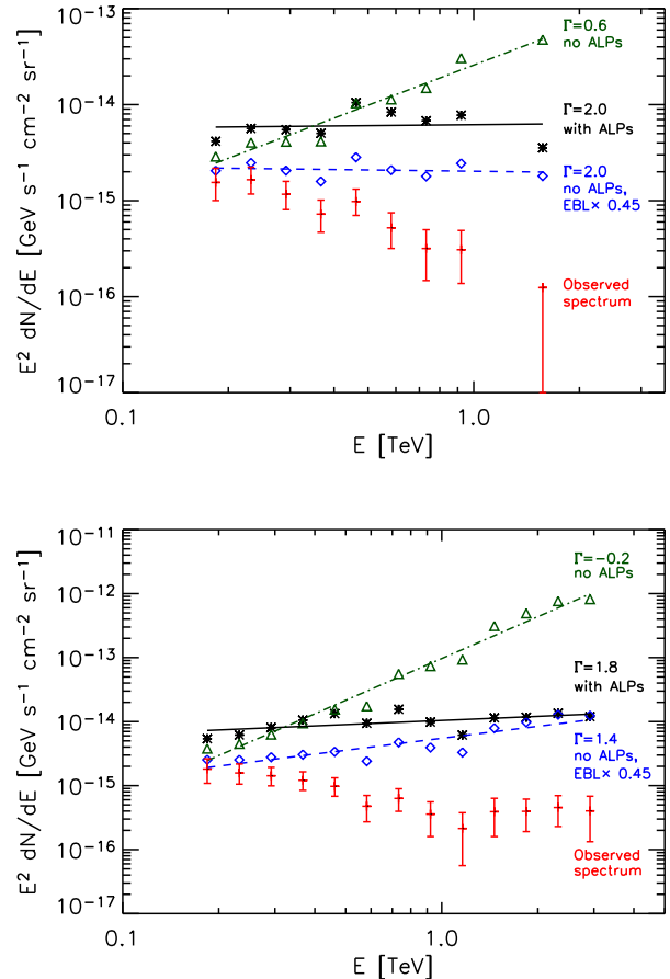
FIG. 4: The points shown with error bars represent the observed gamma-ray spectrum of H 2356-309 (top) and 1ES1101-232 (bottom), from the data of Ref. [2]. The other points shown denote the spectra required to be injected at the source in order to generate the observations after accounting for the absorption by the EBL. Using a conventional EBL spectrum and density, the reconstructed source spectra are required to be extremely hard ( dN/dE \propto E^{-0.6} and dN/dE \propto E^{0.2} ). The mechanism of photon-ALP mixing, however, can soften the required spectral slope at injection to acceptable values. See text for more details.
