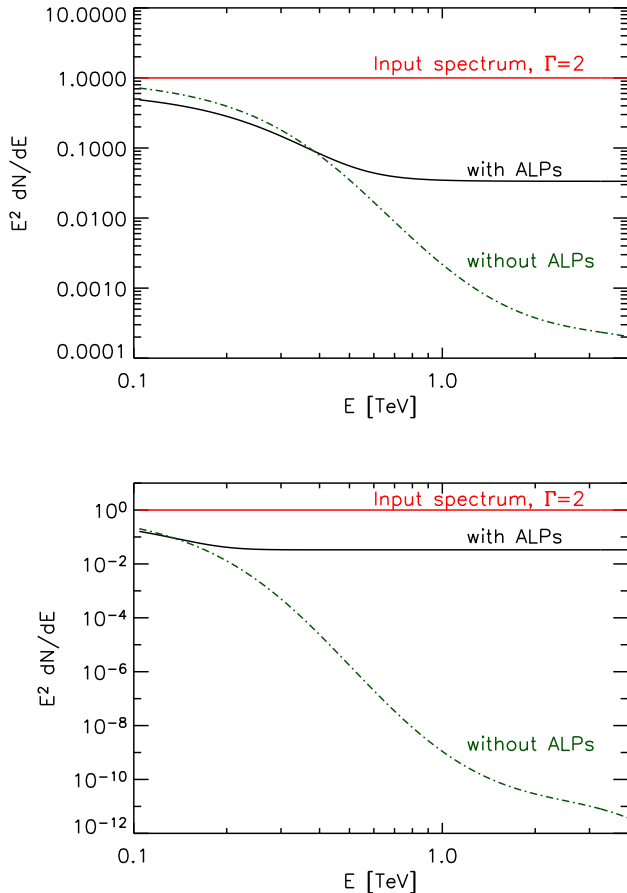
FIG. 3: The gamma-ray spectrum from a source with an injected spectrum of dN/dE \propto E^{-2} , after propagation over a distance of z = 0.2 (top) and z = 0.5 (bottom). Results are shown with and without the effect of photon-ALP oscillations. The ALP-photon mixing mitigates the impact of absorption via pair production and leads to a plateau in the spectrum at high energies. We have calculated the effects of ALP-photon mixing assuming a source conversion probability of 0.3 and a Milky Way reconversion probability of 0.1. The vertical axis is in arbitrary units.
