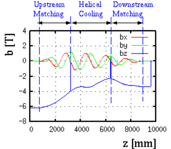
Figure 3: Field strength along the reference orbit in the MANX channel.
