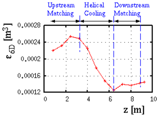
Figure 4: 6D emittance evolution in MANX.
