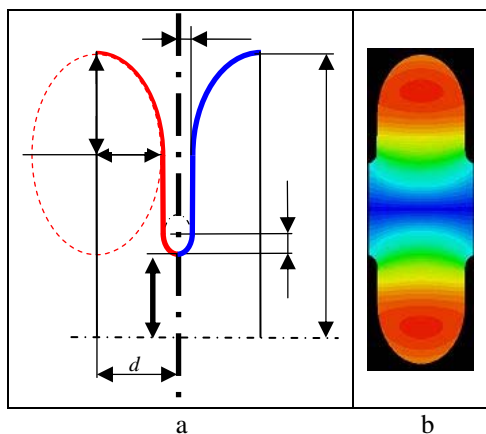
Figure 1. Cell geometry of the superconducting TW accelerating (STWA) structure: (a) STWA structure cavity shape; (b) magnetic field distribution in the STWA cell.
