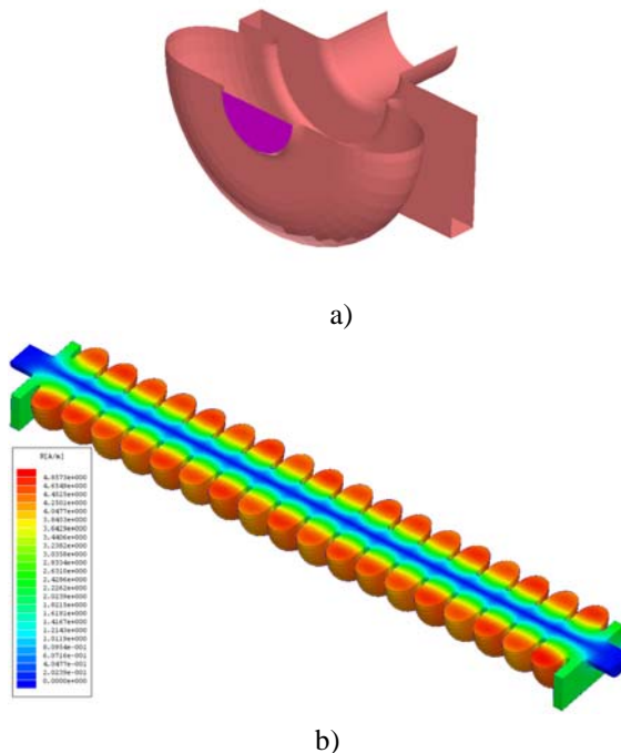
Figure 2. a) Transverse cuts through the rectangular waveguide coupling section for the L-band SCTW accelerating structure, side view; b) Magnetic field of the 18-cell SCTW cavity with the optimized coupling section.
