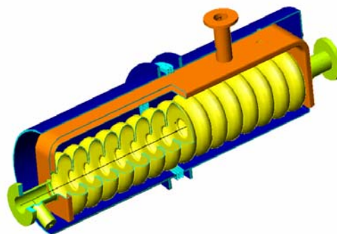
Figure 1. 15-cell SC TW structure with a waveguide inserted into the liquid helium volume.
