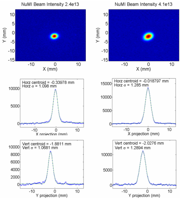
Figure 3: NuMI OTR beam images and horizontal and vertical projections with Gaussian fits for 2.4 \times 10^{13} and 4.1 \times 10^{13} protons per bunch.
