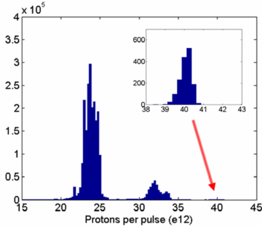
Figure 2: NuMI beam pulse intensities for \sim 80 days of operation while OTR foil is in beam path.
