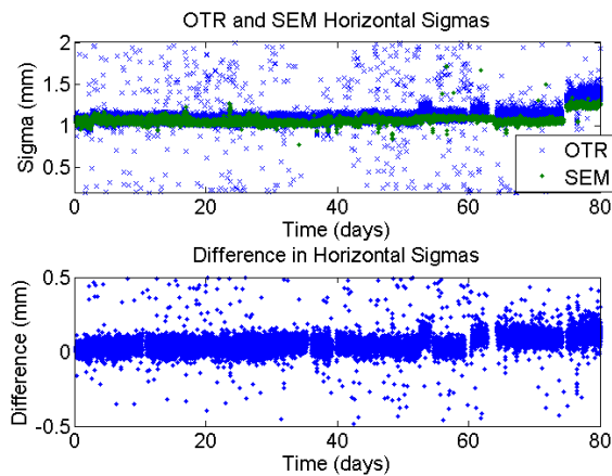
Figure 4: Comparison of the horizontal \sigma between the SEM monitor and the OTR detector over time.
