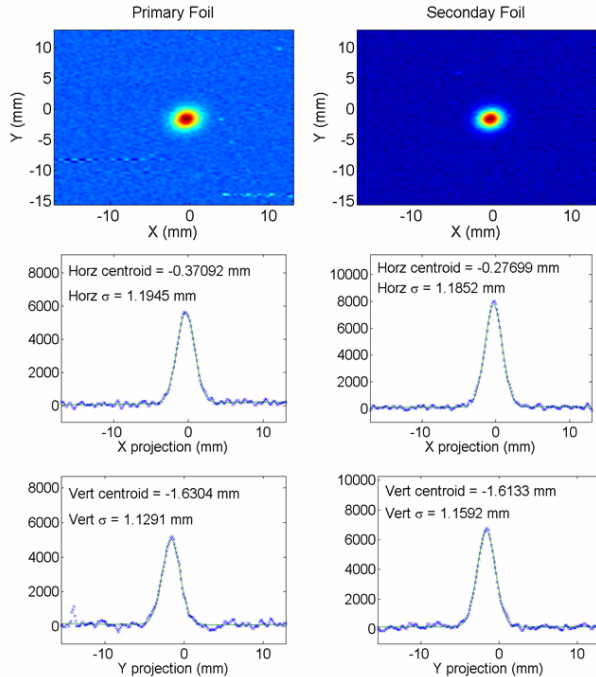
Figure 5: Comparison of OTR images taken with the primary and the secondary foils under similar beam conditions after \sim 70 days of primary foil operation.
