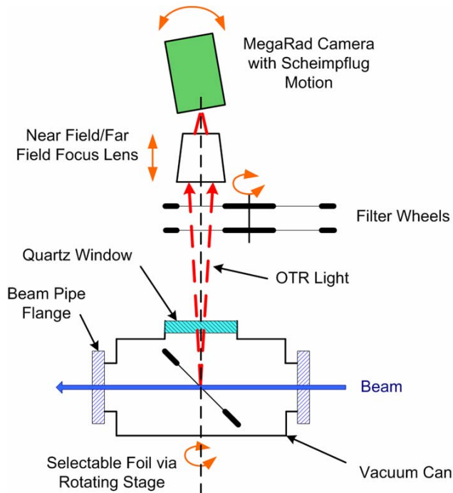
Figure 1: Block diagram of FNAL OTR detector.
