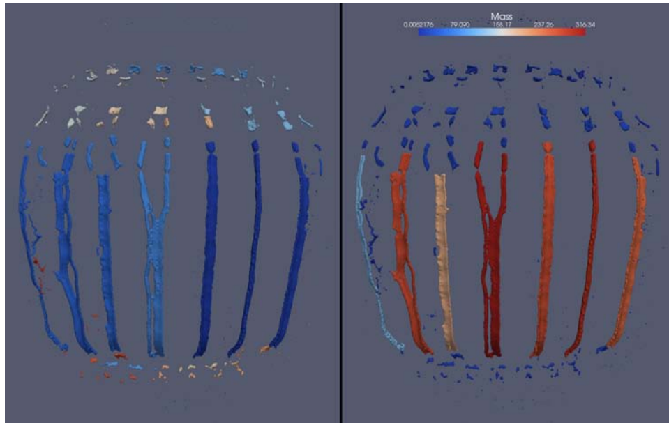
Figure 15: Quarter-symmetry CTH simulation at 2.00e-04 seconds. The left image is colored by fragment ID. The right image is colored by fragment mass.
