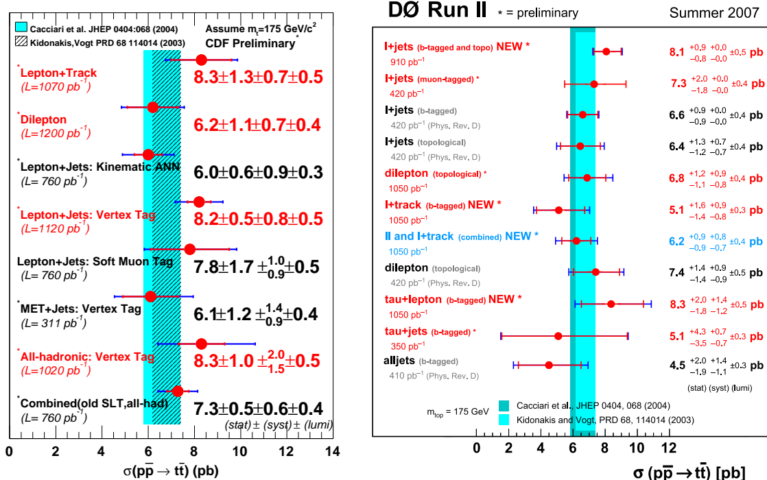
Figure 1: Top quark pair production cross-section measurements by CDF (left) and D0 (right) in comparison with theory predictions shown as coloured bands. If a systematic uncertainty is shown as 0, it is included in the statistical uncertainty.
