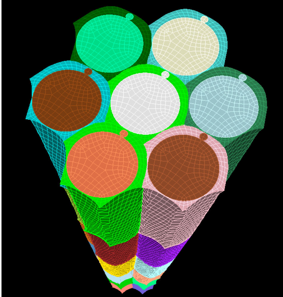
Figure 7: 7 pin wire-wrapped fuel pin lattice, with sodium region shown.
