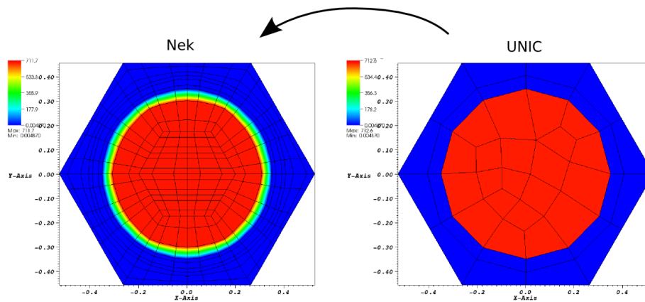
Figure 4: q''' mapped from UNIC to Nek, horizontal cross-section through the middle of a single pin with sodium. In the case of Nek, inner nodes are rendered (order of spectral elements is 4).
