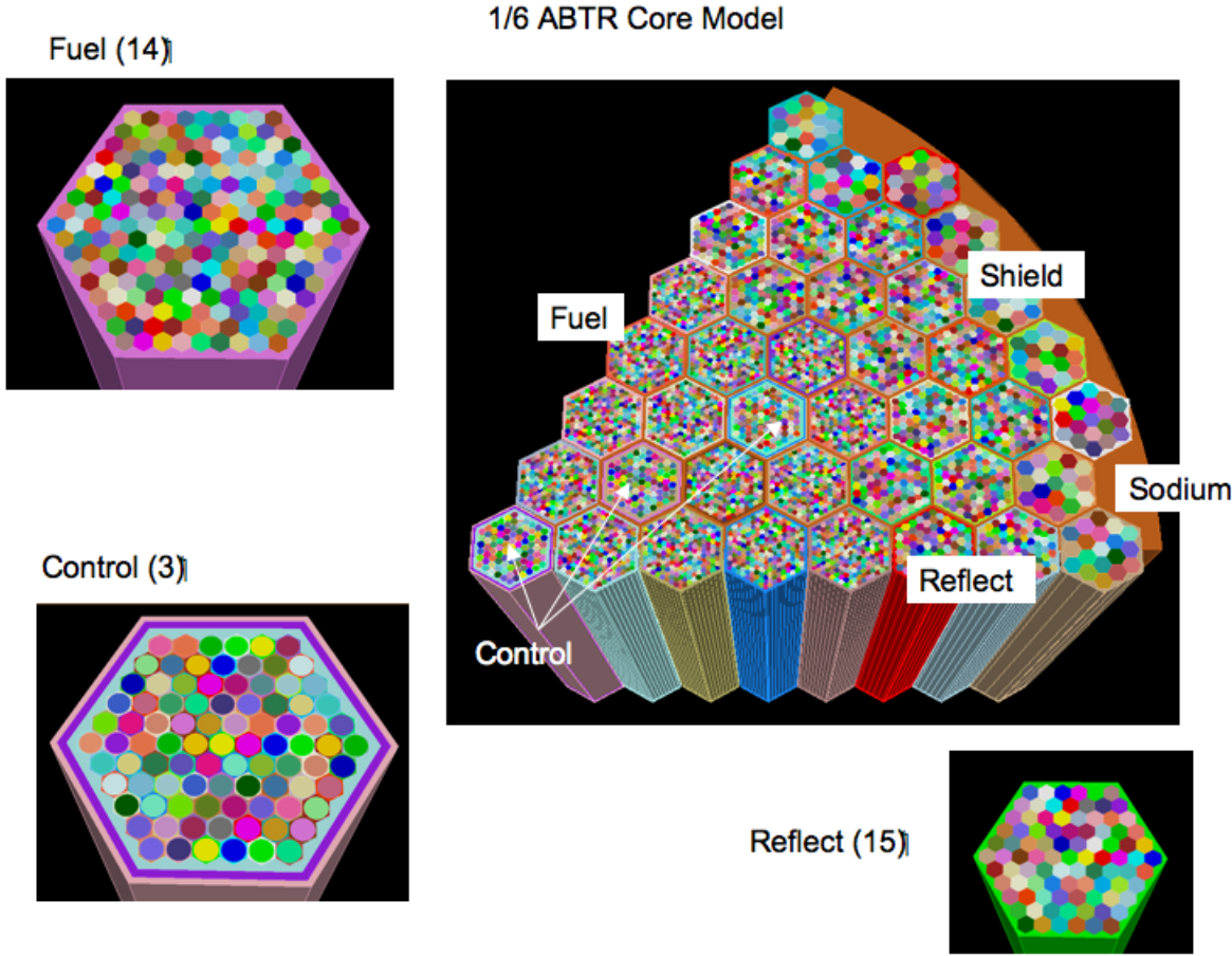
Figure 5: The ABTR core model developed in CUBIT. This model contains 5744 distinct 3D volumes and almost 50,000 surfaces.
