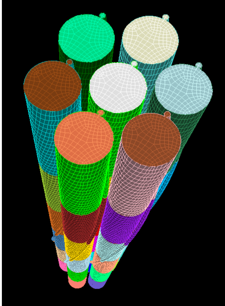
Figure 6: 7 pin wire-wrapped fuel pin lattice, showing surface mesh and without sodium.
