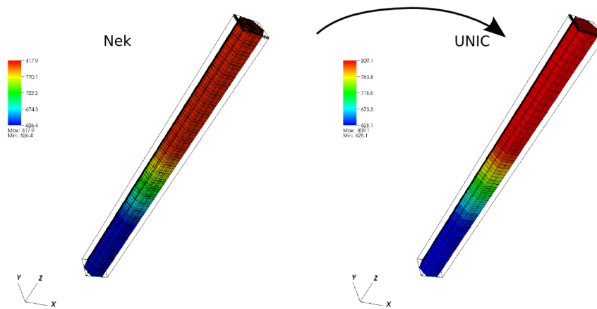
Figure 3: T mapped from Nek to UNIC blocks, single pin. The range of values differs due to block-averaging. Vertical axis has been scaled by a factor of 0.05.
