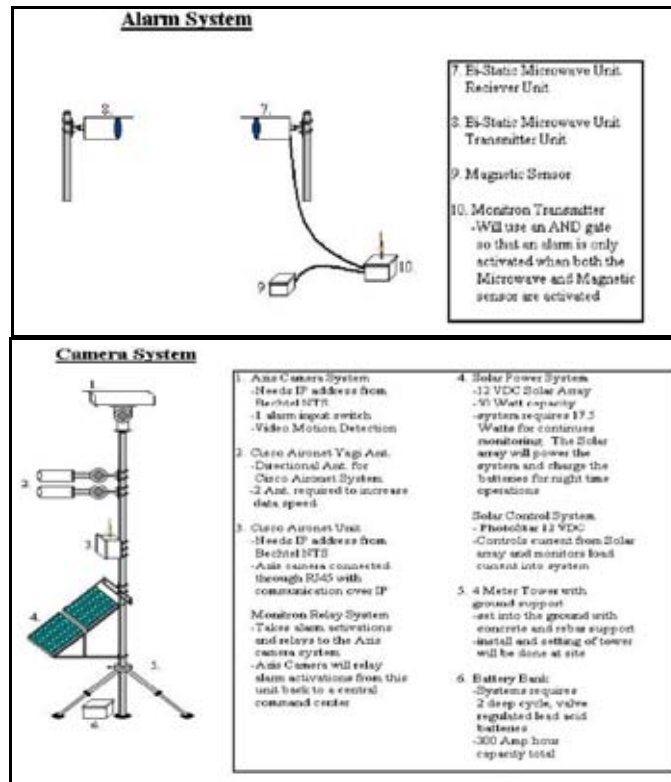
Figure 13. An Example of a Sensor-Activated Remote Monitoring System
