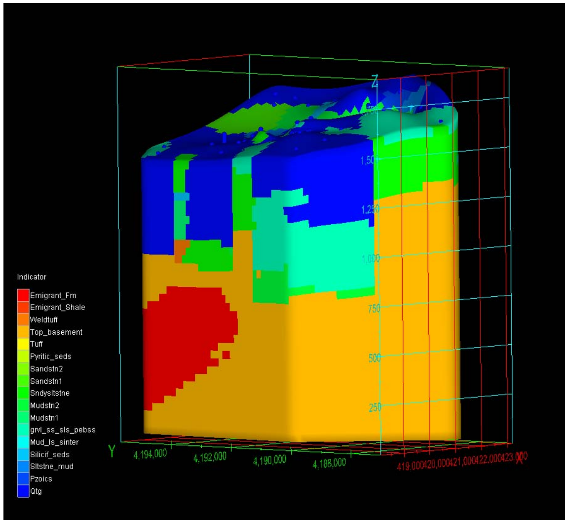
Figure 14. Side-view of 3-D geologic block model of Emigrant Geothermal Prospect area. The 3-D block modeling facilitates stripping areas away for detailed views as will be seen in following figures.
