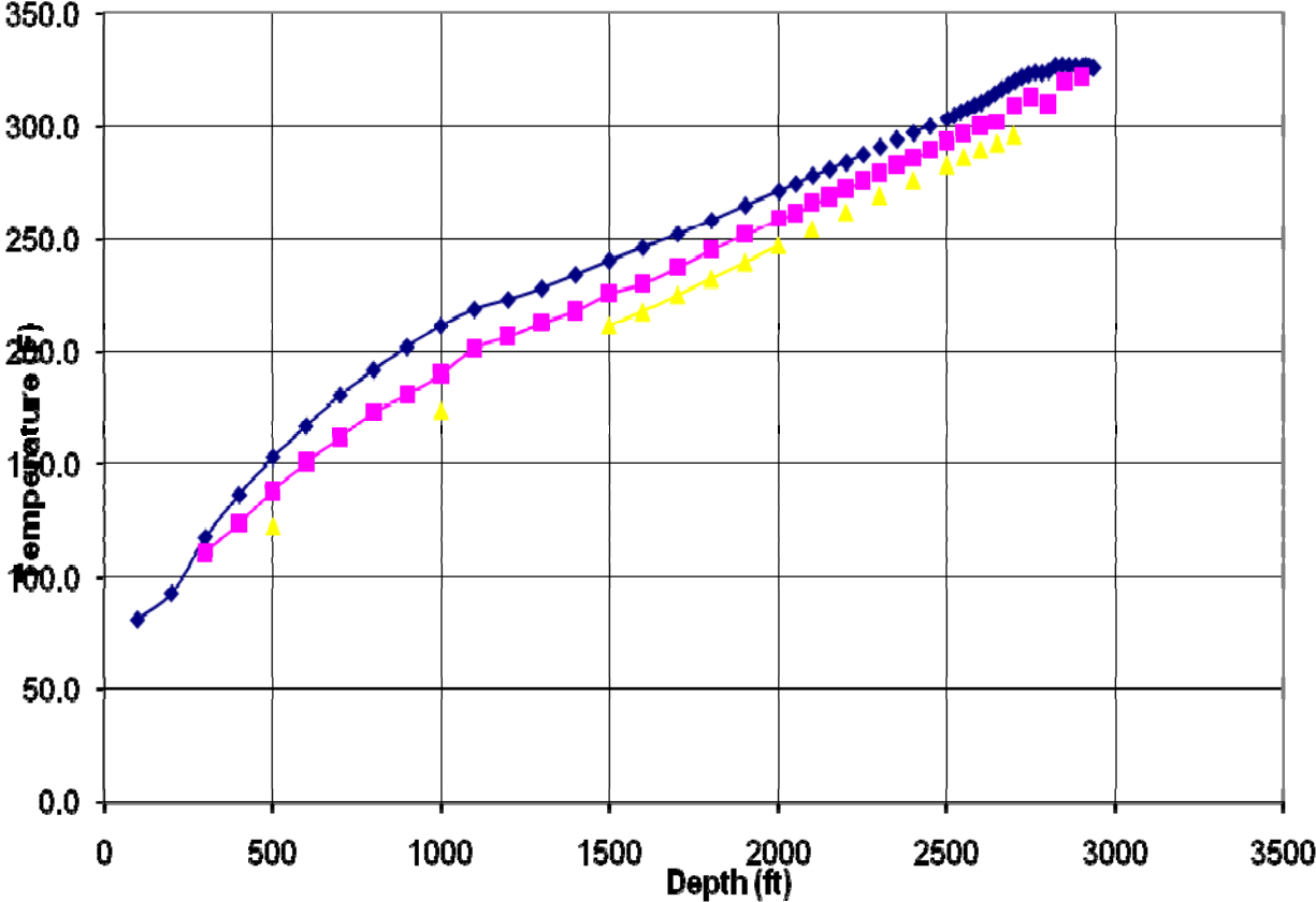
Figure 1. Temperature profiles for 17-31.
