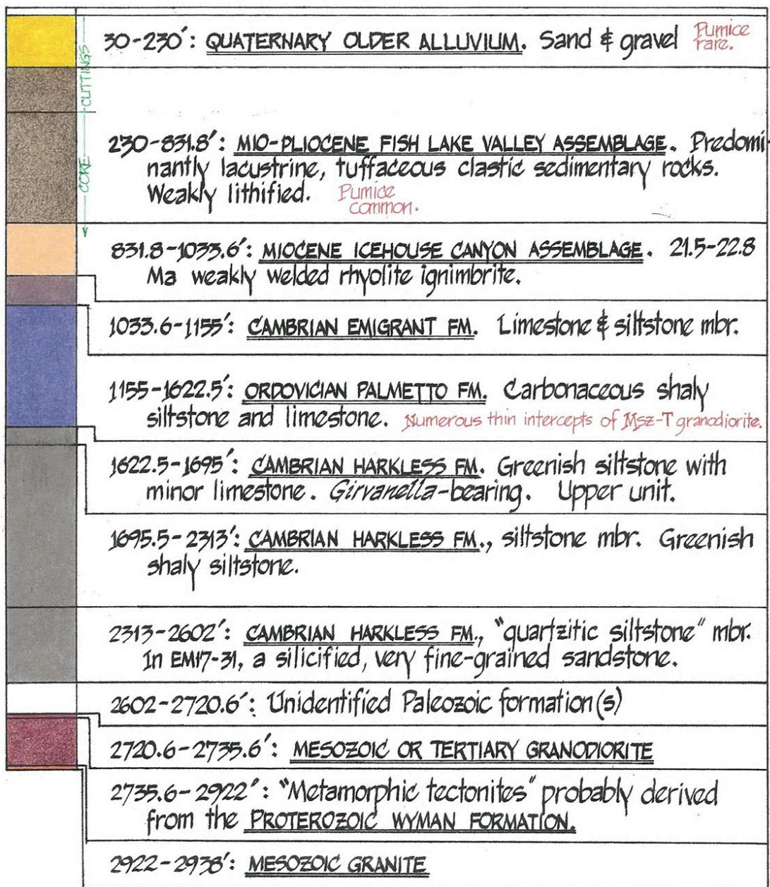
FIGURE 2. COREHOLE 17-31: CORRELATION OF PENETRATED ROCKS WITH ESTABLISHED STRATIGRAPHIC UNITS IN AND NEAR THE SILVER PK. RANGE. Based on descriptions, in Albers & Stewart ('72), Oldow et al. (2003), and Hulen et al. (2005), and on reconnaissance examination of formation outcrops near the Emigrant prospect by J. Hulen.
