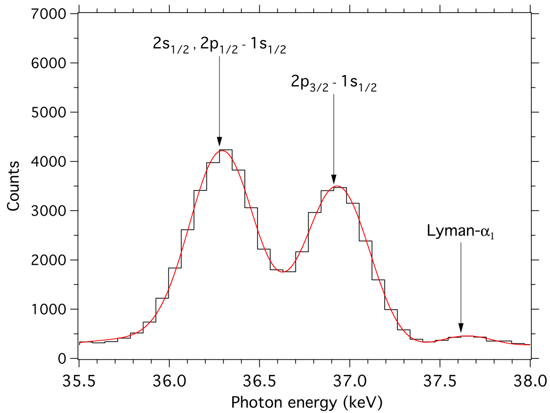
FIG. 3: Spectrum of K-shell praseodymium obtained with the germanium detector.
