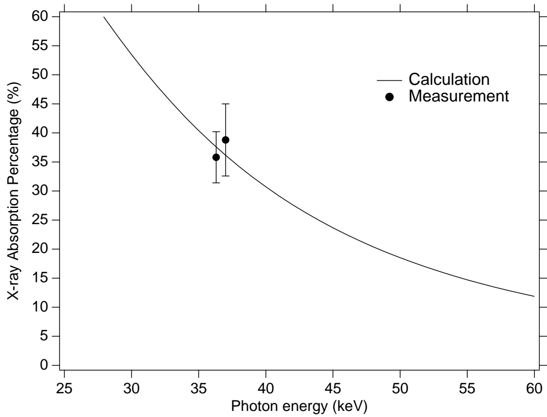
FIG. 1: Quantum efficiency of 30 \mu m bismuth.
