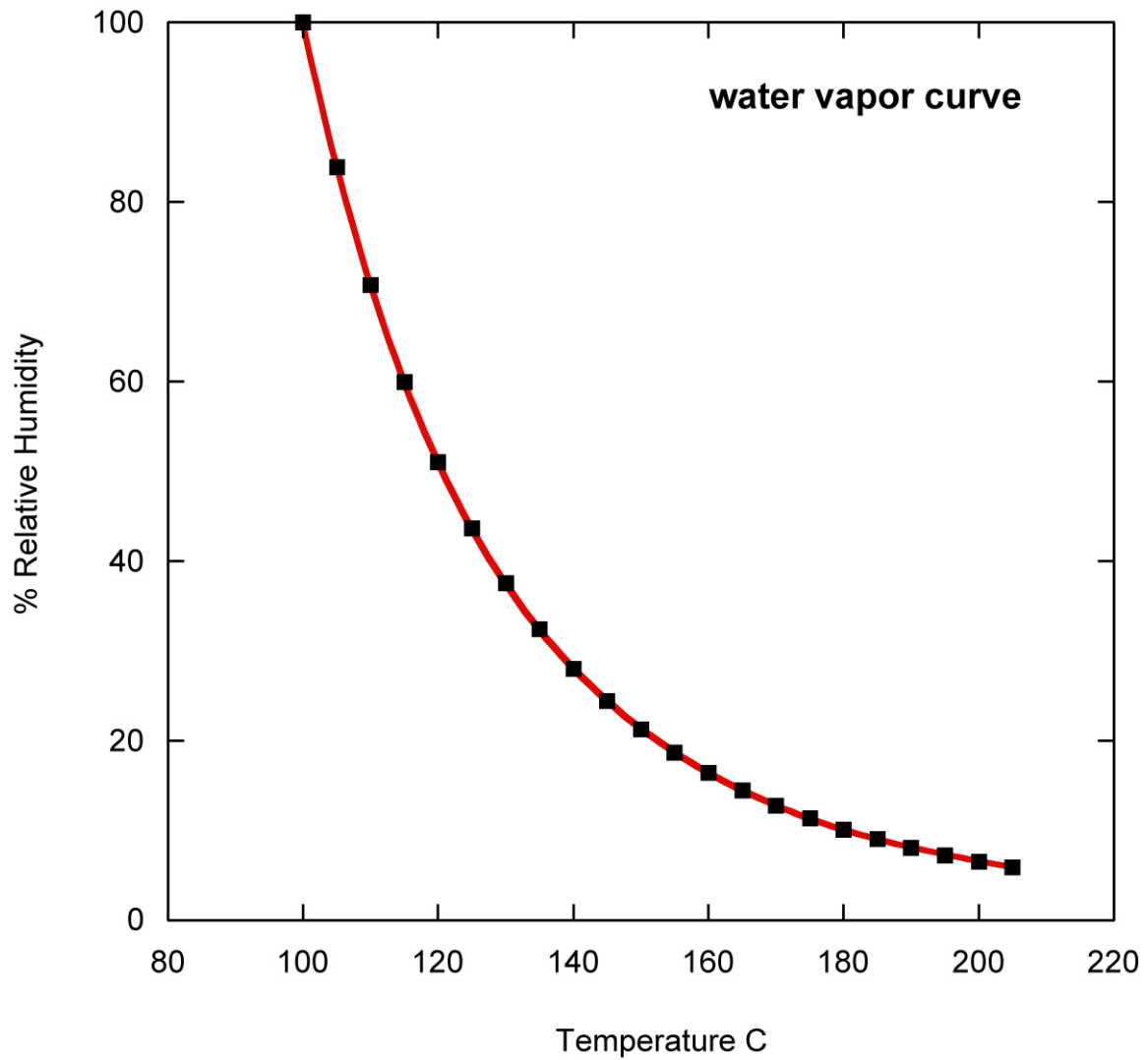
Figure 2.5. Temperature dependence of the vapor pressure of pure water. (Weast et al. 1987).
